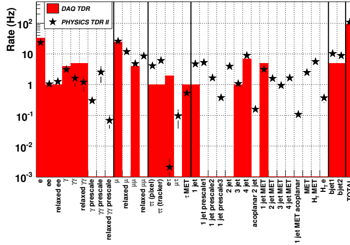
Figure 2.12.: The bandwidths for the different trigger paths. Source: [9]
