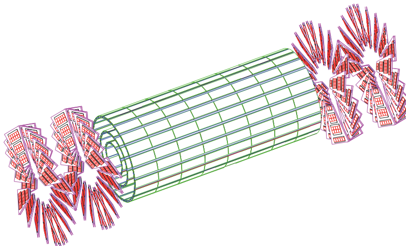
Figure 2.3.: Sketch of the CMS silicon pixel vertex detector. Though all three barrel layers are shown here, only two will be used simultaneously during the different phases of operation. [10]
