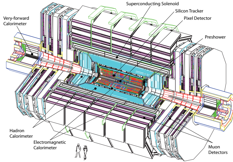
Figure 2.2.: Cut of the CMS detector with its different components. [9]
