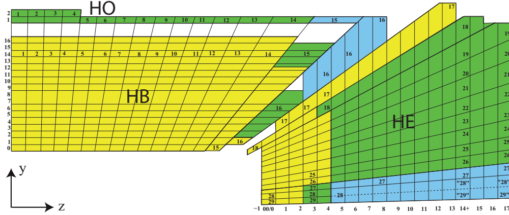
Figure 2.9.: Quarter view of the hadronic calorimeter in the r - z -plane. Shown are the hadron barrel (HB), the hadron outer (HO) and the hadron end cap (HE) calorimeter with their projective geometry.
