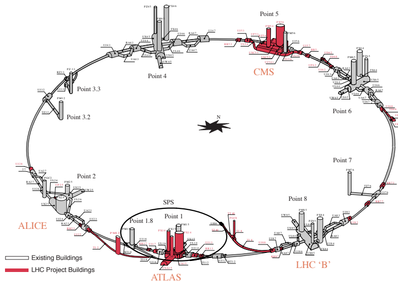
Figure 2.1.: The LHC ring with the old LEP (light grey) and the new LHC (red) facilities. On the four interaction points the six experiments are located. TOTEM and LHCf are not shown here and share their interaction point with CMS and ATLAS.
