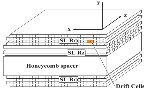
Figure 2.11.: Cross section of a CMS drift tube. It consists of three superlayers of each four layers. The outer superlayers are aligned along the beam line. The middle one is rotated by 90 degree to measure the z coordinate. Source: [9]
