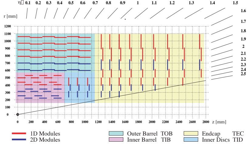
Figure 2.5.: A quarter view of the tracking detector. The different parts of the detector are indicated by colour. The lines represent the silicon modules, which are either single sided (red) or double sided (blue).
