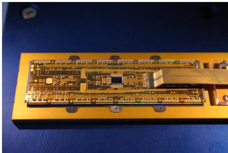
Figure 2.4.: Picture of a CMS Pixel Module. The pixels have a pitch of 100 \times 150 \mu\text{m}^2 . [9]
