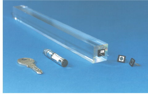
Figure 2.7.: Picture of a CMS Ecal crystal. The scintillation light is collected and amplified by avalanche photodiodes.
