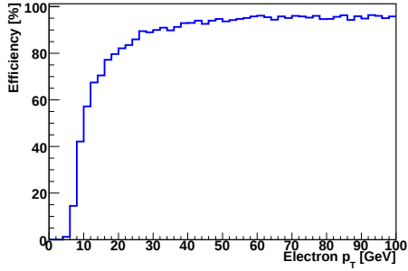
Figure 6.11.: Electron efficiency over electron p_T .
