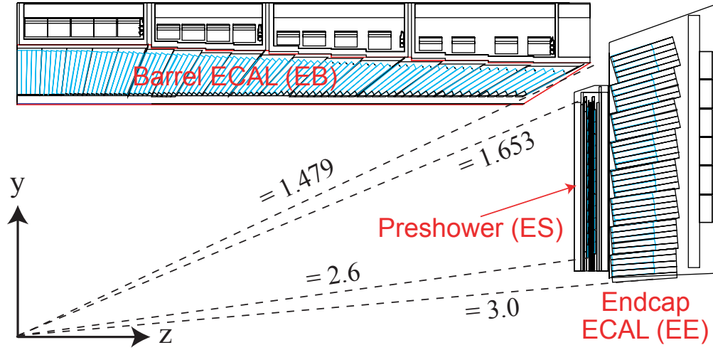
Figure 2.8.: An r-z-view of the CMS electromagnetic calorimeter. The ECal consists of three parts, the barrel, the preshower and the end cap. All crystals are mounted in quasi projective geometry.
