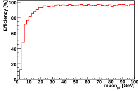
Figure 6.4.: Reconstruction efficiency of isolated muons as function of generated p_T .
