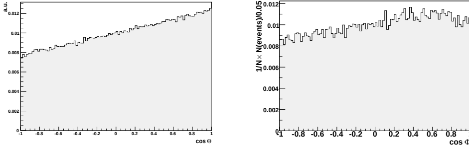
Figure 7.9.: Dilution of the opening angle distribution. On the left the initial generator information. On the right the result after selection and reconstruction.
