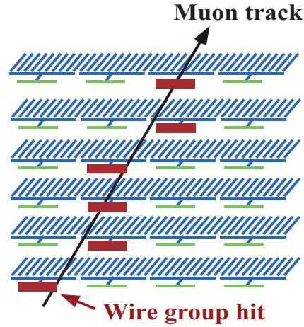
Figure 6.2.: Local reconstruction in the CSC. This \phi view shows the wires hit by a transversing muon. The hits are used to retrieve the R coordinates of the trajectory.
