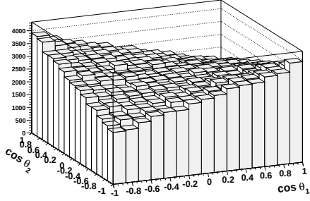
Figure 4.8.: Double differential distribution for the SM model case.
