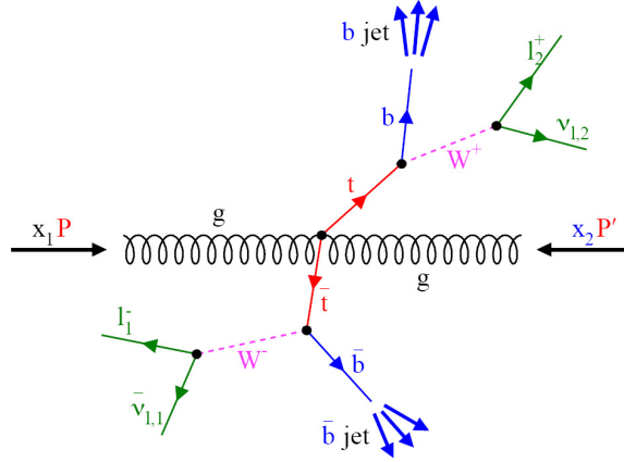
Figure 4.4.: The dileptonic decay of t\bar{t} -pairs is characterized by two b-quarks, two charged leptons and two neutrinos in the final state. In the detector the b-quarks will be visible as b-jets and together with the two charged leptons, this decay leaves a clear experimental signature.
