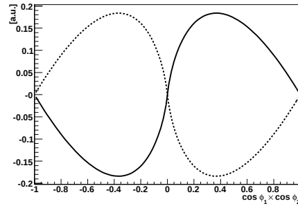
Figure 4.12.: Difference between distribution A = 0 and other scenarios for A = -1 (solid line) and A = 1 (dashed line).
