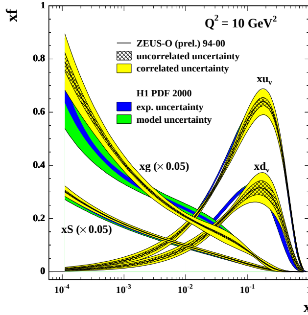
Figure 3.1.: Parton density functions. Here a comparison of ZEUS and H1. Shown are the density of u and d valence quarks, gluons and sea quarks. [26]
