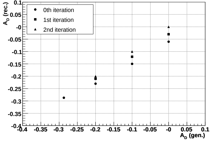
Figure 7.16.: Unfolding of observable A_D . Starting assumption for the unfolding procedure is the SM prediction A_D = -0.287 .
