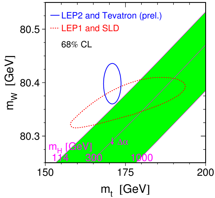
Figure 4.1.: Limit to the Higgs mass from radiative corrections. The contours are the experimental mass limits obtained from direct and indirect measurements from SLD, LEP and Tevatron. The band indicates the higgs masses which are compatible with the SM. [30]
