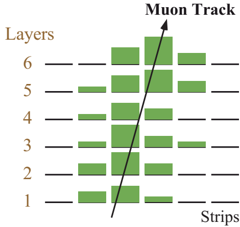
Figure 6.1.: Local reconstruction in the CSC. This R view shows the charge deposition of a transversing muon in the cathode strips. This information is used to reconstruct the \phi coordinates of the trajectory.
