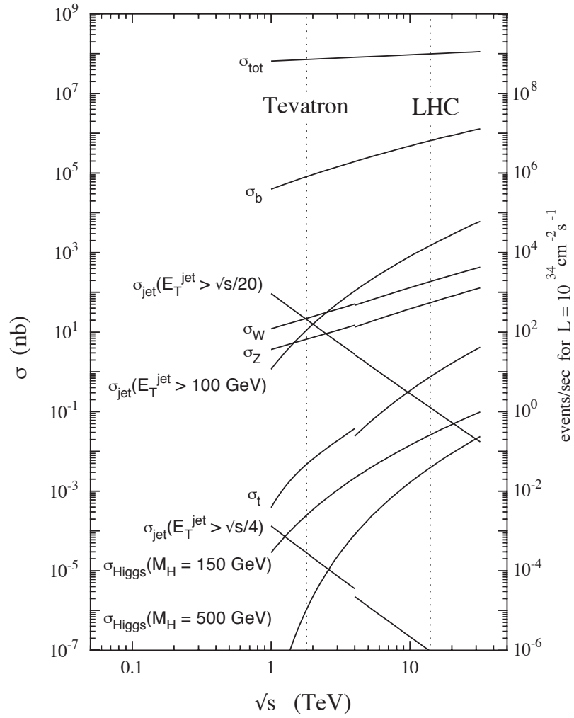
Figure 3.2.: Cross sections and event rates for some characteristic standard model processes as function of the center of mass energy. Two lines indicate the proton–antiproton collider Tevatron and the proton–proton collider LHC. Source: [29]
