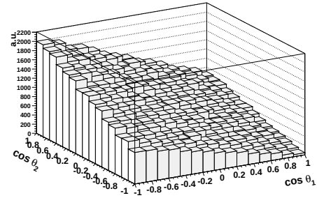
Figure 5.4.: Double differential distribution for the \downarrow\uparrow helicity state.
