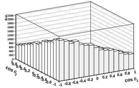
Figure 5.2.: Double differential distribution for the \downarrow\downarrow helicity state.
