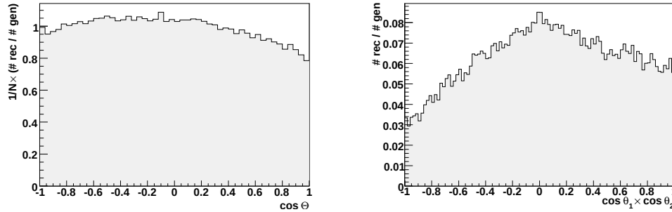
Figure 7.10.: On the left the efficiency for A_D , on the right the efficiency for A comparing the information before and after selection.
