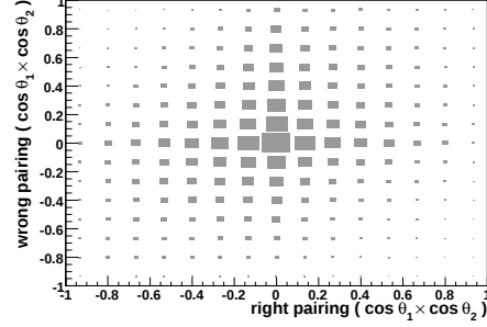
Figure 7.14.: Migration due to wrong pairing
