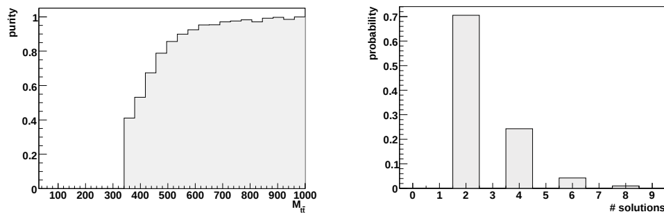
Figure 7.3.: Left: the probability to get a solution for the wrong pairing decreases with higher energies. Right: total number of solutions taking both pairings into account.
