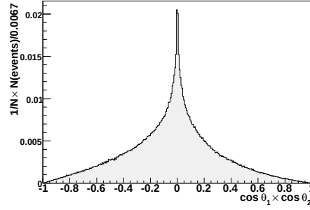
Figure 4.10.: The double differential distribution as projection to \cos \theta_1 \cdot \cos \theta_2 in the SM case.
