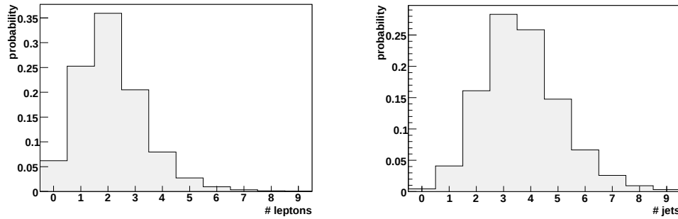
Figure 7.2.: Number of leptons (left) and jets (right) after reconstruction. The proper leptons and jets have to be selected.
