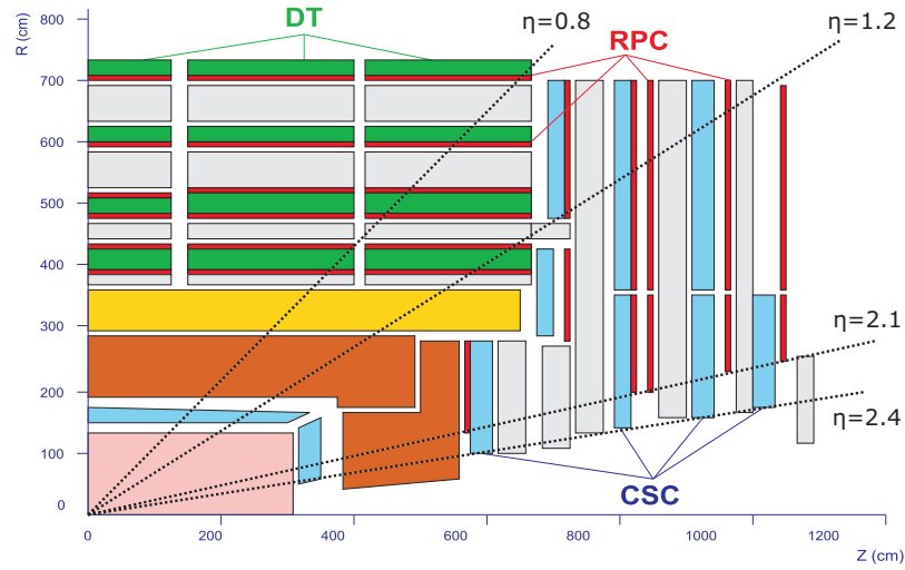
Figure 2.10.: CMS muon system cross section. Three different detector types are used. Drift tubes (DT), Cathode Strip Chambers (CSC) and Resistive Plate Chambers (RPC).
