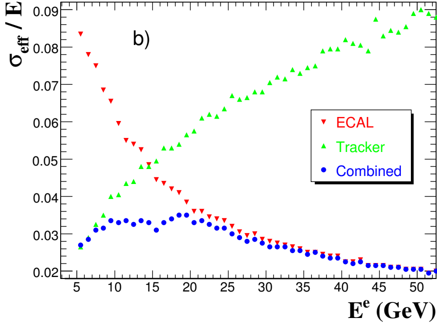
Figure 6.10.: The electron energy resolution using ECal energy deposits (red), tracker information (green) and the combination of both (blue). In this study the electron resolution is mainly dominated by the Ecal resolution. [9]
