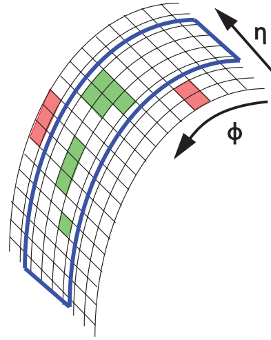
Figure 6.9.: The energy depositions corresponding to one electron (green) can be separated in \phi due to several effects. The super cluster algorithm is used to combine the energy of several clusters into a supercluster, here indicated by the blue line. [78]
