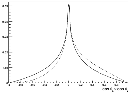
Figure 4.11.: Theoretical distribution for A = 0 (solid line) or A = +1 spin correlation (dashed line).
