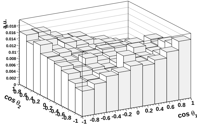
Figure 7.18.: Spin–spin-correlation distribution after application of Bayesian unfolding.
