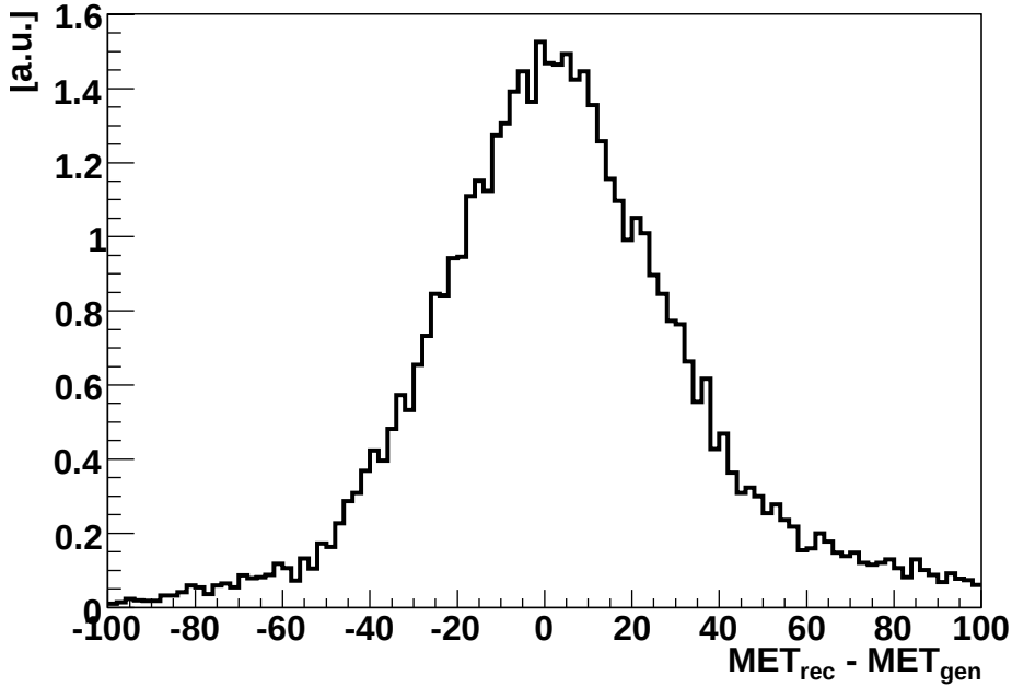
Figure 6.18.: Resolution of the MET reconstruction.
