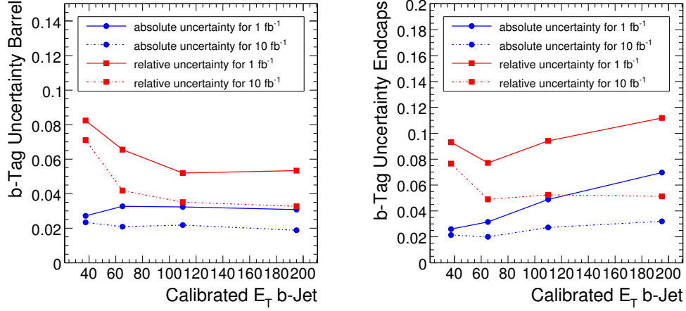
Figure 7.21.: Estimates for the b-tagging uncertainty at different luminosities for barrel (left) and endcap (right). [9]
