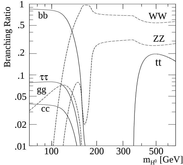
Figure 3.3.: Branching ratios for different decay modes of the SM higgs. According to these ratios there exist different search strategies for different mass regions.
