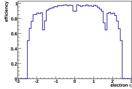
Figure 6.12.: Electron efficiency over electron \eta . The dips are due to the border between barrel and endcap.
