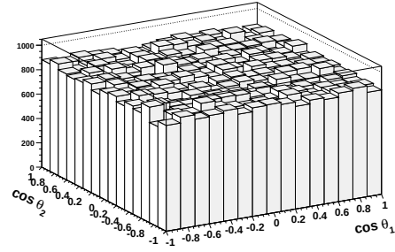
Figure 4.9.: The double differential distribution for the case of no spin-spin-correlation.
