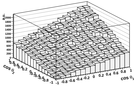
Figure 5.1.: Double differential distribution for the \uparrow\uparrow helicity state.
