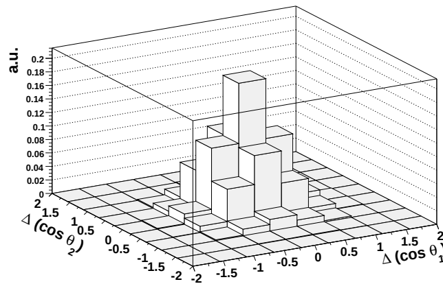
Figure 7.12.: Migration of the helicity angles \cos \theta . Plotted are the differences between generated and reconstructed value.
