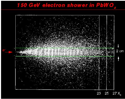
Figure 2.6.: Simulation of a shower caused by an 150 GeV electron stopped in \text{PbWO}_4 . The green lines indicate the size of the crystals used in CMS. Source: Based on [17]
