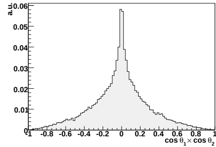
Figure 7.8.: Dilution of the spin asymmetry observable \cos \theta_1 \times \cos \theta_2 . On the left the initial generator information. On the right the result after selection and reconstruction.
