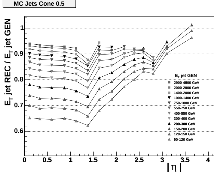
Figure 6.14.: Comparison of transverse jet energy E_T from MC and calorimeter clustering. [9]
