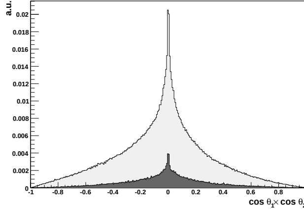
Figure 7.19.: Signal (grey) and background contribution (black) for the measurement of A . The background has the shape of an uncorrelated sample.
