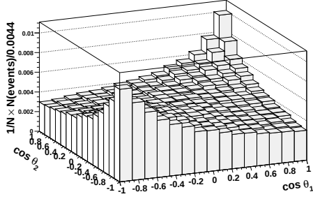
Figure 7.13.: Double differential distribution with wrong pairing
