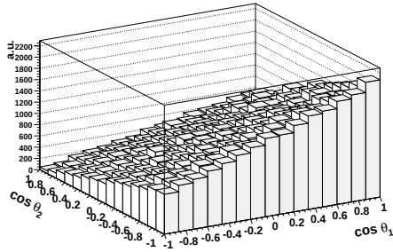
Figure 5.3.: Double differential distribution for the \uparrow\downarrow helicity state.
