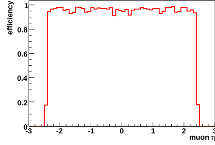
Figure 6.5.: Reconstruction efficiency of isolated muons as function of the generated \eta .
