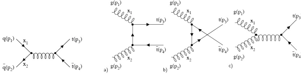
Figure 4.2.: Feynman diagrams of the production processes of t\bar{t} -pairs at a proton-proton-collider.
