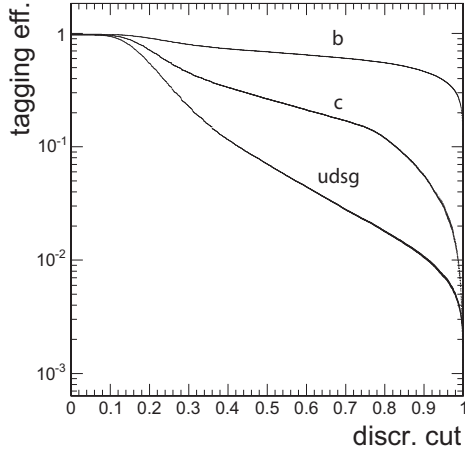
Figure 6.16.: The efficiency of the b tagging algorithm for different flavours and discriminator cuts. It was created using QCD events with 30 \text{ GeV} < p_T < 200 \text{ GeV} and |\eta| < 2.4 . [87]
