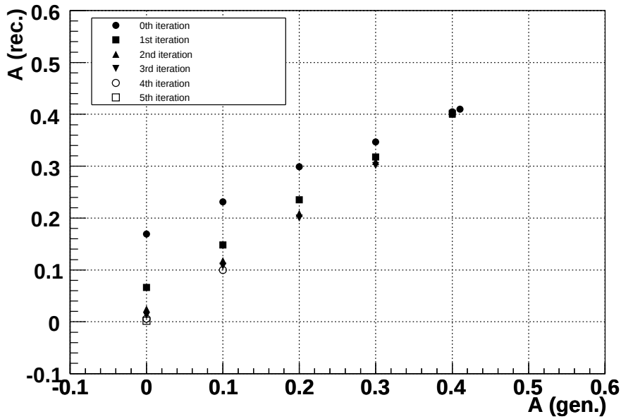
Figure 7.15.: Unfolding of observable A with different start values. During the iteration steps the computed value gets closer to the input value.
