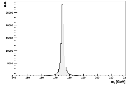
Figure 7.6.: The generator mass of the top quarks.
