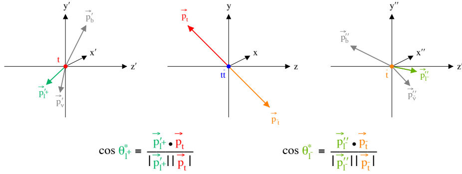
Figure 4.7.: Explanation of the helicity basis. The helicity angle of a lepton is calculated by the angle between the lepton momentum in the rest frame of the corresponding top and the top momentum in the t\bar{t} rest frame. [52]
