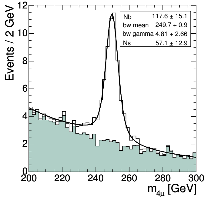
Figure 3.4.: Simulated higgs signal in the four muon channel. It can be seen as peak above the continuous background. This channel is one of the performance channels for the CMS detector design. [33]
