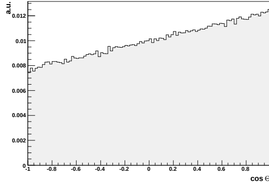
Figure 4.6.: One dimensional distribution of the lepton opening angle for the SM case. It is used to measure the observable \mathcal{O}_1 . In this case the parameter is -0.290 .
