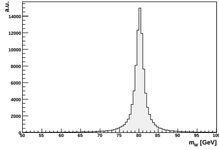
Figure 7.5.: The generator mass of the W bosons.
