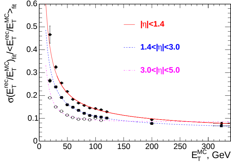
Figure 6.15.: The transverse jet energy resolution for iterative cone R = 0.5 jets after Monte-Carlo calibration. [9]
