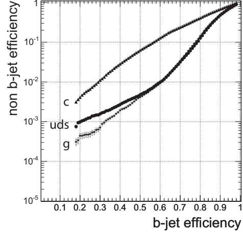
Figure 6.17.: Comparison of bjet mistagging and b jet tagging efficiency for different jet flavours. The data was retrieved using semileptonic t\bar{t} events. [87]
