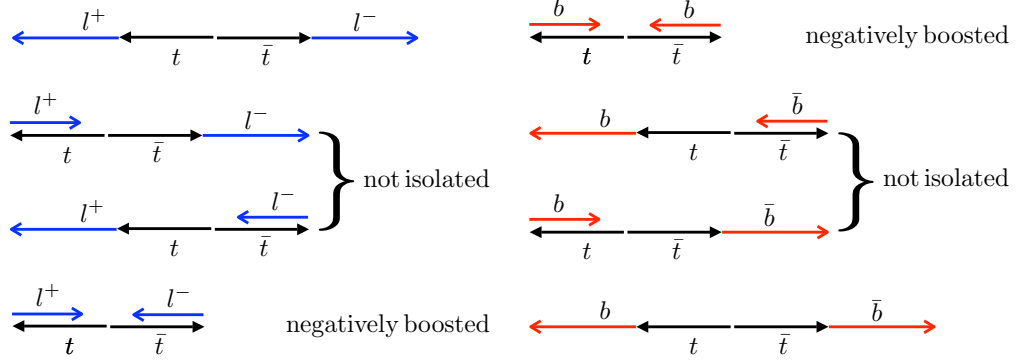
Figure 7.11.: A simplified view of the kinematics for the four border cases of the double differential distribution. A superposition of all these effects leads to the shape of the acceptance function.
