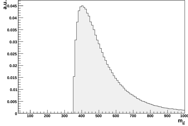
Figure 4.13.: Distribution of m_{t\bar{t}} . An upper cut of 550 GeV is chosen to improve the spin-correlation.
