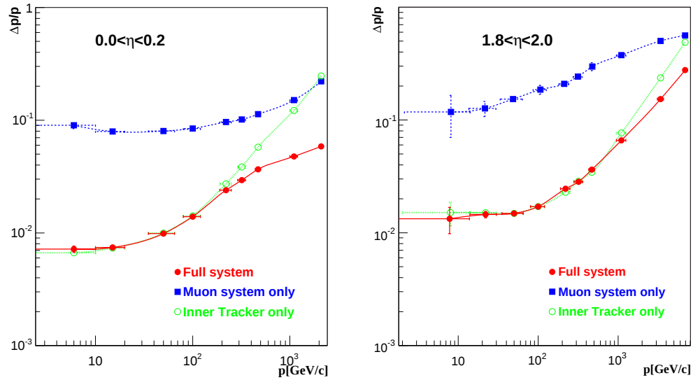
Figure 6.3.: Resolution of muon reconstruction from muon system only, tracker only, and both combined. [9]
