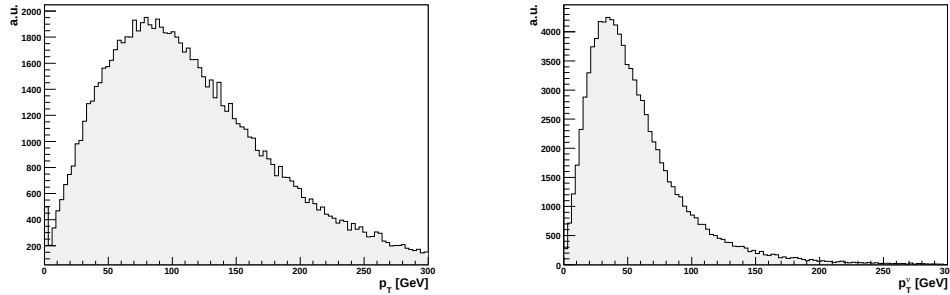
Figure 7.4.: The p_T spectra used for weighting the kinematical hypotheses. On the left the p_T spectrum of the top quarks. It is almost independent from the production process and thus not biasing; on the right the neutrino spectrum. Both are combined into a probability for weighting the multiple event hypotheses.
