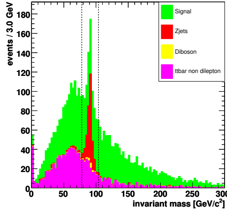
Figure 7.1.: The invariant mass of both leptons could be used to suppress the Z background. While this cut was used successfully in other studies, the cut is rejected for the study of spin correlations. [33]
