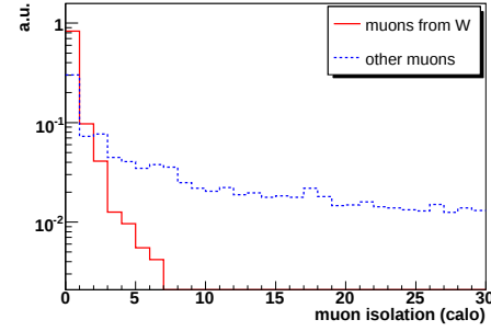
Figure 6.6.: Muon isolation criteria to distinguish muons from W (red) and muons from other sources (blue). Both isolation criteria are explained in the text.
