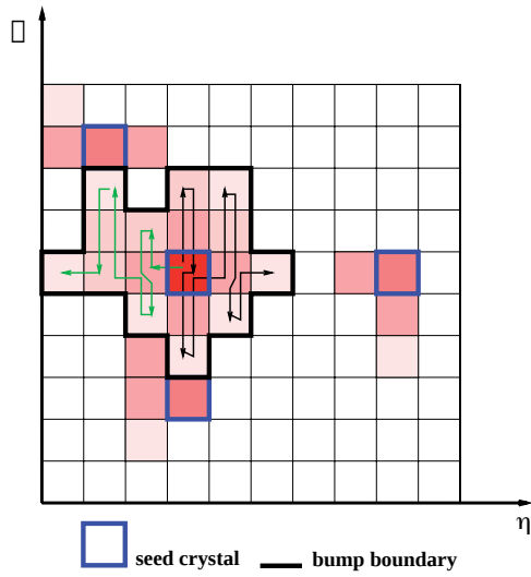
Figure 6.8.: The calorimeter cells have different energy deposits as indicated by brightness. The blue bordered cells have an energy exceeding the seed threshold. The black line indicates one cluster reconstructed by the island algorithm. The arrows are included to show the evolution of the algorithm. [78]
