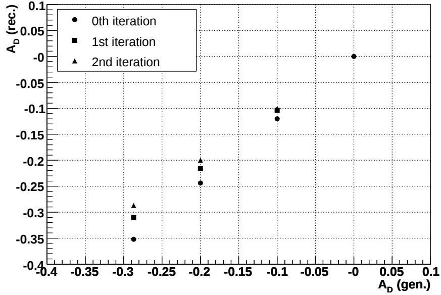
Figure 7.17.: Unfolding of observable A_D . Starting assumption is a parameter of A_D = 0.0 .
