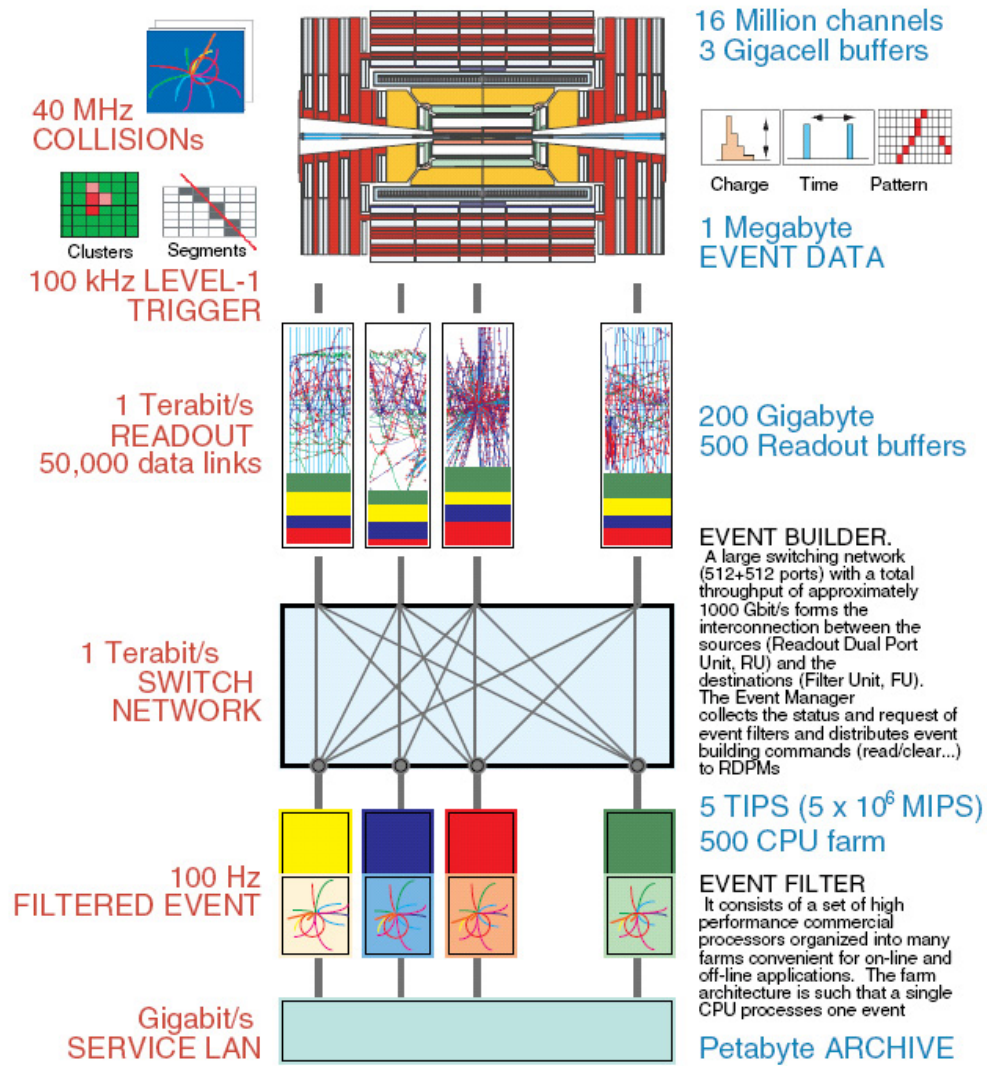
Figure 2.13.: A schematic view of the trigger system.
