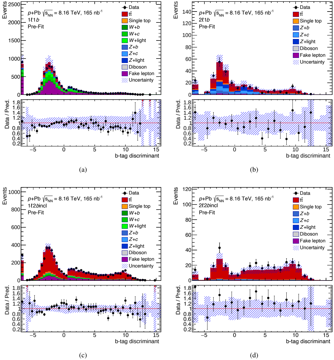
Figure 4.7: Pre-fit distributions of the b -tag discriminant in the four signal regions: (a) 1\ell 1b , (b) 2\ell 1b , (c) 1\ell 2\text{bincl} , and (d) 2\ell 2\text{bincl} . Pre-fit uncertainties are represented by the hatched area. The full markers in the bottom panels show a ratio of data and a sum of predictions. Arrows indicate bins with entries that are outside the ratio range. The first and last bins include underflow and overflow events, respectively.
