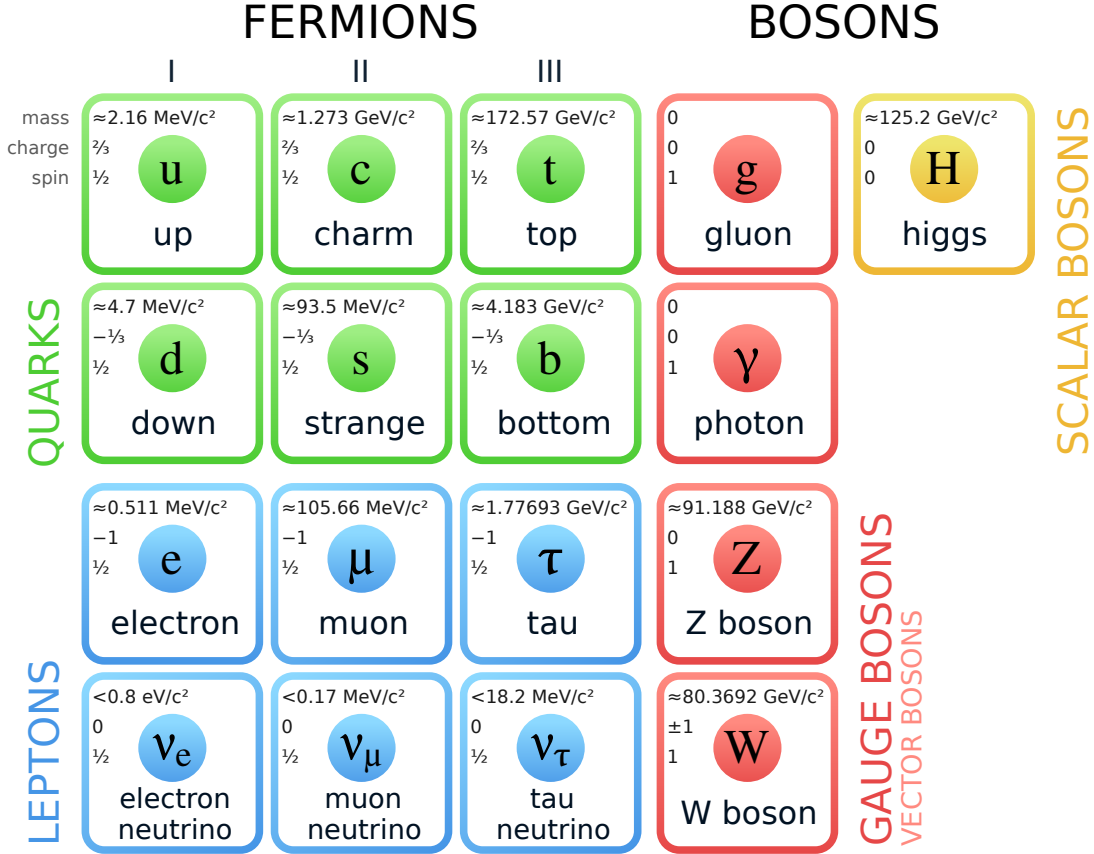
Figure 1.1: Scheme of the Standard Model [20].
