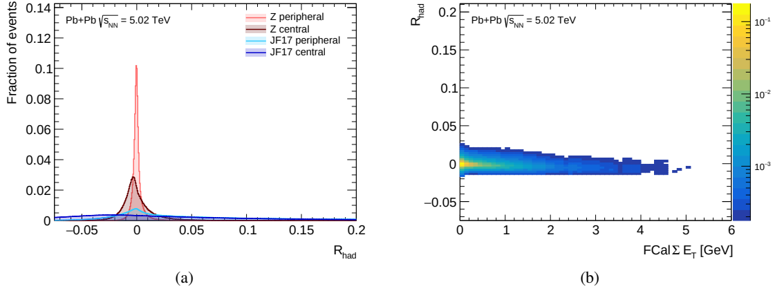
Figure A.18: Distribution of the R_{\text{had}} electron discriminating variable (a) for signal and background electrons in central and peripheral Pb+Pb collisions, and (b) for signal electrons as a function of centrality.
