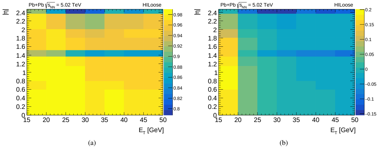
Figure A.39: (a) The measured identification efficiency and (b) the relative difference between optimised and measured efficiencies as a function of electron E_T and |\eta| for the HILoose working point.
