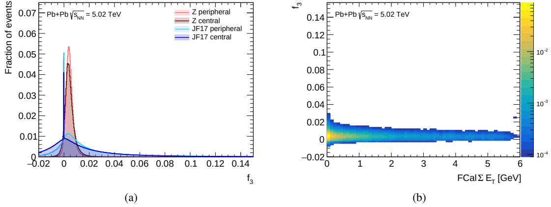
Figure A.15: Distribution of the f_3 electron discriminating variable (a) for signal and background electrons in central and peripheral Pb+Pb collisions, and (b) for signal electrons as a function of centrality.
