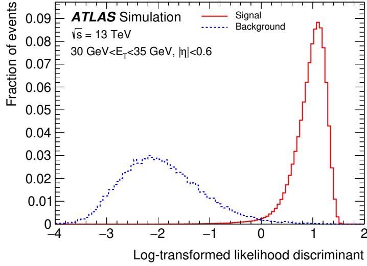
Figure 3.5: Distributions of log-transformed discriminants d'_L for reconstructed electron candidates. The red and blue histograms represent signal Z \rightarrow e^+e^- and background simulation samples, respectively [130].
