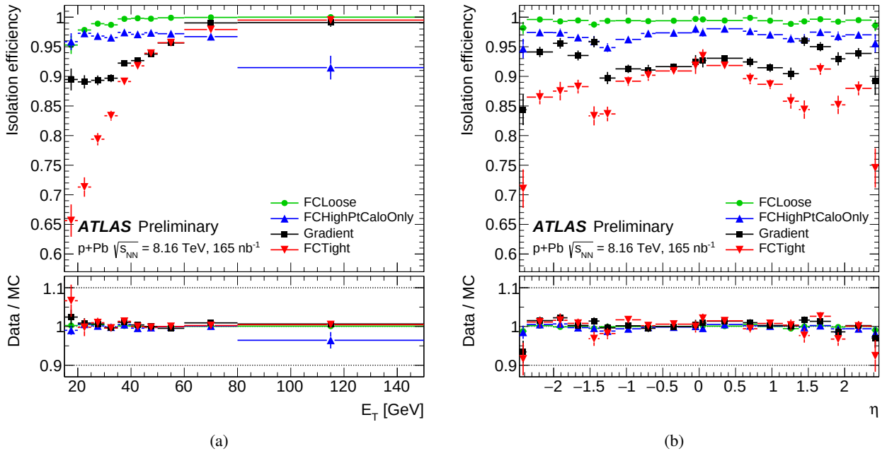
Figure 3.9: The electron isolation efficiency in Z \rightarrow e^+e^- events as a function of electron (a) E_T and (b) \eta evaluated in 2016 p +Pb data for the FCLoose, HighPtCaloOnly, Gradient, and FCTight working points. The bottom panels show the data-to-simulation ratios. Error bars represent the total uncertainties composed of statistical and systematic components added in quadrature [128].
