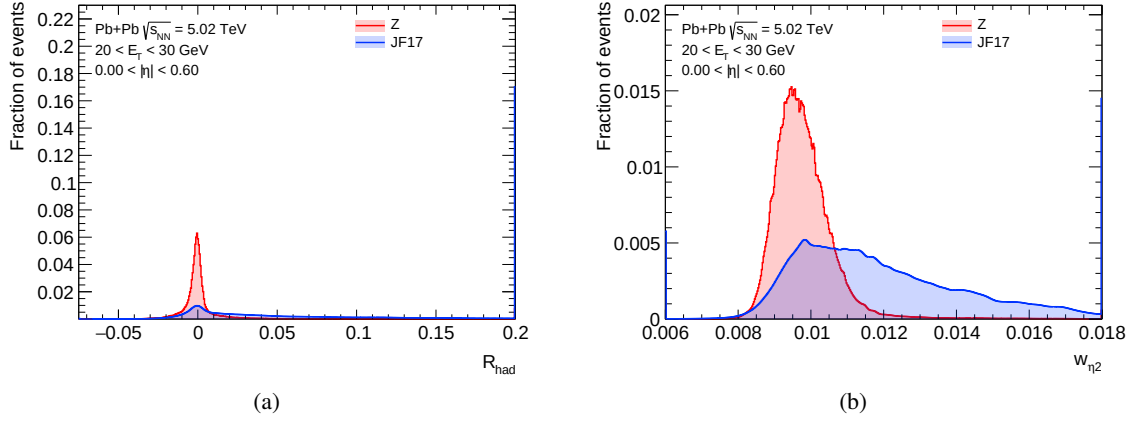
Figure A.29: Probability distribution functions of the (a) R_{had} and (b) w_{\eta 2} electron discriminating variables for signal and background electrons.
