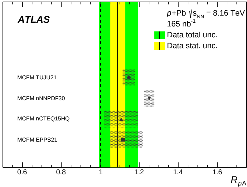
Figure 4.20: Comparison between measured and predicted values of R_{pA} . The measurement, represented by the solid black line, is compared with theoretical predictions based on four nPDF sets, calculated at NNLO precision in QCD and scaled to the p +Pb system [39].
