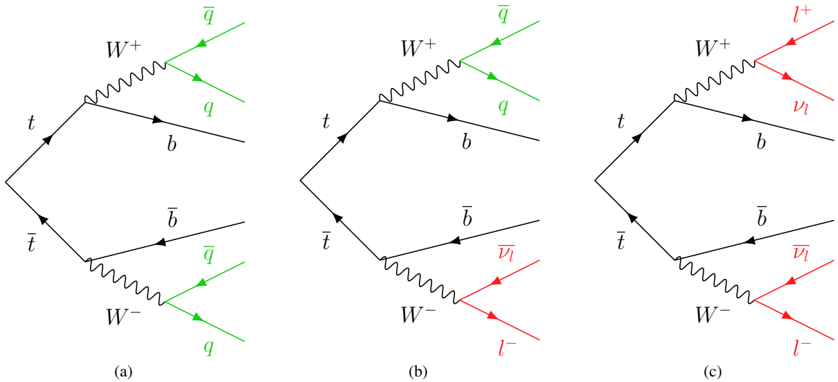
Figure 1.12: Feynman diagrams for top-quark pair decay channels: (a) all-hadronic, (b) \ell +jets, and (c) dilepton.
