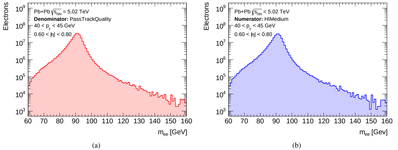
Figure 3.22: Invariant-mass distributions of electron pairs in signal Z \rightarrow e^+e^- MC simulation in the (a) denominator and (b) numerator of the identification efficiency for the HIMedium working point in an exemplary electron E_T and |\eta| bin.
