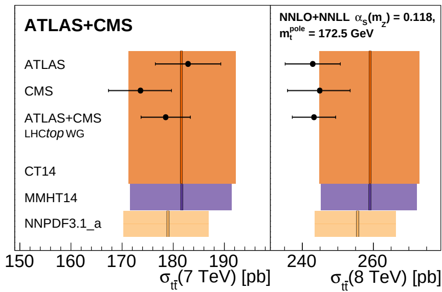
Figure 1.15: Measured t\bar{t} production cross sections in pp collisions at \sqrt{s} = 7 and 8 TeV [72], compared with the theoretical predictions using different PDF sets.
