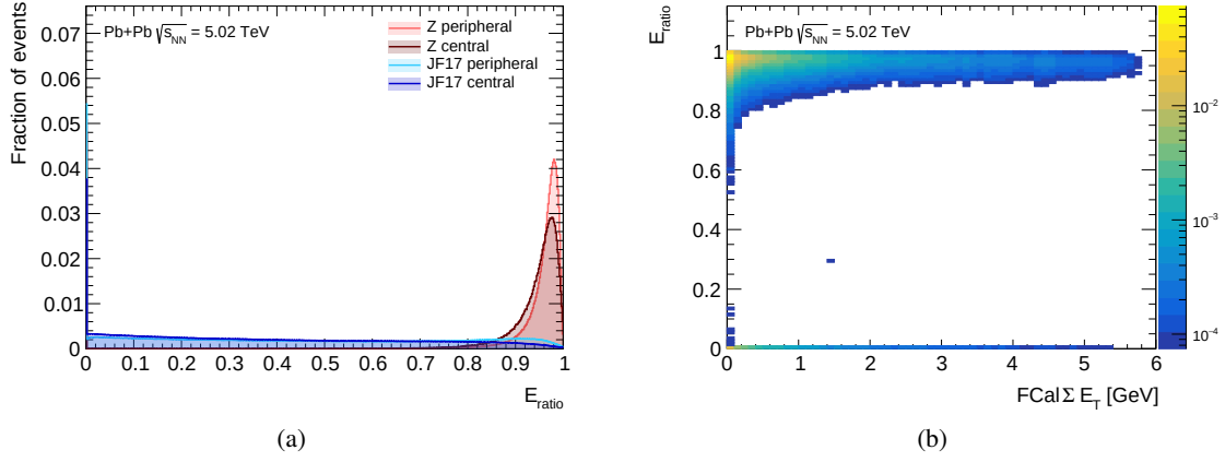
Figure A.20: Distribution of the E_{\text{ratio}} electron discriminating variable (a) for signal and background electrons in central and peripheral Pb+Pb collisions, and (b) for signal electrons as a function of centrality.
