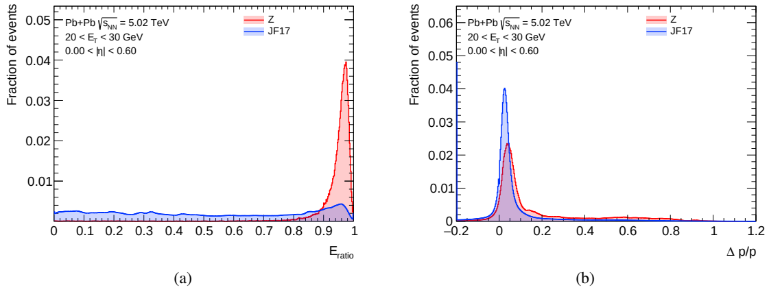
Figure A.30: Probability distribution functions of the (a) E_{ratio} and (b) \Delta p/p electron discriminating variables for signal and background electrons.
