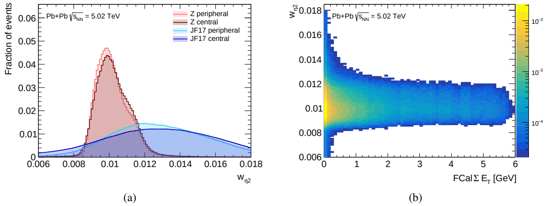
Figure A.19: Distribution of the w_{\eta 2} electron discriminating variable (a) for signal and background electrons in central and peripheral Pb+Pb collisions, and (b) for signal electrons as a function of centrality.
