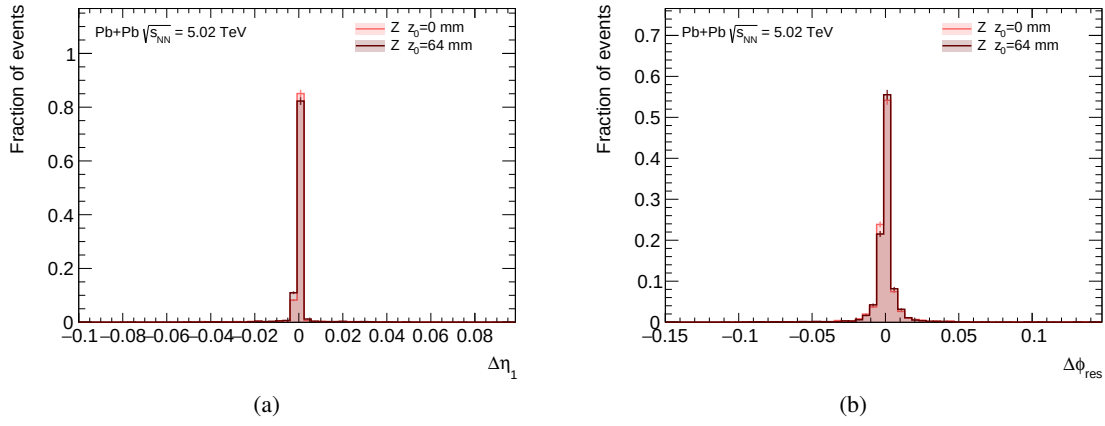
Figure A.12: Distributions of the (a) \Delta\eta_1 and (b) \Delta\phi_{res} electron discriminating variables for two fixed z_0 vertex positions. Error bars denote statistical uncertainties.
