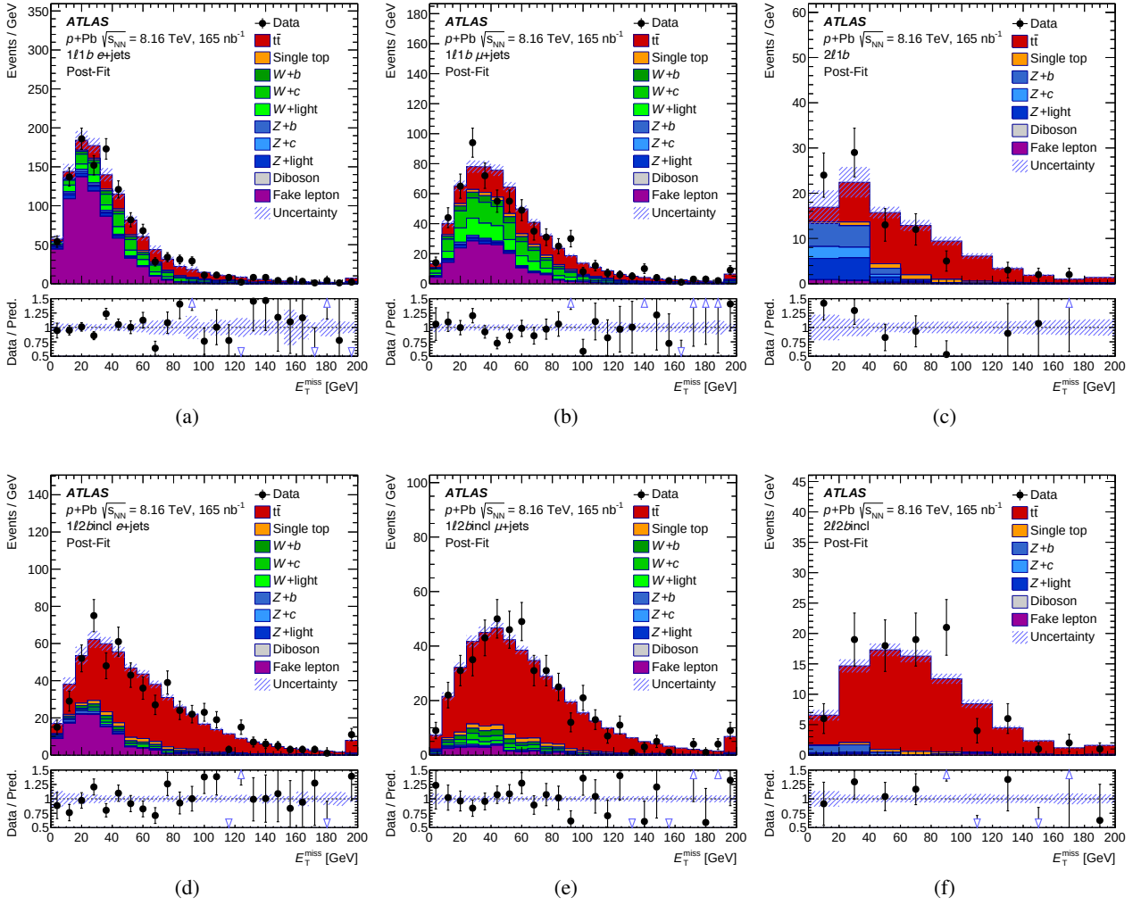
Figure 4.8: Post-fit E_T^{\text{miss}} distributions in the six signal regions ( e +jets: (a) 1\ell 1b and (d) 1\ell 2\text{bincl} , \mu +jets: (b) 1\ell 1b and (e) 1\ell 2\text{bincl} , dilepton: (c) 2\ell 1b and (f) 2\ell 2\text{bincl} ). Post-fit uncertainties are represented by the hatched area. The full markers in the bottom panels show a ratio of data and a sum of predictions. Open triangles indicate bins with entries that are outside the ratio range. The last bin includes overflow events [39].
