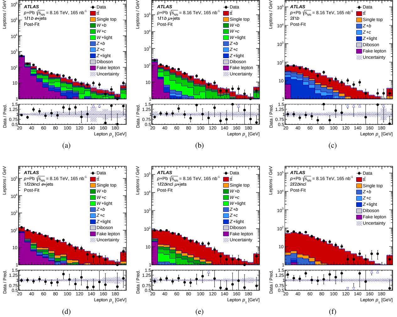
Figure 4.2: Post-fit lepton p_T distributions in the six signal regions ( e +jets: (a) 1\ell 1b and (d) 1\ell 2bincl , \mu +jets: (b) 1\ell 1b and (e) 1\ell 2bincl , dilepton: (c) 2\ell 1b and (f) 2\ell 2bincl ). Post-fit uncertainties are represented by the hatched area. The full markers in the bottom panels show a ratio of data and a sum of predictions. Open triangles indicate bins with entries that are outside the ratio range. The last bin includes overflow events [39].
