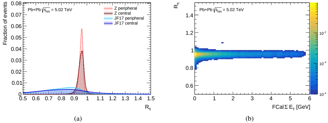
Figure A.16: Distribution of the R_\eta electron discriminating variable (a) for signal and background electrons in central and peripheral Pb+Pb collisions, and (b) for signal electrons as a function of centrality.
