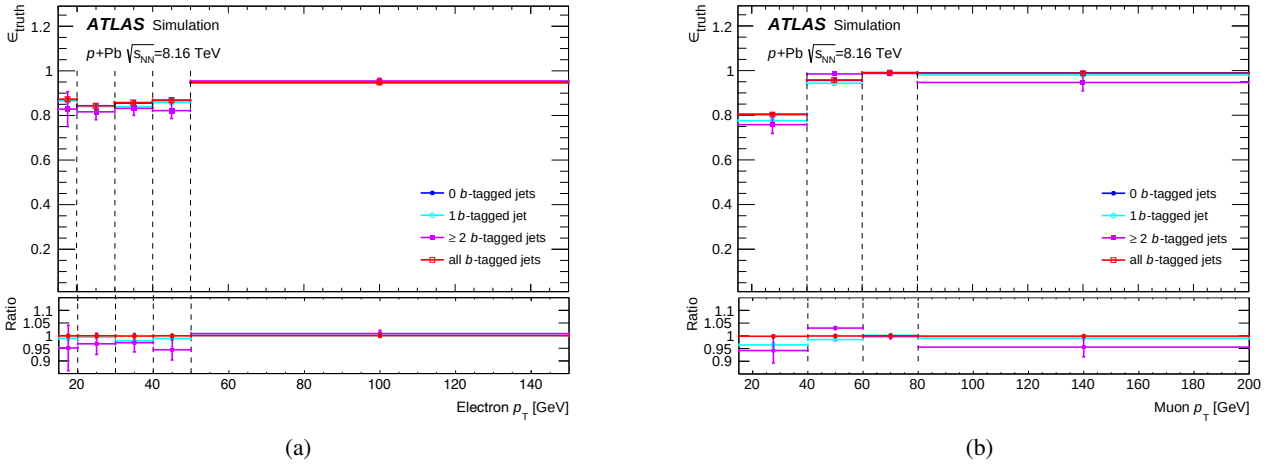
Figure 4.9: The real-lepton efficiency for (a) electrons and (b) muons as a function of lepton p_T for a varying number of b -tagged jets in the event. The bottom panels show a ratio of events for different b -tagged jet multiplicities to the number of events with zero b -tagged jets [39].
