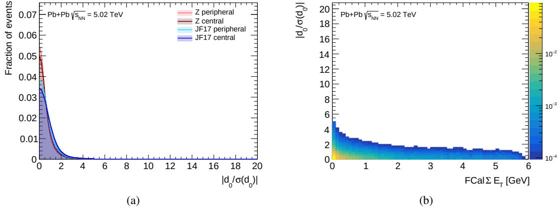
Figure A.23: Distribution of the |d_0/\sigma(d_0)| electron discriminating variable (a) for signal and background electrons in central and peripheral Pb+Pb collisions, and (b) for signal electrons as a function of centrality.
