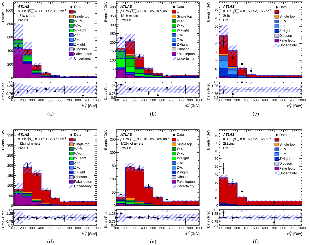
Figure 4.11: Comparison of data and total pre-fit prediction for the H_T^{\ell,j} distribution in each of the six signal regions ( e +jets: (a) 1l1b and (d) 1l2bincl, \mu +jets: (b) 1l1b and (e) 1l2bincl, dilepton: (c) 2l1b and (f) 2l2bincl), with uncertainties represented by the hatched area. The full markers in the bottom panels show a ratio of data and a sum of predictions. Arrows indicate bins with entries that are outside the ratio range [39].
