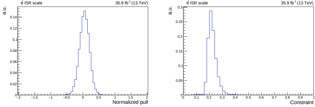
Figure D.3: Distributions of the pulls (left) and constraints (right) on the t\bar{t} ISR scale uncertainty obtained using toy templates.
