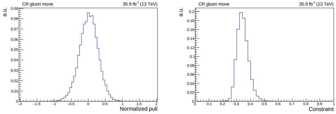
Figure D.6: Distributions of the pulls (left) and constraints (right) on the gluon move CR model obtained using toy templates.
