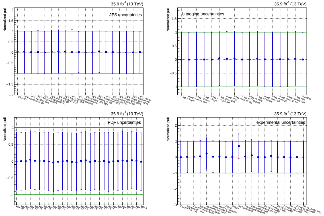
Figure C.1: Pulls and constraints on the nuisance parameters in the cross-check fit of m_t^{\text{MC}} . The plots refer to the JES (upper left), b tagging (upper right), PDF (lower left), and other experimental uncertainties (lower right).
