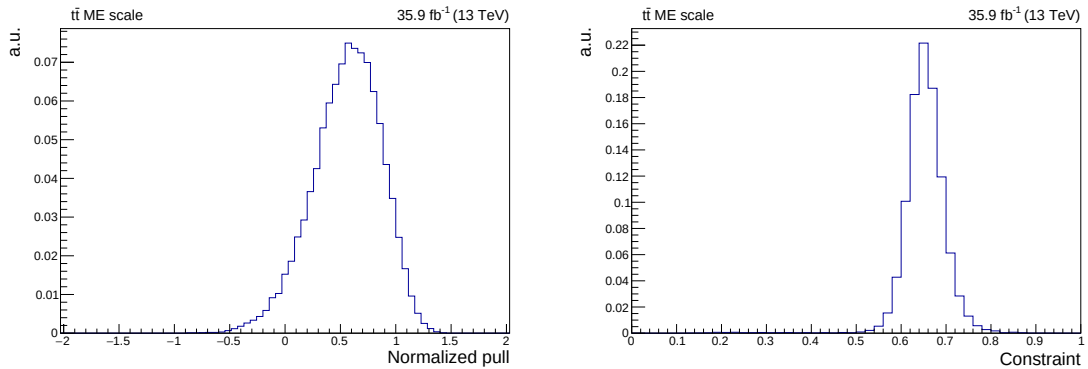
Figure D.1: Distributions of the pulls (left) and constraints (right) on the t\bar{t} ME scale uncertainty obtained using toy templates.
