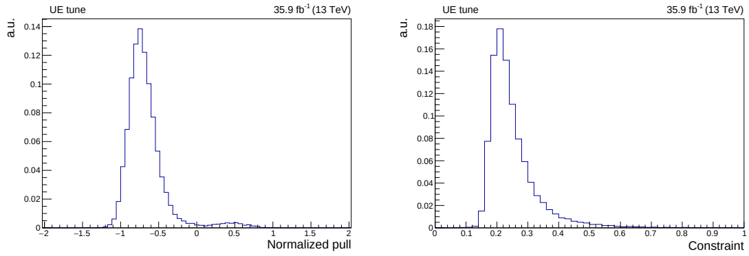
Figure D.12: Distributions of the pulls (left) and constraints (right) on the UE tune uncertainty obtained using toy templates.
