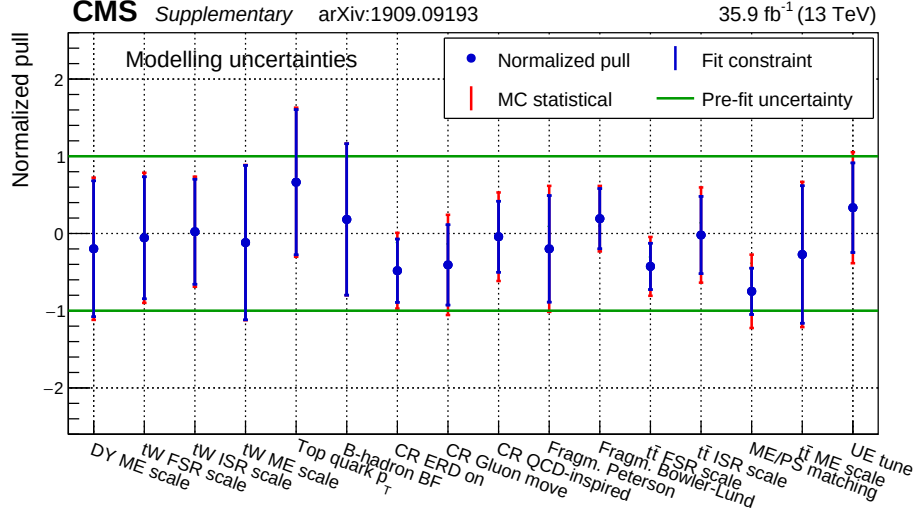
Figure 6.4: Normalized pulls and constraints of the nuisance parameters related to the modelling uncertainties. The pulls, defined as the difference between the post-fit and pre-fit values of a nuisance parameter in units of the corresponding pre-fit uncertainty, are represented by the points, while the constraints, defined as the ratio between the post-fit and pre-fit uncertainties on a nuisance parameter, correspond to the inner vertical bars. The horizontal lines represent the pre-fit uncertainty, and the outer vertical bands indicate the additional uncertainty due to the limited statistics in the simulation, as determined using pseudo-experiments [23].
