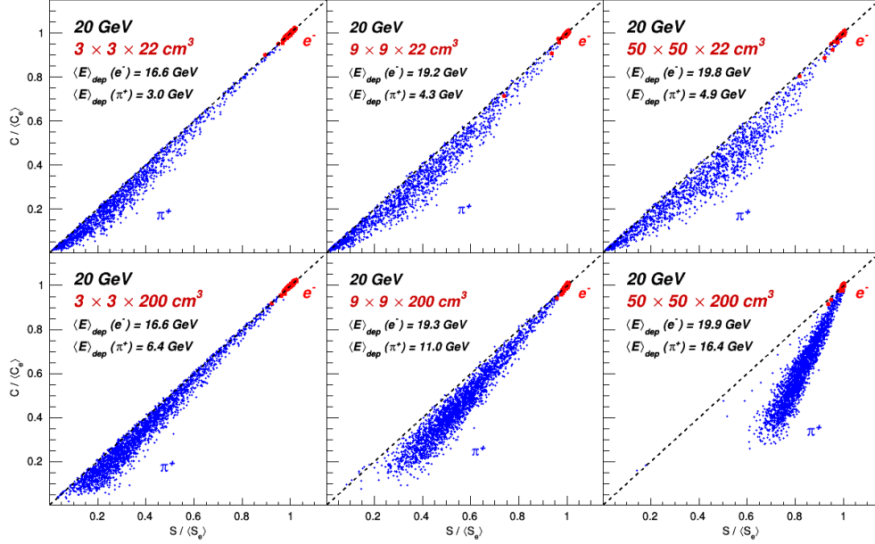
Figure 9.1: Scatter plots of the normalized number of Cherenkov and scintillation photons produced by 20 GeV electrons (red) and pions-induced showers (blue) for different PbWO 4 crystal sizes. The bisector C = S was drawn as a dotted black line to better understand the applicability of the DREAM collaboration method to evaluate the f_{\text{em}} information.
