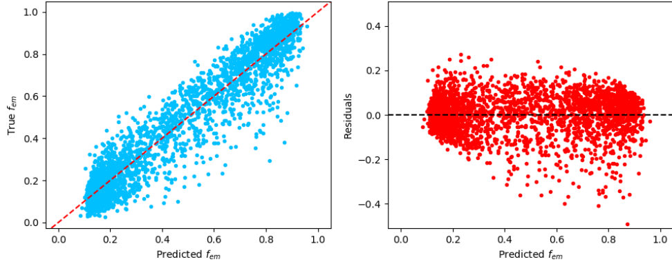
Figure 9.5: Left: true f_{\text{em}} value given in input to the machine learning program against the value predicted. Right: scatter plot of the residuals (true f_{\text{em}} - predicted f_{\text{em}} ) versus the value of f_{\text{em}} predicted by the algorithm.
