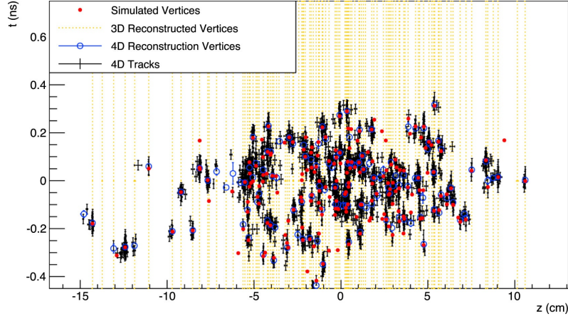
Figure 1.12: Simulated and reconstructed vertices in a bunch crossing with 200 pileup interactions, considering a MIP timing detector with approximately 30 ps time resolution covering the barrel and endcaps. The red dots represent the simulated vertices, while the vertical yellow lines indicate 3D-reconstructed vertices (without using timing information). Instances of vertex merging are visible throughout the display in the 3D-reconstructed vertices. The black crosses and blue open circles represent tracks and vertices reconstructed using a method that incorporates the time information, referred to as “4D”. With the use of time information, many of the vertices that appeared merged in the spatial dimension are now clearly separated. From reference [23].
