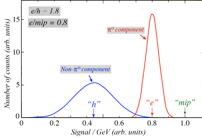
Figure 1.8: Distributions of the signal per unit deposited energy for both the electromagnetic and non-electromagnetic components of the hadron showers, normalized to the response for minimum ionizing particles (“mip”). The average values of the electromagnetic and non-electromagnetic distributions represent the electromagnetic response (“e”) and the non-electromagnetic response (“h”) of the calorimeter. From reference [15].
