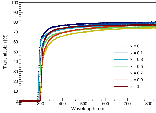
Figure 4.2: Trasmission spectra measured for the plate-shaped samples with variable Ge fraction x along their thinnest dimension. Adapted from reference [60].
