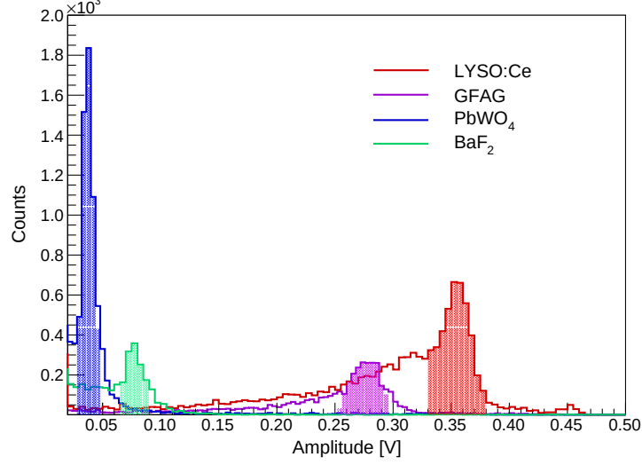
Figure 8.6: Energy signal amplitude distributions for LYSO:Ce, GFAG, PbWO 4 , and BaF 2 samples. The highlighted regions contain the events where the incoming pion deposited some of its energy along the entire sample length..
