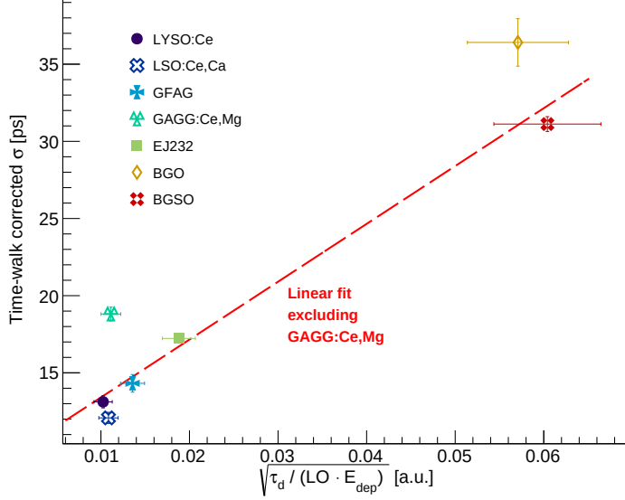
Figure 8.11: Time-walk corrected \sigma values of the samples exhibiting a large scintillation light yield against the quantity \sqrt{\tau_d / (LO \cdot E_{dep})} which is proportional to the expected time resolution. The red line fits the data points excluding the one corresponding to GAGG:Ce,Mg.
