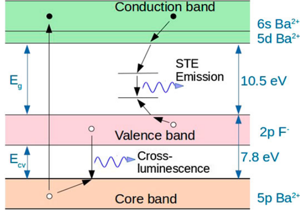
Figure 2.2: Illustrative representation of the band-gap diagram for BaF 2 along with corresponding emission mechanisms. From reference [34]
