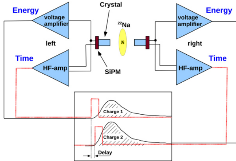
Figure 3.7: Schematic of the CTR setup measuring samples at 511 keV. From reference [46].
