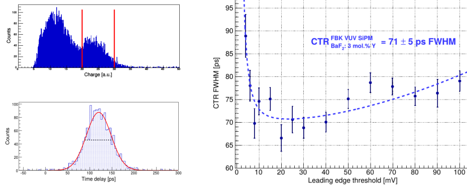
Figure 5.6: Left: charge and time delay distributions for a 2 \times 2 \times 3 \text{ mm}^3 3 mol.% Y-doped sample read out by an FBK SiPM, setting a 20 mV threshold on its time signal. Right: CTR FWHM plotted against the leading edge threshold set on the time signal for a 2 \times 2 \times 3 \text{ mm}^3 3 mol.% Y-doped \text{BaF}_2 sample coupled to an FBK device.
