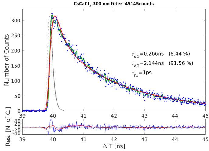
Figure 5.15: Rising edge of the scintillation-time distributions of CsCaCl 3 measured under X-ray excitation applying a) 254 nm and b) 300 nm bandpass filters in front of the hybrid PMT photocathode. The black dotted line represents the IRF of the setup, the green line is a sliding average of the distribution, and the red line is the fit of the data. From reference [88].
