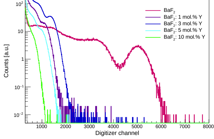
Figure 5.2: Integrated charge distributions of 3 \times 3 \times 3 mm 3 BaF 2 and BaF 2 :Y samples under 662 keV \gamma -ray irradiation.
