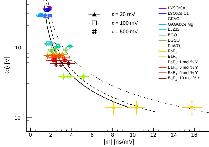
Figure 8.12: Average energy pulse amplitude \langle\varphi\rangle produced by a charged pion traversing the full length of the crystal plotted against the unsigned slope |m| obtained from the linear fit of the time delay - amplitude scatter plot (as shown in Figure 8.7) at 20, 100, and 500 mV thresholds on the time signal.
