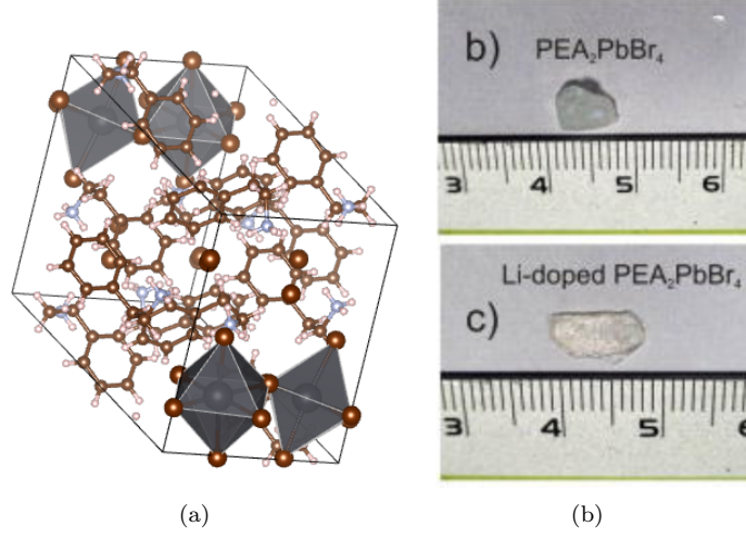
Figure 6.1: Crystallographic structure of PEA 2 PbBr 4 and pictures of two PEA 2 PbBr 4 and lithium-doped PEA 2 PbBr 4 samples. From reference [101].
