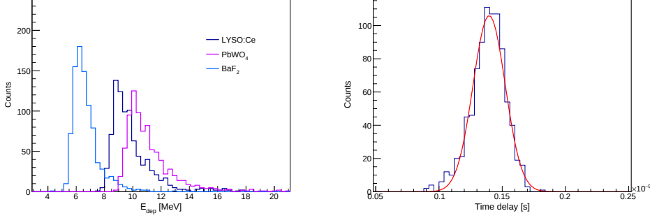
Figure 7.1: Energy deposited by the \pi^+ beam in 10 mm long LYSO:Ce, PbWO 4 and BaF 2 (left) and timestamps distribution extracted from a 2 \times 2 \times 10 \text{ mm}^3 LYSO:Ce pixel fitted using a Gaussian function (right).
