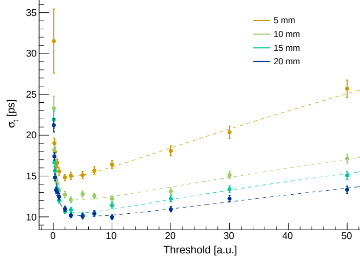
Figure 7.2: Time resolution achieved for 2 \times 2 \times L mm 3 LYSO:Ce crystals (with L = 5, 10, 15 or 20 mm) against the threshold employed to extract the timestamp from the digitalized pulses in output from the simulations. The time performance of each detector is evaluated at the fit minimum. As the single SPAD pulse simulated has an amplitude of about 0.6 in these arbitrary units, the optimum is usually achieved for a threshold corresponding to about 10 times the single SPAD amplitude.
