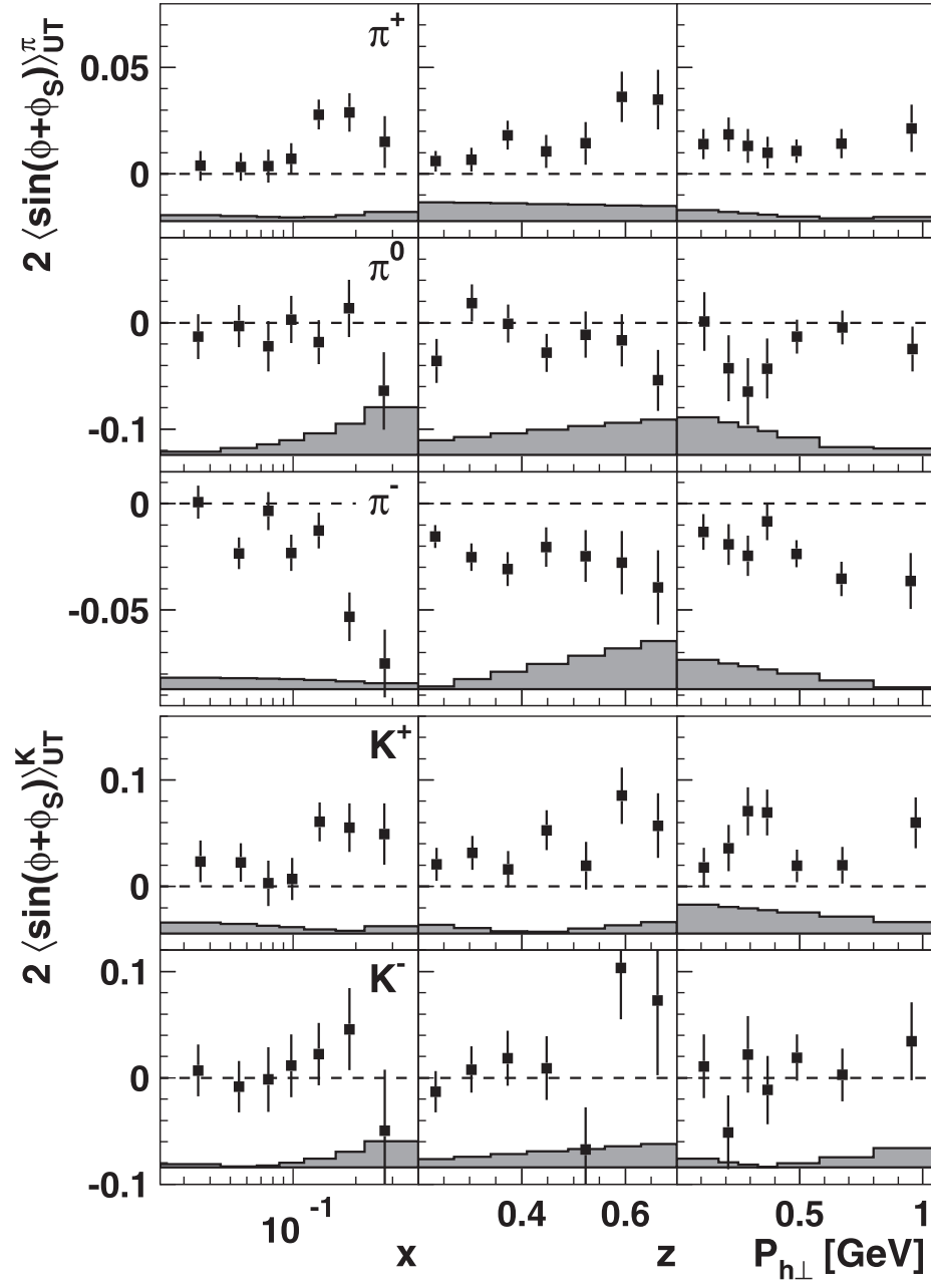
Figure 2.9: Results of the Collins asymmetry measured at HERMES on a proton target [30].
