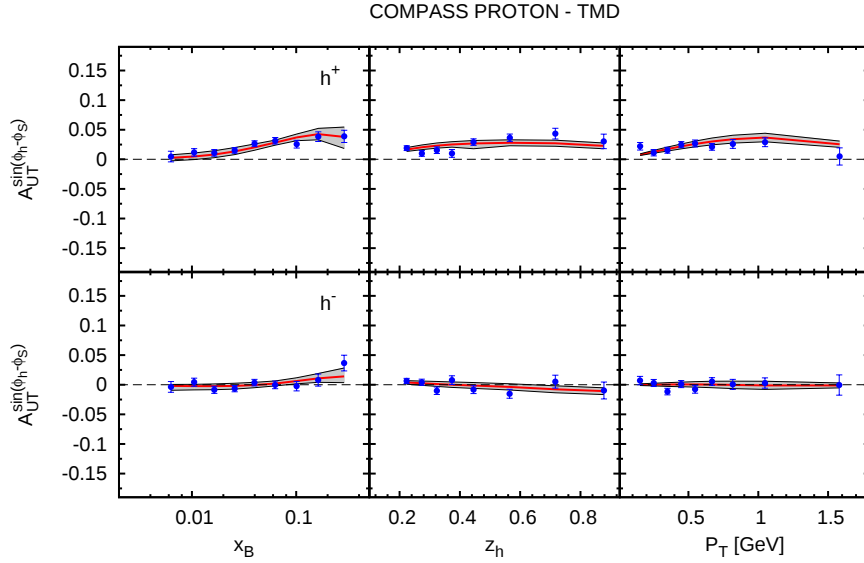
Figure 6.15: Sivers asymmetry for unidentified hadrons from COMPASS 2010 run together with TMD evolution fit by Anselmino et al. [74].
