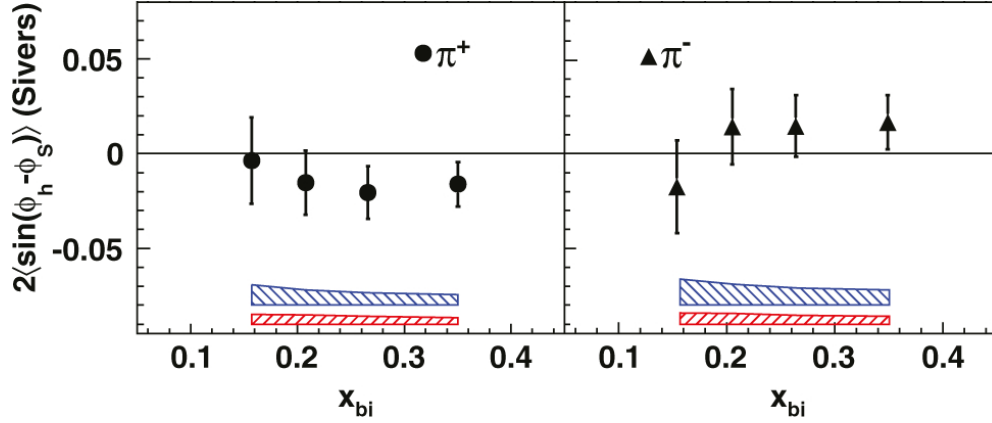
Figure 2.15: The extracted Sivvers asymmmtries at JLab HallA [35].
