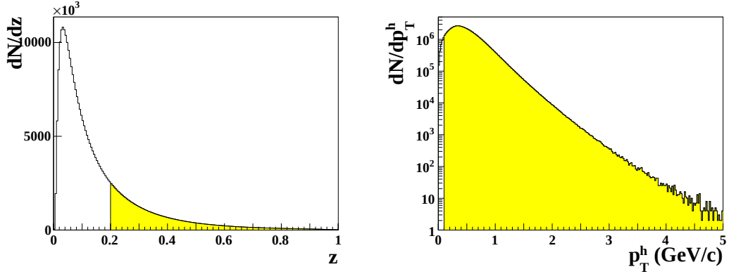
Figure 4.5: Kinematic distribution of z (left) and p_T^h (right) before (white) and after (yellow) the specific cuts.
