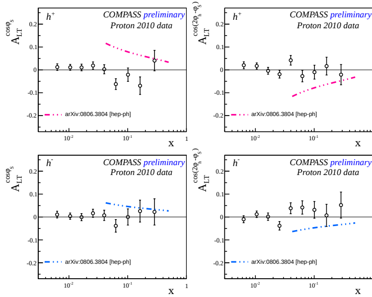
Figure 6.25: A_{LT}^{\cos(\phi_S)} (left) and A_{LT}^{\cos(2\phi_h - \phi_S)} (right) asymmetry for unidentified hadrons in bins of x with the model predictions of [78].
