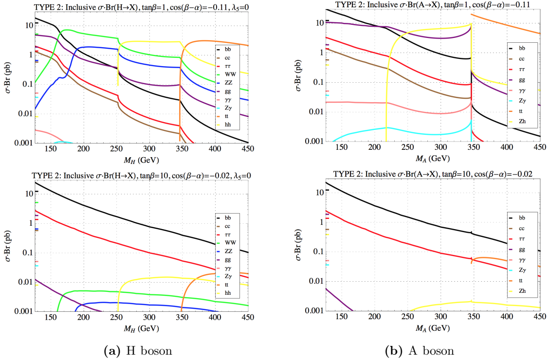
Figure 1.5: Inclusive production \sigma \times \mathcal{B} for an example of a type-II 2HDM, for (a) the H boson and (b) the A boson. The top figures use \tan\beta=1 and \cos(\beta - \alpha) = -0.11 , the bottom figures are made for \tan\beta=10 and \cos(\beta - \alpha) = -0.02 . At low \tan\beta the H \rightarrow hh and A \rightarrow Zh decays are enhanced for masses up to 350 GeV [54].
