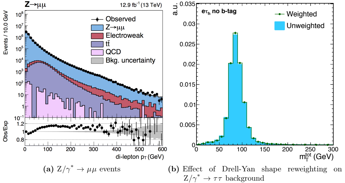
Figure 5.13: (a) The mis-modelling in the di-lepton p_T distribution as observed in Z/\gamma^* \rightarrow \mu\mu events, used to derive the correction and (b) the impact of applying the Drell-Yan shape reweighting on the total transverse mass distribution of the Z/\gamma^* \rightarrow \tau\tau background in the no b-tag category of the e\tau_h channel. The events shown in (a) were selected by requiring two oppositely charged muons, passing kinematic cuts, identification and isolation requirements equivalent to the selections applied to muons as described in section 5.2.2.
