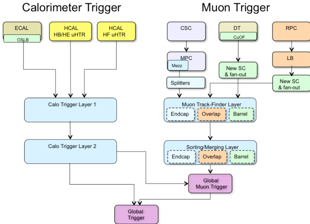
Figure 2.9: Schematic of the different components of the L1 trigger [91].
