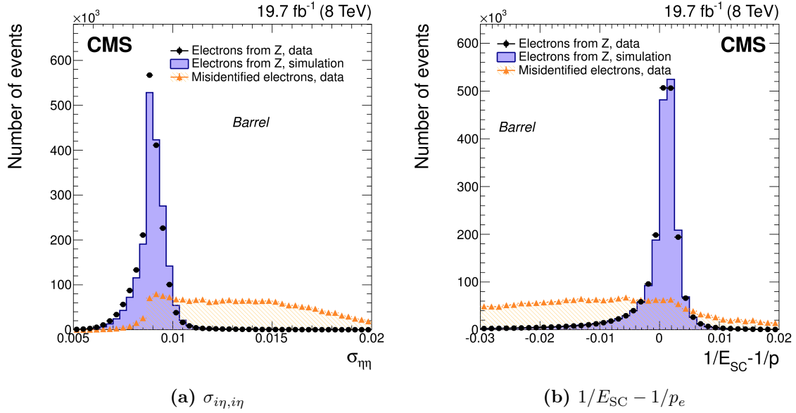
Figure 3.2: (a) \sigma_{i\eta,i\eta} and (b) 1/E_{\text{SC}} - 1/p_e for real (black points) and misidentified (yellow triangles) electrons in a dataset corresponding to 19.7 fb -1 taken at \sqrt{s} = 8 TeV, overlaid on the distributions for simulated real electrons in purple [99].
