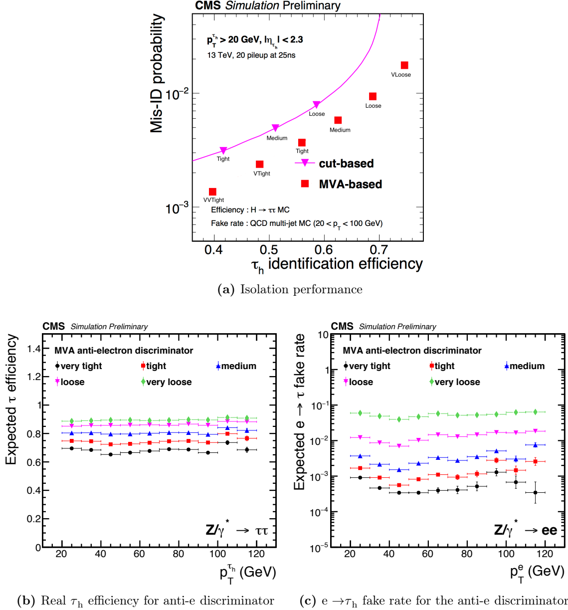
Figure 3.5: (a) The jet \rightarrow \tau_h fake rate in simulated QCD multijet events versus \tau_h identification efficiency for simulated H \rightarrow \tau\tau events, comparing the MVA-based isolation discriminator in red with the cut-based isolation discriminator in pink. Tighter working points give lower hadronic tau identification efficiencies and lower fake rates, and for the same \tau_h identification efficiency the fake rate from the MVA-based discriminator is lower than from the cut-based discriminator. Figure adapted from [119]. (b) The \tau_h identification efficiency in simulated Z/\gamma^* \rightarrow \tau\tau events for different working points of the anti-electron discriminator as a function of the p_T of the \tau_h , and (c) the e \rightarrow \tau_h fake rate in simulated Z/\gamma^* \rightarrow ee events for different working points of the anti-electron discriminator, as a function of the p_T of the electron [119]. Note that the efficiencies and fake rates are fully derived from simulation and serve to give an indication of the efficiencies of the different working points relative to each other.
