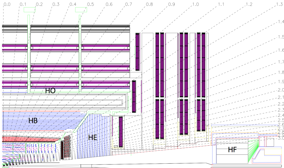
Figure 2.7: Illustration of a quadrant of the HCAL, showing the different sub-systems of the detector [80].
