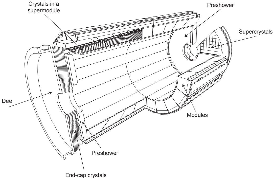
FIGURE 3.5: Layout of the CMS Electromagnetic calorimeter.
