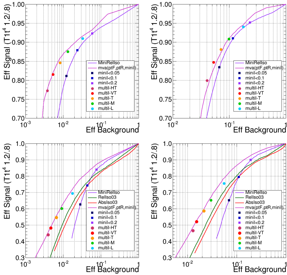
FIGURE 9.5: Prompt lepton selection efficiency versus misidentified lepton efficiency for electrons (left) and muons (right) with p_T > 25 GeV (top) and 10 < p_T < 25 GeV (bottom) in T1tttt (1.2/0.8) events. The tight working point corresponds to the orange full circle, and the loose working point to the green full circle. The standard isolation is indicated by the black point and the pure mini isolation by the violet line.
