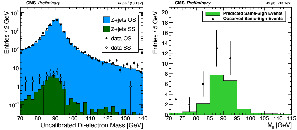
FIGURE 9.12: Left: Opposite-sign and same-sign di-electron events that are used to extract the charge misidentification probability. Right: Closure test on the charge misidentification probability. The measured charge misidentification probability is applied to a opposite-sign events in a Z +jets sample and comparing them to the observed same-sign events in the same sample without truth-matching
