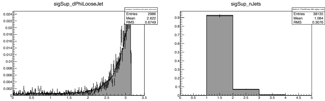
FIGURE 5.3: \Delta\phi(\text{lep}, \text{jet}) (left) and N_{\text{jets}} distribution of the events in the QCD control sample. Most of the events have one jet and in such case it tends to be away from the lepton.
