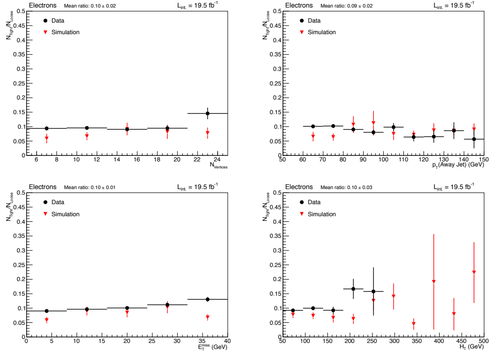
FIGURE 5.8: Fake ratios for electrons as a function of the number of vertices (top left), away jet p_T (top right), E_T^{\text{miss}} (bottom left) and H_T (bottom right). The red markers depict the values obtained from a cocktail of Standard-Model Monte-Carlo samples including QCD, top and electro-weak processes.
