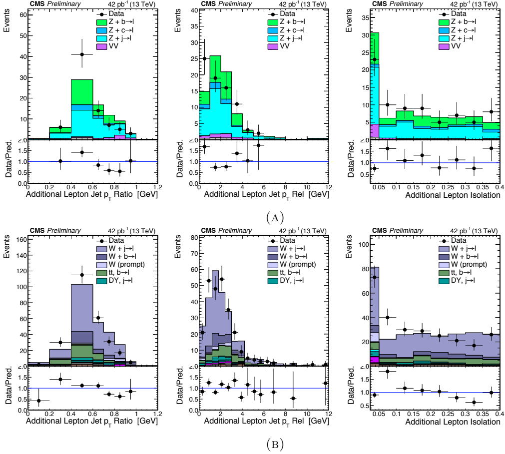
FIGURE 9.7: Data to simulation comparisons for lepton identification performance studies. From left to right the probe lepton p_T^{\text{ratio}} , p_T^{\text{rel}} and I_{\text{mini}} . Z+\ell control region (Fig. 9.7a) is displayed on top and W+\ell (Fig. 9.7b) on the bottom row.
