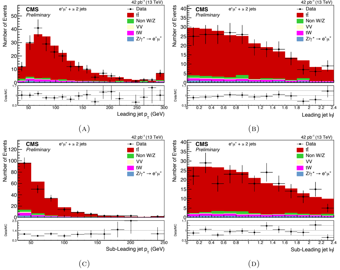
FIGURE 8.6: The distributions for 8.6a p_T and 8.6b \eta for the highest- p_T jet, and for 8.6c p_T and 8.6d \eta for the second highest- p_T jet after all selections. The expected distributions for t\bar{t} signal and individual backgrounds are shown after data-based corrections are applied; for the left plots 8.6a, 8.6c the last bin contains the overflow events. The ratios of data to the sum of the expected yields are given at the bottom of each panel.
