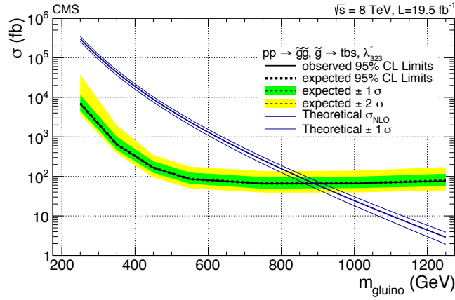
FIGURE 6.10: 95% CL upper limit on the gluino production cross section for an RPV simplified model, pp \rightarrow \tilde{g}\tilde{g}, \tilde{g} \rightarrow tbs(\bar{t}\bar{b}\bar{s}) .
