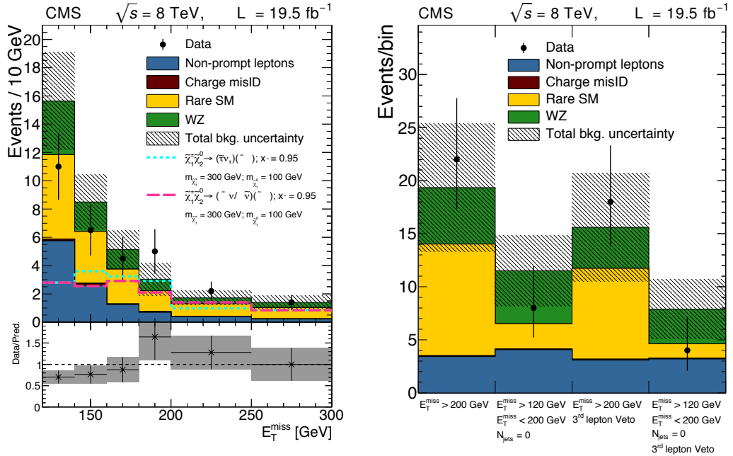
FIGURE 7.4: Left: E_T^{\text{miss}} distribution for same-sign dilepton candidates in comparison with the SM expectations. The bottom panel shows the the ratio and corresponding uncertainty of the observed and total SM expected distributions. The third lepton veto is not applied. The distributions of example signal scenarios are overlaid. Right: Observed yields and expected backgrounds for the different search regions. In both plots, events with E_T^{\text{miss}} > 120 \text{ GeV} are displayed, and the hashed band shows the combined statistical and systematic uncertainties of the total background.
