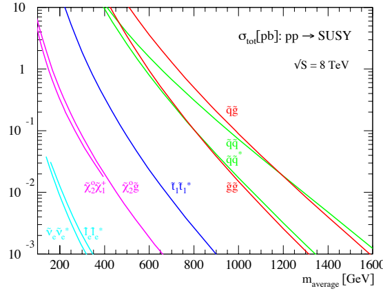
FIGURE 5.1: Production cross section for several SUSY processes at proton-proton collisions at a center of mass energy of 8 TeV.
