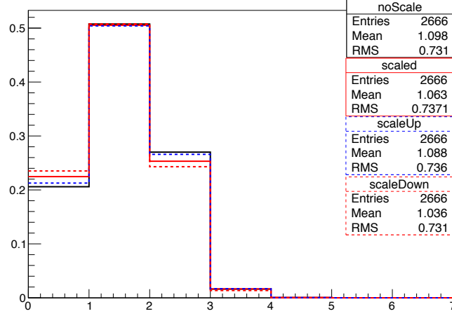
FIGURE 6.1: N_{\text{b-jets}} distribution for t\bar{t} W MC sample to illustrate the effect of the b-tag scale factors on the number of b-tagged jets in a sample.
