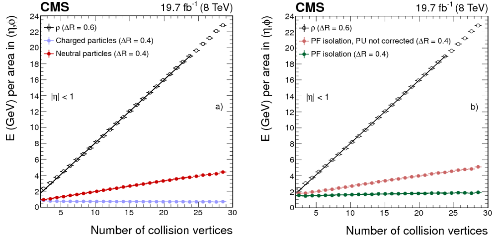
FIGURE 4.3: Average energy density as a function of the number of reconstructed proton-proton collision vertices, for electron candidates with p_T > 20 GeV and |\eta| < 1 from data dominated by Z \rightarrow e^+e^- events. The energy density is shown a) for the event \rho (open dots) and separated components of the particle isolation: neutral particles (red dots) and charged particles associated with the vertex (blue dots), and b) after the correction for pile-up on PF isolation.
