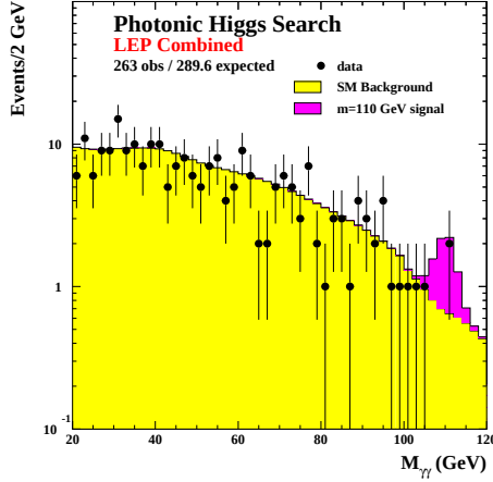
Figure 1. Distribution of the reconstructed di-photon invariant mass for all final states combined. The combined LEP data are shown together with the background and a Higgs boson signal with mass m_h = 110 GeV.
