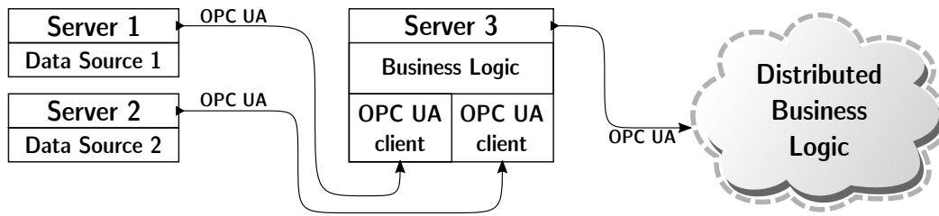
Figure 5.10: An example of a chained OPC UA system with multiple clients and servers. The lines and arrows illustrate the information flow.
