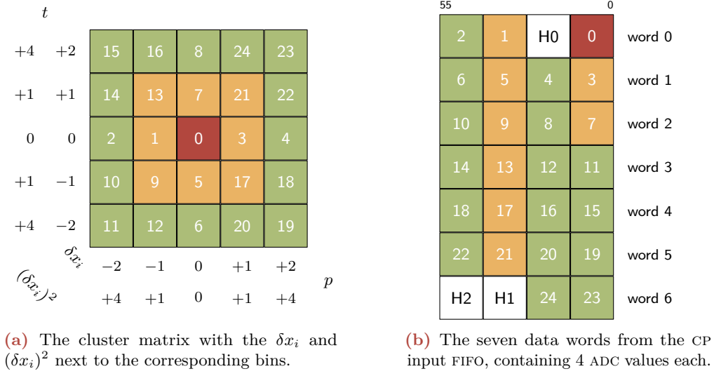
Figure 5.23: Mapping of the cluster data to the CP input FIFO.
