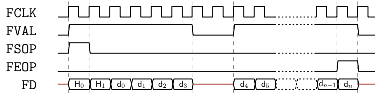
Figure 4.3: The transmission protocol towards the data path wrapper. The data stream consists of two header words, followed by the actual data. The SOP flag must be high for the very first word of a package, while the EOP marks the very last one. The valid flag is used to specify when the data is to be used, based on [49].
