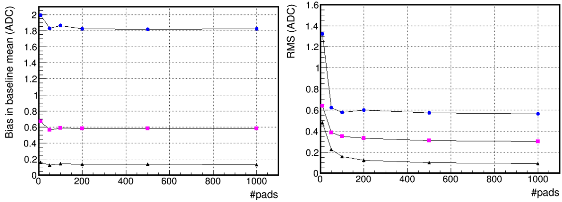
Figure 3.3: Remaining bias of the ADC value (left) and additional noise from the CM effect (right) after correcting with the averaging method. The result is shown as a function of number of pads which were taken into account. The three different colours show the three different peak exclusion algorithms (fixed threshold in blue, complete peak removal in black and in magenta where the first time bin of the peak was still included in the averaging), taken from [33].
