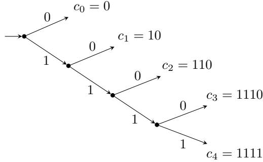
Figure 3.4: Example of a small Huffman tree with only five codes.
