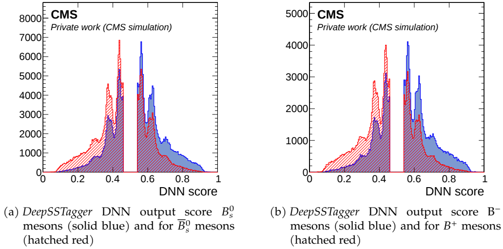
Figure 10.1: DeepSSTagger DNN output score in B_s^0 \rightarrow J/\psi \phi(1020) (left) and B^+ \rightarrow J/\psi K^+ (right) samples
