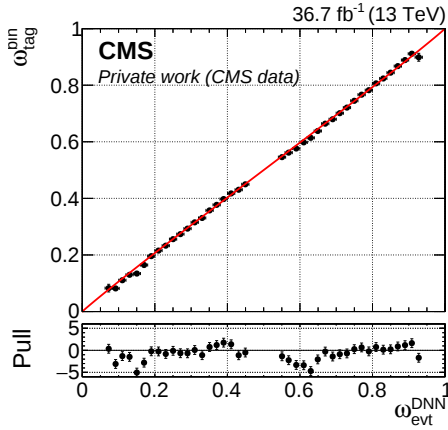
(a) DeepSSTagger calibration plot for the 2017 B^+ \rightarrow J/\psi K^+ data sample.
