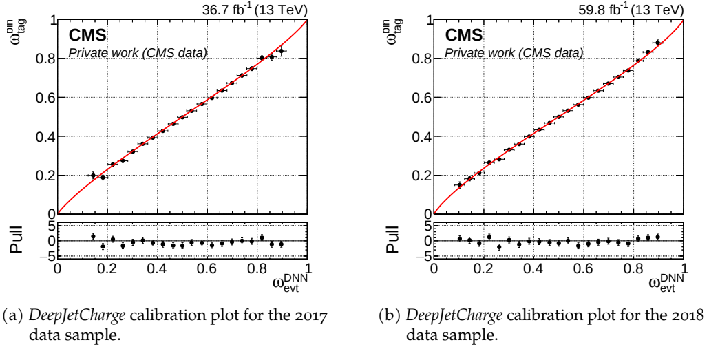
Figure 9.4: Result of the mistag probability calibration fit for DeepJetCharge on B^+ \rightarrow J/\psi K^+ decays from data. The solid red line shows the calibration fit to data (solid markers).
