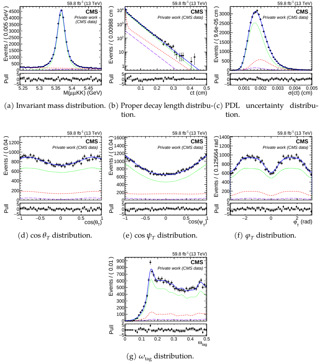
Figure 13.21: Distribution of the input observables and the corresponding fit projections in dataset_JpsiMuon (2018).
