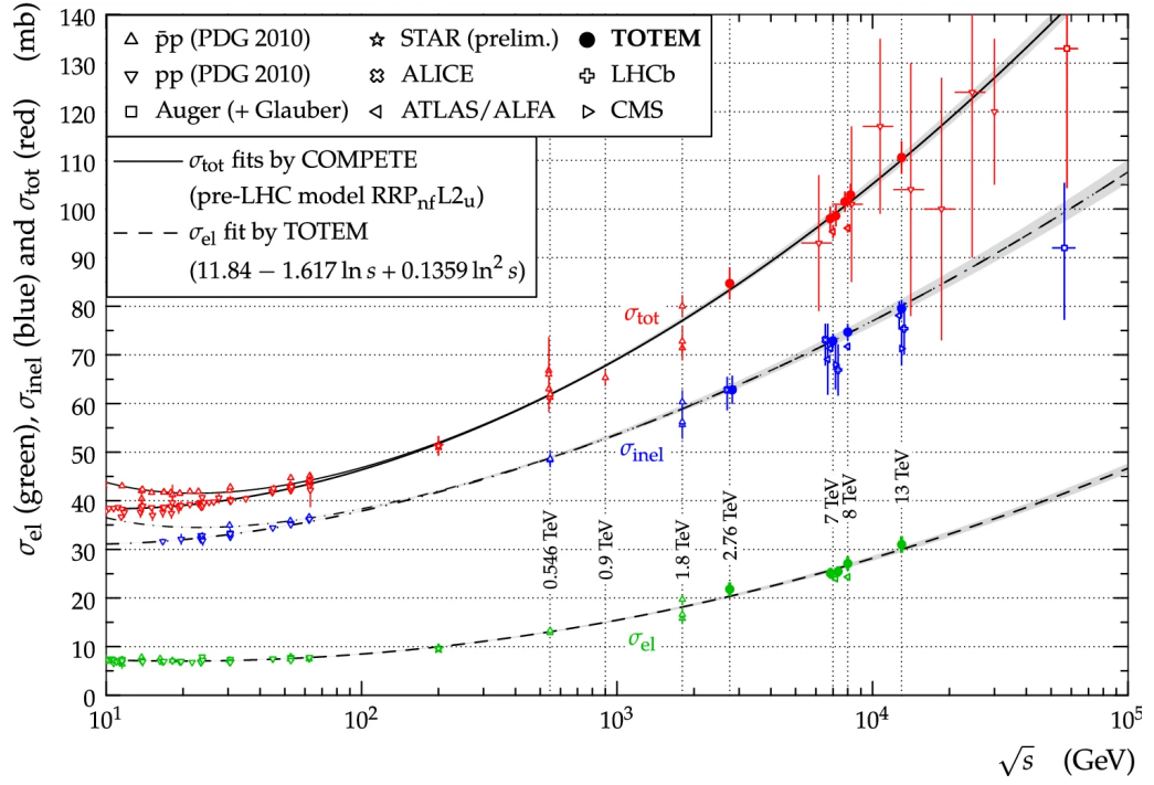
Figure 3.3: Overview of the elastic ( \sigma_{\text{el}} ), inelastic ( \sigma_{\text{inel}} ) and total ( \sigma_{\text{tot}} ) cross-section for pp collisions as a function of \sqrt{s} . The continuous black lines (lower for pp , upper for p\bar{p} ) represent the best fits of the total cross section data by the COMPETE collaboration. The dashed line results from a fit of the elastic cross section data. The dash-dotted lines refer to the inelastic cross section and are obtained as the difference between the continuous and dashed fits [62]
