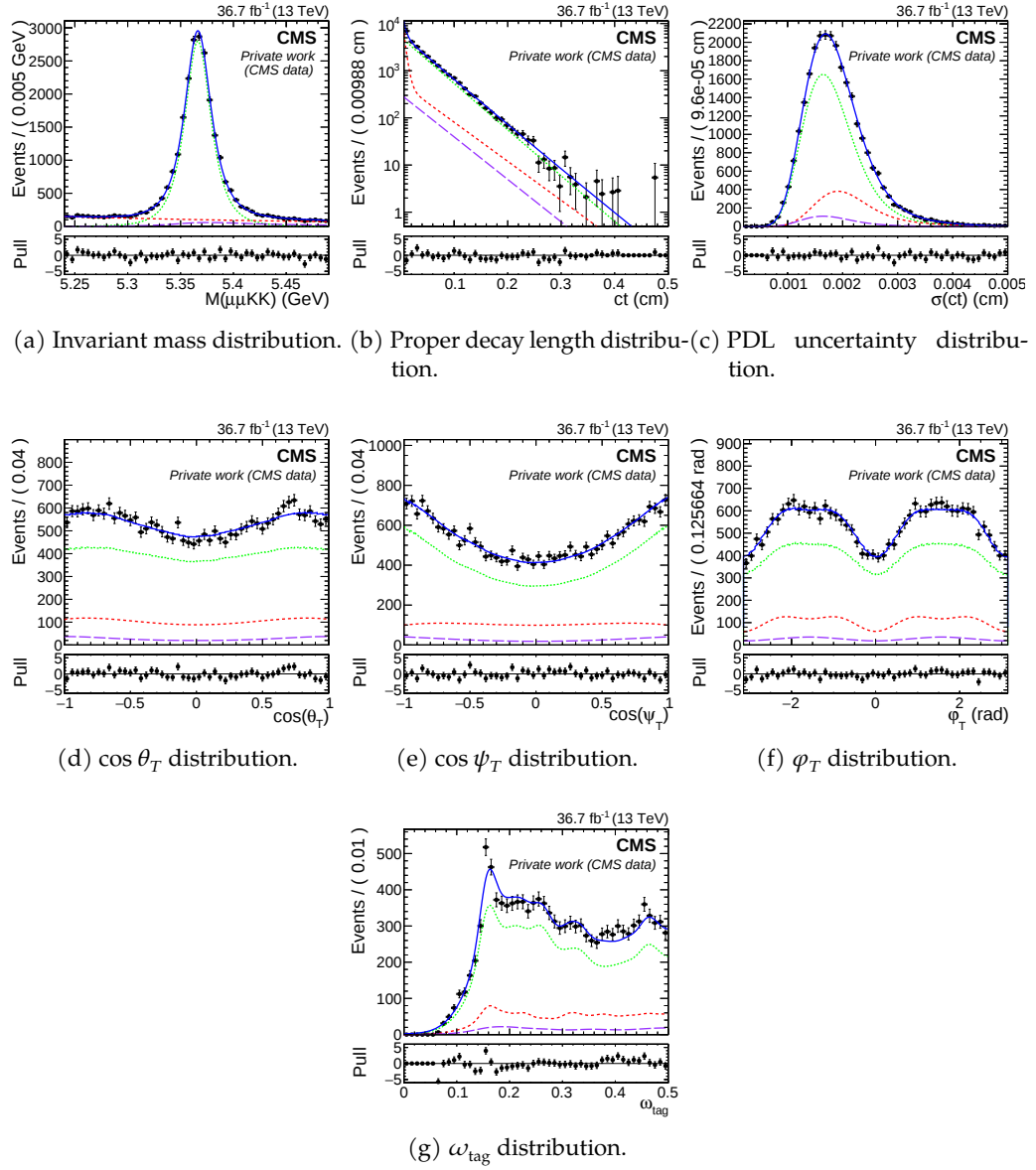
Figure 13.20: Distribution of the input observables and the corresponding fit projections in dataset_JpsiMuon (2017).
