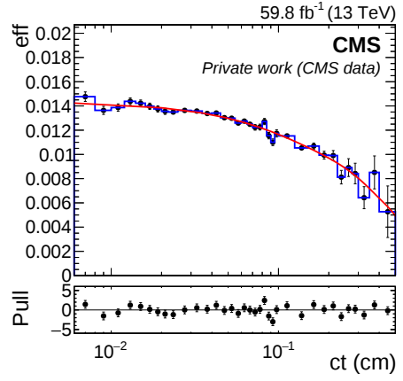
(b) PDL efficiency in dataset_JpsiMuon (2018).
