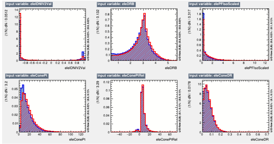
(b) From left to right, top to bottom: \text{eleIDNIV2Val} , \Delta R_{\eta,\phi}(e, B) , \text{Iso}_e , p_T^{\text{cone}} , p_T^{\text{el}} and \Delta R_{\eta,\phi}(w, \text{cone}) .
