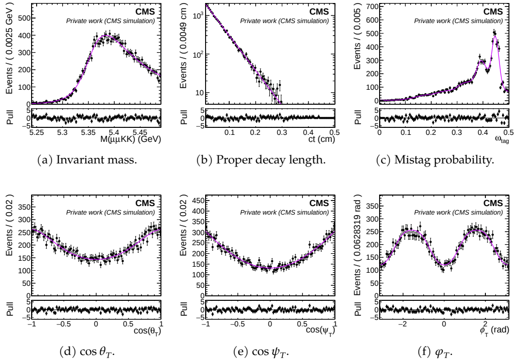
Figure 13.7: Physics observables distributions for B_s^0 \rightarrow J/\psi \phi(1020) candidates reconstructed in B^0 \rightarrow J/\psi K^*(892)^0 simulated events for dataset_JpsiTrkTrk (2018). The PDL uncertainty is not shown as it is not used. The solid line represents the 1D projection of the P_{\text{bkg}B^0} fit.
