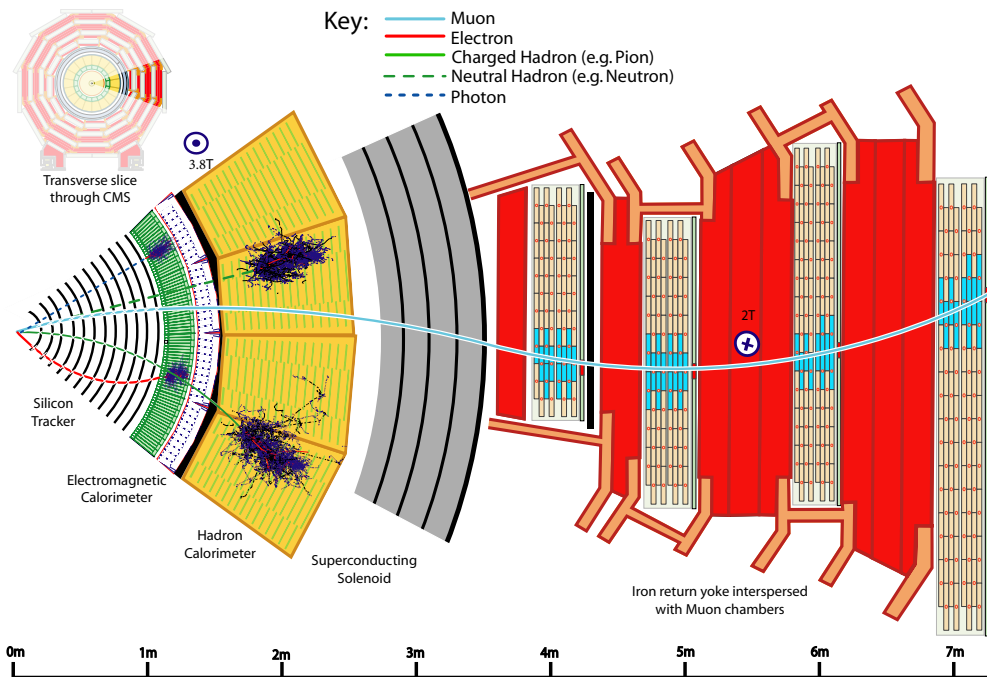
Figure 3.13: View of a transverse slice of the CMS detector with its sub-systems. A schematic view of the specific particle interactions, from the beam interaction region to the muon system, is also shown. The muon and the charged pion are positively charged, and the electron is negatively charged. Figure from Ref. [76].
