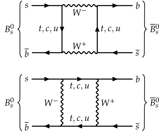
Figure 2.3: Leading order diagrams for B_s^0 - \bar{B}_s^0 mixing.
