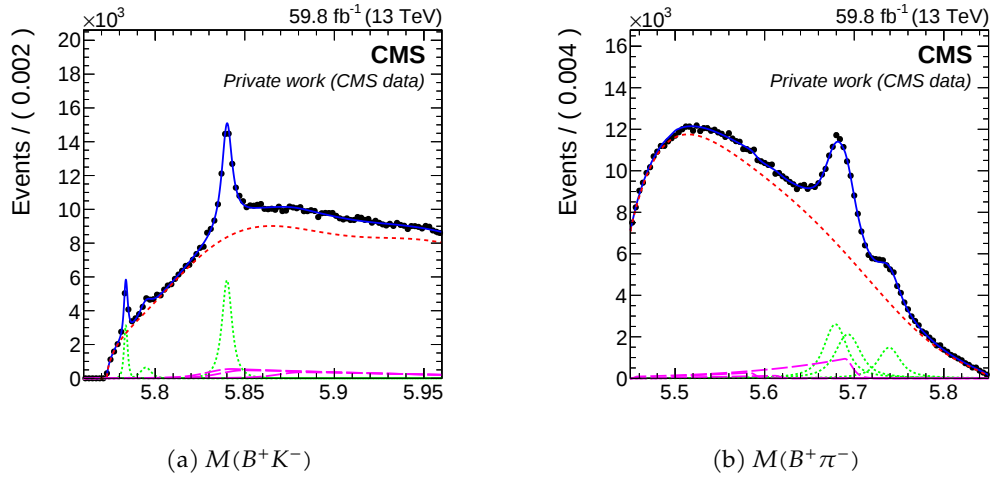
Figure 10.5: Final result of the fit to the mass of the B_s^{*+} and B^{0*+} resonances. The short-dashed green curves represent the correctly reconstructed resonances, depending on the plot, while the long-dashed purple represents the wrong reconstructed resonance. In both plots the red curve represents the combinatorial background.
