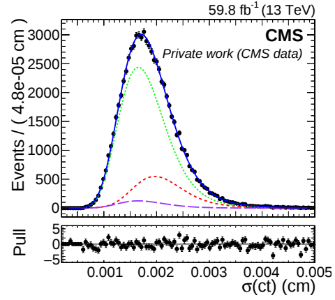
(b) PDL uncertainty distribution.
