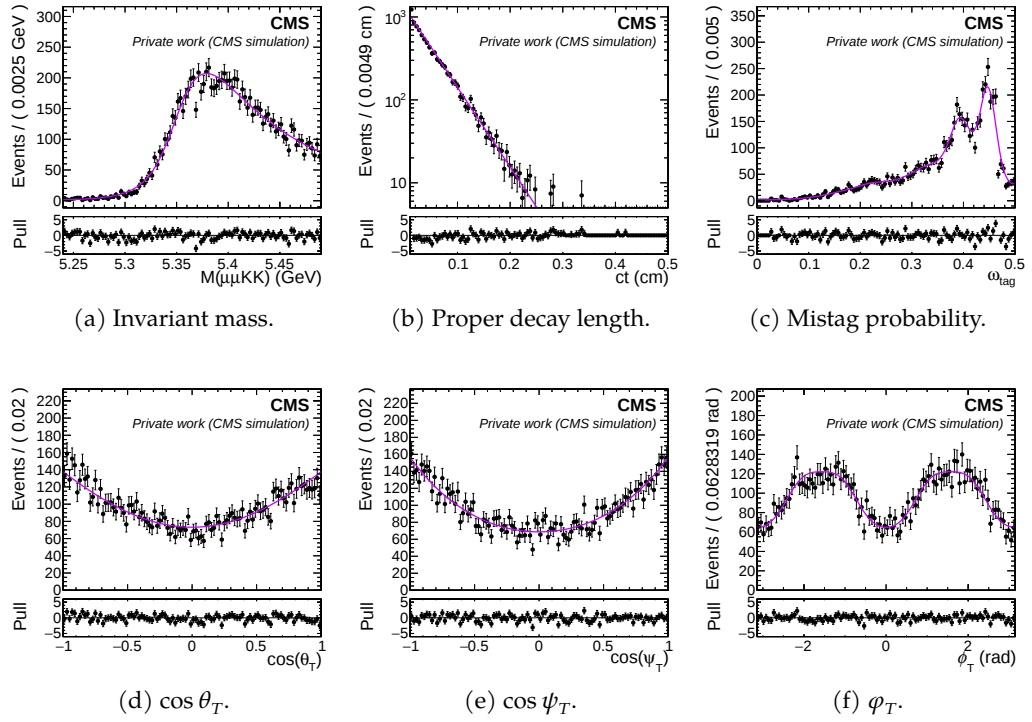
Figure 13.6: Physics observables distributions for B_s^0 \rightarrow J/\psi \phi(1020) candidates reconstructed in B^0 \rightarrow J/\psi K^*(892)^0 simulated events for dataset_JpsiTrkTrk (2017). The PDL uncertainty is not shown as it is not used. The solid line represents the 1D projection of the P_{\text{bkg}B^0} fit.
