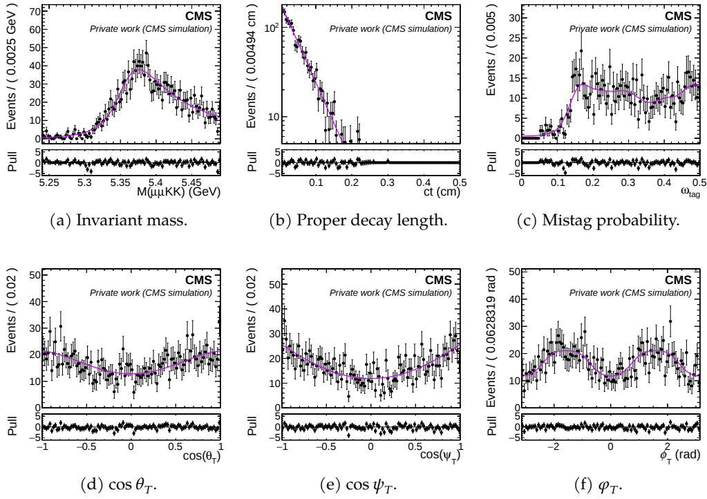
Figure 13.5: Physics observables distributions for B_s^0 \rightarrow J/\psi \phi(1020) candidates reconstructed in B^0 \rightarrow J/\psi K^*(892)^0 simulated events for dataset_JpsiMuon (2018). The PDL uncertainty is not shown as it is not used. The solid line represents the 1D projection of the P_{\text{bkg}B^0} fit.
