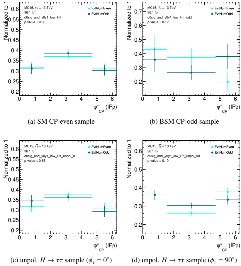
Figure C.4: The \phi_{CP}^* distribution comparing two randomly chosen, equally sized subsets of the CP-even or CP-odd H \rightarrow \tau\tau signal samples in the IP- \rho d_0^{\text{sig}}/Y_{\pm} low preselection region.
