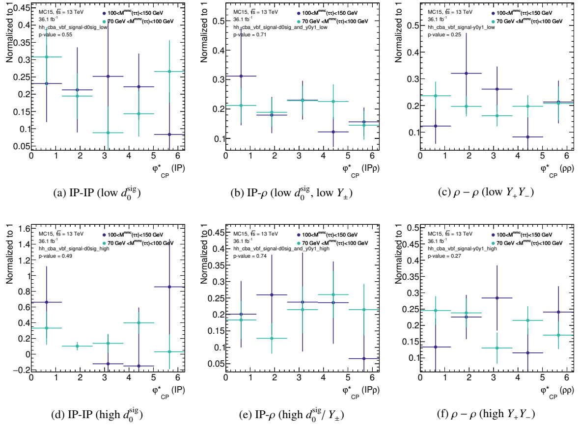
Figure F.6: \phi_{CP}^* distribution of SHERPA2.2 Z \rightarrow \tau\tau in the vbf signal region in the H and Z mass window
