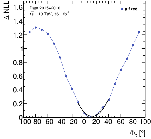
Figure 8.22: \Delta \text{NLL} curve for the fit to \varphi_{CP}^* combining all decay modes using data with a constant H \rightarrow \tau\tau signal strength \mu including systematic and statistical uncertainties.
