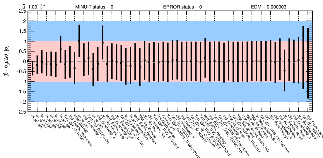
Figure G.9: Pull distribution of all NPs included in the fit sorted by their constraint for \phi_\tau = 90^\circ .
