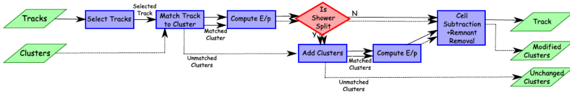
Figure 3.9: Sketch of the jet particle flow algorithm procedure[95].
