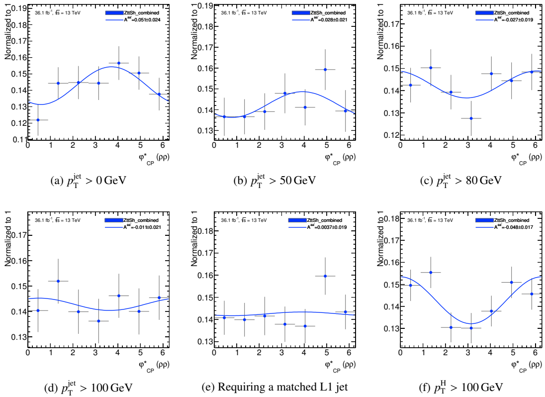
Figure 5.4: \phi_{CP}^* distribution in Z \rightarrow \tau\tau events after the Z region selection for different cuts on p_T^{\text{jet}} , p_T^{\text{H}} and a matched L1 jet.
