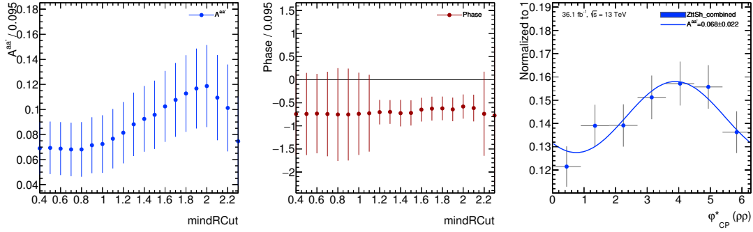
(a) Vary the minimum \Delta R_{\tau\tau} cut. The \varphi_{CP}^* distribution presented requires the Z \rightarrow \tau\tau selection and \Delta R_{\tau\tau} > 0.8 .
