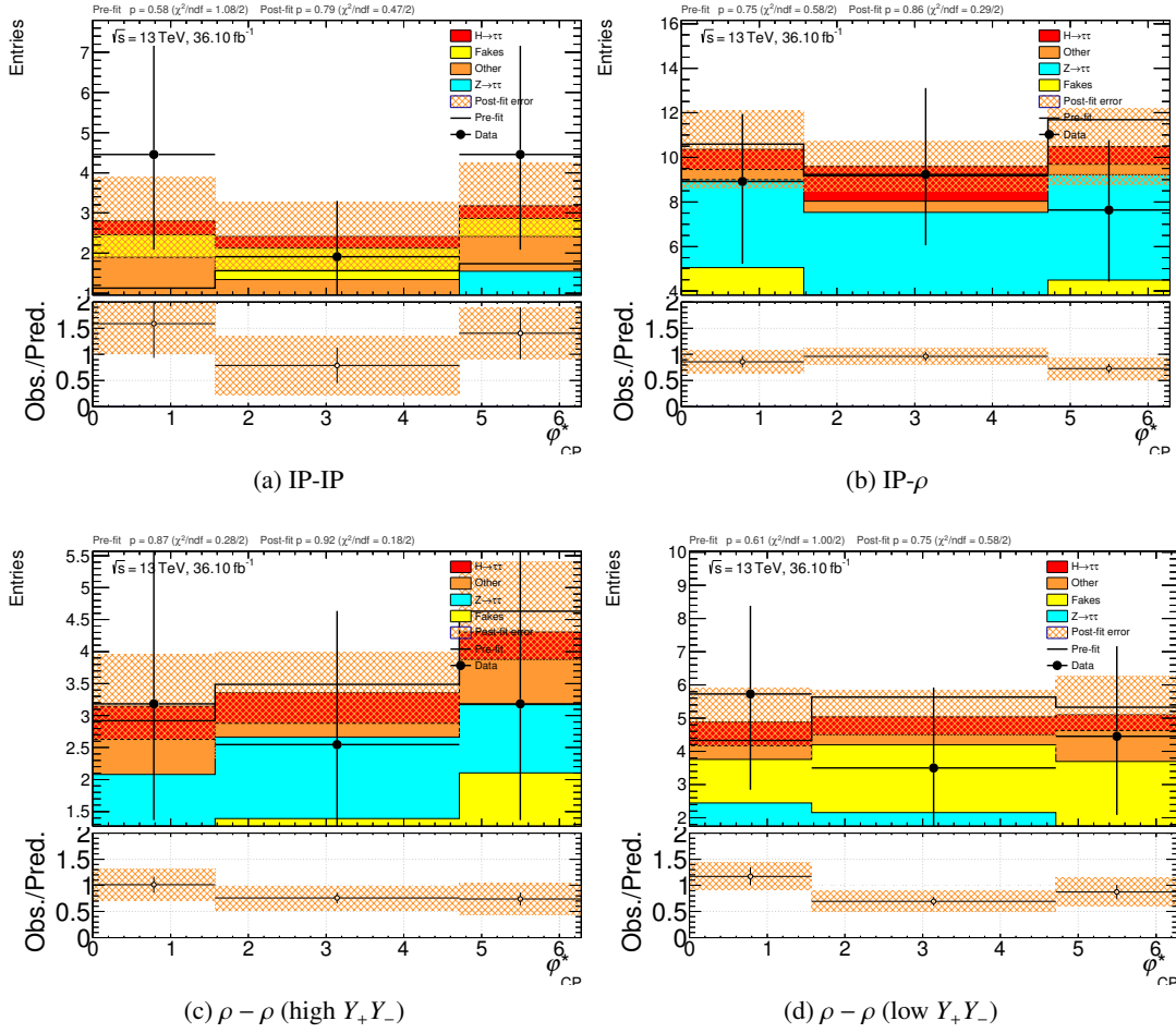
Figure 8.18: Post-fit \varphi_{CP}^* distributions in the vbf signal regions after the fit to data with a luminosity of \mathcal{L} \approx 36.1 \text{ fb}^{-1} at a CMS energy of \sqrt{s} = 13 \text{ TeV} .
