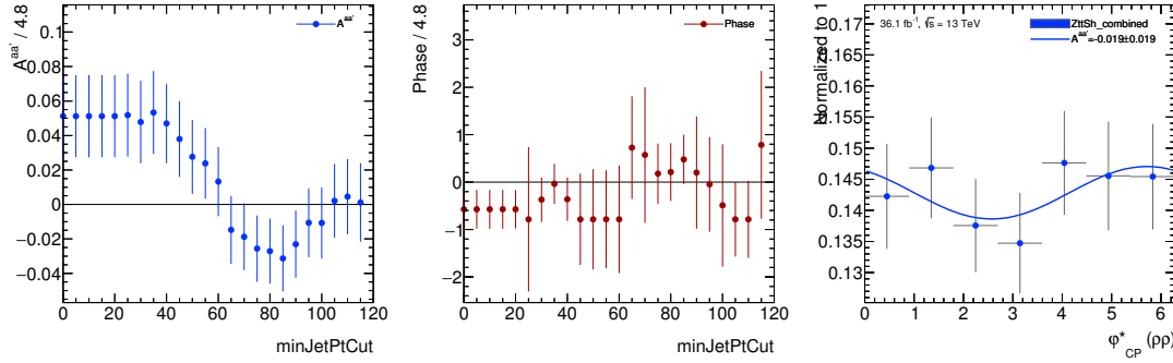
Figure 5.3: Asymmetry and phase of the \phi_{CP}^* distribution after variation of the minimum jet p_T cut. The presented \phi_{CP}^* distribution requires p_T^{\text{jet}} > 70 GeV as it is needed if using the 2016 trigger in the analysis.
