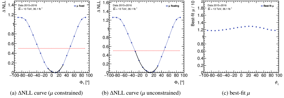
Figure 8.21: \Delta \text{NLL} curve for the fit to \varphi_{CP}^* combining all decay modes using data with the H \rightarrow \tau\tau signal strength \mu constrained to unity (a) and an unconstrained \mu (b). The best-fit \mu distribution is shown in (c).
