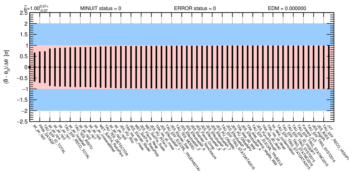
Figure 8.15: Pull distribution of all systematic uncertainty NPs included after a fit to Asimov data sorted by their constraint for \phi_r = 0^\circ .
