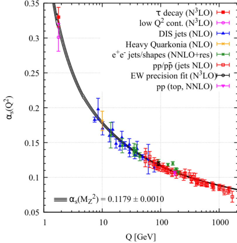
FIGURE 1.1: Summary of measurements of the strong coupling constant \alpha_s , as a function of energy scale Q , from [7]. The order to which perturbative QCD is applied is given in the brackets.
