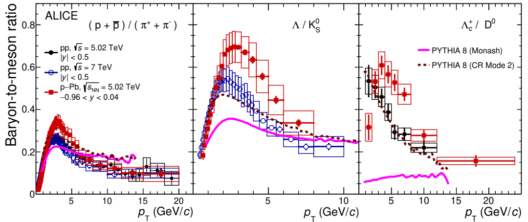
FIGURE 5.13: The baryon-to-meson ratios in the light-flavour and charm sector; p/\pi in pp collisions at \sqrt{s} = 5.02 TeV and 7 TeV and p-Pb collisions at \sqrt{s_{NN}} = 5.02 TeV [69], \Lambda/K_S^0 in pp collisions at \sqrt{s} = 7 TeV and p-Pb collisions at \sqrt{s_{NN}} = 5.02 TeV [108, 109] (middle), and \Lambda_c^+/D^0 in pp collisions at \sqrt{s} = 5.02 TeV and p-Pb collisions at \sqrt{s_{NN}} = 5.02 TeV (right). The data are compared to predictions from PYTHIA 8 [24, 25]. See text for model details.
