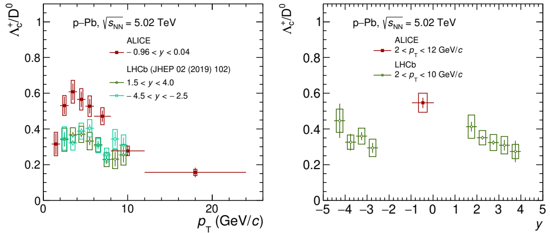
FIGURE 5.12: The \Lambda_c^+/D^0 ratio measured in p-Pb collisions at \sqrt{s_{NN}} = 5.02 \text{ TeV} , compared with the measurement at forward and backward rapidity [72] by the LHCb collaboration. The measurements are shown as a function of p_T (left) and as a function of y (right).
