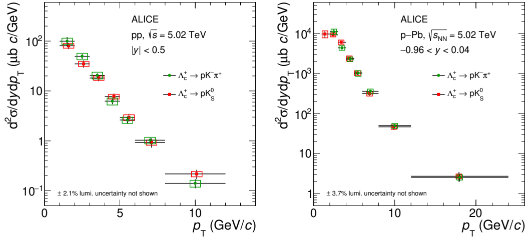
FIGURE 5.4: Left: p_T -differential prompt \Lambda_c^+ -baryon cross section in pp collisions at \sqrt{s} = 5.02 TeV in the interval 1 < p_T < 12 GeV/c. Right: p_T -differential prompt \Lambda_c^+ -baryon cross section in p-Pb collisions at \sqrt{s_{NN}} = 5.02 TeV in the interval 1 < p_T < 24 GeV/c. The statistical uncertainties are shown as vertical bars and the systematic uncertainties are shown as boxes.
