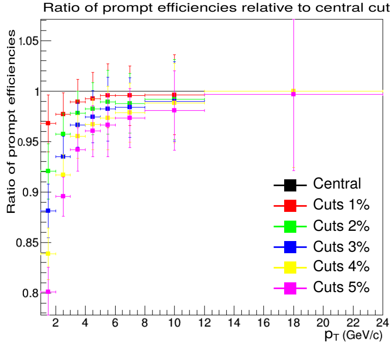
FIGURE 3.21: Ratio of prompt \Lambda_c^+ efficiencies for the different topological cuts (with range up to 5% change of cut parameters) for the study of the 1-2 GeV/ c bin.
