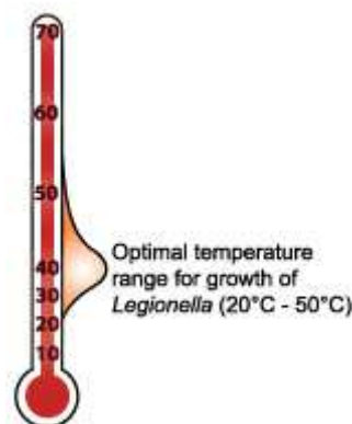
Figure XV: Optimal temperature range for growth of Legionella
