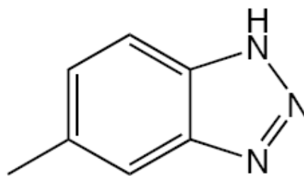
Tolyltriazole (TT)
