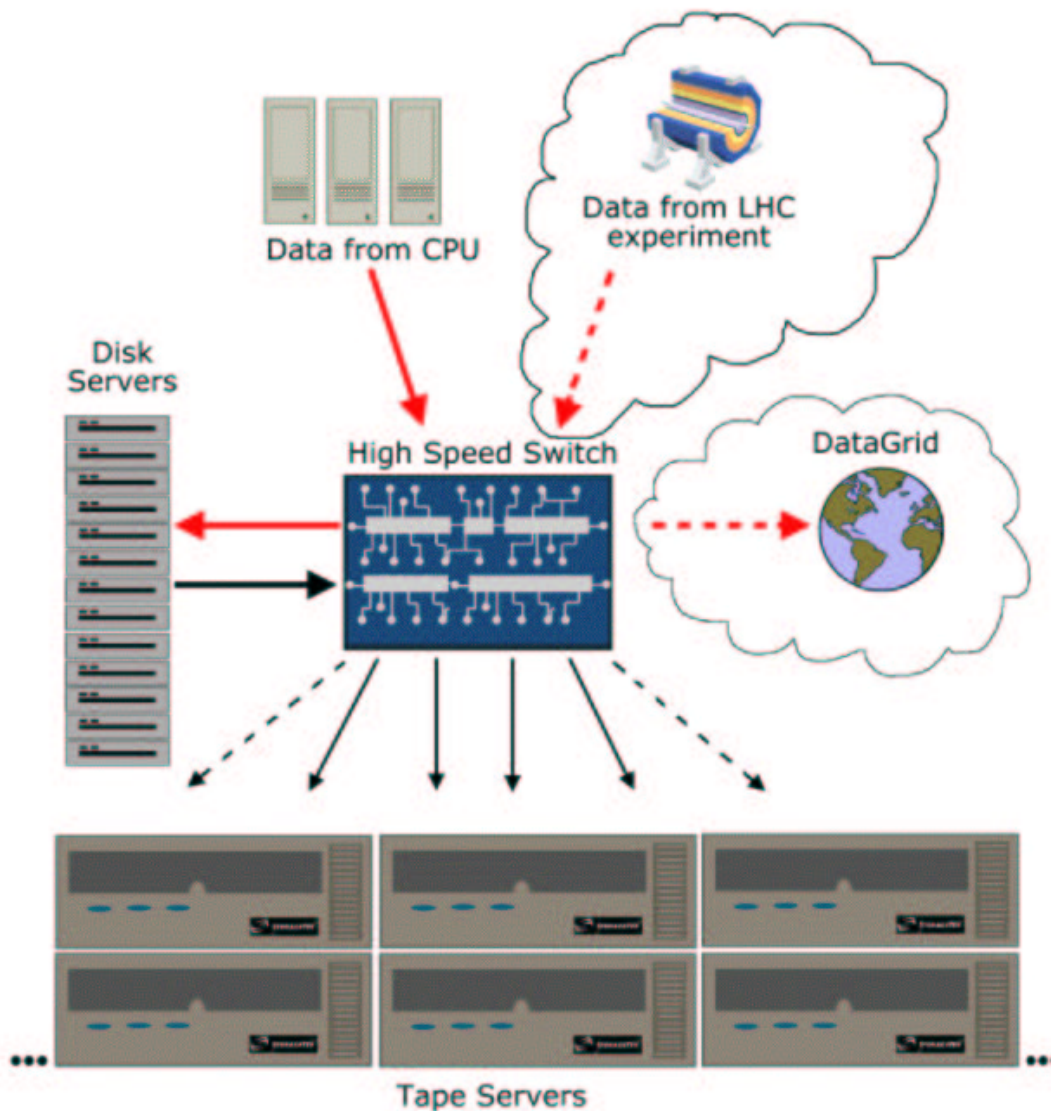
Figure 1.1: Schematic of the data setup for the storage-to-tape challenge. Data, in this case generated by 40 compute servers, is temporarily stored to disk, then copied to the 45 StorageTek tape servers. Once the Large Hadron Collider is running at CERN, the data will come directly from the experiments and a copy will be distributed onto the DataGrid that CERN and partners are currently developing.
