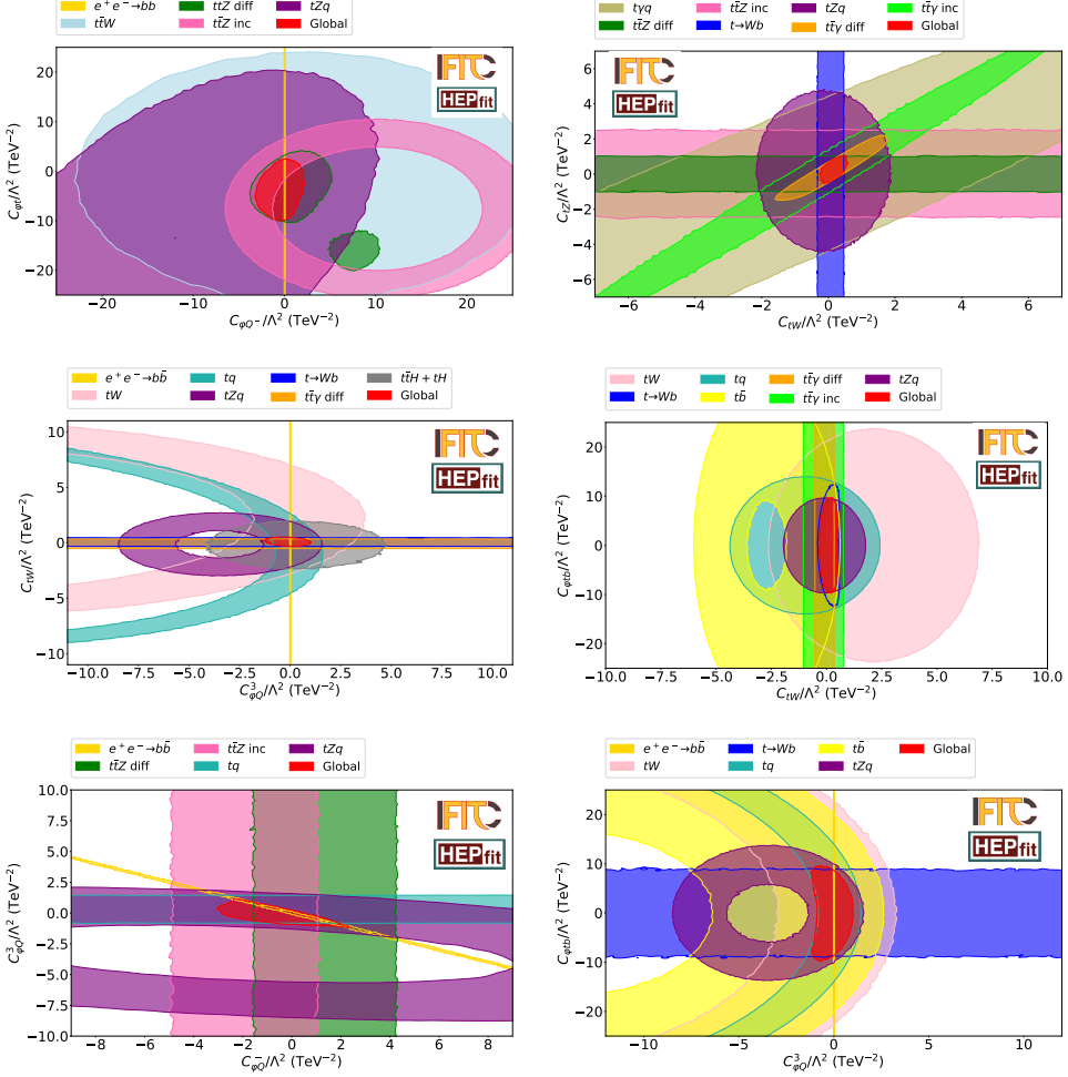
Figure 4.6: Two-dimensional 95% probability bounds on pairs of Wilson coefficients, C_{\phi Q}^- and C_{\phi t} in the upper leftmost panel, C_{tW} and C_{tZ} in the upper rightmost panel, C_{\phi Q}^3 and C_{tW} in the middle leftmost panel, C_{tW} and C_{\phi tb} in the middle rightmost panel, C_{\phi Q}^3 and C_{\phi Q}^2 in the lower leftmost panel, and C_{\phi tb} and C_{\phi Q}^3 in the lower rightmost panel. Bounds are presented for two-parameter fits to the most constraining measurements. The global fit results, marginalising over all other Wilson coefficients, are also shown (red area). All these fits include \Lambda^{-4} terms. Besides QCD production, in the case of t\bar{t}W process, the contribution of the electro-weak t\bar{t}Wq production is also included.
