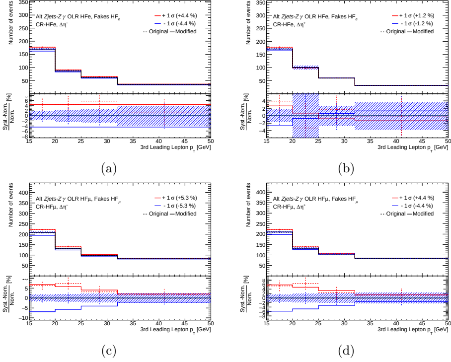
Figure D.4: Alternative Z +jets modelling for (a) CR-HF _e \Delta\eta^- , (b) CR-HF _e \Delta\eta^+ , (c) CR-HF _\mu , and (d) CR-HF _\mu . Uncertainty bands cover MC statistical uncertainties of the nominal sample.
