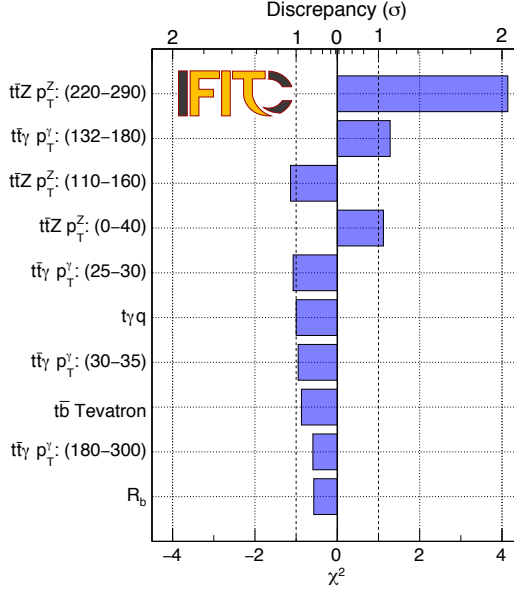
Figure 4.2: Contributions to the \chi^2_{SM} of some of the input measurements, together with their discrepancy with respect to the SM predictions. The full fit has 30 data points and a cumulative \chi^2_{SM} \sim 21.3 . The negative values indicate that the prediction is lower than the measurement. Both theoretical and experimental uncertainties are considered.
