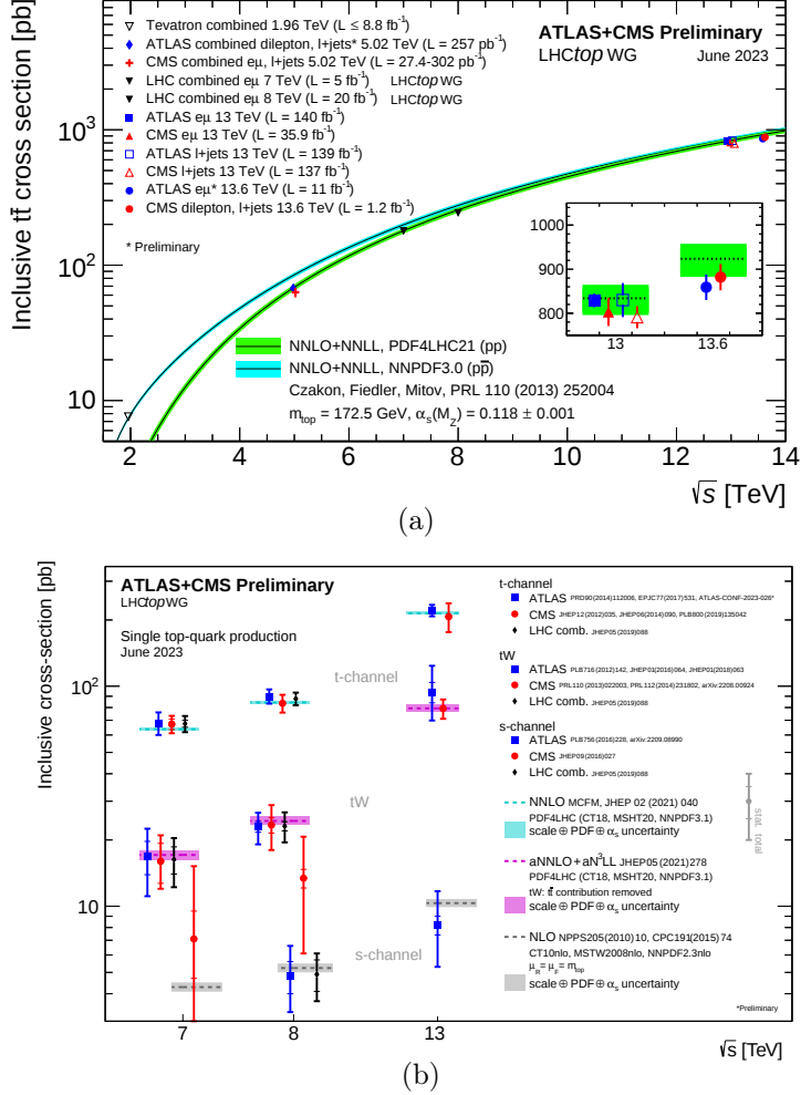
Figure 3.3: (a) Comparison of the measured t\bar{t} production cross-section as a function of the COM energy with the theoretical predictions at NNLO+NNLL accuracy. (b) Comparison of the measured single-top quark production cross-section for each channel, at different COM energies, with the theoretical predictions based on NLO, NLO+NNLL and NNLO ( t -channel only). In both, theory bands cover uncertainties due to renormalisation and factorisation scales, as well as those from parton density functions and the strong coupling. All calculations are done with m_t = 172.5 \text{ GeV} . Source: Ref. [158].
