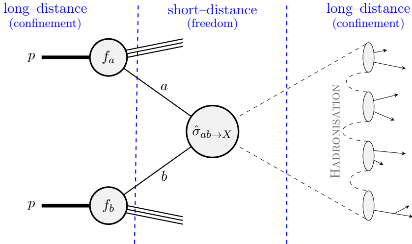
Figure 2.3: Schematic representation of a hard process in pp collisions.
