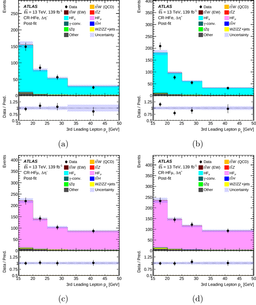
Figure 5.21: Comparison between data and the post-fit predictions in (a,b) CR-HF e and (c,d) CR-HF μ . The distributions show the p_T of the third lepton (electron or muon), which is the variable that is used for the binned likelihood fit. The regions are separated between |\Delta\eta_\ell^{\text{BDT}}| \leq 0 ( \Delta\eta^- ) and |\Delta\eta_\ell^{\text{BDT}}| > 0 ( \Delta\eta^+ ). The error bands include the total uncertainties in the post-fit predictions. The ratios of the data to the total post-fit predictions are shown in the lower panels. Events with the p_T of the third lepton above 50 GeV are included in the overflow bins.
