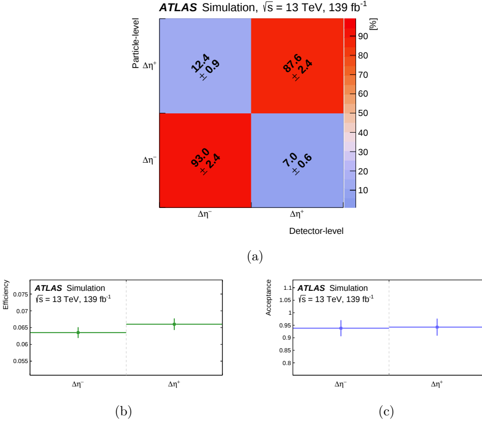
Figure G.1: (a) The migration matrix and (b) the efficiency and (c) the acceptance corrections that are used as input for the unfolding of SR-2b-high N_{\text{jets}} . The matrices are normalised such that the sum of any given row is 100%, although small differences may be present due to rounding. The error bars of the efficiency and acceptance correction terms represent the MC statistical uncertainties per bin based on the nominal t\bar{t}W SHERPA sample.
