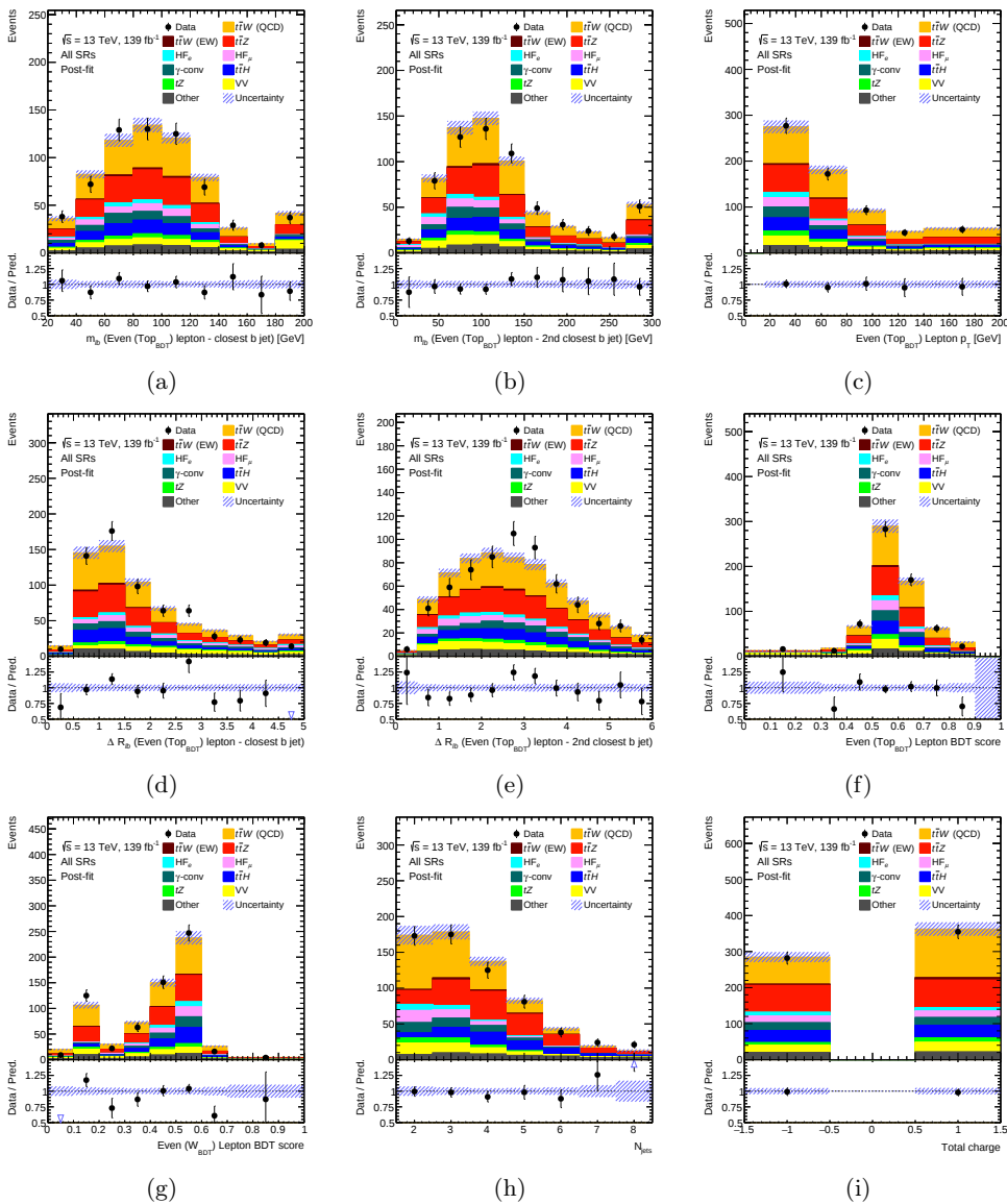
Figure 5.24: Comparison between data and the post-fit predictions, combining the four SRs, for the BDT input variables of the selected even lepton: (a) m_{\ell b_0} , (b) m_{\ell b_1} , (c) lepton p_T , (d) \Delta R_{\ell b_0} , (e) \Delta R_{\ell b_1} . Then, BDT discriminator values for the two even leptons: (f) selected lepton, (g) background lepton. Finally, (h) N_{\text{jets}} and (i) total charge of the leptons. The error band includes the total uncertainties of the post-fit predictions. The ratio of the data to the total post-fit predictions is shown in the lower panel.
