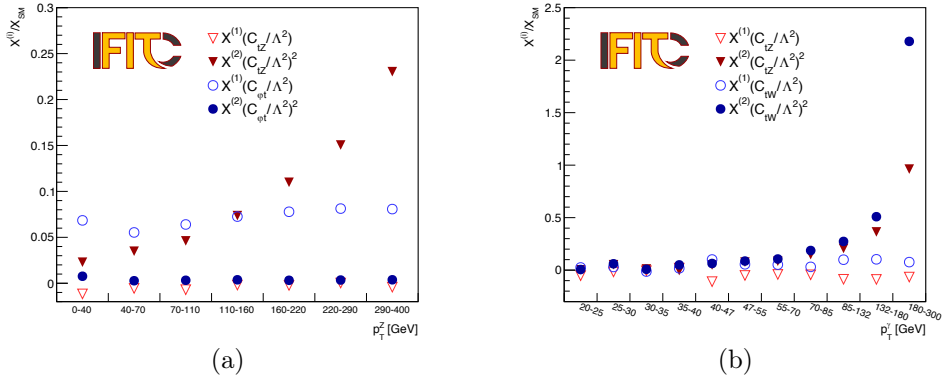
Figure 4.4: Linear (empty markers) and quadratic (filled markers) parameterisations for each of the bins in the differential (a) t\bar{t}Z and (b) t\bar{t}\gamma cross-sections. The most sensitive operators to these processes ( C_{tZ} , C_{\phi t} and C_{tW} ) are shown.
