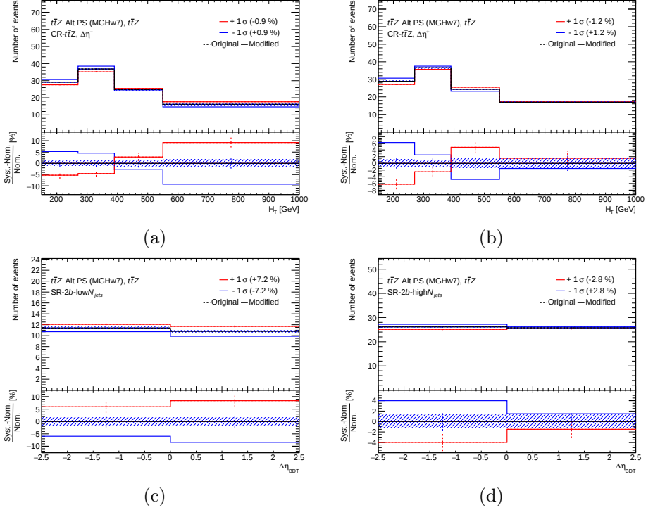
Figure D.1: Alternative t\bar{t}Z PS modelling for (a) CR- t\bar{t}Z \Delta\eta^- , (b) CR- t\bar{t}Z \Delta\eta^+ , (c) SR-2b-low N_{\text{jets}} , and (d) SR-2b-high N_{\text{jets}} . Uncertainty bands cover MC statistical uncertainties of the nominal sample.
