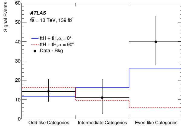
Figure 6.6: Signal yields to with the \mathcal{CP} -even (blue) and the \mathcal{CP} -odd (red) hypothesis compared to data. The data is shown with fitted background subtracted and the error bars includes the statistical uncertainty. The three categories (Odd-like, Intermediate and Even-like) are labelled corresponding to the CP BDT score ranges that they cover. In the last bin, the SM \mathcal{CP} -even coupling is favoured.
