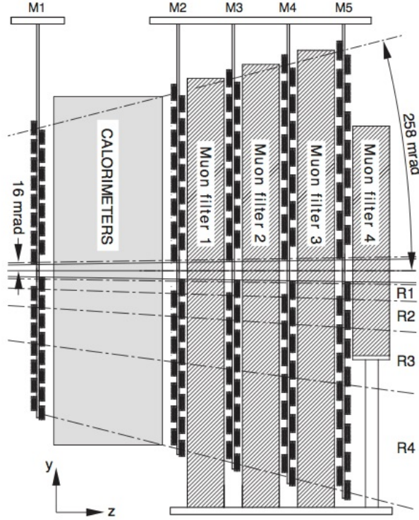
Figure 3.15: Side view of the muon system. Figure taken from Ref. [147].
