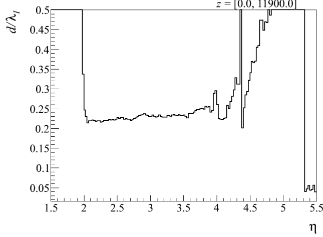
Figure 4.3: Material thickness of the LHCb detector until the end of the RICH2 detector as a function of pseudorapidity, for a particle produced in the nominal pp interaction point and unbent by the magnetic field. The thickness is quantified in interaction-lengths units and is averaged over the azimuthal angle \phi . The peak at \eta = 4.38 , corresponding to a polar angle of 25 mrad, is due to the conical beam pipe inside the RICH1 detector [163]. Figure taken from Ref. [162].
