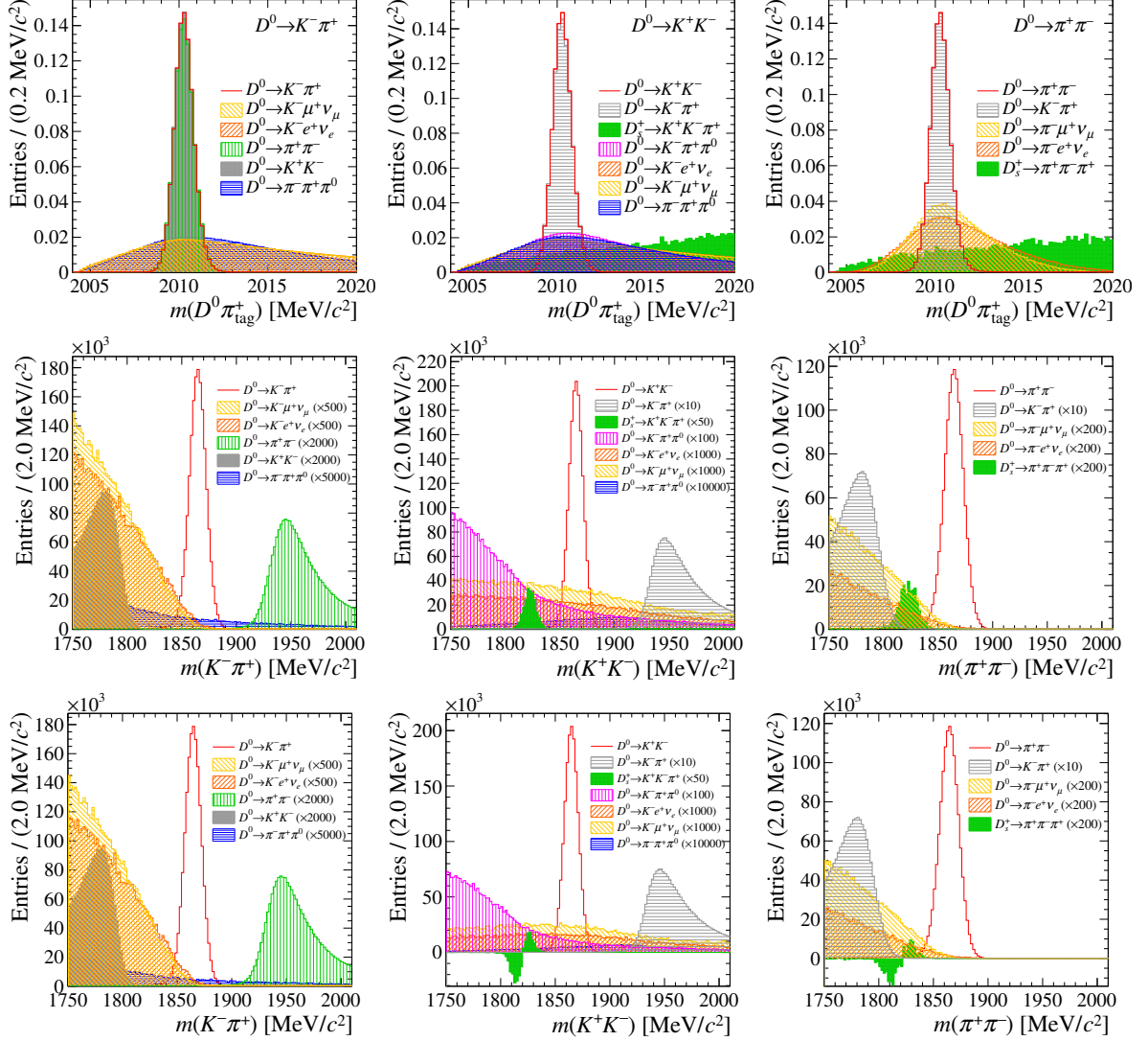
Figure 7.8: RAPIDSIM distributions of (top) m(D^0\pi_{\text{tag}}^+) , (centre) m(h^+h^-) of the candidates in the m(D^0\pi_{\text{tag}}^+) signal window and (bottom) m(h^+h^-) of the selected candidates after the removal of the m(D^0\pi_{\text{tag}}^+) background, for all signal and background decays listed in Table 7.3. For the m(h^+h^-) plots, the normalisations relative to the signal component are shown in the legend, using the D_s^{*-} -to- D^{*+} cross-section ratio from Ref. [126]. Left, centre and right plots correspond to the K^-\pi^+ , K^+K^- and \pi^+\pi^- decay channels.
