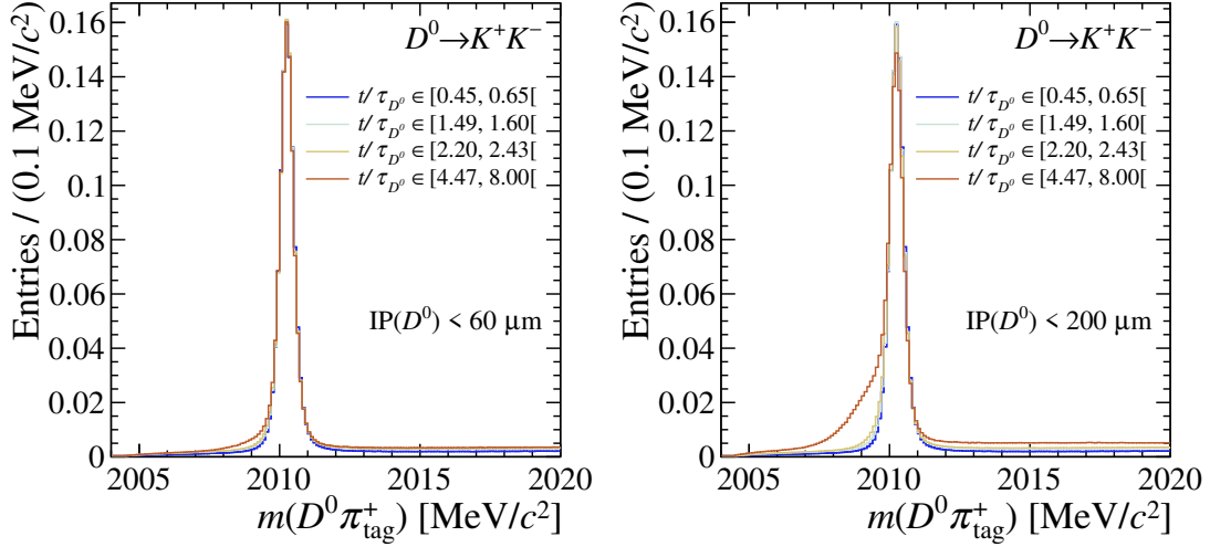
Figure 6.3: Distributions of m(D^0\pi_{\text{tag}}^+) with (left) the baseline and (right) a looser requirement on the \text{IP}(D^0) , for the 0 th , 10 th , 15 th and 20 th bins of decay time. The tail on the left of the m(D^{*+}) peak at large decay times is due to secondary decays.
