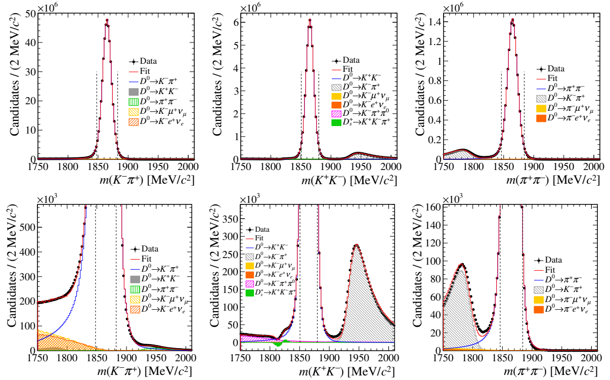
Figure 7.13: Nominal template fit to the time and flavour integrated m(h^+h^-) distributions of (left) K^-\pi^+ , (centre) K^+K^- and (right) \pi^+\pi^- decays. Bottom plots are magnified to put the background components in evidence.
