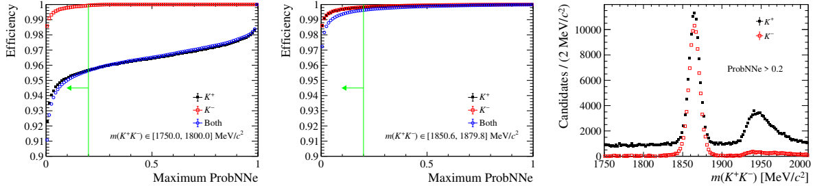
Figure E.2: Selection efficiency of the requirement \text{ProbNNe}(K^\pm) < 0.2 for the candidates in the (left) m(K^+K^-) \in [1750, 1800] \text{ MeV}/c^2 lateral window and (centre) signal window. The green vertical lines indicate the baseline requirement. (Right) m(K^+K^-) distribution of the candidates rejected by the \text{ProbNNe}(K^\pm) < 0.2 requirement.
