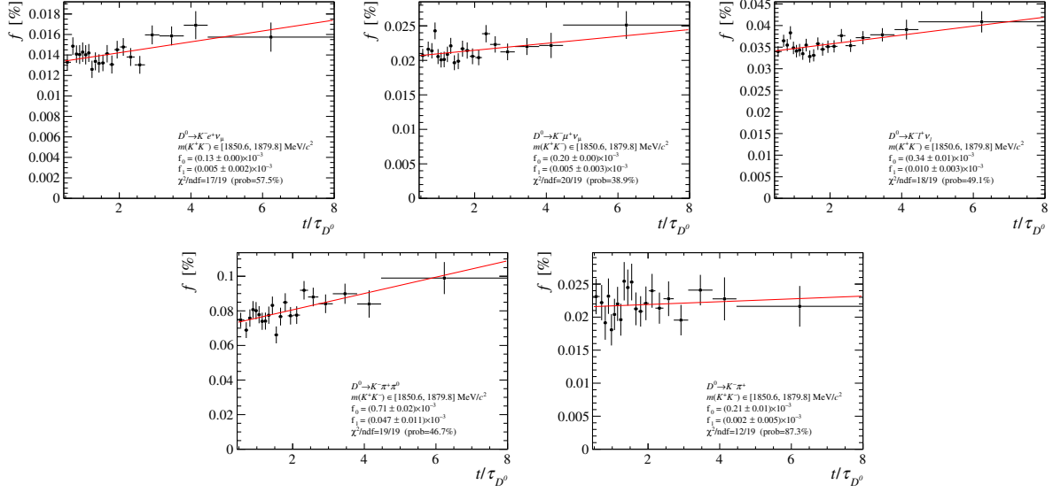
Figure E.7: Linear fit to the time-dependent fraction of background candidates in the m(K^+K^-) signal region, for all relevant backgrounds components.
