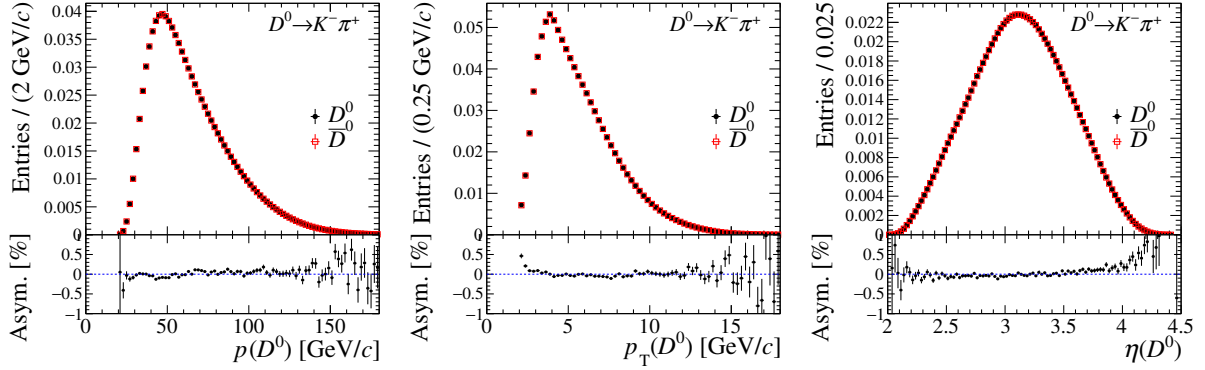
Figure 5.5: Residual asymmetries of the D^0 momentum, transverse momentum and pseudorapidity, after the weighting of the vector-momentum distribution of the \pi_{\text{tag}}^\pm mesons.
