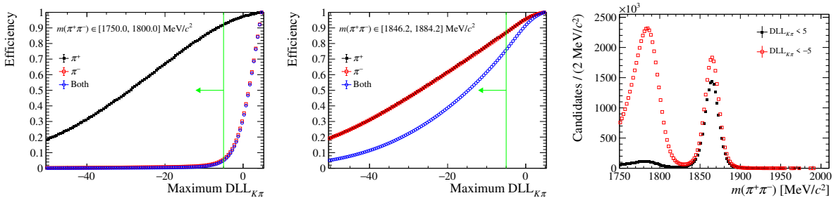
Figure E.1: Selection efficiency of the requirement \text{DLL}_{K\pi}(\pi^\pm) < -5 , normalised to that of the requirement \text{DLL}_{K\pi}(\pi^\pm) < 5 which is implemented at the trigger level, for candidates in the (left) m(\pi^+\pi^-) \in [1750, 1800] \text{ MeV}/c^2 lateral window and (centre) signal window. The green vertical lines indicate the baseline requirement. (Right) m(\pi^+\pi^-) distribution of the candidates before and after the \text{DLL}_{K\pi}(\pi^\pm) < -5 requirement.
