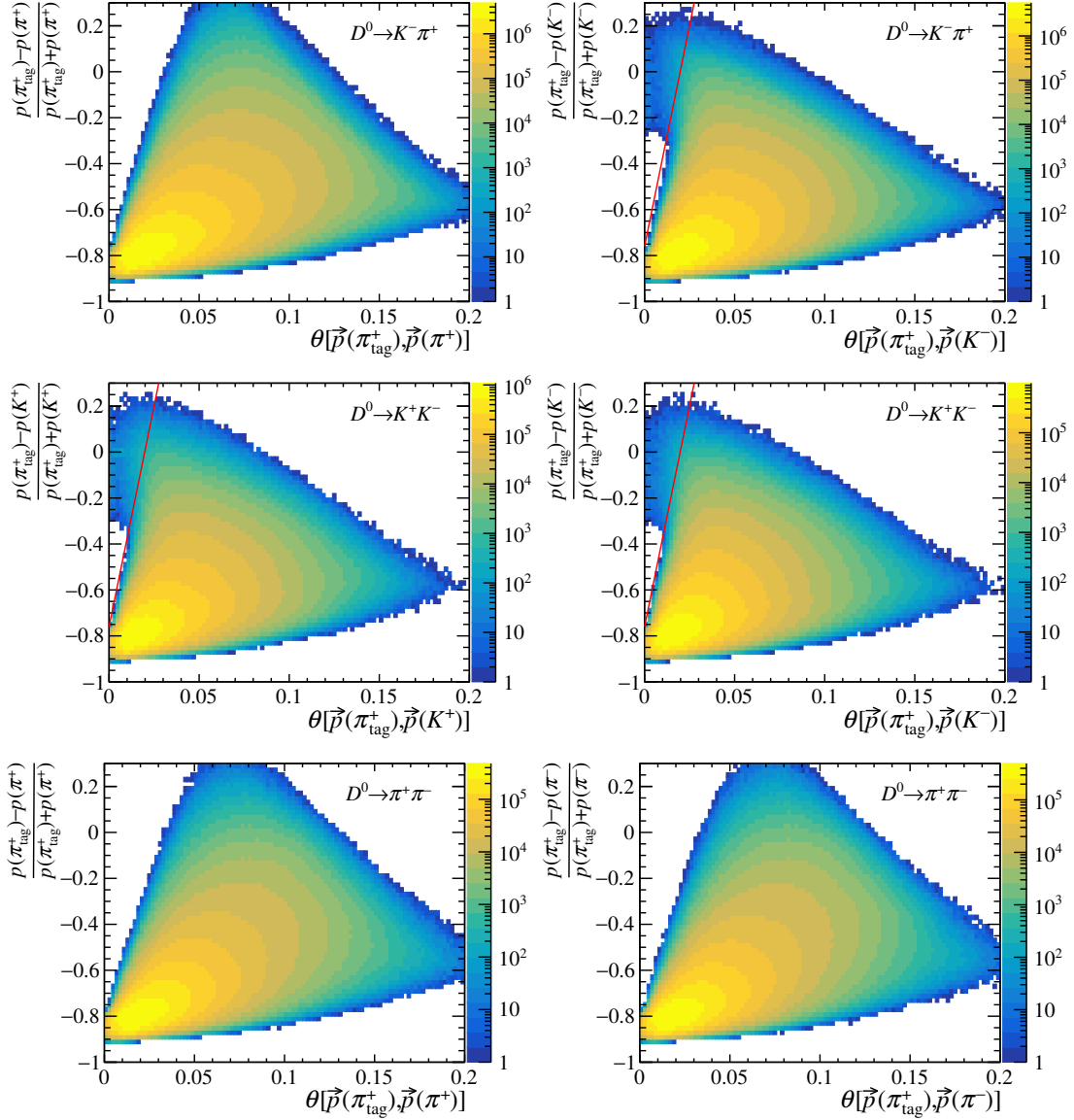
Figure 4.5: Asymmetry and angle between the momenta of one of the D^0 final-state hadrons and the \pi^+_{\text{tag}} meson for (top) D^0 \rightarrow K^- \pi^+ , (centre) D^0 \rightarrow K^+ K^- and (bottom) D^0 \rightarrow \pi^+ \pi^- decays. The requirement of Eq. (4.3), which rejects the clones concentrated near the point (0,0), is displayed wherever applied.
