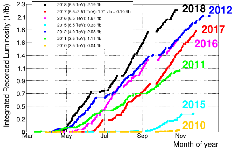
Figure 3.1: Integrated luminosity of pp collisions recorded by the LHCb experiment in each data-taking year. The beam energy, corresponding to half of the centre-of-mass energy \sqrt{s} , is reported as well.
