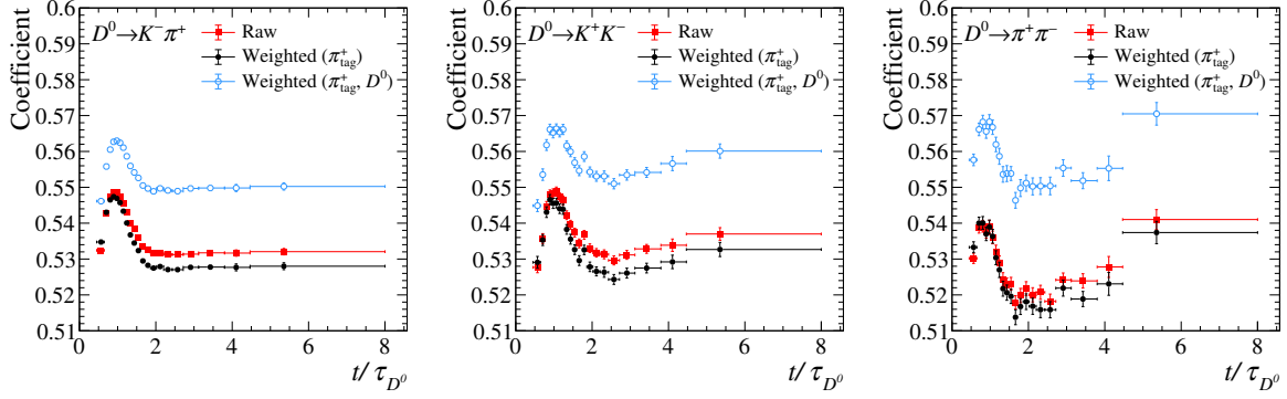
Figure D.4: Absolute value of the coefficient used in the subtraction of the m(D^0\pi^+) background described in Sect. 4.3, for raw data and after each of the two steps of the kinematic weighting, for the (left) K^-\pi^+ , (centre) K^+K^- and (right) \pi^+\pi^- decay channels.
