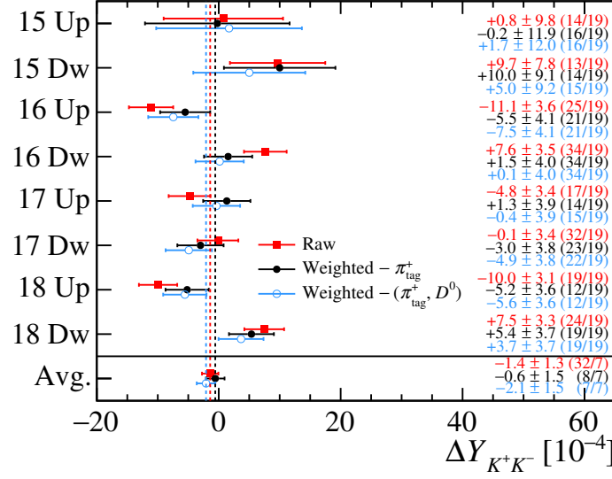
Figure 5.11: Summary of the fitted values of \Delta Y_{K^+K^-} in the eight subsamples divided according to the year and magnet polarity, together with their average. The numerical values of \Delta Y_{K^+K^-} and the \chi^2/\text{ndf} of the fits are reported on the right. The global p-values of the eight linear fits to the time-dependent asymmetry are 7.4%, 42% and 41% for raw data and after the first and second steps of the kinematic weighting, respectively, whereas the p-values of the average of \Delta Y_{K^+K^-} are 4 \times 10^{-5} , 33% and 45%, respectively.
