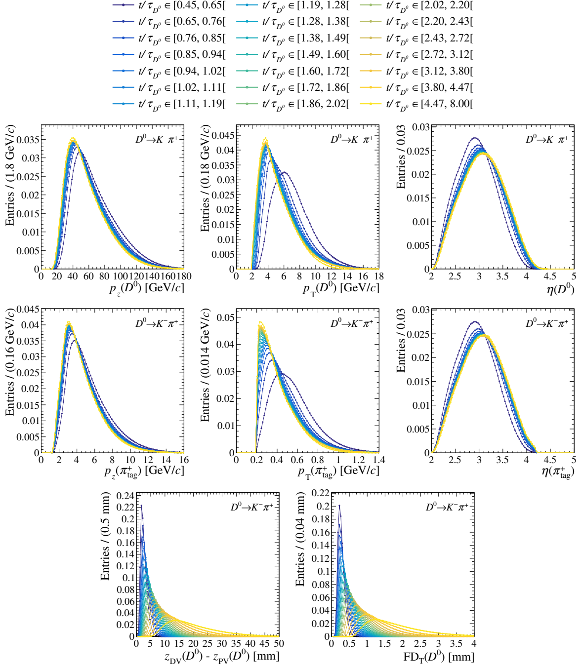
Figure 5.3: Normalised distributions of the z and transverse components and of the pseudorapidity of the D^0 - and \pi^+_{tag} momentum, and of the z and transverse components of the D^0 flight distance, in different colours for different decay-time bins.
