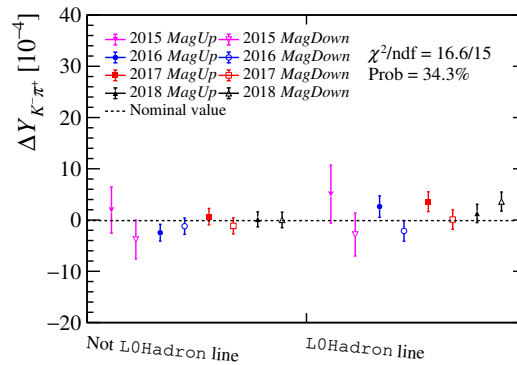
Figure 8.7: Measurements of \Delta Y_{K^-\pi^+} performed separately in the subsample where the L0 hadronic trigger line is fired by the D^0 candidate and in its complimentary (and, for each of them, separately for different data-taking years and magnet polarities). The weights are calculated independently for each subsample. The p-value of the dispersion of the measurements around the baseline one is displayed as well.
