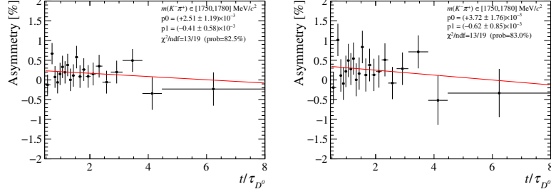
Figure E.10: Linear fit to the time-dependent asymmetry (left) in the m(K^-\pi^+) \in [1750, 1780] \text{ MeV}/c^2 window and (right) of the D^0 \rightarrow K^-\ell^+\nu_\ell background, calculated by dividing the asymmetry by the D^0 \rightarrow K^-\ell^+\nu_\ell fraction in the corresponding window.
