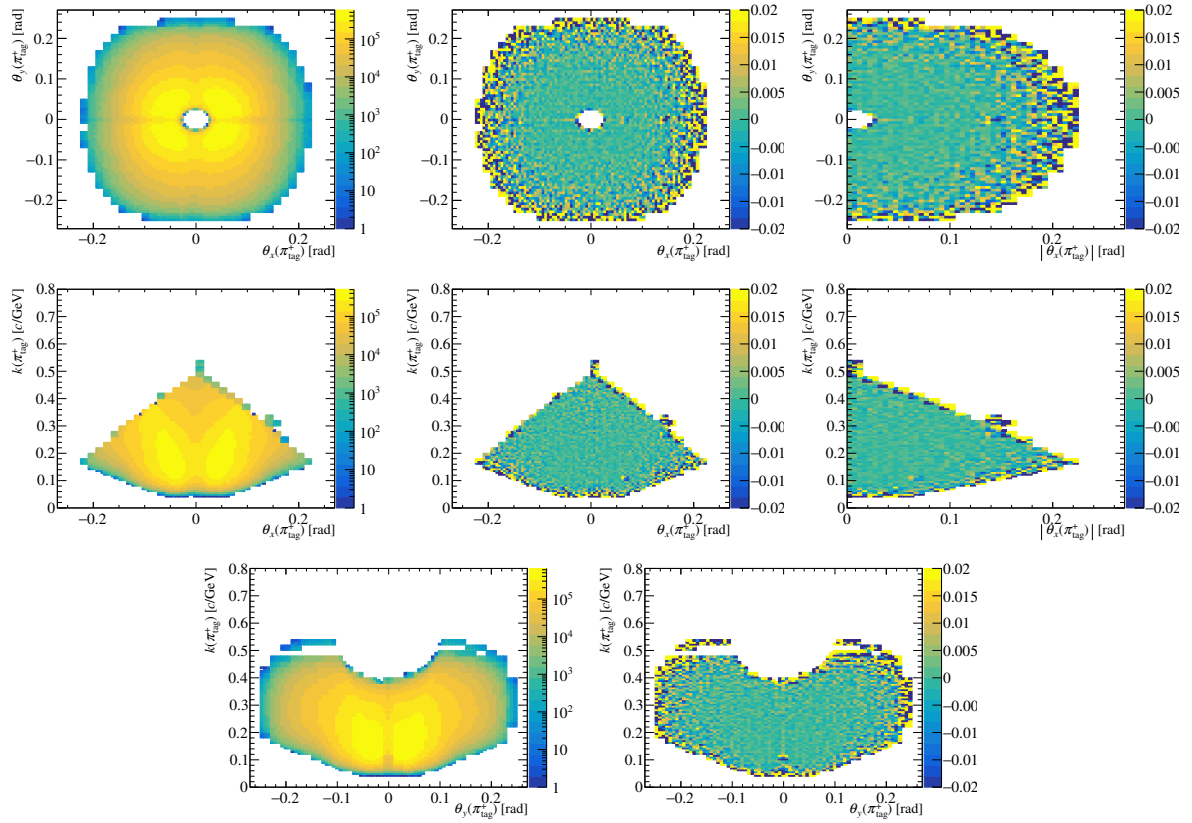
Figure D.9: Two-dimensional distributions and asymmetries of the vector momentum of the \pi^+_{\text{tag}} meson, for the full D^0 \rightarrow K^- \pi^+ data sample.
