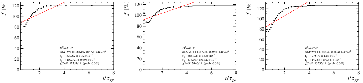
Figure E.9: Linear fit to the time-dependent fraction of signal candidates in the m(h^+h^-) signal region, for the (left) K^- \pi^+ , (centre) K^+ K^- and (right) \pi^+ \pi^- decay channels. The fractions are calculated as the ratio of the RAPIDSIM template (with the normalisation taken from the results of the template fit of Sect. 7.5) to the data.
