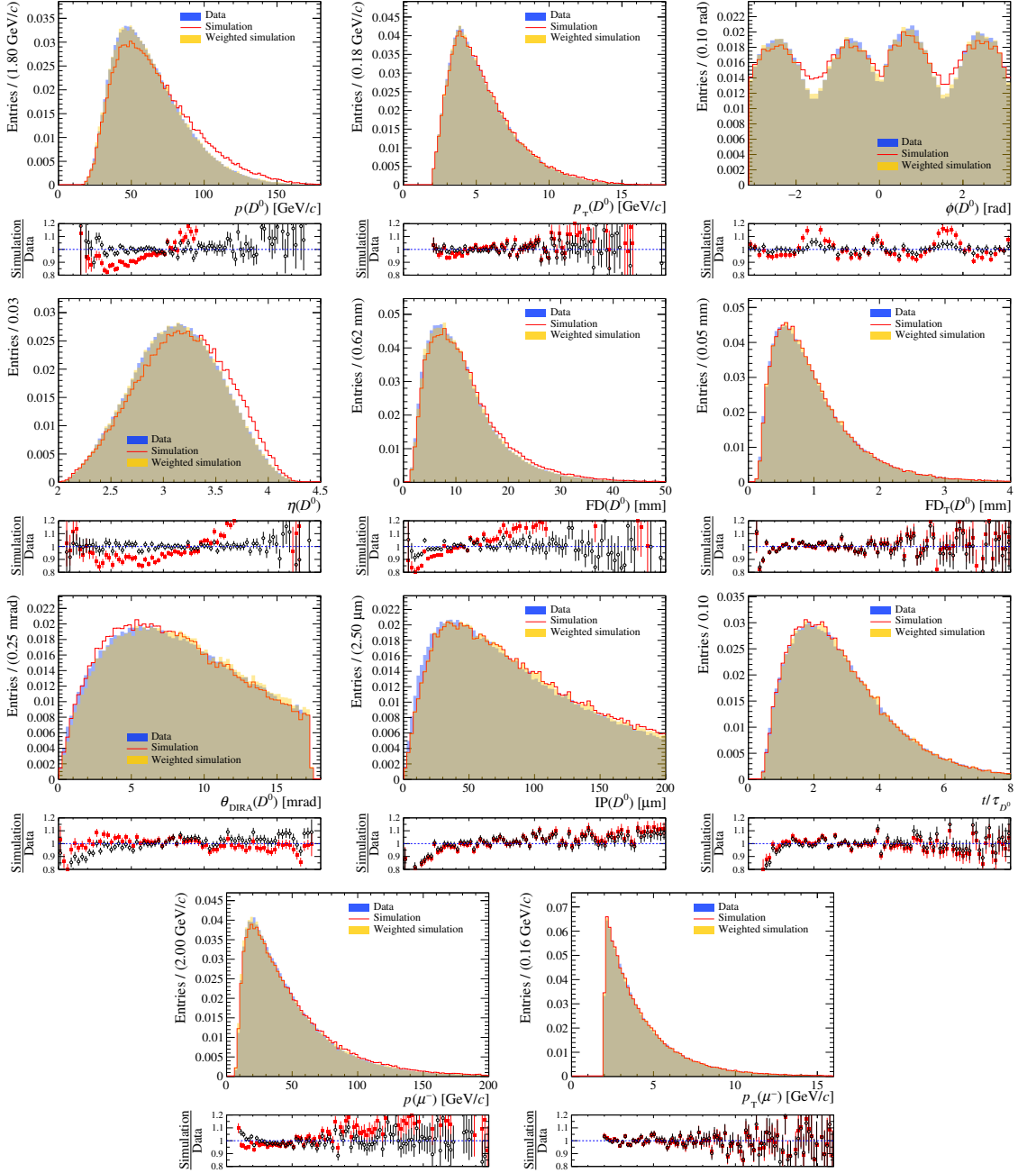
Figure 4.14: Comparison between the kinematic distributions of D^{*+}\mu^- secondary candidates in data and simulation, both before and after the three-dimensional ( p_T, \eta, \phi ) weighting of the D^0 momentum. The data sample of secondary decays is selected using 1/6 of the candidates satisfying the requirement \text{IP}(D^0) < 200 \mu\text{m} . In the plots displaying the ratio of simulated to real data, full red squares (open black circles) correspond to simulated data before (after) the weighting.
