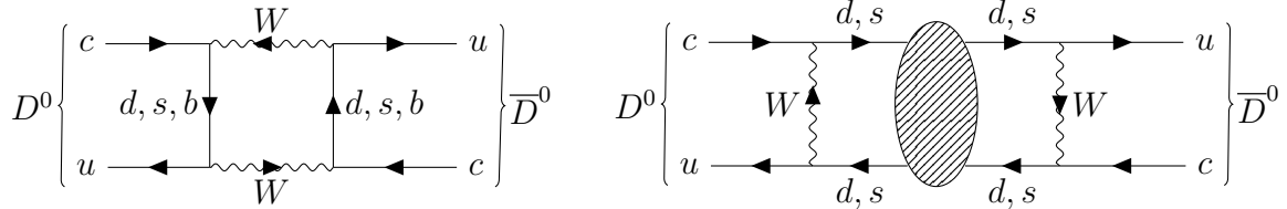
Figure 1.4: Feynman diagrams of (left) short-distance and (right) long-distance contributions to D^0 mixing. In the right diagram, the blob stands for low-energy QCD interactions, possibly involving the exchange of hadrons on the mass shell.
