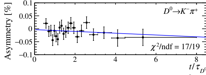
Figure 6.12: Linear fit to the time-dependent asymmetry of the full D^0 \rightarrow K^- \pi^+ sample after the kinematic weighting and the subtraction of the contribution of secondary decays to the asymmetry.
