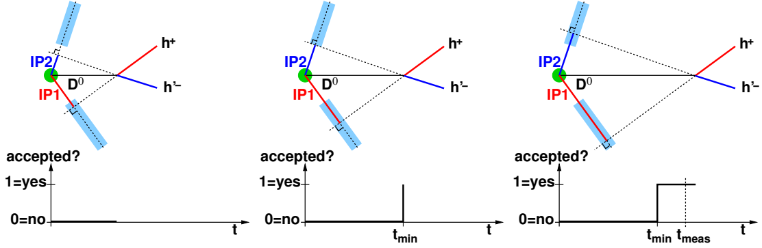
Figure 2.1: Evolution of the decay-time acceptance for a D^0 \rightarrow h^+ h^- decay when moving the pp vertex along the D^0 momentum vector. The trigger requires the impact parameter of the hadron tracks with respect to the pp vertex to be larger than a fixed value. The shaded light-blue regions show the bands for accepting a track impact parameter. While the impact parameter of the negative track (IP2) is too low in the left plot, it reaches the accepted range in the central one. The actual measured decay time, t_{\text{meas}} , lies in the accepted region, which continues to larger decay times (right plot). Figure taken from Ref. [113].
