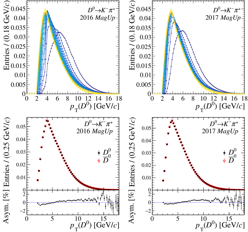
Figure 5.4: (Top) Normalised distributions of the D^0 transverse momentum, in different colours for each decay time bin. Blue (yellow) colours correspond to lower (higher) decay times. (Bottom) Asymmetry of the normalised p_T distributions of D^0 and \bar{D}^0 mesons. All plots correspond to the D^0 \rightarrow K^- \pi^+ sample, collected during (left) 2016 and (right) 2017 with the MagUp polarity.
