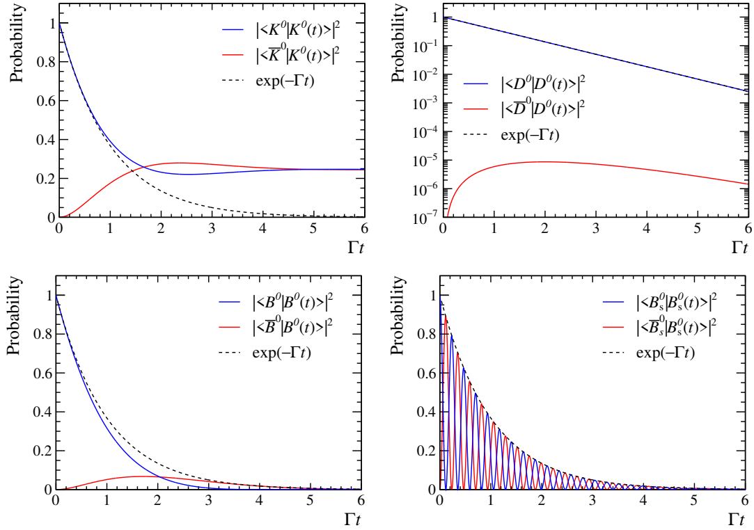
Figure 1.3: Probability for a neutral flavoured meson to oscillate in its relative antimeson (red) or to preserve its flavour quantum numbers (blue) as a function of time, under the assumption that |q/p| = 1 . The plots correspond, from left to right and from top to bottom, to K^0 , D^0 (in logarithmic scale), B^0 and B_s^0 mesons. The exponential function that would be measured in absence of mixing is drawn as well as a black-dashed line.
