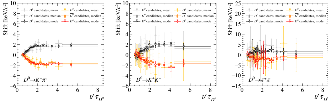
Figure 7.1: Shift of the m(D^0\pi^+_{\text{tag}}) signal distribution of D^{*+} and D^{*-} candidates as a function of D^0 decay time for the (left) K^-\pi^+ , (centre) K^+K^- and (right) \pi^+\pi^- decay channels. The shift is estimated as the difference of the mean, median and mode of the D^{*+} ( D^{*-} ) signal PDF, as obtained in the fits described in Sect. 4.3, and the corresponding values obtained in the fit to the D^{*+} and D^{*-} candidates combined. In both fits the whole, kinematically weighted data sample is employed. Note that the range of the y axis for the \pi^+\pi^- decay channel is different from the others.
