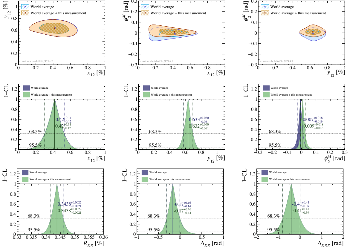
Figure B.1: Impact of the present measurement of \Delta Y on the knowledge of the parameters quantifying mixing and time-dependent CP violation in D^0 mesons, in the superweak approximation. The fit has a \chi^2/\text{nfd} equal to 58/44, corresponding to a p-value of 8%.
