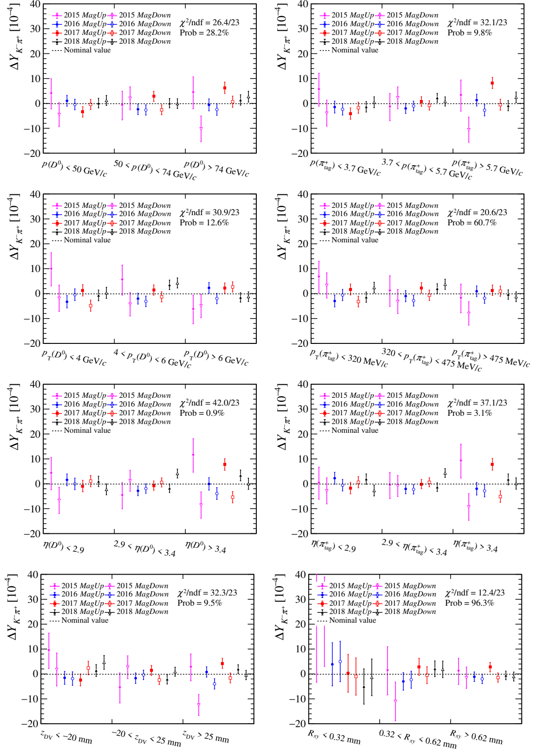
Figure 8.1: Measurements of \Delta Y_{K^- \pi^+} performed separately in three bins of the momentum, transverse momentum and pseudorapidity of the D^0 and \pi_{\text{tag}}^+ mesons and of the position of the D^0 decay vertex along the beam direction and in the plane transverse to it. Each of these bins is further divided in eight subsamples corresponding to different data-taking years and magnet polarities. The p-value of the dispersion of the measurements around the baseline one is displayed as well.
