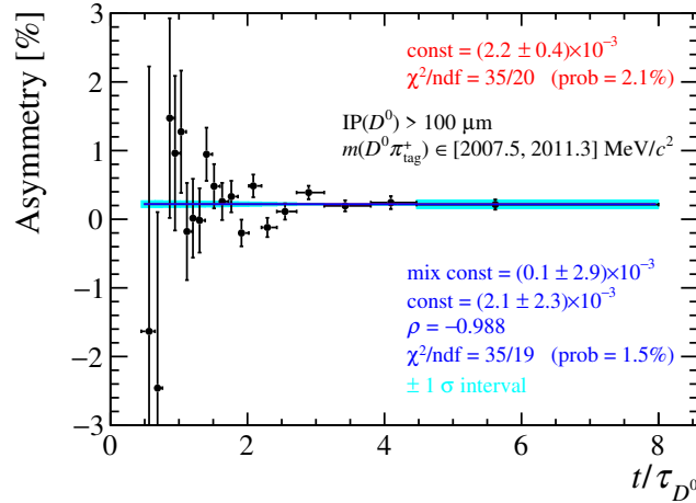
Figure 6.11: Asymmetry of D^0 \rightarrow K^- \pi^+ candidates with \text{IP}(D^0) > 100 \mu\text{m} in the enlarged signal region m(D^0 \pi_{\text{tag}}^+) \in [2007.5, 2011.3] \text{ MeV}/c^2 , after the kinematic weighting of Sect. 5.2. The fits with a constant function and a constant plus the cyan template from Fig. 6.9 (right), which overlap nearly perfectly, are superimposed. The cyan band represents the 1\sigma confidence interval of the results of the fit modelling the B^0 mixing.
