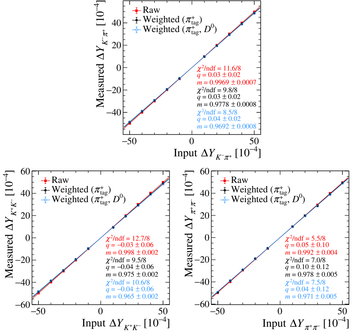
Figure 5.14: Measured value of (top) \Delta Y_{K^- \pi^+} (bottom left) \Delta Y_{K^+ K^-} and (bottom right) \Delta Y_{\pi^+ \pi^-} as a function of the time-dependent asymmetry \Delta Y_f^{\text{inj}} injected into the data sample. In each plot, the result obtained for \Delta Y_f^{\text{inj}} = 0 is subtracted from all the other points.
