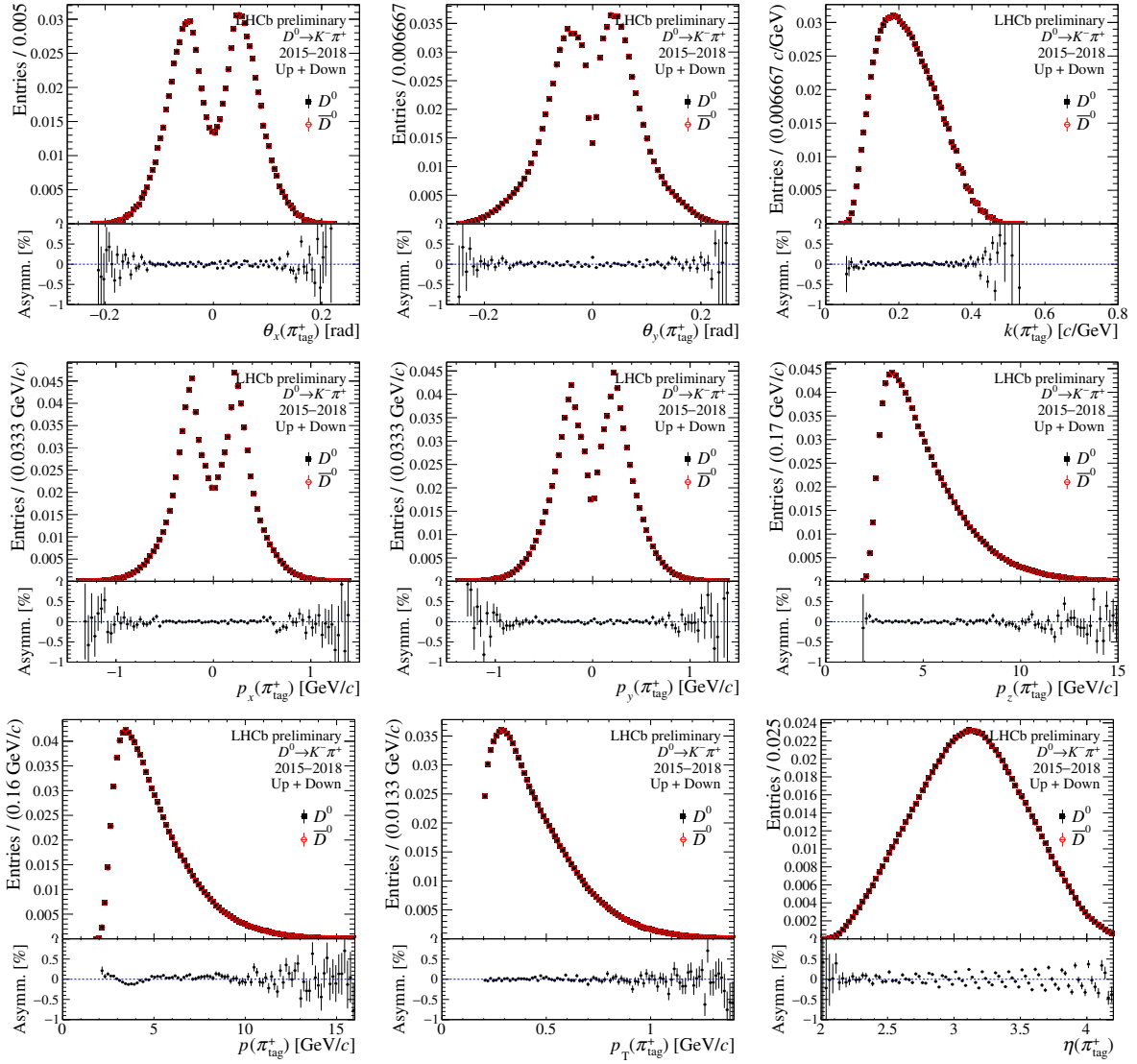
Figure D.10: Distributions and asymmetries of the momentum of the \pi^+ tag meson for the full D^0 \rightarrow K^- \pi^+ data sample.
