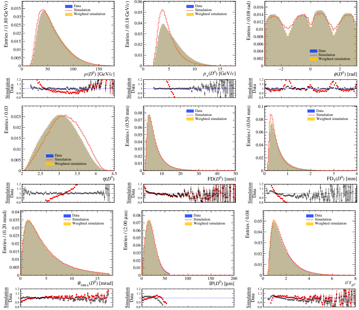
Figure 4.12: Comparison between the kinematic distributions of D^0 \rightarrow K^- \pi^+ primary decays in data and simulation, both before and after the three-dimensional ( p_T, \eta, \phi ) weighting of the D^0 momentum. The data sample of primary decays is selected using 1/150 of the candidates satisfying the requirement \text{IP}(D^0) < 60 \mu\text{m} . In the plots displaying the ratio of simulated to real data, full red squares (open black circles) correspond to simulated data before (after) the weighting.
