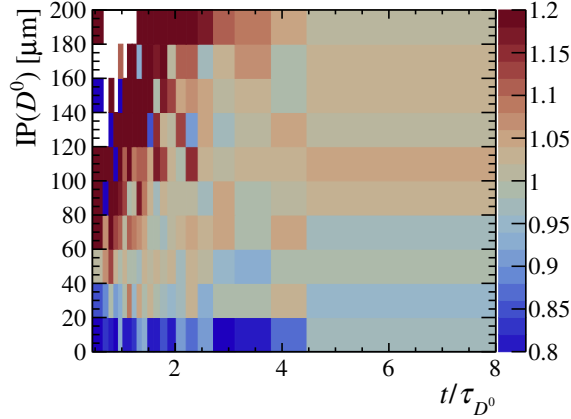
Figure 7.5: Ratio between the \text{IP}(D^0) vs. t(D^0) normalised distributions of simulation to data of D^{*+}\mu^- pairs.
