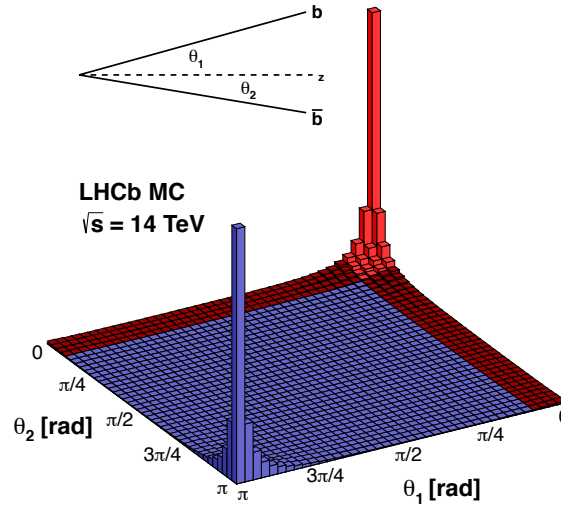
Figure 3.2: Production cross-section of b\bar{b} pairs as a function of their polar angle with respect to the beam axis, for pp collisions simulated with PYTHIA [145] at a centre-of-mass energy of 14 TeV. The LHCb acceptance is displayed in red. The plot is taken from Ref. [146].
