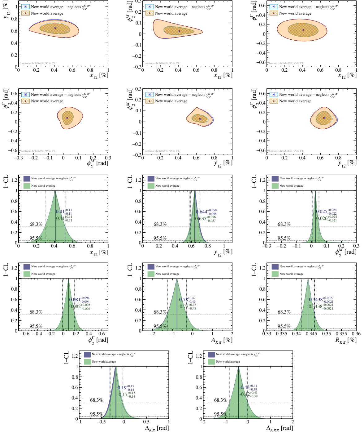
Figure B.4: Impact of neglecting the contribution of y_{CP}^{K^-\pi^+} in the measurement of the y_{CP} parameter on the knowledge of the parameters quantifying mixing and time-dependent CP violation in D^0 decays, in the theoretical parametrisation. The fits employ all the measurements listed in Table B.1.
