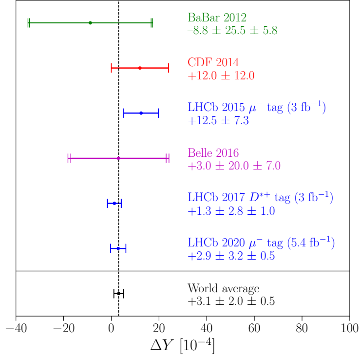
Figure 2.2: Summary of the most precise measurements of the parameter \Delta Y to date (final-state dependent contributions are neglected). Measurements references, from top to bottom: BaBar 2012 [62], CDF 2014 [117], LHCb 2015 \mu^- tag [118], Belle 2016 [64], LHCb 2017 D^{*+} tag [116], LHCb 2020 \mu^- tag [120]. The LHCb 2015 \mu^- tag and LHCb 2017 D^{*+} tag measurements employ the data collected during 2011–2012, while the LHCb 2020 \mu^- tag employs the data collected during 2016–2018. All of the other experiments employ the data sample collected during their whole lifetime.
