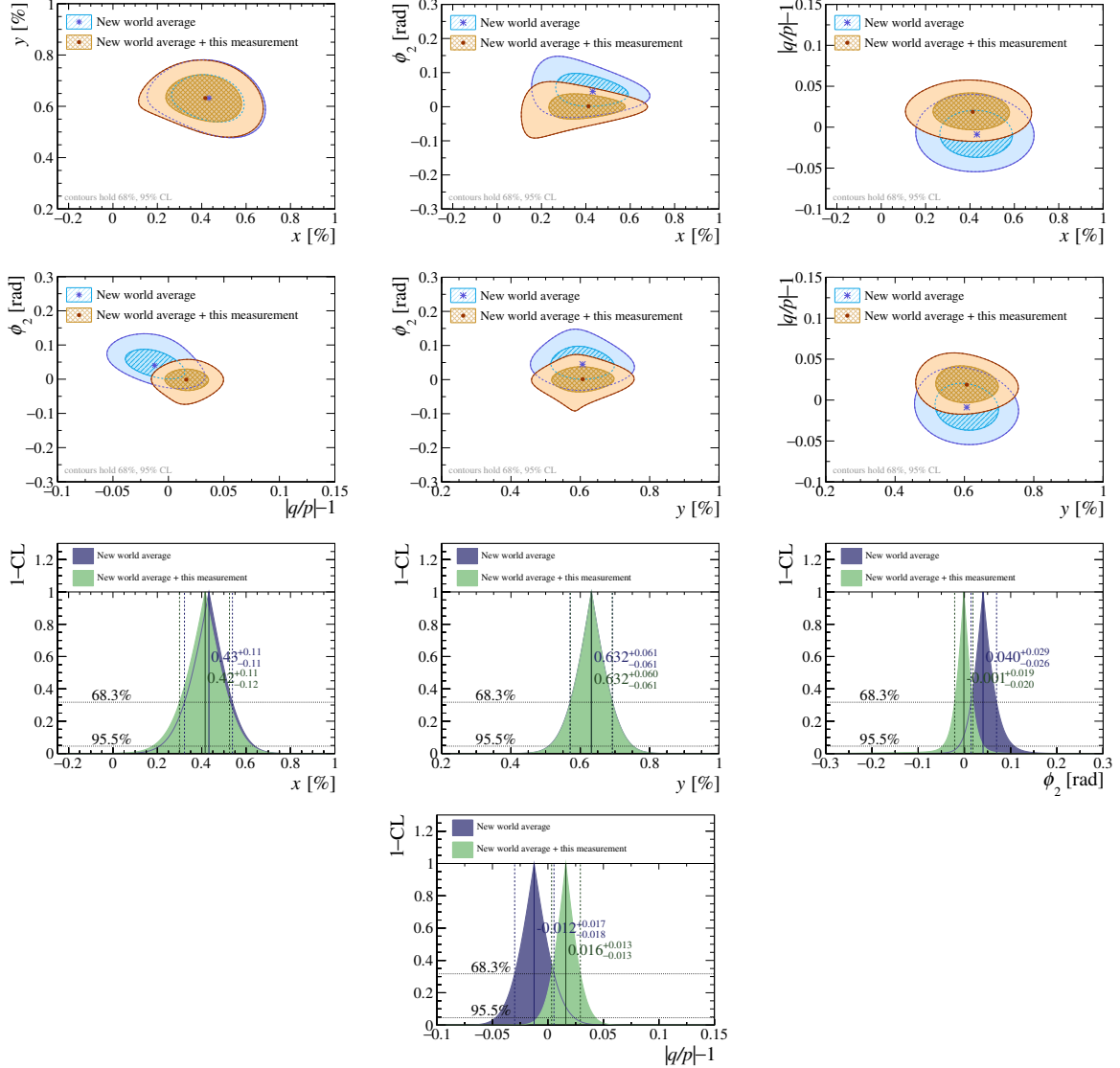
Figure B.2: Impact of the present measurement of \Delta Y on the knowledge of the parameters quantifying mixing and time-dependent CP violation in D^0 mesons, in the phenomenological approximation. The results for the parameters A_{K\pi} , R_{K\pi} , \Delta_{K\pi} and \Delta_{K\pi\pi} are the same as in Fig. 9.3. The fit has a \chi^2/\text{ndf} equal to 56/42, corresponding to a p-value of 8%.
