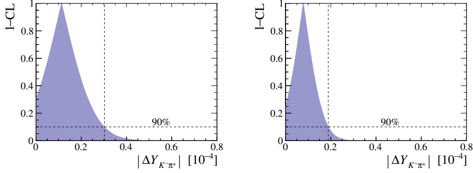
Figure B.3: Lower confidence interval on the absolute value of \Delta Y_{K^- \pi^+} , obtained with all measurements in Table B.1, (left) except and (right) including the one presented in this thesis.
