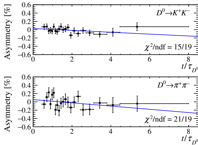
Figure 9.1: Linear fit to the time-dependent asymmetry of (top) D^0 \rightarrow K^+ K^- and (bottom) D^0 \rightarrow \pi^+ \pi^- candidates.
