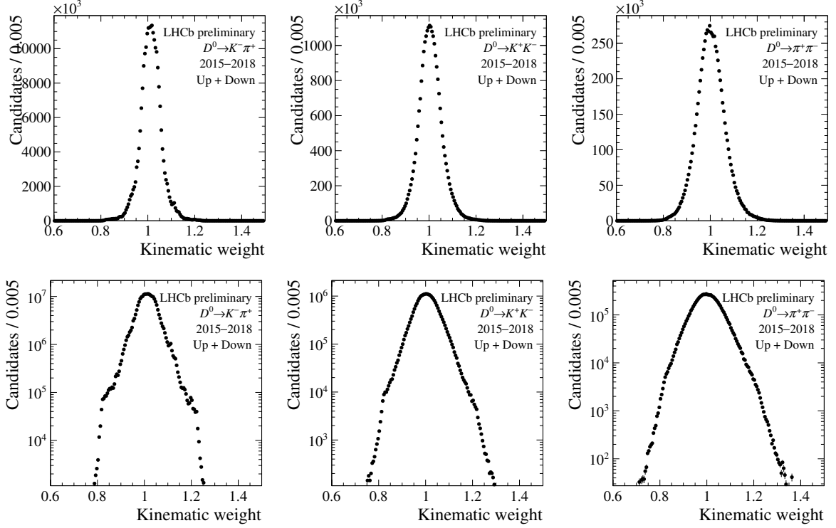
Figure D.2: Distribution of the weights of the kinematic equalisation of Sect. 5.2 for the (left) K^- \pi^+ , (centre) K^+ K^- and (right) \pi^+ \pi^- decay channels, in (top) linear and (bottom) logarithmic scale.
