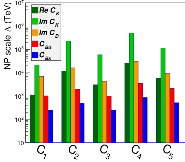
Figure 1.5: Summary of the 95% probability lower bound on the scale of new-physics (NP) interactions beyond the SM, \Lambda , for strongly interacting NP. Results from all of the neutral meson systems are shown. Figure taken from Ref. [17].
