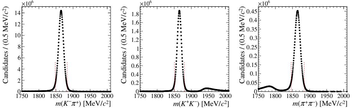
Figure 4.9: Distribution of m(h^+h^-) after the subtraction of the m(D^0\pi_{\text{tag}}^+) background for the (left) D^0 \rightarrow K^-\pi^+ , (centre) D^0 \rightarrow K^+K^- and (right) D^0 \rightarrow \pi^+\pi^- samples. The signal window is delimited by the vertical dashed lines.
