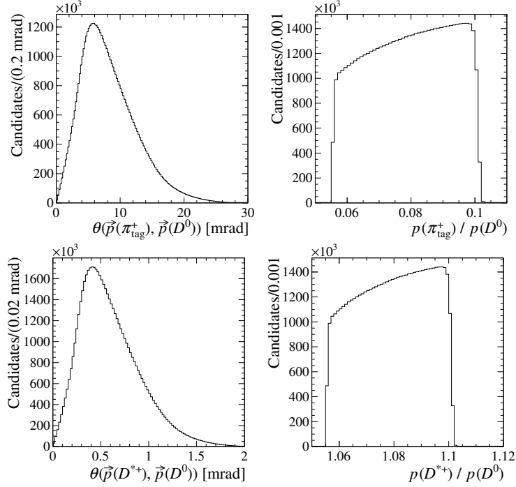
Figure 5.2: Distributions of the (left) angle and (right) ratio between the momenta of the (top) \pi_{\text{tag}}^+ and D^0 mesons and (bottom) D^{*+} and D^0 mesons.
