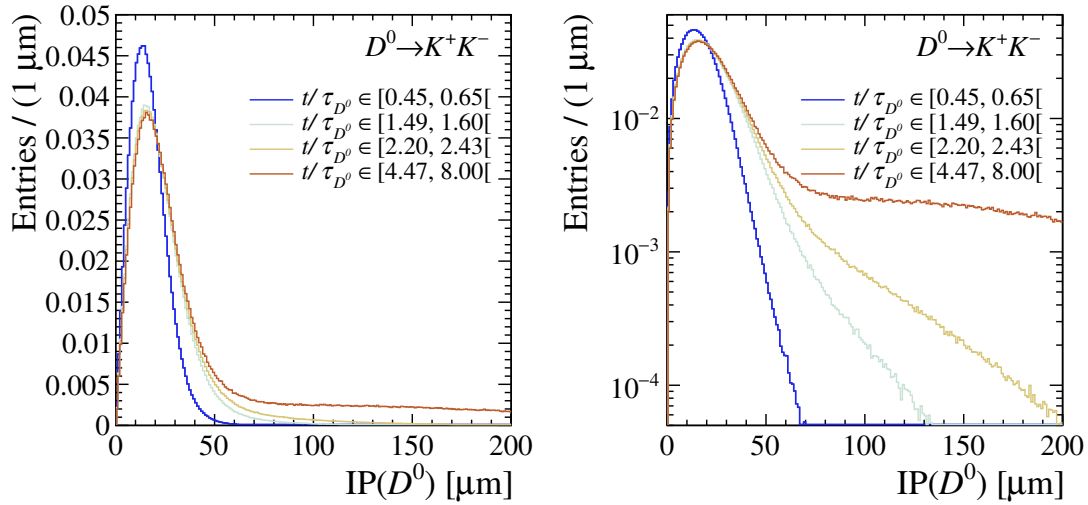
Figure 6.2: Distributions of the D^0 IP in (left) linear and (right) logarithmic scale, for the 0 th , 10 th , 15 th and 20 th bins of decay time. The long tails of the distributions at high decay times are due to secondary decays.
