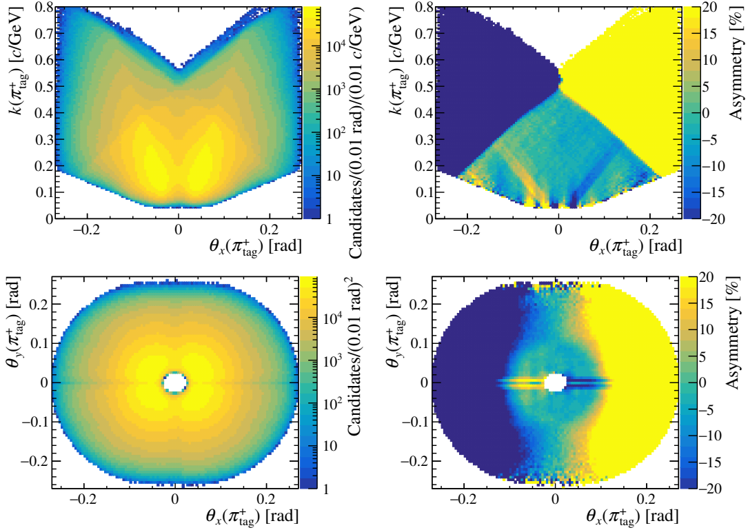
Figure 5.1: (Left) sum and (right) asymmetry of the distributions of \pi_{\text{tag}}^+ and \pi_{\text{tag}}^- candidates, in the (top) k vs. \theta_x and (bottom) \theta_y vs. \theta_x planes, for the D^0 \rightarrow K^- \pi^+ sample recorded during 2017 with the MagUp polarity. The angle \theta_{x(y)} \equiv \arctan(p_{x(y)}/p_z) is the emission angle of the \pi_{\text{tag}}^+ meson in the bending (vertical) plane, and k \equiv 1/\sqrt{p_x^2 + p_z^2} is proportional to its curvature in the magnetic field. The asymmetries during other data-taking years are similar, and opposite in sign for the data collected with the MagDown polarity. Regions of the distributions with asymmetries whose magnitude is larger than 20% are plotted with the same colour as \pm 20\% . These regions are discarded from the data sample after the kinematic weighting.
