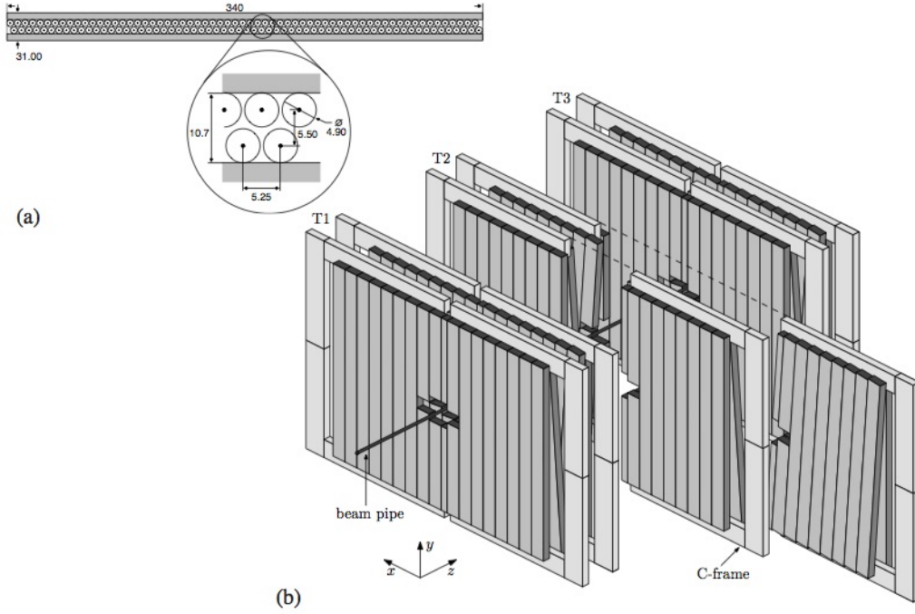
Figure 3.10: (a) Section of an OT detection plane. (b) Arrangement of OT straw-tubes modules in planes and stations. The second station is partially opened. Figures taken from Ref. [150].
