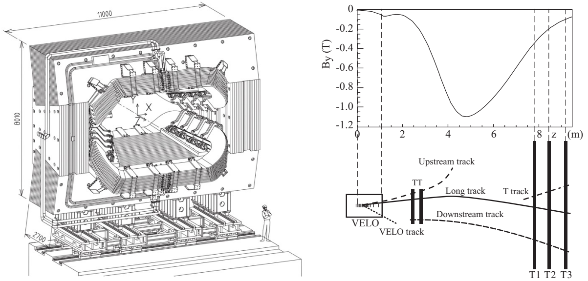
Figure 3.8: (Left) Perspective view of the LHCb dipole magnet (lengths are expressed in millimetres); the interaction point lies behind the magnet. (Right) Vertical magnetic field measured on the z axis, as a function of the z coordinate. The z location of the tracking detectors is shown, as well as the names given to reconstructed tracks, depending on the detectors where they have left a detectable signal. Only long tracks, i.e. tracks with segments reconstructed in all of the three tracking detectors, are employed in the present measurement. Figures taken from Ref. [147].
