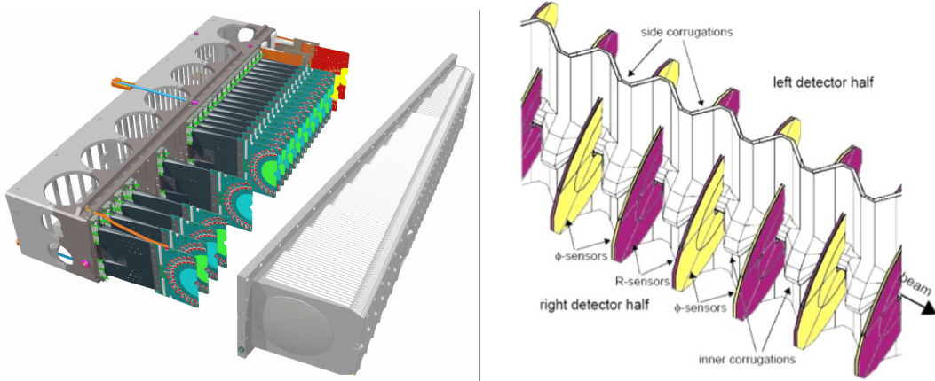
Figure 3.6: (Left) Exploded view of the module support and the modules (on the left), and of the RF box (on the right). The corrugated foil on the front face of the box, which forms a beam passage, can be seen. Its shape allows the two halves to overlap when in the closed position. (Right) Inner view of the RF-boxes, with the detector halves in the fully closed position. The edges of the boxes are cut away to show the overlap between the sensors of the two halves. R - and \phi -sensors are coloured in yellow and purple, respectively. Figures taken from Ref. [147].
