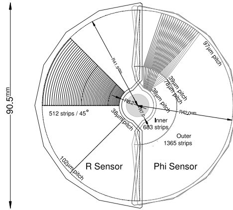
Figure 3.5: Geometrical scheme of the R and \phi VELO sensors. For clarity, only a portion of the strips are illustrated. In the \phi -sensor, the strips on two adjacent modules are indicated, to highlight the stereo angle. Figure taken from Ref. [148].
