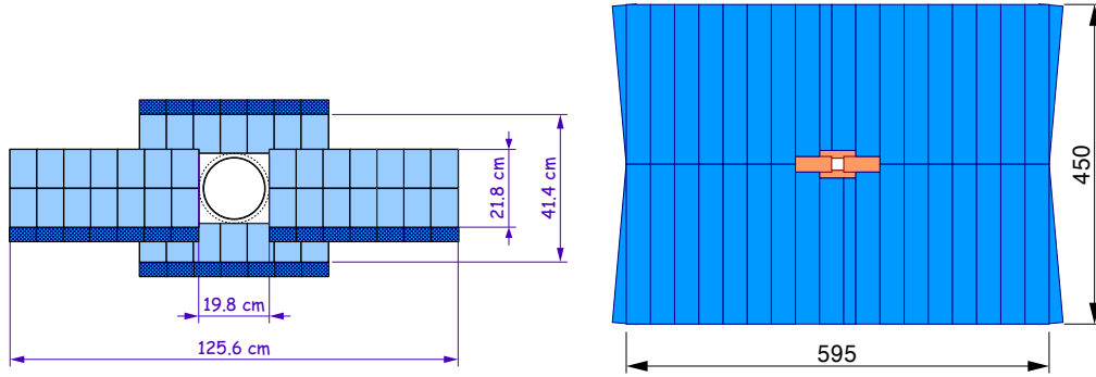
Figure 3.9: (Left) Front view of a layer of the inner tracker. (Right) Front view of one of the T-stations (lengths are expressed in centimetres). The inner tracker is drawn in orange and the outer tracker in blue. Figures taken from Ref. [149].
