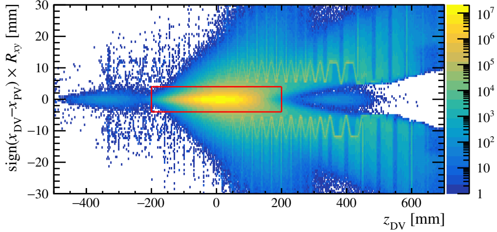
Figure 4.4: Signed radial distance of the DV of the D^0 meson with respect to its PV, as defined in Eq. (4.2), vs. its z coordinate. Vertical lines corresponding to VELO sensors and the wavy shape of the shielding RF foil are visible in the region R_{xy} > 5 mm. Only the candidates within the red rectangle ( R_{xy} < 4 mm \wedge |z_{DV}| < 200 mm) are selected for further analysis.
