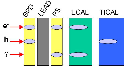
Figure 3.13: Energy deposited in the different detectors of the calorimetric system by electrons, hadrons and photons. Figure taken from Ref. [154].
