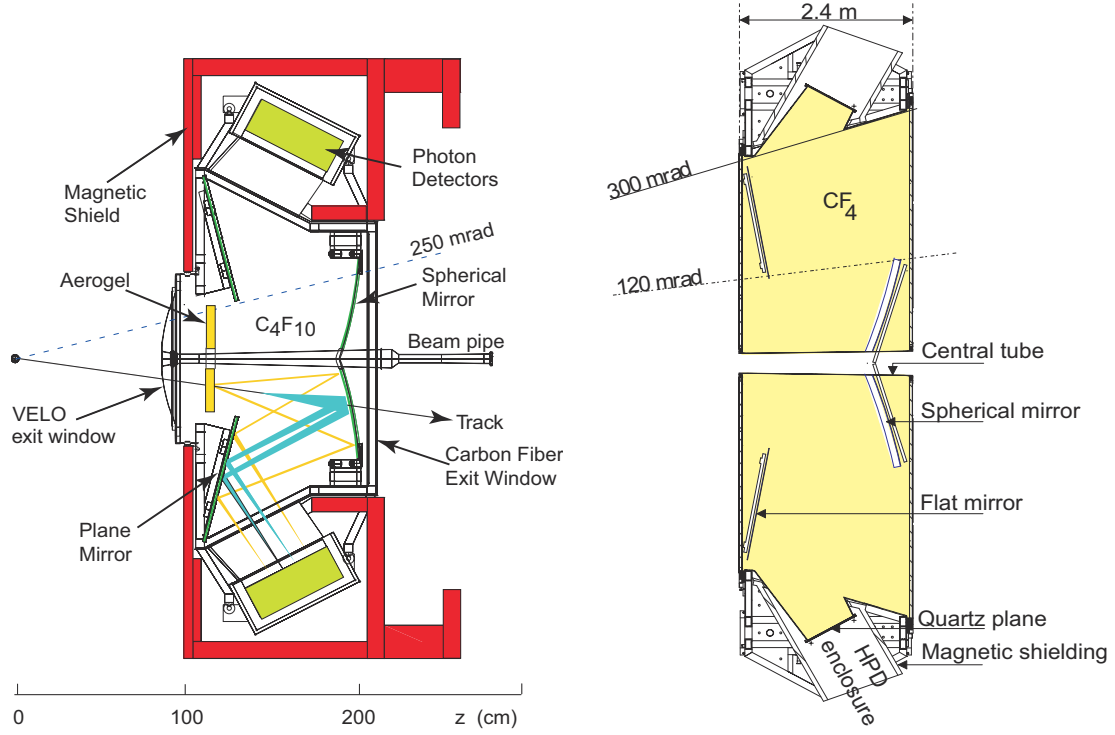
Figure 3.12: Side-view schematic layout of the (left) RICH1 and (right) RICH2 detectors. Figures taken from Ref. [147].
