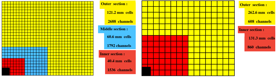
Figure 3.14: Segmentation of one quadrant (left) of the SPD, PS and ECAL and (right) of the HCAL. The black sector, corresponding to the beam pipe, is outside of the LHCb acceptance. Figure taken from Ref. [147].
