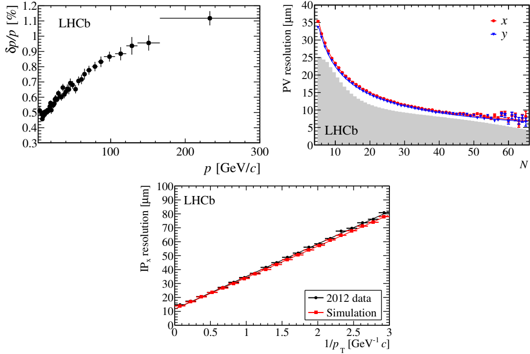
Figure 3.17: Performance of the tracking system of the LHCb detector. (Top left) Relative momentum resolution as a function of momentum, for long tracks from the decay of J/\psi particles. (Top right) Primary vertex resolution in the x and y directions, for events with one reconstructed PV, as a function of tracks multiplicity, whose distribution is reported in grey in arbitrary units. (Bottom) Resolution of the x projection of the impact parameter with respect to the primary vertex, as a function of 1/p_T . Figures taken from Ref. [148].
