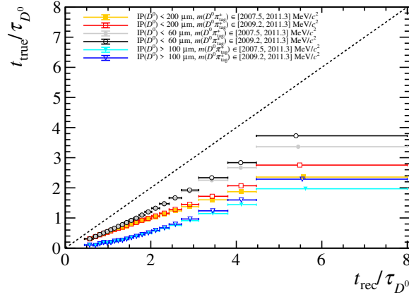
Figure 6.13: True decay time of secondary D^0 mesons as a function of their measured decay time.
