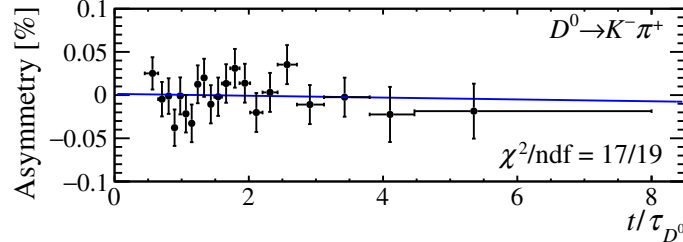
Figure 5.8: Linear fit to the time-dependent asymmetry of the full D^0 \rightarrow K^- \pi^+ sample after the kinematic weighting.
