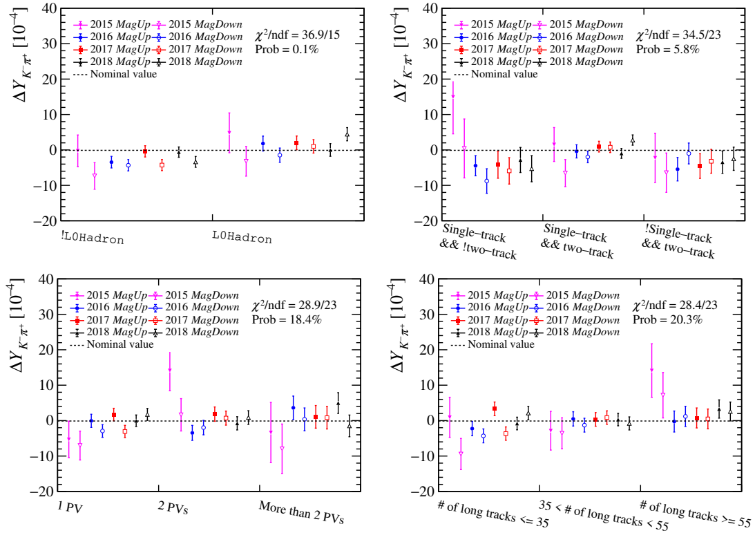
Figure 8.4: Measurements of \Delta Y_{K^- \pi^+} performed separately in subsamples corresponding to different trigger requirements and detector occupancies (and, for each subsample, separately for different data-taking years and magnet polarities). The p-value of the dispersion of the measurements around the average of the baseline one is displayed as well.
