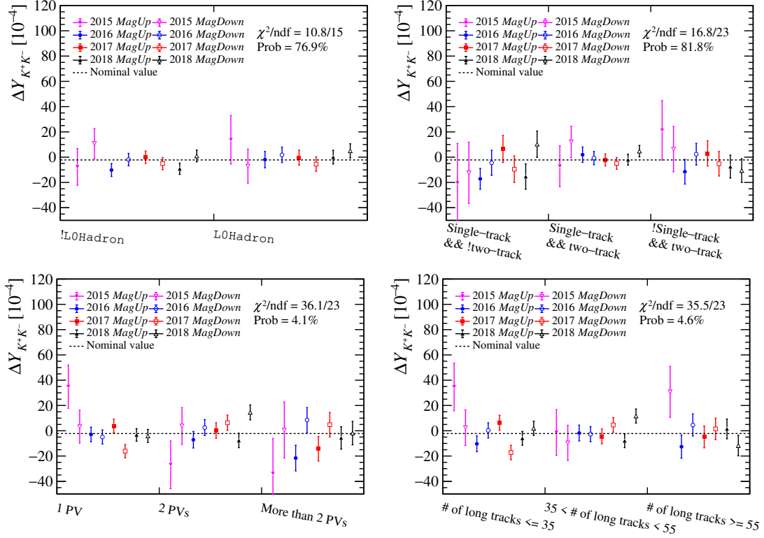
Figure 8.5: Measurements of \Delta Y_{K^+K^-} performed separately in subsamples corresponding to different trigger requirements and detector occupancies (and, for each subsample, separately for different data-taking years and magnet polarities). The p-value of the dispersion of the measurements around the baseline one is displayed as well.
