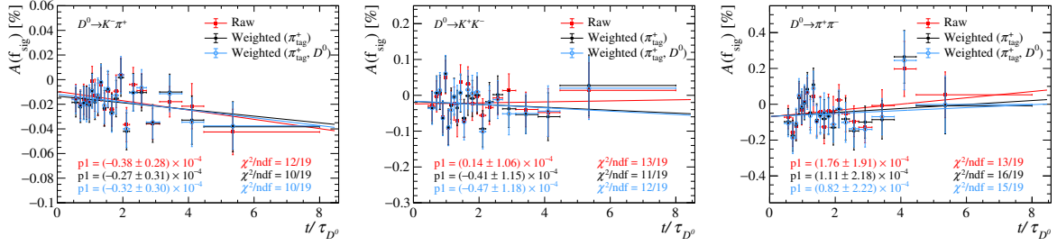
Figure 7.2: Asymmetry of the fraction of D^{*+} and D^{*-} candidates selected by the baseline m(D^0\pi_{\text{tag}}^+) signal window as a function of the D^0 decay time, for the (left) K^-\pi^+ , (centre) K^+K^- and (right) \pi^+\pi^- decay channels. The fractions are taken from the fits described in Sect. 4.3, which employ the whole data sample. Note that the range of the y axis depends on the decay channel.
