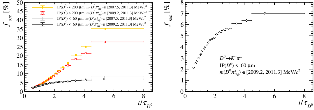
Figure 6.7: (Left) Fraction of secondary decays obtained in the template fit to the D^0 \rightarrow K^- \pi^+ two-dimensional distributions of D^0 \rightarrow K^- \pi^+ decays. (Right) Magnification of the left plot for the data with the baseline IP and m(D^0\pi^+_{\text{tag}}) requirements. Only the statistical uncertainty is reported.
