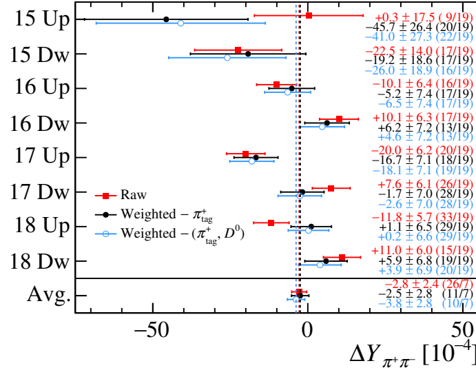
Figure 5.12: Summary of the fitted values of \Delta Y_{\pi^+\pi^-} in the eight subsamples divided according to the year and magnet polarity, together with their average. The numerical values of \Delta Y_{\pi^+\pi^-} and the \chi^2/\text{ndf} of the fits are reported on the right. The global p-values of the eight linear fits to the time-dependent asymmetry are 40%, 37% and 31% for raw data and after the first and second steps of the kinematic weighting, respectively, whereas the p-values of the average of \Delta Y_{\pi^+\pi^-} are 0.05%, 14% and 17%, respectively.
