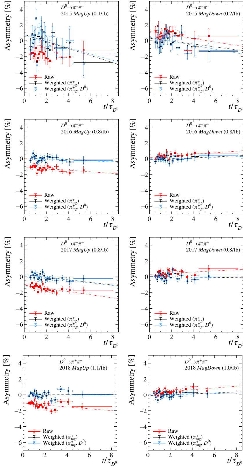
Figure 5.10: Linear fit to the time-dependent asymmetry of the D^0 \rightarrow \pi^+ \pi^- sample (red) for raw data, (black) after the first kinematic weighting and (azure) after the second kinematic weighting.
