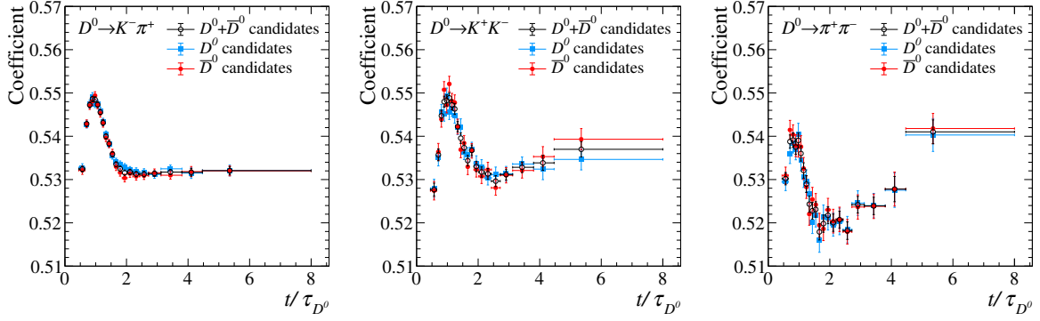
Figure 4.8: Magnitude of the coefficient used to remove the m(D^0\pi_{\text{tag}}^+) background as a function of decay time, as calculated from the results of the fits to the m(D^0\pi_{\text{tag}}^+) distributions.
