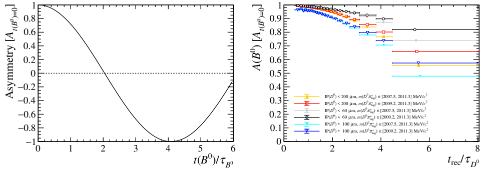
Figure 6.9: Impact of B^0 mixing on the time variation of the asymmetry of the number of D^{*+} mesons from B^0 decays, as a function of the (left) B^0 true decay time and (right) D^0 measured decay time. The asymmetry is zero after half of the B^0 mesons have oscillated, at t = \pi\tau_{B^0}/2x \approx 2.04\tau_{B^0} . The second plot is produced using the approximate estimated value of the B^0 decay time (see the text for details); its shape reproduces closely that of the left plot in the range [0, 1.4]\tau_{B^0} . The unit of measurement of the y axis is the production asymmetry of D^{*+} mesons coming from B^0 mesons that decayed at zero decay time, denoted as A_{B^0} in Eq. (6.3).
