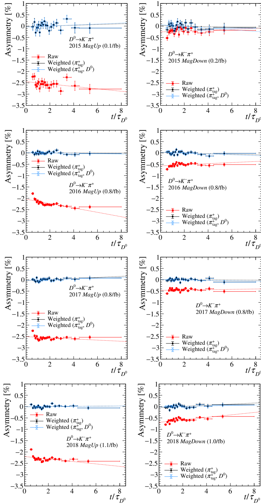
Figure 5.6: Linear fit to the time-dependent asymmetry of D^0 \rightarrow K^- \pi^+ decays (red) for raw data, (black) after the first kinematic weighting and (azure) after the second kinematic weighting.
