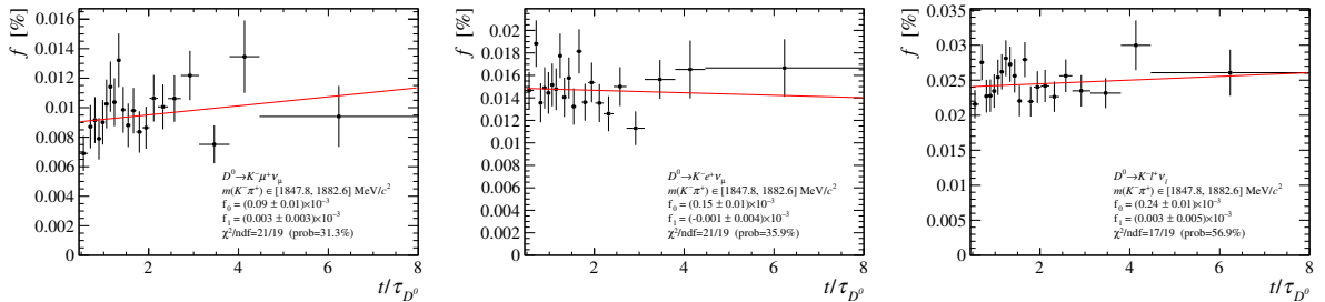
Figure E.6: Linear fit to the time-dependent fraction of background candidates in the m(K^-\pi^+) signal region, for all relevant backgrounds components.
