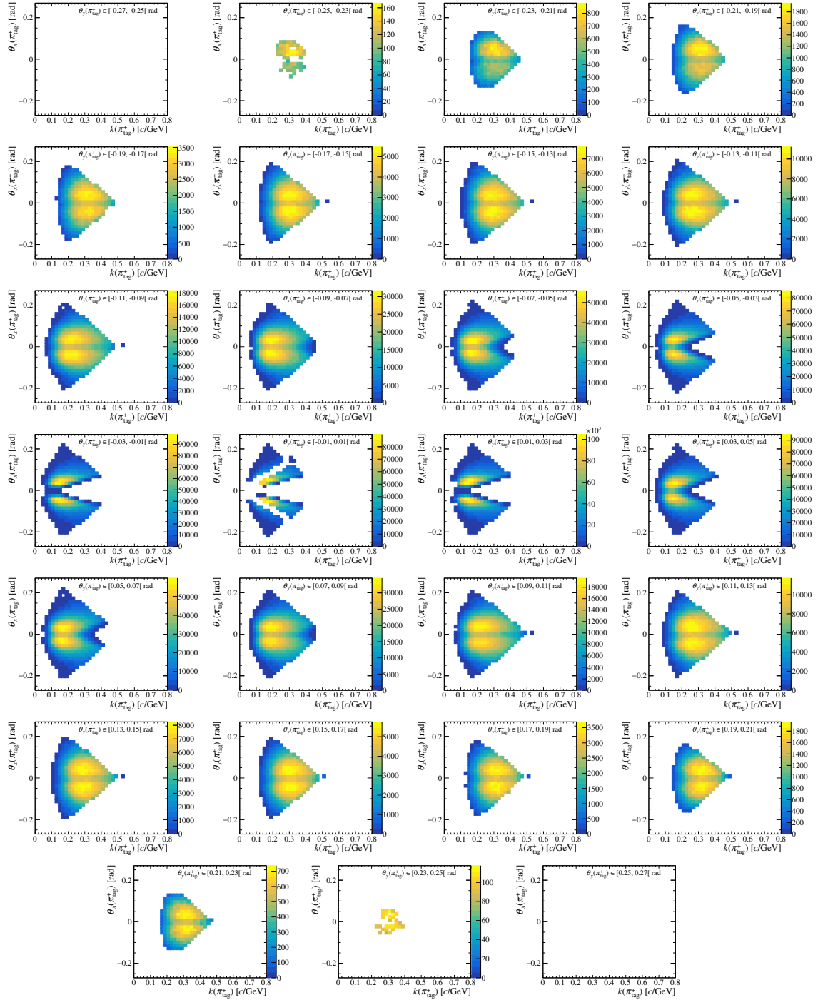
Figure D.3: Distribution of k vs. \theta_x of the candidates of the K^-\pi^+ subsample, collected during 2017 with the MagUp polarity, which are not rejected by the requirements on the minimum number of events and maximum asymmetry per bin in the first step of the kinematic weighting. The distributions are shown for each bin of the third weighted variable, \theta_y . The requirements reject many of the candidates with low curvature ( cf. Fig. 5.1), as well as those that are deflected into the LHC beam pipe by the magnet, corresponding to the empty diagonal bands of the plot corresponding to \theta_y \in [-10, 10] mrad.
