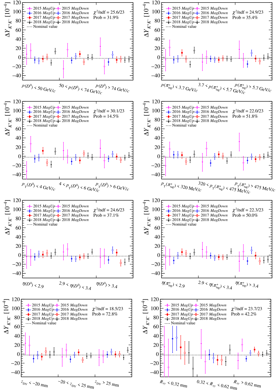
Figure 8.2: Measurements of \Delta Y_{K^+K^-} performed separately in three bins of the momentum, transverse momentum and pseudorapidity of the D^0 and \pi^+_{\text{tag}} mesons and of the position of the D^0 decay vertex along the beam direction and in the plane transverse to it. Each of these bins is further divided in eight subsamples corresponding to different data-taking years and magnet polarities. The p-value of the dispersion of the measurements around the baseline one is displayed as well.
