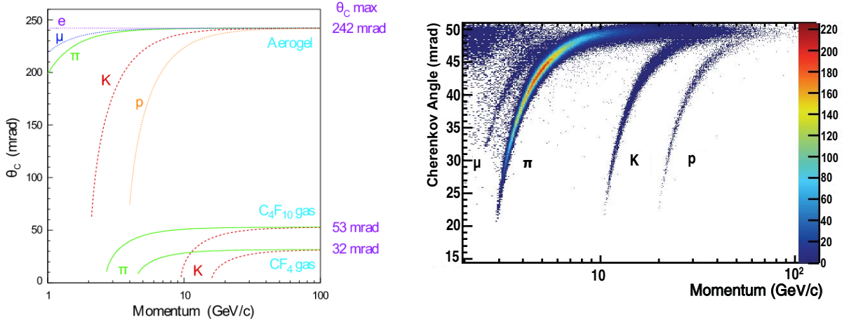
Figure 3.11: Cherenkov angle as a function of particle momentum (left) for the RICH radiators and for different particle masses and (right) for isolated tracks, defined as tracks whose Cherenkov ring does not overlap with any other ring, in the C_4F_{10} radiator. Figures taken from Refs. [147, 152].
