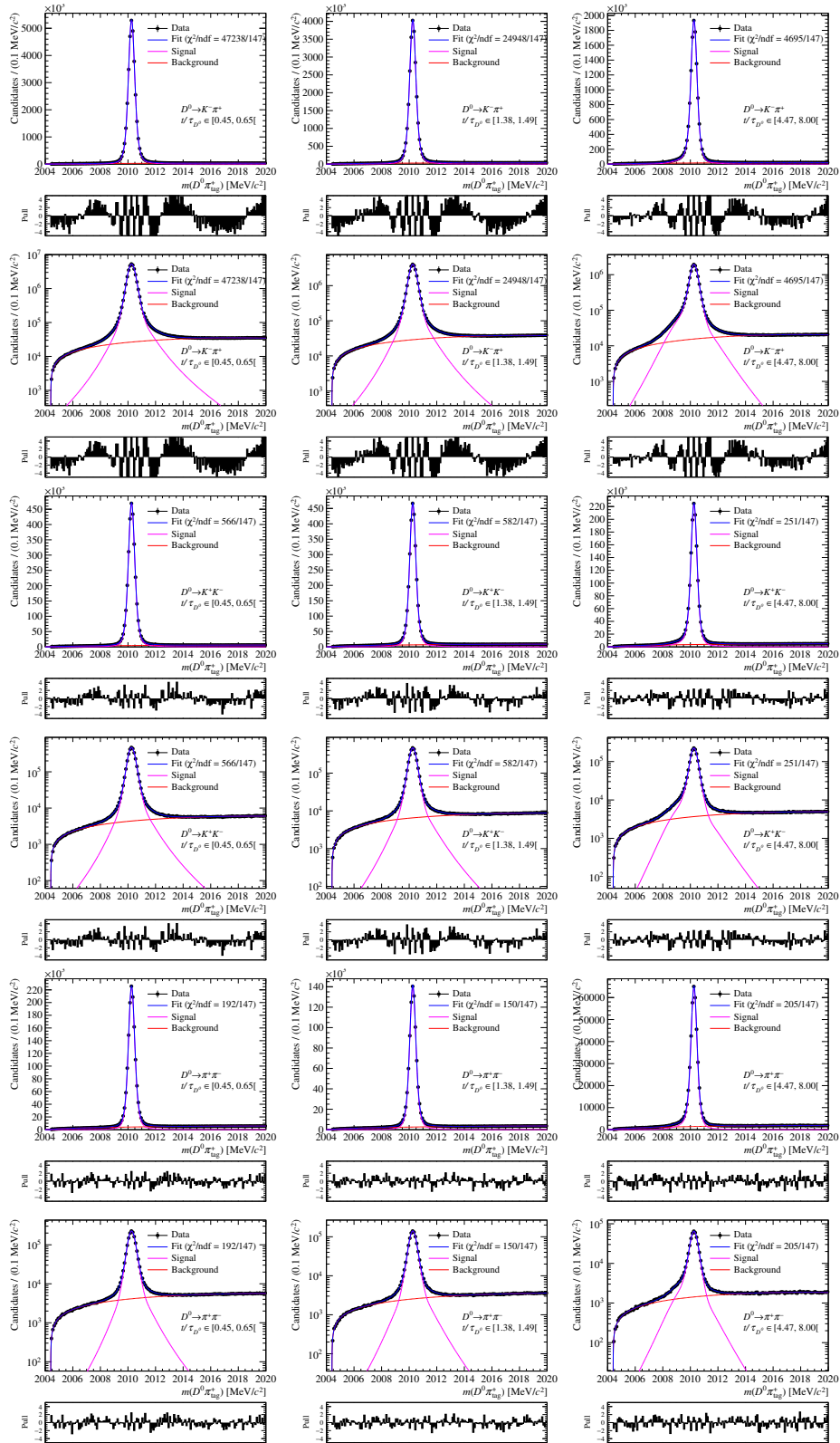
Figure 4.7: Distribution of m(D^0 \pi^+_{\text{tag}}) , with fits superimposed, for the (top) K^- \pi^+ , (centre) K^+ K^- and (bottom) \pi^+ \pi^- decay channels, both in linear and in logarithmic scales. Left, central and right plots correspond to the first, tenth and last bin of decay time, respectively.
