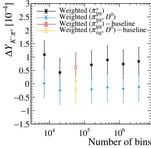
Figure 7.6: Measurements of \Delta Y_{K^- \pi^+} as a function of the number of bins employed in the kinematic weighting. The definition of the binnings is provided in Table 7.2.
