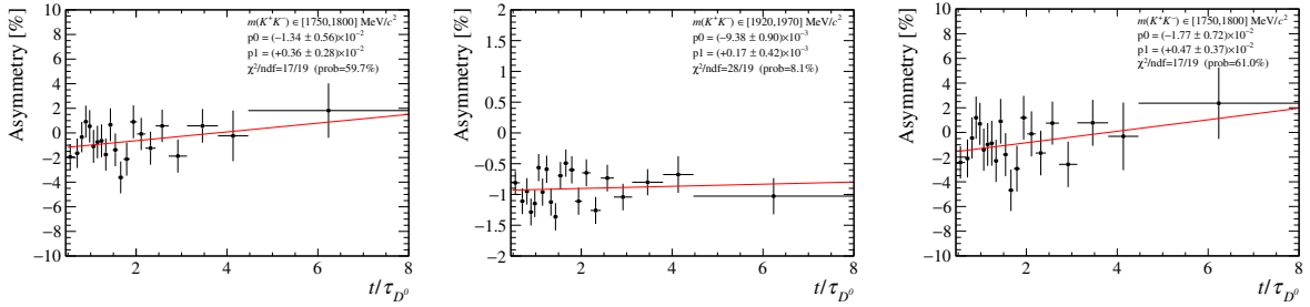
Figure E.11: Linear fit to the time-dependent asymmetry (left) in the m(K^+K^-) \in [1750, 1800] \text{ MeV}/c^2 window, (centre) in the m(K^+K^-) \in [1920, 1970] \text{ MeV}/c^2 window and (right) of the D^0 \rightarrow K^-\pi^+\pi^0 background, calculated by dividing the asymmetry of the left plot by the D^0 \rightarrow K^-\pi^+\pi^0 background fraction in the corresponding window.
