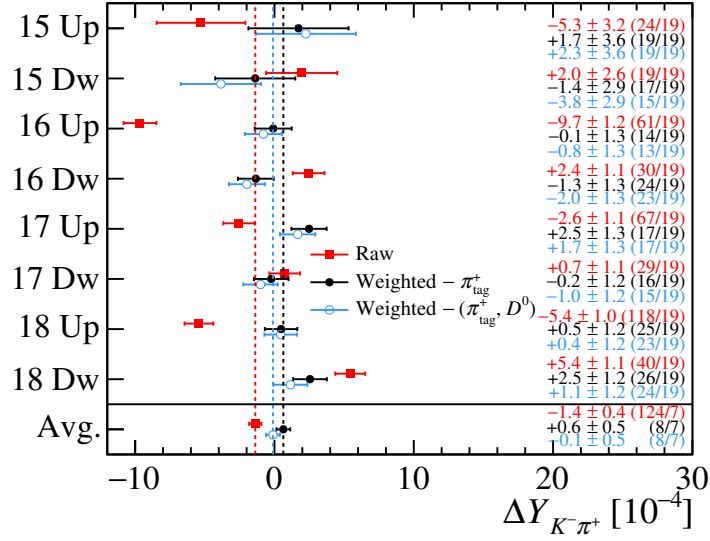
Figure 5.7: Summary of the fitted values of \Delta Y_{K^- \pi^+} in the eight subsamples divided according to the year and magnet polarity, together with their average. The numerical values of \Delta Y_{K^- \pi^+} and the \chi^2/\text{ndf} of the fits are reported on the right. The global p-values of the eight linear fits to the time-dependent asymmetry are 7 \times 10^{-23} , 45% and 64% for raw data and after the first and second step of the kinematic weighting, respectively, whereas the p-values of the average of \Delta Y_{K^- \pi^+} are 1 \times 10^{-21} , 30% and 31%, respectively.
