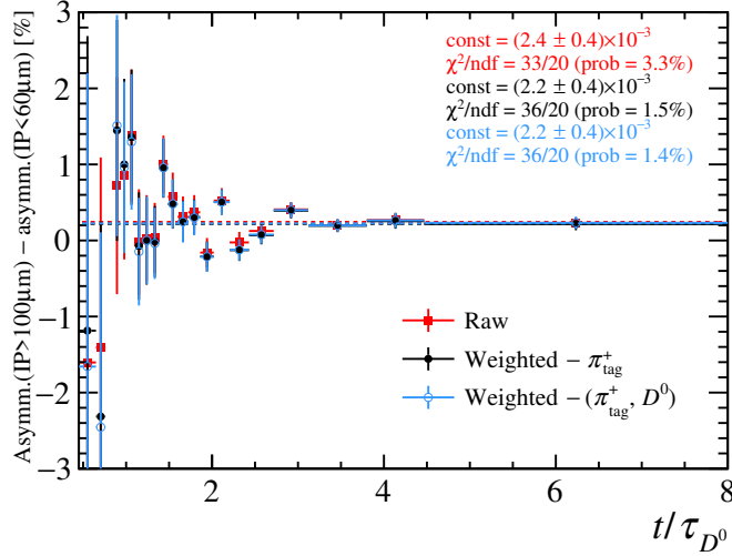
Figure D.5: Asymmetry difference of secondary and primary K^-\pi^+ candidates, before and after the kinematic weighting. This is calculated as the difference of the asymmetry of the candidates with \text{IP} > 100 \mu\text{m} and those satisfying \text{IP}(D^0) < 60 \mu\text{m} . These categories are good proxies of secondary and primary decays, while the subtraction allows to cancel the nuisance detection asymmetries also before the kinematic weighting. A constant fit is superimposed. The results show that the asymmetry difference changes by less than 10% after the kinematic weighting.
