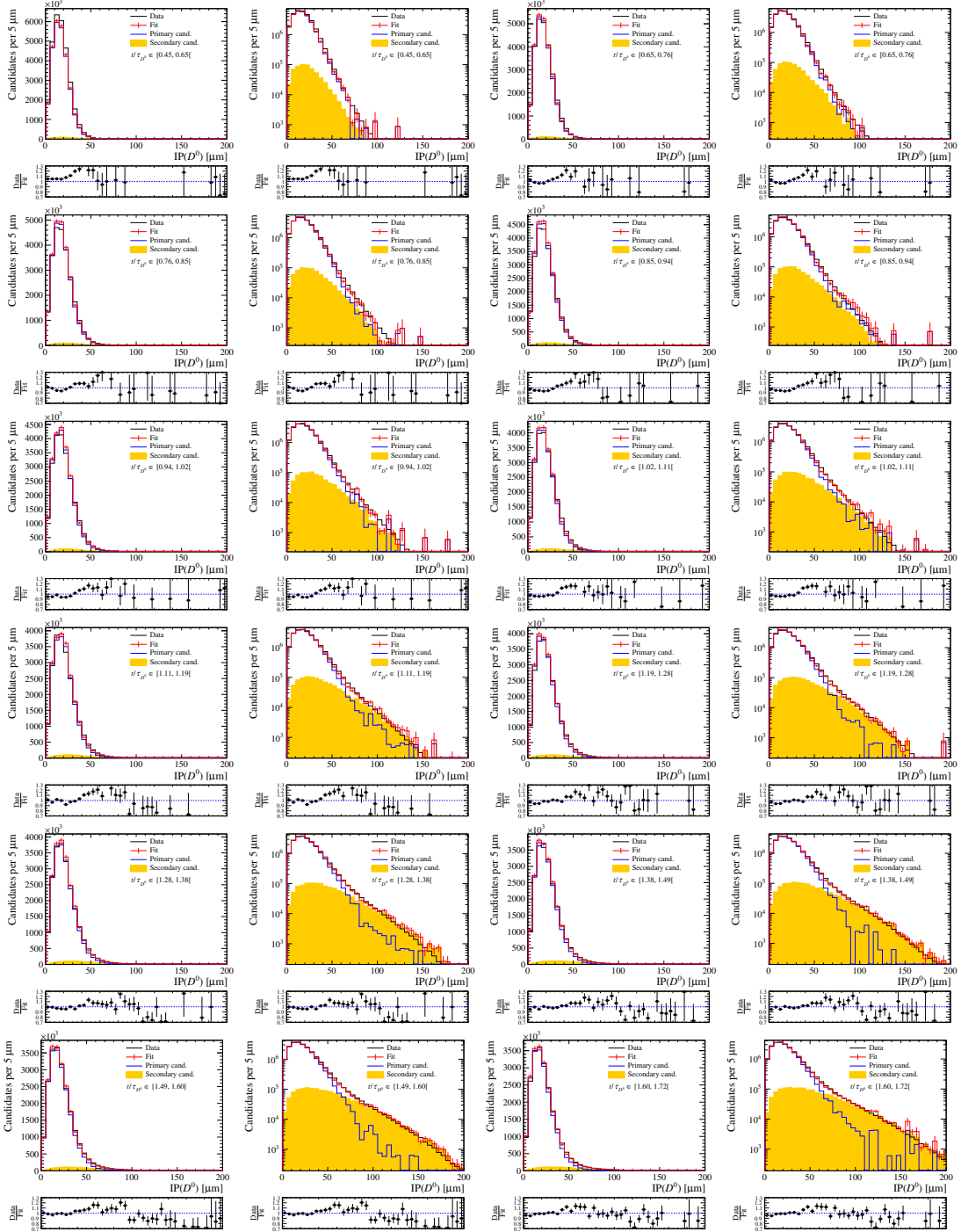
Figure 6.5: Projections of the template fit to the \text{IP}(D^0) vs. t(D^0) distribution of D^0 \rightarrow K^-\pi^+ and \bar{D}^0 \rightarrow K^+\pi^- decays combined, for the time bins from 1 to 12. A looser requirement m(D^0\pi_{\text{tag}}^+) \in [2007.5, 2011.3] \text{ MeV}/c^2 is applied with respect to the baseline selection of Sect. 4.3. The templates are taken from simulation for both primary and secondary decays and only the relative time-integrated abundance is left free to vary in the fit.
