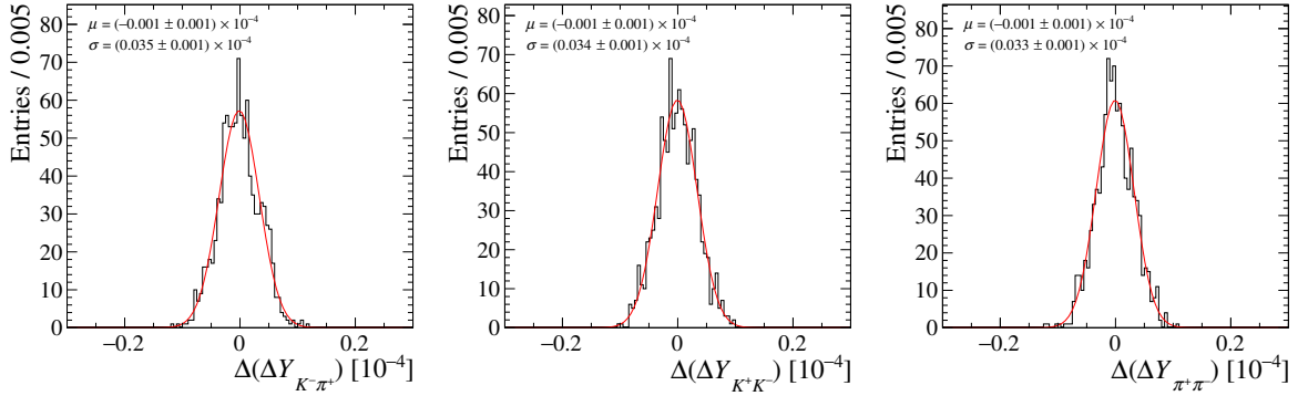
Figure 7.3: Difference between the fitted value of \Delta Y obtained in 1000 pseudoexperiments where the constant asymmetry difference of secondary and primary decays is varied within its uncertainty, and the baseline one.
