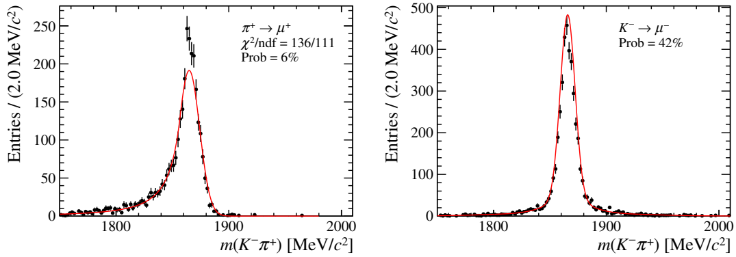
Figure 7.12: Fits to the mass distribution of simulated D^0 \rightarrow K^-\pi^+ decays, where the (left) \pi^+ meson and (right) K^- meson pass through all of the muon stations and are thus identified as muons.
