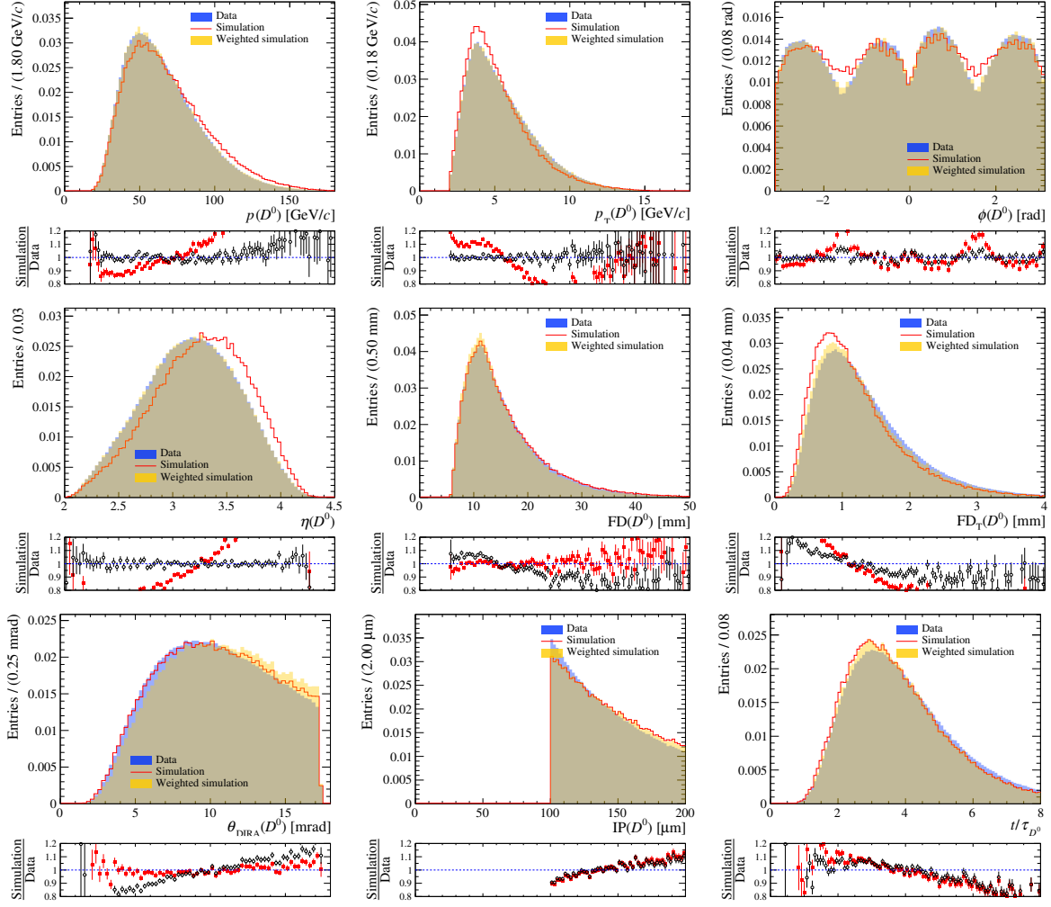
Figure 4.13: Comparison between the kinematic distributions of D^0 \rightarrow K^- \pi^+ secondary decays in data and simulation, both before and after the three-dimensional ( p_T, \eta, \phi ) weighting of the D^0 momentum. The data sample of secondary decays is selected using 1/6 of the candidates satisfying the requirement 100 < \text{IP}(D^0) < 200 \mu\text{m} . In the plots displaying the ratio of simulated to real data, full red squares (open black circles) correspond to simulated data before (after) the weighting.
