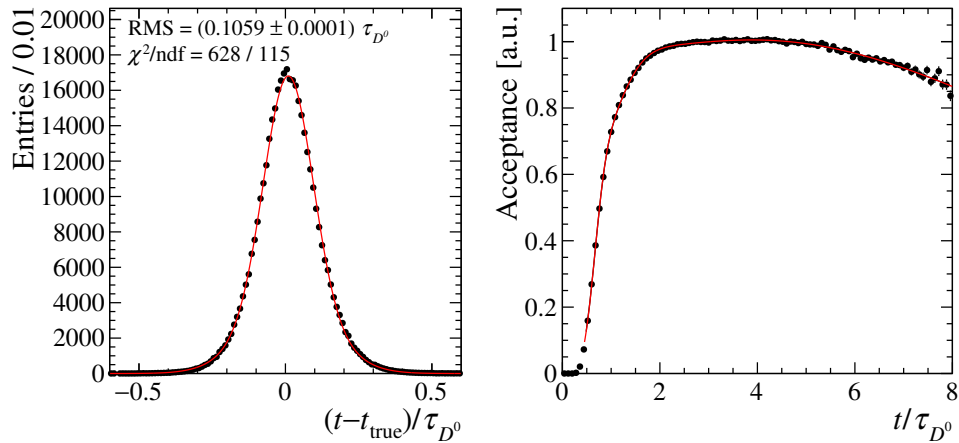
Figure 7.14: (Left) Decay-time resolution, as measured in the simulation of D^0 \rightarrow K^-\pi^+ decays. The result of a fit of the sum of two Gaussian functions is superimposed. (Right) Fit to the decay-time acceptance, defined as the ratio of the decay-time distribution of D^0 \rightarrow K^+K^- data over an exponential function convolved with the resolution function fitted in the left plot.
