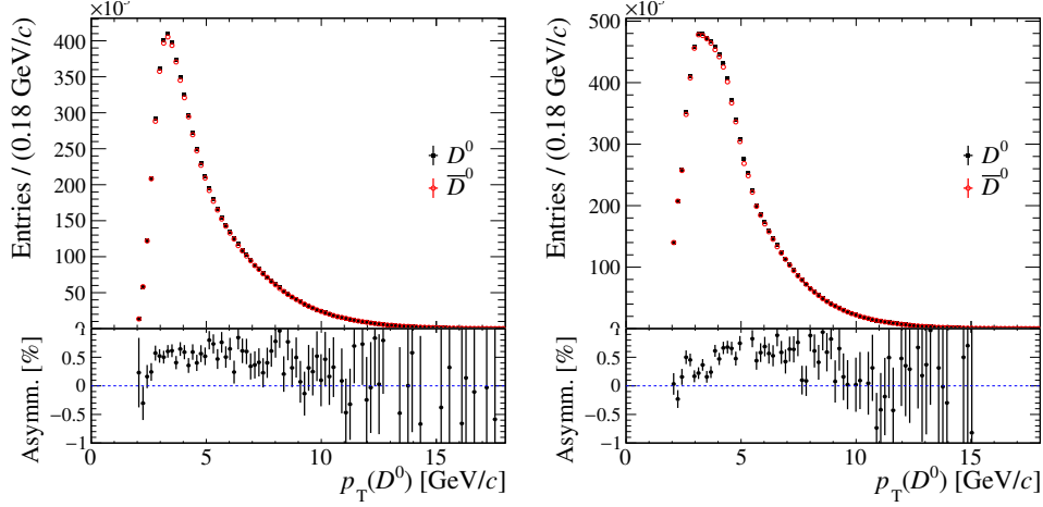
Figure D.13: Asymmetry of the p_T(D^0) kinematically weighted distribution in the (left) leftmost and (right) baseline m(D^0\pi_{\text{tag}}^+) sidebands.
