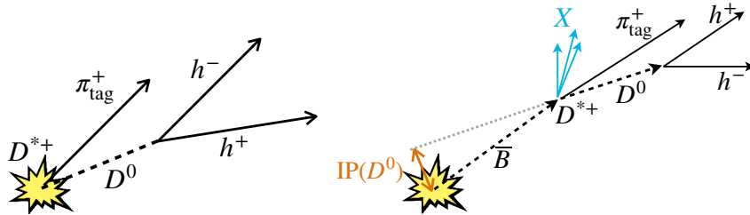
Figure 6.1: Topologies of (left) primary and (right) secondary decays. In the right figure, X stays for all particles other than the D^{*+} meson which are produced in the decay of the B meson.
