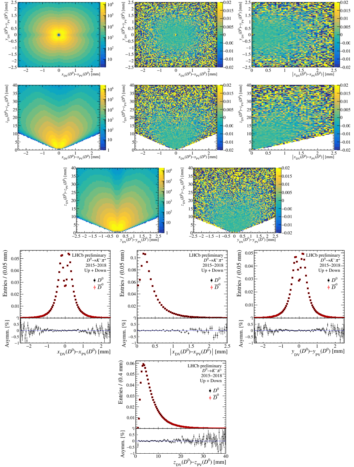
Figure D.11: Distributions and asymmetries of the D^0 flight distance for the full D^0 \rightarrow K^- \pi^+ data sample.
