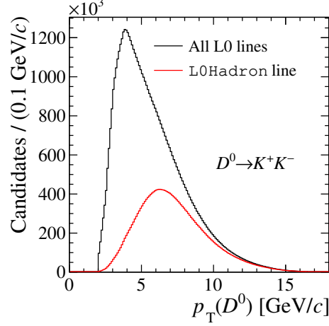
Figure 4.1: Distribution of the D^0 transverse momentum, for all selected signal candidates and for those where the D^0 meson fired the L0Hadron hardware-trigger line.
