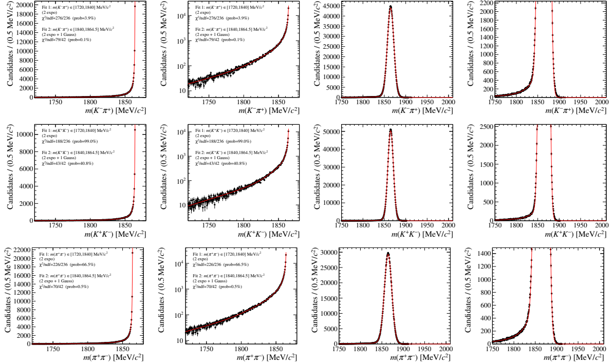
Figure 7.10: Fits to the RAPIDSIM m(h^+ h^-) signal distribution for events with FSR, in (left) linear and (centre-left) logarithmic scale. The true values of the momenta are used and only events more distant than 0.5 \text{ MeV}/c^2 from the D^0 mass peak are taken into account. Centre-right and right plots display the cross-check fit where the FSR distributions is fixed to that obtained in the left plot, is convolved with a Gaussian resolution function and is compared with the RAPIDSIM distribution (calculated using smeared momenta) of all data, including candidates without FSR. Top, centre and bottom plots correspond to the K^- \pi^+ , K^+ K^- and \pi^+ \pi^- decay channels.
