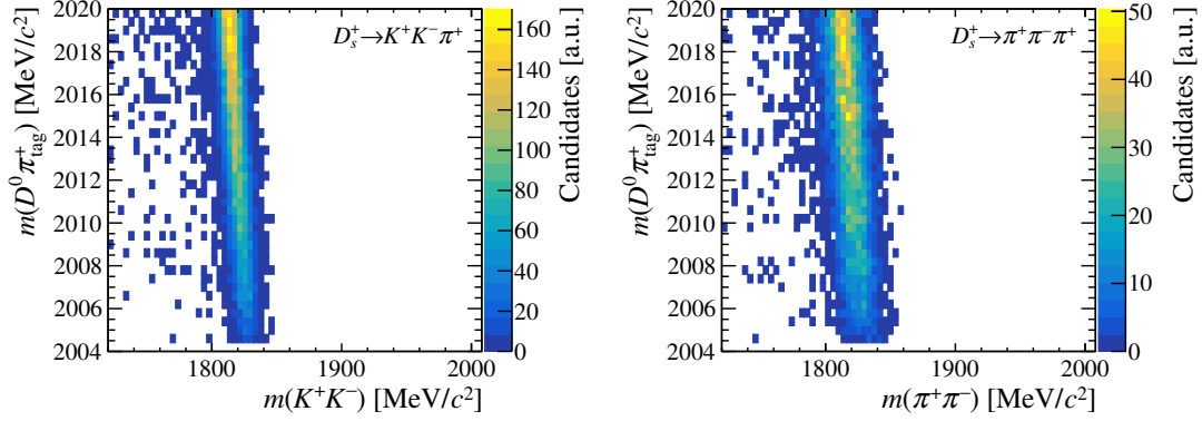
Figure 7.9: (Left) Distribution of D_s^+ \rightarrow K^+ K^- \pi^+ decays in the m(D^0 \pi_{\text{tag}}^+) vs. m(K^+ K^-) plane, when they are reconstructed as D^0 \rightarrow K^+ K^- candidates coming from a D^{*+} \rightarrow D^0 \pi_{\text{tag}}^+ decay. (Right) Distribution of D_s^+ \rightarrow \pi^+ \pi^- \pi^+ decays in the m(D^0 \pi_{\text{tag}}^+) vs. m(\pi^+ \pi^-) plane, when they are reconstructed as D^0 \rightarrow \pi^+ \pi^- candidates coming from a D^{*+} \rightarrow D^0 \pi_{\text{tag}}^+ decay.
