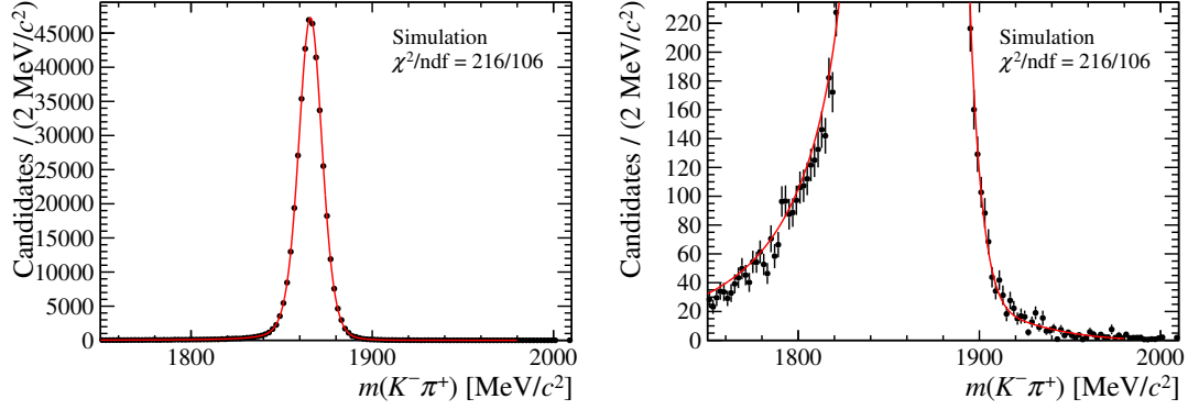
Figure 7.11: (Left) Result of the fit of the resolution to the distribution of simulated m(K^-\pi^+) decays, where both K^- and \pi^+ candidates are required not to pass through all of the muon chambers. The shape of the FSR is fixed to that obtained in the fit to the RAPIDSIM simulation in Fig. 7.10, and only the resolution function, parametrised as the sum of four Gaussian functions with shared mean, is left free to vary. (Right) Magnification of the left plot.
