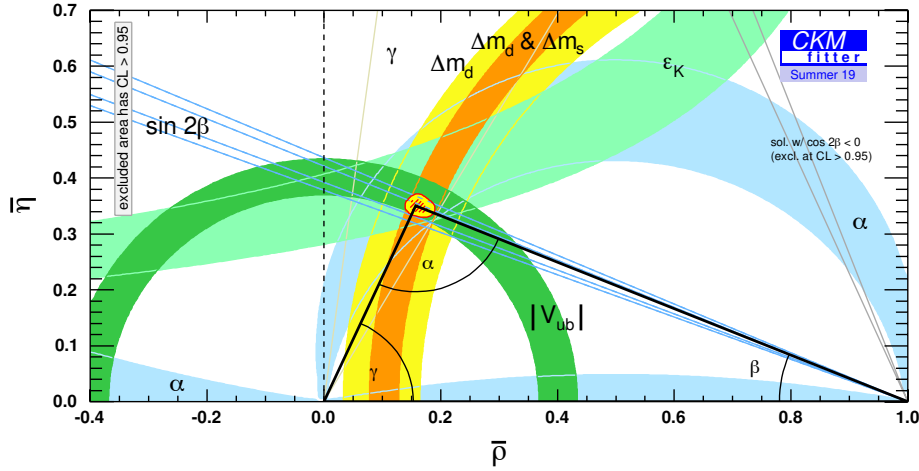
Figure 1.2: Constraints on the (\bar{\rho}, \bar{\eta}) plane. The red hashed region of the global combination corresponds to 68% CL. Figure taken from Ref. [47].
