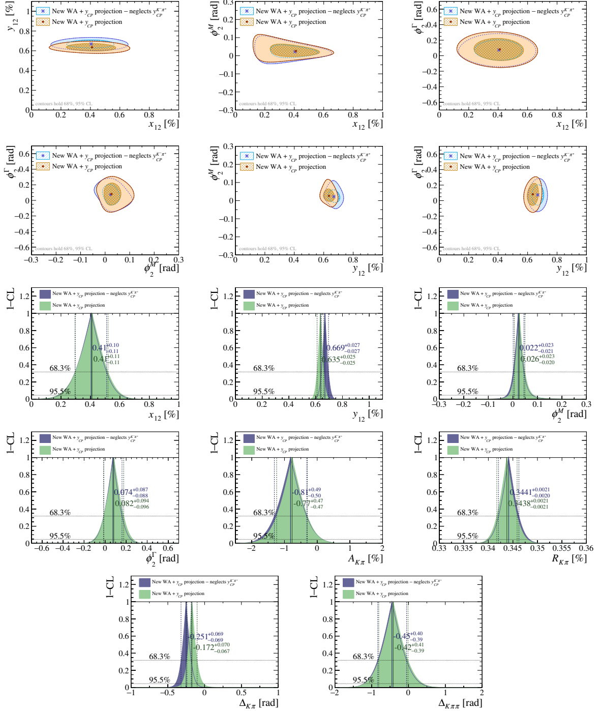
Figure B.5: Impact of neglecting the contribution of y_{CP}^{K^- \pi^+} in the measurement of the y_{CP} parameter on the knowledge of the parameters quantifying mixing and time-dependent CP violation in D^0 decays, in the theoretical parametrisation. The fits employ all the measurements listed in Table B.1 plus a measurement of the parameter y_{CP} - y_{CP}^{K^- \pi^+} , whose value is equal to its point estimate based on the results of the current fit and whose uncertainty, 0.03 \times 10^{-3} , is approximately equal to the precision expected for the measurement with the LHCb 2015–2018 D^{*+} -tagged data sample.
