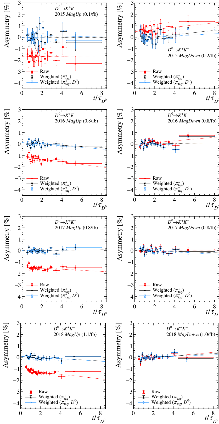
Figure 5.9: Linear fit to the time-dependent asymmetry of the D^0 \rightarrow K^+ K^- sample (red) for raw data, (black) after the first kinematic weighting and (azure) after the second kinematic weighting.
