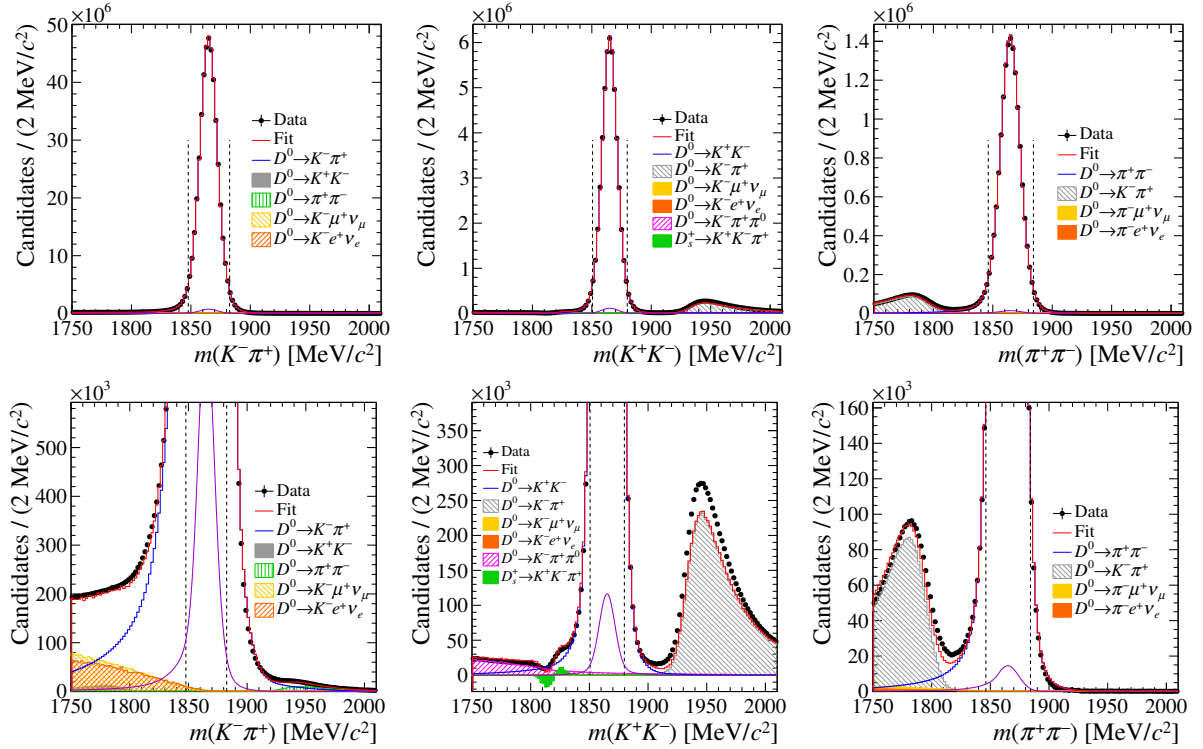
Figure E.4: Template fit to the time and flavour integrated m(h^+h^-) distributions of (left) K^-\pi^+ , (centre) K^+K^- and (right) \pi^+\pi^- decays. The relative normalisation between the background components and the signal is fixed to the expectations of RAPIDSIM and PIDCALIB; the signal component due to decays in flight of D^0 daughter mesons into muons is shown in violet. Bottom plots are magnified to put the background components in evidence.
