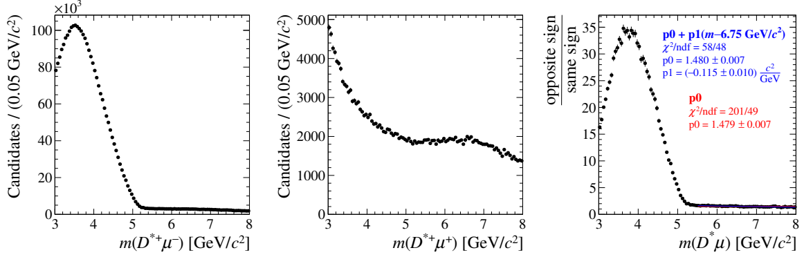
Figure 4.11: Invariant-mass distribution of the combination of the D^{*+} meson with a muon with (left) opposite and (centre) equal charge. The ratio of the two distributions is shown in the right plot, together with the \chi^2 fits of a constant and a linear function in the range [5.5, 8] \text{GeV}/c^2 .
