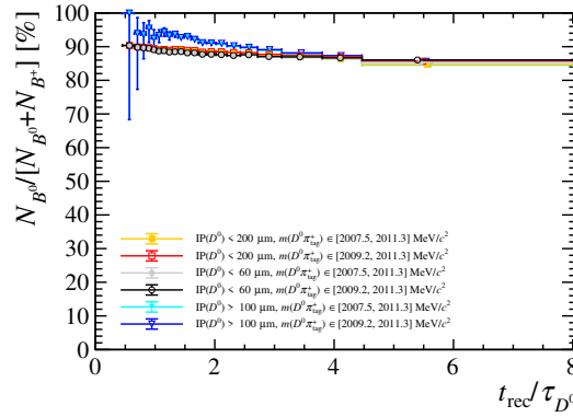
Figure 6.4: Fraction of B^0 mesons with respect to the total number of B mesons as a function of the measured decay time of secondary decays in simulation.
