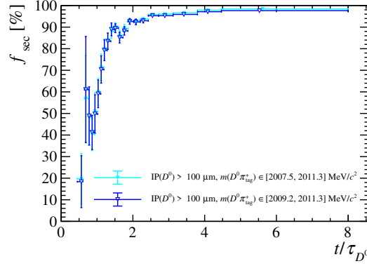
Figure 6.10: Fraction of secondary decays in data satisfying \text{IP}(D^0) > 100 \mu\text{m} , as calculated from the results of the template fit to the \text{IP} vs. t distribution of D^0 mesons, in the enlarged ( [2007.5, 2011.3] \text{ MeV}/c^2 ) and in the nominal ( [2009.2, 2011.3] \text{ MeV}/c^2 ) m(D^0\pi_{\text{tag}}^+) signal window.
