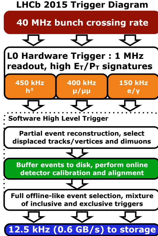
Figure 3.16: Trigger scheme of the LHCb experiment during 2015–2018.
