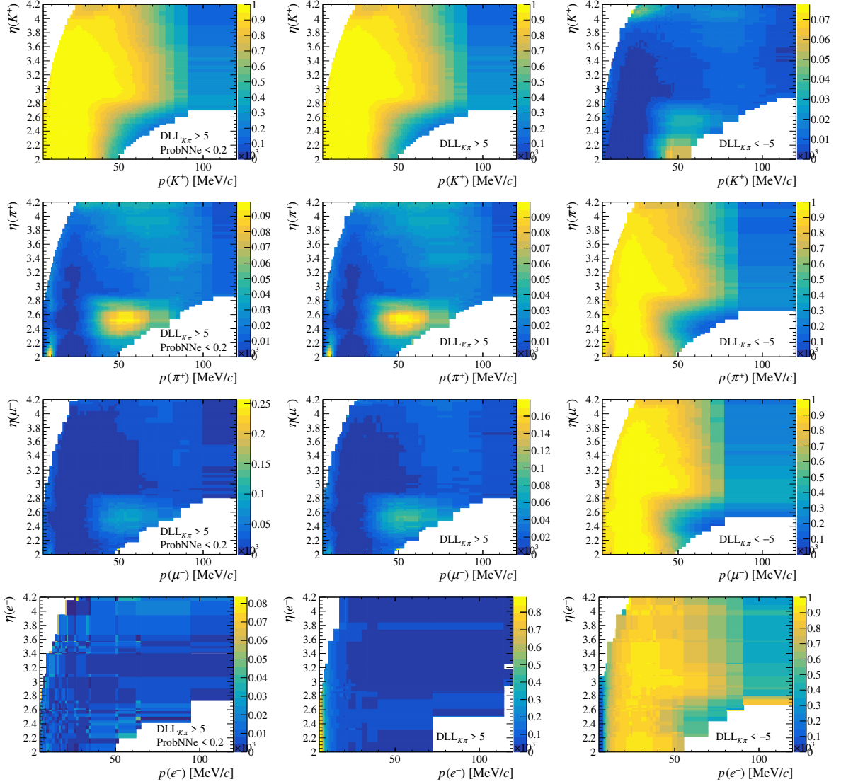
Figure E.3: PID efficiency for identifying a (top) K meson, (centre-top) \pi meson, (centre-bottom) muon or (bottom) electron as (left) a charged kaon with electron veto, (centre) a charged kaon without electron veto or (right) a pion, as a function of the momentum and pseudorapidity.
