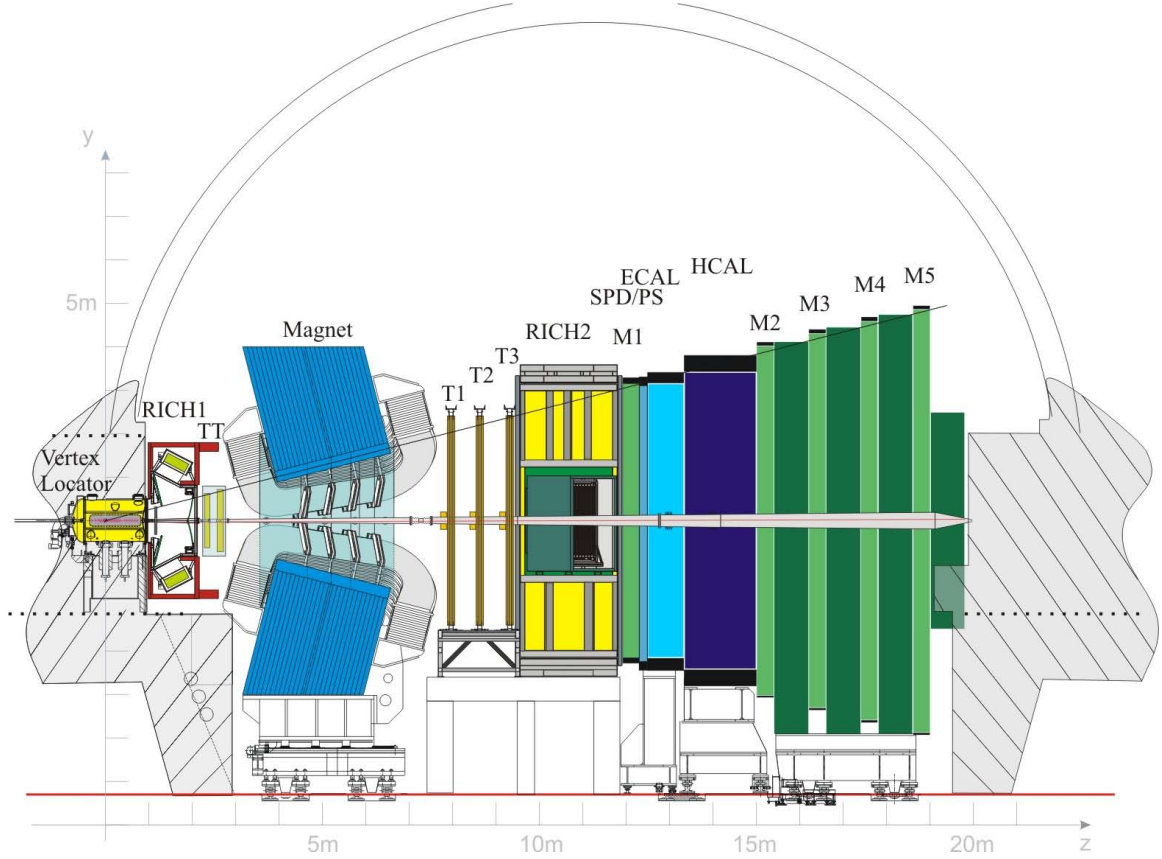
Figure 3.3: Side view of the LHCb spectrometer.
