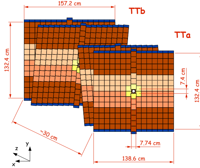
Figure 3.7: Scheme of the TT detector. Different readout sectors are indicated by different shadings. Figure taken from Ref. [149].
