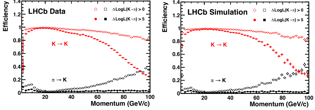
Figure 3.18: Kaon identification efficiency and pion misidentification rate as a function of track momentum for two different requirements on \Delta\text{LogL}_{K\pi} . The left and right figures correspond to data and to the expectations from simulation, respectively. Figures taken from Ref. [148].
