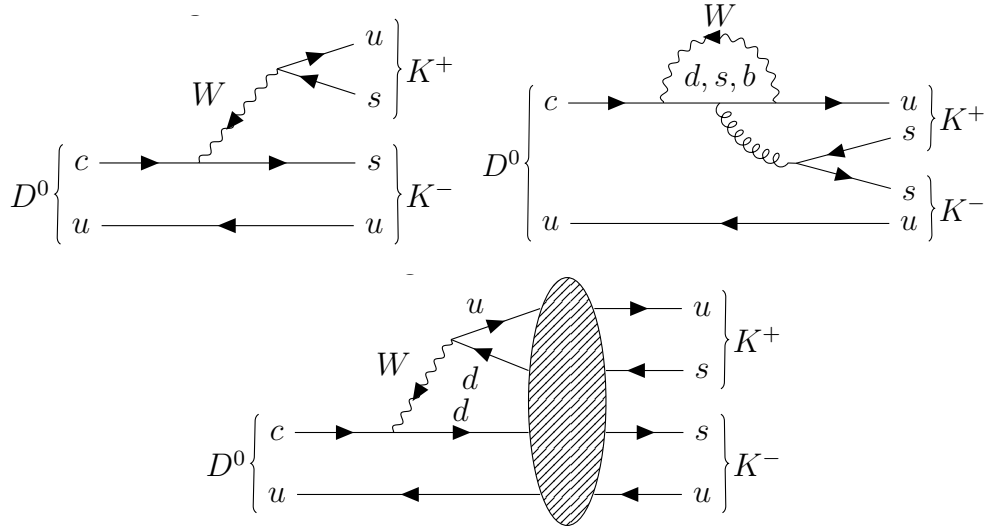
Figure 1.6: Examples of Feynman diagrams contributing to the D^0 \rightarrow K^+ K^- decay. The tree diagram (top left) is proportional to \lambda_{cu}^s , while the electroweak-loop diagram (top right) is proportional to \lambda_{cu}^q , where q is the internal quark of the loop. Finally, the bottom diagram represents one of the possible contributions to rescattering, where the blob is a placeholder for the rescattering of the \pi^+ \pi^- state into the K^+ K^- final state through strong interactions. This diagram is proportional to \lambda_{cu}^d = -\lambda_{cu}^s - \lambda_{cu}^b .
