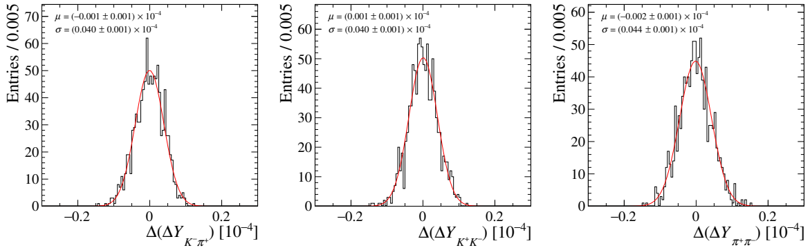
Figure 7.4: Difference between the fitted value of \Delta Y obtained in 1000 pseudoexperiments that take into account the impact of B^0 mixing on the secondary asymmetry, within the uncertainty of its fitted value, and that of the baseline model that assumes a time-independent asymmetry.
