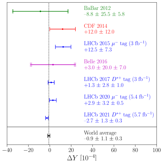
Figure 9.2: Summary of the most precise measurements of the parameter \Delta Y to date, including the present one. The measurements are compatible with each other, with a p-value of 38%. The world average without including the present measurement was \Delta Y = (3.1 \pm 2.0 \pm 0.5) \times 10^{-4} . Measurements references, from top to bottom: BaBar 2012 [62], CDF 2014 [117], LHCb 2015 \mu^- tag [118], Belle 2016 [64], LHCb 2017 D^{*+} tag [116], LHCb 2020 \mu^- tag [120], LHCb 2021 D^{*+} tag [135].
