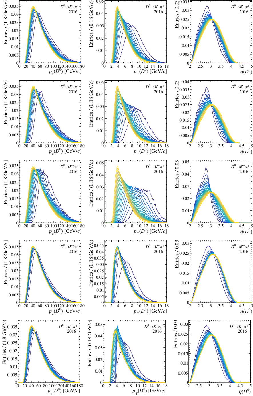
Figure D.1: Normalised distributions of the z and transverse components and of the pseudorapidity of the D^0 momentum, in different colours for different decay time bins, and for different first-stage software-trigger requirements. Blue (yellow) dots correspond to low (high) decay times, see Fig. 5.3 for the legend. The plots are produced using events where the D^0 meson was responsible for the first-stage software-trigger decision, for the following trigger lines, from top to bottom: the single-track line, with the \alpha_0 parameter equal to 1.1, 1.6 and 2.3, and the two-track line with the classifier threshold equal to 0.95 and 0.97.
