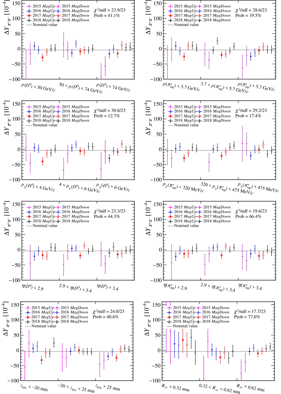
Figure 8.3: Measurements of \Delta Y_{\pi^+\pi^-} performed separately in three bins of the momentum, transverse momentum and pseudorapidity of the D^0 and \pi_{\text{tag}}^+ mesons and of the position of the D^0 decay vertex along the beam direction and in the plane transverse to it. Each of these bins is further divided in eight subsamples corresponding to different data-taking years and magnet polarities. The p-value of the dispersion of the measurements around the baseline one is displayed as well.
