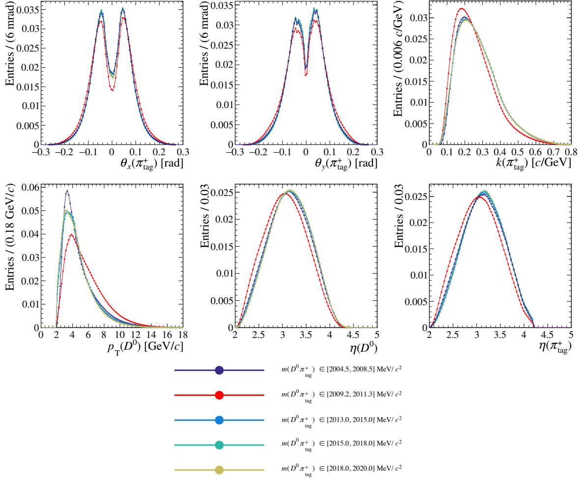
Figure D.12: Normalised distributions of the kinematic variables employed in the weighting of Sect. 5.2 in the m(D^0\pi_{\text{tag}}^+) signal window and in the baseline and alternative lateral windows defined in Sect. 7.1.
