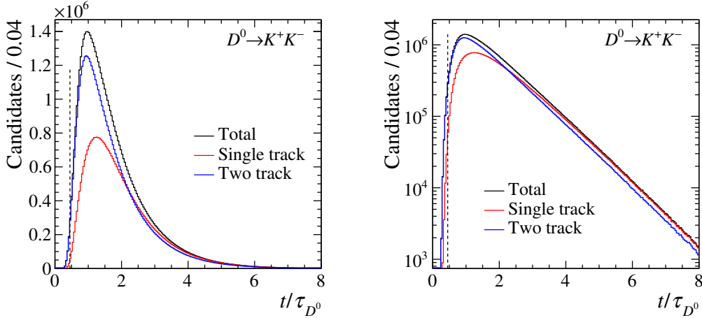
Figure 4.10: Distribution of the D^0 decay time, separately for different HLT1 lines, in (left) linear and (right) logarithmic scale. The vertical dashed line represents the lower requirement on decay time ( 0.45\tau_{D^0} ), while the upper requirement is at 8\tau_{D^0} .
