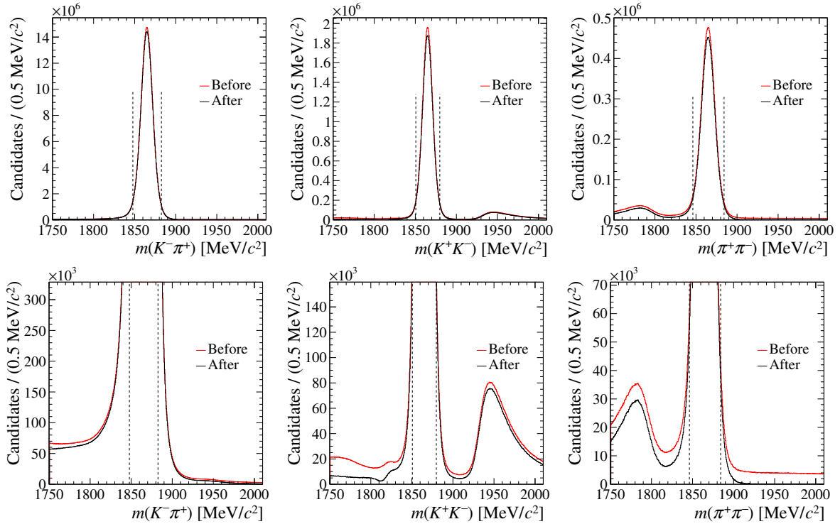
Figure 7.7: (Top): distribution of the invariant mass m(h^+h^-) of the final-state particles of the D^0 candidate (red) before and (black) after the removal of the m(D^0\pi_{\text{tag}}^+) background. The vertical dashed lines delimit the signal window. (Bottom): Magnification to put in evidence the shape of the residual background under the m(D^0) peak.
