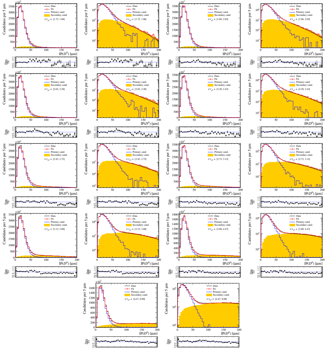
Figure 6.6: Projections of the template fit to the \text{IP}(D^0) vs. t(D^0) distribution of D^0 \rightarrow K^-\pi^+ and \bar{D}^0 \rightarrow K^+\pi^- decays combined, for the time bins from 13 to 21. A looser requirement m(D^0\pi_{\text{tag}}^+) \in [2007.5, 2011.3] MeV/ c^2 is applied with respect to the baseline selection of Sect. 4.3. The templates are taken from simulation for both primary and secondary decays and only the relative time-integrated abundance is left free to vary in the fit.
