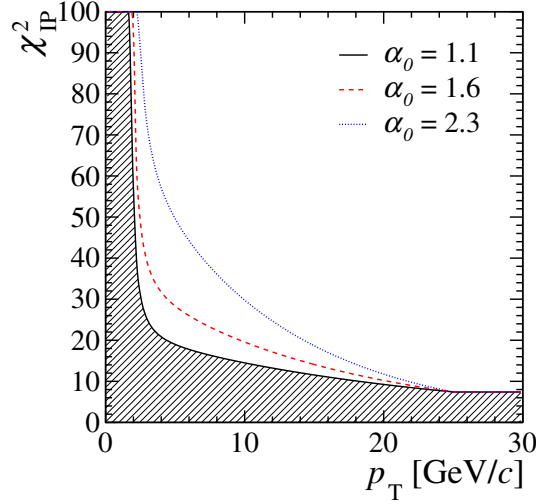
Figure 4.2: Requirement of the single-track line of the first-stage software trigger in the \chi^2_{\text{IP}} vs. p_T plane, for the three values of the parameter \alpha_0 .
