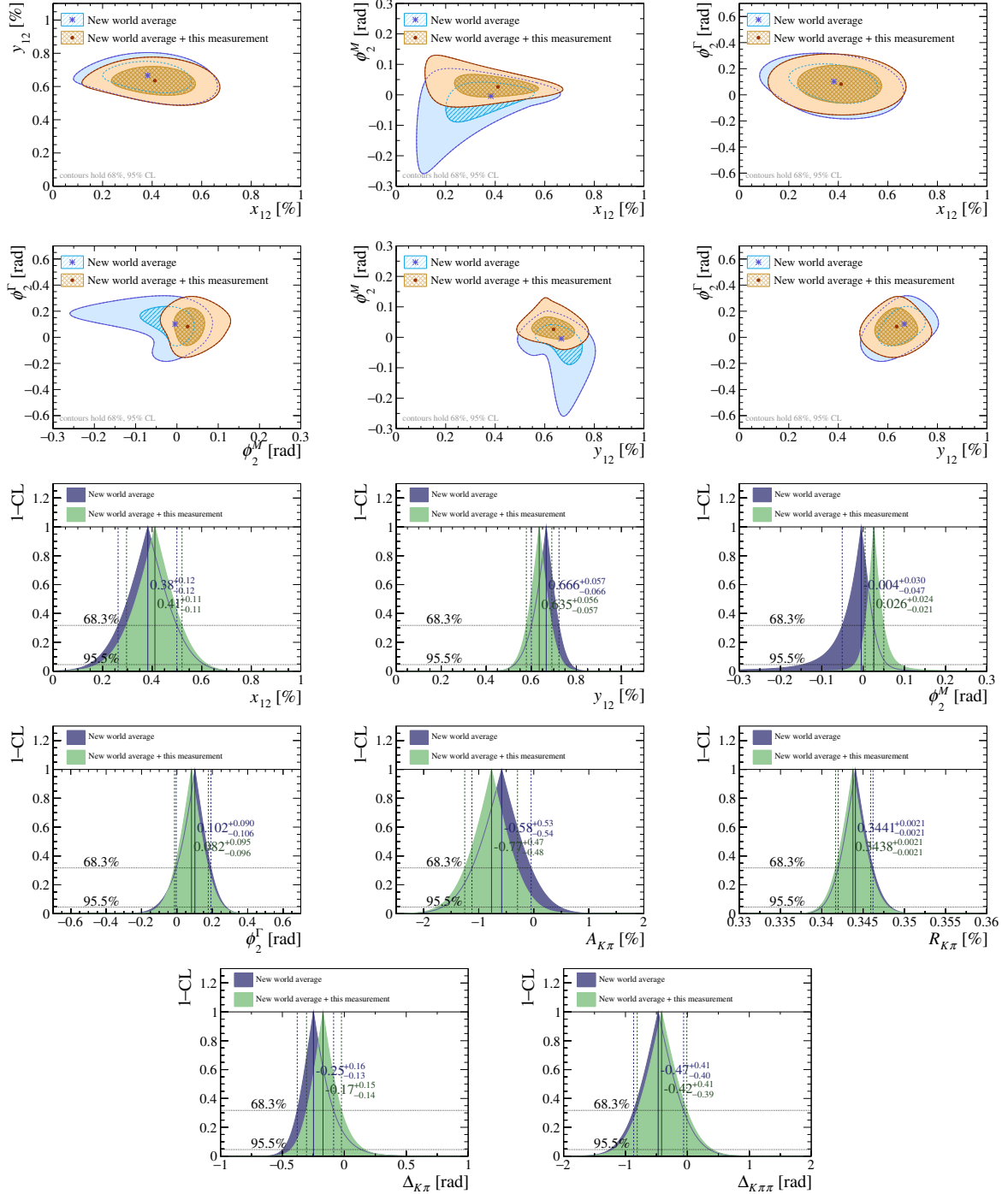
Figure 9.3: Impact of the present measurement on the knowledge of mixing and time-dependent CP violation in D^0 decays, in the theoretical parametrisation. The parameters A_{K\pi} and \Delta_{K\pi} are defined as A_{K\pi} \equiv (R_{K^-\pi^+}^+ - R_{K^-\pi^+}^-)/(R_{K^-\pi^+}^+ + R_{K^-\pi^+}^-) and \Delta_{K\pi} \equiv \Delta_{K^-\pi^+} . The details of the fit performed to obtain these results are reported in Appendix B. The fit has a \chi^2/\text{ndf} equal to 56/42, corresponding to a p-value of 8%.
