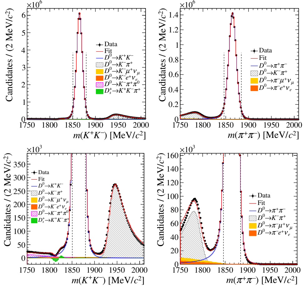
Figure E.5: Template fit to the time-integrated m(h^+h^-) distribution of (left) D^0 \rightarrow K^+K^- and (right) D^0 \rightarrow \pi^+\pi^- decays, where all background normalisations are left free to vary, with the exception of the ratio between the normalisations of D^0 \rightarrow h^-e^+\nu_e and D^0 \rightarrow h^-\mu^+\nu_\mu decays, which is fixed to expectations. Bottom plots are magnified to put the background components in evidence.
