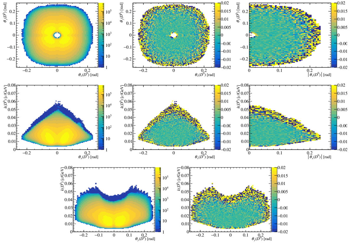
Figure D.7: Two-dimensional distributions and asymmetries of the vector momentum of the D^0 meson, for the full D^0 \rightarrow K^- \pi^+ data sample.
