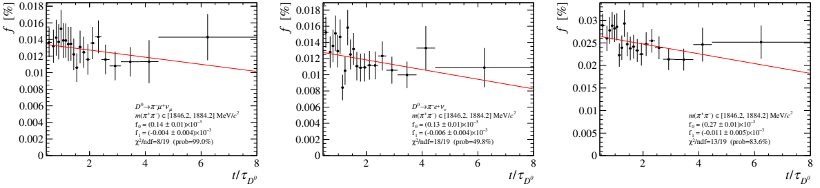
Figure E.8: Linear fit to the time-dependent fraction of background candidates in the m(\pi^+\pi^-) signal region, for all relevant backgrounds components.
