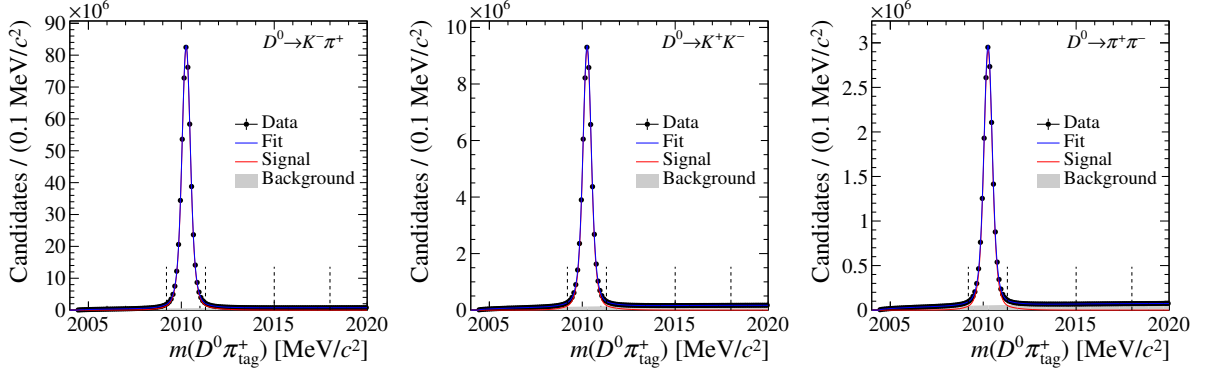
Figure 4.6: Distribution of m(D^0\pi_{\text{tag}}^+) for the (left) K^-\pi^+ , (centre) K^+K^- and (right) \pi^+\pi^- decay channels. The signal window and the lateral window employed to remove the combinatorial background (grey filled area) are delimited by the vertical dashed lines.
