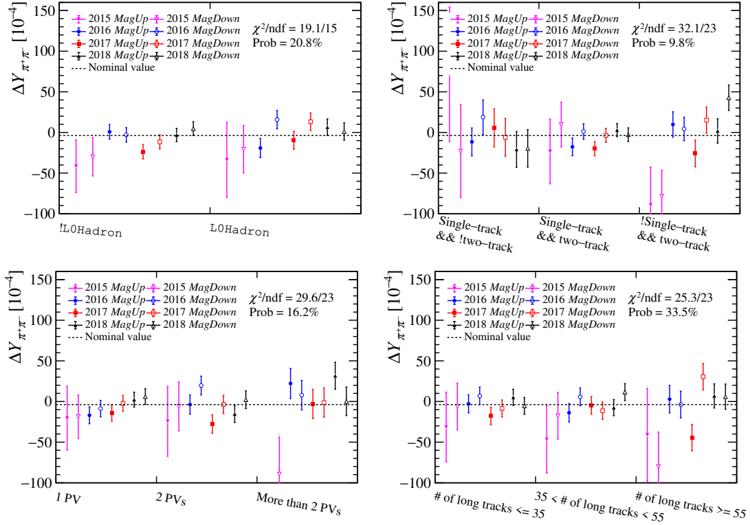
Figure 8.6: Measurements of \Delta Y_{\pi^+\pi^-} performed separately in subsamples corresponding to different trigger requirements and detector occupancies (and, for each subsample, separately for different data-taking years and magnet polarities). The p-value of the dispersion of the measurements around the baseline one is displayed as well.
