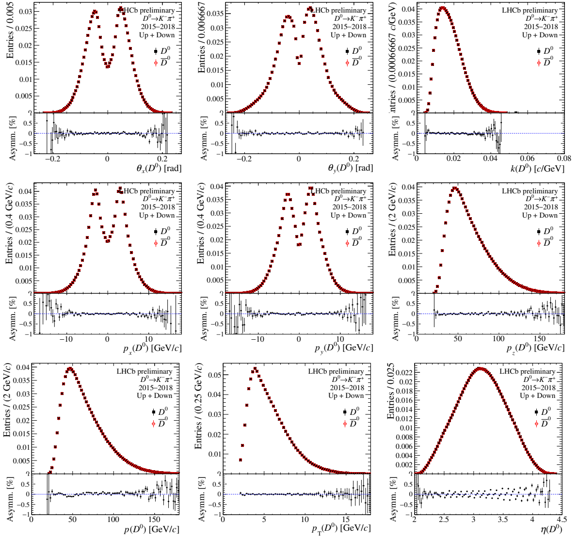
Figure D.8: Distributions and asymmetries of the momentum of the D^0 meson for the full D^0 \rightarrow K^- \pi^+ data sample.
