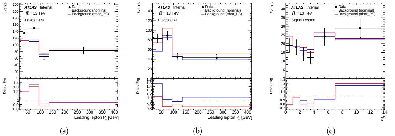
Figure D.2: The expected and observed distributions of the leading lepton p_T in the a) fakes CR with b -veto events, b) fakes CR with one b -tag events and c) \chi^2 variable in the signal region. The blue line is the nominal background and red line is the background with the t\bar{t} NLO generator variation, while black dots are data.
