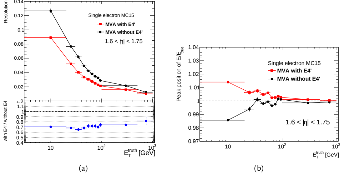
Figure 4.18.: Energy resolution (a) and peak position of E/E_{\text{true}} (b) for electrons as a function of truth transverse energy ( E_T^{\text{truth}} ), comparing the MVA calibration with (red) and without (black) E4' scintillators.
