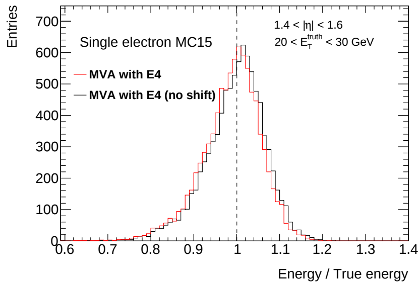
Figure 4.6.: Example of the shift effect for electrons. The distribution of E/E_{\text{true}} is compared before (black) and after (red) the shift.
