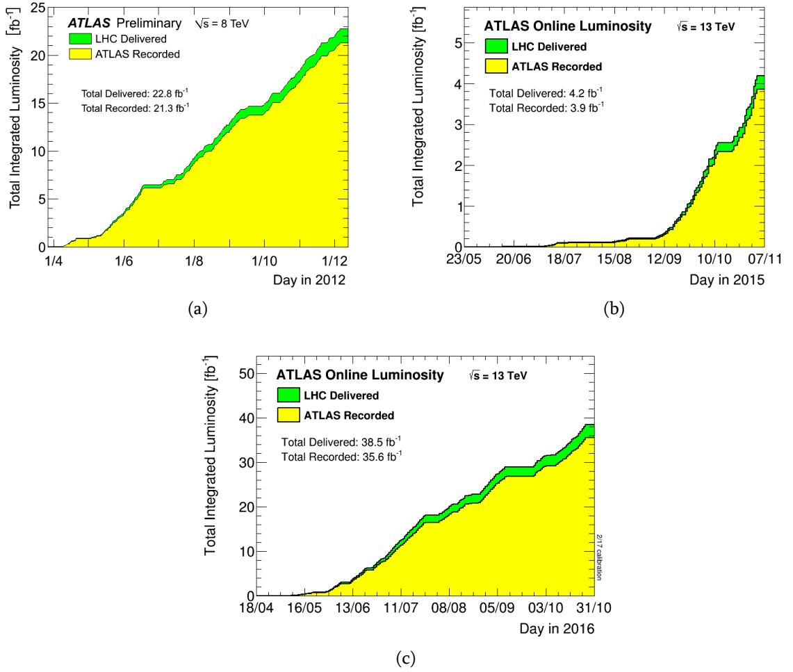
Figure 2.5.: Integrated luminosity versus time delivered by the LHC (green), recorded by ATLAS (yellow), during stable beam conditions for pp collisions at \sqrt{s} = 8 TeV in 2012 (a) and at \sqrt{s} = 13 TeV in 2015 (b) and 2016 (c). Figures are taken from [72] and [73].
