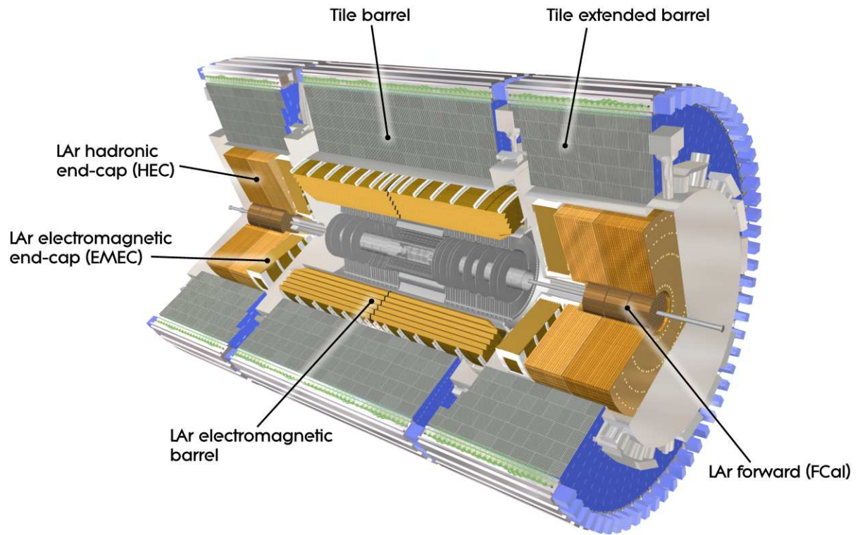
Figure 3.2.: A cut-away drawing of the ATLAS inner detector and calorimeters. Tile Calorimeter consists of one barrel and two extended barrel sections and surrounds the LAr barrel electromagnetic and endcap hadronic calorimeters. Figure is taken from [86].
