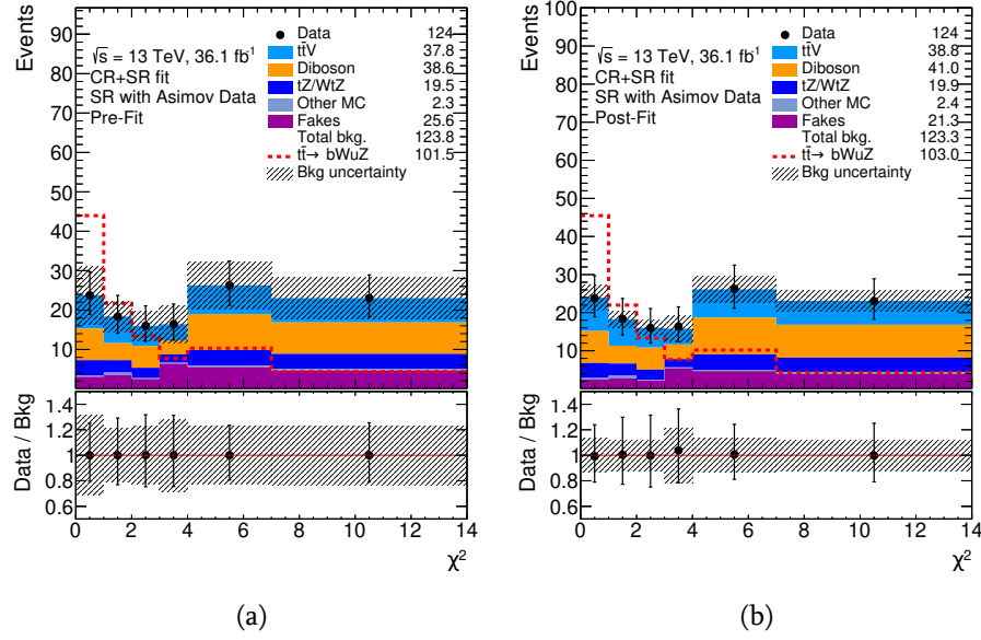
Figure 6.41.: The distributions for the \chi^2 after the event reconstruction in the signal region a) before and b) after the combined fit under the background-only hypothesis. The data points are from the "Asimov dataset", defined as a total expected pre-fit background. The number of signal events is normalized to an arbitrary branching ratio of \text{BR}(t \rightarrow qZ) = 0.1\% . The dashed area represents total uncertainty on the background prediction.
