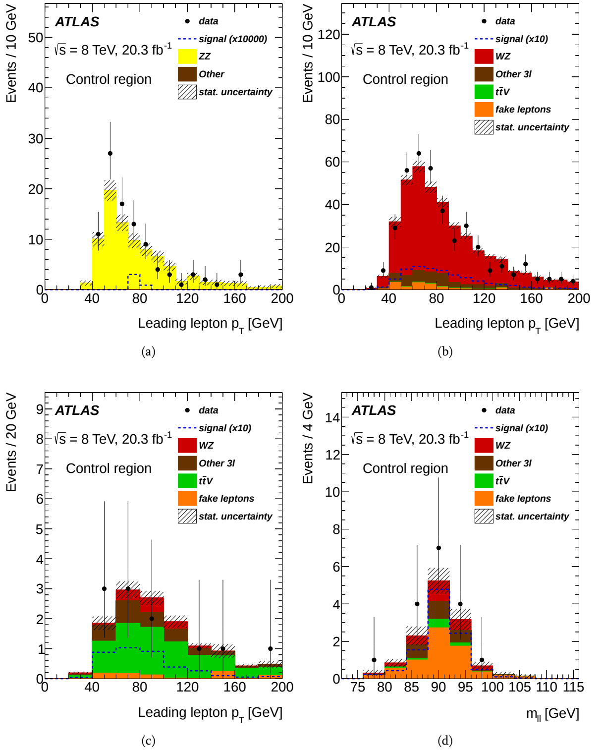
Figure 5.3.: Expected (filled histogram) and observed (points with error bars) distributions for the p_T of the leading lepton in the (a) ZZ , (b) WZ and (c) t\bar{t}Z control regions and (d) reconstructed mass of the two leptons with the same flavour and opposite charge in the fake-lepton control region. For comparison, distributions for the FCNC t\bar{t} \rightarrow bWqZ signal (dashed line), scaled to 10^4 or 10 times the observed 95% CL limit, are also shown. Background statistical uncertainties associated with the number of events in the samples are represented by the hatched areas. Adapted from [2].
