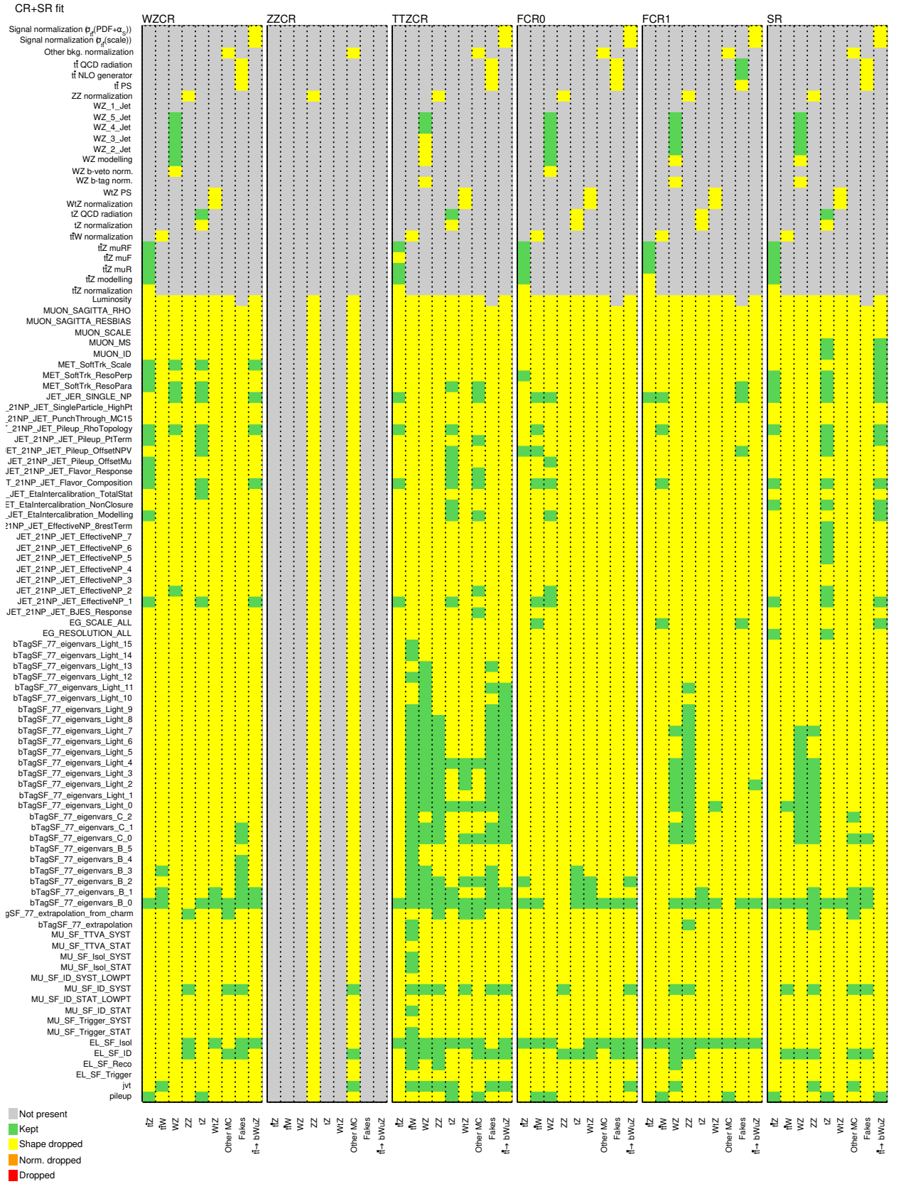
Figure 6.30.: Pruning of the instrumental and modelling systematic uncertainties based on the shape effect for each sample and region in the fit. Pruning algorithm is explained in the text.
