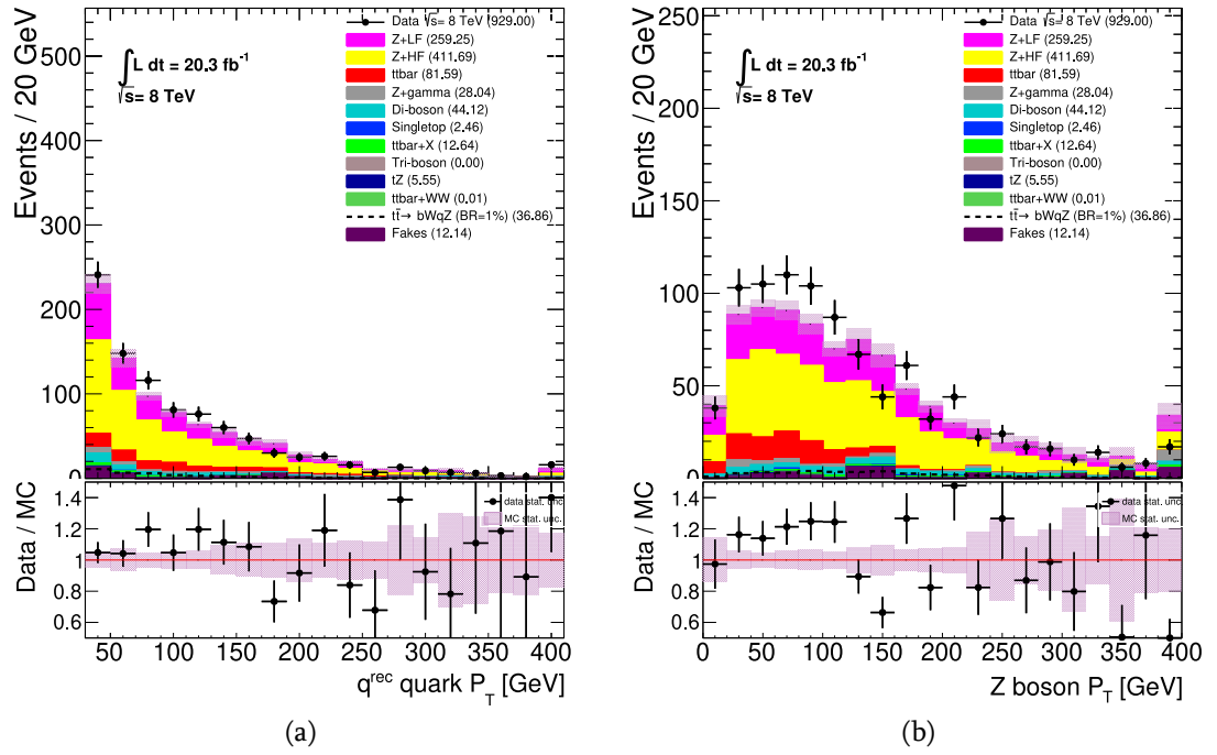
Figure 5.2.: Expected (filled histogram) and observed (points with error bars) distributions for the p_T of the reconstructed a) q -quark and b) Z boson candidates in the Z +HF control region. Background statistical uncertainties associated with the number of events in the samples are represented by the hatched areas.
