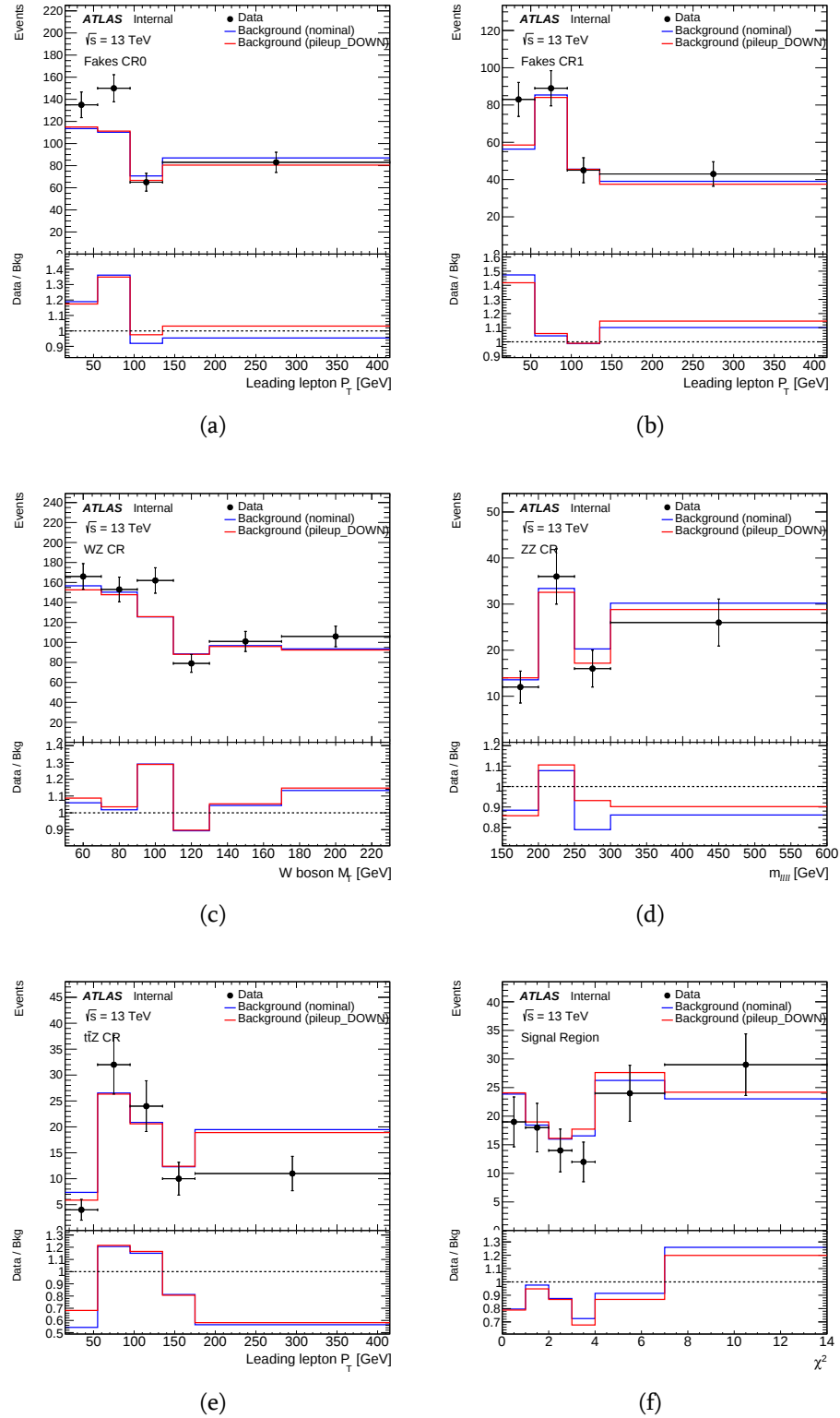
Figure D.5.: The expected and observed distributions of the leading lepton p_T in the a) fakes CR with b -veto events, b) fakes CR with one b -tag events; c) the W boson transverse mass in the WZ CR; d) four lepton system mass in the ZZ CR; e) leading lepton p_T in the t\bar{t}Z CR and f) \chi^2 variable in the signal region. The blue line is the nominal background and red line is the background with down variation of pileup uncertainty, while black dots are data.
