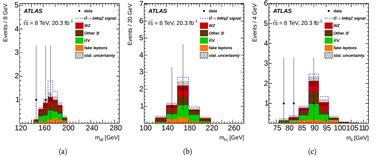
Figure 5.10.: Expected (filled histogram) and observed (points with error bars) distributions in the trilepton signal region for the reconstructed masses of the (a) top quark from the FCNC decay, (b) top quark from the SM decay and (c) Z boson. For comparison, distributions for the FCNC t\bar{t} \rightarrow bWqZ signal (dashed line) normalized to the extracted observed 95% CL limit, are also shown. Background statistical uncertainties associated with the number of events in the samples are represented by the hatched areas. Adapted from [2].
