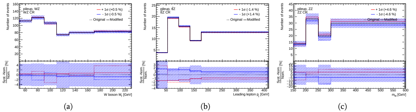
Figure D.8.: The expected distributions (black solid line) of the a) W boson transverse mass in the WZ CR, b) leading lepton p_T in the t\bar{t}Z CR and c) four leptons system mass in the ZZ CR for the WZ , t\bar{t}Z and ZZ background contributions respectively. The dashed red and blue lines represent the \pm 1\sigma variation of pileup systematic uncertainty, while solid red and blue lines show corresponding distributions after applying smoothing algorithm as implemented in the TRExFitter package. The dashed area represents the statistical uncertainty.
