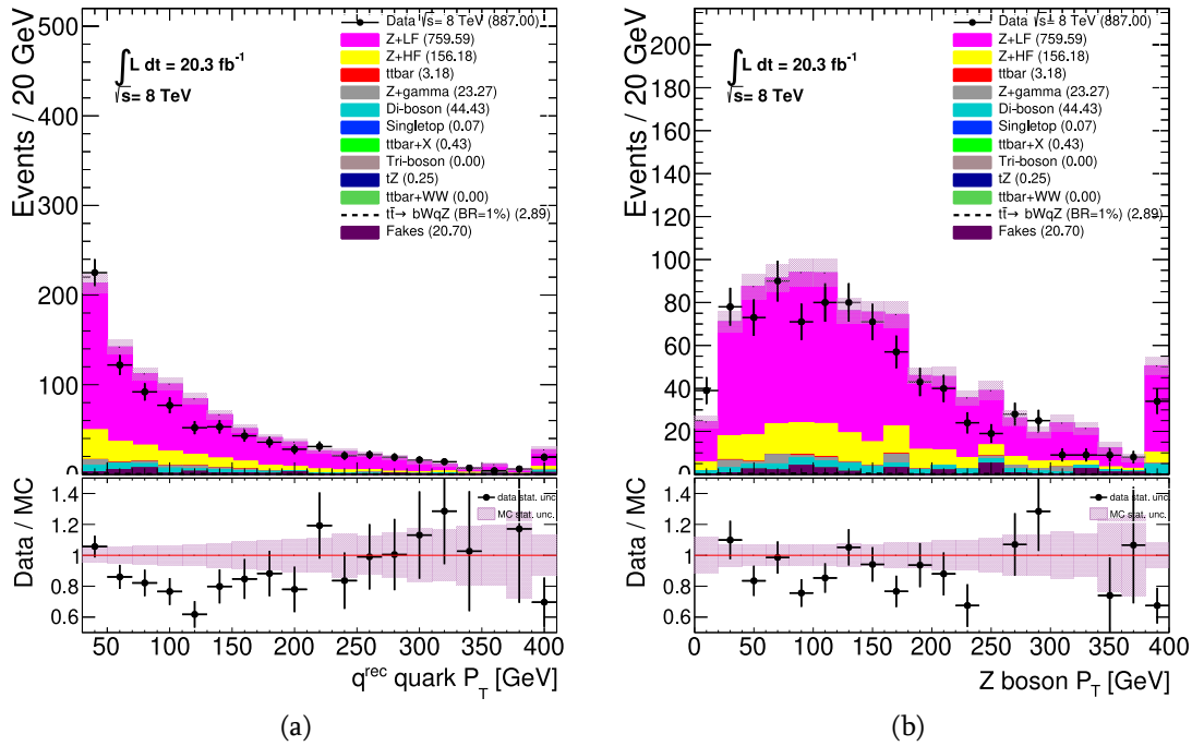
Figure 5.1.: Expected (filled histogram) and observed (points with error bars) distributions for the p_T of the reconstructed a) q -quark and b) Z boson candidates in the Z +LF control region. Background statistical uncertainties associated with the number of events in the samples are represented by the hatched areas.
