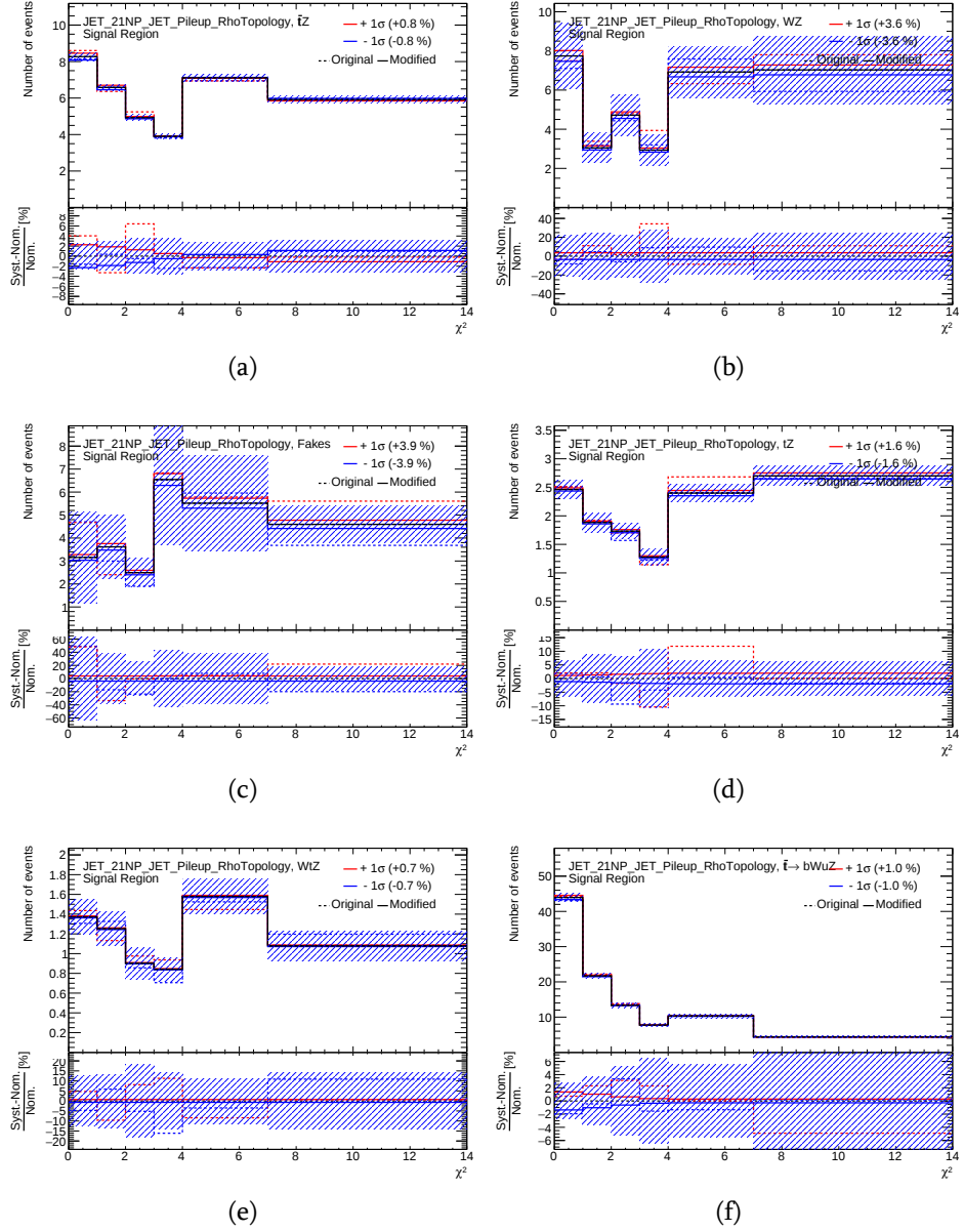
Figure D.10.: The expected distributions (black solid line) of the \chi^2 variable in the signal region for a) t\bar{t}Z , b) WZ , c) Fakes, d) tZ , e) WtZ and d) signal sample. The dashed red and blue lines represent the \pm 1\sigma variation of JET_21NP_JET_Pileup_RhoTopology systematic uncertainty, while solid red and blue lines show corresponding distributions after applying smoothing algorithm as implemented in the TRExFitter package. The dashed area represents the statistical uncertainty.
