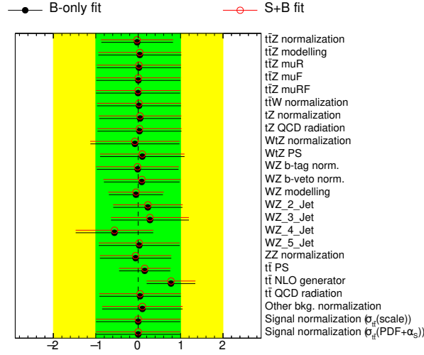
Figure 6.33.: Fitted nuisance parameters corresponding to the theoretical and modelling uncertainties under the background-only hypothesis (black closed circles) and under the signal-plus-background hypothesis (red open circles) in the background control and signal regions. In the signal region "Asimov data" is used, defined as the total expected pre-fit background.
