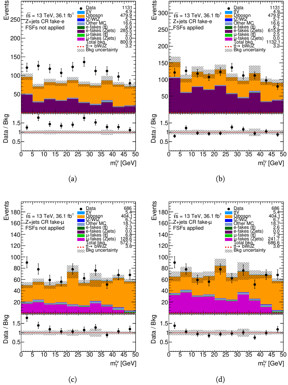
Figure 6.28.: Expected and observed distributions of the transverse mass m_T^{\ell\nu} in the Z+jets CR with fake electron (a,b) and with fake muon (c,d) before (left) and after (right) applying the fake scale factors. The number of signal events is normalized to the expected 95% CL limit. The dashed area represents statistical uncertainty on the background prediction.
