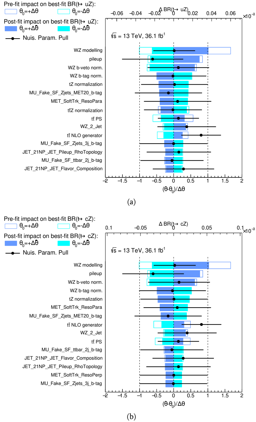
Figure 6.44.: The fitted values of the 15 most important nuisance parameters and their impact on the measured branching ratio of a) t \rightarrow uZ and b) t \rightarrow cZ are presented. The black points, which are plotted according to the bottom horizontal scale, show the deviation of each of the fitted nuisance parameters, \hat{\theta} , from \theta_0 , which is the nominal value of that nuisance parameter, in units of the pre-fit standard deviation \Delta\theta . This represents the preferred shift of the event yield with respect to the nominal prediction in units of its prior uncertainty. The black error bars show the post-fit errors, \sigma_{\theta} , which represent the post-fit uncertainty on the event yield in units of the prior uncertainty. The nuisance parameters are sorted according to the post-fit effect of each on the best-fit branching ratio, with those with the largest impact at the top. The post-fit effect on the best-fit branching ratio, shown according to the top horizontal scale, is calculated by fixing the corresponding nuisance parameter at \hat{\theta} \pm \sigma_{\theta} and redoing the fit.
