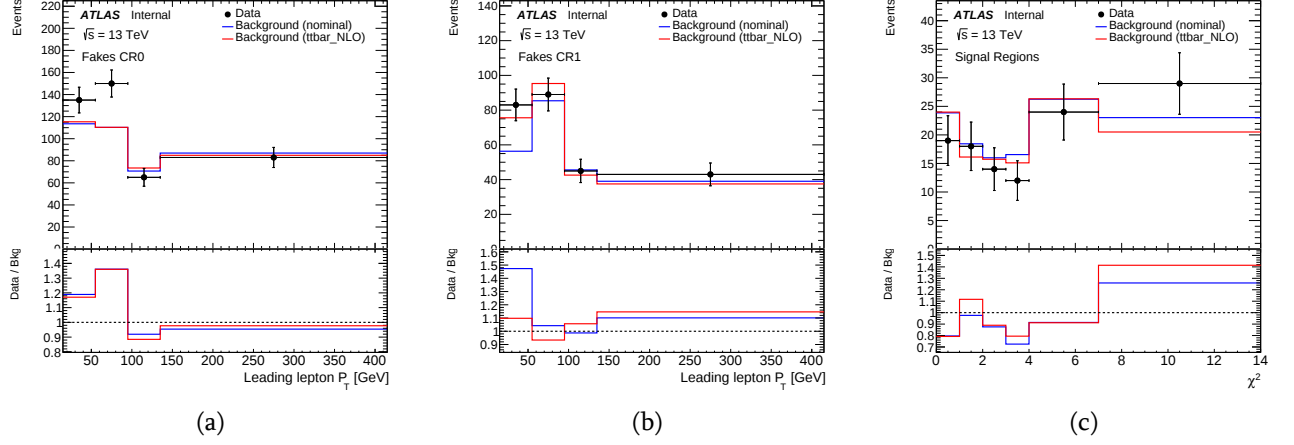
Figure D.1: The expected and observed distributions of the leading lepton p_T in the a) fakes CR with b -veto events, b) fakes CR with one b -tag events and c) \chi^2 variable in the signal region. The blue line is the nominal background and red line is the background with the t\bar{t} Parton Showering variation, while black dots are data.
