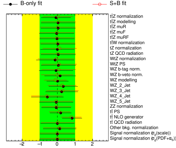
Figure 6.52.: Fitted nuisance parameters corresponding to the theoretical and modelling uncertainties under the background-only hypothesis (black closed circles) and under the signal-plus-background hypothesis (red open circles) in the background control and signal regions with unblinded data.
