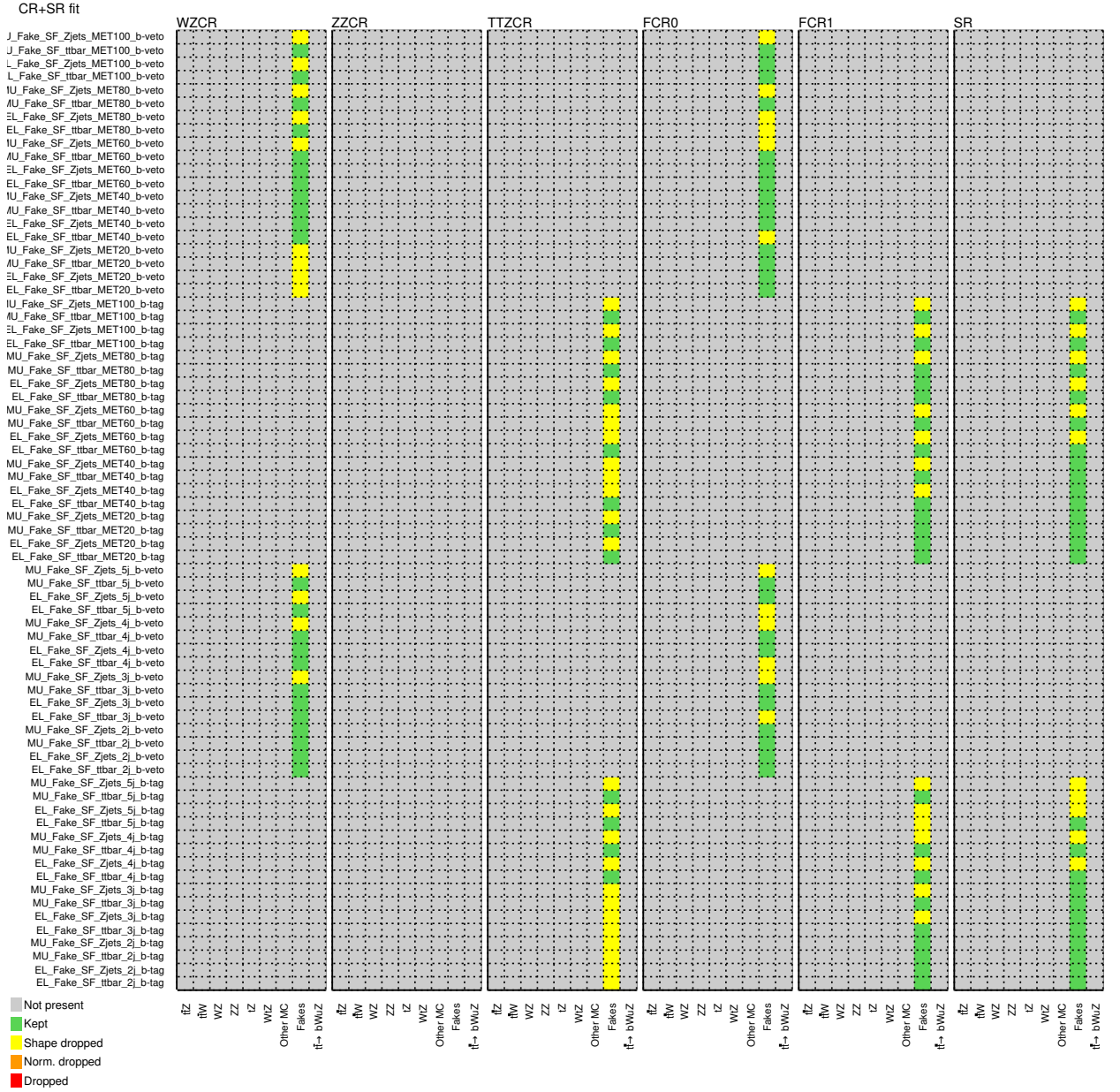
Figure 6.31.: Pruning of the instrumental and modelling systematic uncertainties based on the shape effect for each sample and region in the fit. Pruning algorithm is explained in the text.
