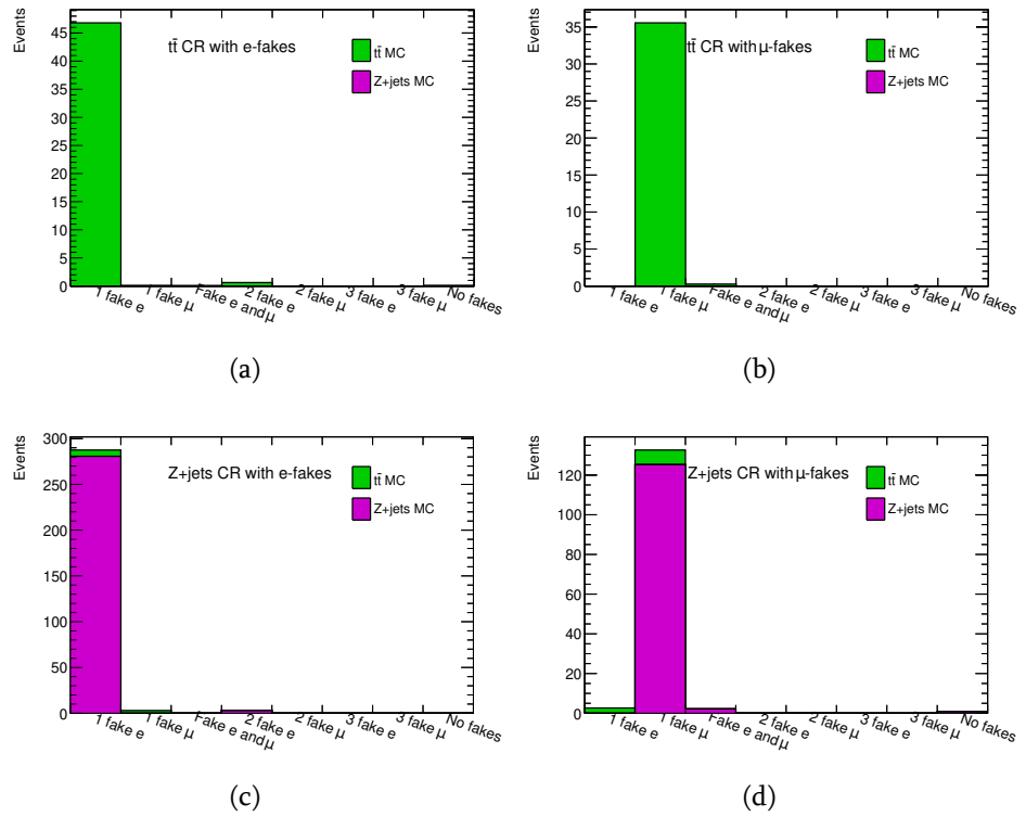
Figure C.1.: The number of fake-leptons in the Z +jets and t\bar{t} MC events in the a) t\bar{t} CR with e-fakes, b) t\bar{t} CR with \mu -fakes, c) Z +jets CR with e-fakes and d) Z +jets CR with \mu -fakes.
