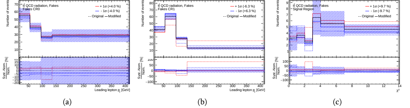
Figure D.18.: The expected distributions (black solid line) of the leading lepton p_T in the fakes control region with a) b -veto events and with b) one b -tag events, and c) the \chi^2 variable in the signal region for the fake-lepton background contribution. The dashed red and blue lines represent the variations obtained by considering alternative sample with additional QCD radiation for the t\bar{t} sample (see Section 6.8). The solid red and blue lines show corresponding distributions after applying smoothing algorithm as implemented in the TRExFitter package. The dashed area represents the statistical uncertainty.
