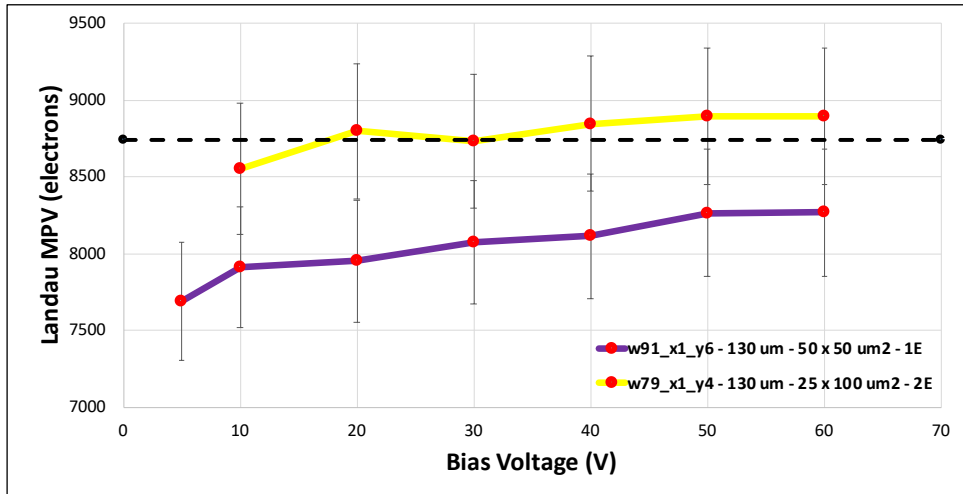
Figure 4.47: Collected charge MPV as a function of the bias voltage for two non-irradiated 3D sensors with small pitch. The sensor thickness is 130\text{ }\mu\text{m} and the pixel size are 25 \times 100\text{ }\mu\text{m}^2 and 50 \times 50\text{ }\mu\text{m}^2 . The horizontal dashed line indicates the expected value.
