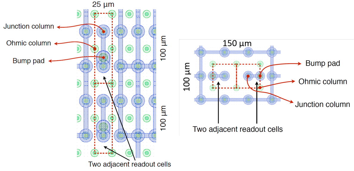
Figure 4.4: Layout of the 25 \times 100 \mu\text{m}^2 (left figure) and 50 \times 50 \mu\text{m}^2 (right figure) pixel cells. Only the cells pointed by the black arrows are readout. The blue layer represents a metallization grid need to short-circuit the pixels that are not readout. The Ohmic columns are shown in light green at the periphery of the cells.
