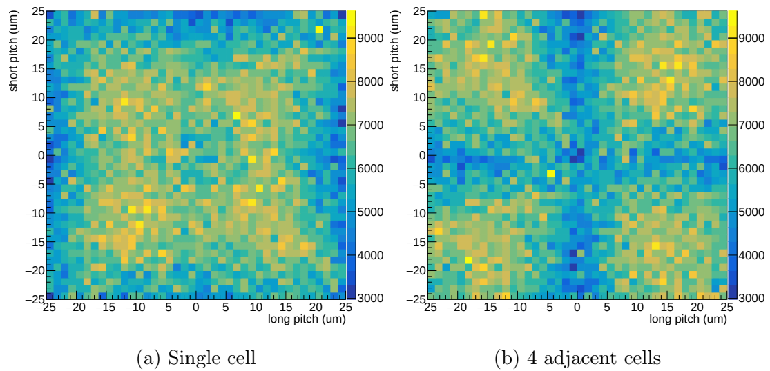
Figure 4.65: Maps of the charge collected by sensor w91_x2y3 at a bias voltage of 128 V.
