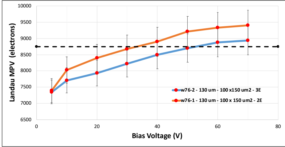
Figure 4.46: Collected charge MPV as a function of the bias voltage for two non-irradiated 3D sensors, one with two junction columns (2E), the other with three (3E). The sensor thickness is 130\text{ }\mu\text{m} and the pixel size is 100 \times 150\text{ }\mu\text{m}^2 . The horizontal dashed line indicates the expected value.
