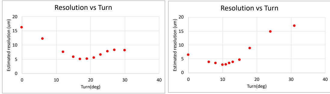
(a) Sensor 1 ( 50 \times 50 \mu m^2 , 130 \mu m active thickness) (b) Sensor 2 ( 25 \times 100 \mu m^2 , 130 \mu m active thickness)
