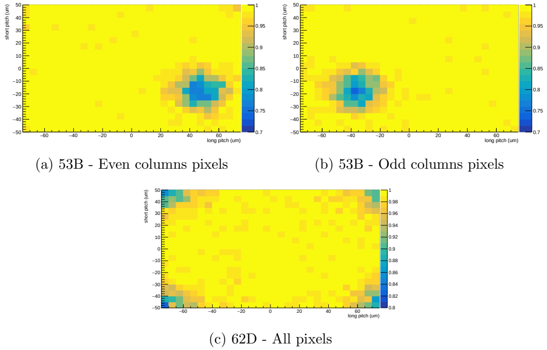
Figure 4.37: Maps of the particle detection efficiency within the pixel cells of the sensors irradiated at the smallest and the intermediate fluence (see Fig. 4.35) at a bias of 500 V and 800 V respectively. The sensor irradiated at intermediate fluence does not have punch-through structures so a cumulative efficiency for odd and even columns pixels is reported.
