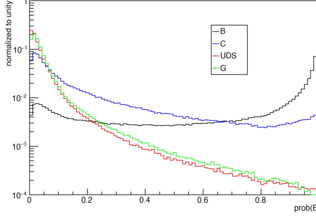
Figure 5.11: Distribution of the DeepFlavour bb+b+lep discriminator value for jets of different flavours in t\bar{t} events.
