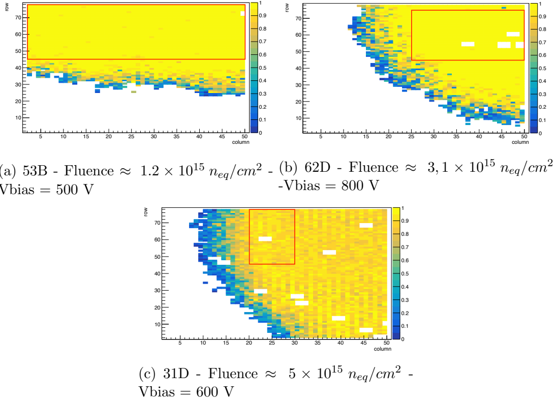
Figure 4.33: Efficiency maps of three irradiated sensors. Pixels selected in the analysis are contoured by a red box.
