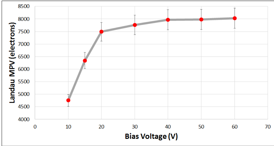
Figure 4.20: MPV of the collected charge as a function of the bias voltage for the 53B planar sensor.
