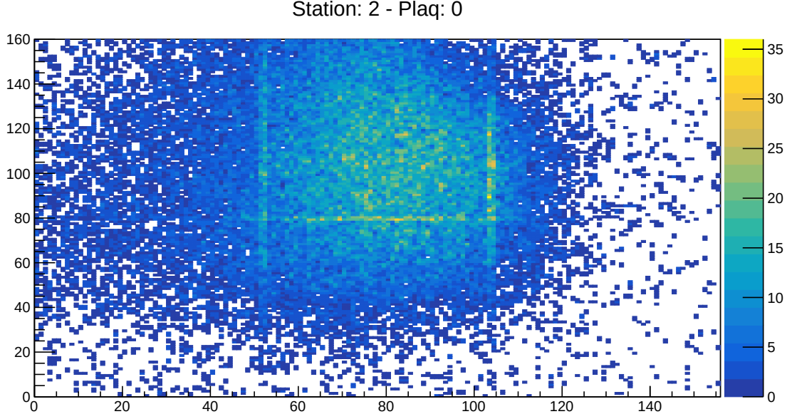
Figure 3.7: Beam spot on one of the telescope detectors.
