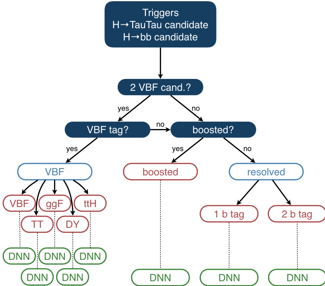
Figure 5.19: Description scheme of event categorization and discriminating variables used in each category. Events in the VBF category are split accordingly to the "most probable process" predicted by the multiclass neural network. In the green boxes, "DNN" represents the Gluon Fusion optimized DNN score which is used for signal extraction both in the GGF and in the VBF categories.
