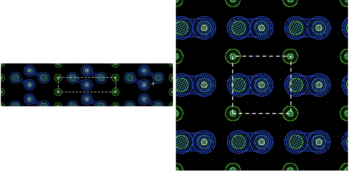
Figure 4.6: Layout of the pixel cells of a 25 \times 100 \mu m^2 1E (left figure) and 50 \times 50 \mu m^2 (right figure) sensors bonded to the RD53A ROC. A single cell is highlighted.
