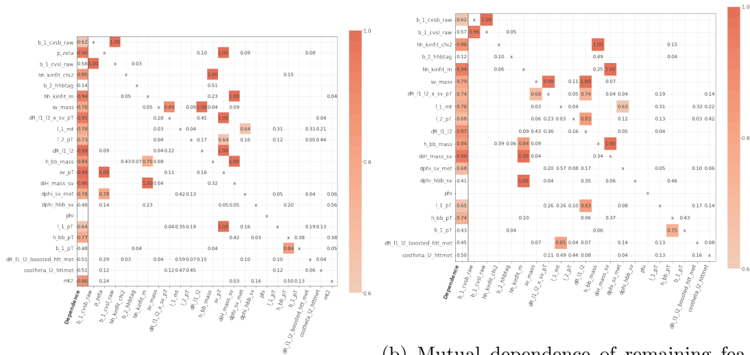
(a) Mutual dependence of features prior to filtering. (b) Mutual dependence of remaining features after filtering. Some remaining features display mutual dependence, however they cannot be safely removed.
