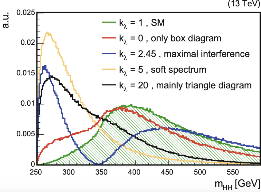
Figure 5.5: Comparison of the m_{HH} distribution for different values of k_\lambda .
