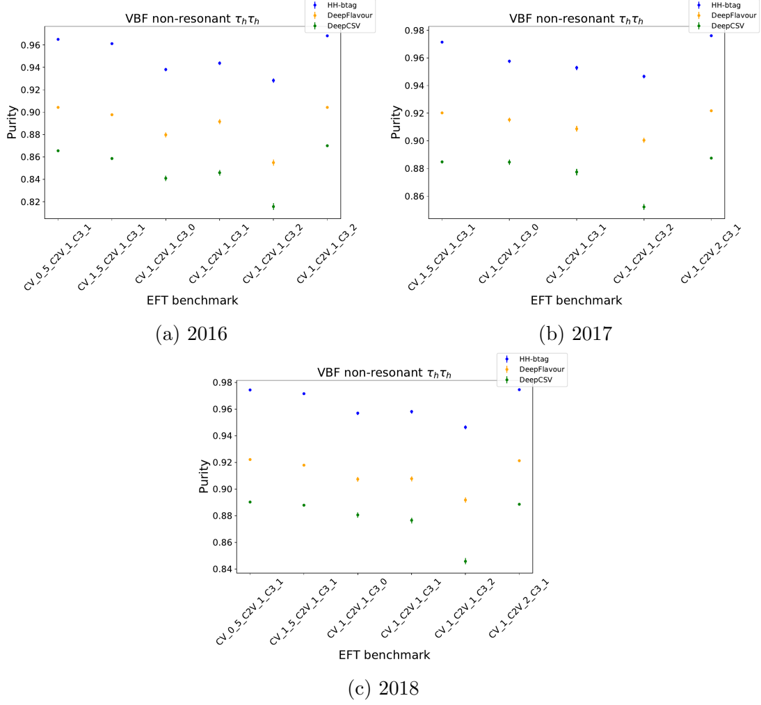
Figure 5.16: Purity distributions for the VBF di-Higgs production in the \tau_h \tau_h channel, using the HH-Btag, DeepFlavour and DeepCSV discriminators
