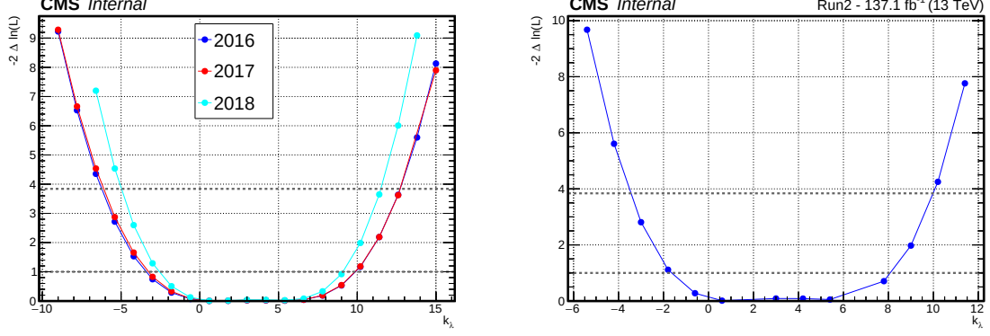
Figure 5.42: Expected likelihood scan as a function of k_\lambda . The plot on the left shows the result split for the three years, while the plot on the right represents the combination of the full Run 2.
