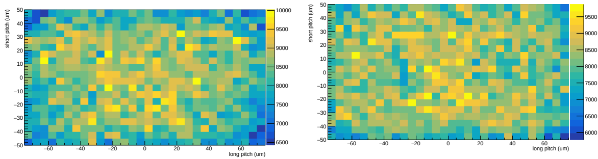
Figure 4.21: Collected charge as a function of the track impact point position on the pixel cells of the 43B and 45B sensors at bias voltage of 40 V.
