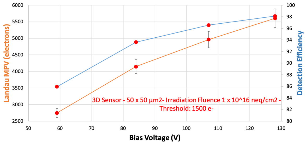
Figure 4.66: Collected charge MPV and decetion efficiency of sensor w91_x2y3 as a function of the bias voltage.
