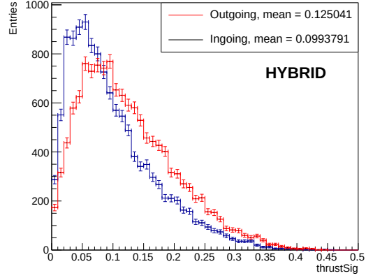
(b) Thrust for the ingoing and outgoing jets in the Hybrid sample. The outgoing jets have 13160 entries and the ingoing jets have 12356 entries.
