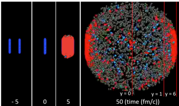
Figure 2: Formation of a QGP at different stages (white vertical lines) of a Pb-Pb collision with an energy of 2.76 TeV per nucleon. The time is given in fm/c. The blue and grey dots denote hadrons, and the red dots denote QGP. Figure adapted from [13].
