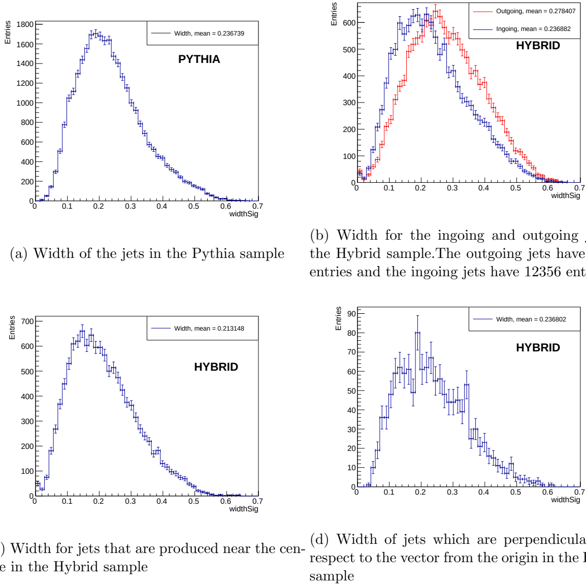
Figure 16: Histograms of jet widths in different cases
