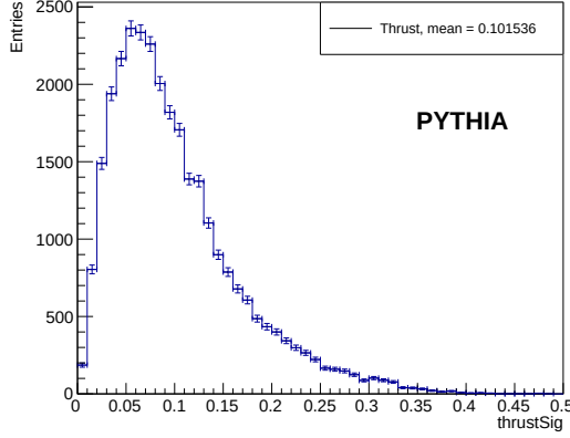
(a) Thrust of the jets in the Pythia sample
