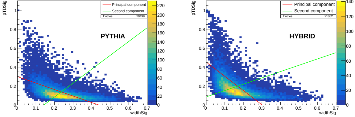
(a) The slope of the PC is -0.684 with eigenvalue 0.0140 . The slope of the second component is 1.463 with eigenvalue 0.00397 . (b) The slope of the PC is -1.498 with eigenvalue 0.0181 . The slope of the second component is 0.667 with eigenvalue 0.00505 .
