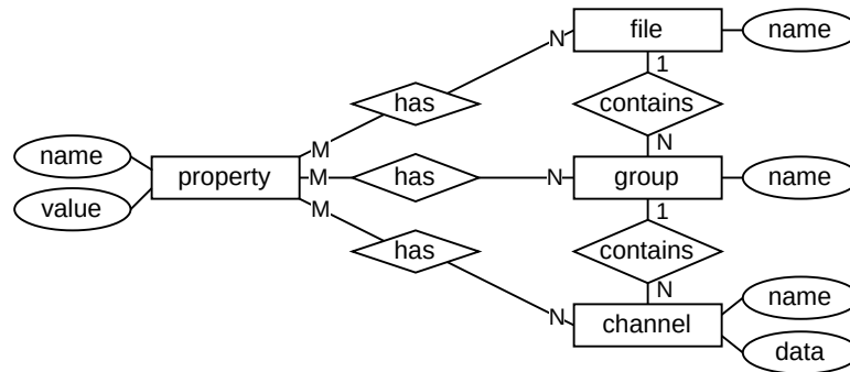
Figure 17: Entity relationship diagram of tdms files
