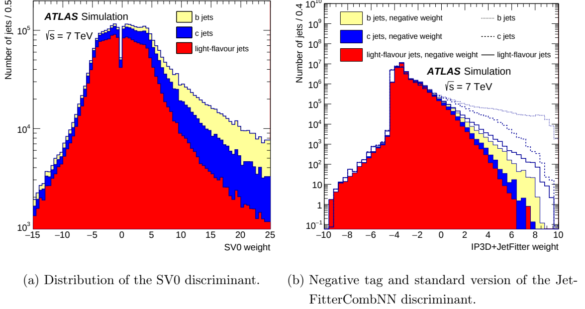
Figure 5.9.: The JetFitterCombNN discriminant on the right changes due to the negative tag weighting in the input variables [64].
