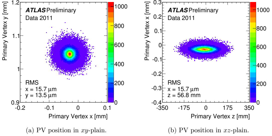
Figure 3.1.: Reconstructed primary vertex position in 2011 data with \sqrt{s} = 7 \text{ TeV} [40]. Here a 400 MeV track cut is used. These plots are updates to [38].
