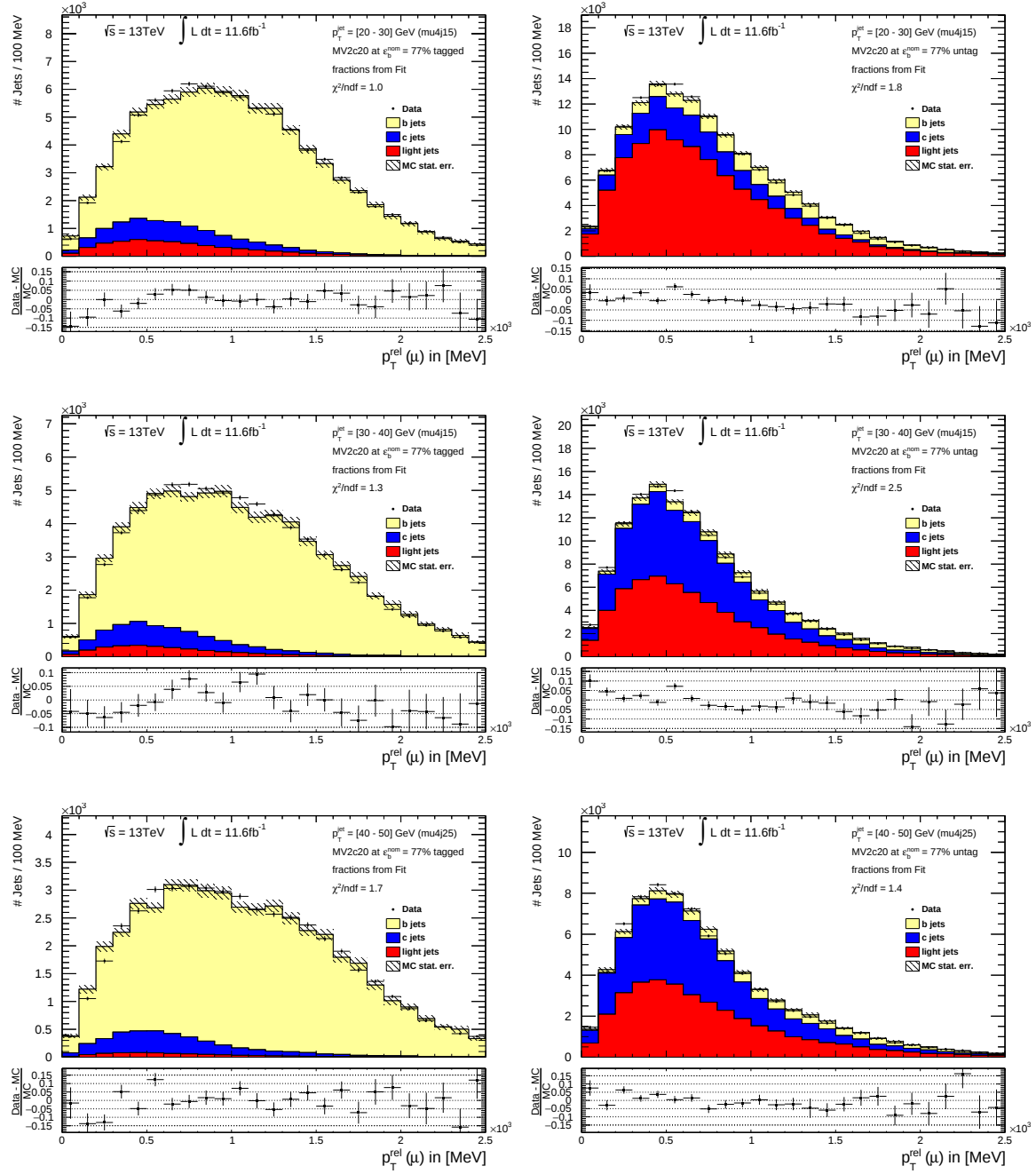
Figure A.3.: Distributions of p_T^{\text{rel}} using b -tagged jets (left) and untagged jets (right). The black dots show the data while the templates are shown as a colored stack. The flavor fractions have been determined by the log-likelihood fit.
