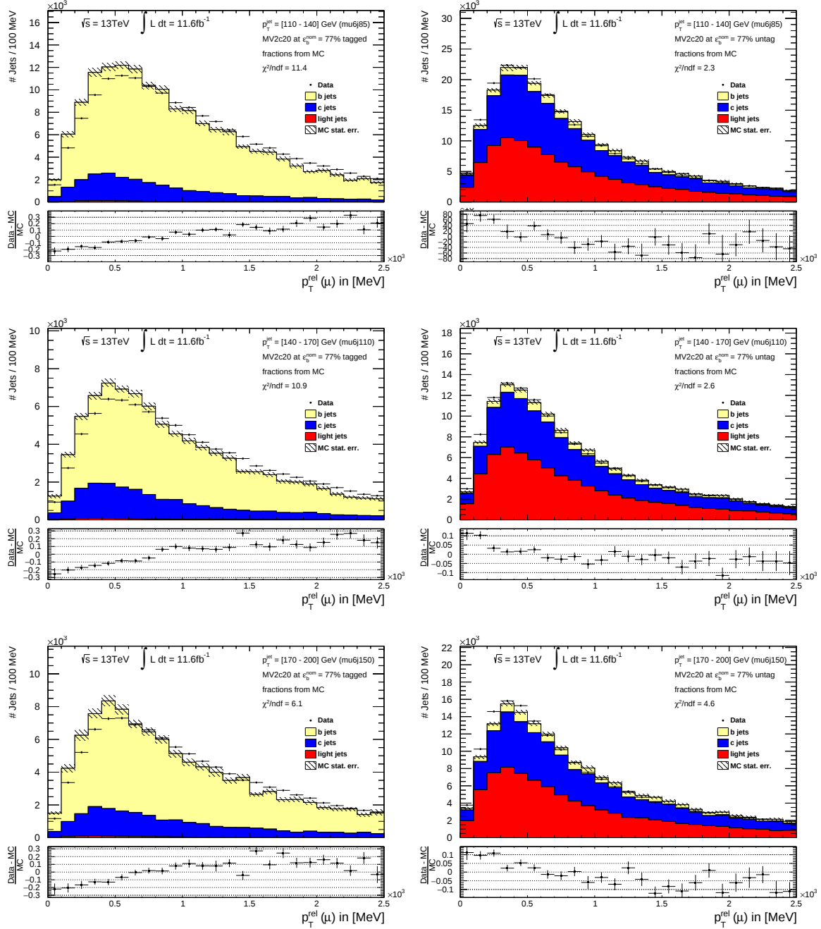
Figure A.8.: Distributions of p_T^{\text{rel}} using b -tagged jets (left) and untagged jets (right). The black dots show the data while the templates are shown as a colored stack. The flavor fractions have been extracted from simulation.
