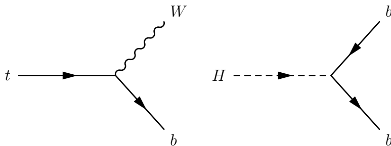
Figure 1.4.: Feynman diagrams for b -quarks produced in decays of t -quarks (left) or Higgs-bosons (right).
