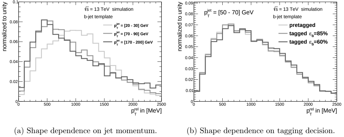
Figure 7.5.: Templates for b -jets in different p_T^{\text{jet}} -regions shown in different shades of gray (left) show a clear momentum dependence. The b -templates show no dependence on the tagging decision (right).
