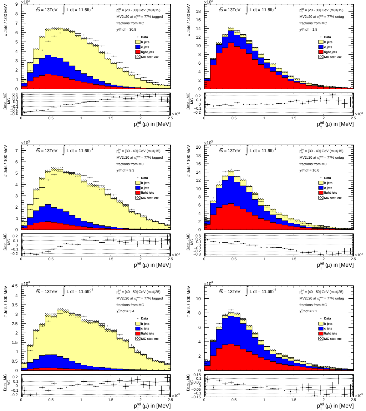
Figure A.6.: Distributions of p_T^{\text{rel}} using b -tagged jets (left) and untagged jets (right). The black dots show the data while the templates are shown as a colored stack. The flavor fractions have been extracted from simulation.
