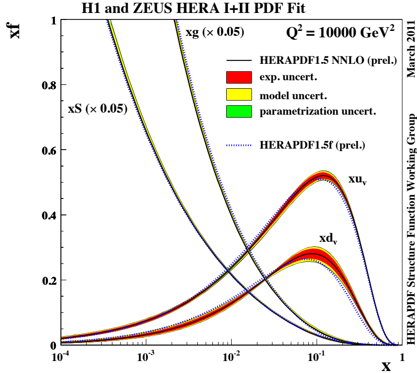
Figure 1.3.: The parton distribution functions from HERAPDF1.5 is shown at an momentum transfer of Q = 100 \text{ GeV} [13]. The contribution of the valence quarks is shown as xd and xu . The gluon and sea contributions are scaled down by a factor of 20 and labeled xg and xS respectively.
