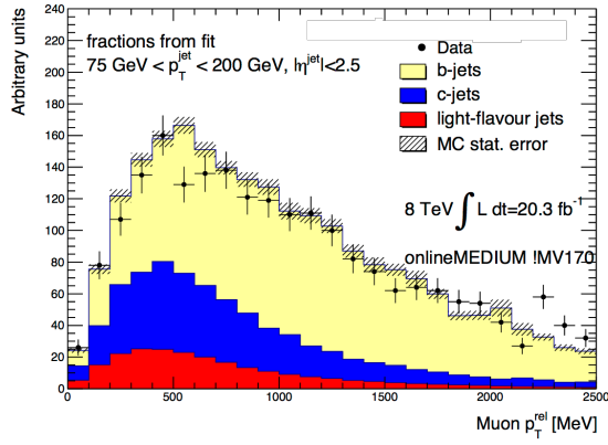
(a) Fit to the \text{trig}|\overline{\text{tag}} -distribution.
