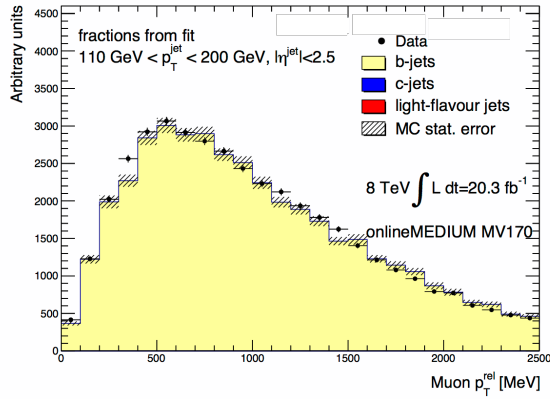
(c) Fit to the \text{trig}|\text{tag} -distribution.
