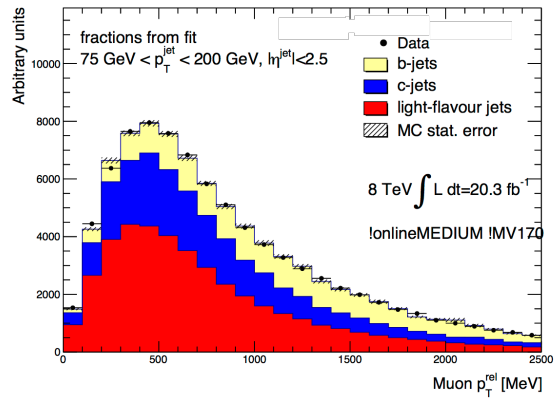
(b) Fit to the \overline{\text{trig}}|\text{tag} -distribution.
