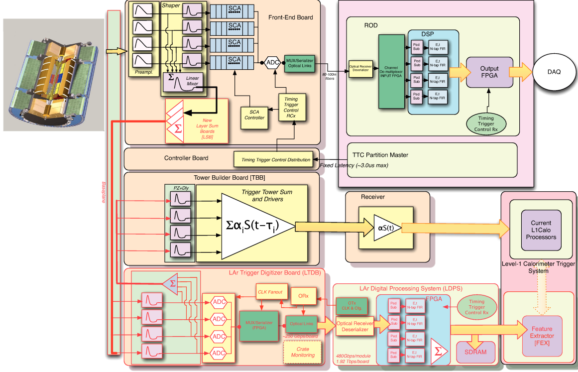
Figure 3.8: Schematic block diagram of the LAr electronics after the Phase 1 upgrade. The first line of blocks corresponds to the standard readout electronic chain. The second line of blocks corresponds to the legacy trigger system based on Trigger Towers. Finally, the last line of blocks corresponds to the new Digital Trigger electronics. Elements affected by the Phase 1 upgrade are marked by red outlines and arrows. From Ref. [57].
