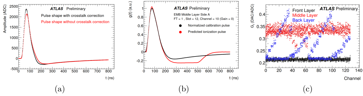
Figure 3.5: (a) Pulse shape from a LAr front layer cell reconstructed in delay runs with (black) and without (red) cross-talk correction.
