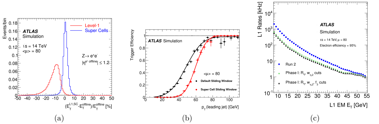
Figure 3.7: (a) Energy resolution on electrons from Z \rightarrow ee computed with Trigger Towers (labelled Level-1, in red) and with Super Cells (in blue) as simulated with Run 3 pile-up conditions \langle\mu\rangle = 80 .
