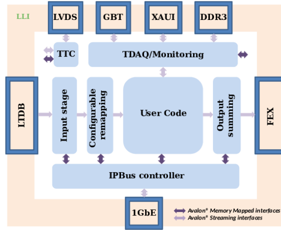
Figure 3.11: Block diagram of the LATOME Firmware. The pale brown frame represents the interface with the hardware. The inner pale blue boxes are functional blocks of the firmware. From Ref. [64].
