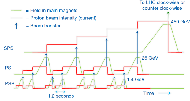
Figure 2.3: Filling and acceleration scheme of the LHC, from the Proton-Synchrotron Boosters (PSB) through the Proton-Synchrotron (PS) and the Super-Proton-Synchrotron (SPS) before sending to the LHC. From Ref. [47].
