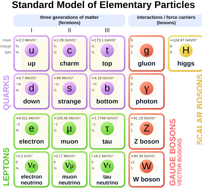
Figure 1.1: The Standard Model particles.
