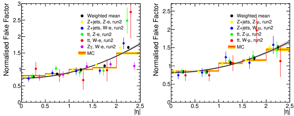
Figure 6.4: Fit of a parabolic function to the weighted mean (black dot) of normalised Fake Factors in bins of |\eta| from the different control regions and for W -leptons and Z -leptons. Electrons and muons are treated separately and displayed on the left and right, respectively. For the representation, x -values of Fake Factors from different control regions (coloured dots) are displaced inside the bin. The shaded band around the fit result displays its 68 % confidence interval. Total uncertainties are displayed.
