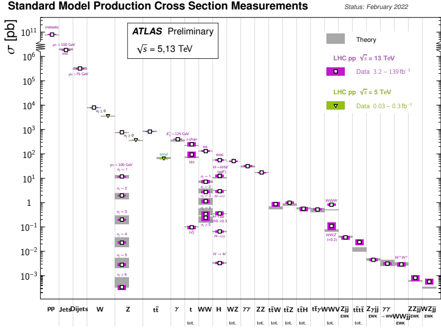
Figure 1: Summary of several Standard Model total and fiducial production cross-section measurements from Run 2 data, corrected for branching fractions, compared to the corresponding theoretical expectations. From Ref. [4].
