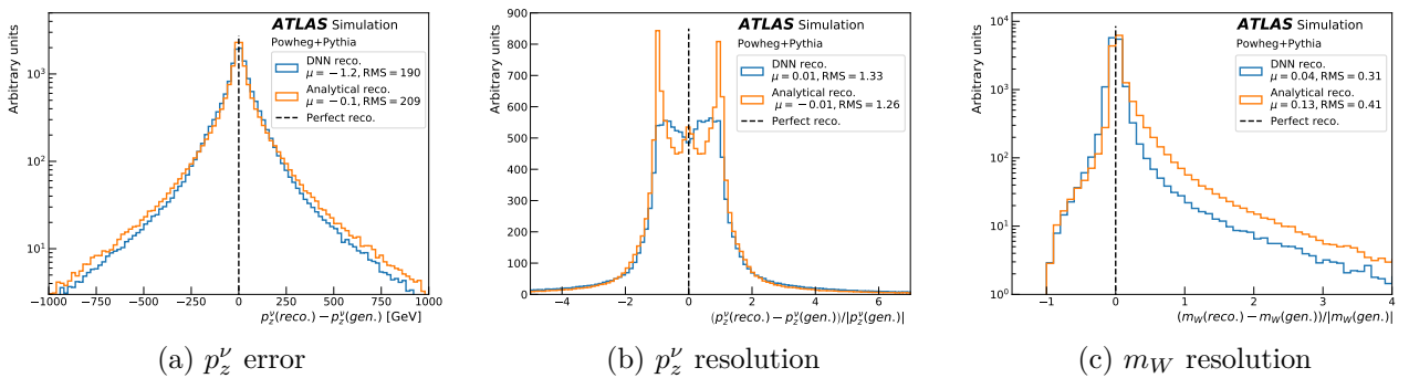
Figure 6.1: Error on p_z^\nu (a), resolution of p_z^\nu (b) and resolution of m_W (c) as reconstructed by the regression DNN (blue) and analytical method (orange). In the legend, \mu notes the mean value and RMS (Root Mean Square) is the standard deviation.
