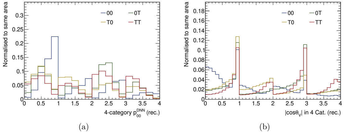
Figure 7.5: All four MGgen joint-polarisation templates for W^\pm Z events with the 4-category p_{00}^{\text{DNN}} (a) and the 4-category |\cos \theta_V| (b) as discriminating variable are represented at detector level. These templates were all rescaled to the same surface area.
