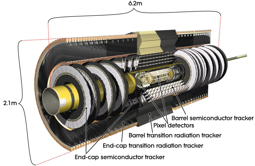
Figure 2.9: The Inner Detector. From Ref. [42].
