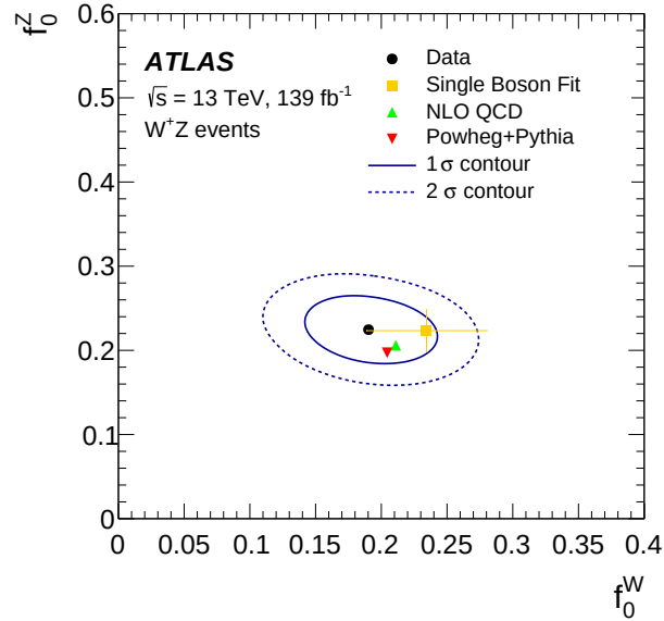
Figure D.3: Measured polarisation fractions f_0^W and f_0^Z in W^+Z events. The black point is the simultaneously measured values from the template fit on the 4-category DNN score distribution. The orange square with uncertainty bars is the measured value from two single boson polarisation template fits to q_W \cdot \cos \theta_{\ell W}^* and \cos \theta_{\ell Z}^* distributions. The red triangle is the theoretical predictions at NLO in QCD and LO for the electroweak interaction from POWHEG+PYTHIA. The solid and dashed ellipses around the data points correspond to one and two standard deviations to the joint measurement of f_0^W and f_0^Z , respectively.
