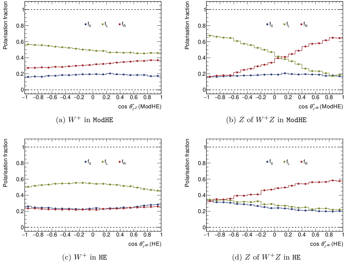
Figure 5.5: Polarisation fractions of W^\pm boson (left) and Z boson (right) in W^+Z events in bins of the \cos \theta_\ell^* of the other boson ( \cos \theta_{\ell Z}^* left, \cos \theta_{\ell W}^* right) extracted from POWHEG+PYTHIA at the particle level in the total phase space. The top plot have the \cos \theta_\ell^* defined in the Modified Helicity frame (ModHE), the bottom plot have the \cos \theta_\ell^* defined in the Helicity frame (HE).
