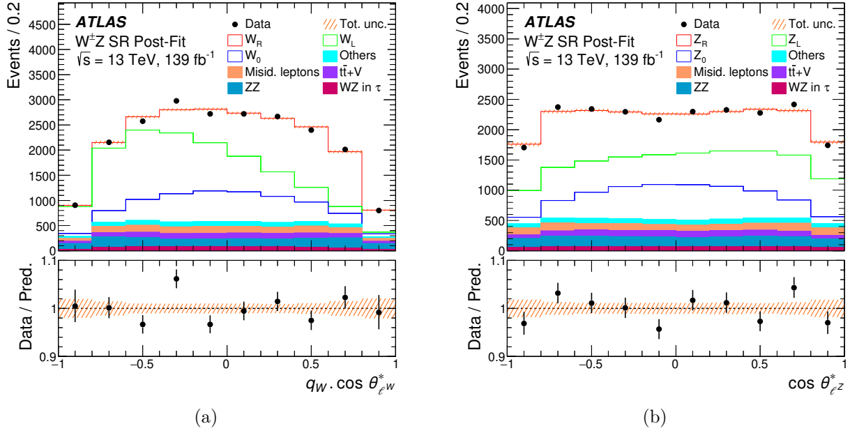
Figure 7.23: Post-fit distribution of q_W \cdot \cos \theta_{\ell W}^* (a) and \cos \theta_{\ell Z}^* (b) in the W^\pm Z events selection at detector level. In the top panel, respective contributions of the W^\pm Z single polarisation templates 0, L and R of the W^\pm boson or the Z boson and backgrounds are stacked on top of each other in the same order as in the legend. The uncertainty band around the expectation includes all systematic uncertainties as obtained from the fit. The ratio of data to prediction is represented in the bottom panel.
