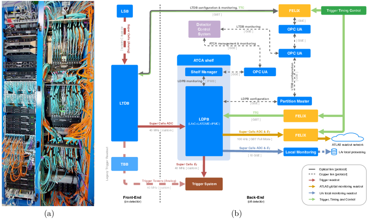
Figure 3.9: (a) Picture of the Digital Trigger rack in the USA15 counting room. In the left rack are the Run Control, Detector Control System, Local Monitoring and FELIX systems. The three ATCA crates are visible on the right rack. (b) Data paths of the Digital Trigger. From Ref. [57].
