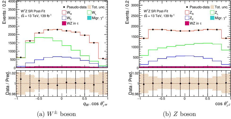
Figure 7.7: Independent closure test at reconstructed level for the W^\pm boson (a) and the Z boson (b). The polarisation templates were generated with the reweighting each of a different subset of the POWHEG+PYTHIA sample. The \tau decay and migrating \gamma^* background contributions in the inclusive sample have their separate templates included but left unaffected by the template fit.
