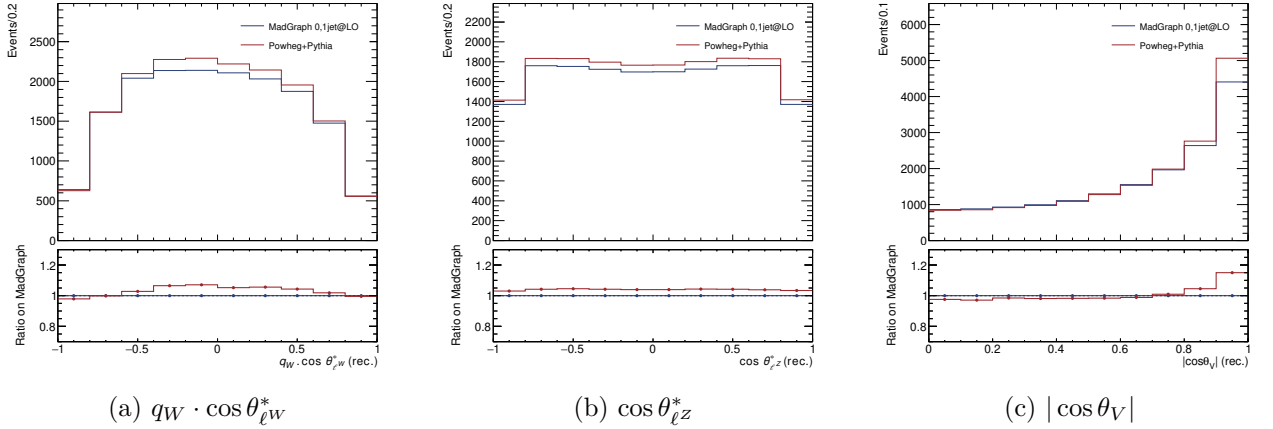
Figure 5.3: Comparison between distributions of q_W \cdot \cos \theta_{\ell W}^* (a), \cos \theta_{\ell Z}^* (b) and |\cos \theta_V| (c) of inclusive Monte Carlo samples MADGRAPH0,1j@LO and POWHEG+PYTHIA at detector level for W^\pm Z events.
