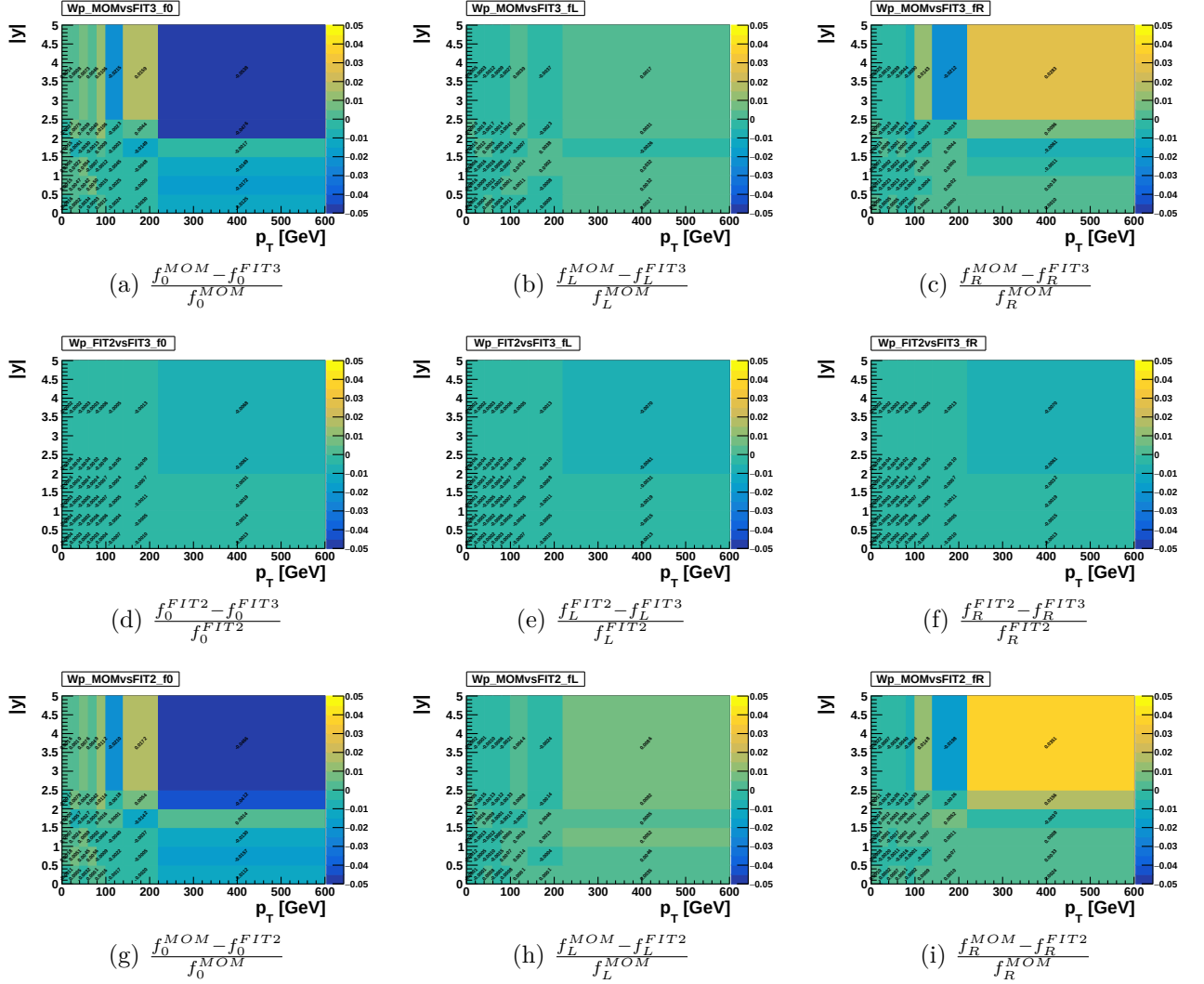
Figure B.2: Relative difference on fractions obtained by two different methods, extracted from POWHEG+PYTHIA in the total phase space, in bins of p_T and |y| , for the W^+ boson. From left to right are shown f_0 , f_L and f_R .
