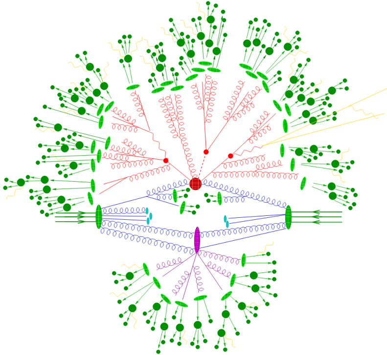
Figure 1.5: Sketch of all the different processes in a pp collision as modeled by a Monte Carlo generator. The incoming protons are represented by green blobs in the horizontal direction. The blue lines represent the interacting partons and their initial state radiations. The red blob in the centre represents the hard scattering between two partons. The subsequent parton shower is represented in the tree like structure in red. The following hadronisation is represented in light green, with each small dark green blob denoting a decaying hadron. The radiated photons are represented by yellow lines. A secondary parton interaction is represented in the purple blob. The beam remnants are the light blue blobs. From Ref. [34].
