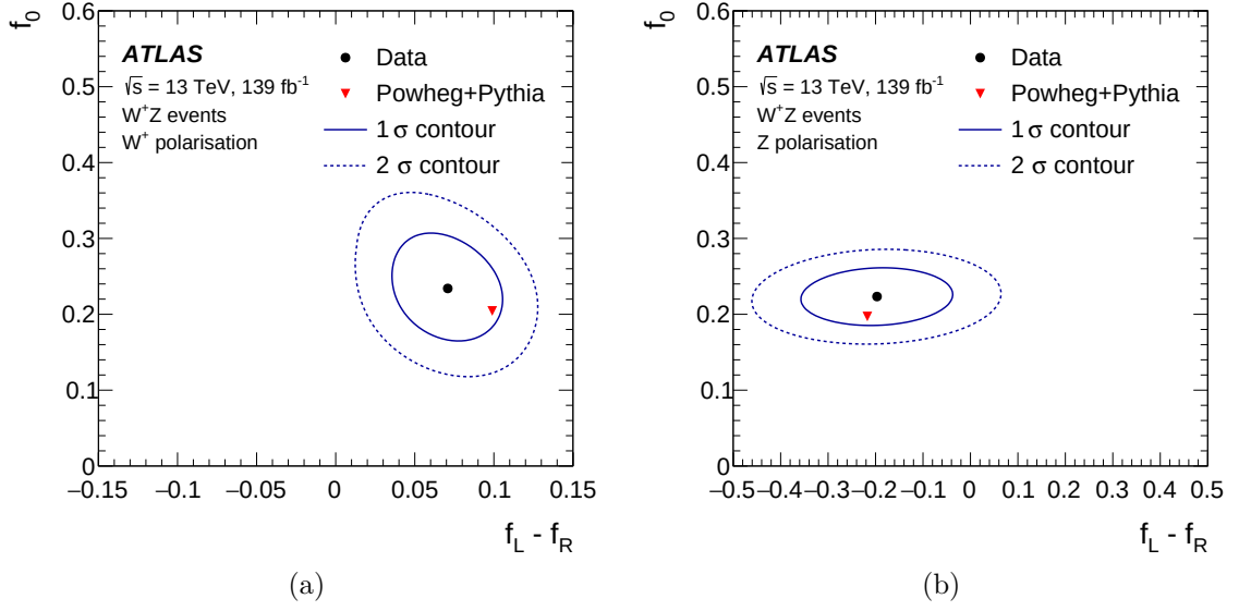
Figure D.2: Single boson polarisation fractions f_0 and f_L - f_R measured for the W^+ boson (a) and Z boson (b) in W^+Z events, compared with predictions from POWHEG+PYTHIA with \sin^2 \theta_w = 0.23152 (red triangle). The effect of PDF and QCD scale uncertainties on the POWHEG+PYTHIA predictions are of the same size as the triangle marker. The solid and dashed ellipses around the data points correspond to one and two standard deviations, respectively.
