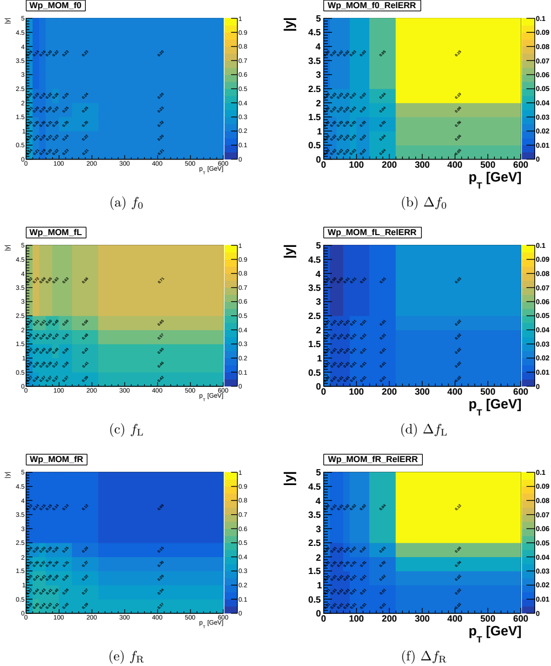
Figure B.1: W^+ boson polarisation fractions at particle level in the total phase space, extracted from POWHEG+PYTHIA with the moments method. The fractions, from top to bottom f_0 , f_L , f_R , are shown in the left column in bins of p_T and |y| of the W^+ boson, along with their associated statistical uncertainties in the right column.
