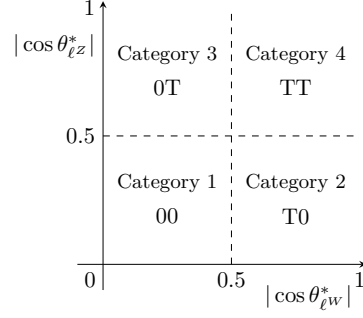
Figure 7.4: Scheme of categories as function of \cos \theta_{\ell}^* and \cos \theta_{\ell}^* .
