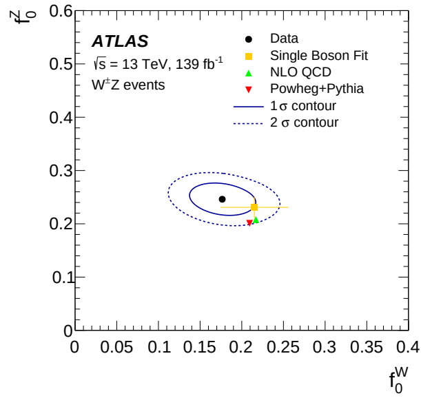
Figure 7.25: Measured polarisation fractions f_0^W and f_0^Z in W^\pm Z events. The black point is the simultaneously measured values from the template fit on the 4-category DNN score distribution. The orange square with uncertainty bars is the measured value from two single boson polarisation template fits to q_W \cdot \cos \theta_{\ell W}^* and \cos \theta_{\ell Z}^* distributions. The red triangle is the theoretical predictions at NLO in QCD and LO for the electroweak interaction from POWHEG+PYTHIA. The solid and dashed ellipses around the data points correspond to one and two standard deviations to the joint measurement of f_0^W and f_0^Z , respectively.
