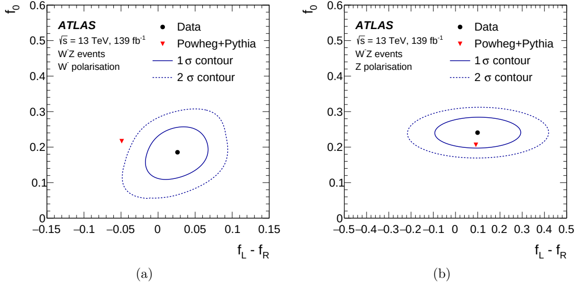
Figure D.6: Single boson polarisation fractions f_0 and f_L - f_R measured for the W^- boson (a) and Z boson (b) in W^-Z events, compared with predictions from POWHEG+PYTHIA with \sin^2 \theta_w = 0.23152 (red triangle). The effect of PDF and QCD scale uncertainties on the POWHEG+PYTHIA predictions are of the same size as the triangle marker. The solid and dashed ellipses around the data points correspond to one and two standard deviations, respectively.
