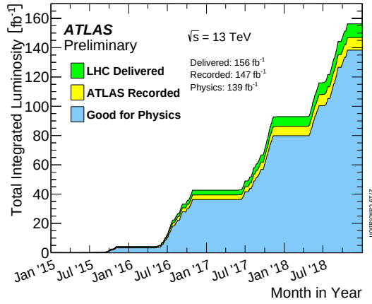
Figure 2.4: Cumulative luminosity versus time delivered to ATLAS (green), recorded by ATLAS (yellow), and certified to be good quality data (blue), during stable beams for pp collisions at 13 TeV centre-of-mass energy in 2015-2018. From Ref. [50].
