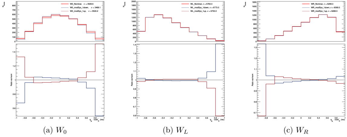
Figure 7.17: Modelling uncertainty Up and Down variations on the distributions of q_W \cdot \cos \theta_{\ell W}^* in W^\pm template 0 (a) template L (b) and template R (c). The bottom panels provide ratios of the variations to the nominal distribution.
