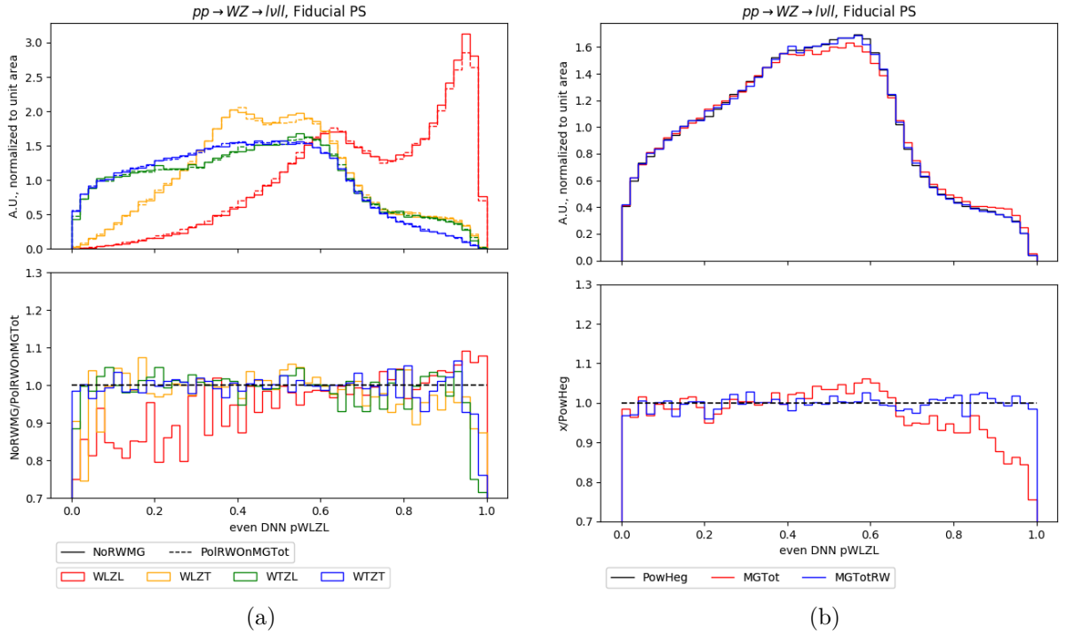
Figure 7.12: Distributions of p_{00}^{\text{DNN}} in the fiducial phase space in W^\pm Z events. All distributions were rescaled to the same surface area. In (a), the MGgen distributions in solid lines are compared one to one to the reweighted inclusive MADGRAPH0,1j@LO distributions in dashed lines for all four joint-polarisation states. In (b), the POWHEG+PYTHIA distribution in black is compared to the reweighted inclusive MADGRAPH0,1j@LO distribution in blue and the original MADGRAPH0,1j@LO distribution in red. In both cases, the bottom panels provide ratios between the compared distributions.
