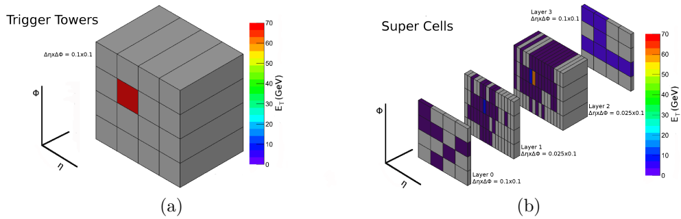
Figure 3.1: An electron with E_T = 70 GeV as seen by the Level-1 Calorimeter electronics with inputs from Trigger Tower (a) and from SuperCells (b). From Ref. [57].
