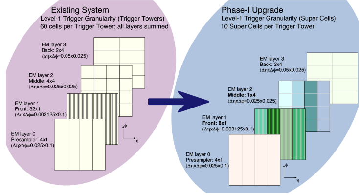
Figure 3.6: Representation in the (\eta, \phi) plane and in the four transversal layers of an EMB Trigger Tower (left) and the 10 Super Cells within (right). From Ref. [57].
