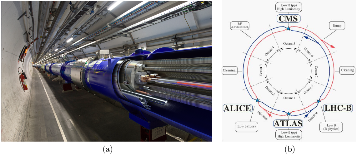
Figure 2.1: (a) A dipole magnet in the LHC tunnel. The two beam pipes are made visible by the 3D cut inside the magnet yoke. (b) Schematic layout of the LHC and its four experiments ATLAS, ALICE, CMS and LHCb. Figure from Ref. [41].
