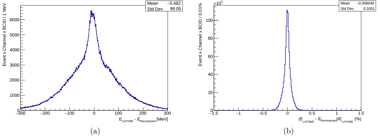
Figure 4.7: (a) Histogram of the difference between E_{\text{LATOME}} the E_T output of the LATOME and E_{\text{Recomputed}} from the offline computation with the full float precision for the OFCs. The bins width is 1 MeV, well below the computational resolution at 12.5 MeV.
