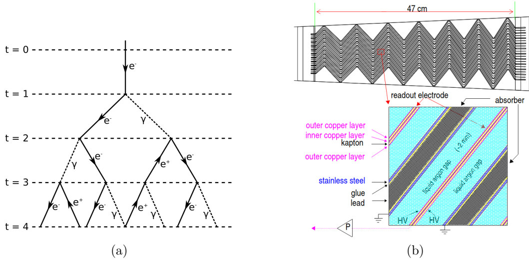
Figure 2.11: (a) Sketch of an electromagnetic shower. (b) Internal structure of the LAr Electromagnetic Barrel accordion shape with alternate layers of active material (liquid Argon, in blue), absorber (lead plates, in grey) and readout electrode (copper, in pink). From Ref. [56].
