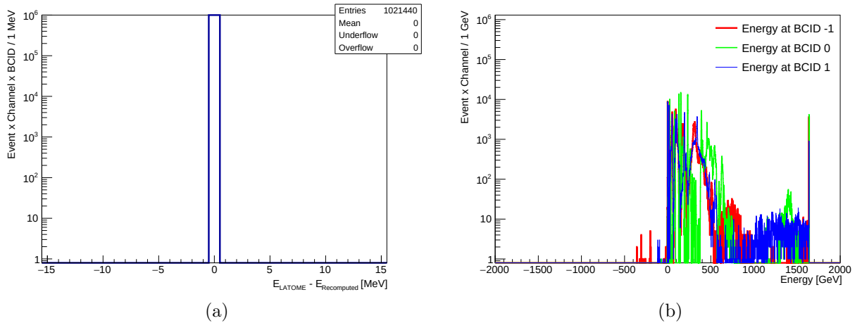
Figure 4.5: (a) Histogram of the difference between E_{\text{LATOME}} the E_T output of the LATOME and E_{\text{Recomputed}} from the offline computation. The bins width is 1 MeV, well below the computational resolution at 12.5 MeV, and the bins height is in log scale.
