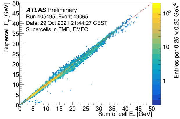
Figure 4.8: The measured E_T in Super Cells from all layers of the LAr Electro-Magnetic Barrel (EMB) and Electro-Magnetic End-Caps (EMEC) are compared to the summed E_T from their constituent LAr cells, obtained through the main readout path. The data are from a single event of a beam splash run, where energy calculations are performed offline using optimal filtering with preliminary calibration constants. The diagonal red line of equation y = x marks the agreement of both values. From Ref. [69].
