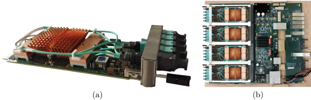
Figure 3.10: Picture of a LATOME board equipped with optical fibers and a copper heatsink (a), and picture of a LAr Carrier equipped with four LATOME boards (b).
