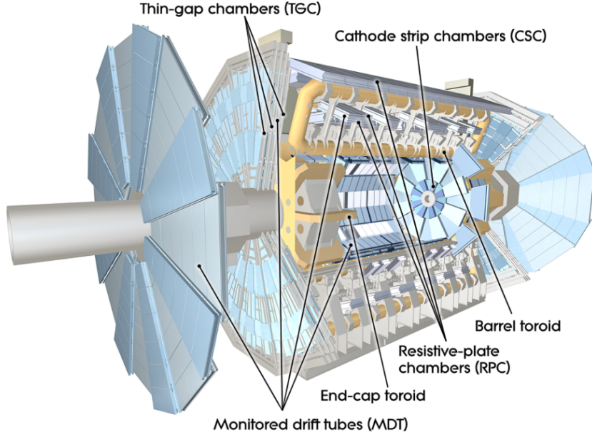
Figure 2.13: Muon detectors in ATLAS. Taken from Ref. [42].
