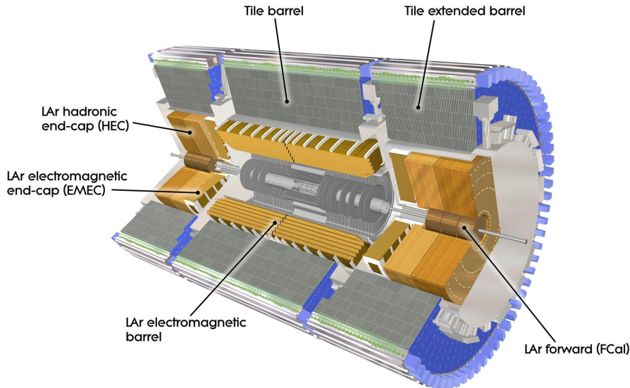
Figure 2.10: Calorimeters in ATLAS. From Ref. [42].
