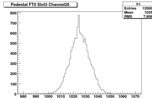
Figure 3.4: Pedestal distribution in ADC count for one LAr cell over 2000 events with 6 samples recorded. From Ref. [61].
