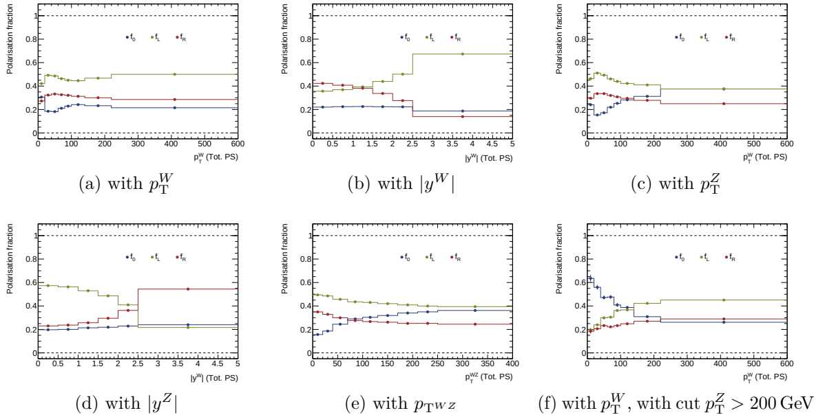
Figure 7.6: Evolution of the three polarisation fractions f_0 , f_L and f_R of a W^+ boson with respect to different kinematic variables, extracted from POWHEG+PYTHIA in the total phase space with the moments method.
