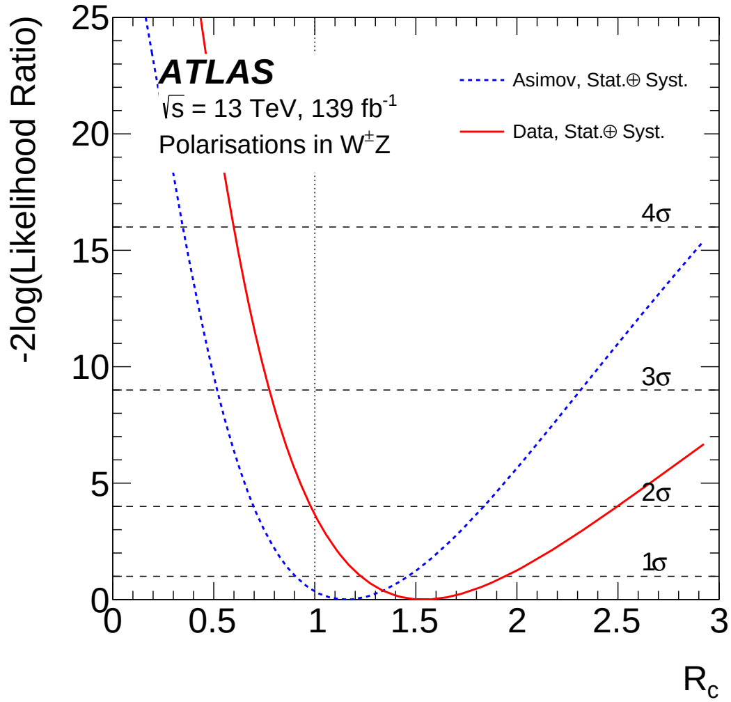
Figure 7.26: Curve of the test statistic -2\log(\text{Likelihood Ratio}) along the ratio R_c in W^\pm Z events. The likelihood ratio is profiled for all systematic uncertainties. Its width at the 1\sigma horizontal line gives the total statistical and systematic asymmetrical uncertainty on R_c . The blue dashed curve represent the expected result, from an Asimov fit at reconstructed level. The red curve represents the result on Run 2 data. The vertical line at 1 corresponds to the absence of spin correlation hypothesis.
