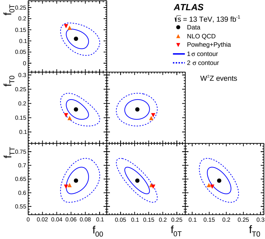
Figure 7.22: Measured joint-polarisation fractions f_{00} , f_{0T} , f_{T0} and f_{TT} of the W^\pm and Z bosons in W^\pm Z events, compared to NLO QCD fixed-order predictions [77] (orange triangle) and to Monte Carlo predictions from POWHEG+PYTHIA (red triangle). The effect of PDF and QCD scale uncertainties on the POWHEG+PYTHIA and NLO QCD fixed-order predictions are of the same size as the respective markers. The solid and dashed ellipses around the data points correspond to one and two standard deviations, respectively.
