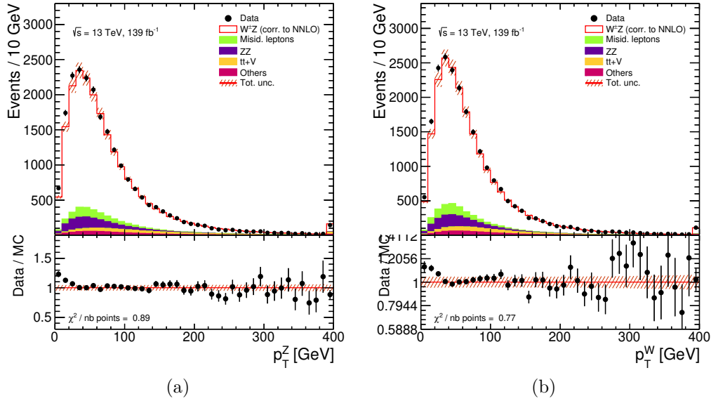
Figure 6.6: Control distributions of the W^\pm boson p_T (b) and of the Z boson p_T (a). All Monte Carlo expectations are scaled to the integrated luminosity of the data using the predicted Monte Carlo cross sections of each sample. The dashed red band represents the quadrature sum of all systematic uncertainties on the total Monte Carlo expectation (see text for details) and a 1.7% systematic uncertainty on the luminosity [49].
