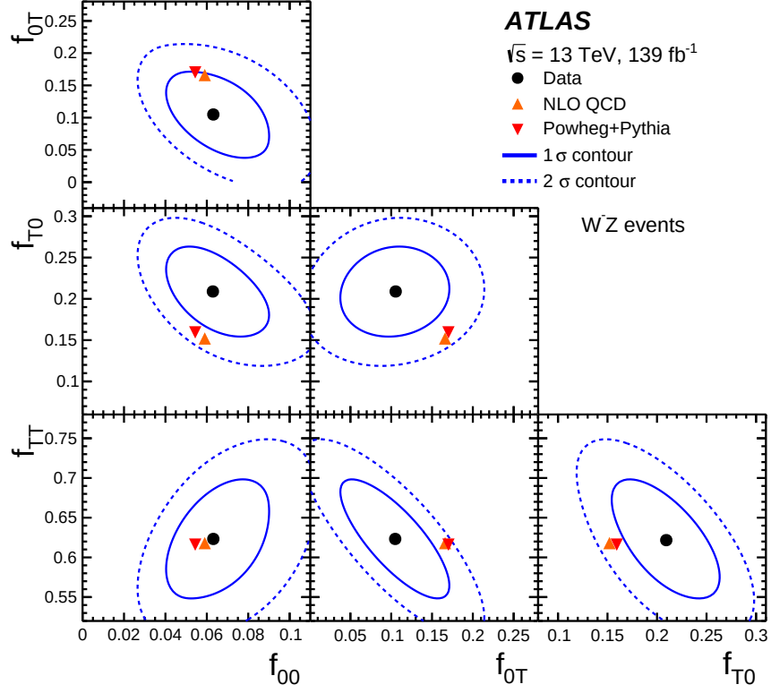
Figure D.5: Measured joint-polarisation fractions f_{00} , f_{0T} , f_{T0} and f_{TT} of the W^- and Z bosons in W^-Z events, compared to NLO QCD fixed-order predictions [77] (orange triangle) and to Monte Carlo predictions from POWHEG+PYTHIA (red triangle). The effect of PDF and QCD scale uncertainties on the POWHEG+PYTHIA and NLO QCD fixed-order predictions are of the same size as the respective markers. The solid and dashed ellipses around the data points correspond to one and two standard deviations, respectively.
