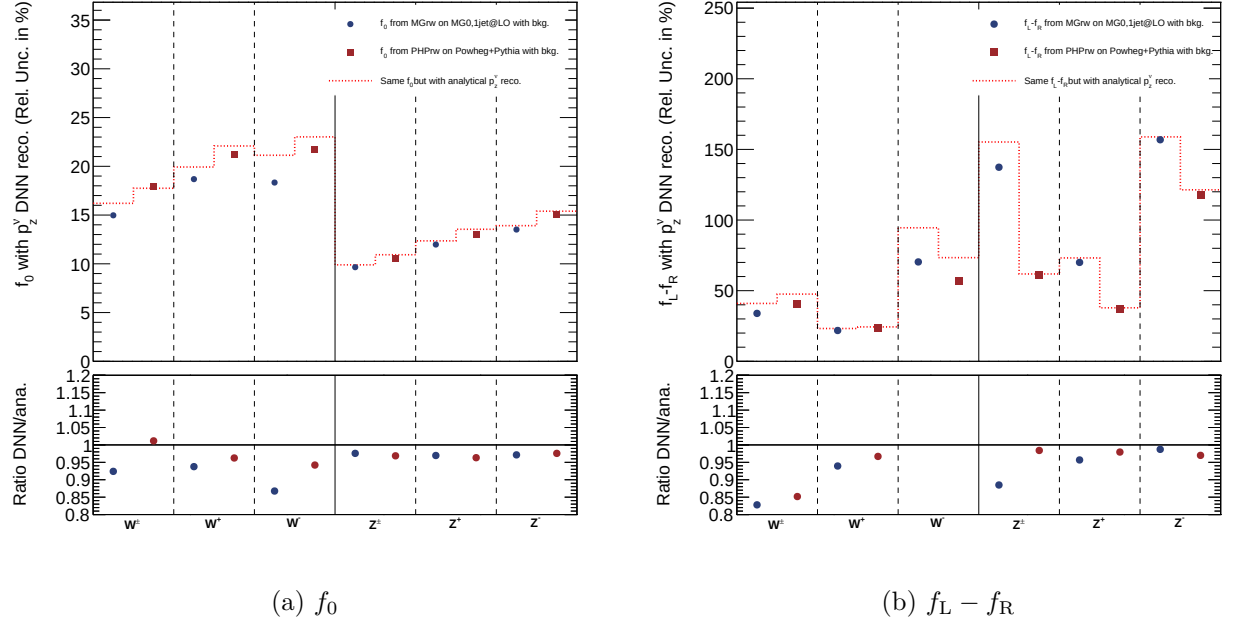
Figure C.3: Relative uncertainties on parameters of interest from an Asimov fit of signal and backgrounds. f_0 (a) and f_L - f_R (b) uncertainties are shown using analytical (red dotted line) and DNN-based (points) p_z^\nu reconstruction, for templates MGrw and PHPrw and for W^\pm and Z boson in all charge configurations. The bottom plot shows the ratio between the uncertainty values for both methods of p_z^\nu reconstruction.
