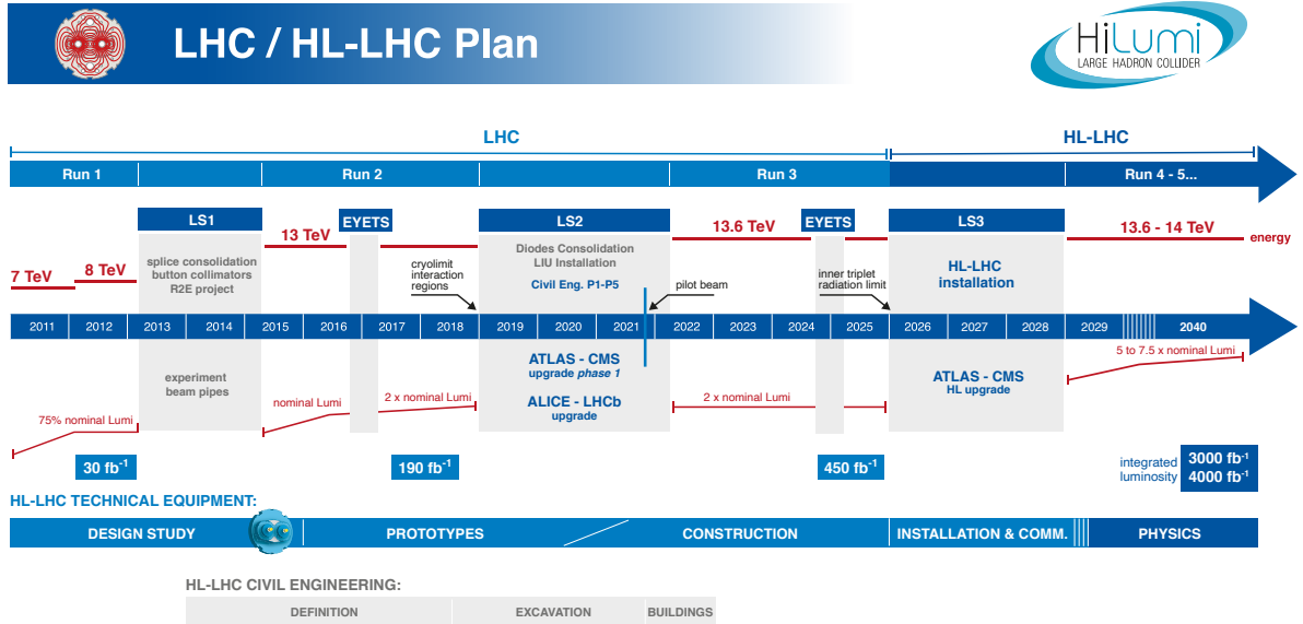
Figure 2.6: LHC baseline plan for the next decade and beyond showing the collision energy (upper line) and instantaneous luminosity (lower line). Plan as taken from Ref. [51] last updated in February 2022.
