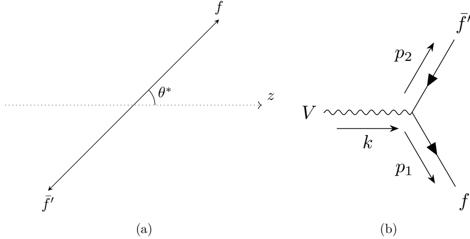
Figure 5.1: Decay of a vector boson V in its rest frame (a), and the Feynman diagram associated to this process (b).
