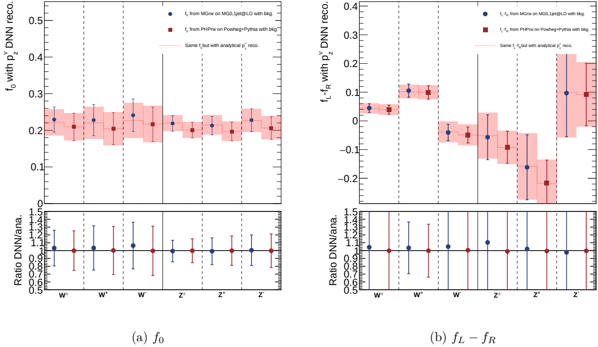
Figure C.2: Central value of parameters of interest from an Asimov fit of signal and backgrounds. f_0 (a) and f_L - f_R (b) central values are shown using analytical (red dotted line) and DNN-based (points) p_z^\nu reconstruction, for templates MGrw and PHPrw and for W^\pm and Z boson in all charge configurations. The bottom plot shows the ratio between the uncertainty values for both methods of p_z^\nu reconstruction.
