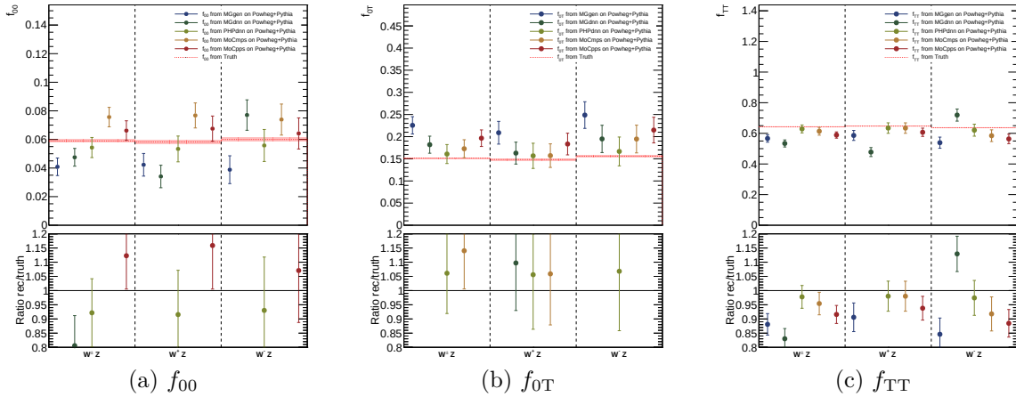
Figure 7.15: Results of signal only fits of POWHEG+PYTHIA at detector level for the parameters of interest f_{00} (a), f_{0T} (b) and f_{TT} (c) for all five templates MGgen , MGdnn , PHPdnn , MoCmps and MoCpps in all charge configurations. Uncertainties are from statistical origin only.
