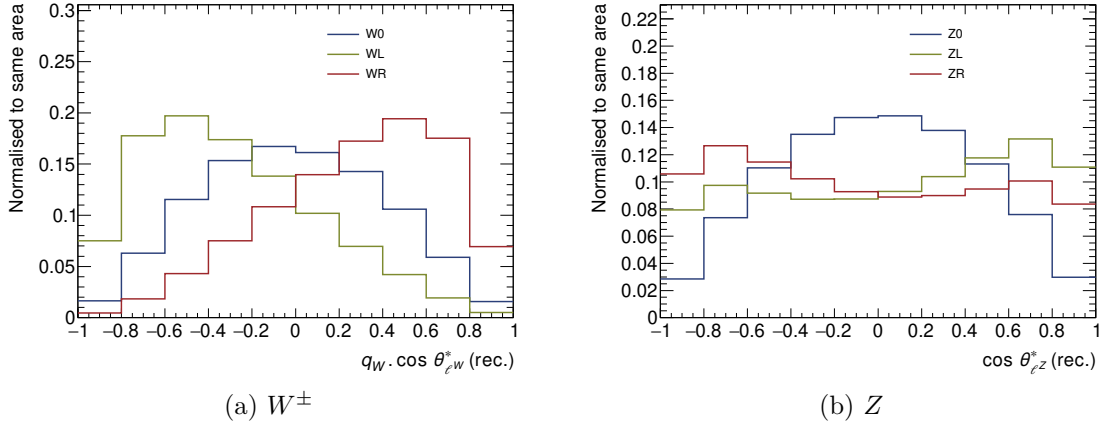
Figure 7.1: All three single boson polarisation templates at detector level for W^\pm boson using q_W \cdot \cos \theta_{\ell W}^* (left) and for Z boson using \cos \theta_{\ell Z}^* (right) in W^\pm Z events. These templates were all rescaled to the same surface area.
