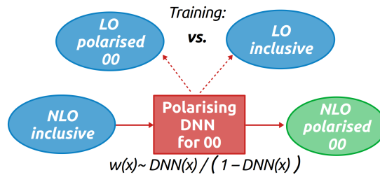
Figure 7.11: Sketch of the DNN-based reweighting of an inclusive NLO sample to a polarised NLO sample for the 00 joint-polarisation state. In blue are the samples used as input, and in green is the newly obtained sample. The DNN represented in red, applying to each event x the weight w(x) = \text{DNN}(x) / (1 - \text{DNN}(x)) , classifies event between the 00 joint-polarisation with target 1 and the inclusive sample with target 0.
