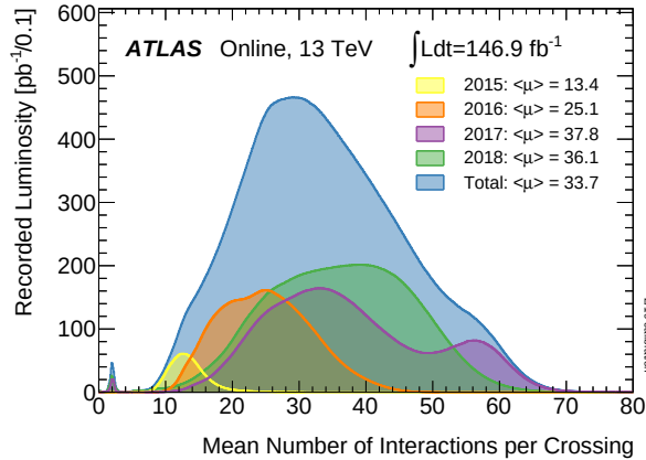
Figure 2.5: Shown is the luminosity-weighted distribution of the mean number of interactions per crossing \mu for pp collision data at 13 TeV centre-of-mass energy, for the full Run 2 data taking period (blue) and per year: 2015 (yellow), 2016 (orange), 2017 (violet) and 2018 (green). The overall mean number of collisions \langle\mu\rangle is given per period in the legend. From Ref. [50].
