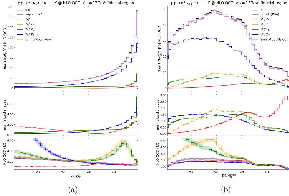
Figure 7.9: Particle-level in the fiducial phase space distribution of |\cos \theta_V| (a) and p_{00}^{\text{DNN}} (b) in pp \rightarrow e^+ \nu_e \mu^+ \mu^- events. From top down: NLO QCD differential cross-sections, NLO QCD normalised distribution shapes (integral equal to 1), K -factors (NLO QCD / LO).
