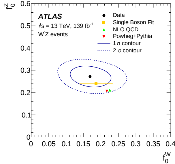
Figure D.7: Measured polarisation fractions f_0^W and f_0^Z in W^-Z events. The black point is the simultaneously measured values from the template fit on the 4-category DNN score distribution. The orange square with uncertainty bars is the measured value from two single boson polarisation template fits to q_W \cdot \cos \theta_{\ell W}^* and \cos \theta_{\ell Z}^* distributions. The red triangle is the theoretical predictions at NLO in QCD and LO for the electroweak interaction from POWHEG+PYTHIA. The solid and dashed ellipses around the data points correspond to one and two standard deviations to the joint measurement of f_0^W and f_0^Z , respectively.
