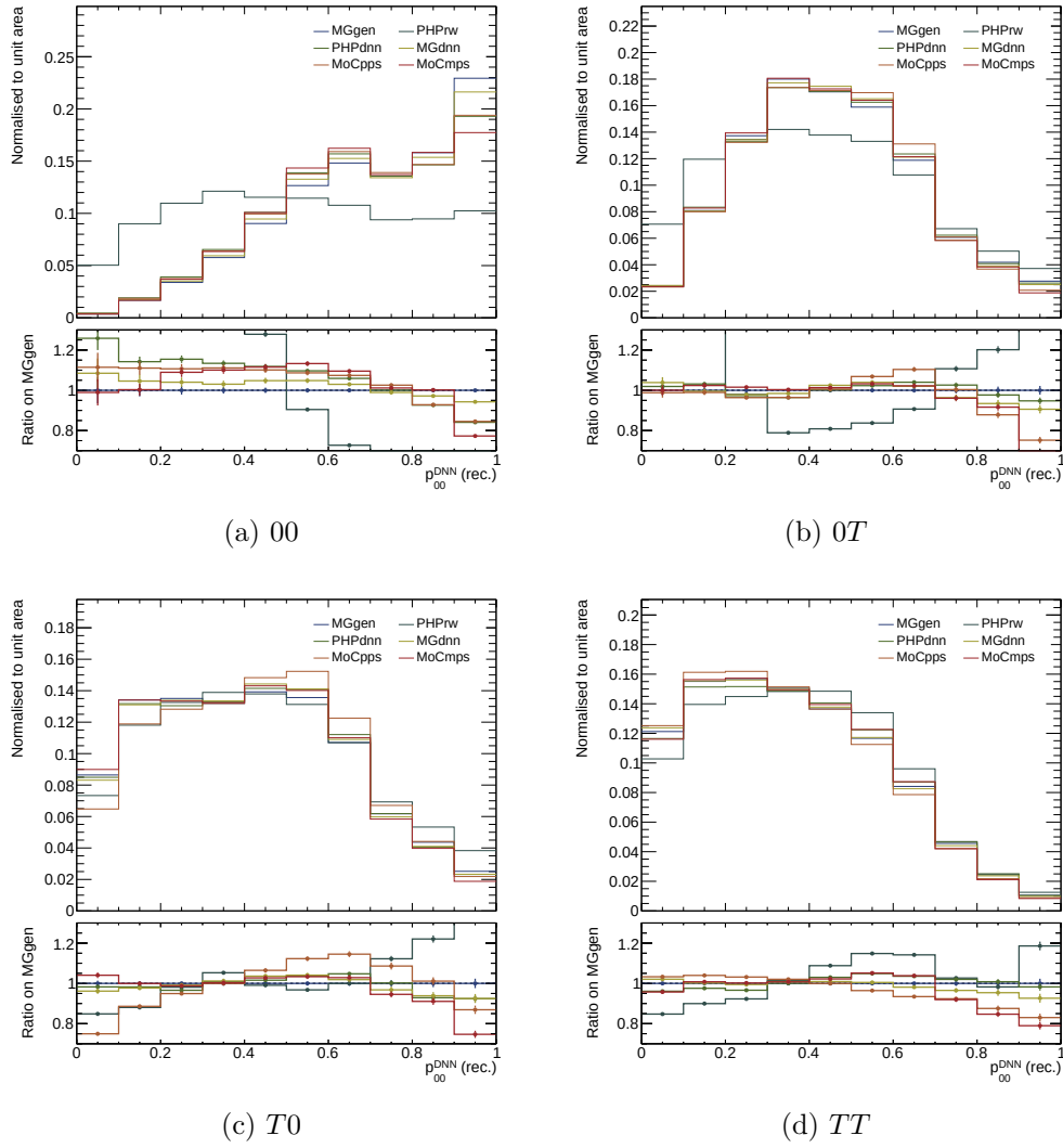
Figure 7.14: Distributions at detector level of p_{00}^{\text{DNN}} for the six sets of polarisation templates at hand MGgen, PHPrw, MGdnn, PHPdnn, MoCmps and MoCpps, for W^\pm Z events and for polarisations 00 (a), 0T (b), T0 (c) and TT (d). These templates were all rescaled to the same surface area.
