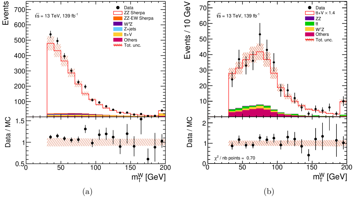
Figure 6.2: Control distribution of m_T^W in the ZZ control region (a) and in the t\bar{t} + V validation region (b). The composition of both regions are estimated by Monte Carlo scaled to the expected luminosity in Run 2. The dashed red band incorporates a 1.7 % systematic uncertainty on the luminosity [49] and an overall normalisation uncertainty of 10 % for the ZZ sample in (a) and 15 % for the rescaled t\bar{t} + V sample in (b).
