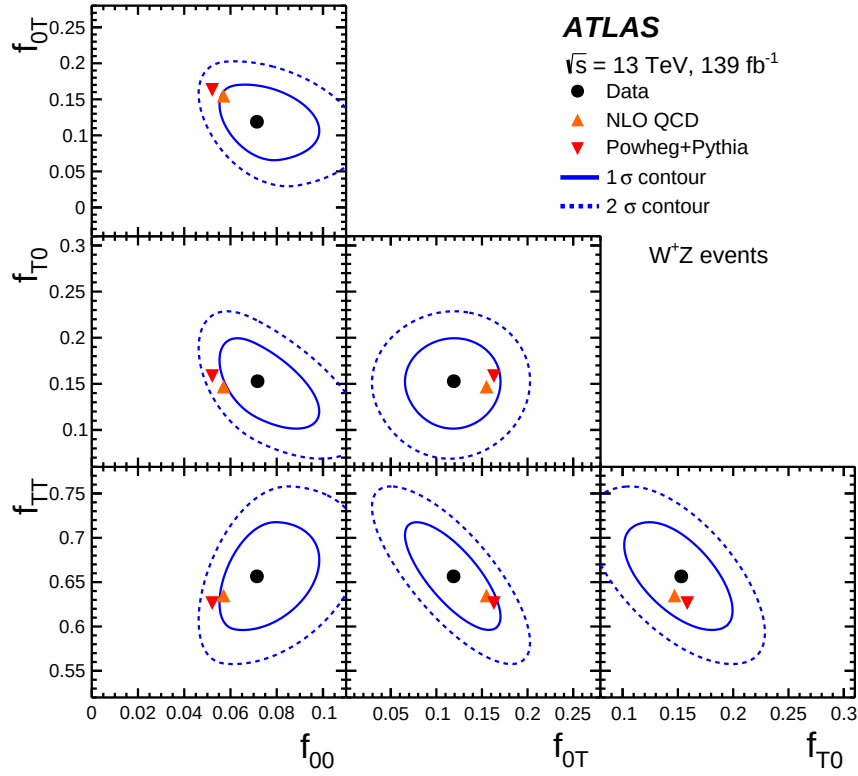
Figure D.1: Measured joint-polarisation fractions f_{00} , f_{0T} , f_{T0} and f_{TT} of the W^\pm and Z bosons in W^+Z events, compared to NLO QCD fixed-order predictions [77] (orange triangle) and to Monte Carlo predictions from POWHEG+PYTHIA (red triangle). The effect of PDF and QCD scale uncertainties on the POWHEG+PYTHIA and NLO QCD fixed-order predictions are of the same size as the respective markers. The solid and dashed ellipses around the data points correspond to one and two standard deviations, respectively.
