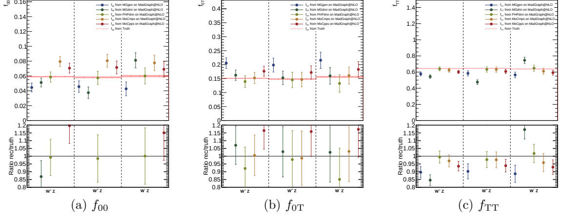
Figure 7.16: Results of signal only fits of MADGRAPH@NLO at detector level for the parameters of interest f_{00} (a), f_{0T} (b) and f_{TT} (c) for all five templates MGgen , MGdnn , PHPdnn , MoCmps and MoCpps in all charge configurations. Uncertainties are from statistical origin only.
