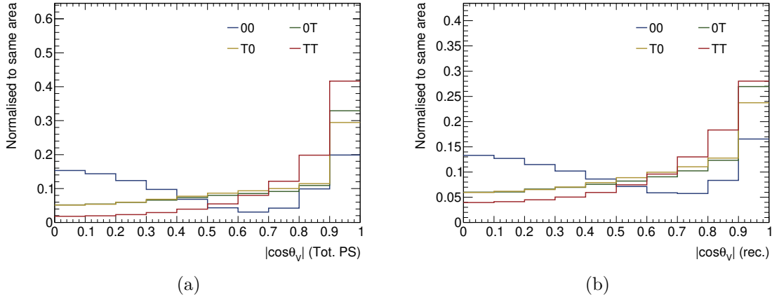
Figure 7.2: All four MGgen joint-polarisation templates for W^\pm Z events with |\cos \theta_V| as discriminating variable are represented at particle level in the total phase space (a) and at reconstructed level (b). These templates were all rescaled to the same surface area.
