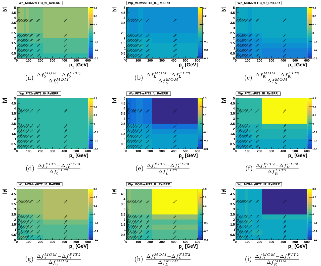
Figure B.3: Relative statistical uncertainty difference on fractions obtained by two different methods, extracted from POWHEG+PYTHIA in the total phase space, in bins of p_T and |y| , for the W^+ boson. From left to right are shown f_0 , f_L and f_R .
