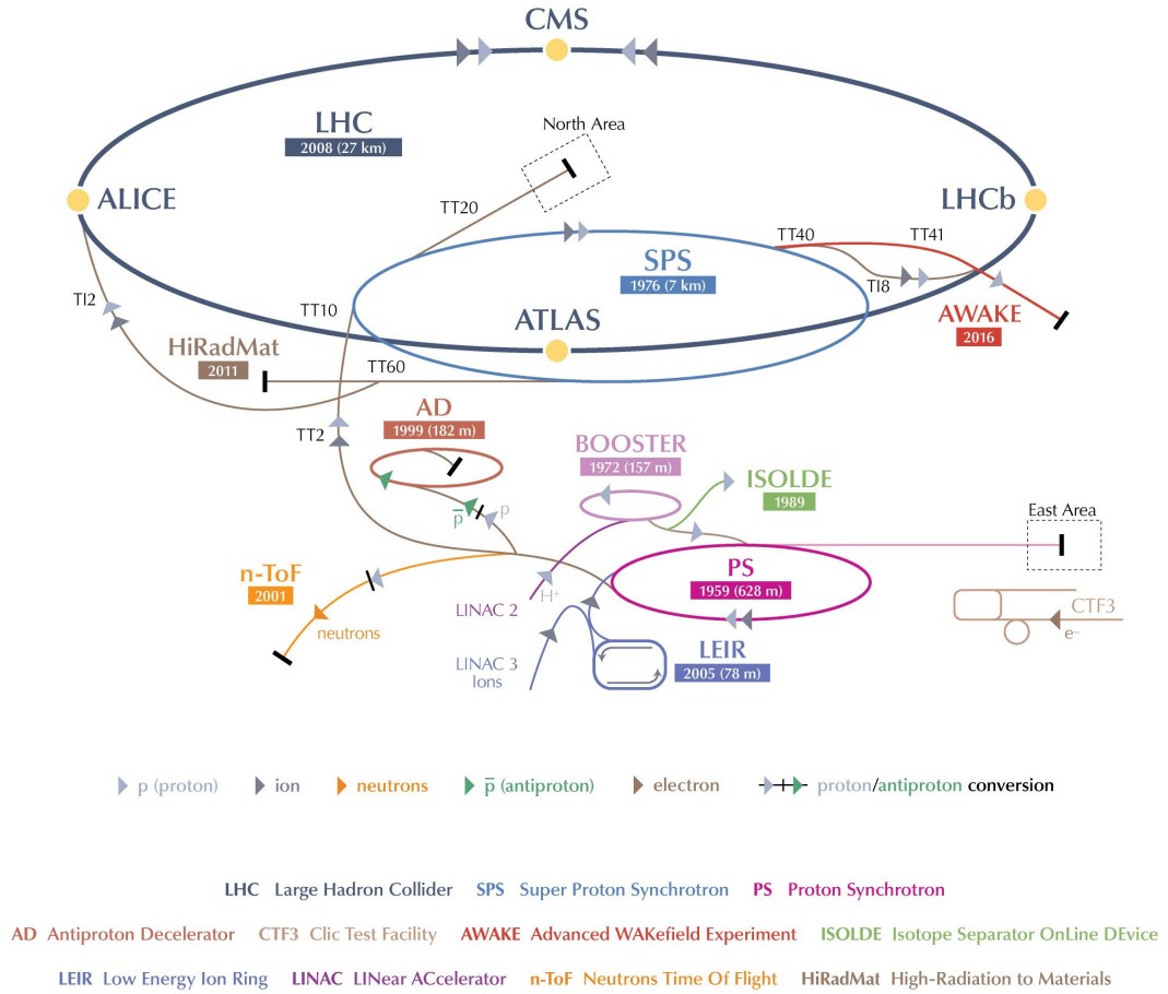
Figure 3.2: Illustration of the CERN accelerator complex. The LHC is supplied with protons or heavy ions by the SPS via two transfer lines which additionally provides beams to several non-LHC experiments. The SPS is fed with preaccelerated protons by the PS. PS was CERN's first synchrotron and it continues to supply smaller experiments with protons. The first circular accelerator in the proton-proton injection chain is PSB which is filled by the linear accelerator LINAC2. For beams of heavy ions the injection chain begins with LINAC3 which feeds PS via the LEIR. (©CERN, 2013–2016) [12]
