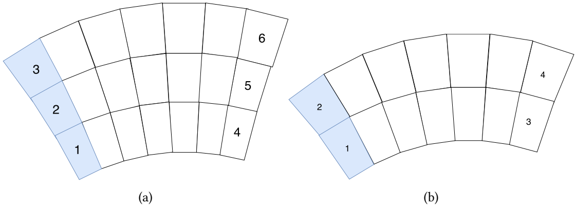
Figure 6.10: Illustration of the chamber ID assignment for CSCs in an EMTF processor for the station closest to the interaction region, station 1 (a), as well as station 2/3/4 (b). These chamber IDs are used to address track segments in the μGMT cancel-out system. Shaded chambers are associated with the neighbouring sector, but used for track finding to retain high efficiency at the overlaps.
