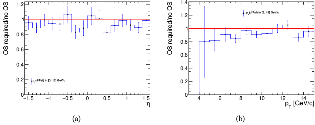
Figure 7.6: Plots of J/ψ trigger efficiency for the opposite sign (OS) double muon trigger path in the invariant mass window 3 GeV to 3.2 GeV plotted against the J/ψ pseudorapidity (a) and transverse momentum (b).
