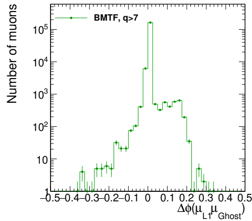
(c) Azimuthal distance between two duplicates in the BMTF system.
