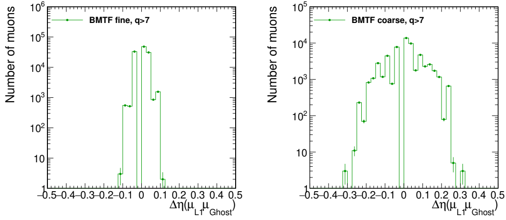
(a) Distance in pseudorapidity between two duplicates in the BMTF system where both muons have a well measured pseudorapidity.
