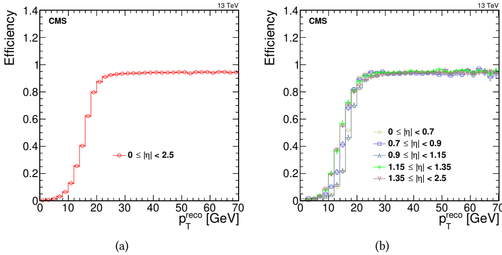
Figure 7.21: Single muon efficiencies for the Level-1 trigger as a function of muon transverse momentum as determined by the offline reconstruction algorithm. Curves drawn for complete coverage (a) as well as different pseudorapidity regions corresponding to track finder coverage and overlap regions (b). The efficiency is derived from a single muon sample of a data set taken in 2016.
