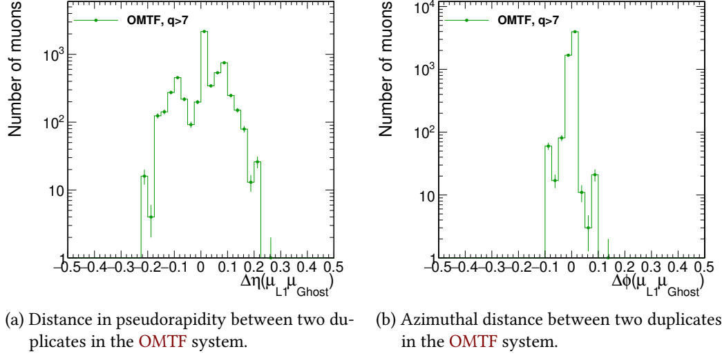
Figure 7.9: Distance between two muons reconstructed by the OMTF in events with a single generated muon. A threshold of q > 7 on the output quality was applied.
