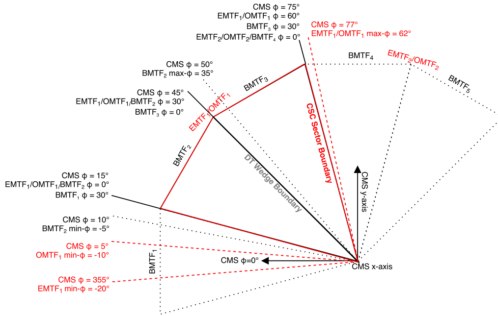
Figure 6.4: The relative \phi -scale for the track finders has its origin at the edge of the wedge or sector under consideration. The range is different for BMTF as it processes 30° wedges (black), compared to OMTF and EMTF which process 60° sectors (red).
