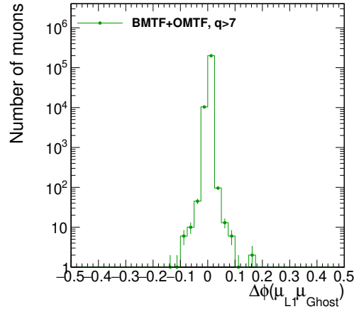
(c) Azimuthal distance between two duplicates in the BMTF and OMTF systems.
