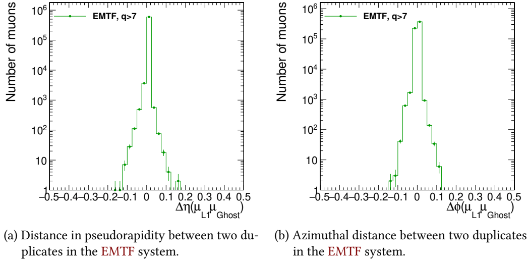
Figure 7.10: Distance between two muons reconstructed by the EMTF in events with a single generated muon. A threshold of q > 7 on the output quality was applied.
