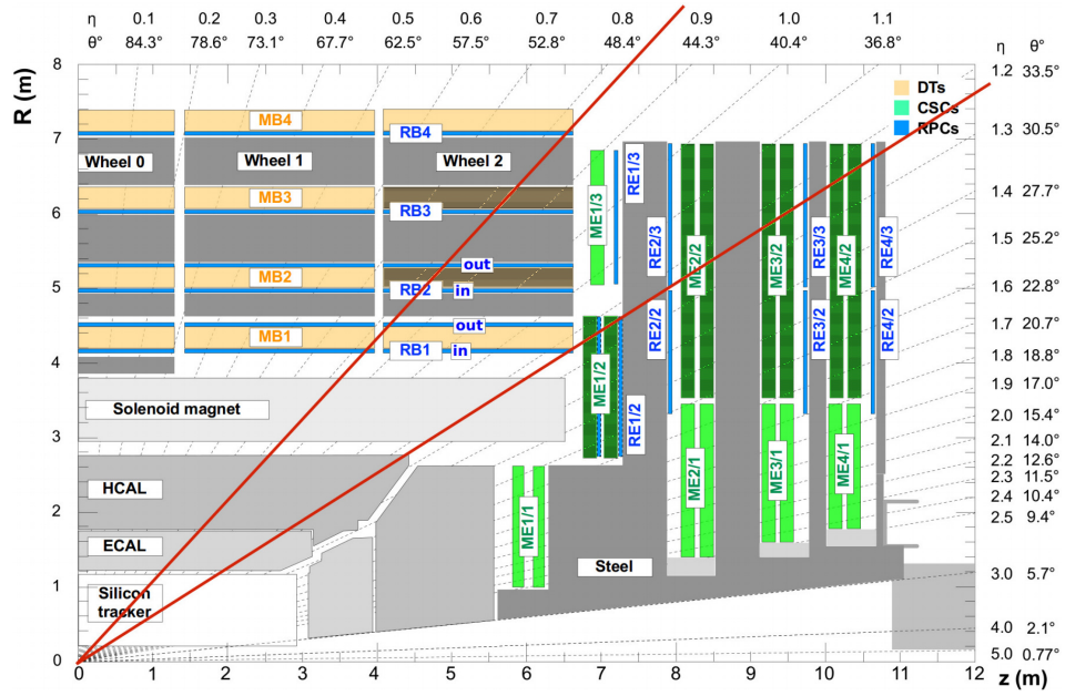
Figure 6.5: Cross-sectional view of a quarter of the CMS detector. The muon system is split in coverage by \eta . The BMTF , OMTF , and EMTF systems receive track segments from their respective pseudorapidity region (see section 5.3.3). A complication arises because certain muon stations (drawn hatched in the figure) are shared between neighbouring track finder systems. Track segments from these stations are sent to both track finding systems and lead to possible duplicates. Figure adapted from [95].
