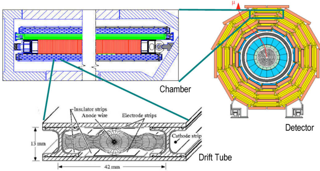
Figure 4.9: Depiction of the DT system in the CMS detector. A muon station (or DT chamber) consists of three SLs that are made of 4 layers of DT cells. A SL measuring the z-coordinate (in green) and a honeycomb spacer (red) are positioned between two \phi -measuring SLs (blue). [59]
