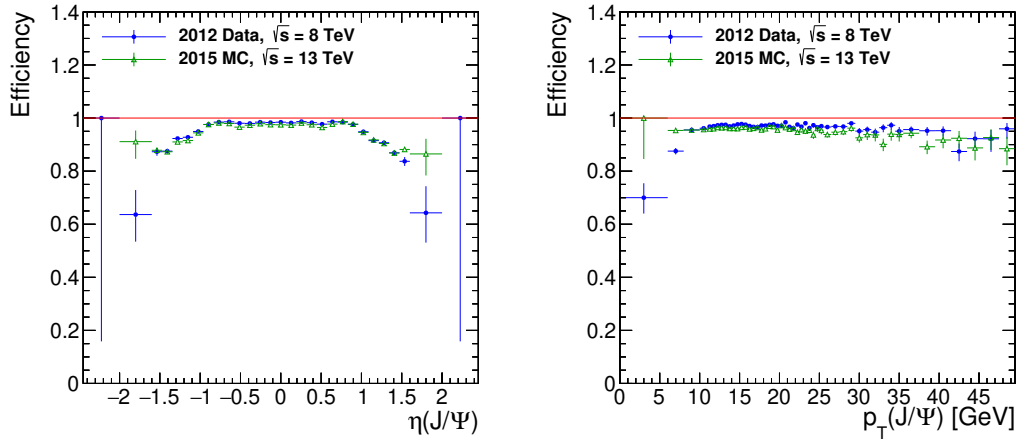
(a) The efficiency of the opposite charge requirement as a function of \eta . High efficiency is shown in the barrel region while the efficiency drops in the forward direction. (b) Plot of the opposite charge requirement efficiency vs. transverse momentum. The efficiency remains stable for moderately high transverse momentum J/\psi mesons.
