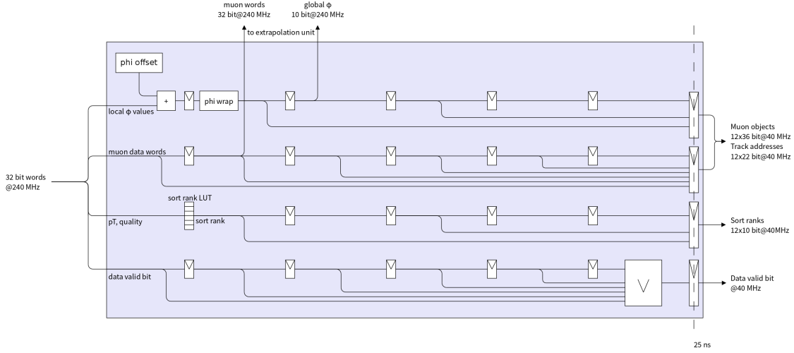
Figure 6.2: The muon deserialisation unit for a single input link. A 32 bit data word from a track finder is received at 240 MHz and separated into parallel streams. The entire link words are processed by a deserialisation pipeline that stores the current value at each 240 MHz clock tick. This allows the construction of a large 3 \times 62 bit data structure that contains the three input muons. In parallel, the data word corresponding to the local \phi value is extracted and used to calculate the global azimuthal coordinate by adding a configurable value depending on which track finder processor is connected to the given unit. Care must be taken close to \phi = 0 in order to correctly treat the wrap-around. Additionally, a rank is computed from p_T and the quality value from the track finders using a LUT . Finally, the data valid bit, generated by the link logic is OR-ed and stored for usage in the serialisation logic before transmission to the \mu GT.
