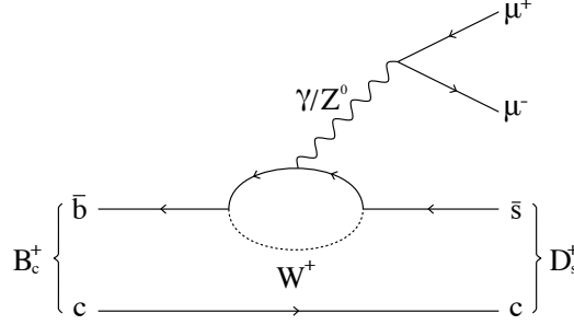
Figure 3.4: EWP decay topology for B_c^+ \rightarrow D_s^+ \mu^+ \mu^- .
