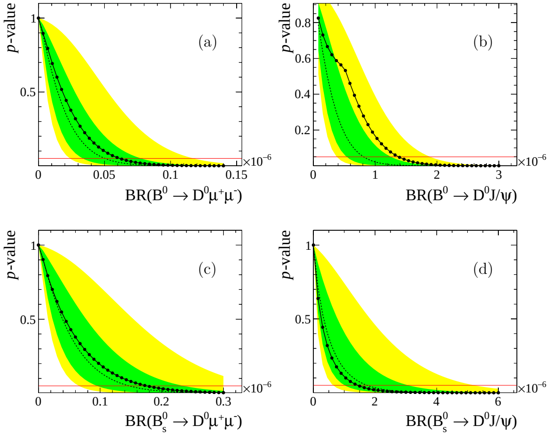
Figure 4.28: The variation in p -value with branching ratio for (a) B^0 \rightarrow \bar{D}^0 \mu^+ \mu^- , (b) B^0 \rightarrow \bar{D}^0 J/\psi , (c) B_s^0 \rightarrow \bar{D}^0 \mu^+ \mu^- , and (d) B_s^0 \rightarrow \bar{D}^0 J/\psi decays. The dotted lines show the variation taking into account the signal component, and the dashed lines the variation only considering the background component. The green and yellow filled areas correspond to 1\sigma and 2\sigma from the background-only hypothesis. The upper limits are taken to be the values where the dotted lines cross the red line, corresponding to the 95% confidence level, and are given in Table 4.26.
