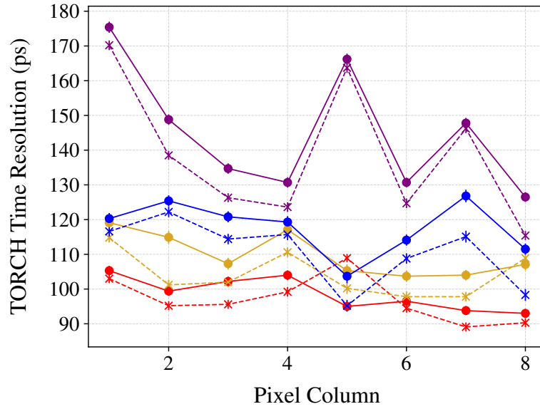
Figure 6.29: The single-photon time resolutions measured in the October 2018 test-beam as a function of MCP-PMT column number. The red points show position 1, yellow position 3, blue position 4 and purple position 5. The crossed points connected with dotted lines are measured using proton samples, the dotted points connected with solid lines with pion samples. Positions 1, 3, 4, and 5 are at distances -175 mm, -488 mm, -801 mm, and -1115 mm from the top of the radiator plate respectively, as per Fig. 6.10.
