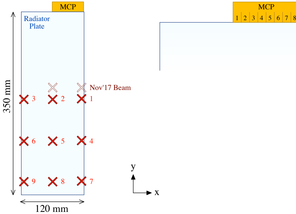
Figure 6.9: The position of the beam relative to Mini-TORCH in the June 2018 test-beam run. The values of the positions are given in Table 6.3. The positions used in November 2017 are shown for comparison as dotted crosses.
