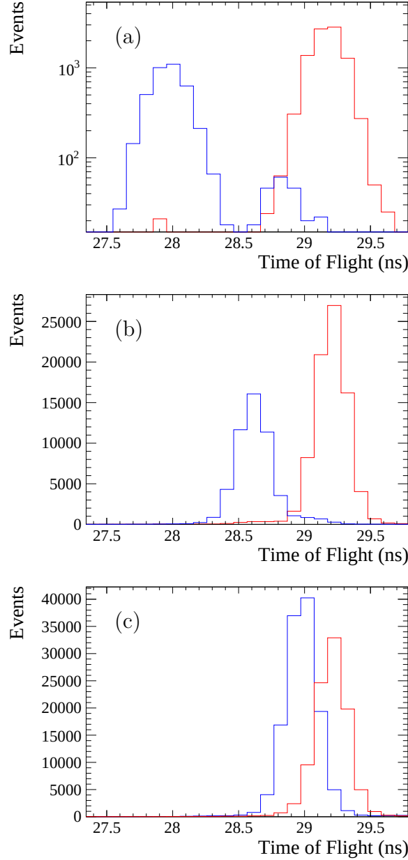
Figure 6.15: Particle times of flight measured in June 2018 at the nominal beam momenta of (a) 3.5 GeV/ c , (b) 5 GeV/ c , and (c) 8 GeV/ c , coloured according to whether or not a signal was seen in the Cherenkov counters. Red indicates a signal was seen, and hence corresponds to pions; blue indicates no signal was seen, corresponding to protons. In (a), a second blue peak can be seen at 28.8 ns, corresponding to a small kaon signal. In (b), part of the upper tail of the proton peak may be attributed to kaons. In (c), any kaon signal is impossible to distinguish. Note the x -axis range is the same for all three plots for ease of comparison, however only (a) has a logarithmic y -axis.
