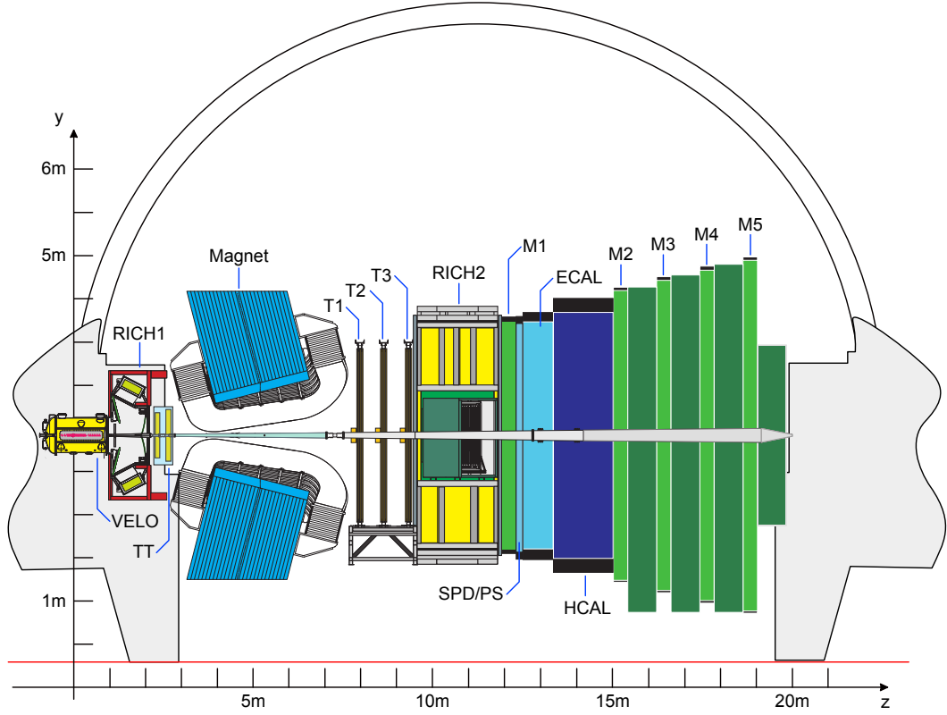
Figure 2.3: Side-view of the LHCb detector showing the arrangement of the sub-detector systems. Reproduced from Ref. [3].
