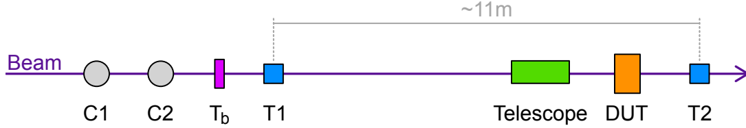
Figure 6.3: The test-beam infrastructure used in the three test-beam campaigns. C1 & C2 are threshold Cherenkov counters, T_b a large scintillator, T1 & T2 timing stations, and DUT either Mini-TORCH or Proto-TORCH depending on the test-beam campaign. The position of each item of infrastructure relative to the others is shown, although not to scale.
