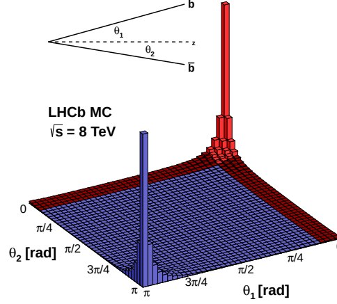
Figure 2.2: The b\bar{b} production angles at an LHC collision energy of 8 TeV, with the LHCb angular acceptance shown in red. Taken from Ref. [5].
