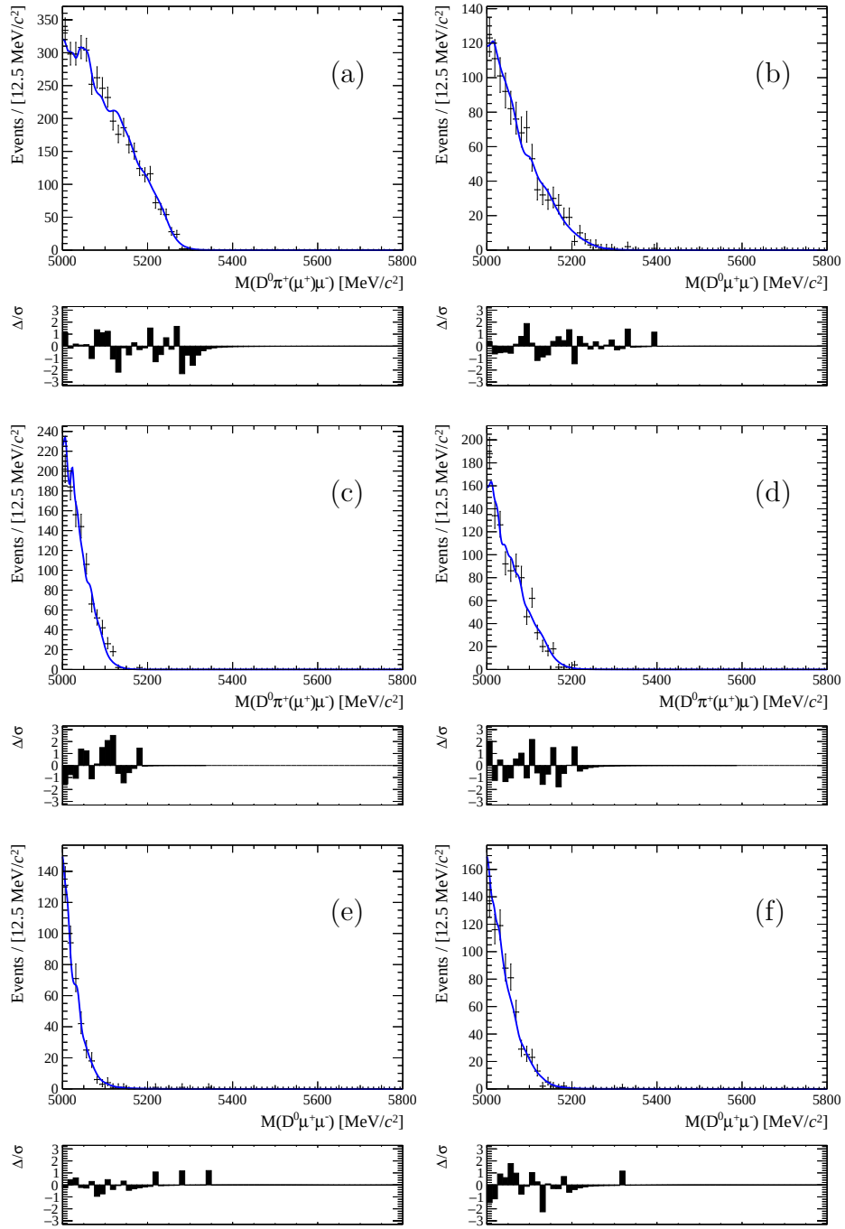
Figure 4.17: Simplified simulation samples [62] of (a) B^0 \rightarrow \bar{D}^0 \pi^- \mu^+ \nu_\mu , (b) B_s^0 \rightarrow (D_{s2}^{*-}(2573) \rightarrow D^0 K^-) \mu^+ \nu_\mu , (c, d) B^0 \rightarrow \bar{D}^{*0} \pi^- \mu^+ \nu_\mu , and (e, f) B_s^0 \rightarrow (D_{s1}(2536) \rightarrow D^{*0} K^-) \mu^+ \nu_\mu decays, with (c, e) D^{*0} \rightarrow D^0 \pi^0 and (d, f) D^{*0} \rightarrow D^0 \gamma . The \pi^- particles are reconstructed as muons, the K^- decays via K^- \rightarrow \mu^- \nu_\mu , and neutral particles are not reconstructed. The samples are fit with probability density functions generated using kernel density estimation from separate, independent samples.
