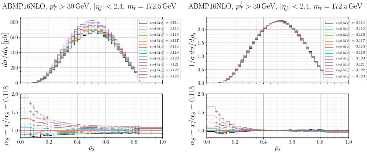
Figure 2.19: The absolute (left) and normalized (right) differential t\bar{t} +jet cross section as a function of \rho for varying values of \alpha_S [160]. The bottom panel shows the ratio to a central value of \alpha_S = 0.118 .
