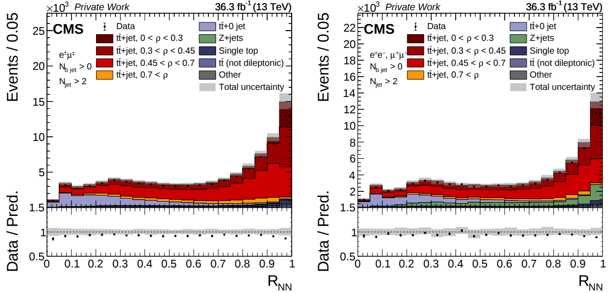
Figure 6.21: The observed (points) and MC predicted (stacked histograms) signal and background yields as a function of the R_{NN} variable. The left (right) plot shows the e^\pm \mu^\mp (same-flavor) dilepton channel. The vertical bars on the points represent the statistical uncertainty in the data. The hatched band represents the total uncertainty in the sum of the simulated signal and background predictions. The lower panels show the ratio of the data to the sum of the signal and background predictions.
