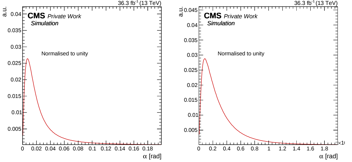
Figure 6.6: Distributions of the angle between the true and the reconstructed directions for jets (left) and leptons (right) used in the smearing for the full kinematic reconstruction.
