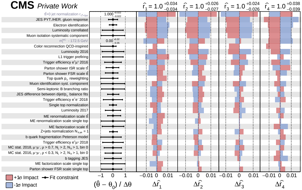
Figure 7.5: The fitted nuisance-parameter values and their impacts \Delta\hat{r}_k on the signal strengths \hat{r}_k from the fit to the data, ordered by their relative summed impact. Only the 30 highest ranked parameters are shown. The resulting fitted values of \hat{r}_k and their total uncertainties are also given. The nuisance-parameter values ( \hat{\theta} , black lines) are shown in comparison to their input values \theta_0 before the fit and relative to their uncertainty \Delta\theta . The impact \Delta\hat{r}_k for each nuisance parameter is the difference between the nominal best fit value of r_k and the best fit value when only that nuisance parameter is set to its best fit value \hat{\theta} while all others are left free. The red and blue lines correspond to the variation in \Delta\hat{r}_k when the nuisance parameter is varied up and down by its fitted uncertainty ( \Delta\theta ), respectively. The corresponding gray, red, and blue regions show the expected values from fits to pseudo-data. For the nuisance parameters associated with the t\bar{t}+0 jet normalization and m_t^{\text{MC}} , the values after the fit to the data are given, because no prior pdf is assigned.
