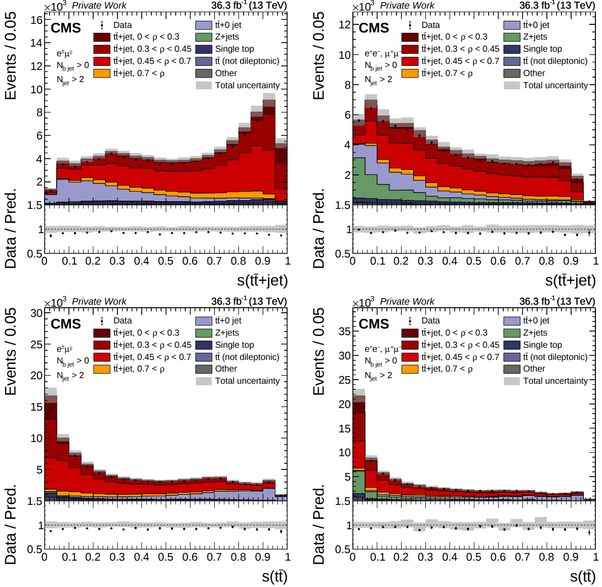
Figure 6.19: The observed (points) and MC predicted (stacked histograms) signal and background yields as a function of the signal (upper row) and t\bar{t} +0 jet (lower row) output node scores of the classifier NN. The left (right) column shows the e^{\pm}\mu^{\mp} (same-flavor) dilepton channel. The vertical bars on the points represent the statistical uncertainty in the data. The hatched band represents the total uncertainty in the sum of the simulated signal and background predictions. The lower panels show the ratio of the data to the sum of the signal and background predictions.
