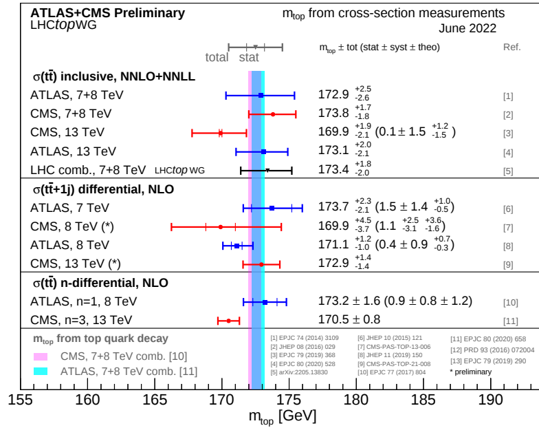
Figure 2.16: Recent results obtained by the LHC experiments on the value of the top quark pole mass [152].
