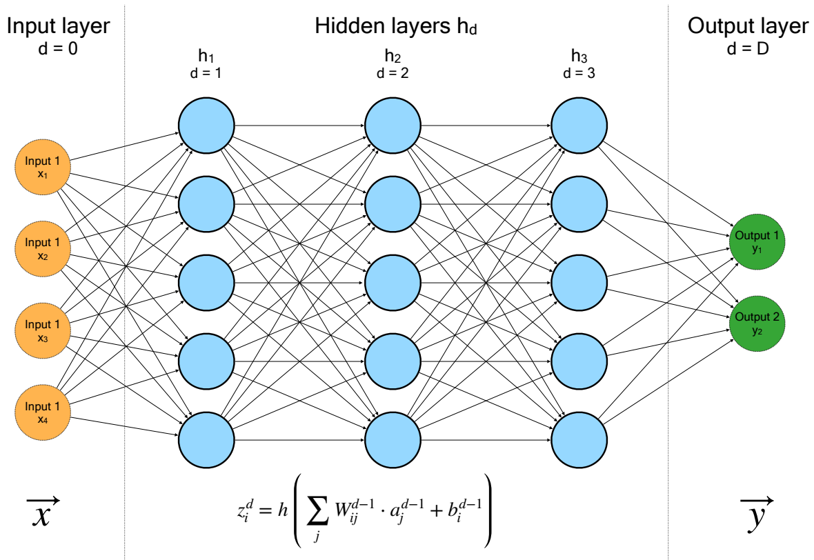
Figure 5.2: An illustration of a feedforward fully connected neural network. The orange (green) blobs indicate nodes of the input (output) layer with depth d = 0 ( d = D ), corresponding each to one input (output) variable. The blue blobs stand for nodes in the hidden layers with depth 0 < d < D .
