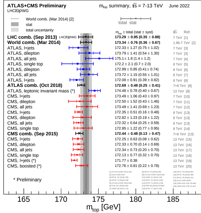
Figure 2.15: Recent results obtained by the LHC experiments on the value of m_t^{\text{MC}} [152].
