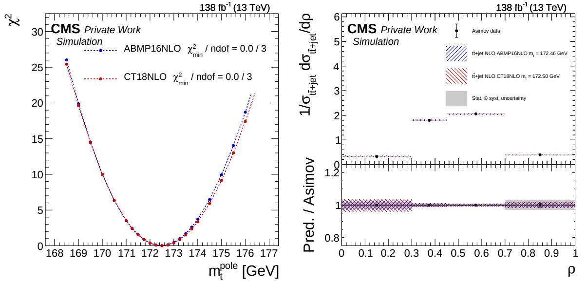
Figure 7.7: Left: the \chi^2 values versus m_t^{\text{pole}} from the fit of the measured normalized t\bar{t} +jet differential cross sections to the theoretical predictions using the ABMP16NLO (blue points) and CT18NLO (red points) PDF sets. The minimum \chi^2 value and the number of degrees of freedom (ndof) are given for each fit. Right: the expected measured normalized t\bar{t} +jet differential cross section (points) as a function of \rho , compared to the predictions using the two PDF sets and the corresponding best fit values for m_t^{\text{pole}} (hatched bands). The lower panel gives the ratio of the theoretical predictions to the measured values. For both panels, the vertical bars on the points show the statistical uncertainty in the Asimov data, the height of the hatched bands represent the theoretical uncertainties in the predictions, and the gray band gives the total uncertainty in the measured cross section.
