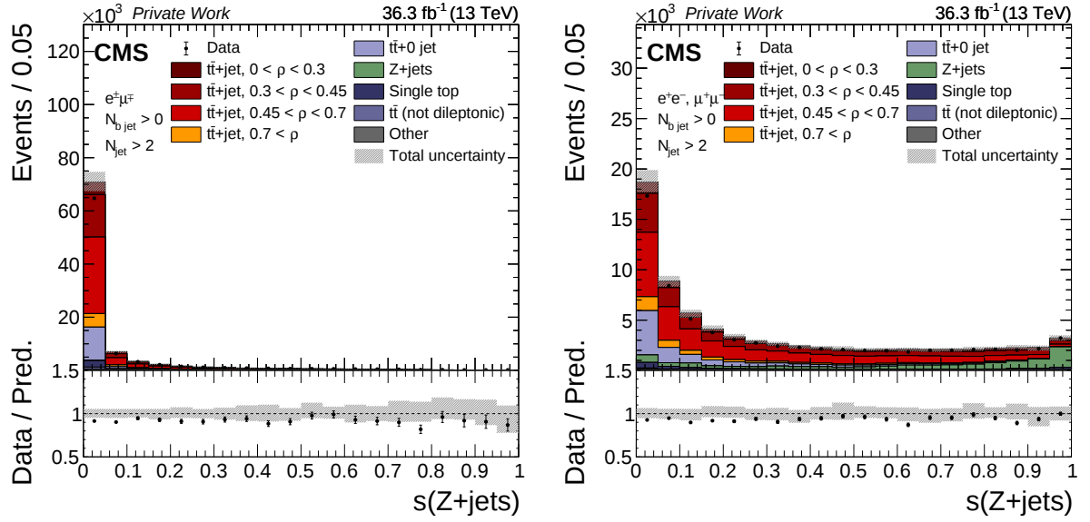
Figure 6.20: The observed (points) and MC predicted (stacked histograms) signal and background yields as a function of the Z+jets background output node. The left (right) plot shows the e^\pm \mu^\mp (same-flavor) dilepton channel. The vertical bars on the points represent the statistical uncertainty in the data. The hatched band represents the total uncertainty in the sum of the simulated signal and background predictions. The lower panels show the ratio of the data to the sum of the signal and background predictions.
