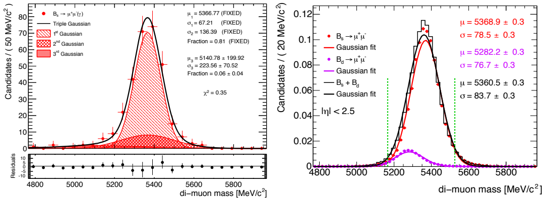
Fig. 8.25. Left: fit to the signal including the radiative component B_s^0 \rightarrow \mu^+ \mu^- \gamma . The first and second Gaussian are the same as in the exclusive fit, while the third takes care of the radiative tail. Right: fits to the signal mass distribution in the full pseudo-rapidity range for both the B_s^0 and the B^0 signals normalised to the relative (SM) production cross section ratio, as well as fit on the sum of these two distributions.
