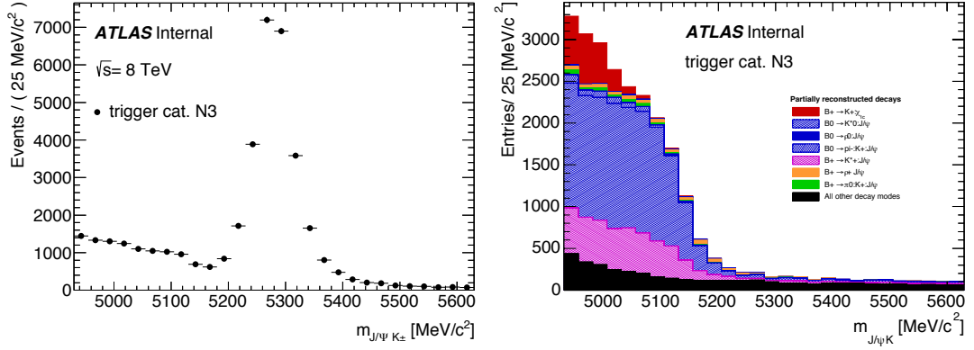
Fig. 8.20. Left: J/\psi K^\pm invariant mass distribution for all B^\pm candidates for the trigger category N_3 in 2012 data. Right: partially reconstructed B decays contributing to the background as described by MC.
