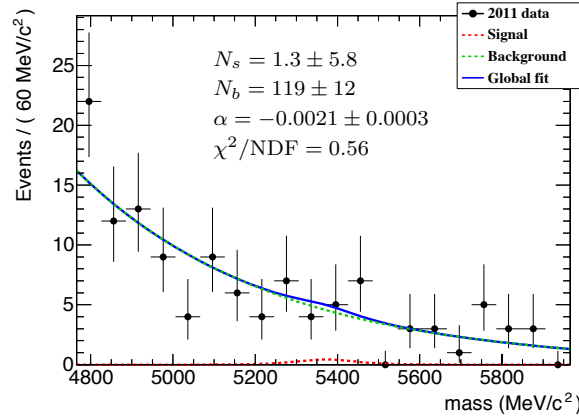
Fig. 6.15. Invariant mass fit on the 2011 un-blinded data for \text{BDT} > 0.08 optimised on 2011 MC events (the parameter \alpha is the slope of the exponential function).
