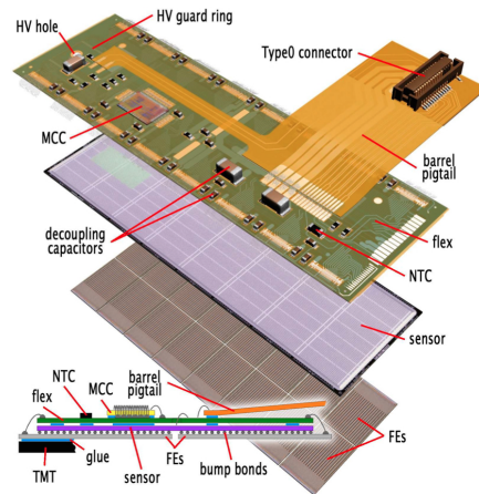
Fig. 2.13. Elements of a pixel barrel module [59].
