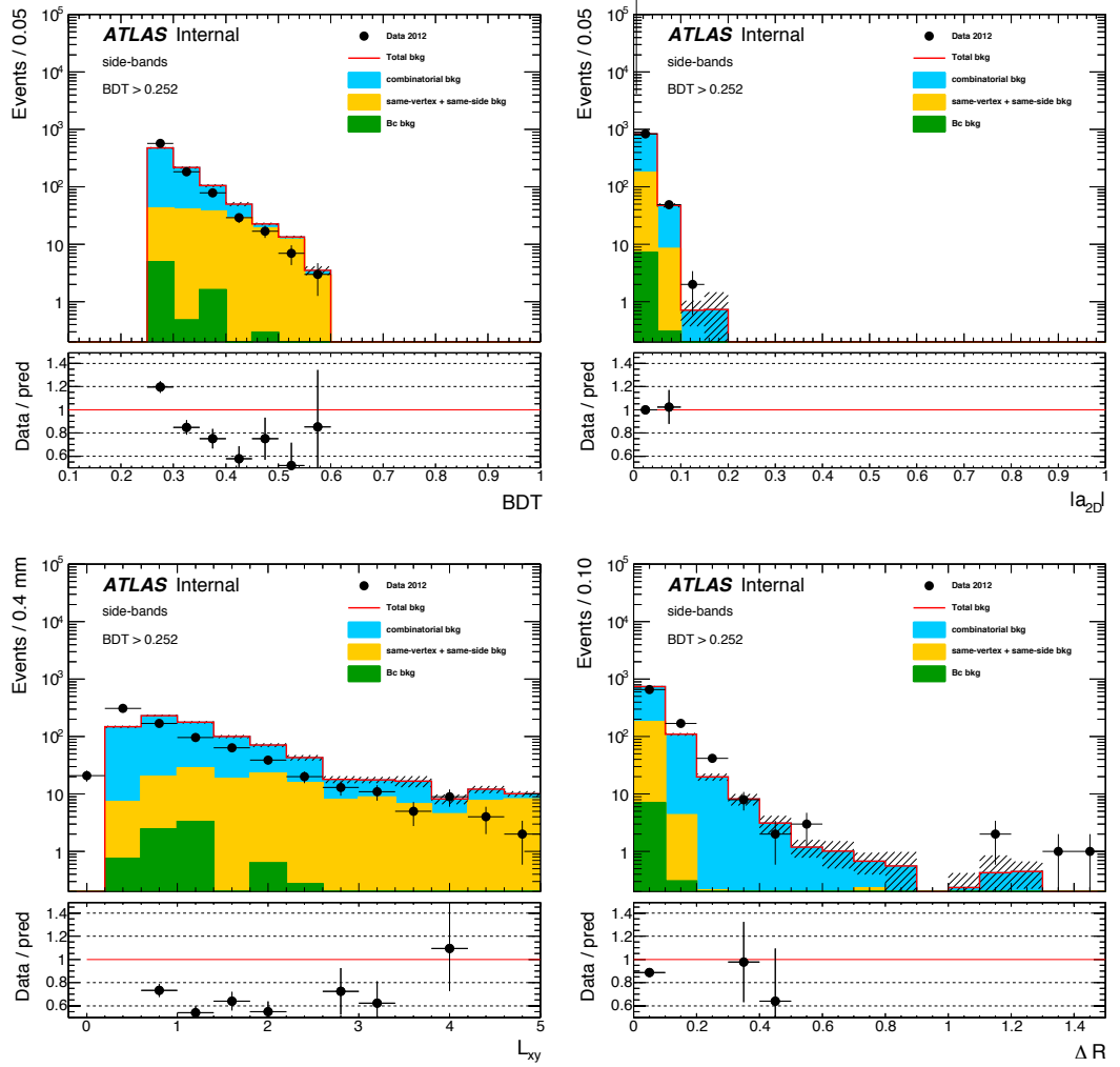
Fig. 8.30. Distributions of sideband data and four-corners MC sample after all selections, and after requiring the continuum-BDT > 0.252. The normalisation of the four-corners sample is done after the selection on continuum-BDT. From left to right, from top to bottom: continuum-BDT variable, \alpha_{2D} , L_{xy} and \Delta R .
