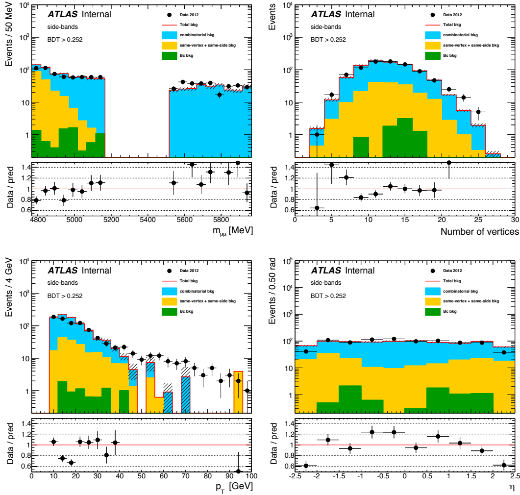
Fig. 8.29. Distributions of sideband data and four-corners MC sample after all selections, and after requiring continuum- BDT > 0.252 . The normalisation of the four-corners sample is done after the selection on continuum- BDT . From left to right, from top to bottom: invariant mass, number of primary vertices, B meson p_T and \eta .
