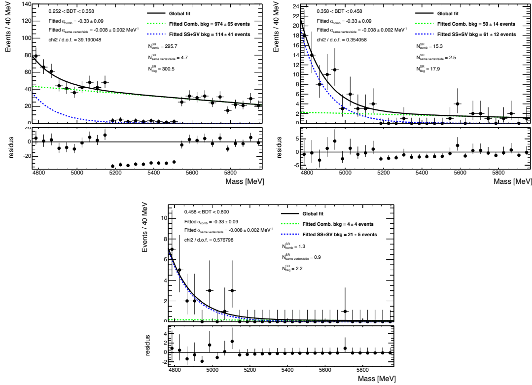
Fig. 8.36. Invariant mass distributions in sideband events superimposed with the fit to the two main background components.
