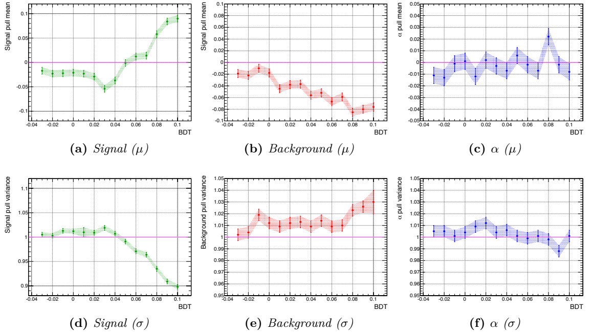
Fig. 6.13. Mean and variance of the pull distributions for the signal yield (left), background yield (middle) and background slope \alpha (right) obtained considering the 2011 statistic.
