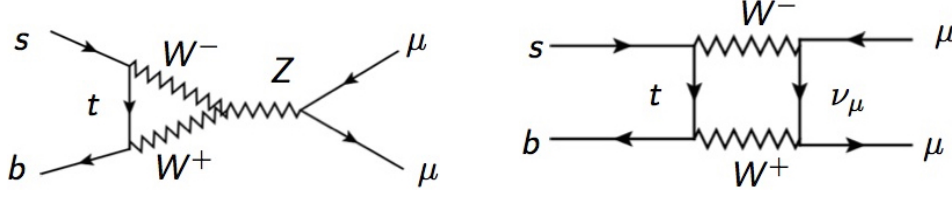
Fig. 1.5. Example of penguin (left) and box (right) diagrams.
