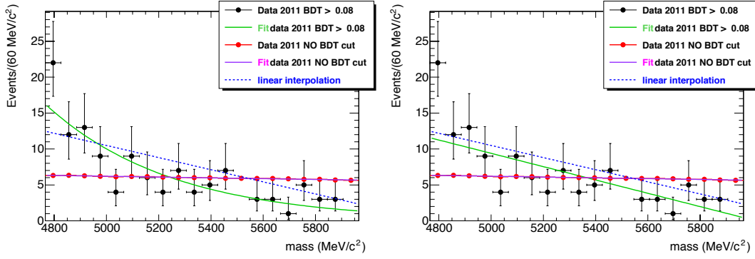
Fig. 6.29. Comparison of the linear interpolation (blue dashed lines) with the exponential (left) and linear (right) background mass fit (green solid lines) on 2011 un-blinded data for BDT > 0.08 . For shape comparison, the un-blinded dataset with no BDT selection applied (red dots), rescaled to the number of events obtained for BDT > 0.08 , is reported with the related exponential fit (violet solid lines).
