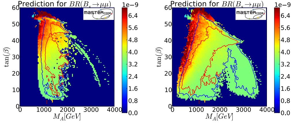
Fig. 1.10. Prediction of the B_s^0 \rightarrow \mu^+\mu^- branching ratio in the M_A - \tan\beta plane for CMSSM (left) and NUHM1 (right) models. The red (blue) contour shows the 68 % (95 %) CL exclusion obtained including the results from LHCb, CMS, ATLAS and CDF available in 2012 [45].
