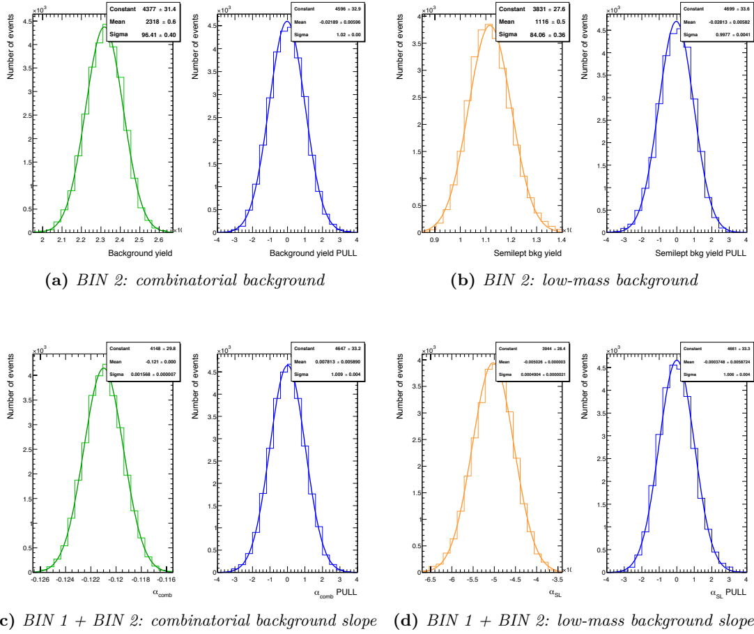
Fig. B.17. Distribution of the parameters of interest with the related pull for the BDT categorised invariant mass fit obtained running 30,000 toy MC experiments and generating the statistic expected in 2012 ( B_s and low-mass yields are fixed in the first bin).
