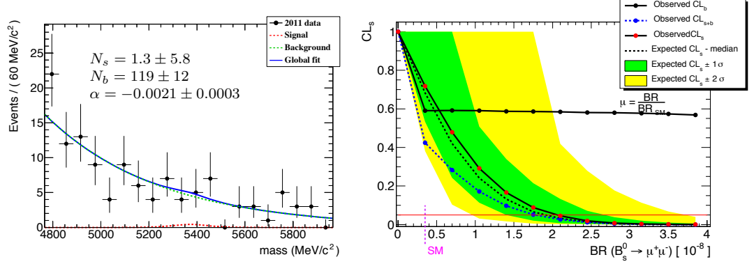
(b) CL_s on the un-blinded data modelling the background with an exponential function.
