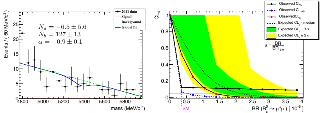
(c) CL_s on the un-blinded data modelling the background with a linear function.
