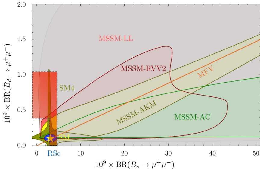
Fig. 1.11. Correlation between the branching ratios of B_s^0 \rightarrow \mu^+\mu^- and B_d \rightarrow \mu^+\mu^- in MFV, SM4 and four SUSY flavour models (see text) [50]. The grey area is excluded by the experiments (2012). The red area has been added to the original plot and takes into account of the latest combination presented by CMS and LHCb [28].
