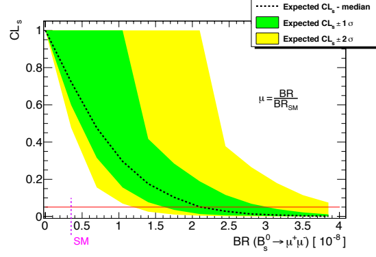
(a) Expected CL_s obtained with the blinded dataset.
