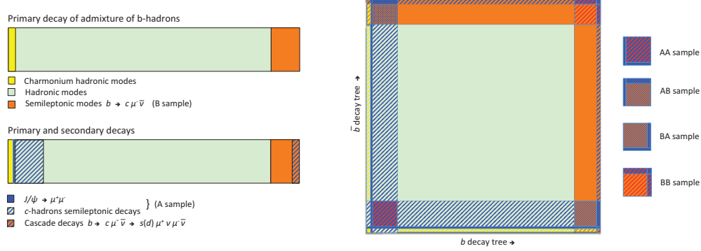
Fig. 8.4. Left: schematic diagram of the b decay channels: events are classified according to the presence of muons in the final state, distinguishing primary ( b -hadron) and secondary ( c -hadron) decays. Right: diagram of the combinations of b and \bar{b} decays: events containing muons from both decay trees are in the four corners, labelled as shown in the legend.
