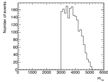
(c) Invariant mass of the \pi - \mu system.
