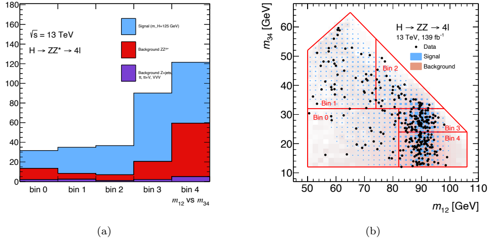
Figure 6.17: Expected m_{12} vs. m_{34} distribution of signal and ZZ^* background for 115 < m_{4\ell} < 130 GeV (a) and the corresponding bin boundaries (b). A SM Higgs with m_H = 125 GeV has been assumed, with a luminosity of 138.9 \text{ fb}^{-1} .
