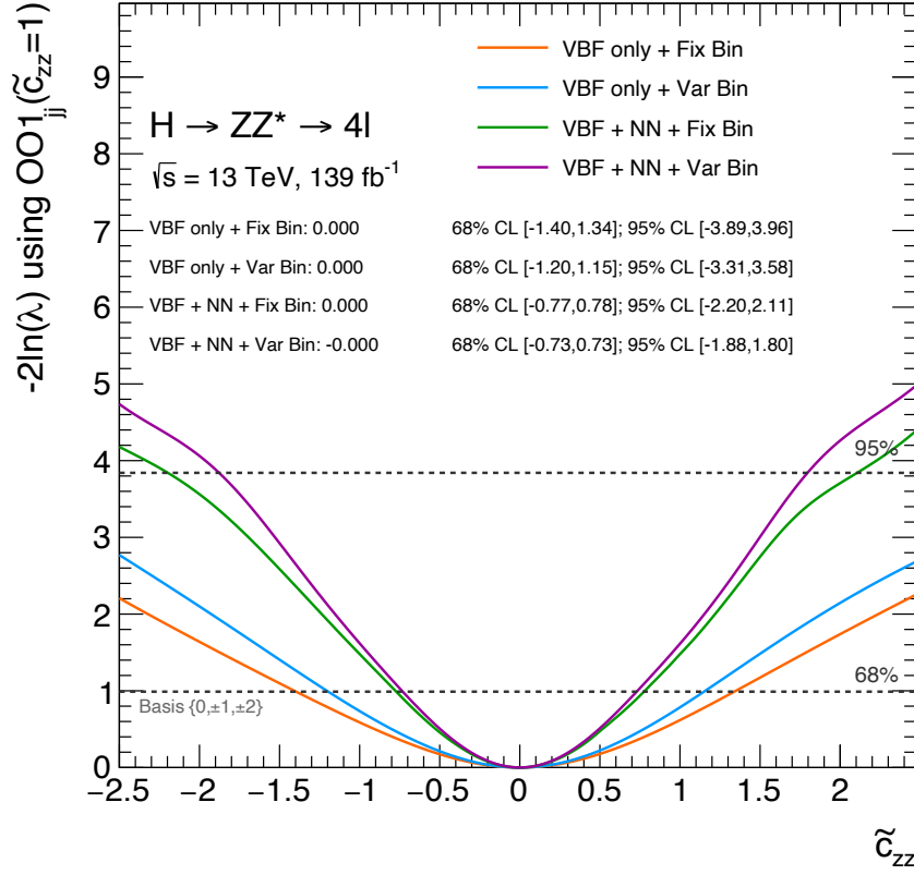
Figure 7.38: NLL comparison with different configurations: only VBF-enriched category using \mathcal{O}_{1,jj}(\tilde{c}_{zz} = 1) distribution with 12 equally sized bins (orange line), only VBF-enriched category using \mathcal{O}_{1,jj}(\tilde{c}_{zz} = 1) distribution with 12 equally populated bins (blue line) and adding NN categories (green and purple lines respectively)
