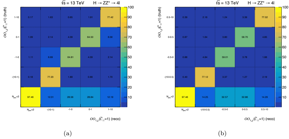
Figure 6.20: Migration matrices for the Optimal Observable \mathcal{OO}_{1,jj}(\tilde{c}_{zz} = 1) using two different binning choices: (a) [N_{jets} < 2, -10.0, -1.0, 0.0, 1.0, 10] and (b) [N_{jets} < 2, -10.0, -0.50, 0.0, 0.50, 10] . In the second case in which the external bin width is 9.5, the migration is larger with respect to first case with a bin width of 9; and the central bins show diagonal elements < 60\% . Figure 6.21a shows the middle case with binning choice [N_{jets} < 2, -10.0, -0.75, 0.0, 0.75, 10] , with an acceptable level of migration of the central bins.
