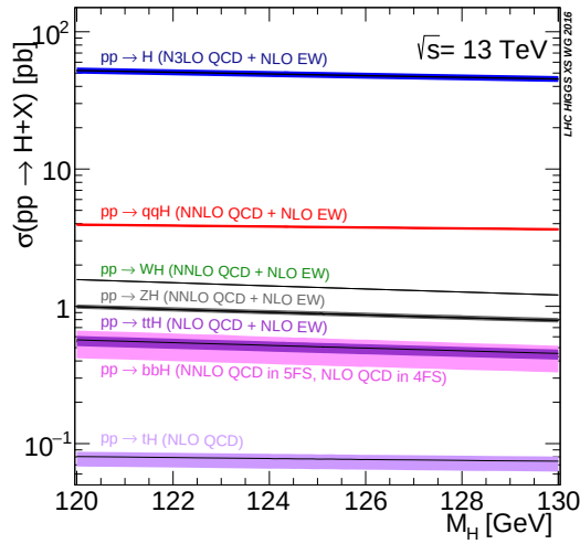
Figure 1.7: Standard Model Higgs boson production cross sections at \sqrt{s} = 13 TeV as a function of the Higgs boson mass [25].
