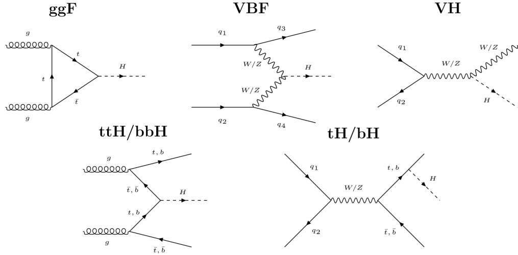
Figure 1.6: Examples of leading-order Feynman diagram for Higgs boson production via ggF, VBF, VH, ttH/bbH and tH/bH production processes.
