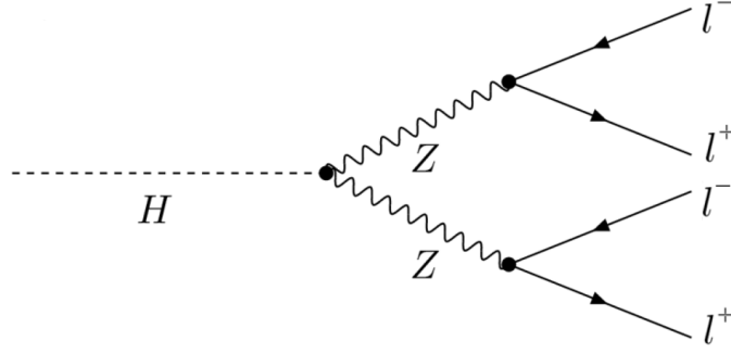
Figure 5.1: Feynman diagram of H \rightarrow ZZ^* \rightarrow 4l decay channel.
