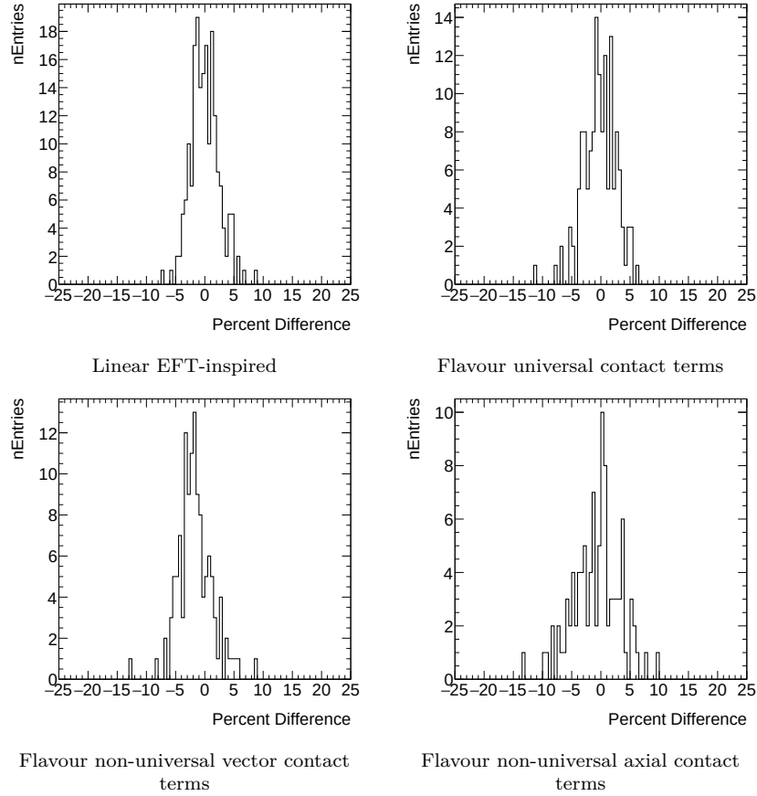
Figure 7.7: Percent difference between the two exclusion methods for all the interpretation scenarios.
