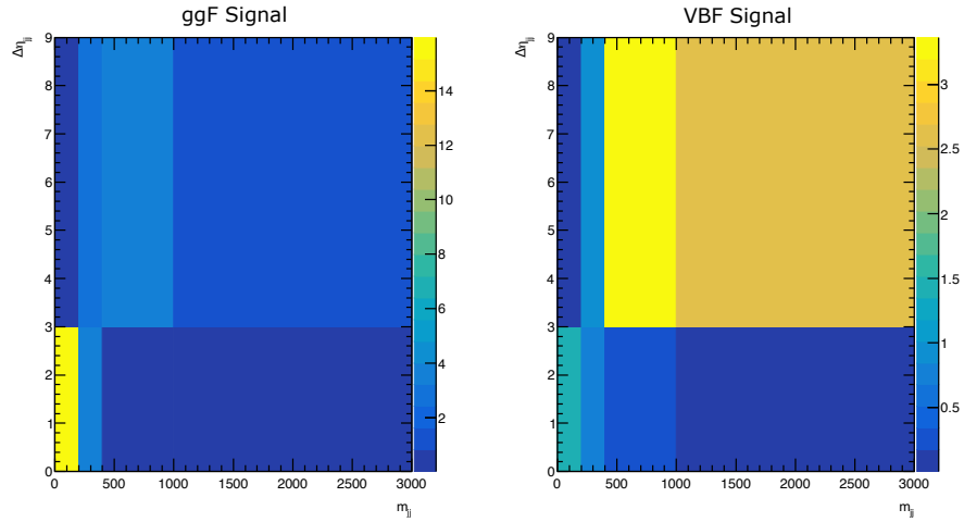
Figure 6.43: 2D events distribution for the ggF signal ( on the left ) and VBF signal ( on the right ) in m_{jj} vs. \Delta\eta_{jj} , in a mass region 115 < m_{4\ell} < 130 GeV.
