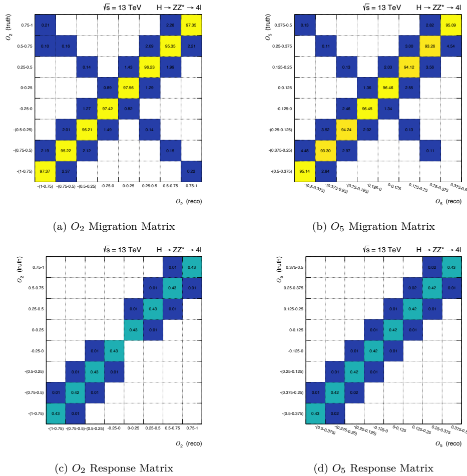
Figure 6.19: Migration and response matrices for or the CP-odd angular observable O_2 (a and c) and O_5 (b and d), evaluated using signal MC (mc16a+mc16d+mc16e) at m_H = 125 GeV for mass window of 105 < m_{4\ell} < 160 GeV (summing over all production modes). Only reconstructed events that have been matched to truth events are included.
