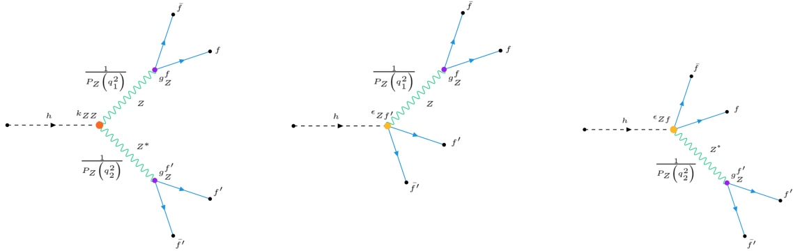
Figure 7.1: Feynman diagrams Pseudo-Observables.
