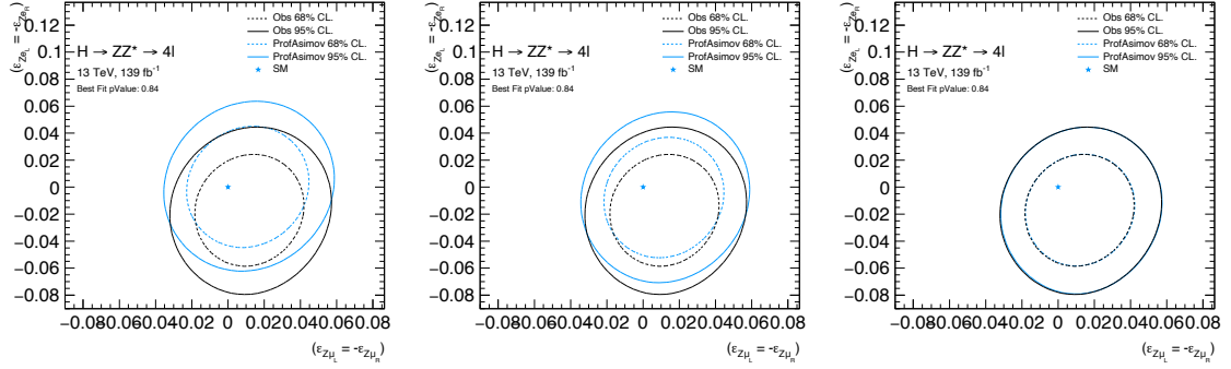
Figure 7.18: Observed exclusion limits (black lines) compared with ones obtained from the asimov dataset (blue lines) generated with \sigma_{bin3\ell\ell ee} equal to 1 (on the left), 0.8 (in the center), 0.58 (on the right) times the expected value, and the others XS equal to the SM value, in the non-universal axial contact terms scenario.
