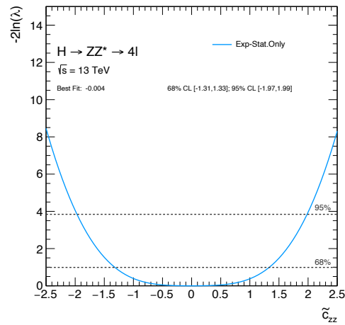
Figure 7.35: Expected NLL scan and expected exclusion limits for \tilde{c}_{zz} . The dashed horizontal lines represent the 68% CL and the 95% CL.
