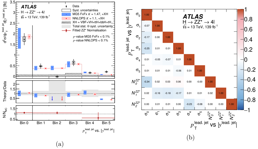
Figure A.32: a Double differential fiducial cross section for the transverse momentum of the leading jet vs. the rapidity of the leading jet, p_T^{\text{lead. jet}} vs. |y^{\text{lead. jet}}| , and b the corresponding correlation matrix between the measured cross sections and the ZZ^* background normalisation factors. The bin boundaries are defined in Figure A.15.
