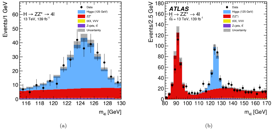
Figure 5.7: FSR-corrected m_{4\ell} distribution of the selected candidates, compared to the background expectation (a) in the low mass region and (b) in the whole mass spectrum of the analysis.
