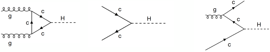
Figure 7.21: Feynman diagrams showing coupling between the Higgs boson and charm quark.
