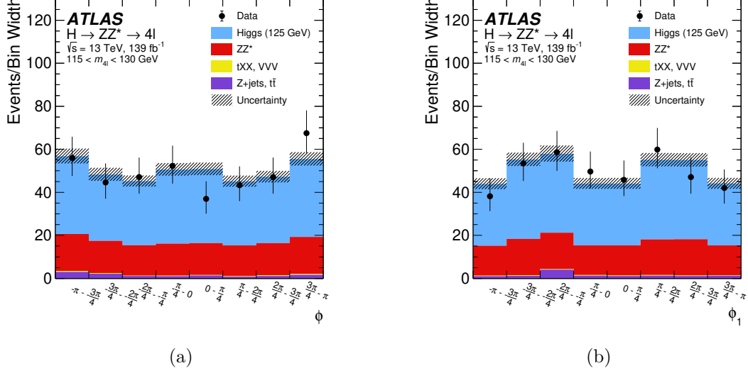
Figure A.4: The observed and expected (pre-fit) distributions of a \phi , and b \phi_1 in the mass region 115 < m_{4\ell} < 130 GeV, for an integrated luminosity of 139 \text{ fb}^{-1} collected at \sqrt{s} = 13 TeV. A SM Higgs boson signal with a mass m_H = 125 GeV is assumed. The uncertainty in the prediction is shown by the hatched band, which includes the theoretical uncertainties of the SM cross section for the signal and the ZZ^* background.
