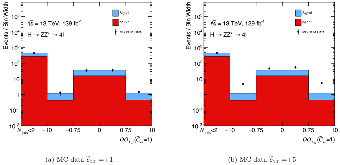
Figure 6.9: The SM expected distributions of the \mathcal{OO}_{1,jj}(\tilde{c}_{zz} = 1) in the range 105 < m_{4\ell} < 160 GeV compared with the BSM simulated data (black dots) for coupling value of (a) \tilde{c}_{zz} = +1 and (b) \tilde{c}_{zz} = +5 .
