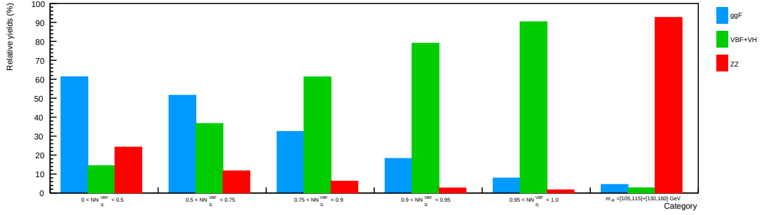
Figure 7.36: Expected percentage contribution of each process ggF, VBF + VH and ZZ* in each NN bin in the m_{4\ell} Signal Region and in the m_{4\ell} Control Region.
