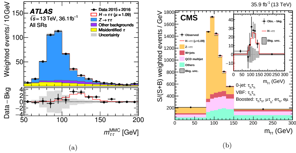
Figure 1.9: Distribution of the reconstructed di- \tau invariant mass m_{\tau\tau} from (a) ATLAS [31] and (b) CMS experiments [32].
