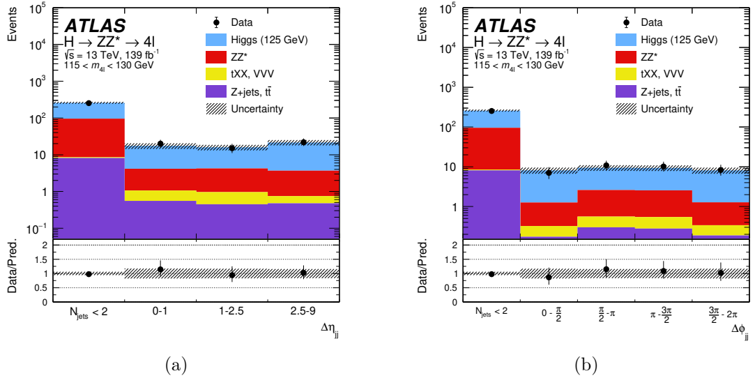
Figure A.7: The observed and expected (pre-fit) distributions of a \Delta\eta_{jj} , and b \Delta\phi_{jj} in the mass region 115 < m_{4\ell} < 130 GeV, for an integrated luminosity of 139 \text{ fb}^{-1} collected at \sqrt{s} = 13 TeV. A SM Higgs boson signal with a mass m_H = 125 GeV is assumed. The uncertainty in the prediction is shown by the hatched band, which includes the theoretical uncertainties of the SM cross section for the signal and the ZZ^* background.
