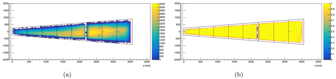
Figure 4.62: (a) Reconstructed track map and (b) efficiency map of software layer 0 (which corresponds to Layer 1 of the IP-side modules) from the cosmic results on A02.
