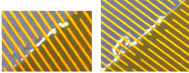
Figure 4.40: Damages due to the discharges along the piralux rim.
