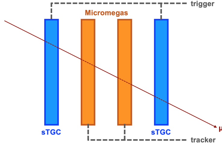
Figure 3.6: Detector order in z direction in the NSW: sTGC - MM - MM - sTGC.
