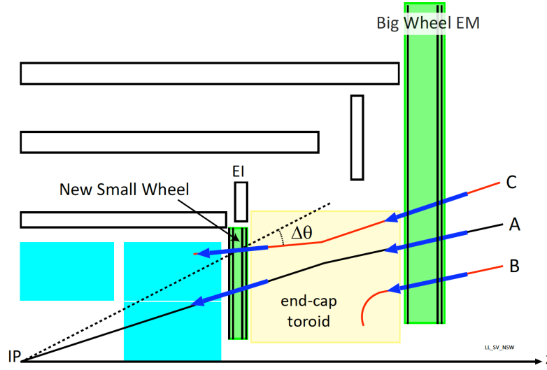
Figure 3.5: Schematic of the Muon endcap trigger. The existing Big Wheel trigger accepts all three tracks shown. With the NSW enhancement of the Muon endcap trigger only track ‘A’, the desired track, which is confirmed by both the Big Wheel and the New Small Wheel, will be accepted. Track ‘B’ will be rejected because the NSW does not find a track coming from the interaction that matches the Big Wheel candidate. ‘C’ will be rejected because the NSW track does not point to the interaction point. The NSW logic requires that \Delta\theta < \pm 7 mrad
