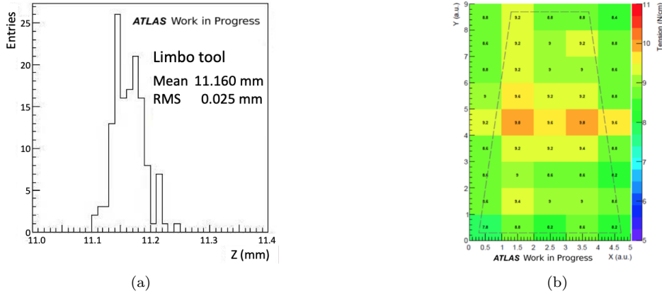
Figure 4.3: (a) Measurement of the thickness and planarity for a drift panel and (b) the mesh tension map.
