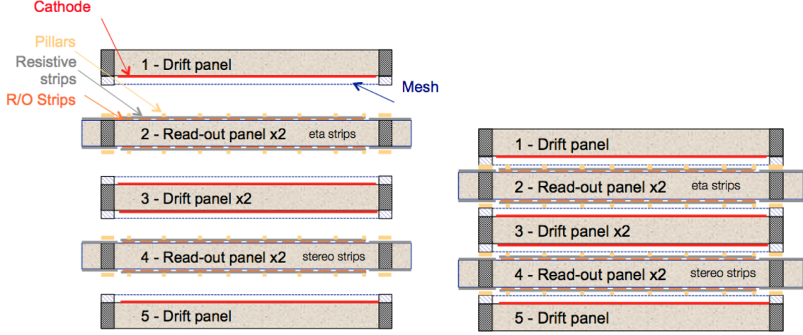
Figure 3.14: A schematic view of the five panels of a MM quadruplet.
