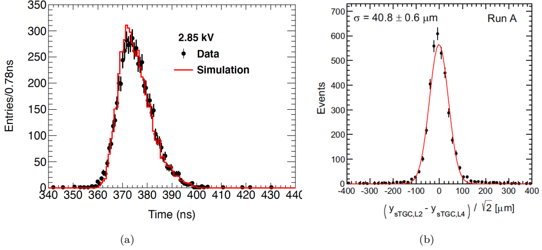
Figure 3.9: Comparison of a simulated time spectrum with experimental data taken using wire voltage of 2.85 kV (a). The horizontal axis has an arbitrary offset [7]. In (b) the resolution estimate based on adjacent sTGC strip-layer position residual distributions for a representative sTGC standalone data taking run is reported [81].
