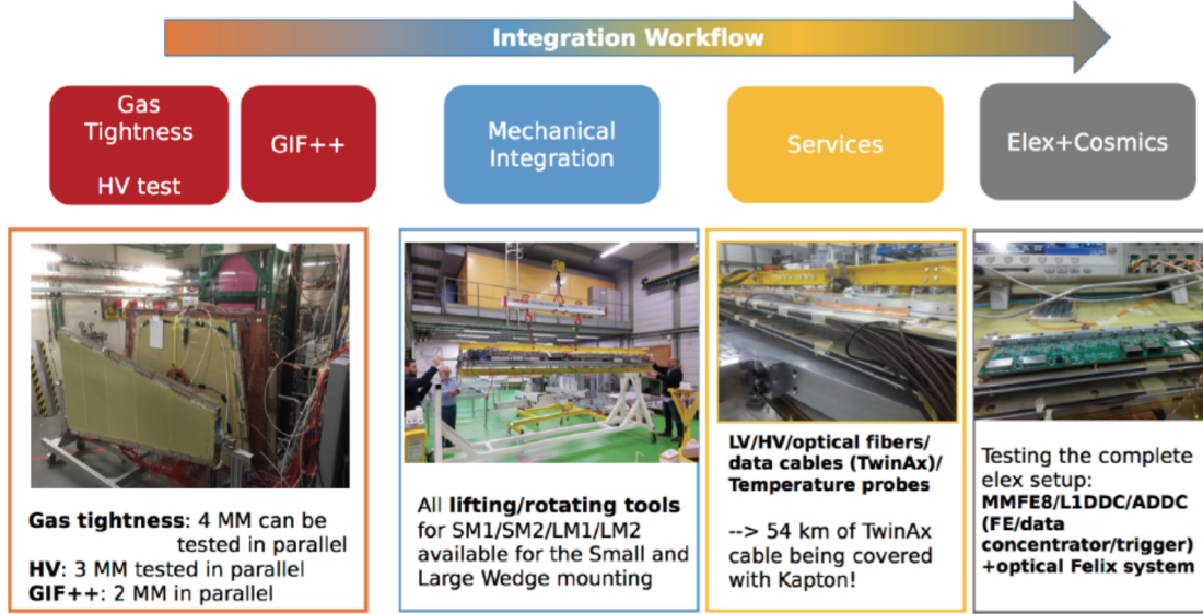
Figure 4.53: Micromegas modules integration workflow at CERN Building BB5.
