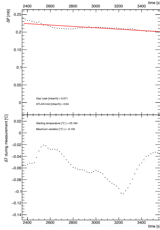
Figure 4.16: Pressure drop plot to measure the gas tightness of the chamber. The red line represent the linear fit to extrapolate the gas leak measurement. The bottom panel shows the Clean Room temperature variation during the measurement.
