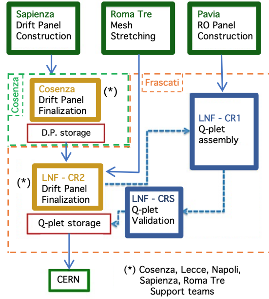
Figure 4.1: INFN production scheme of SM1.
