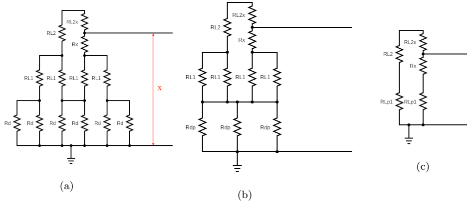
Figure 4.45: Sketch of the PCB circuit with approximation used to built the recursive model. The three figure show the equivalent circuits of the first one (a) after the resistance re-definitions.
