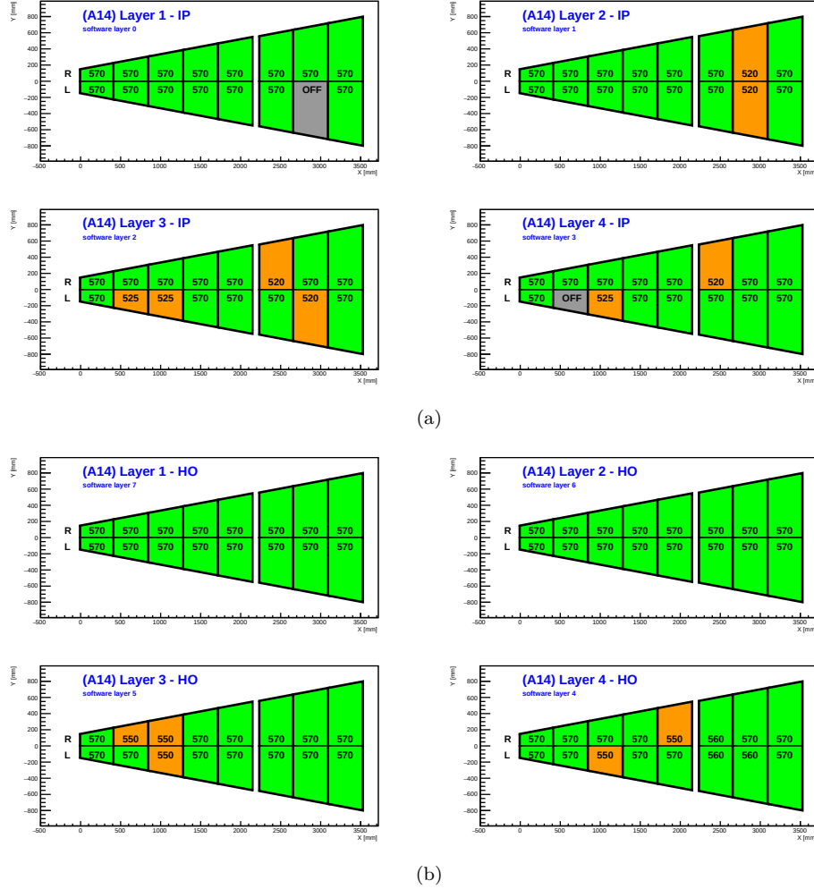
Figure 4.58: Final HV map of the Double Wedge A14: (a) IP and (b) HO side.
