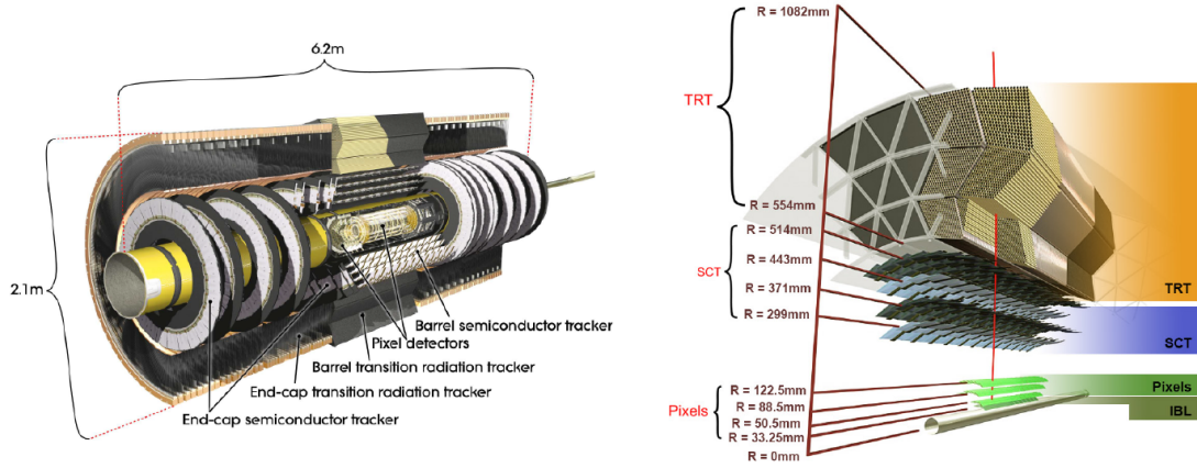
Figure 2.5: The ATLAS Inner Detector (ID) scheme [3]. On the right is shown a detailed layout of the ID including the new Insertable B-Layer (IBL).
