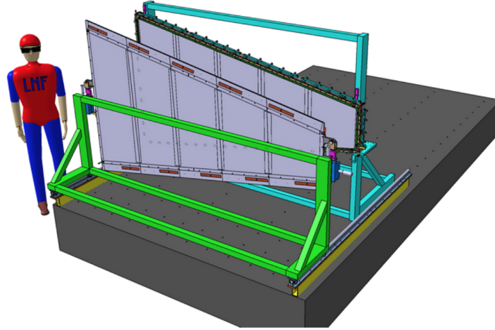
Figure 4.6: Picture of the assembly tool installed in the Clean Room at LNF.
