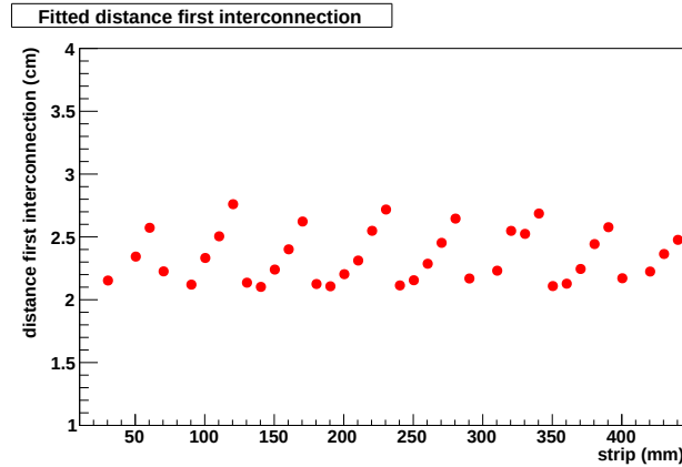
Figure 4.49: First interconnection distance d obtained from the fit on the measured resistance along the strips.
