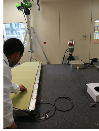
(b) Data acquisition with Laser Tracker
