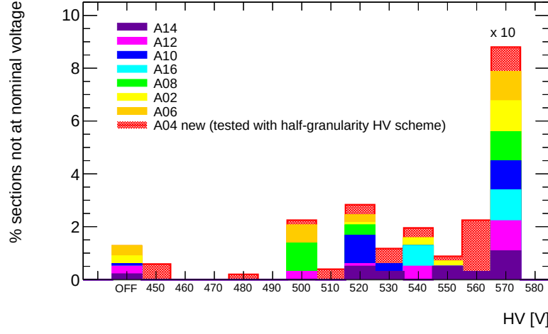
Figure 4.61: Summary of the HV values applied at each section of all the Small Double Wedges including the new A04 tested with the half-granularity HV scheme. The plot shows the percentage of the sections connected at a given HV value. The data at 570 V have to be scales \times 10 .
