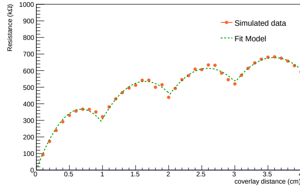
Figure 4.47: Strip resistance as function of the distance from the coverlay in the simulated data fitted with the recursive model.
