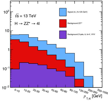
Figure 6.11: Distribution and binning choice for p_T : for each bin, signal and background yields are reported for 115 < m_{4\ell} < 130 GeV together with S/B and expected significance values. A SM Higgs with m_H = 125 GeV has been assumed.
