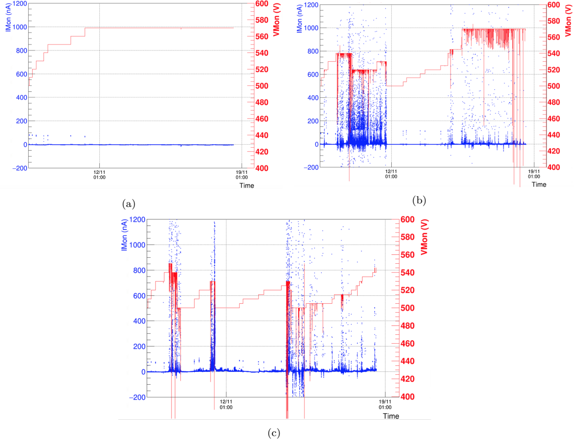
Figure 4.21: Different HV behaviour. Each plot show in red the monitored HV (VMon) and in blue the monitored current (IMon). In (a) it is shown an example of a good sector. In particular in this plot it can be seen also the ramp-up step at the beginning of the plot. In (b) it is shown an example of a sector which shows a bad HV behaviour at the beginning. For this reason the HV has been lowered up to 500 V, when it became again stable. Then the ramp up procedure has been performed again and the sector reached 580 V showing a number of spark < 6/min, and it has been left at this HV value to condition. In (c) it is shown an example of a bad behaving section. This plot shows the continuous HV drops due to the sparks which can be recovered just lowering the HV up to 500 V, and finally show a spiky behaviour even at this HV value.
