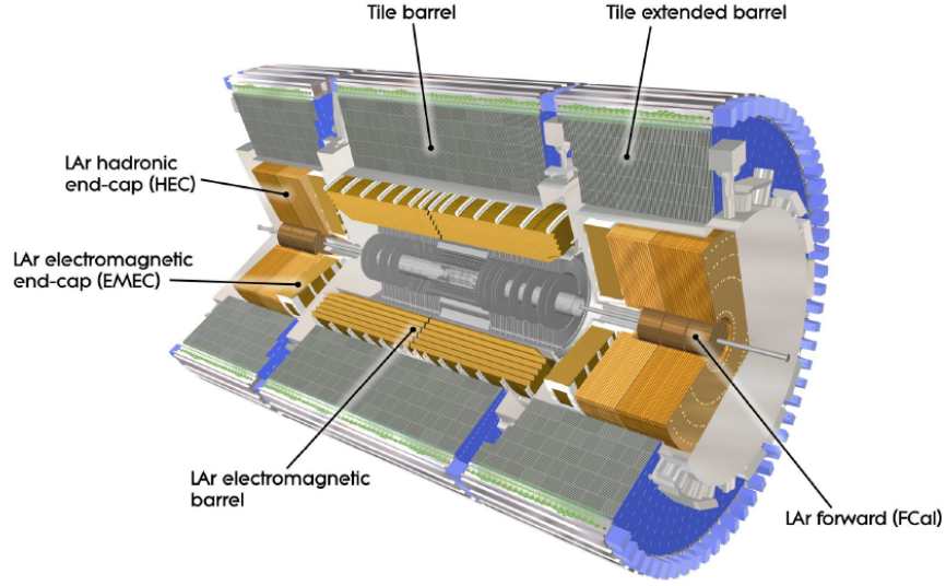
Figure 2.6: The ATLAS Calorimeter System [3] .
