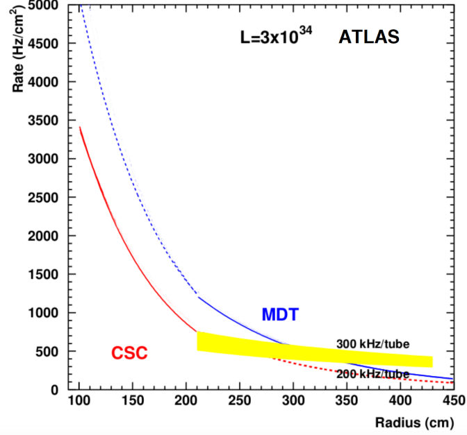
Figure 3.2: Extrapolated hit rate in the CSC and MDT regions for a luminosity of 3 \times 10^{34} \text{ cm}^{-2}\text{s}^{-1} at \sqrt{s}=7 \text{ TeV} as a function of the radial distance from the beam line. The yellow band is the range of tube rates of 200-300 kHz [7].
