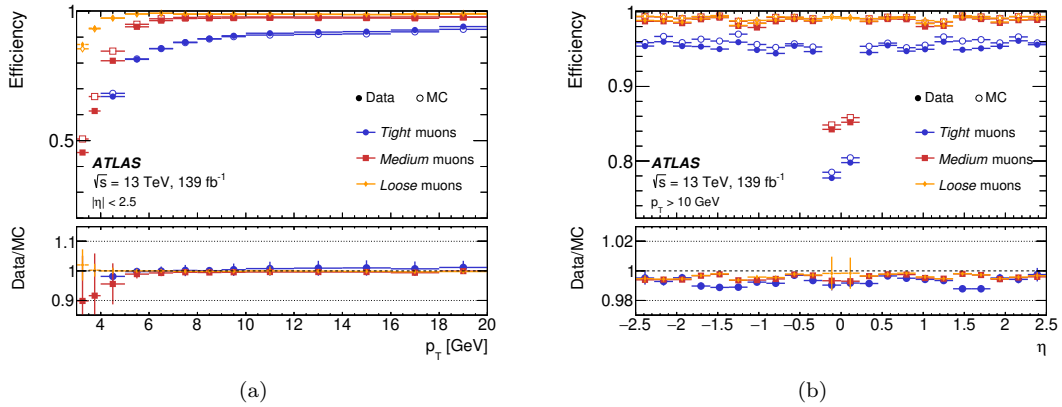
Figure 2.13: Muon reconstruction and identification efficiency for Loose , Medium and Tight criteria (a) from J/\psi \rightarrow \mu\mu events as function of p_T and (b) from Z \rightarrow \mu\mu events as function of \eta for muons with p_T > 10 GeV (on the right) [77].
