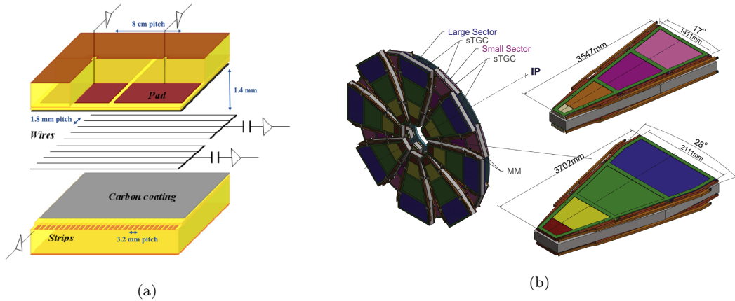
Figure 3.8: Schematic diagram of the basic sTGC structure (a) and the scheme of the small and large sectors that make up the New Small Wheel (b). Each sector consists of two quadruplets of sTGC with eight Micromegas(MM) detector plane in between [81].
