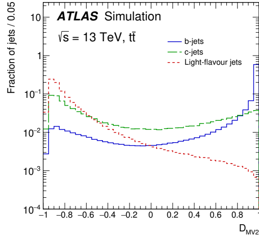
Figure 2.14: The b-tagging discriminant used to distinguish b -jets from jets containing charm and other light flavours. [80].
