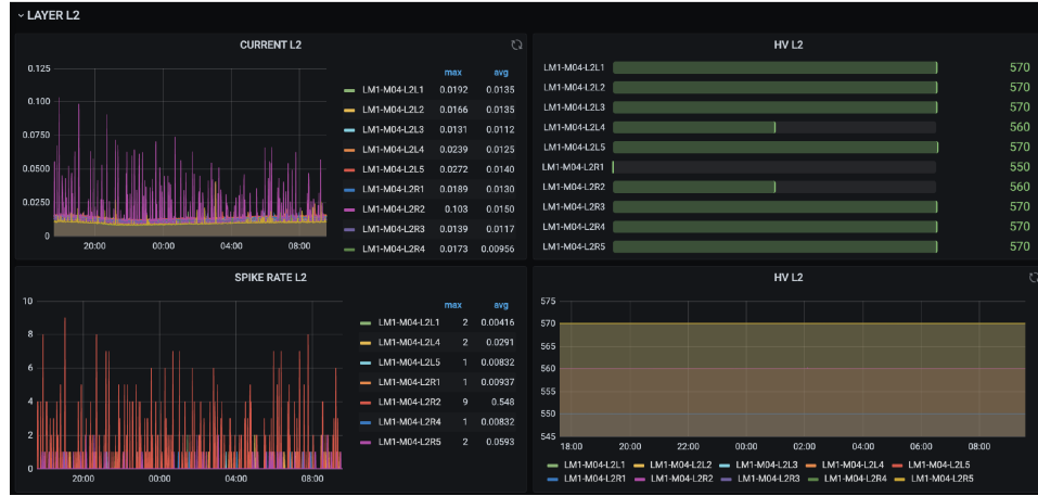
Figure 4.20: HV monitoring system used at LNF to perform the HV test uses Grafana dashboard to monitor the currents of different HV sections.
