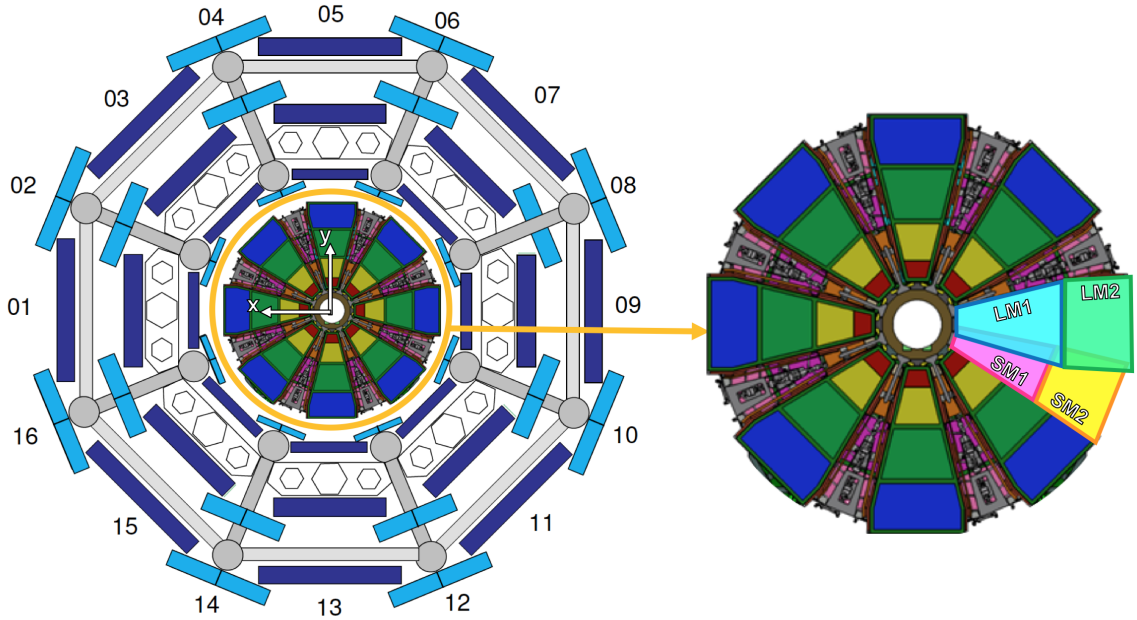
Figure 3.7: The left picture show the barrel scheme with the definition of the 16 sectors of the ATLAS muon spectrometer (dark blue sectors represent the large sectors, the light blue represent the small ones). Inside of the barrel scheme a sketch of the NSW is represented and the detailed view is shown in the right picture. This shows the 8 large sectors in which only the sTGC wedge are visible. The large and small MM sectors with the corresponding LM1, LM2, SM1 and SM2 modules segmentation are also represented.
