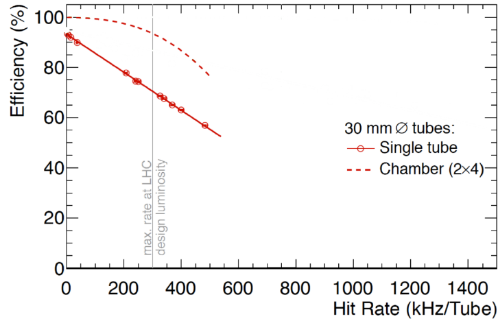
Figure 3.3: MDT tube hit (solid line) and track segment efficiency (dashed line, referring to a MDT chamber with 2x4 tube layers) as a function of tube rate estimated with test-beam data. Instantaneous luminosity of 1 \times 10^{34} \text{ cm}^{-2}\text{s}^{-1} is referred in this plot as ‘design luminosity’. Points on the plots are result of test beam measurements [7].
