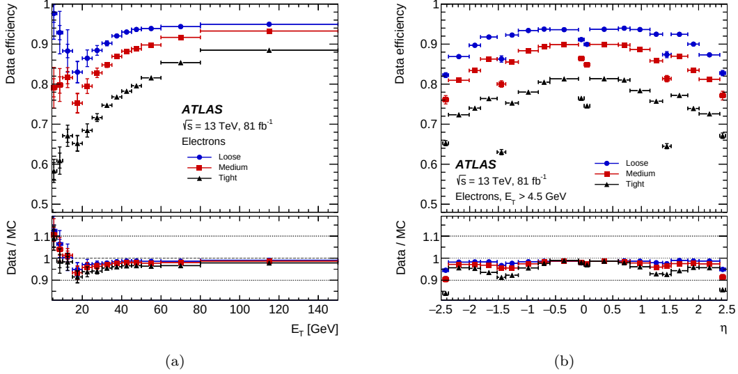
Figure 2.12: The efficiency to identify electrons from Z \rightarrow ee decays as function of (a) E_T and as function of (b) \eta for Loose, Medium and Tight operating point [75].
