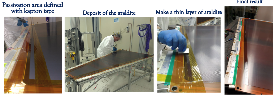
Figure 4.41: Different steps of the passivation procedure.
