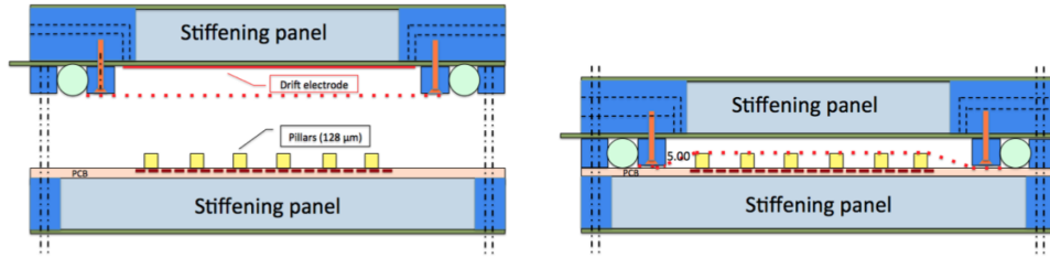
Figure 3.12: Schematic of a single MM plane assembly. On the left : the drift panel (top) and the readout panel (bottom) are shown in open position. The mesh is an element integrated in the drift panel, glued on an aluminum frame (the mesh frame). On the right : the drift panel is coupled up to the readout panel.
