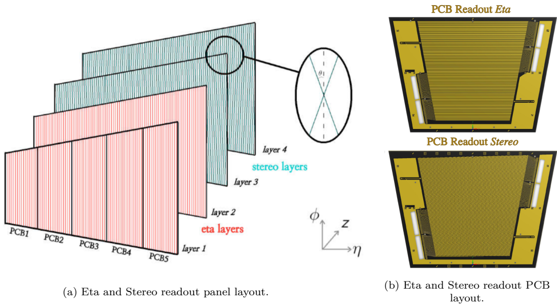
Figure 3.15: Layout of the Eta and Stereo readout (a) panel and (b) PCB.
