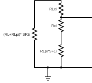
Figure 4.46: Sketch of the PCB circuit used to built the recursive model.
