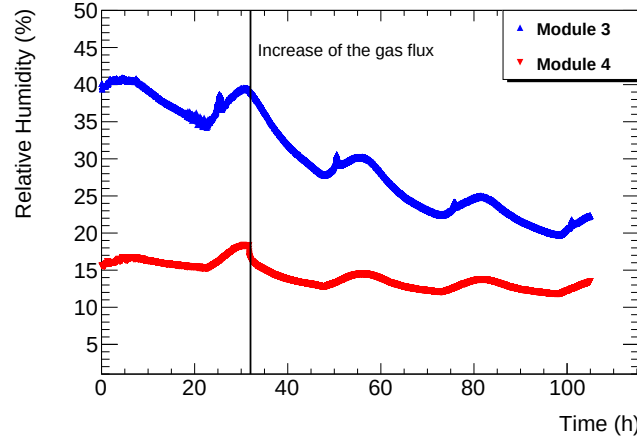
Figure 4.32: Relative humidity in time of the SM1 modules M3 and M4 connected in series (M3→M4). It shows the decrease of the RH with the increase of the gas flux.
