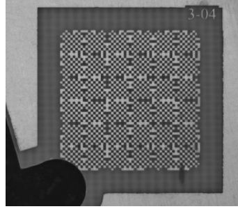
Figure 4.17: Rasmask installed on the PCBs.
