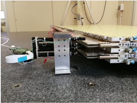
(a) 4-Rasfork setup during a measurement.
