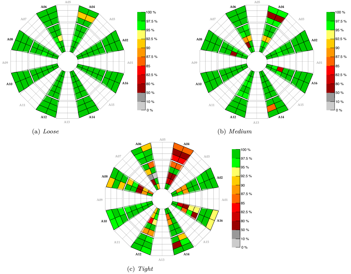
Figure 4.65: 2D map of the segment reconstruction efficiency using the small Micromegas DWs of the NSW-A for three different working points: (a) Loose , (b) Medium and (c) Tight . This efficiency has been computed using the theoretical curve extrapolated from the average efficiency curve of the Small Double Wedges, based on the HV maps of each DW.
