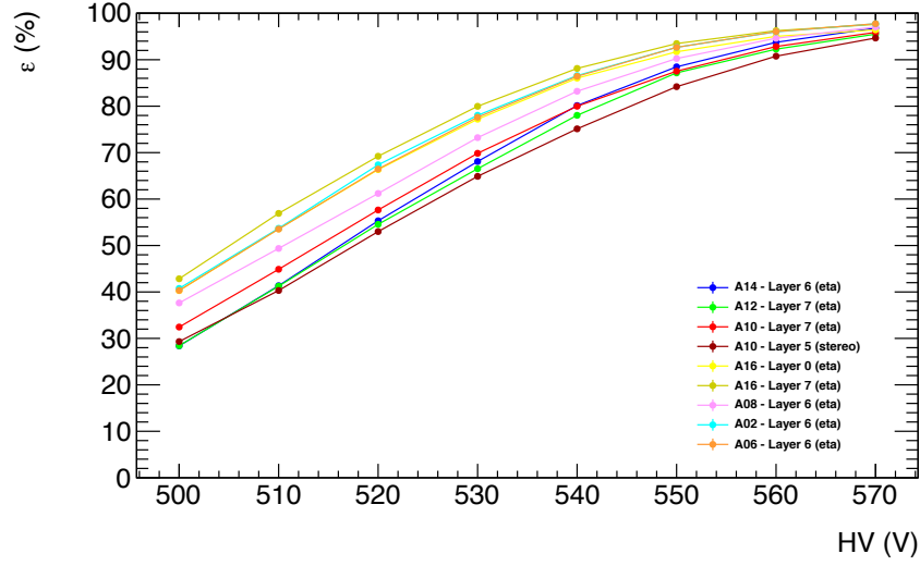
Figure 4.63: Measured layer efficiency as a function of the HV on the Small Double Wedges.
