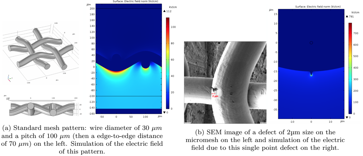
Figure 4.33: Comparison of mesh electric field simulation in presence of mesh imperfections with nominal.
