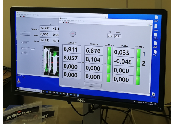
(b) Monitoring of the weight loaded on the two pins using load cells.
