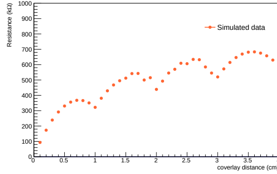
Figure 4.44: Strip resistance as function of the distance from the coverlay in the simulated data.
