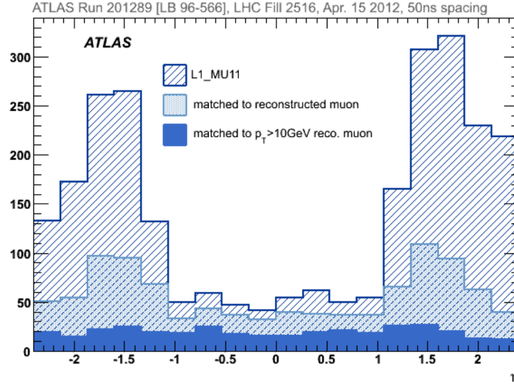
Figure 3.4: \eta distribution of Level-1 muon signal ( p_T > 10 GeV) (L1_MU11) with the distribution of the subset with matched muon candidate (within \Delta R < 0.2 ) to an offline well reconstructed muon (combined inner detector and muon spectrometer track with p_T > 3 GeV), and offline reconstructed muons with p_T > 10 GeV [7].
