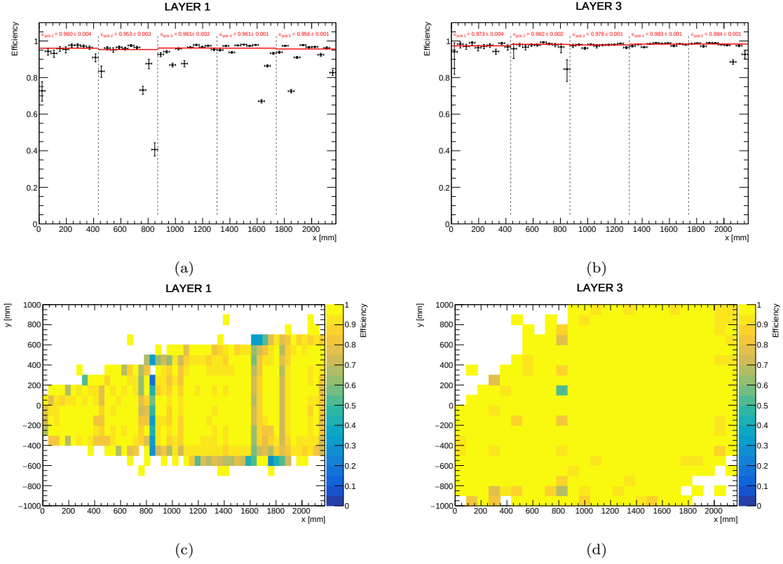
Figure 4.24: 1D e 2D efficiency plot per Layer 1 and Layer 3.
