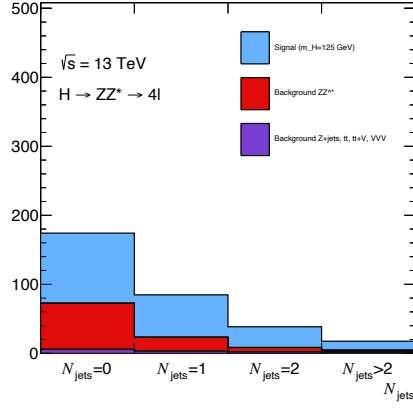
Figure 6.13: Distribution and binning choice for N_{\text{jets}} : for each bin, signal and background yields are reported for 115 < m_{4\ell} < 130 GeV together with S/B and expected significance values. A SM Higgs with m_H = 125 GeV has been assumed.
