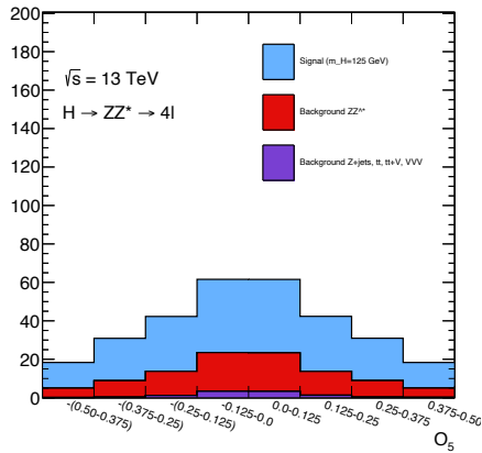
Figure 6.23: Distribution and binning choice for O_5 : for each bin, signal and background yields ( ggZZ^* , t\bar{t}V + VVV not included) are reported for 115 < m_{4\ell} < 130 GeV together with S/B and expected significance values.
