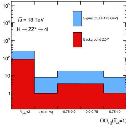
Figure 6.24: Distribution and binning choice for \mathcal{OO}_{1,jj}(\tilde{c}_{zz} = 1) : for each bin, signal and background yields (only qqZZ^* ) are reported for 115 < m_{4\ell} < 130 GeV together with S/B and expected significance values.
