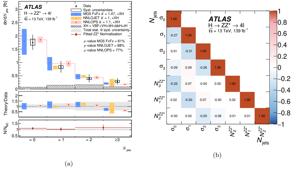
Figure 6.36: (a) Differential fiducial cross section for the number of jets N_{\text{jets}} , along with (b) the corresponding correlation matrix between the measured cross sections and the ZZ^* background normalisation factors.
