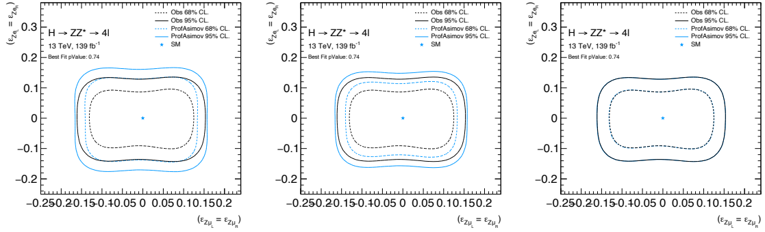
Figure 7.19: Observed exclusion limits (black lines) compared with ones obtained from the asimov dataset (blue lines) generated with \sigma_{bin3\ell\ell ee} equal to 1 (on the left), 0.8 (in the center), 0.58 (on the right) times the expected value, and the others XS equal to the SM value, in the non-universal vector contact terms scenario.
