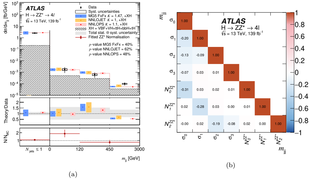
Figure 6.37: (a) Differential fiducial cross section for the di-jet invariant mass m_{jj} , along with (b) the corresponding correlation matrix between the measured cross sections and the ZZ^* background normalisation factors.
