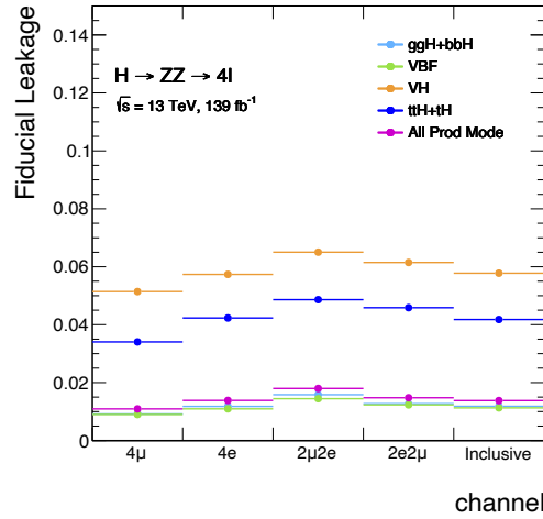
Figure 6.7: Comparing the fiducial leakage at m_H = 125 GeV using the dressed truth lepton definition in the mass range 105 < m_{4\ell} < 160 GeV for different production mode in the four final states.
