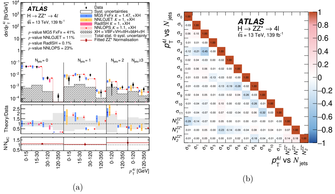
Figure A.26: a Double differential fiducial cross sections of the p_T^{4\ell} distribution in N_{\text{jets}} bins. The corresponding correlation matrix between the measured cross sections and the ZZ^* background normalisation factors is shown in b . The p -values shown are calculated for all bins across both p_T^{4\ell} and N_{\text{jets}} simultaneously.
