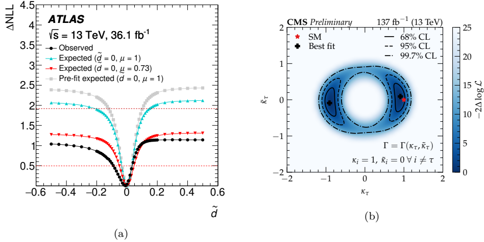
Figure 1.16: (a) The observed and expected negative log-likelihood (NLL) scan curve as a function of \tilde{d} values [46]. (b) Two-dimensional scan of CP-even \kappa_\tau and CP-odd \tilde{\kappa}_\tau Yukawa coupling between Higgs boson and \tau lepton [47].
