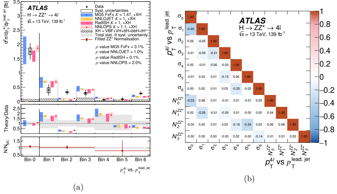
Figure A.30: a Double differential fiducial cross section for the transverse momentum of the four-lepton system vs. the transverse momentum of the leading jet, p_T^{4\ell} vs. p_T^{\text{lead, jet}} , and b the corresponding correlation matrix between the measured cross sections and the ZZ^* background normalisation factors. The bin boundaries are defined in Figure A.13.
