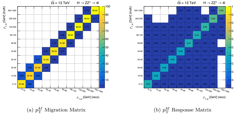
Figure 6.12: (a) Migration and (b) response matrix for p_T^{4\ell} , evaluated using signal MC (mc16a+mc16d+mc16e) at m_H = 125 GeV for mass window of 105 < m_{4\ell} < 160 GeV (summing over all production modes). Only reconstructed events that have been matched to truth events are included.
