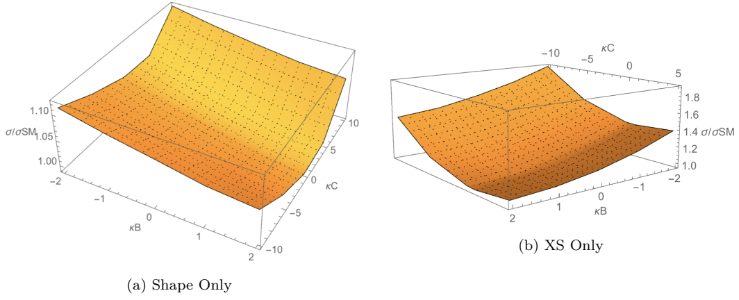
Figure 7.23: Modification of the predicted XS in different bins of p_T^H as a function of \kappa_b and \kappa_c .
