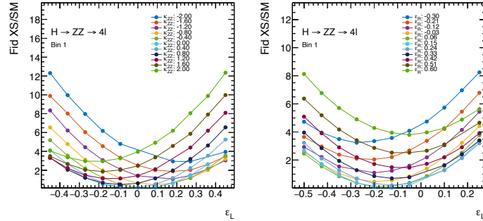
Figure 7.17: Modification of the predicted cross section in bin1 of m_{12} vs. m_{34} distribution as function of the \epsilon_L for Linear-EFT (on the left) and universal contact terms (on the right) scenarios.
