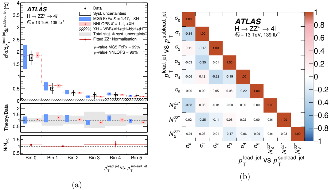
Figure A.31: a Double differential fiducial cross section for the transverse momentum of leading vs. subleading jet, p_T^{\text{lead, jet}} vs. p_T^{\text{sublead, jet}} , and b the corresponding correlation matrix between the measured cross sections and the ZZ^* background normalisation factor. The bin boundaries are defined in Figure A.14.
