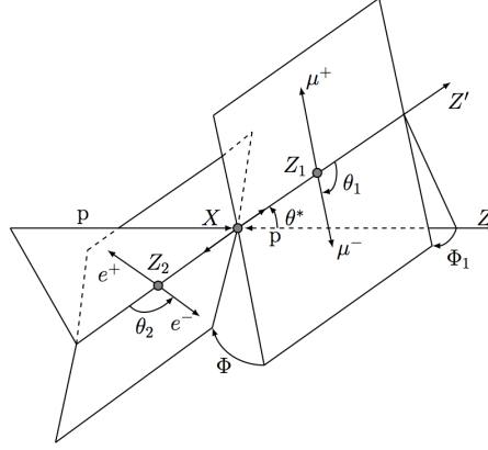
Figure 6.1: Diagram of decay angles for the H \rightarrow 4\ell decay.
