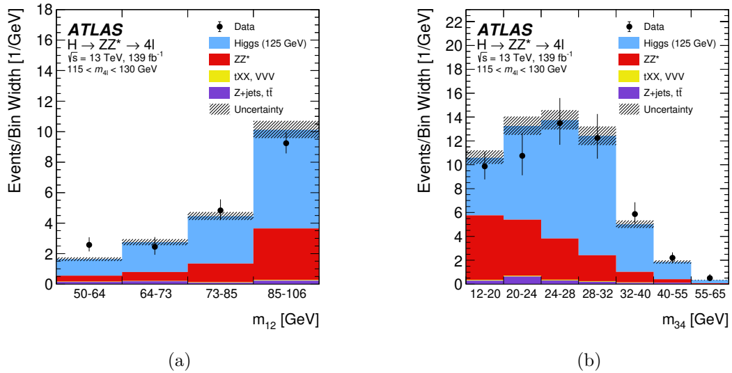
Figure A.1: The observed and expected (pre-fit) distributions of a m_{12} , and b m_{34} in the mass region 115 < m_{4\ell} < 130 GeV, for an integrated luminosity of 139 \text{ fb}^{-1} collected at \sqrt{s} = 13 TeV. A SM Higgs boson signal with a mass m_H = 125 GeV is assumed. The uncertainty in the prediction is shown by the hatched band, which includes the theoretical uncertainties of the SM cross section for the signal and the ZZ^* background.
