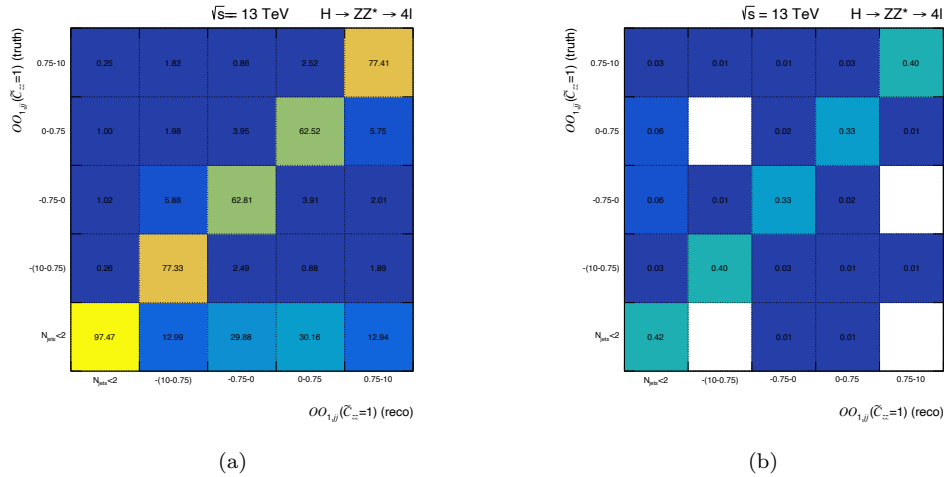
Figure 6.21: Migration matrix (a) and response matrix (b) evaluated using signal MC (mc16a+mc16d+mc16e) at m_H = 125 GeV for mass window of 105 < m_{4\ell} < 160 GeV (summing over all production modes) for the Optimal Observable \mathcal{OO}_{1,jj}(\tilde{c}_{zz} = 1) . Only reconstructed events that have been matched to truth events are included.
