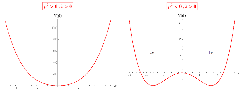
Figure 1.2: The Higgs potential V(\Phi) as a function of the complex scalar field \Phi for \mu^2 > 0 (on the left) and \mu^2 < 0 (on the right).
