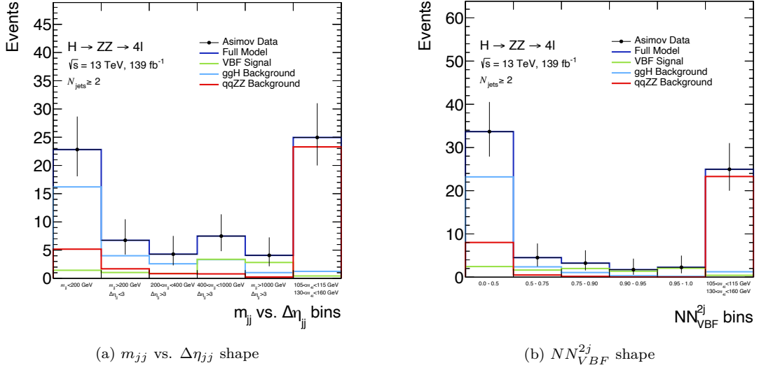
Figure 6.44: Shape for the bin N_{jets} \geq 2 of the a m_{jj} vs. \Delta\eta_{jj} and b NN_{VBF}^{2j} template distributions in the range 115 < m_{4\ell} < 130 \text{ GeV} . The last bin of the template represents the sideband-bin with all the events in 105 < m_{4\ell} < 115 \text{ GeV} and 130 < m_{4\ell} < 160 \text{ GeV} .
