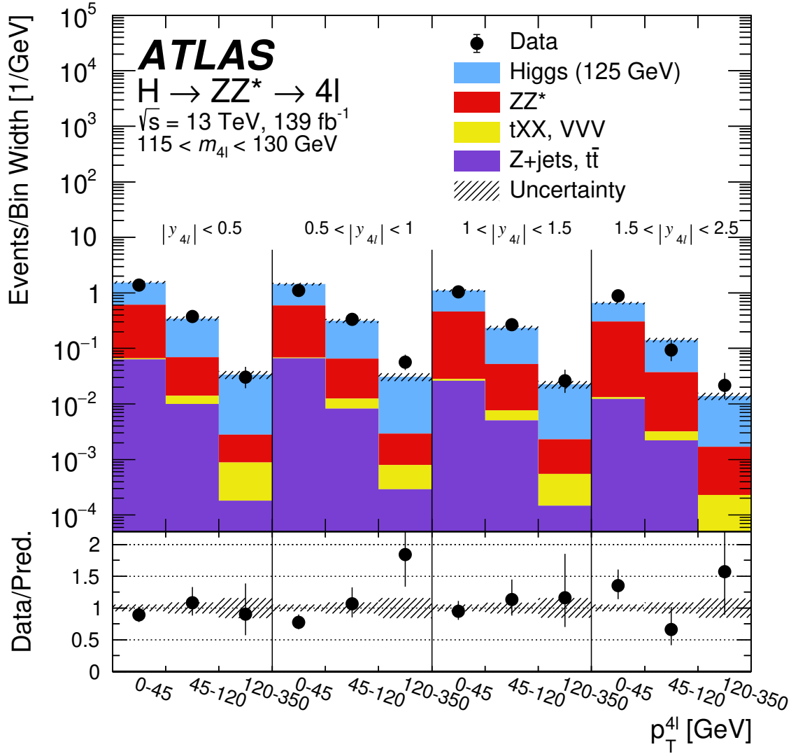
Figure A.10: The observed and expected (pre-fit) distributions of p_T^{4\ell} in |y_{4\ell}| bins in the mass region 115 < m_{4\ell} < 130 \text{ GeV} , for an integrated luminosity of 139 \text{ fb}^{-1} collected at \sqrt{s} = 13 \text{ TeV} . A SM Higgs boson signal with a mass m_H = 125 \text{ GeV} is assumed. The uncertainty in the prediction is shown by the hatched band, which includes the theoretical uncertainties of the SM cross section for the signal and the ZZ^* background.
