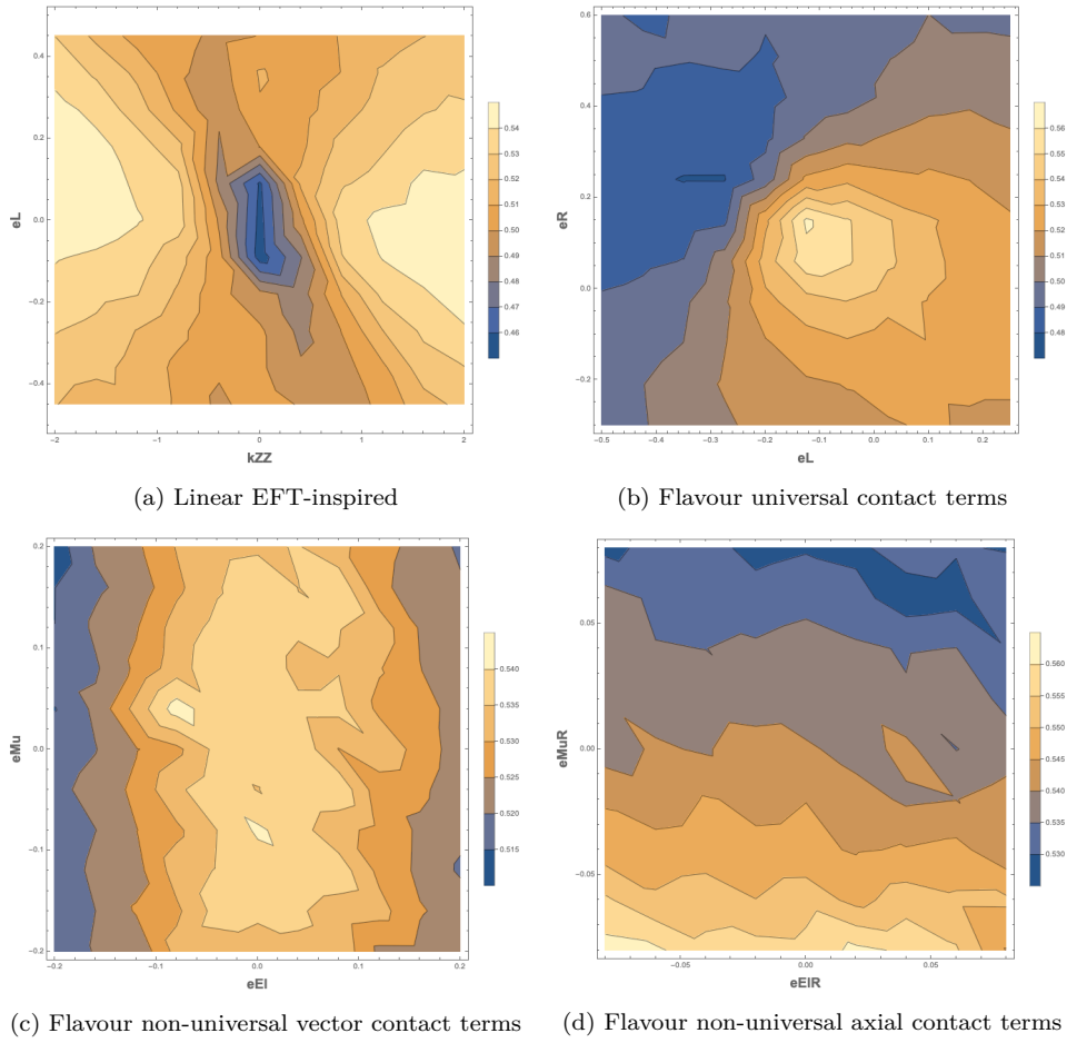
Figure 7.4: Acceptance variation in the inclusive fiducial phase space as a function of the POs for linear-EFT inspired and flavour universal contact terms scenarios in inclusive final state and flavour non-universal with vector and axial contact terms scenarios in the \ell\ell e and \ell\ell\mu\mu final states.
