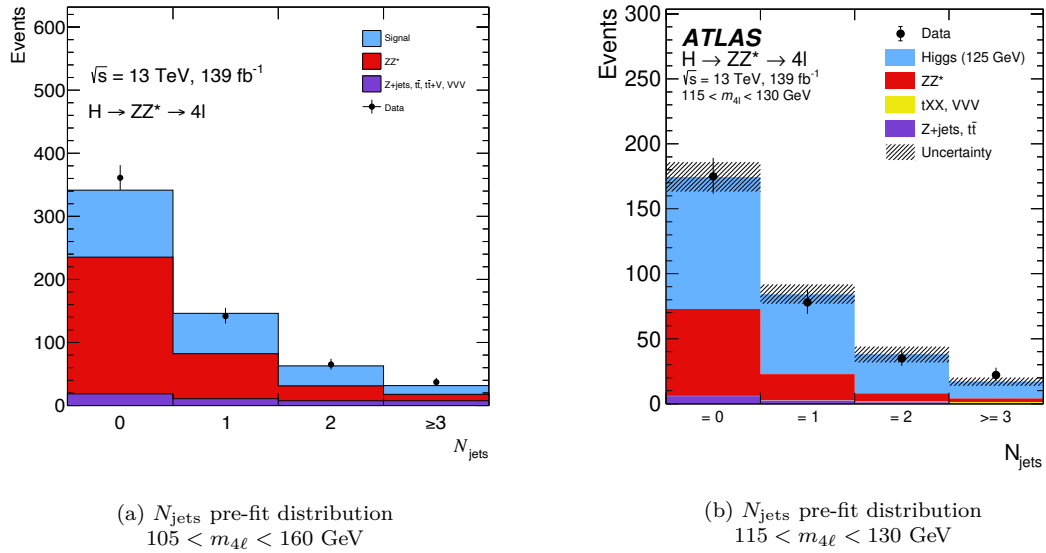
Figure 6.30: The observed and expected (pre-fit) distributions of N_{\text{jets}} in the range of (a) 105 < m_{4\ell} < 160 GeV and (b) 115 < m_{4\ell} < 130 GeV. The black dots depict pre-fit data while the blue, red and violet (and yellow) areas represent the signal, the ZZ^* background and the reducible background, respectively. In (b) the uncertainty in the prediction is shown by the hatched band, which include the theoretical uncertainties of the SM cross section for the signal and ZZ^* background.
