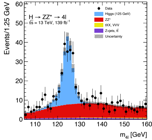
Figure 6.26: 105 < m_{4\ell} < 160 GeV
