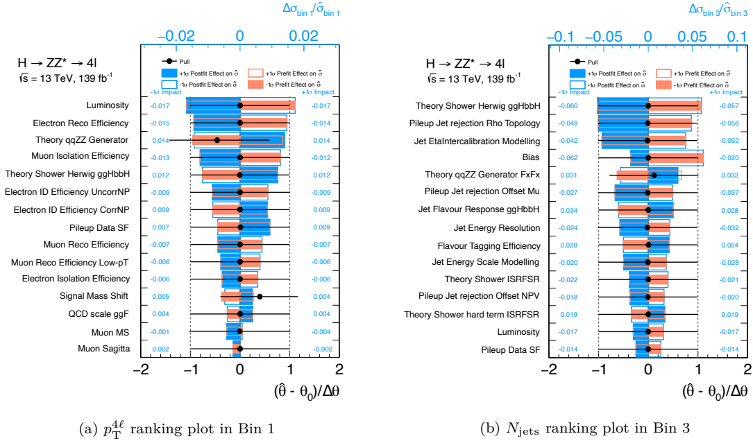
Figure 6.25: Ranking plots for (a) p_T^{4\ell} and (b) N_{\text{jets}} distribution for response matrix unfolding. Only the first 15 most highly ranked parameters are shown. The pink rectangles correspond to the pre-fit impact on the cross section \hat{\sigma} instead the blue rectangles to the post-fit impact, in case that the NP is fixed to +1\sigma (empty rectangles) or -1\sigma (filled rectangles) away from the nominal values \theta_0 . The impact of each nuisance parameter \Delta\sigma on the cross section is computed by comparing the nominal best-fit value \sigma with the result of the fit when fixing the considered nuisance parameter to its best fit value \hat{\theta} , shifted by its pre-fit (post-fit) uncertainties \pm\Delta\theta(\pm\Delta\hat{\theta}) . The impact on the cross section with fixed NP to \pm 1\sigma , \Delta\sigma/\hat{\sigma} refers to the scale on the top axis, and the \pm 1\sigma impact of each NP is written on the side of rectangles. The black points show the pulls of the nuisance parameters relative to their nominal values, \theta_0 . These pulls and their relative post-fit errors (\hat{\theta} - \theta_0)/\Delta\theta , refer to the scale on the bottom axis.
