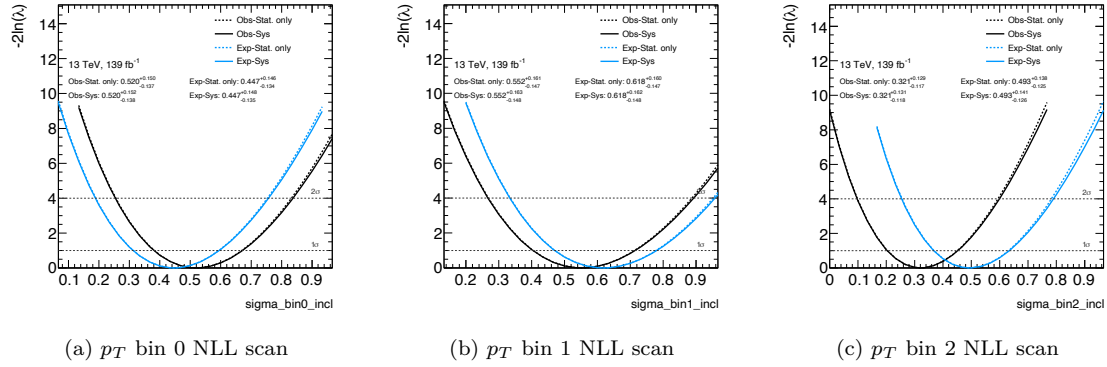
Figure 6.34: Negative log likelihood scans of the cross sections in the first three bin of the p_T^{4\ell} distribution for response matrix unfolding using data (in black) and the Asimov dataset (in blue) with luminosity 139\text{ fb}^{-1} for 105 < m_{4\ell} < 160\text{ GeV} has been considered. Expected and observed cross sections are reported. Systematic uncertainties are included.
