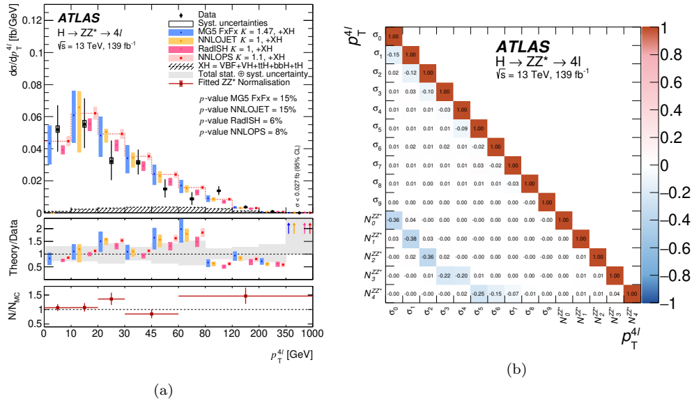
Figure 6.35: (a) Differential fiducial cross section for the transverse momentum p_T^{4\ell} of the Higgs boson, along with (b) the corresponding correlation matrix between the measured cross sections and the ZZ^* background normalisation factors.
