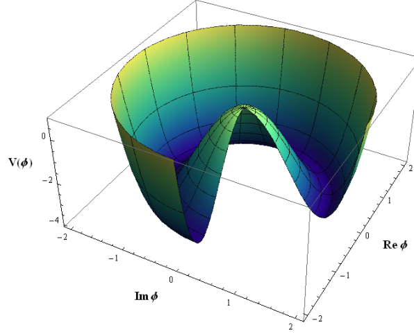
Figure 1.3: The Higgs potential shape known as the "mexican hat".
