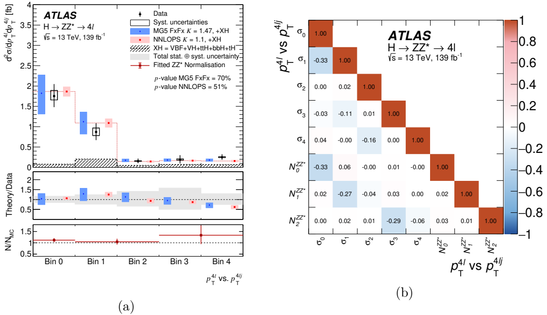
Figure A.29: a Differential fiducial cross section for the transverse momentum of the four-lepton system vs. the transverse momentum of the four-lepton plus jet system, p_T^{4l} vs. p_T^{4lj} and b the corresponding correlation matrix between the measured cross sections and the ZZ^* background normalisation factors. The bin boundaries are defined in Figure A.12.
