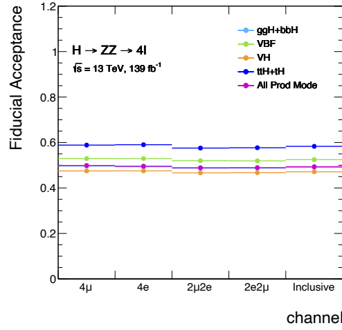
Figure 6.5: Comparison of the acceptance at m_H = 125 GeV using the dressed truth lepton definition in the mass range 105 < m_{4\ell} < 160 GeV for different production mode in the four final states.
