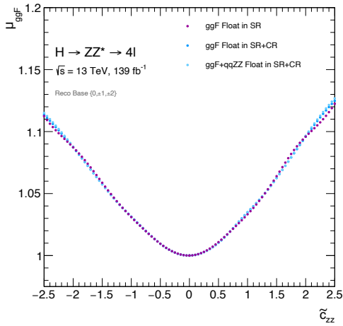
(b) \mu_{\text{ggF}} scan results
