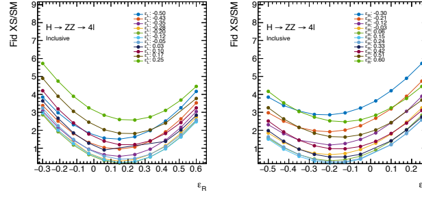
(b) Flavour universal contact terms
