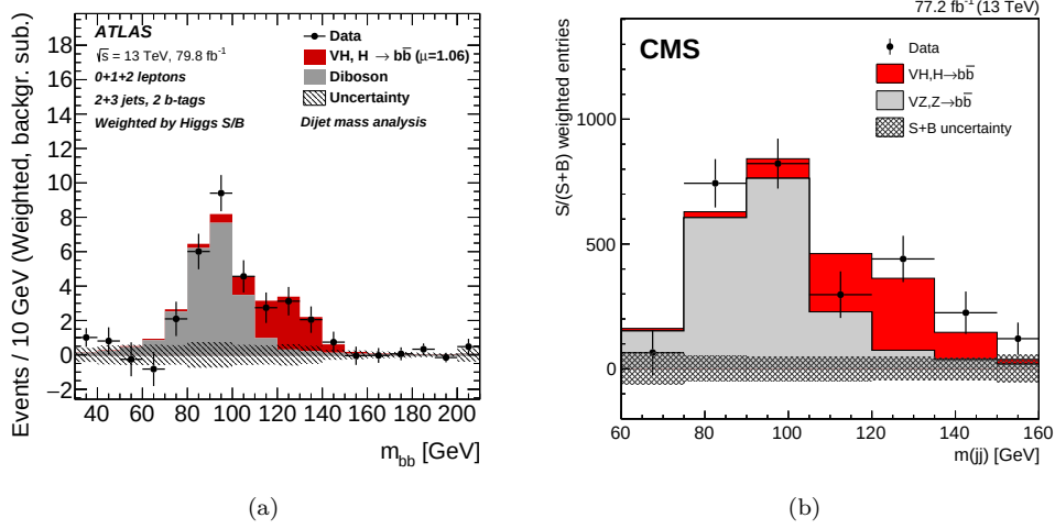
Figure 1.11: Distribution of the reconstructed di-jet invariant mass m_{bb} from (a) ATLAS [35] and (b) CMS experiment [36].
