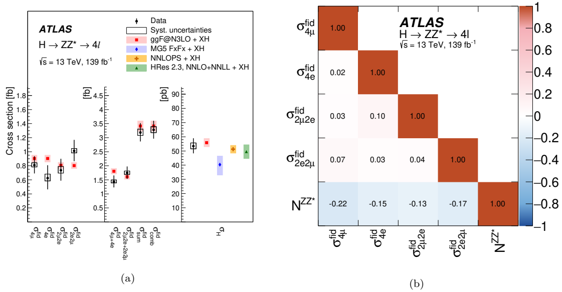
Figure 6.33: (a) The fiducial cross sections (left two panels) and total cross section (right panel) of Higgs boson production measured in the 4\ell final state. The fiducial cross sections are shown separately for each decay final state, and for same- and different-flavour decays. The inclusive fiducial cross section is measured as the sum of all final states, as well as by combining the per-final-state measurements assuming SM ZZ^{(*)} \rightarrow 4\ell relative branching ratios. The error bars on the data points show the total uncertainties, while the systematic uncertainties are indicated by the boxes. The shaded bands around the theoretical predictions indicate the PDF and scale uncertainties. (b) The correlation between the fiducial cross sections for the four individual decay final states and the ZZ^{(*)} normalisation factor.
