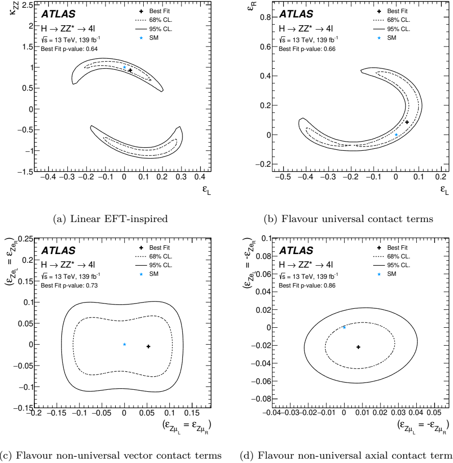
Figure 7.14: Observed exclusion plots for the four scenarios. The dashed line represents the 68% CL and the continuous line the 95% CL.
