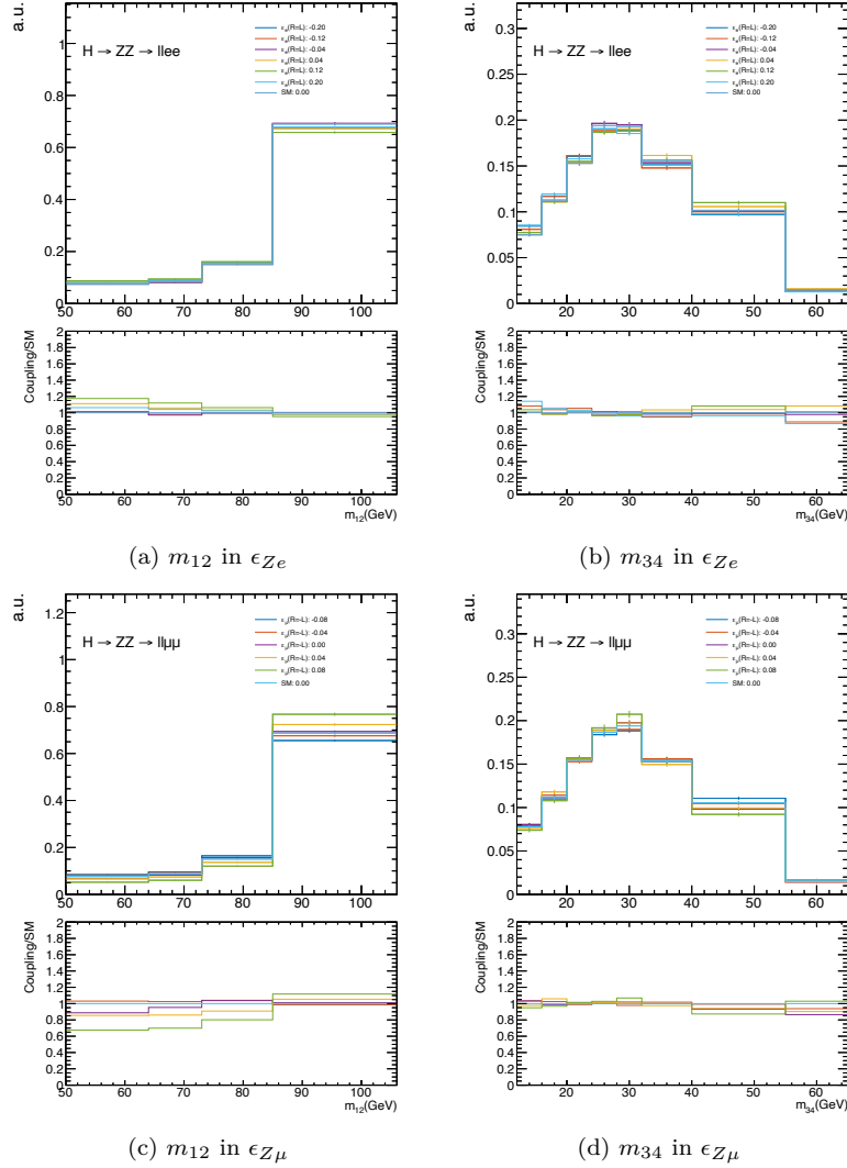
Figure 7.3: Modification of the m_{12} and m_{34} spectra for non-universal flavour couplings \epsilon_{Ze} (with \epsilon_{Ze(L)} = \epsilon_{Ze(R)} ) in \ell\ell ee final state and \epsilon_{Z\mu} (with \epsilon_{Ze(L)} = -\epsilon_{Ze(R)} ) in \ell\ell\mu\mu final state.
