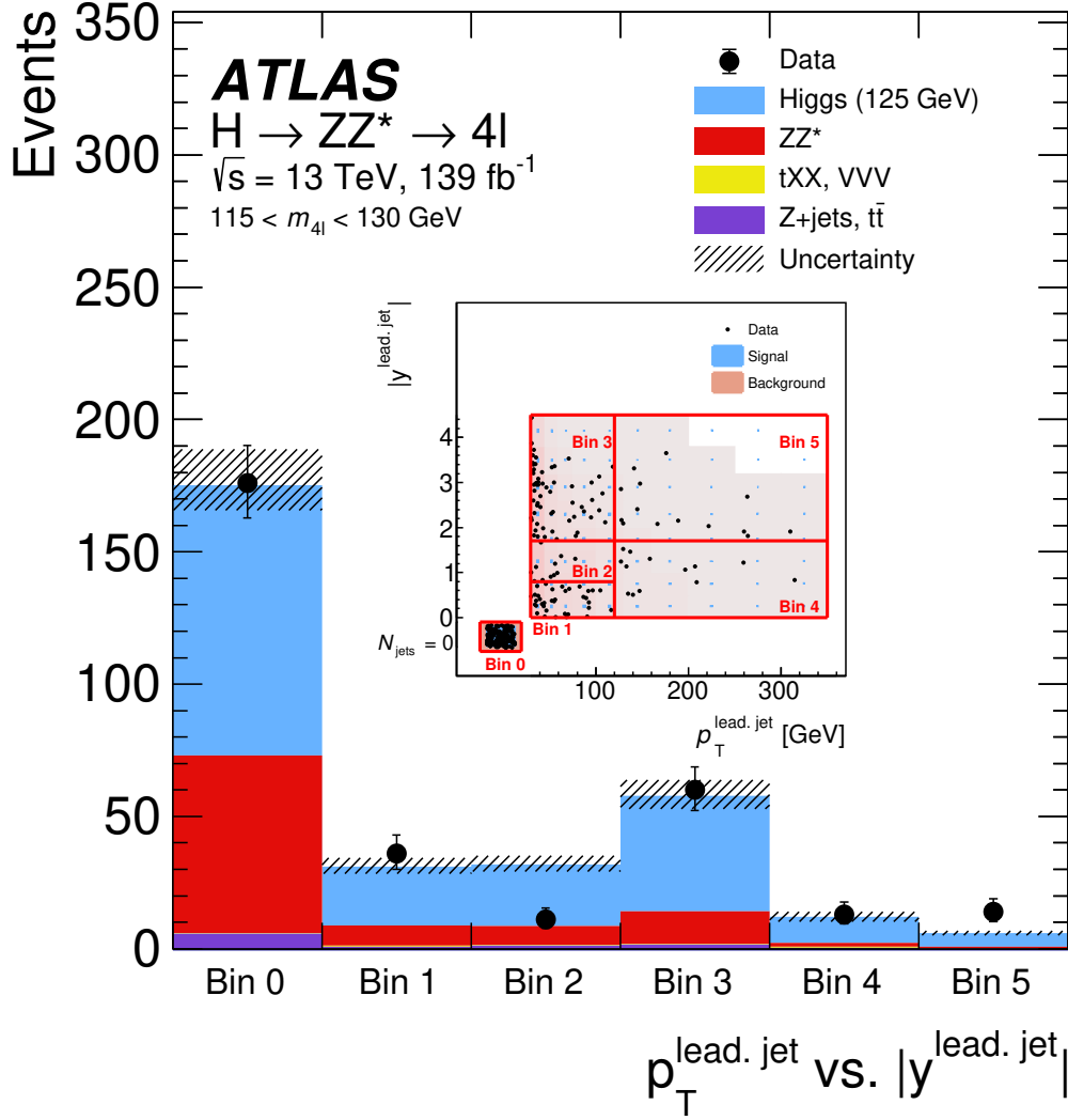
Figure A.15: The observed and expected (pre-fit) distribution in bins of the transverse momentum vs. the rapidity of the leading jet, p_T^{\text{lead. jet}} vs. |y^{\text{lead. jet}}| . The same distribution in the 2D plane is provided in the inset plot, where the black dots depict data and the blue and pink shaded areas represent simulated signal and background, respectively. The red lines depict the bin boundaries. These distributions correspond to the mass region 115 < m_{4\ell} < 130 GeV, for an integrated luminosity of 139 \text{ fb}^{-1} collected at \sqrt{s} = 13 TeV. A SM Higgs boson signal with a mass m_H = 125 GeV is assumed. The uncertainty in the prediction is shown by the hatched band, which includes the theoretical uncertainties of the SM cross section for the signal and the ZZ^* background.
