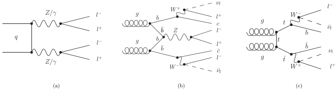
Figure 5.2: Feynman diagrams for the dominant background processes in the H \rightarrow ZZ^* \rightarrow 4l decay channel: (a) (Z^{(*)}/\gamma^*) (Z^{(*)}/\gamma^*) continuum production, (b) Z + \text{jets} production and (c) t\bar{t} production.
