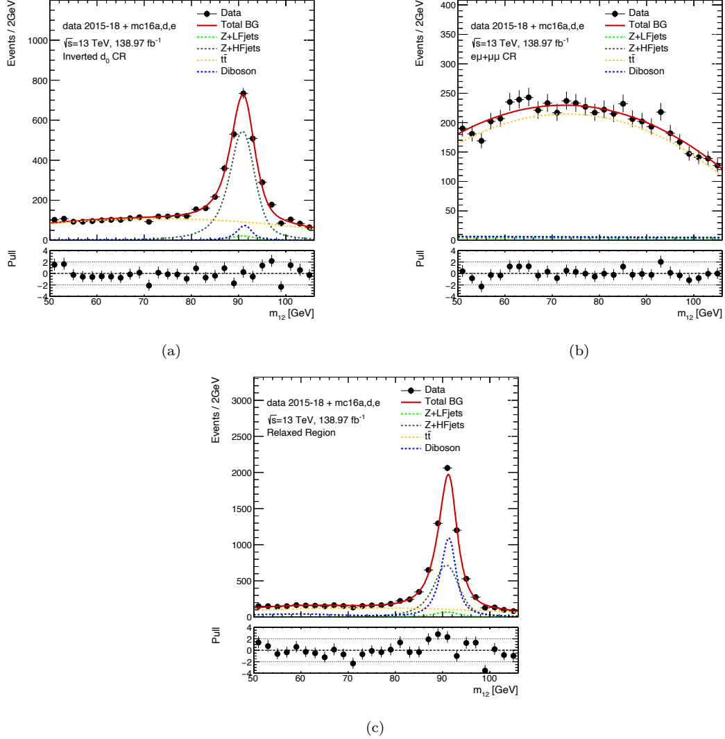
Figure 5.5: Distributions of m_{12} for the full Run2 data compared to the modelled background components in the (a) inverted- d_0 and (b) e\mu+\mu\mu CRs and in the (c) Relaxed region. The lower panels show the fit pulls.
