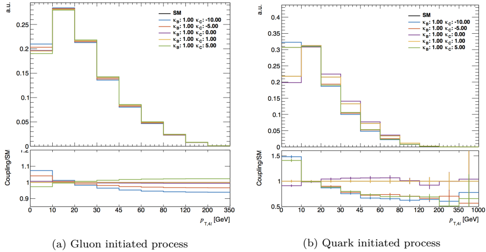
Figure 7.22: Modification to the p_T^H shape from gluon- (left) and quark- (right) initiated processes.
