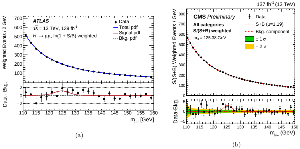
Figure 1.13: Dimuon invariant mass spectra from (a) ATLAS [37] and (b) CMS experiment [38].
