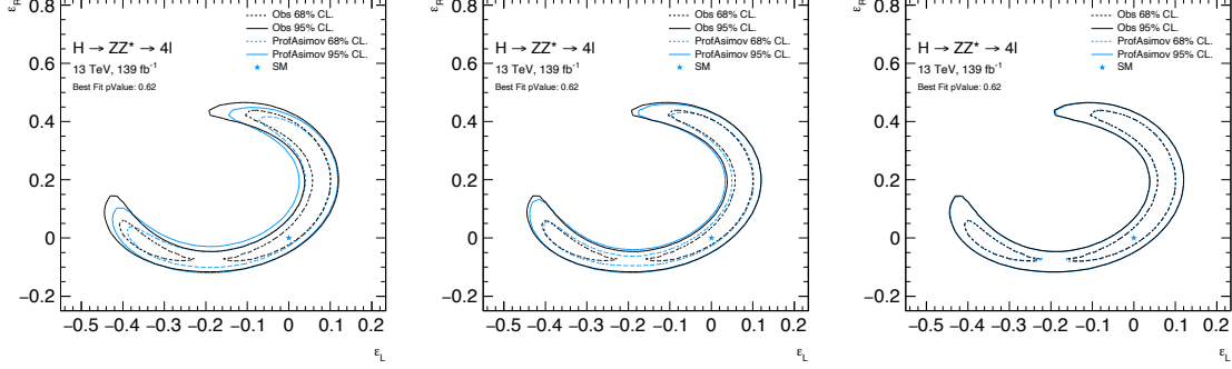
Figure 7.15: Observed exclusion limits (black lines) compared with ones obtained from the asimov dataset (blue lines) generated with \sigma_{bin1_{incl}} equal to 1 (on the left), 1.2 (in the center), 1.29 (on the right) times the expected value, and the others XS equal to the SM value, in the universal contact terms scenario.
