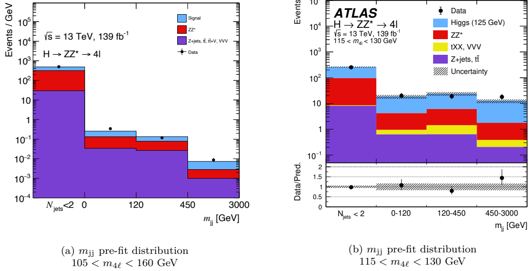
Figure 6.31: The observed and expected (pre-fit) distributions of m_{jj} in the range of (a) 105 < m_{4\ell} < 160 GeV and (b) 115 < m_{4\ell} < 130 GeV. The black dots depict pre-fit data while the blue, red and violet (and yellow) areas represent the signal, the ZZ^* background and the reducible background, respectively. In (b) the uncertainty in the prediction is shown by the hatched band, which include the theoretical uncertainties of the SM cross section for the signal and ZZ^* background.
