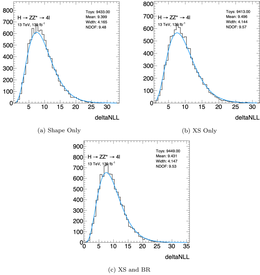
Figure 7.26: Distribution of the -2 \ln \lambda of the toys generated at SM point with a \chi^2 fit function to check the number of degrees of freedom.
