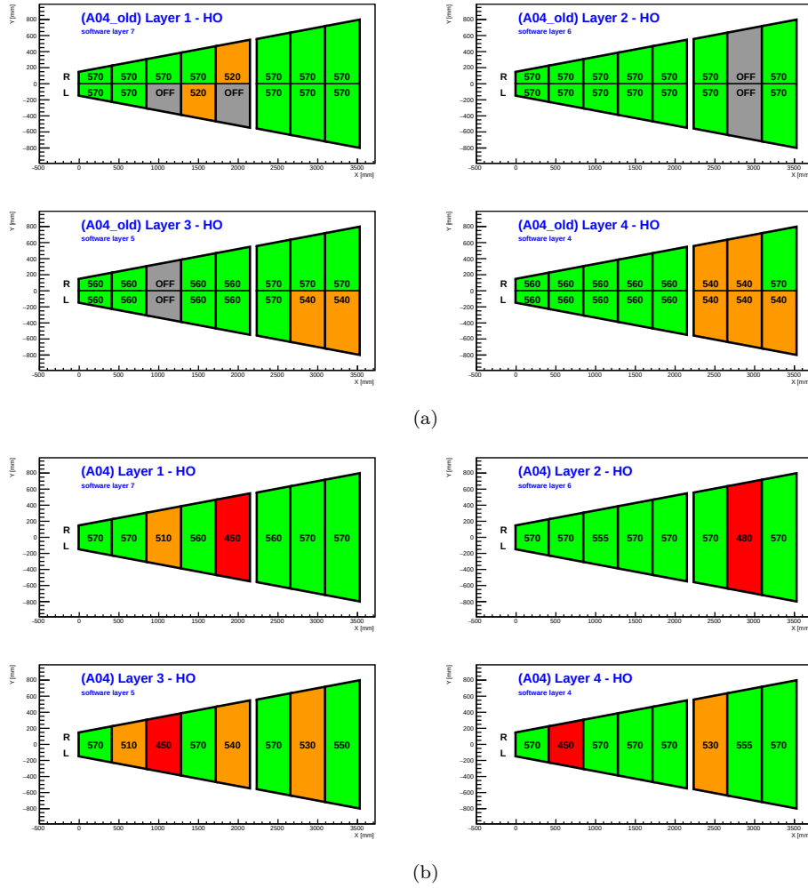
Figure 4.60: Comparison of the HV maps of the Double Wedge A04 HO side with the two different HV scheme: (a) old splitter box and (b) new half-granularity configuration
