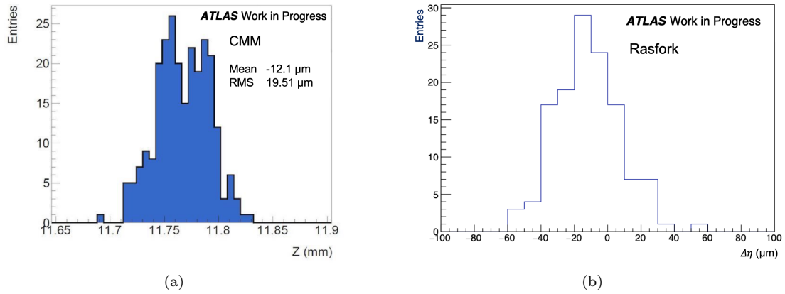
Figure 4.5: (a) Mean and RMS value of a stereo panel planarity measurements and (b) mis-alignment of the readout strips along the precise coordinate measured with the Rasfork .
