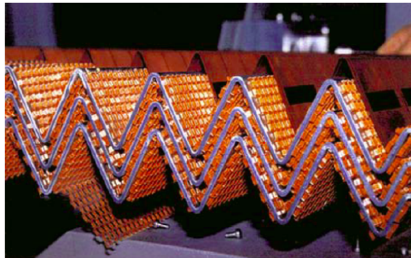
Figure 2.7: The accordion structure of Electromagnetic Barrel Calorimeter. Honeycomb spacers position the electrodes between the lead absorber plates.
