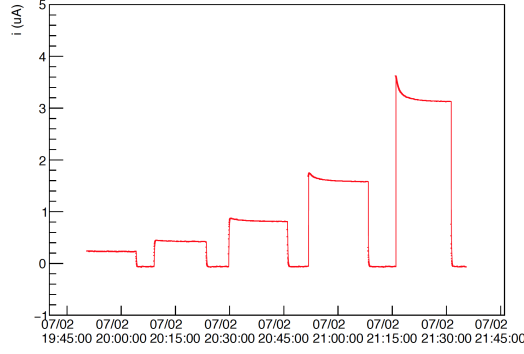
Figure 4.55: Attenuation scan performed at GIF++ of Micromegas modules. In Figure 4.55 the monitored current in time during the data taking is reported. The different steps show the increase of the mean current drawn by the HV section using different filters: 22, 10, 6.9, 4.6 and 1. This numbers represents the attenuation factor with respect to the photon flux emitted by the source at the peak of 662 keV.
