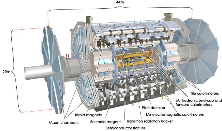
Figure 2.3: The cut-away view of the ATLAS detector. The various detector sub-systems are labelled. The dimensions of the detector are 25 m in height and 44 m in length. The overall weight of the detector is approximately 7000 tonnes [3] .
