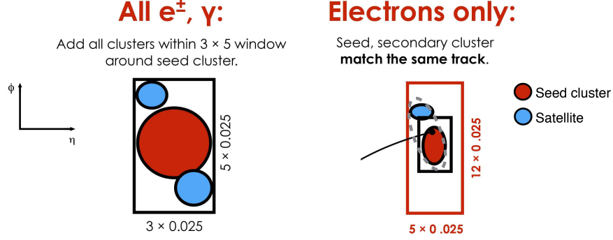
Figure 2.11: Diagram of superclustering algorithm for electrons. Seed clusters are shown in red, satellite clusters in blue.
