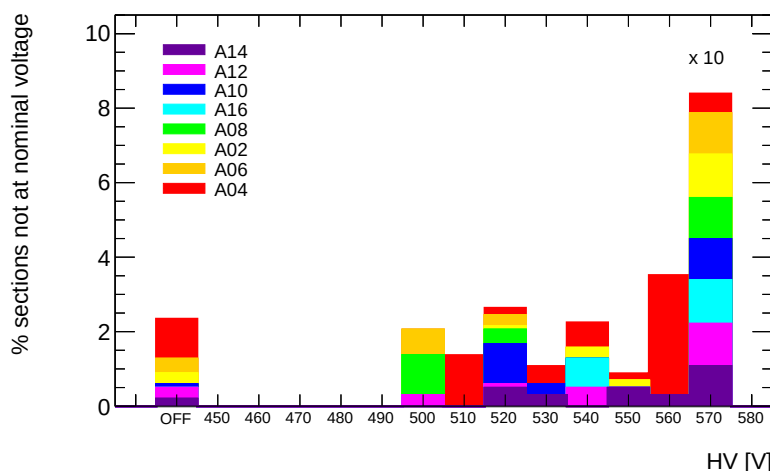
Figure 4.59: Summary of the HV values applied at each section of the Small Double Wedges following the splitter box scheme. The plot shows the percentage of the sections connected at a given HV value. The data at 570 V have to be scales \times 10 .
