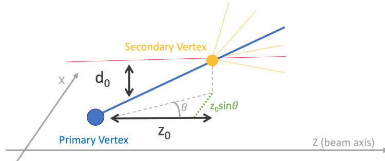
Figure 5.3: Sketch of the impact parameters definition.
