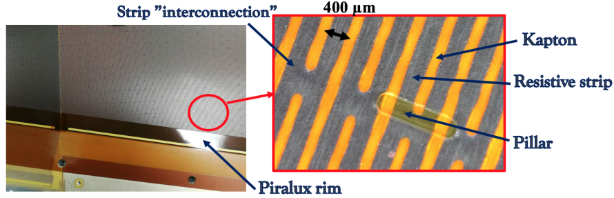
Figure 4.36: The resistive strips on PCBs shows a defined pattern with an array of interconnection between one strip and the next one at regular distance of 10 mm.
