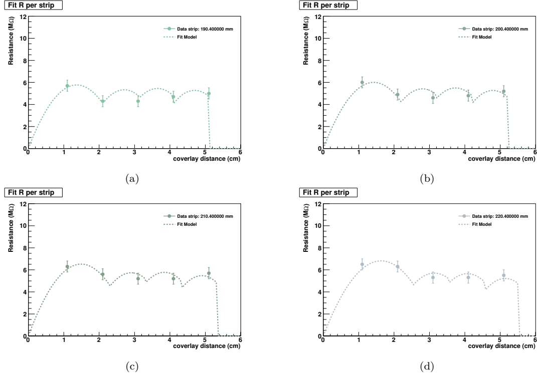
Figure 4.50: Fit on the measured data for four example strips.
