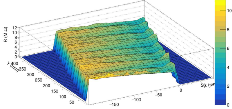
Figure 4.48: 2D resistance map of an SM1 Eta PCB.
