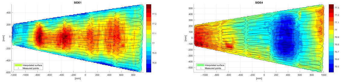
Figure 4.14: Point clouds obtained with the Laser Tracker and the interpolated surfaces of the two sides of the module for the planarity and thickness measurements.
