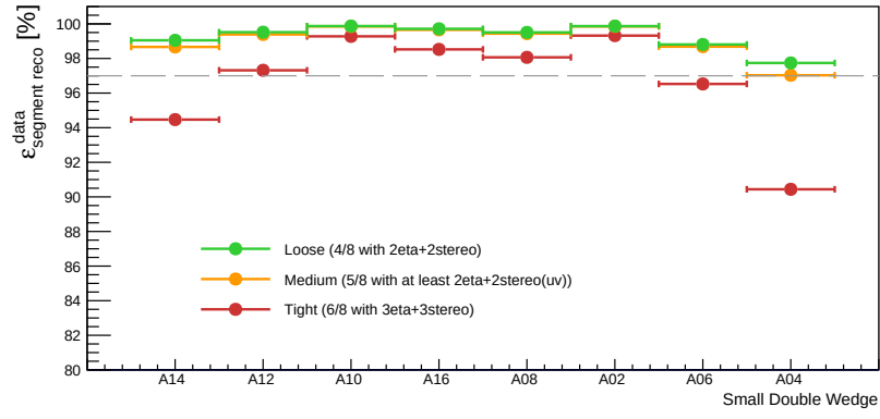
Figure 4.66: Segment reconstruction efficiency of the Small Double Wedges computed from the experimental efficiency measured from the cosmic data. The green, orange and red points represent the three working points Loose , Medium and Tight respectively. The grey line represent the 97% efficiency level.
