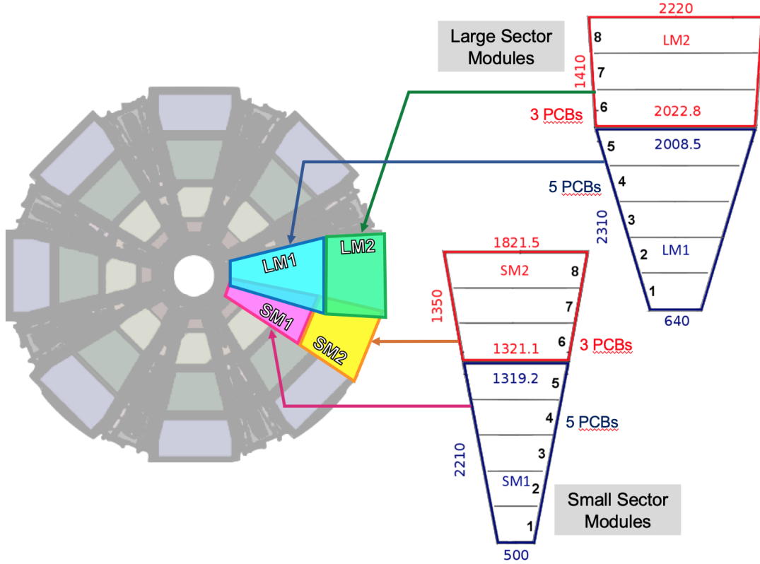
Figure 3.13: The New Small Wheel subdivision in small (S) and large (L) sectors and the division of the sectors' readout planes into 8 anode PCBs grouped in two modules (5 PCBs + 3 PCBs)
