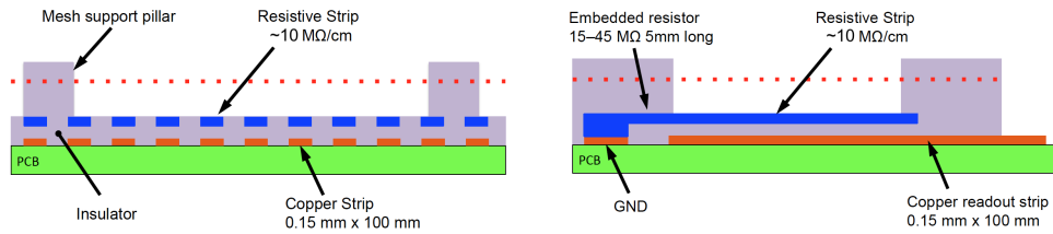
Figure 3.11: Spark protection principle.
