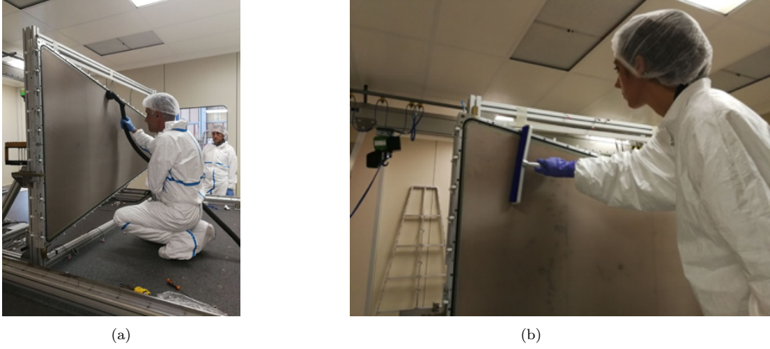
Figure 4.9: Dry cleaning procedure performed on the panel surfaces (a) with vacuum cleaner and (b) with electrostatic roller.
