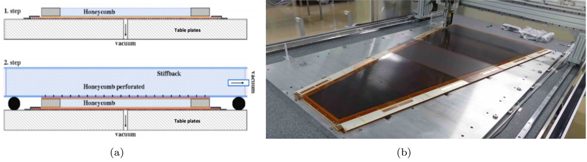
Figure 4.4: (a) The stiff-back technique scheme and (b) the final readout panel.
