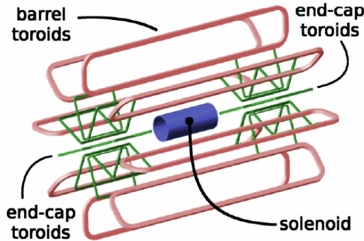
Figure 2.4: The ATLAS magnetic system.
