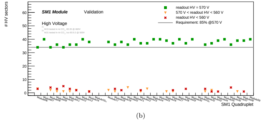
Figure 4.30: Summary HV results.
