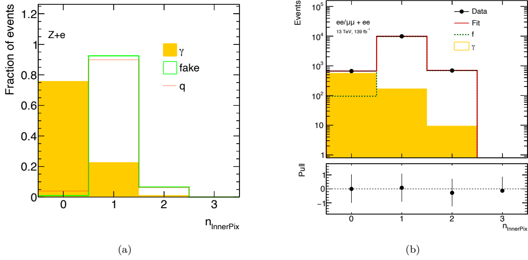
Figure 5.6: In (a) templates used in the 3\ell + X fit to n_{\text{InnerPix}} for the different sources of background ( \gamma , f ), extracted from MC simulation in the Z + X control sample. The q component (real electrons from heavy-flavour decays) is extracted from 3\ell + X events in simulation. All distributions are normalised to unit area. In (b) data 3\ell + X events and result of the fit to n_{\text{InnerPix}} , combining 2\mu 2e and 4e channels for the full Run-2 dataset: the lower panel shows the fit pulls. The fit components modeling f and \gamma contributions are also shown.
