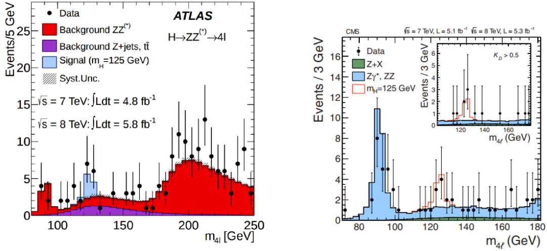
Figure 1.4: The distribution of the four-lepton invariant mass m_{4l} . The signal and the background expectation are shown and compared with the combination of the 7 TeV and 8 TeV data. On the left: ATLAS Collaboration [1]. On the right: CMS Collaboration [2].
