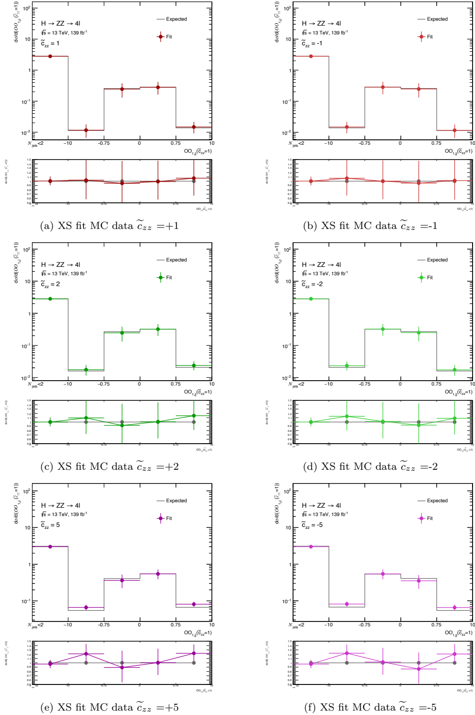
Figure 6.10: Differential cross section results of \mathcal{OO}_{1,jj}(\tilde{c}_{zz} = 1) obtained using unfolding BSM simulated data with SM response matrix compared with the BSM expected cross section in each bin for different coupling values: (a) \tilde{c}_{zz} = +1 , (b) \tilde{c}_{zz} = -1 , (c) \tilde{c}_{zz} = +2 , (d) \tilde{c}_{zz} = -2 , (e) \tilde{c}_{zz} = +5 , (f) \tilde{c}_{zz} = -5 . In the bottom panel the ratio between the fit and the expected cross sections is reported.
