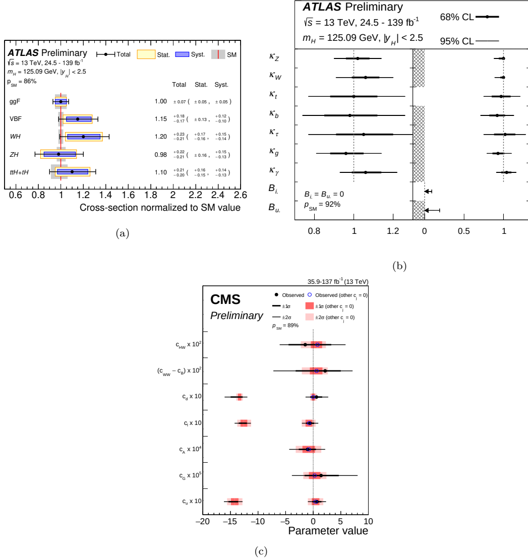
Figure 1.19: (a) Measured cross sections for ggF , VBF , WH , ZH and ttH + tH normalised to their SM predictions, measured assuming SM values for the decay branching fractions [56]. (b) Best-fit values and uncertainties for Higgs boson coupling modifiers per particle type with effective photon and gluon couplings and either B_i = B_u = 0 (left), or include them as free parameters (right) [56]. (c) Summary plot for the effective couplings scans. The best fit values when profiling (fixing) the other parameters are shown by the solid black (hollow blue) points. The \pm 1\sigma and \pm 2\sigma confidence intervals are represented by the thick and thin black lines respectively for the profiled scenario, and the green and yellow bands respectively for the fixed scenario [57].
