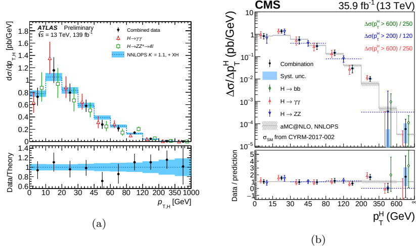
Figure 1.18: Combined differential cross section as function of p_{T,H} from measurement performed in H \rightarrow \gamma\gamma and H \rightarrow ZZ^* \rightarrow 4l by (a) ATLAS [51] and (b) CMS [53].
