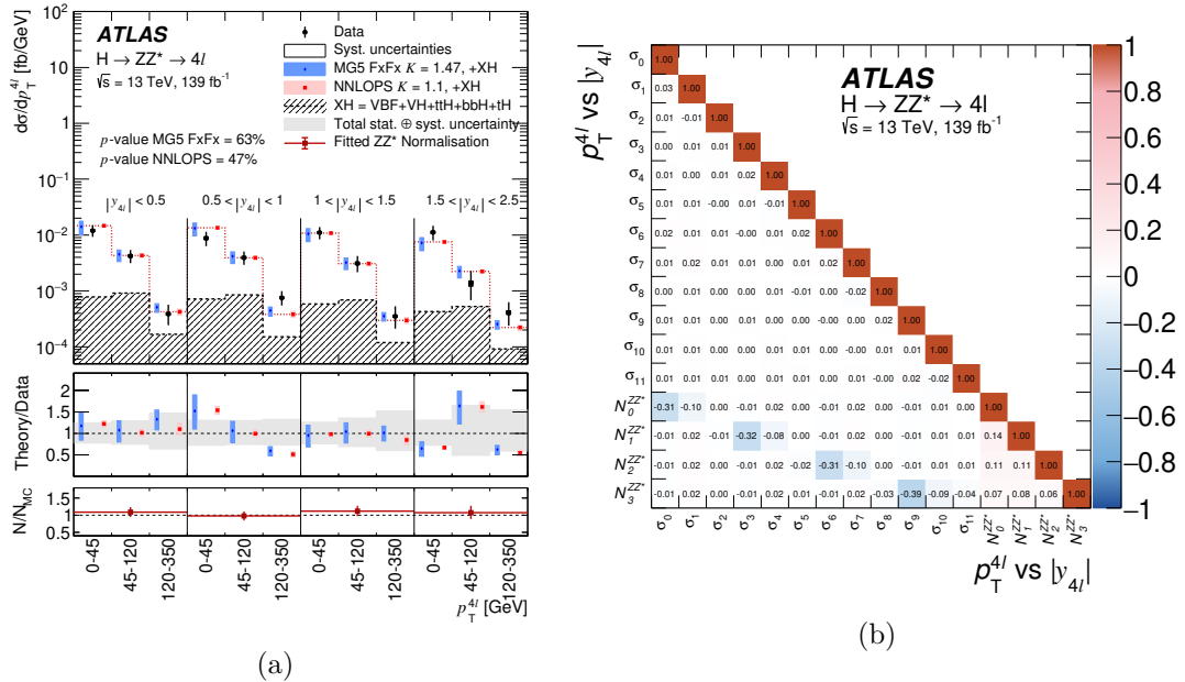
Figure A.27: a Double differential fiducial cross sections of the p_T^{4\ell} distribution in |y_{4\ell}| bins. The corresponding correlation matrix between the measured cross sections and the ZZ^* background normalisation factors is shown in b . The p -values shown are calculated for all bins across both p_T^{4\ell} and |y_{4\ell}| simultaneously.
