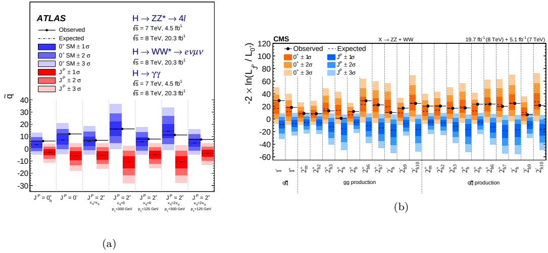
Figure 1.15: Distribution of the test statistics of the SM hypothesis J^P = 0^+ against the alternative spin-parity hypothesis J^P = 0^-, 1^+, 1^-, 2^+ for (a) ATLAS [42] and (b) CMS [43]. The spin-1 hypothesis is in principle excluded due to the observation of the H \rightarrow \gamma\gamma decays and the Landau-Yang theorem, which forbids the decay of a spin-1 particle into two massless vector bosons. Then this hypothesis is not shown in the ATLAS results which includes also the H \rightarrow \gamma\gamma channel in the combination.
