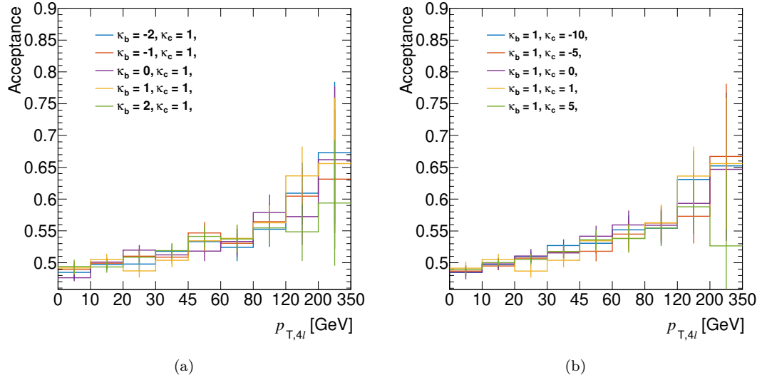
Figure 7.24: Modification of the acceptance in p_T^H bin for different (a) \kappa_b (with \kappa_c = 1 ) and (b) \kappa_c (with \kappa_b = 1 ) values.
