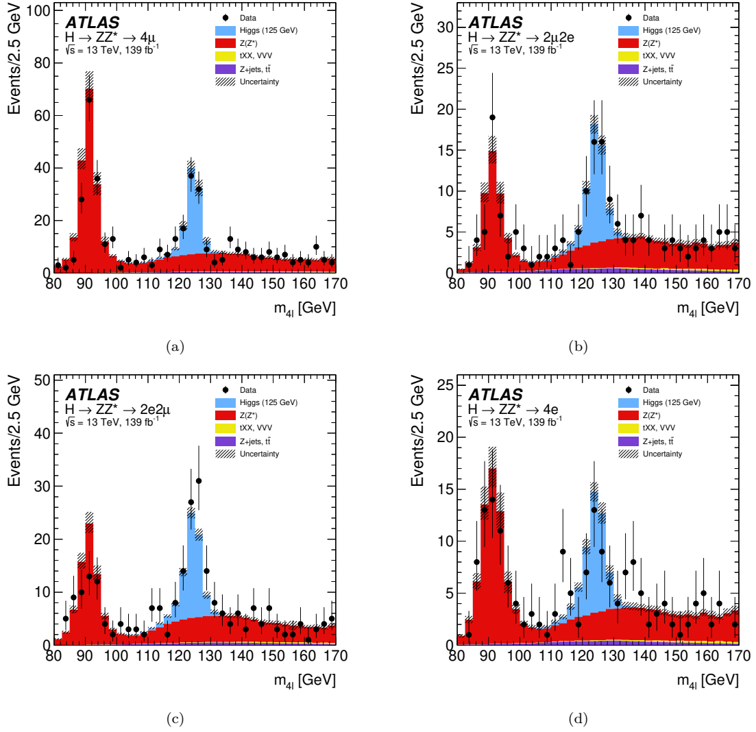
Figure 5.8: FSR-corrected m_{4\ell} distribution of the selected candidates for the different channels of the analysis, compared to the signal and background expectations in the region 80 – 170 GeV: (a) 4\mu , (b) 2\mu 2e , (c) 2e 2\mu , (d) 4e . The contribution of the reducible background is also shown separately.
