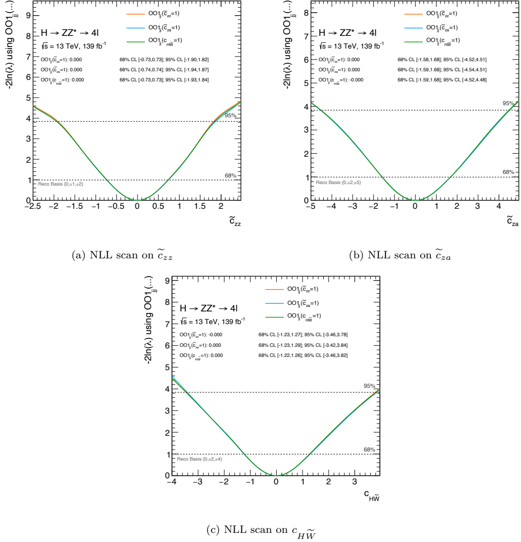
Figure 7.40: NLL scan along \tilde{c}_{zz} (a), \tilde{c}_{za} (b) and c_{H\tilde{W}} (c) fitting Optimal Observables \mathcal{OO}_{1,jj}(\tilde{c}_{zz} = 1) , \mathcal{OO}_{1,jj}(\tilde{c}_{za} = 1) and \mathcal{OO}_{1,jj}(c_{H\tilde{W}} = 1) .
