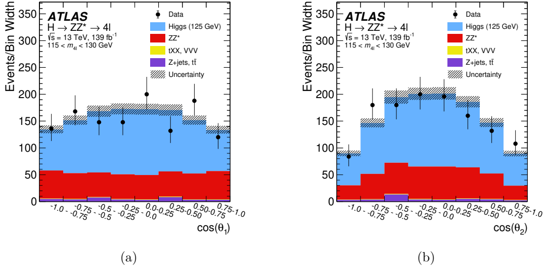
Figure A.3: The observed and expected (pre-fit) distributions of a \cos\theta_1 and b \cos\theta_2 in the mass region 115 < m_{4\ell} < 130 GeV, for an integrated luminosity of 139 \text{ fb}^{-1} collected at \sqrt{s} = 13 TeV. A SM Higgs boson signal with a mass m_H = 125 GeV is assumed. The uncertainty in the prediction is shown by the hatched band, which includes the theoretical uncertainties of the SM cross section for the signal and the ZZ^* background.
