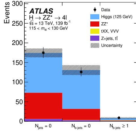
Figure A.5: The observed and expected (pre-fit) distributions of N_{b\text{-jets}} in the mass region 115 < m_{4\ell} < 130 GeV, for an integrated luminosity of 139 \text{ fb}^{-1} collected at \sqrt{s} = 13 TeV. A SM Higgs boson signal with a mass m_H = 125 GeV is assumed. The uncertainty in the prediction is shown by the hatched band, which includes the theoretical uncertainties of the SM cross section for the signal and the ZZ^* background.
