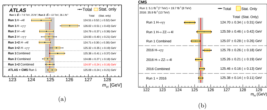
Figure 1.14: Summary of Higgs boson mass measurements from the individual analyses of (a) ATLAS and (b) CMS.
