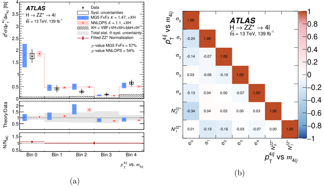
Figure A.28: a Double differential fiducial cross section for the transverse momentum of the four-lepton plus jet system vs. the invariant mass of the four-lepton plus jet system, p_T^{4lj} vs. m_{4lj} and b the corresponding correlation matrix between the measured cross sections and the ZZ^* background normalisation factors. The bin boundaries are defined in Figure A.11.
