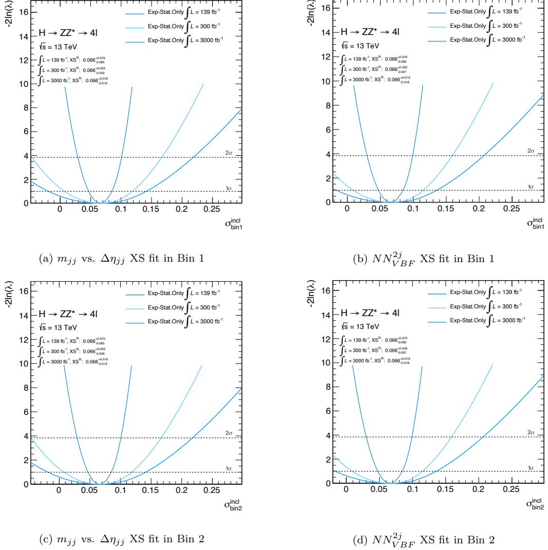
Figure 6.45: Expected results for the fiducial differential VBF cross section measurement in \mathcal{O}_{1,jj}(\tilde{c}_{zz} = 1) bins at 139 fb -1 , 300 fb -1 and 3000 fb -1 and for different template fit variable: m_{jj} vs. \Delta\eta_{jj} (a and c) and NN_{VBF}^{2j} (b and d). Only statistical uncertainties have been considered.
