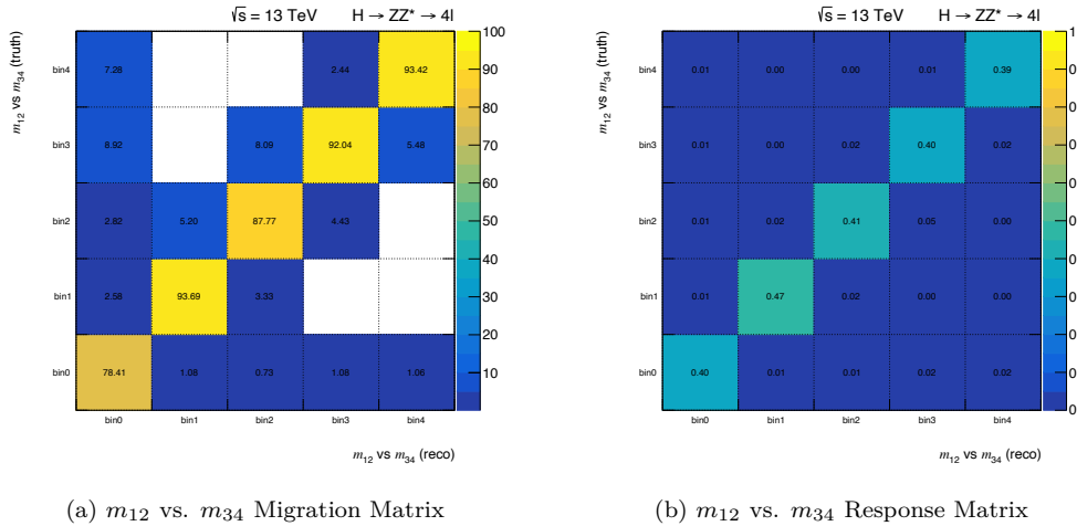
Figure 6.18: (a) Migration and (b) response matrix for m_{12} vs. m_{34} , evaluated using signal MC (mc16a+mc16d+mc16e) at m_H = 125 GeV for mass window of 105 < m_{4\ell} < 160 GeV (summing over all production modes). Only reconstructed events that have been matched to truth events are included.
