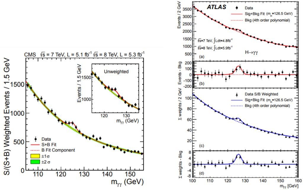
Figure 1.5: The diphoton invariant mass distribution. The result of a fit to the combined 7 TeV and 8 TeV data of the sum of a signal and a background component is superimposed. On the left : CMS Collaboration [2]. On the right : ATLAS Collaboration (the inclusive sample (a,b) and a weighted version (c,d) are shown) [1].
