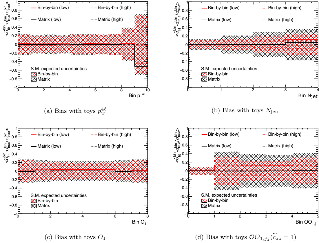
Figure 6.8: Mean cross section bias, as obtained from pseudo experiments tests on samples with different true cross section, as a function of the true cross section for each bin of the variable (a) p_T^{4\ell} , (b) N_{\text{jets}} , (c) \mathcal{O}_1 and (d) \mathcal{OO}_{1,jj}(\tilde{c}_{zz} = 1) . The black and red continuous (dotted) lines show cross section bias for the matrix and bin-by-bin unfolding methods when the truth cross-section is varied within the +1 ( -1 ) sigma expected statistical uncertainty, respectively. The shaded areas show the median statistical uncertainty as obtained from ensemble tests with the true cross section (SM) equal to that used to derive the correction factors and matrices.
