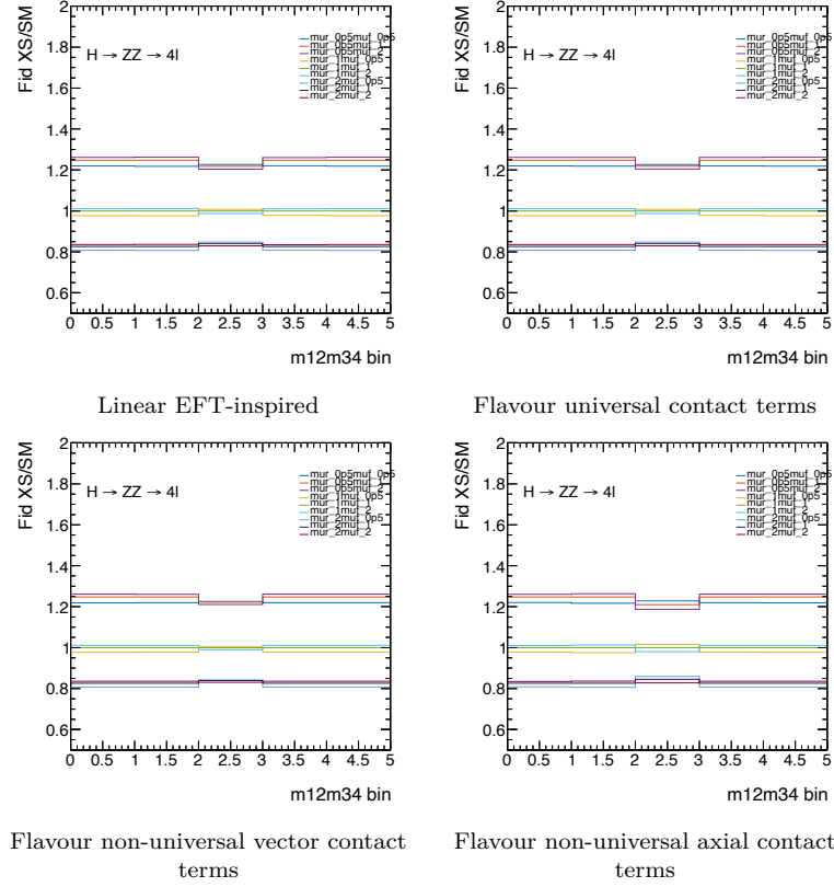
Figure 7.12: Systematic variations for all the interpretation scenarios.
