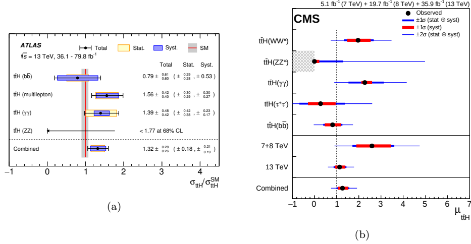
Figure 1.10: (a) combined t\bar{t}H production cross section, as well as cross sections measured in the individual analyses performed by ATLAS experiment [33]. (b) the best fit value of the t\bar{t}H signal strength modifier for each decay channel and the combined results performed by CMS experiment [34].
