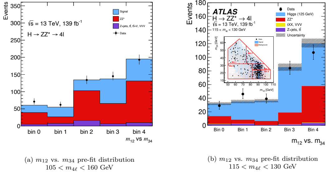
Figure 6.32: The observed and expected (pre-fit) distributions of m_{12} vs. m_{34} in the range of (a) 105 < m_{4\ell} < 160 GeV and (b) 115 < m_{4\ell} < 130 GeV. The black dots depict pre-fit data while the blue, red and violet (and yellow) areas represent the signal, the ZZ^* background and the reducible background, respectively. In (b) the uncertainty in the prediction is shown by the hatched band, which include the theoretical uncertainties of the SM cross section for the signal and ZZ^* background.
