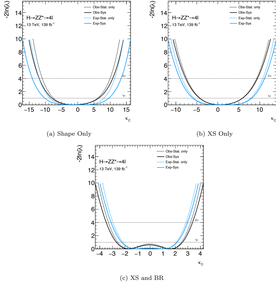
Figure 7.31: Expected and observed NLL scan for the Yukawa coupling \kappa_C .
