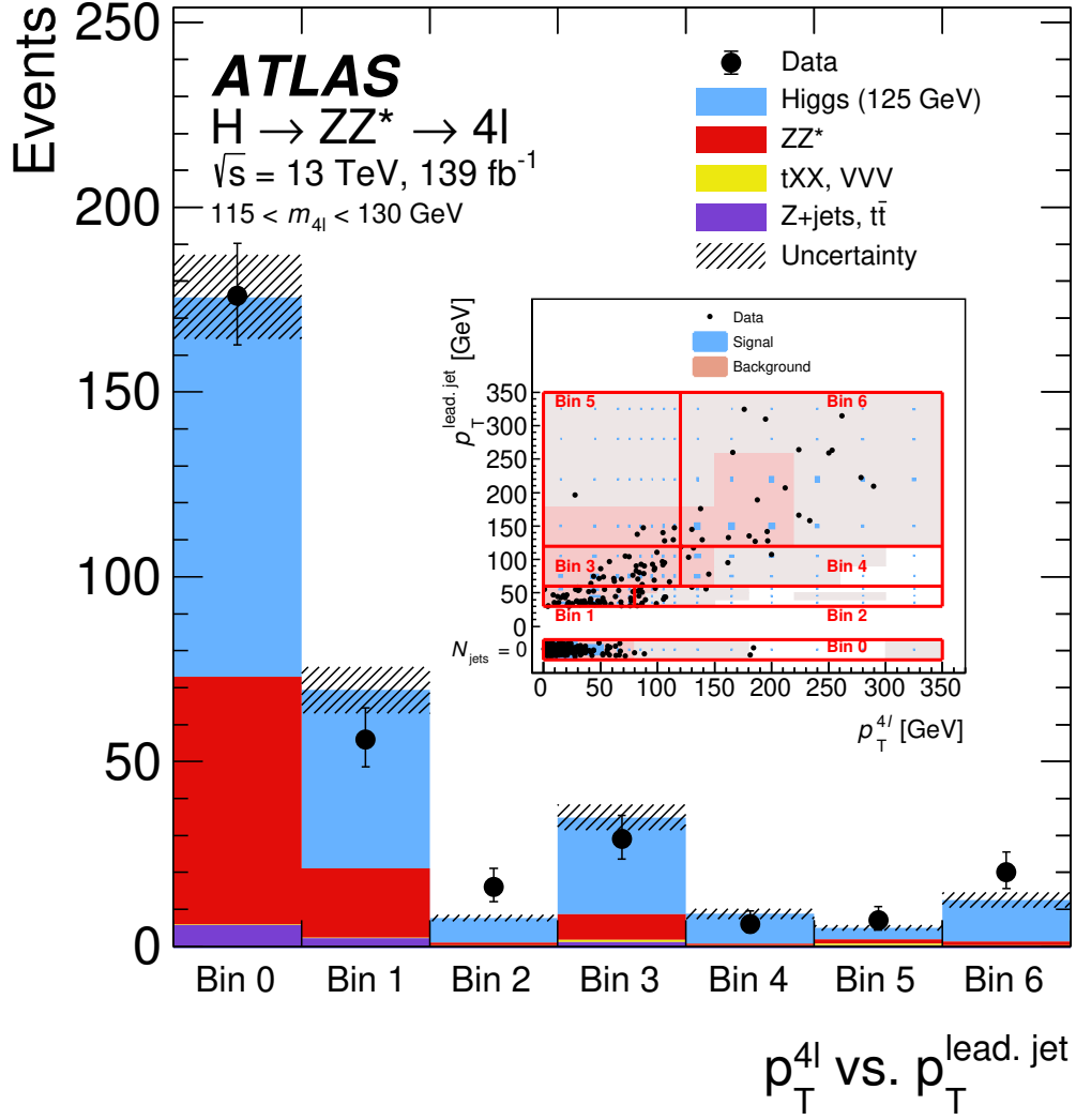
Figure A.13: The observed and expected (pre-fit) distribution in bins of the transverse momentum of the four-lepton system vs. the transverse momentum of the leading jet, p_T^{4l} vs. p_T^{\text{lead. jet}} . The same distribution in the 2D plane is provided in the inset plot, where the black dots depict data and the blue and pink shaded areas represent simulated signal and background, respectively. The red lines depict the bin boundaries. These distributions correspond to the mass region 115 < m_{4l} < 130 \text{ GeV} , for an integrated luminosity of 139 \text{ fb}^{-1} collected at \sqrt{s} = 13 \text{ TeV} . A SM Higgs boson signal with a mass m_H = 125 \text{ GeV} is assumed. The uncertainty in the prediction is shown by the hatched band, which includes the theoretical uncertainties of the SM cross section for the signal and the ZZ^* background.
