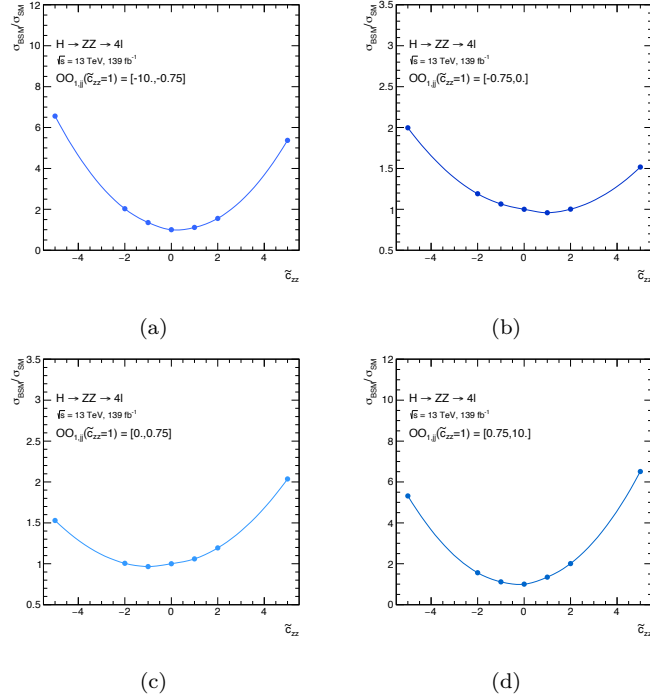
Figure 7.33: Modification of the predicted XS in different \mathcal{OO}_{1,jj}(\tilde{c}_{zz} = 1) bins as a function of \tilde{c}_{zz} .
