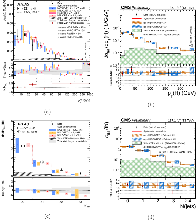
Figure 1.17: (a) - (d) Differential cross sections as function of p_{T,H} and N_{jets} in the H \rightarrow ZZ^* \rightarrow 4l decay channel measured by ATLAS [14] and CMS [54].
