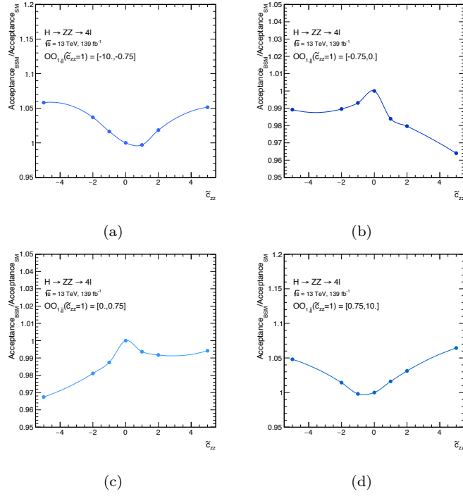
Figure 7.34: Modification of the acceptance in different \mathcal{O}\mathcal{O}_{1,jj}(\tilde{c}_{zz} = 1) bins as a function of \tilde{c}_{zz} .
