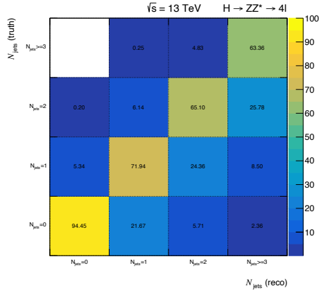
(a) N_{\text{jets}} Migration Matrix
