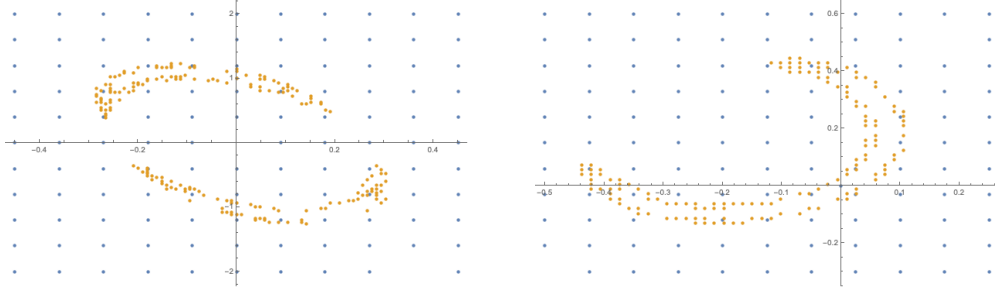
Figure 7.8: Generated point around the expected 68% and 95% limits for the Linear-EFT inspired and flavour universal contact term scenarios.
