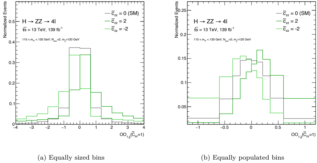
Figure 7.37: Optimal Observable \mathcal{OO}_{1,jj}(\tilde{c}_{zz} = 1) distribution for VBF + VH SM sample with different CP-odd coupling value \tilde{c}_{zz} = \pm 2 with equally sized populated bins (a) and with equally populated bins (b).
