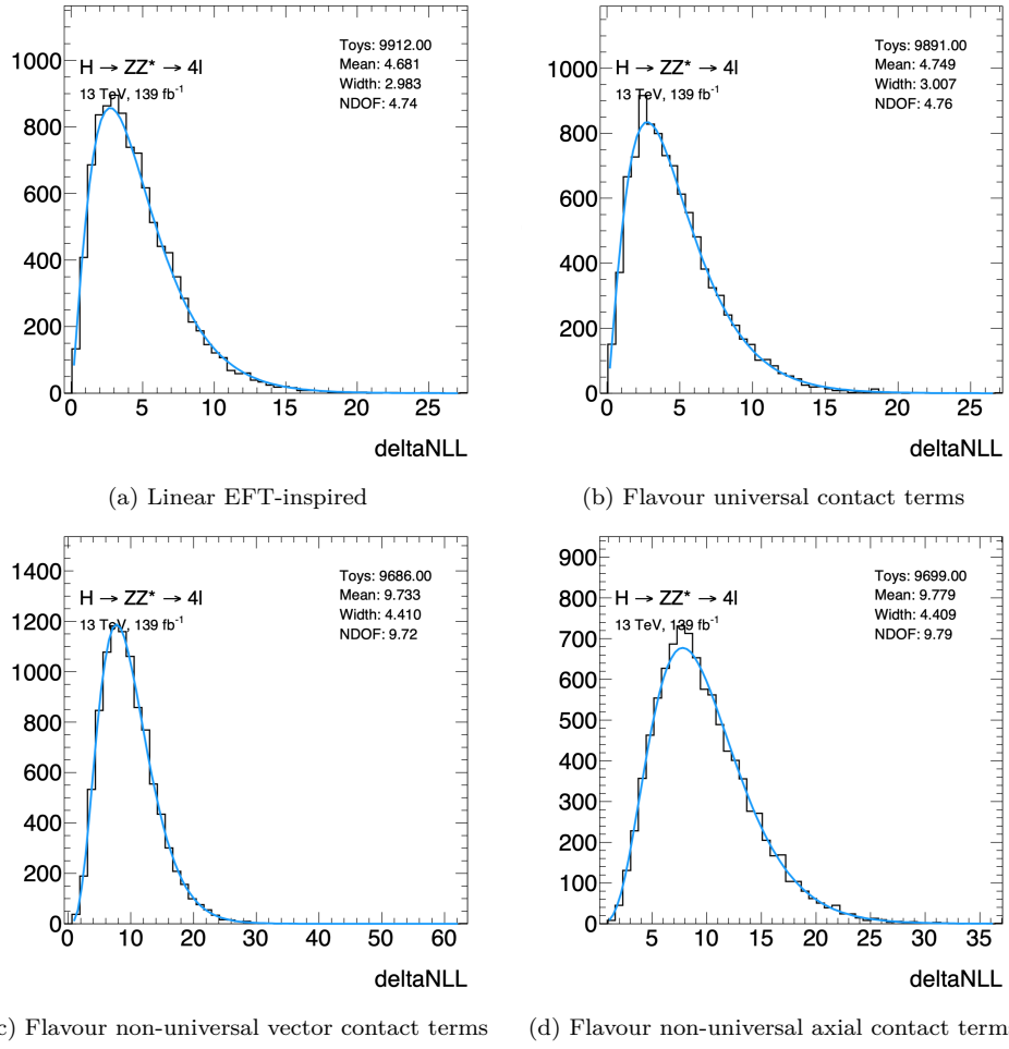
Figure 7.10: Distribution of the -2 \ln \lambda of the toys generated at SM point with a \chi^2 fit function to check the number of degrees of freedom.
