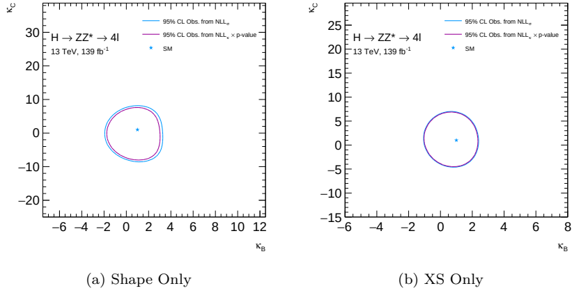
Figure 7.29: Comparison between the two 95% CL obtained with the "XS measurement" approach and with the "Yukawa model" taking into account the compatibility with the data using the p -value for the Shape Only and XS Only scenarios .
