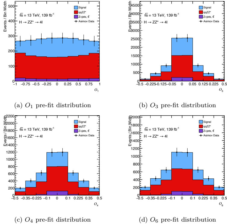
Figure B.1: The expected (pre-fit) distributions of (a) O_1 , (b) O_3 , (c) O_4 and (d) O_6 in the range of 105 < m_{4\ell} < 160 GeV. The black dots depict pre-fit asimov data while the blue, red and violet areas represent the signal, the ZZ^* background and the reducible background, respectively.
