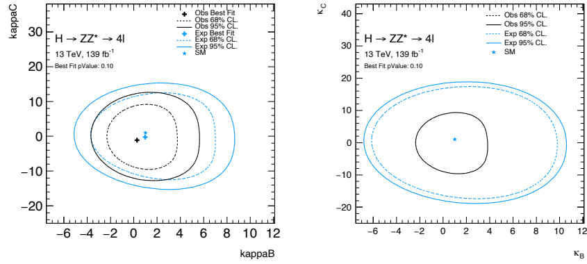
(a) Shape Only
