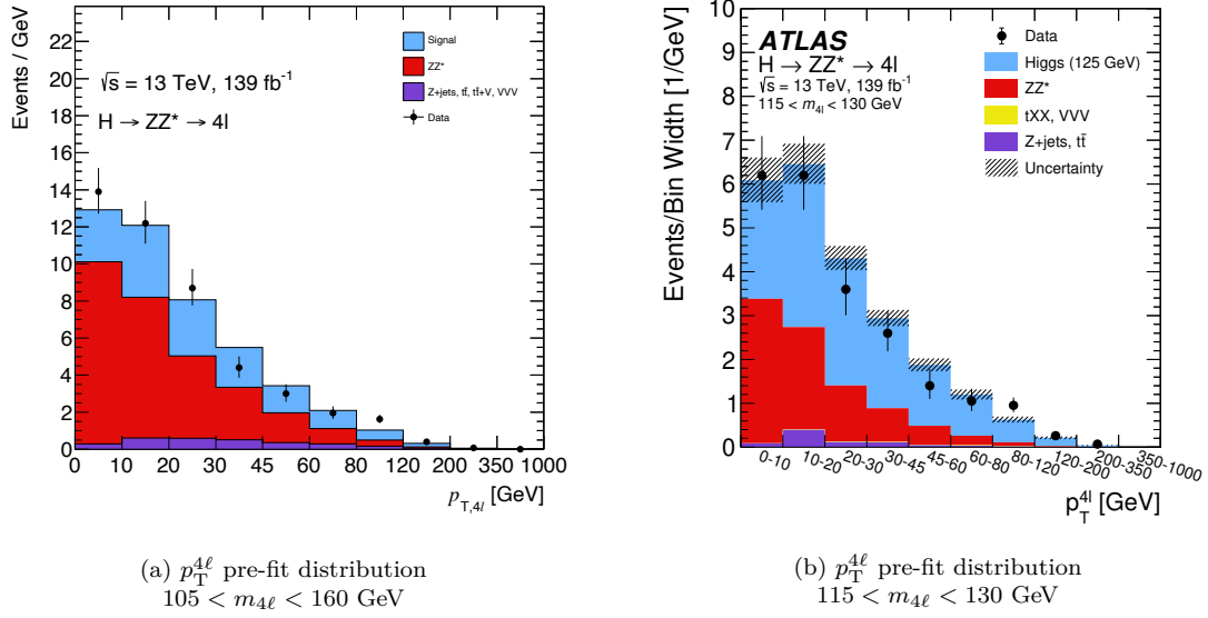
Figure 6.29: The observed and expected (pre-fit) distributions of p_T^{4\ell} in the range of (a) 105 < m_{4\ell} < 160 GeV and (b) 115 < m_{4\ell} < 130 GeV. The black dots depict pre-fit data while the blue, red and violet (and yellow) areas represent the signal, the ZZ^* background and the reducible background, respectively. In (b) the uncertainty in the prediction is shown by the hatched band, which include the theoretical uncertainties of the SM cross section for the signal and ZZ^* background.
