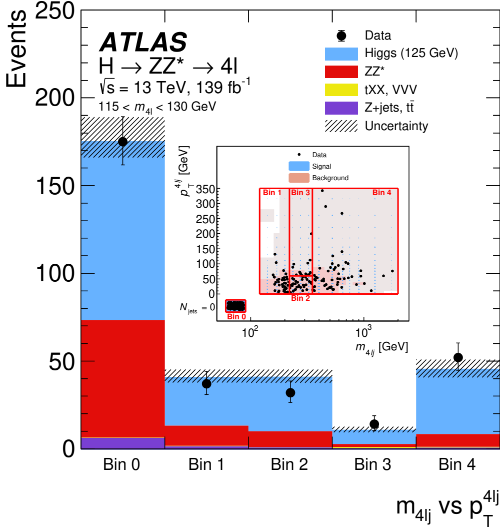
Figure A.11: The observed and expected (pre-fit) distribution in bins of the transverse momentum of the four-lepton plus leading-jet system vs. the invariant mass of the four-lepton plus leading-jet system, p_T^{4lj} vs. m_{4lj} . The same distribution in the 2D plane is provided in the inset plot, where the black dots depict data and the blue and pink shaded areas represent simulated signal and background, respectively. The red lines depict the bin boundaries. These distributions correspond to the mass region 115 < m_{4l} < 130 \text{ GeV} , for an integrated luminosity of 139 \text{ fb}^{-1} collected at \sqrt{s} = 13 \text{ TeV} . A SM Higgs boson signal with a mass m_H = 125 \text{ GeV} is assumed. The uncertainty in the prediction is shown by the hatched band, which includes the theoretical uncertainties of the SM cross section for the signal and the ZZ^* background.
