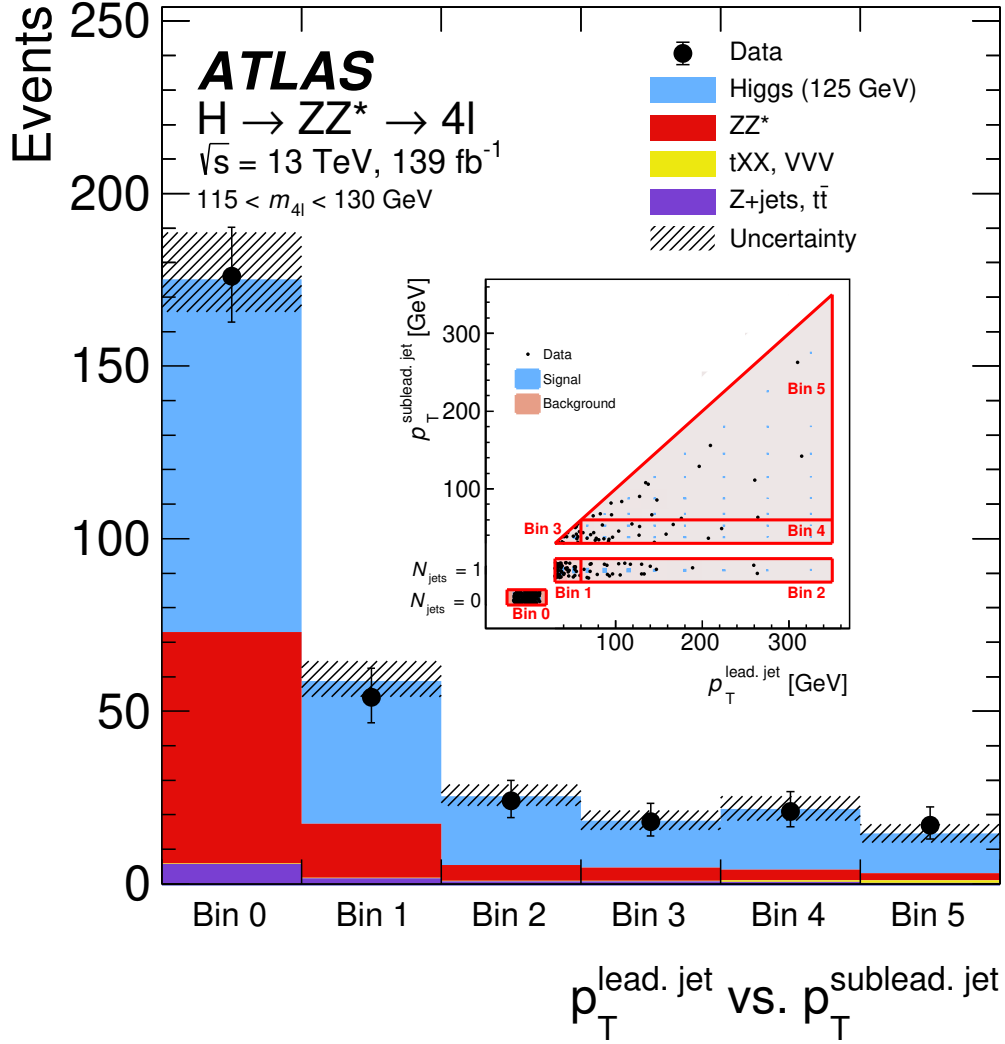
Figure A.14: The observed and expected (pre-fit) distribution in bins of the transverse momentum of the leading vs. subleading jet, p_T^{\text{lead. jet}} vs. p_T^{\text{sublead. jet}} . The same distribution in the 2D plane is provided in the inset plot, where the black dots depict data and the blue and pink shaded areas represent simulated signal and background, respectively. The red lines depict the bin boundaries. These distributions correspond to the mass region 115 < m_{4l} < 130 \text{ GeV} , for an integrated luminosity of 139 \text{ fb}^{-1} collected at \sqrt{s} = 13 \text{ TeV} . A SM Higgs boson signal with a mass m_H = 125 \text{ GeV} is assumed. The uncertainty in the prediction is shown by the hatched band, which includes the theoretical uncertainties of the SM cross section for the signal and the ZZ^* background.
