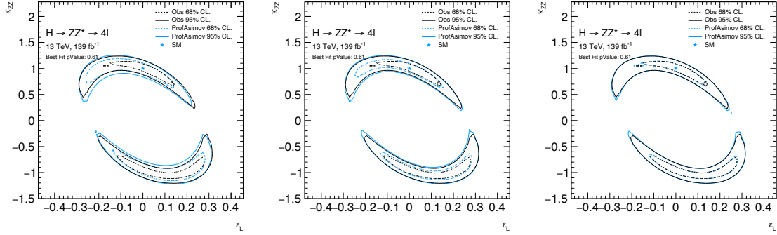
Figure 7.16: Observed exclusion limits (black lines) compared with ones obtained from the asimov dataset (blue lines) generated with \sigma_{bin1_{incl}} equal to 1 (on the left), 1.2 (in the center), 1.29 (on the right) times the expected value, and the others XS equal to the SM value, in the Linear-EFT scenario.
