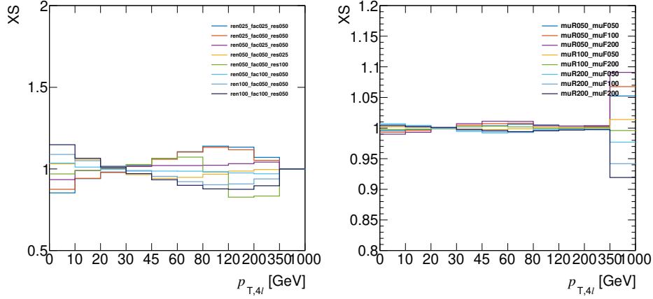
Figure 7.27: Scale variations for the gluon (left) and quark (right) initiated processes for the SM point
