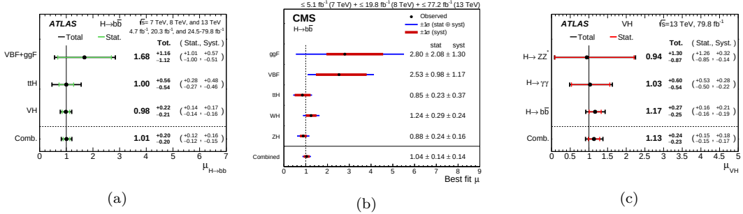
Figure 1.12: Signal strength \mu_{H \rightarrow b\bar{b}} for individual search channels and their combination for the (a) ATLAS [35] and (b) CMS experiment [36]. (c) Signal strength \mu_{VH} for each decay channel search and the combined result for the ATLAS experiment [35].
