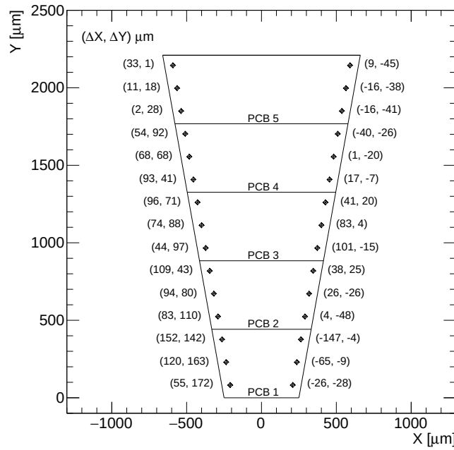
Figure 4.19: Scheme of the \Delta X and \Delta Y displacement of the readout strips between the Eta and the Stereo readout panel.
