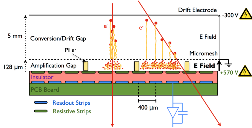
Figure 3.10: Schematic view of the Micromegas detector and the principles of operation.
