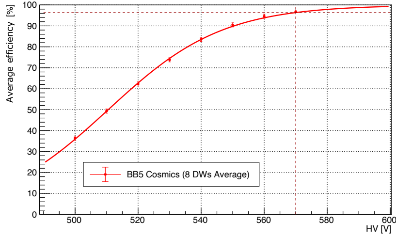
Figure 4.64: Average efficiency as a function of the HV of the Small Double Wedges.
