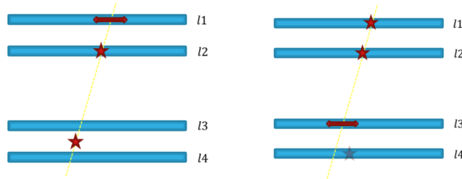
Figure 4.23: The self-tracking algorithm is used to estimate the efficiency on the layer i reconstructing the track on the other N - 1 layer. The method to estimate the efficiency on the Eta layer is shown on the left, in which a super-point from the Stereo layer is used, instead on the right is shown the method used for the Stereo layer (super-point from the other Stereo layer and one of the Eta layer).
