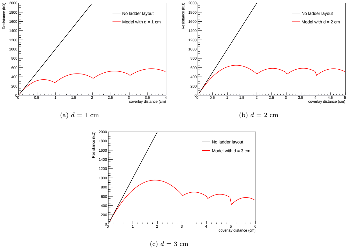
Figure 4.52: Comparison between the resistance as function of the coverlay distance with (red line) and without (black line) the interconnection pattern in the PCB layout. The three plots show different first interconnection distance values: (a) 1 cm, (b) 2 cm and (c) 3 cm.
