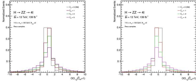
(a) \mathcal{OO}_{1,jj}(\tilde{c}_{zz} = 1) with CP-odd \tilde{c}_{zz} = +1, +2, +5
