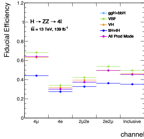
Figure 6.6: Comparing the fiducial efficiency at m_H = 125 GeV using the dressed truth lepton definition in the mass range 105 < m_{4\ell} < 160 GeV for different production mode in the four final states.
