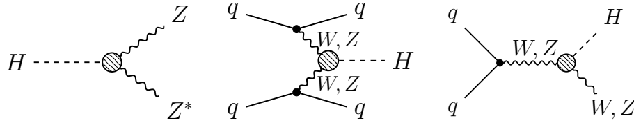
Figure 6.2: Feynman Diagram of the HZZ Higgs decay and VBF and VH Higgs production with effective HVV vertex.
