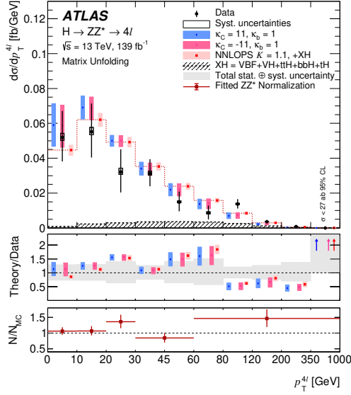
Figure 7.32: p_{T,4\ell} differential cross section measurement compared with predictions at 95% confidence level for \kappa_C for the Shape Only scenario.
