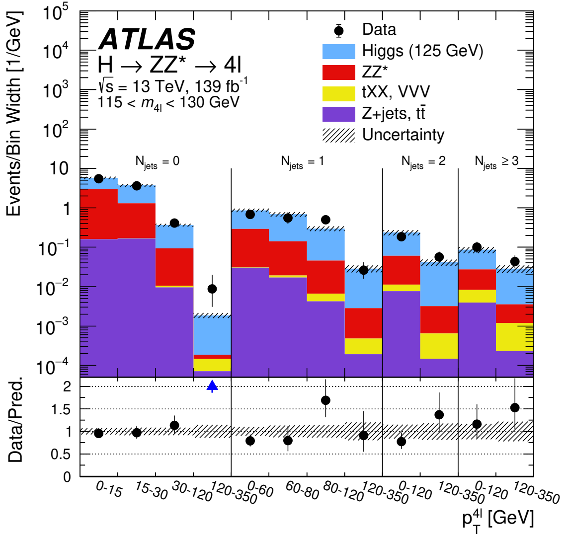
Figure A.9: The observed and expected (pre-fit) distributions of p_T^{4\ell} in N_{\text{jets}} bins in the mass region 115 < m_{4\ell} < 130 \text{ GeV} , for an integrated luminosity of 139 \text{ fb}^{-1} collected at \sqrt{s} = 13 \text{ TeV} . A SM Higgs boson signal with a mass m_H = 125 \text{ GeV} is assumed. The uncertainty in the prediction is shown by the hatched band, which includes the theoretical uncertainties of the SM cross section for the signal and the ZZ^* background.
