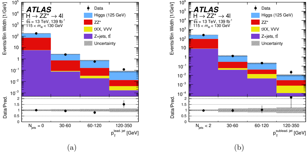
Figure A.6: The observed and expected (pre-fit) distributions of a p_T^{\text{lead. jet}} , and b p_T^{\text{sublead. jet}} in the mass region 115 < m_{4\ell} < 130 GeV, for an integrated luminosity of 139 \text{ fb}^{-1} collected at \sqrt{s} = 13 TeV. A SM Higgs boson signal with a mass m_H = 125 GeV is assumed. The uncertainty in the prediction is shown by the hatched band, which includes the theoretical uncertainties of the SM cross section for the signal and the ZZ^* background.
