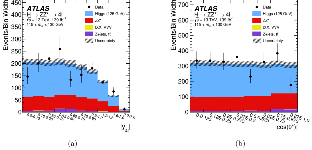
Figure A.2: The observed and expected (pre-fit) distributions of a |y_{4\ell}| and b |\cos\theta^*| in the mass region 115 < m_{4\ell} < 130 GeV, for an integrated luminosity of 139 \text{ fb}^{-1} collected at \sqrt{s} = 13 TeV. A SM Higgs boson signal with a mass m_H = 125 GeV is assumed. The uncertainty in the prediction is shown by the hatched band, which includes the theoretical uncertainties of the SM cross section for the signal and the ZZ^* background.
