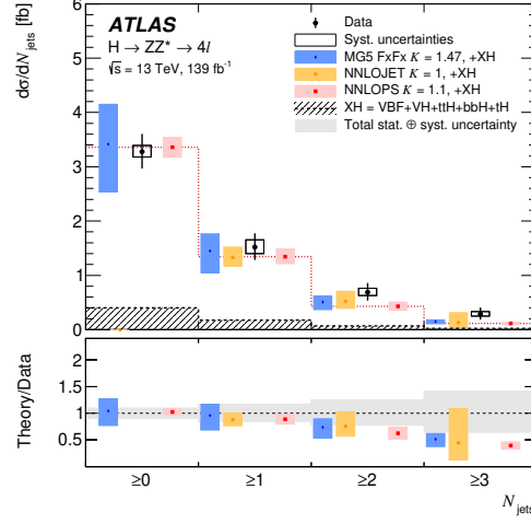
Figure A.20: Differential fiducial cross sections for the inclusive jet multiplicity. In this N_{\text{jets}} distribution all bins are inclusive, with the first bin including all events, the second including all events with at least one jet, and so on.
