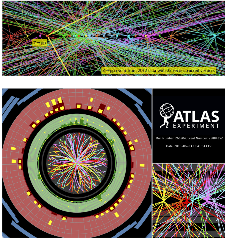
Figure 2.10: On the top : Picture of a Z \rightarrow \mu\mu event recorded by ATLAS with 25 reconstructed primary vertices in 8 TeV collision. On the bottom : Display of a proton-proton collision event recorded by ATLAS on 3 June 2015, with the first LHC stable beams at a collision energy of 13 TeV. Tracks originate from 8 primary vertices recorded in one event.
