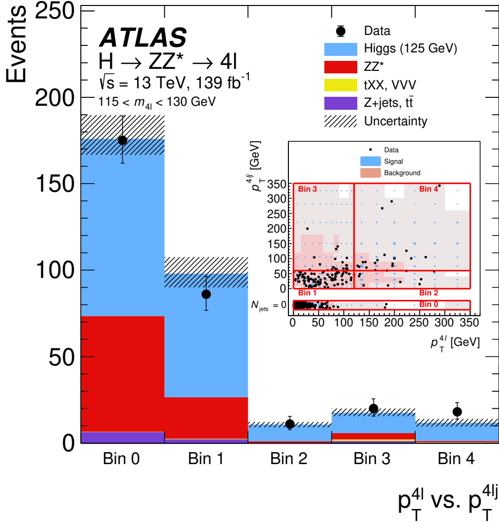
Figure A.12: The observed and expected (pre-fit) distribution in bins of the transverse momentum of the four-lepton system vs. the transverse momentum of the four-lepton plus leading-jet system, p_T^{4l} vs. p_T^{4lj} . The same distribution in the 2D plane is provided in the inset plot, where the black dots depict data and the blue and pink shaded areas represent simulated signal and background, respectively. The red lines depict the bin boundaries. These distributions correspond to the mass region 115 < m_{4\ell} < 130 \text{ GeV} , for an integrated luminosity of 139 \text{ fb}^{-1} collected at \sqrt{s} = 13 \text{ TeV} . A SM Higgs boson signal with a mass m_H = 125 \text{ GeV} is assumed. The uncertainty in the prediction is shown by the hatched band, which includes the theoretical uncertainties of the SM cross section for the signal and the ZZ^* background.
