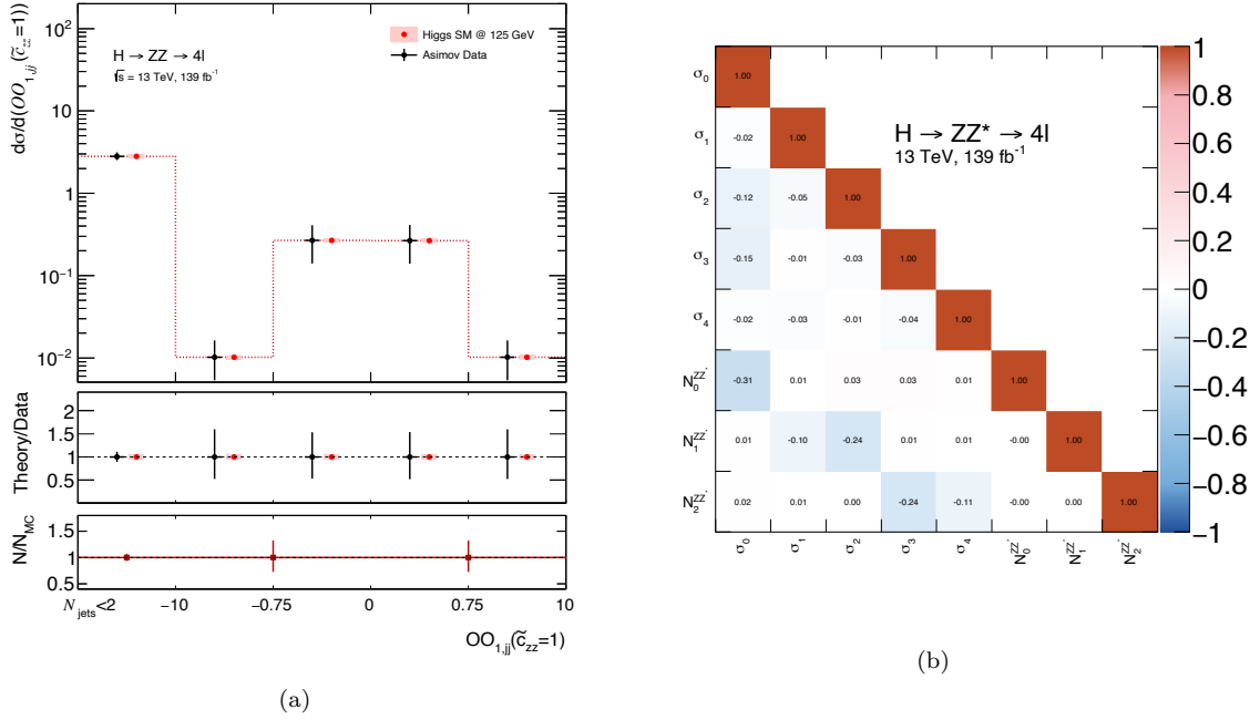
Figure 6.42: (a) Expected results for differential fiducial cross section for \mathcal{O}_{1,jj}(\tilde{c}_{zz} = 1) optimal observable, along with (b) the corresponding correlation matrix between the measured cross sections and the ZZ^* background normalisation factors.
