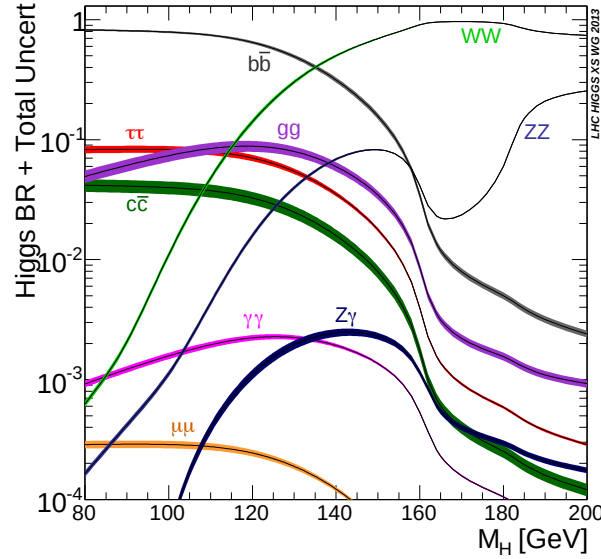
Figure 1.8: Standard Model Higgs boson decay branching ratios as a function of the Higgs boson mass [26].
