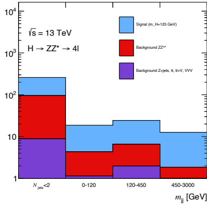
Figure 6.14: Distribution and binning choice for m_{jj} : for each bin, signal and background yields are reported for 115 < m_{4\ell} < 130 GeV together with S/B and expected significance values. A SM Higgs with m_H = 125 GeV has been assumed.
