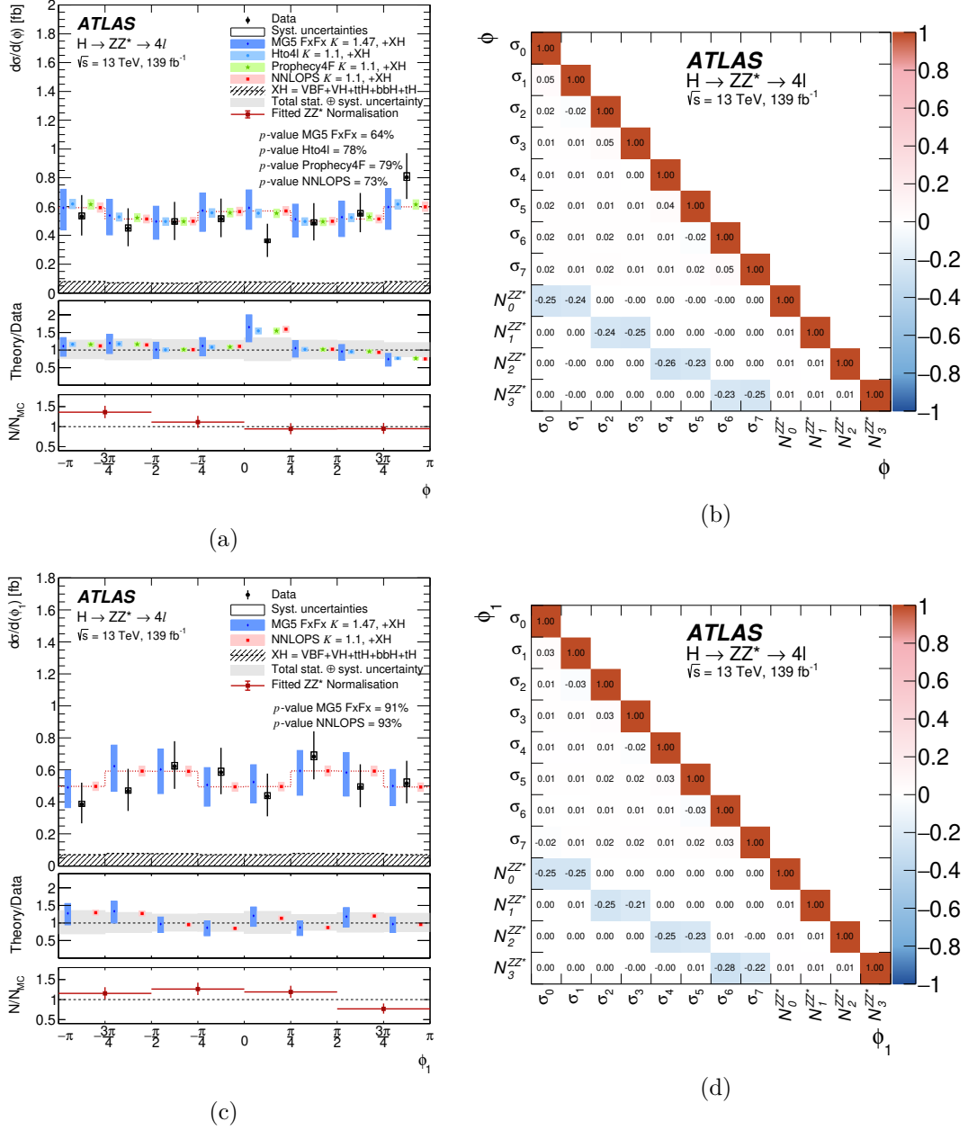
Figure A.19: Differential fiducial cross sections for a the azimuthal angle, \phi , between the decay planes of the two reconstructed Z bosons and c the azimuthal angle, \phi_1 , between the decay plane of the leading Z boson and the plane formed by its four-momentum and the z -axis. The corresponding correlation matrices between the measured cross sections and the ZZ^* background normalisation factors are also shown ( b and d ).
