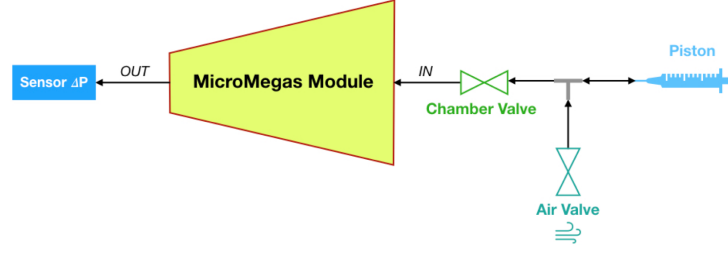
Figure 4.15: Setup scheme used at LNF to perform the pressure drop measurement.
