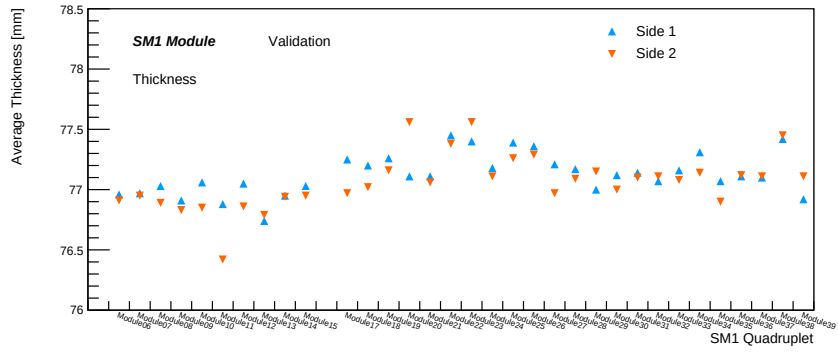
Figure 4.26: Summary thickness measurements.
