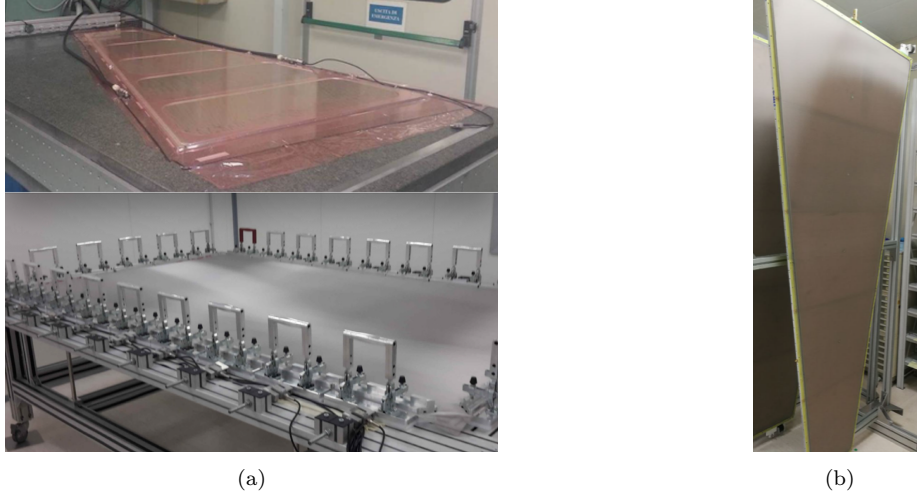
Figure 4.2: Drift panel construction steps: (a) the vacuum bag technique ( on the top ), the mesh on the stretching table ( on the bottom ) and (b) the drift panel finalised.
