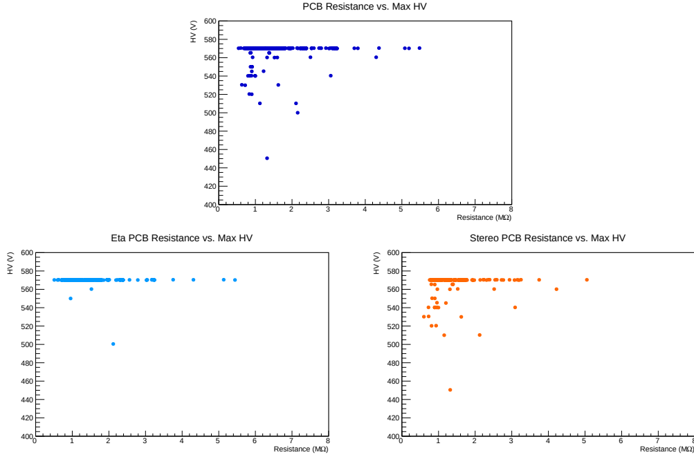
Figure 4.39: Correlation between the resistance measurement performed at Pavia on the PCBs and the HV value of the corresponding HV section measured at LNF. The plots on the bottom show the same statistics, but splitted for Eta PCBs and Stereo PCBs.
