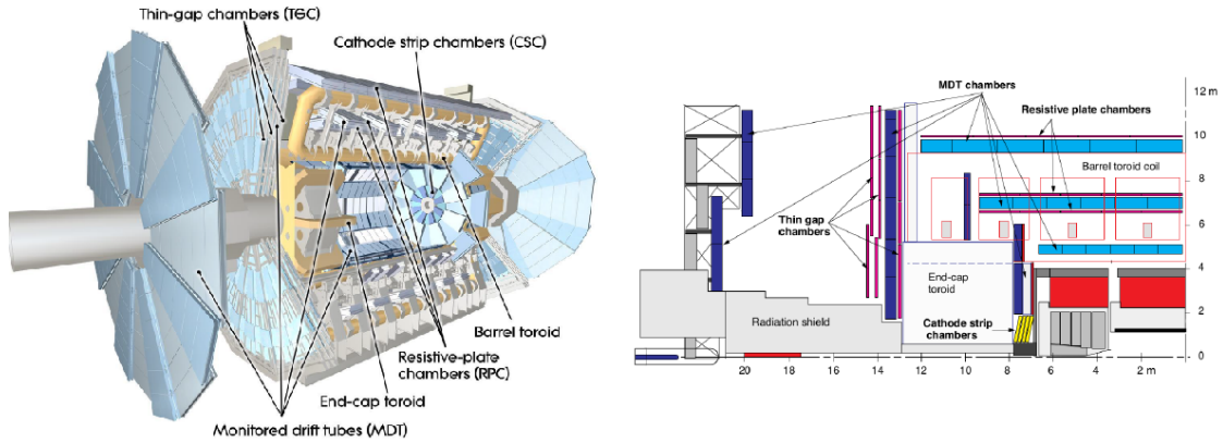
Figure 2.8: The ATLAS Muon Spectrometer [3]. On the right is shown the layout of the muon spectrometer in a quarter of the y - z plane, with the interaction point located in the lower right corner.
