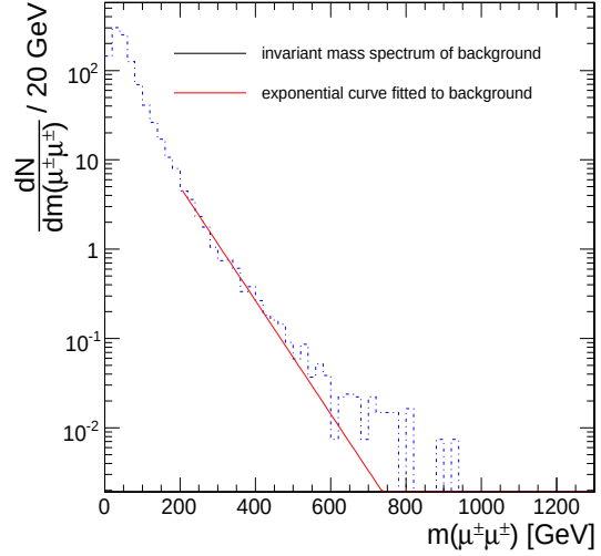
Figure 10.5: Distribution of the invariant reconstructed H^{\pm\pm} mass for all background events at an integrated luminosity of 10 \text{ fb}^{-1} , and the exponential curve fitted to the background.
