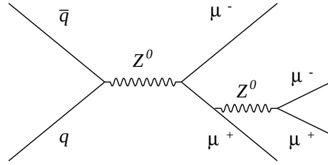
Figure 6.3: s-channel Feynman diagram for the process q\bar{q} \rightarrow ZZ^{(*)} .
