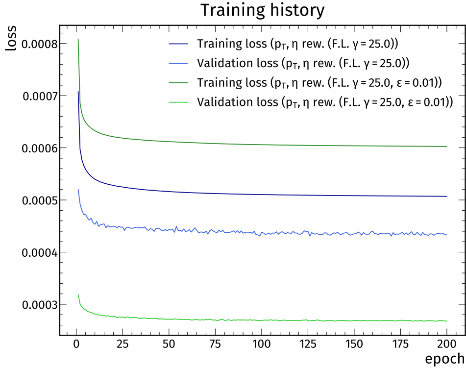
Figure 2.11: Training and validation loss over epoch. The blue curves represent the basic training and the green ones result from the training with adversarial samples. In both cases, the darker colour shows the training loss, while the lighter colour shows the validation loss.
