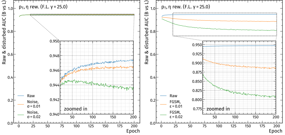
Figure 4.8: Evolution of the BvsL–AUC with the number of epochs for the basic training, evaluated on raw and distorted inputs (adding noise with \sigma = 0.01 and \sigma = 0.02 (left) or by using the FGSM attack with \epsilon = 0.01 and \epsilon = 0.02 (right)).
