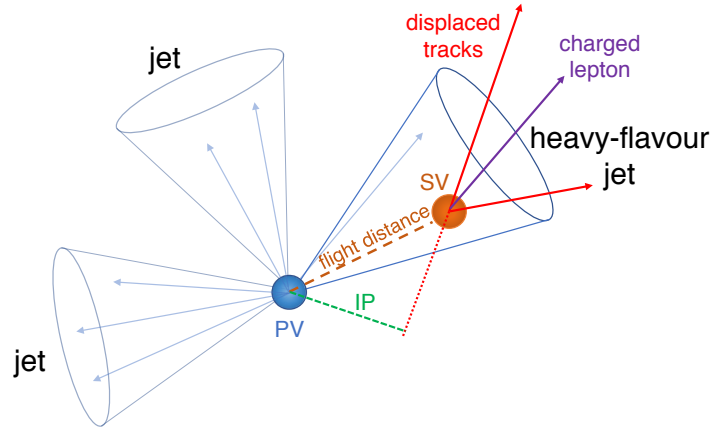
Figure 1.5: Visualization of three jets, emerging from a primary vertex (PV), where distinct properties of the heavy-flavour jet like a secondary vertex (SV) with displaced tracks and a large impact parameter (IP) are highlighted [8].
