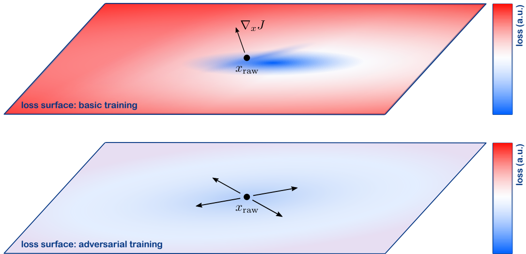
Figure 4.14: Illustration of the assumed geometry of the loss surfaces for the basic as well as the adversarial training. Inspired by Refs. [112, 65, 62]
