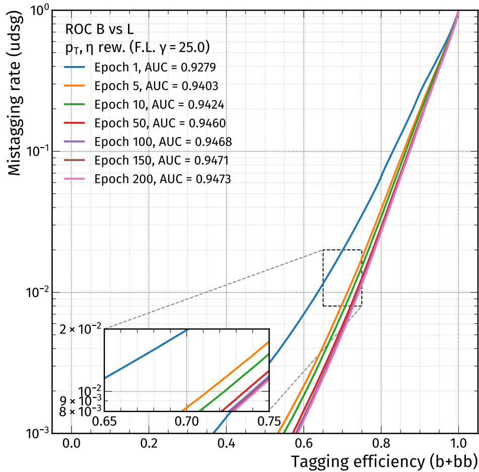
Figure 3.6: ROC curves for the BvsL discriminator, evaluated at different checkpoints of the training. The area under the ROC curve (AUC) increases with more epochs, but the gain in performance becomes smaller as the model converges.
