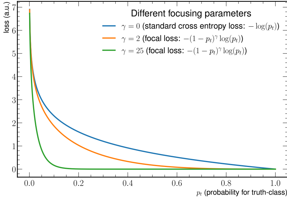
Figure 2.10: Dependence of the focal loss on the chosen focusing parameter. Using \gamma = 0 would restore the standard cross entropy loss function. Higher values like \gamma = 2 (see appendix) or \gamma = 25 (used for the investigations of robustness) suppress easy to classify samples. Adapted from Fig. 1 in Ref. [99], with slightly modified focusing parameters.
