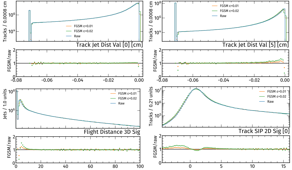
Figure 4.2: Distribution of raw and distorted inputs, for features where the impact of the adversarial attack is visible and results in specific patterns for the ratios. The top row shows the distance between the first (on the left) and sixth track (on the right) and the jet axis at their point of closest approach, while the second row depicts the SV 3D flight distance significance on the left and the the 2D signed impact parameter significance of the first track on the right. For the adversarial attacks, the parameters are either moderate ( \epsilon = 0.01 ) or rather large ( \epsilon = 0.02 ).
