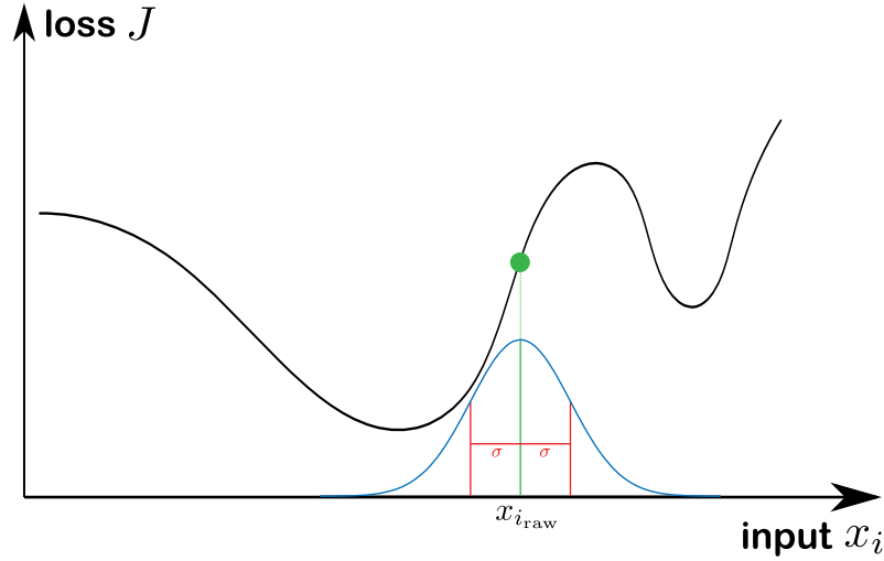
Figure 1.6: Visualization of the random shift of inputs by adding a Gaussian noise term. With the slight distortion based on the blue probability distribution, the formerly green raw data-point is shifted and the corresponding loss is modified. The change of the loss function with respect to the distorted inputs can go in either direction. For all considered inputs where this method is applicable, the small additional noise term is drawn from a normal distribution with the same fixed standard deviation \sigma and in the current setup without any offset ( \mu = 0 ). Gaussian distribution adapted from Ref. [61].
