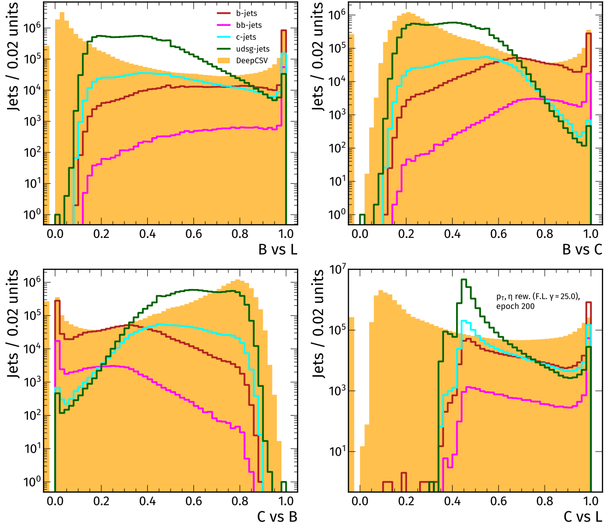
Figure 3.2: Discriminators, evaluating the basic training (split by flavour) and DeepCSV (summed) on test inputs. Each subfigure represents one discriminator between two flavours (with category b and bb merged into “B”) after 200 epochs.
