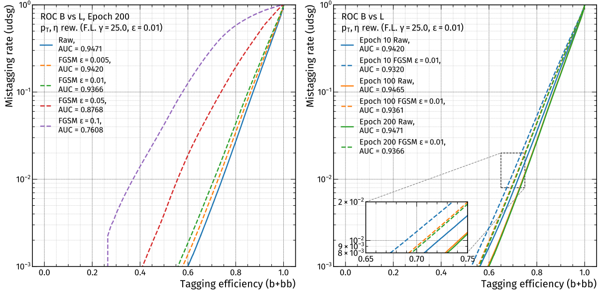
Figure 4.10: ROC curves for the BvsL discriminator, evaluating the adversarially trained model with raw and distorted inputs (FGSM), either with a fixed epoch with different parameters \epsilon , or with a fixed parameter \epsilon , but evaluated at different checkpoints of the training.
