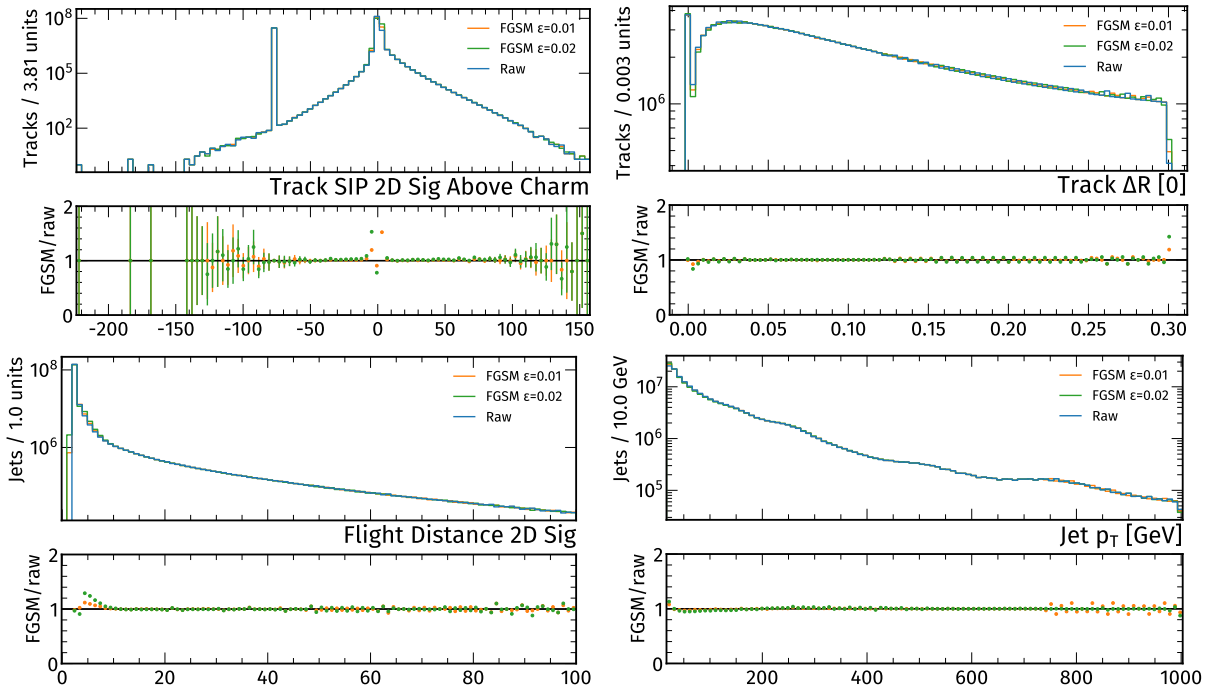
Figure A.8: Systematically distorted inputs that show distinct patterns also for large x axis ranges. For the adversarial attacks, the parameters are either moderate ( \epsilon = 0.01 ) or rather large ( \epsilon = 0.02 ).
