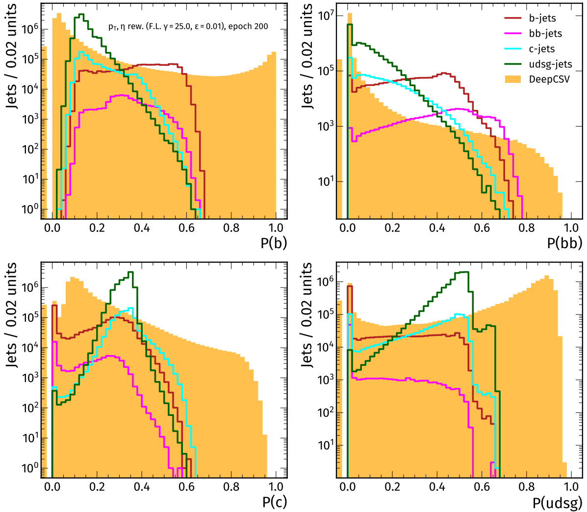
Figure A.12: Tagger outputs, evaluating the adversarial training with \gamma = 25 (split by flavour) and DeepCSV (stacked) on test inputs. Each subfigure represents one output node of the model.
