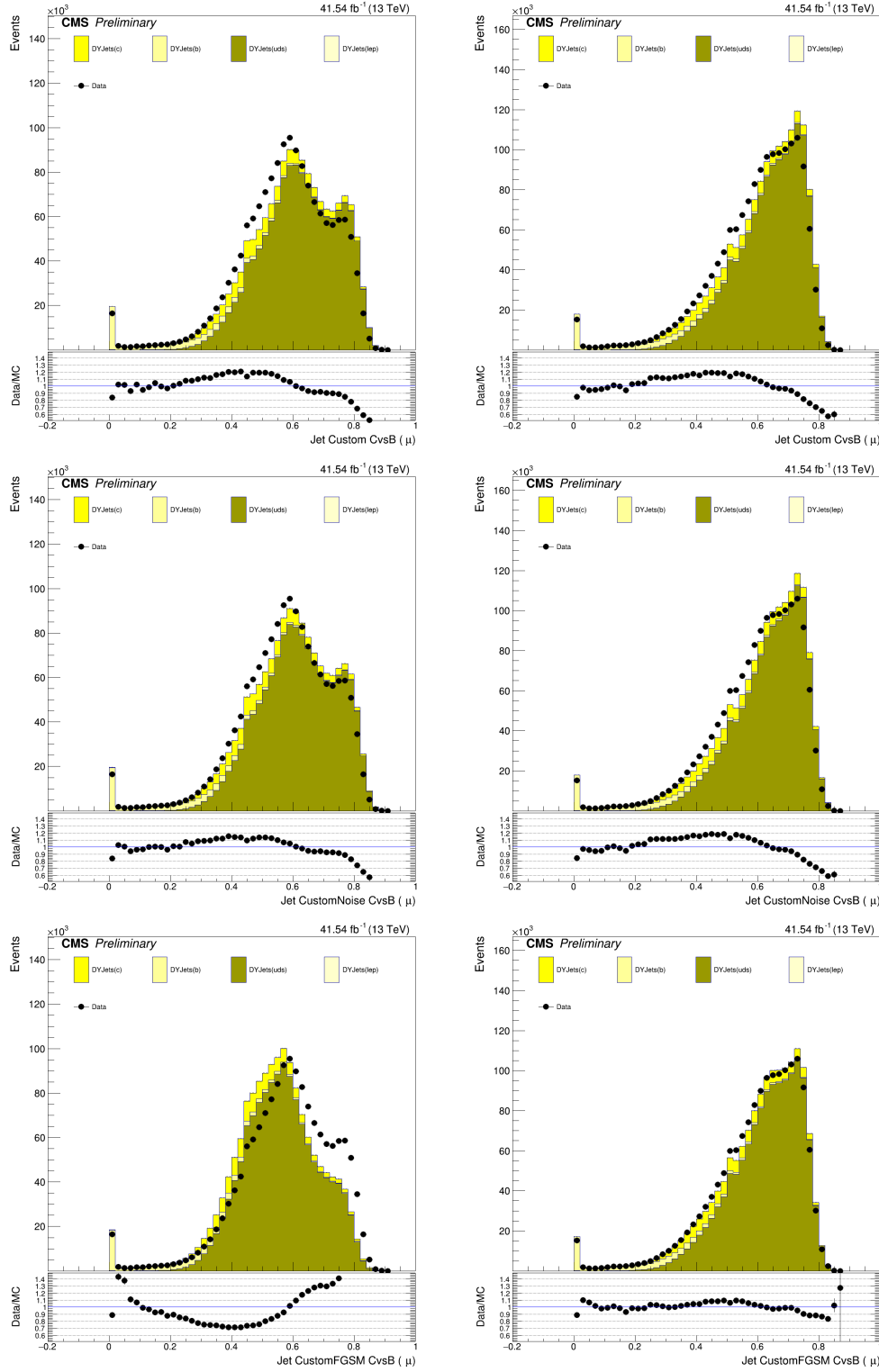
Figure A.19: Stacked histograms of the CvsB discriminator for the DY+jets selection, evaluated with the basic model (left column) and the adversarially trained model (right column). Concerning the simulated samples, the first row utilizes raw inputs, the second row results from the addition of a Gaussian noise term (with \sigma = 0.01 ) and the third row corresponds to systematically distorted inputs (FGSM attack with \epsilon = 0.01 ). The measured data distributions are identical for all plots and have not been modified by any distortion (= raw).
