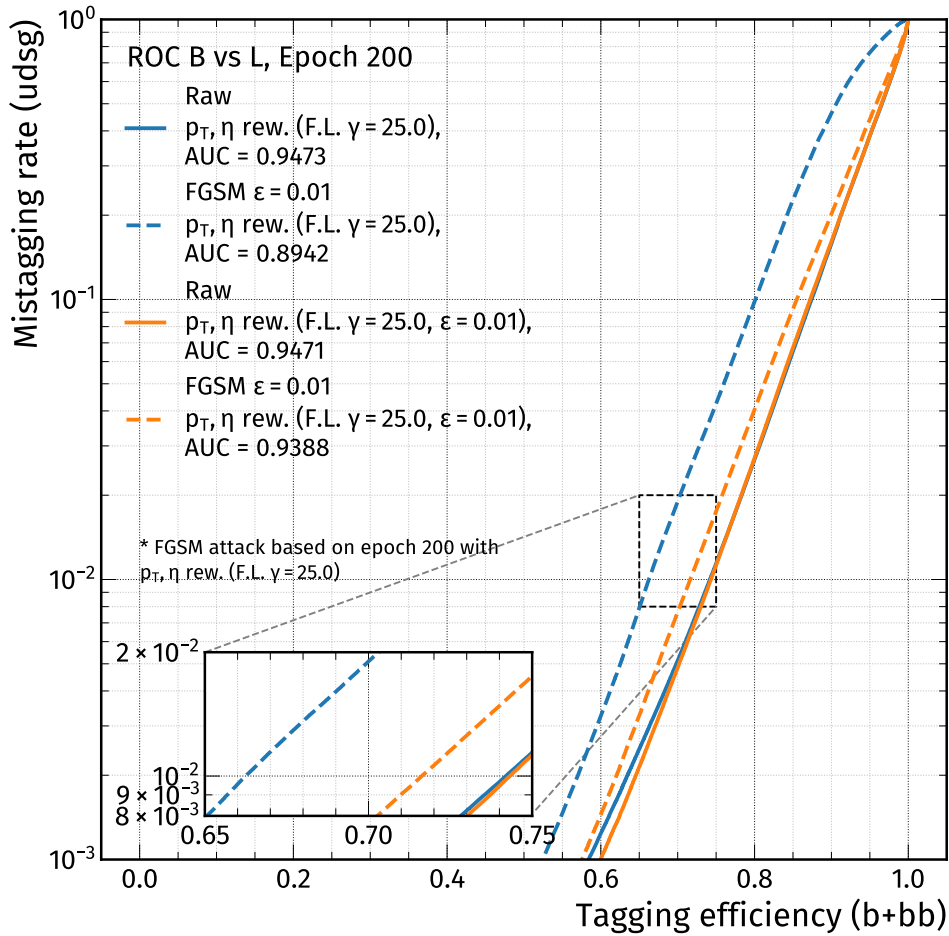
Figure 4.16: ROC curves for the BvsL discriminator, evaluated at epoch 200 with raw and adversarial inputs, using \epsilon = 0.01 for the FGSM attack obtained from the baseline classifier, injected to the basic model as well as the adversarially trained model. Raw performance is visualized with solid lines, the performance on distorted inputs uses dashed lines. The basic (adversarial) training is shown in blue (orange), respectively.
