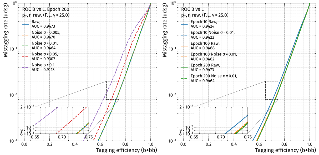
Figure 4.7: ROC curves for the BvsL discriminator, evaluating the basic model with raw and randomly distorted inputs (Gaussian noise), either with a fixed epoch with different parameters \sigma , or with a fixed parameter \sigma , but evaluated at different checkpoints of the training. The left subfigure uses epoch 200, different colours represent different magnitudes of the distortion. On the right, a fixed parameter \sigma = 0.01 (dashed lines) is utilized in comparison with raw inputs (solid lines), for different epochs in different colours.
