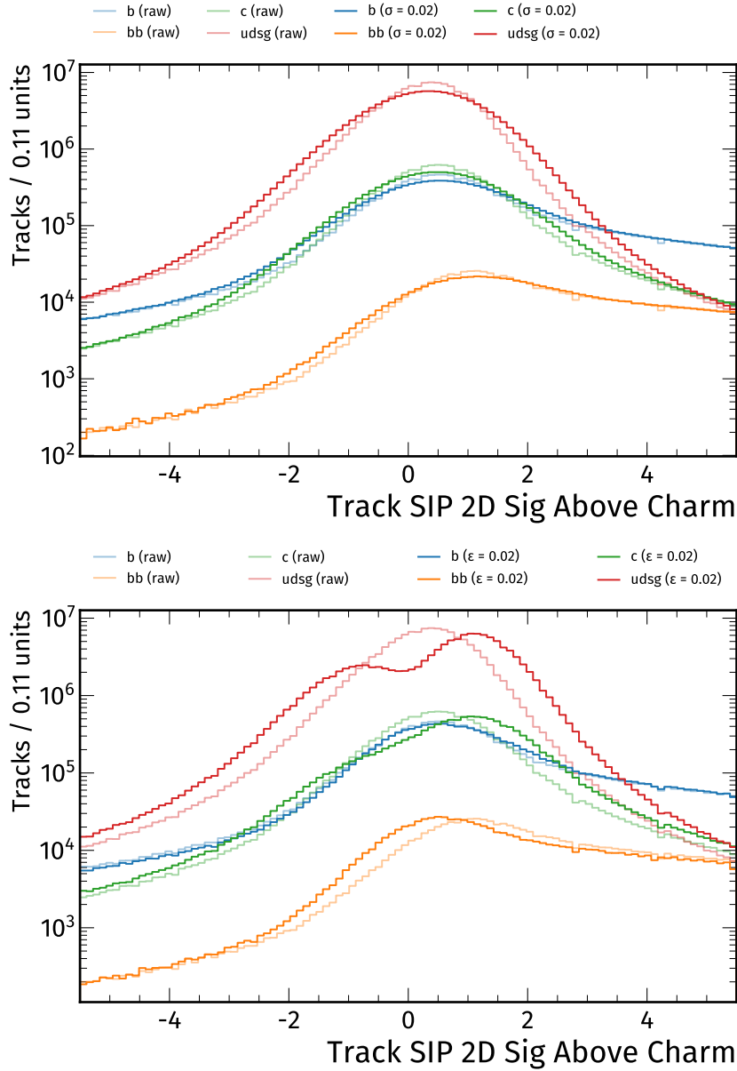
Figure 4.3: Detailed examination of the flavour-dependent impact of adversarial attacks, with a trend towards unphysical shapes. In this example, the 2D signed impact parameter significance for the first track above the charm mass threshold is depicted for raw and distorted inputs, with light and saturated colours, respectively. In a limited interval, using unusually large parameters, the distorted inputs in the top figure contain a noise term ( \sigma = 0.02 ), while for the second figure, the FGSM attack has been applied ( \epsilon = 0.02 ).
