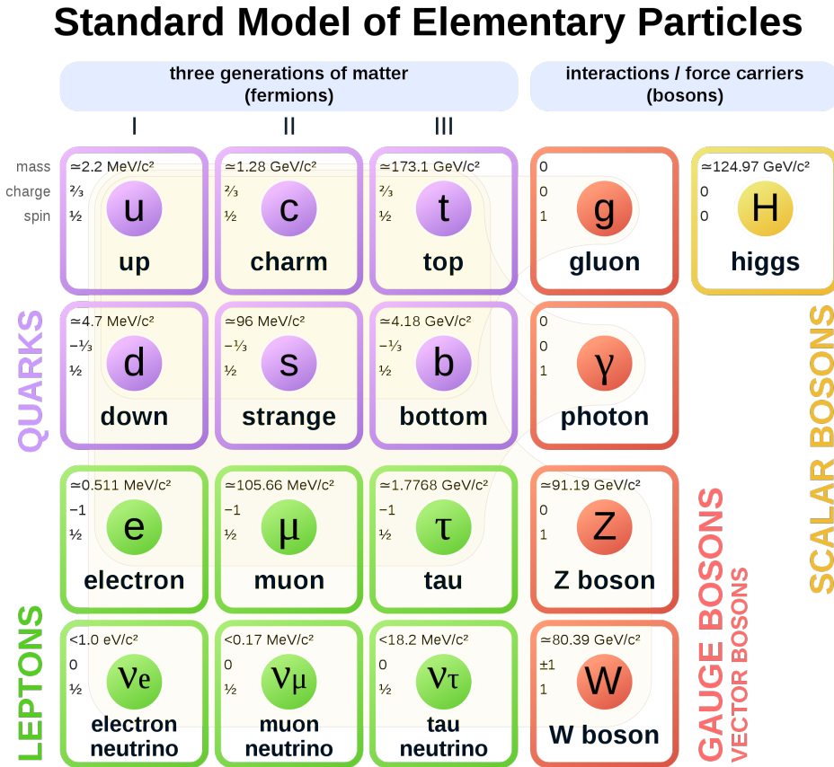
Figure 1.1: The particles in the standard model, including information about the mass, charge and spin of fermions and bosons [13]. Charges are denoted in units of the elementary charge e , the spin is stated in units of \hbar . For all subsequent occurrences, the aforementioned simplification will be used and the constants c (speed of light) and \hbar (reduced Planck constant) will be replaced in accordance with the natural system of units where c = \hbar = 1 .
