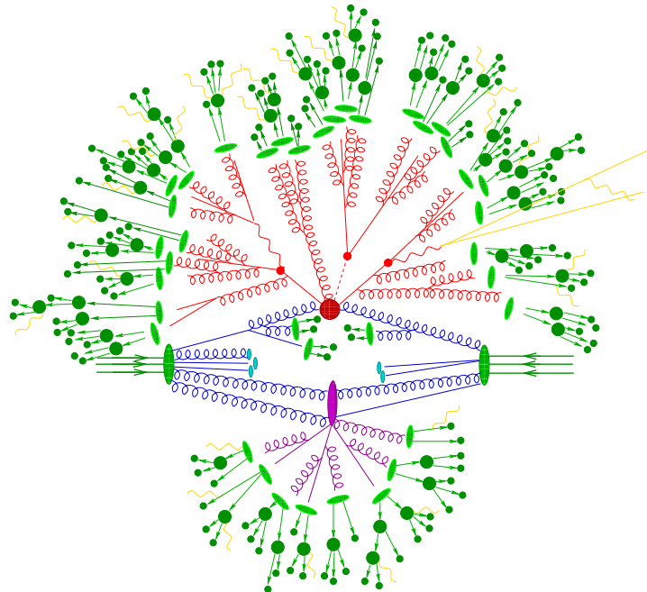
Figure 1.2: Sketch of a hadron collision, resulting from a Monte Carlo event generator [14]. Hard scattering is visualized in the center by a red "blob", a parton shower follows (red). Hadronization is depicted with green blobs, followed by dark green spots that represent hadron decays. Additionally, the purple area shows a secondary hard scattering event (underlying event) [14, 15]. Yellow lines represent soft photon radiation [14].
