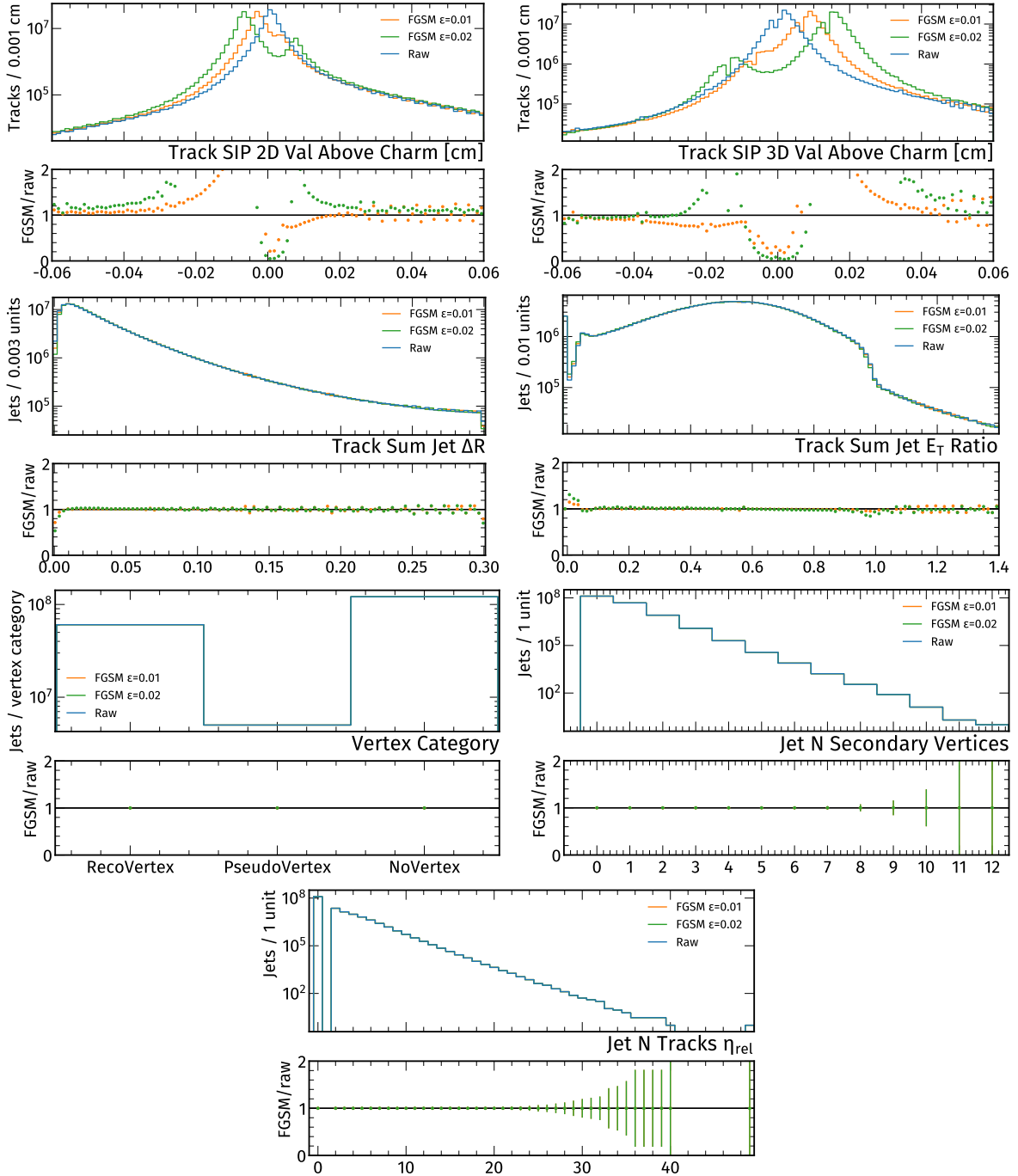
Figure A.9: Remaining jet variables with systematically distorted inputs. For the adversarial attacks, the parameters are either moderate ( \epsilon = 0.01 ) or rather large ( \epsilon = 0.02 ). Note how the categorical or integer features are not modified at all, by construction.
