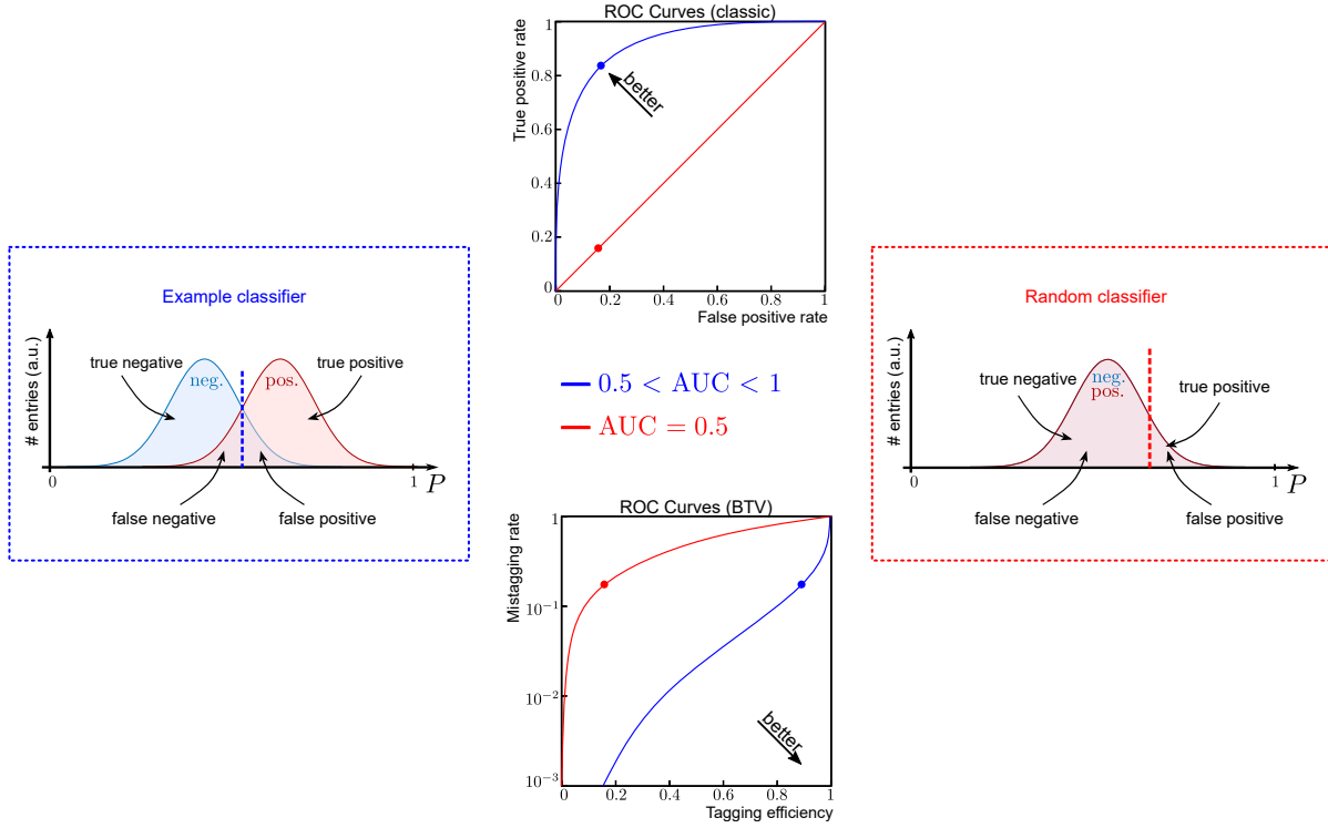
Figure 3.3: Comparison of two hypothetical classifiers, showing the discriminators as well as the corresponding ROC curves. The top ROC curves use the classical axes style and labelling, while the bottom ROC curves adapt the BTV-style. Compared to the example on the left with reasonable tagger performance, the right illustration shows a random classifier. Some possible cutoffs (or thresholds / working points) are given by dashed lines (discriminator shapes) and points (ROC curves). Gaussian distribution adapted from Ref. [61].
