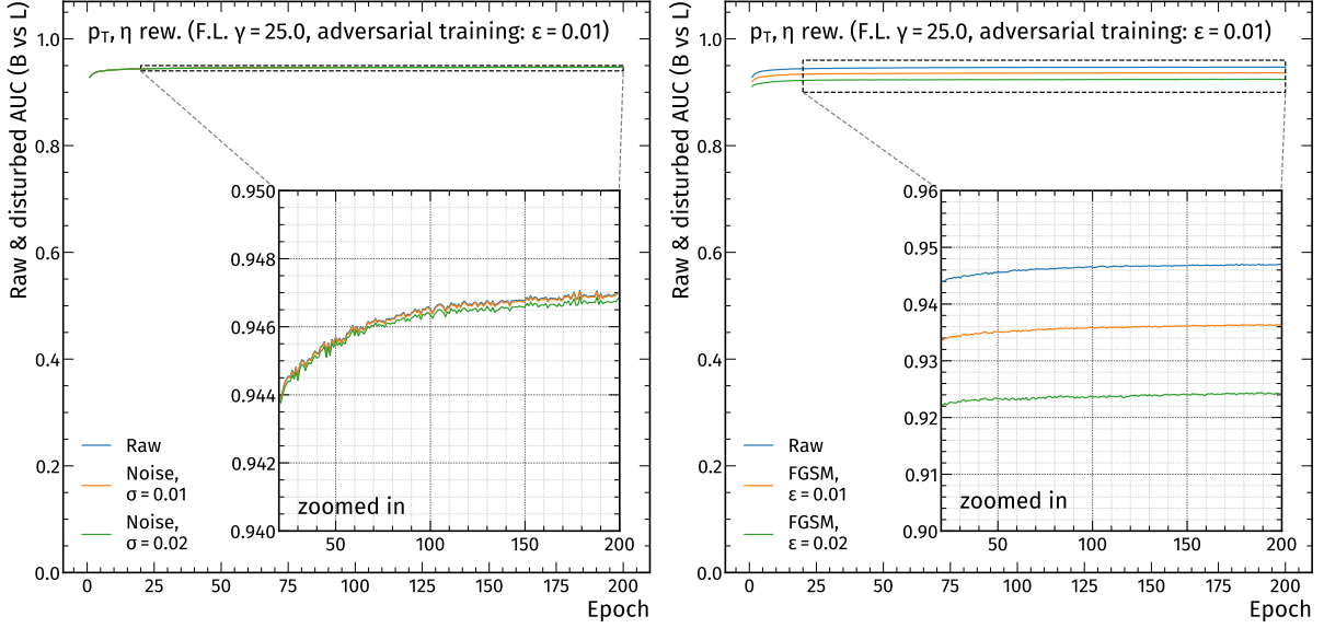
Figure 4.12: Evolution of BvsL–AUC with the number of epochs for the adversarially trained model, evaluated on raw and distorted inputs (adding noise with \sigma = 0.01 and \sigma = 0.02 (left) or by using the FGSM attack with \epsilon = 0.01 and \epsilon = 0.02 (right)).
