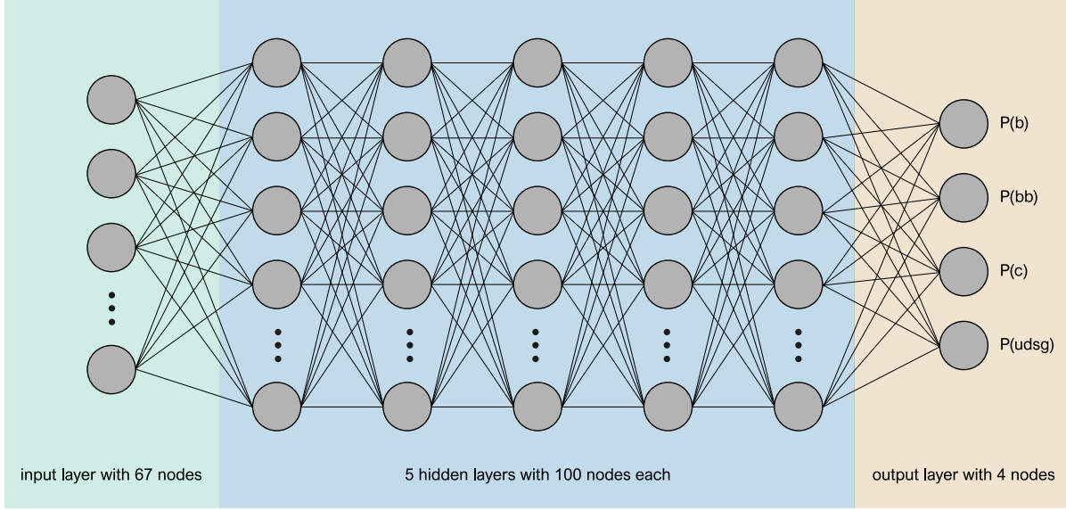
Figure 2.1: Visualization of the network architecture. Modified adaptation of Fig. 1 in Ref. [9].
