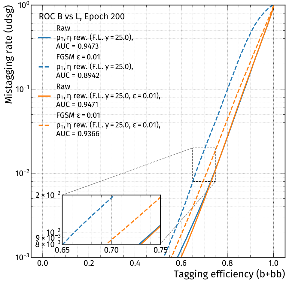
Figure 4.11: ROC curves for the BvsL discriminator, evaluated at epoch 200 with raw and adversarial inputs, using \epsilon = 0.01 for the FGSM attack applied individually to the basic model as well as the adversarially trained model. Raw performance is visualized with solid lines, the performance on distorted inputs uses dashed lines. The basic (adversarial) training is shown in blue (orange), respectively.
