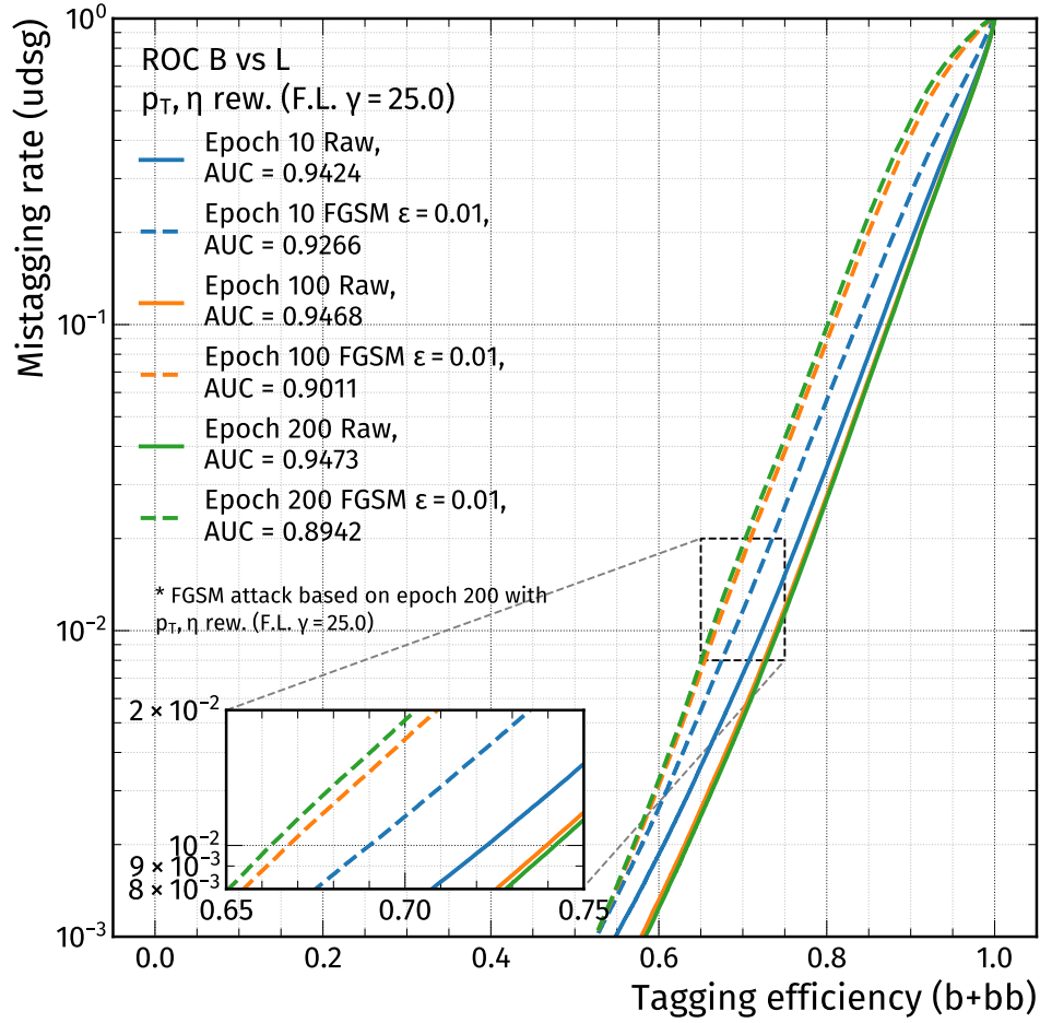
Figure 4.15: ROC curves for the BvsL discriminator, evaluated at epochs 10, 100 and 200 with raw and adversarial inputs, using \epsilon = 0.01 for the FGSM attack on the baseline model, crafted from epoch 200 only and injected to all chosen checkpoints. Different checkpoints are displayed in different colours, ROC curves obtained from raw inputs use solid lines, the ROC curves for distorted inputs use dashed lines.
