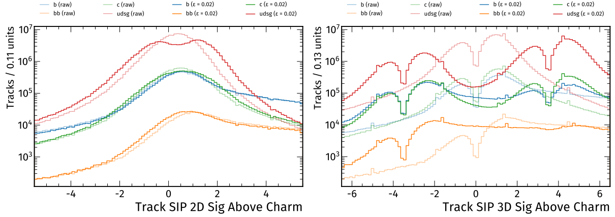
Figure 4.13: Applying the FGSM attack based on an adversarially trained model shows suppressed flavour-dependency and relatively symmetric shapes. The attack uses the parameter \epsilon = 0.02 , which is higher than the moderately chosen parameter of \epsilon = 0.01 during the modified training loop. For comparison, the left figure demonstrates the impact for the 2D signed impact parameter significance for the first track that raises the invariant mass above the charm quark mass, while the right figure depicts the corresponding 3D observable.
