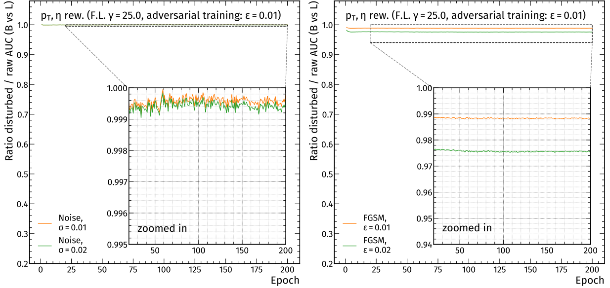
Figure A.18: Evolution of the ratio between distorted and raw BvsL–AUC with the number of epochs for the adversarially trained model, evaluated on raw and distorted inputs (adding noise with \sigma = 0.01 and \sigma = 0.02 (left) or by using the FGSM attack with \epsilon = 0.01 and \epsilon = 0.02 (right)).
