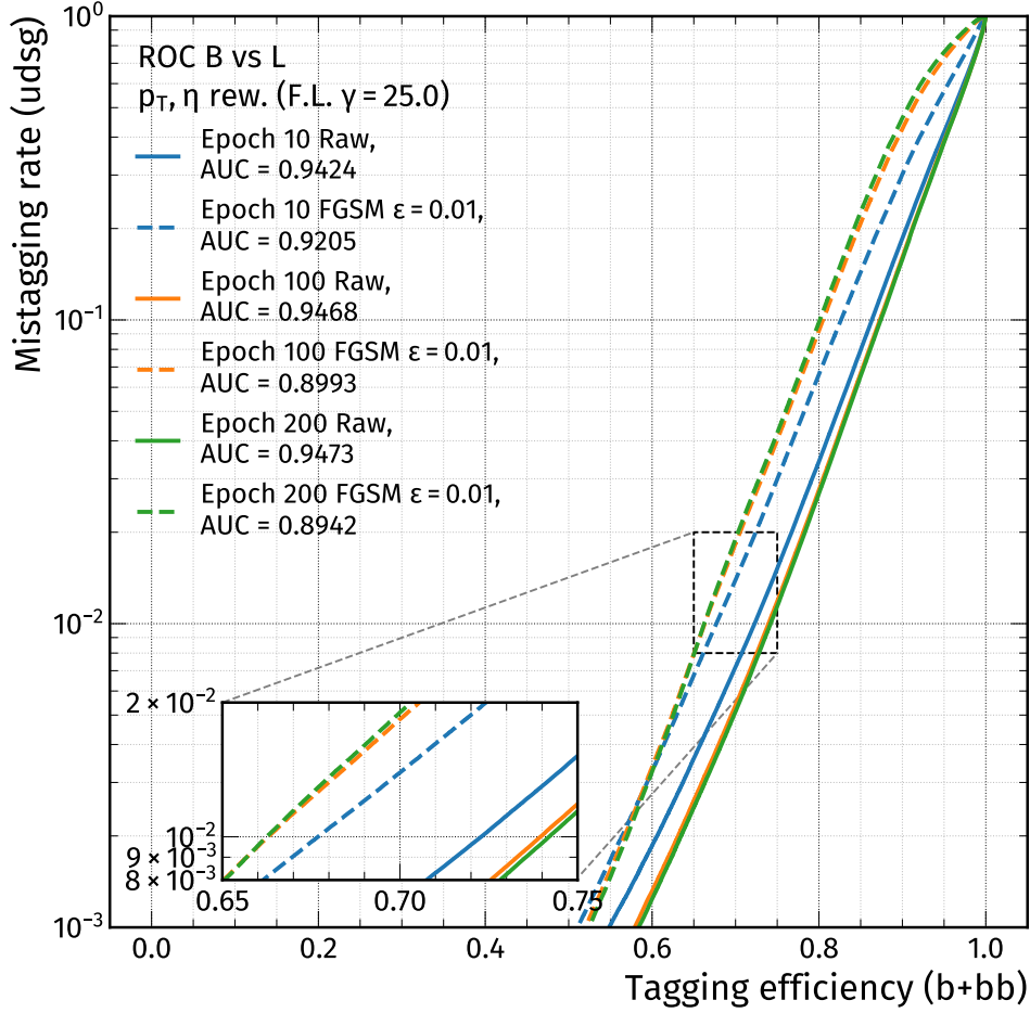
Figure 4.6: ROC curves for the BvsL discriminator, evaluated at epochs 10, 100 and 200 with raw and adversarial inputs, using \epsilon = 0.01 for the FGSM attack on the baseline model, crafted for each epoch individually.
