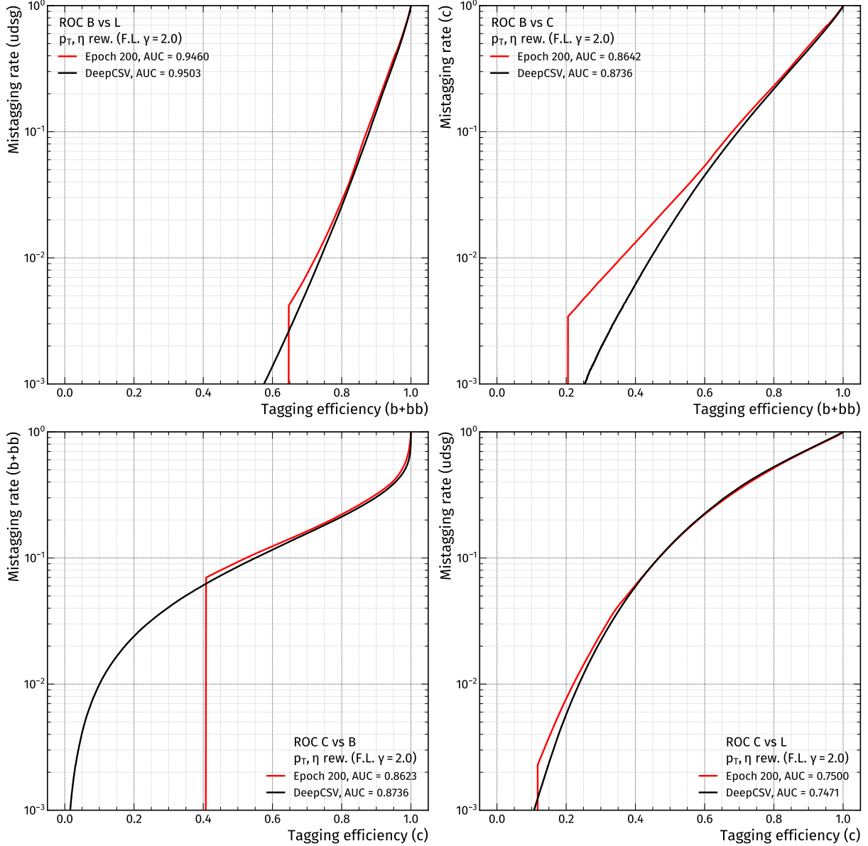
Figure A.6: ROC curves for four different discriminators: BvsL, BvsC, CvsB and CvsL, comparing the custom tagger with \gamma = 2 with DeepCSV. The custom tagger is shown in red, the DeepCSV classifier is visualized with black lines.
