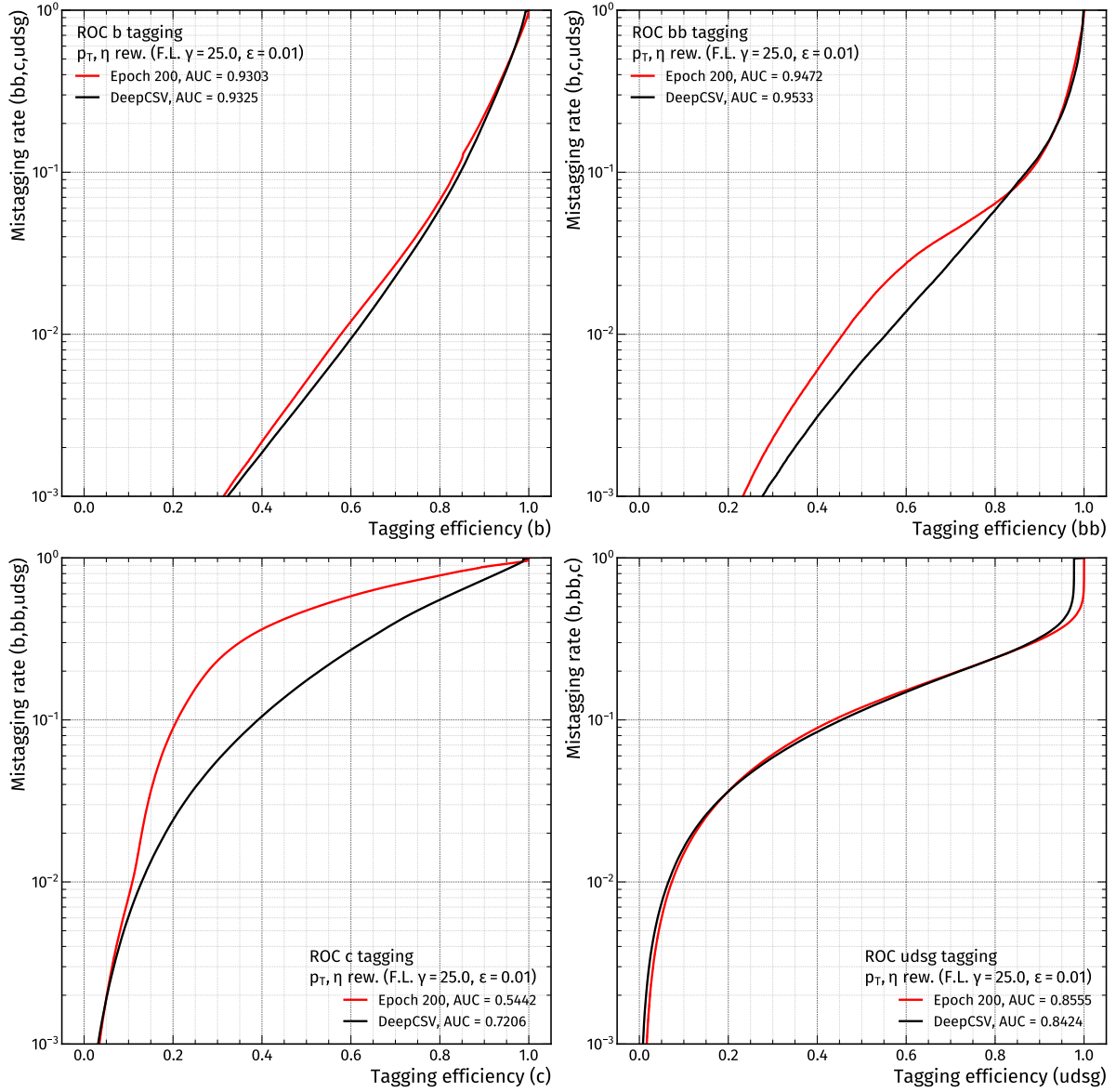
Figure A.14: ROC curves for the adversarial training with \gamma = 25 , when discriminating each flavour (b, bb, c, udsg) against all other flavours. This metric depends on the flavour distribution present in the test sample. Therefore, it is not safe to measure the performance with this method. The custom tagger is shown in red, the DeepCSV classifier is visualized with black lines.
