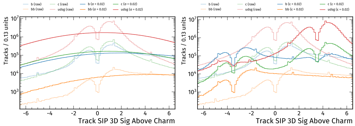
Figure 4.4: Detailed examination of the flavour-dependent impact of adversarial attacks, revealing dramatic unphysical effects. In this example, the 3D signed impact parameter significance for the first track above the charm mass threshold is depicted for raw and distorted inputs, with light and saturated colours, respectively. In a limited interval, using unusually large parameters, the distorted inputs in the left figure contain a noise term ( \sigma = 0.02 ), while for the right figure, the FGSM attack has been applied ( \epsilon = 0.02 ).
