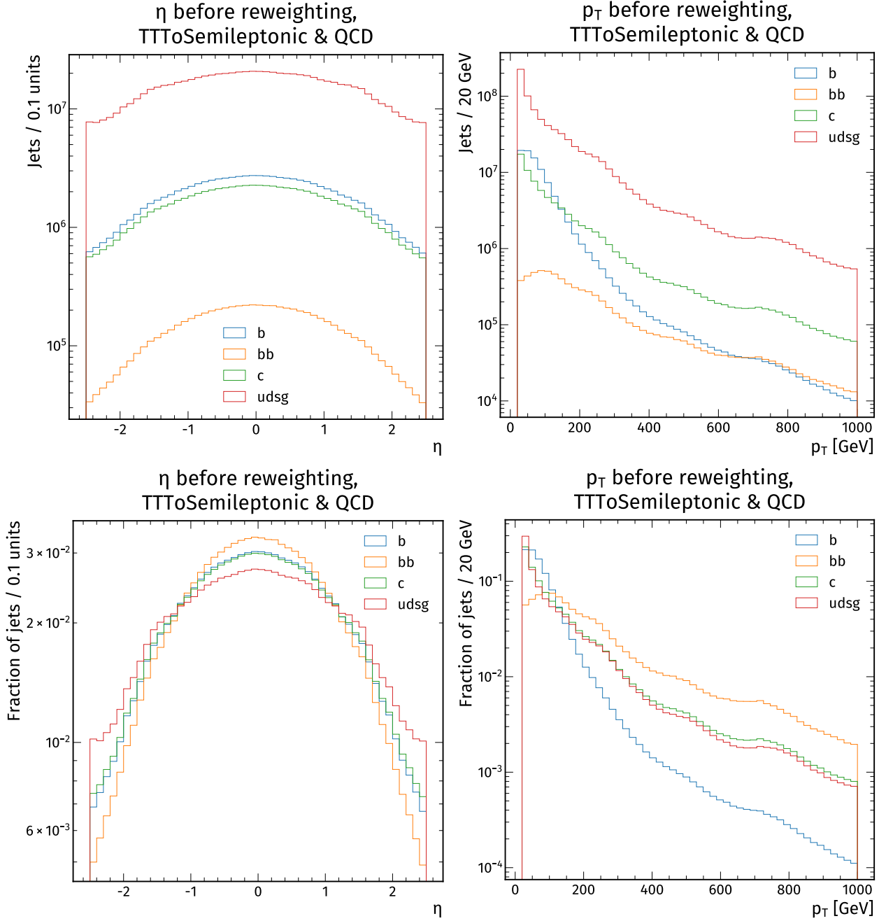
Figure 2.7: \eta distribution before reweighting (left) and p_T distribution before reweighting (right), split by flavour. Obtained by summing over p_T or \eta bins, resulting in marginal distributions in 1D for \eta and p_T . Absolute numbers are given in the first row, while the second row shows the relative fractions.
