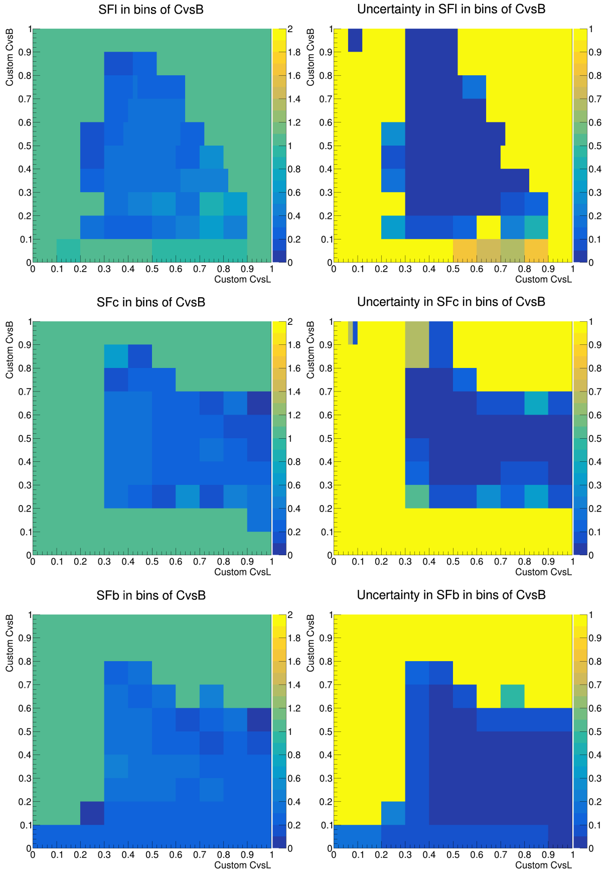
Figure A.21: CvsL / CvsB scale factors in bins of CvsB, for the adversarial training at epoch 200, evaluated on raw inputs. The scale factors are given in the left column, with corresponding uncertainties in the right column. The rows correspond to the different selections (l, c, b).
