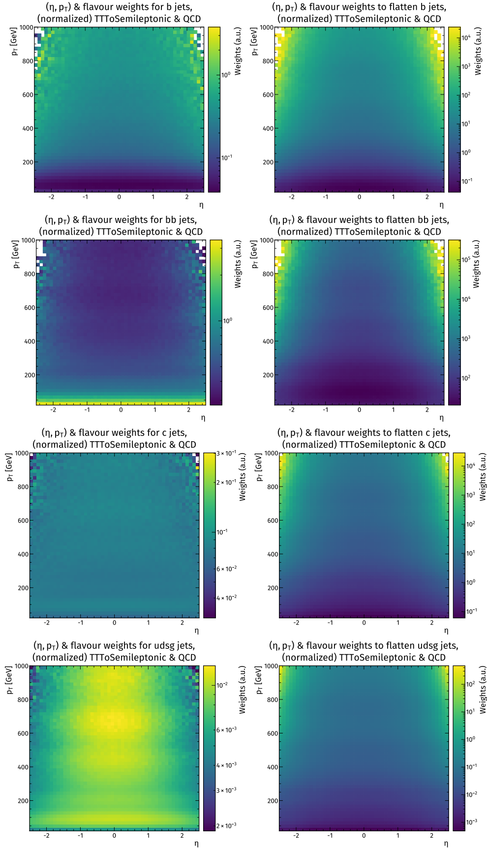
Figure 2.8: 2D (\eta, p_T) weights with two different reweighting approaches, split by flavour. The variant that takes averages per bin is displayed on the left, the one that produces flat distributions is shown on the right. Both columns reveal qualitative differences between the respective reweighting strategies. On the left side, the differences per flavour are clearly visible, on the right side, the differences are not as pronounced, because all flavours are “similarly” far away from a flat distribution. Therefore, absolute scales can not be compared directly.
