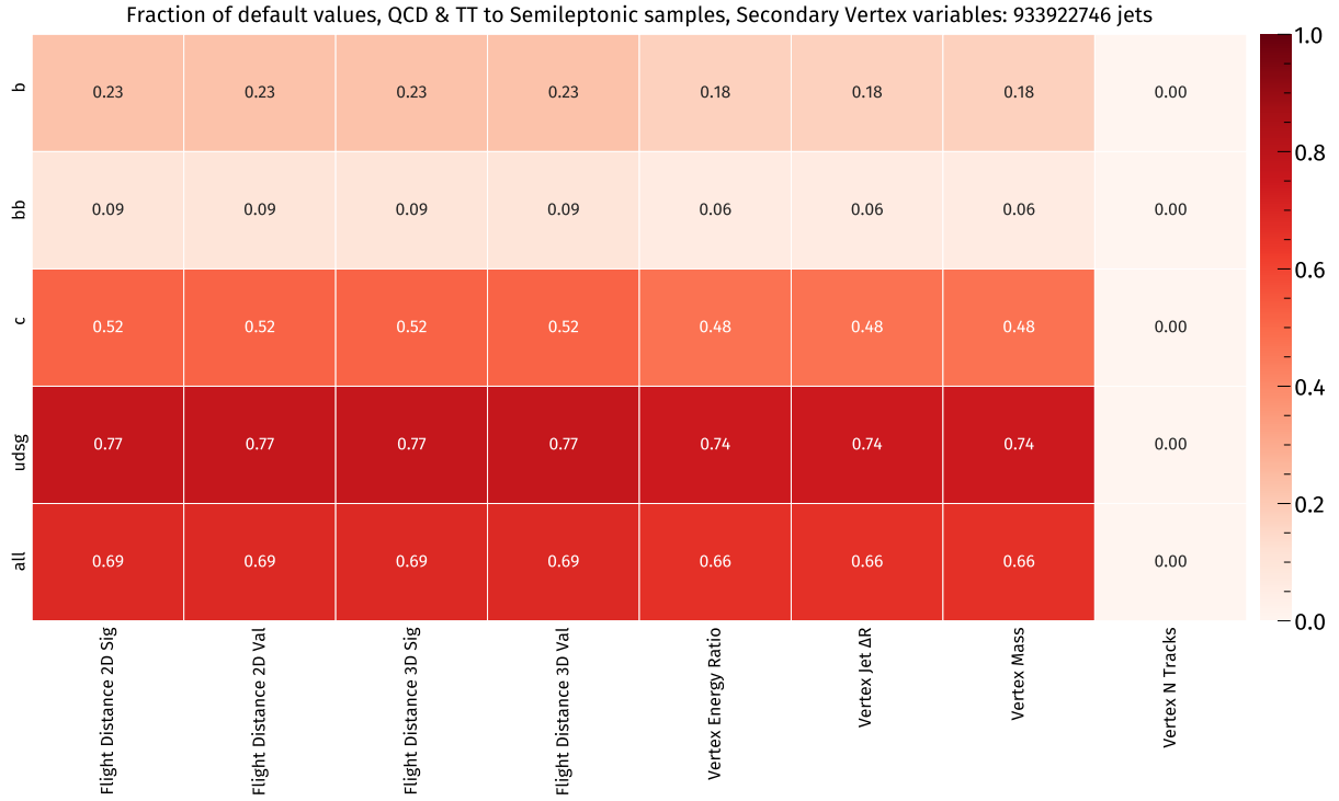
Figure 2.4: Fraction of default values for secondary vertex variables, split by flavour or obtained from all available jets.
