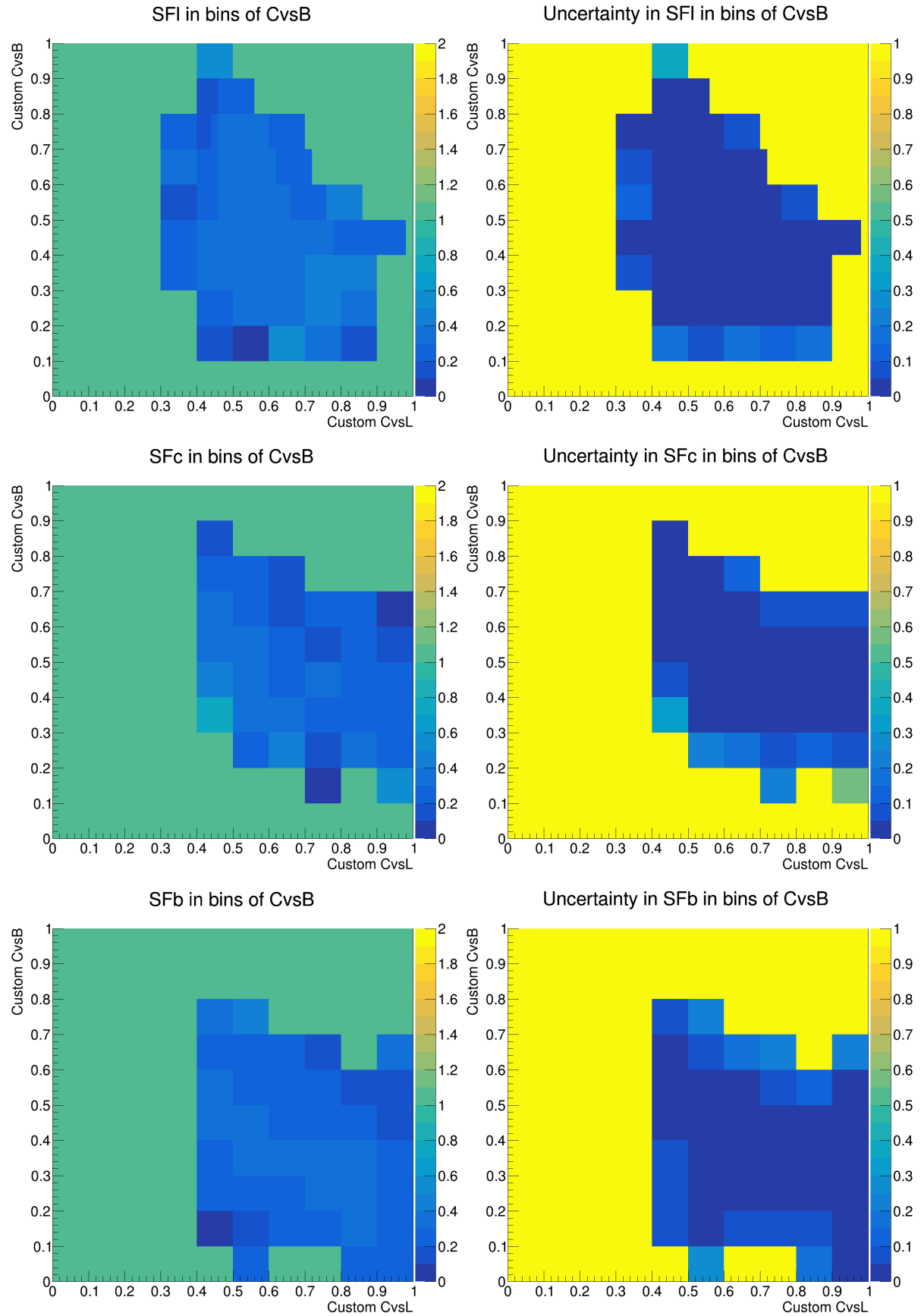
Figure A.20: CvsL / CvsB scale factors in bins of CvsB, for the basic classifier at epoch 200, evaluated on raw inputs. The scale factors are given in the left column, with corresponding uncertainties in the right column. The rows correspond to the different selections (l, c, b).
