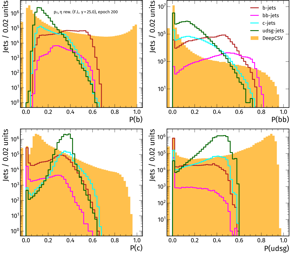
Figure 3.1: Tagger outputs, evaluating the basic training (split by flavour) and DeepCSV (summed) on test inputs. Each subfigure represents one output node of the model after 200 epochs.
