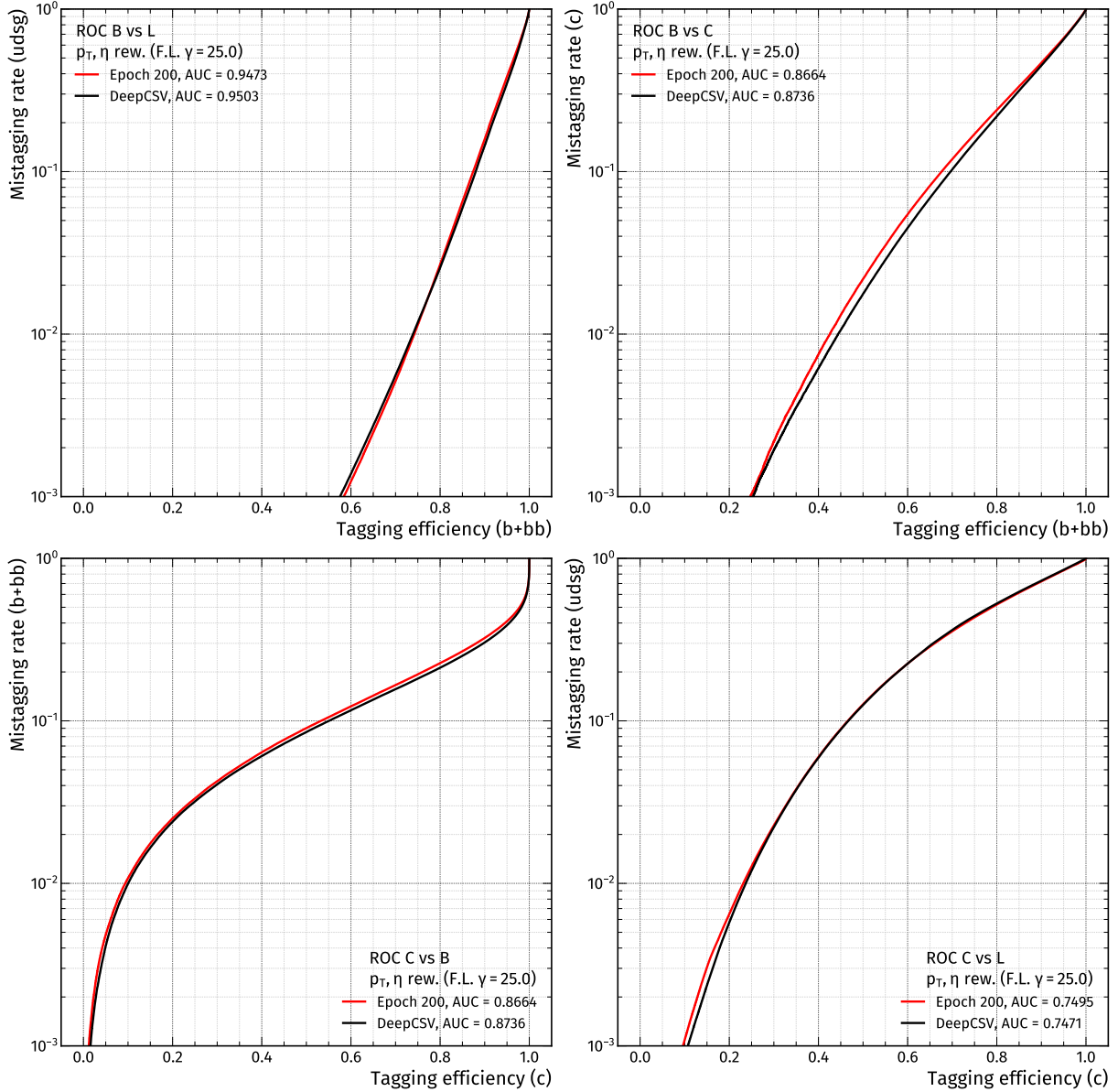
Figure 3.5: ROC curves for four different discriminators: BvsL, BvsC, CvsB and CvsL. The custom tagger is shown in red, the DeepCSV classifier is visualized with black lines.
