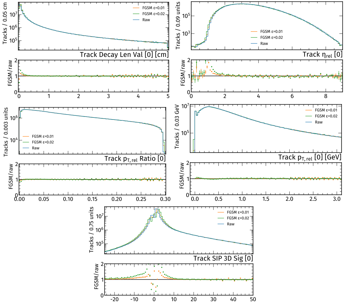
Figure A.10: Remaining first track variables with systematically distorted inputs. For the adversarial attacks, the parameters are either moderate ( \epsilon = 0.01 ) or rather large ( \epsilon = 0.02 ). The qualitative behaviour for the second to sixth track is similar and is not displayed here.
