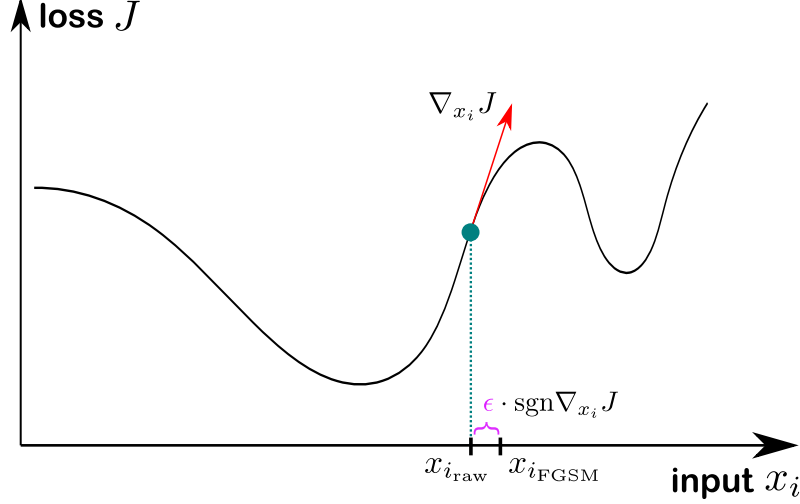
Figure 1.7: Visualization of the generation of adversarial inputs by applying the FGSM attack. The distorted inputs are created in such a way that the loss is maximized, as explained in the text. Only one input is shown, in the real application, the gradients are computed multidimensionally for all inputs, but each shift uses the same limiting parameter \epsilon .
