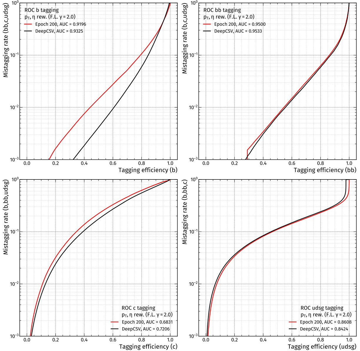
Figure A.5: ROC curves when discriminating each flavour (b, bb, c, udsg) against all other flavours, comparing the custom tagger with \gamma = 2 with DeepCSV. The custom tagger is shown in red, the DeepCSV classifier is visualized with black lines.
