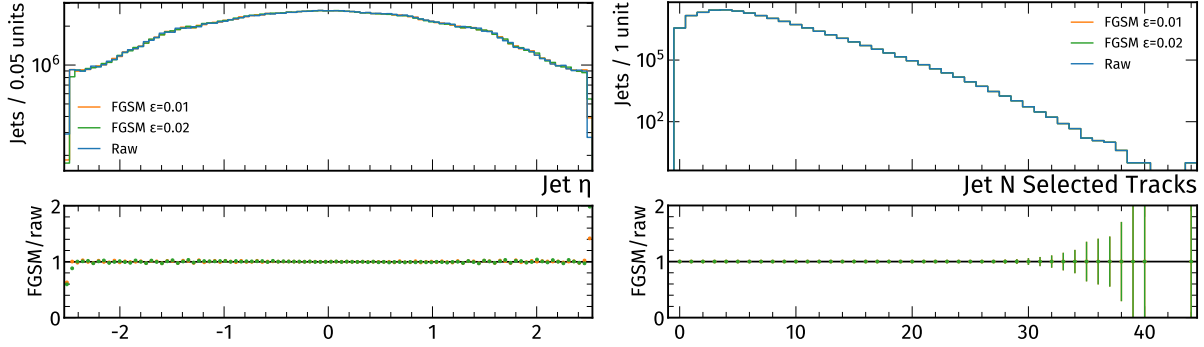
Figure 4.1: Distribution of raw and distorted inputs, for features where the impact of the adversarial attack is marginal or where the attack does not modify the distribution at all, by construction. The left figure shows the jet pseudorapidity with slight distortions, while the right figure demonstrates an example of an integer variable that is left unchanged. For the adversarial attacks, the parameters are either moderate ( \epsilon = 0.01 ) or rather large ( \epsilon = 0.02 ).
