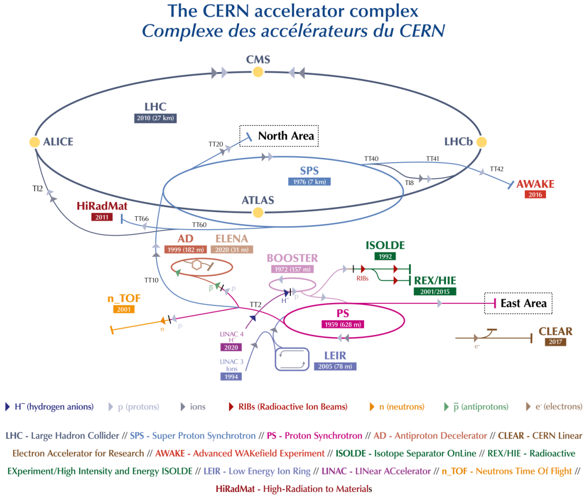
Figure 1.3: Sketch of the LHC and its experiments at the CERN accelerator complex [23].
