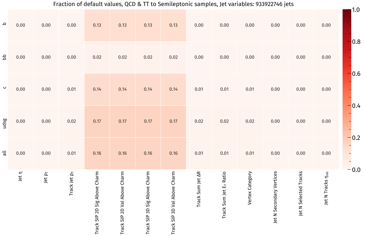
Figure 2.2: Fraction of default values for global jet variables, split by flavour or obtained from all available jets.
