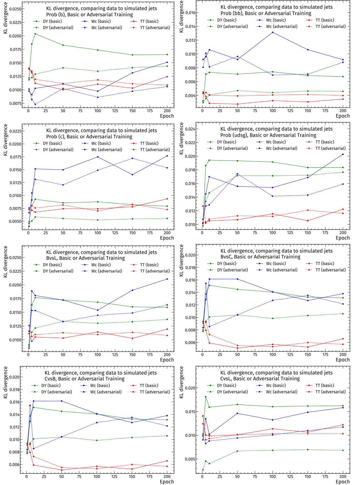
Figure A.22: KL divergences for tagger outputs and discriminators between data and simulation for a set of checkpoints of the basic training (solid lines) and adversarial training (dashed lines), split by selection. Every individual figure shows one output (b, bb, c, udsg) or discriminator (BvsL, BvsC, CvsB, CvsL) only, the colours indicate the selection (DY: green, W+c: blue, semileptonic t\bar{t} : red).
