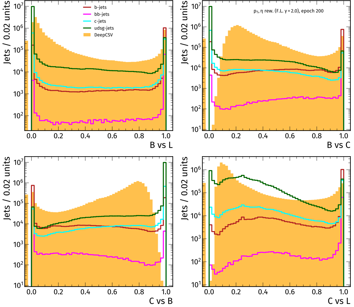
Figure A.4: Discriminators, evaluating the basic training with \gamma = 2 (split by flavour) and DeepCSV (stacked) on test inputs. Each subfigure represents one discriminator between two flavours (with category b and bb merged into "B").
