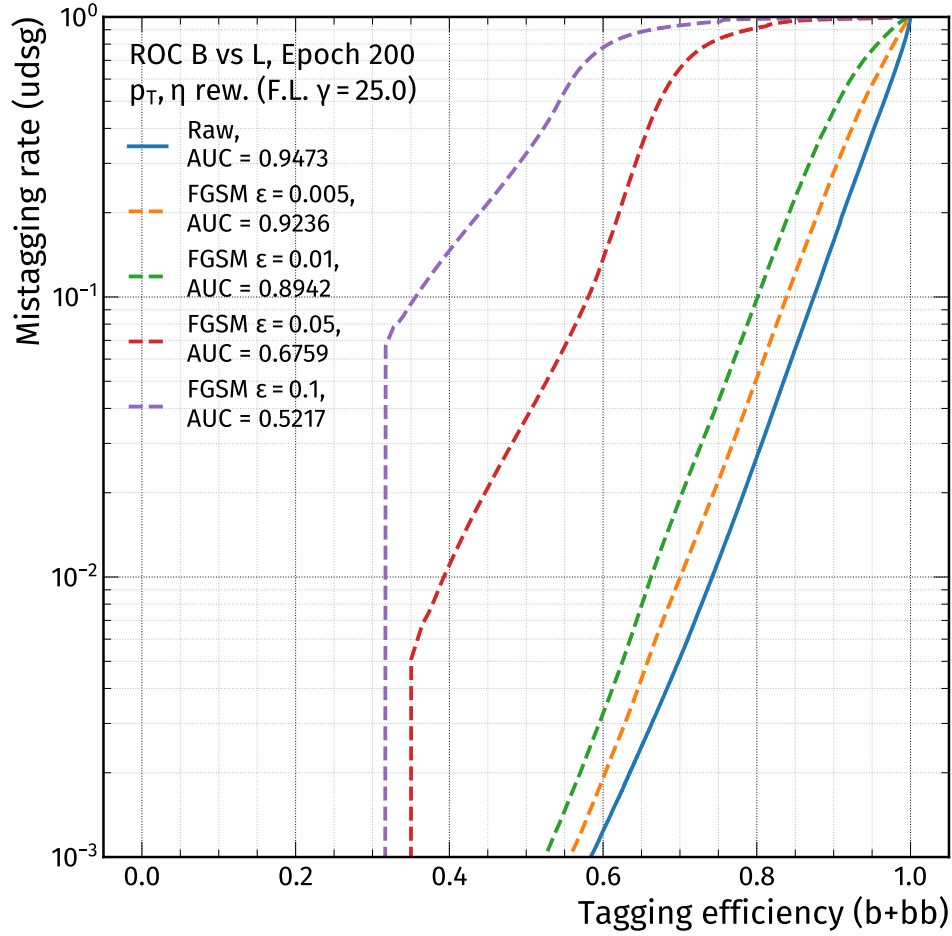
Figure 4.5: ROC curves for the BvsL discriminator, evaluated at epoch 200 with raw and adversarial inputs, using different parameters \epsilon for the FGSM attack on the baseline model.
