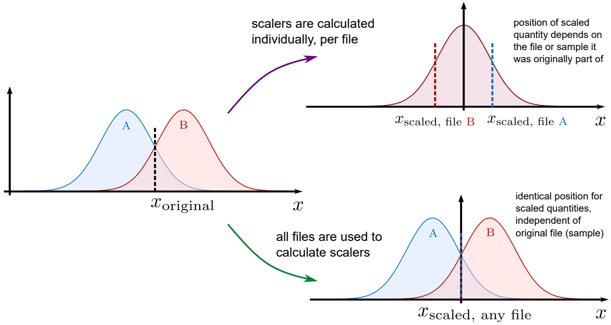
Figure 2.5: Visualization of two different approaches for the scaling of the input distributions. The first method calculates individual scalars per file, while the second takes all samples from all training files into account. Gaussian distribution adapted from Ref. [61].
