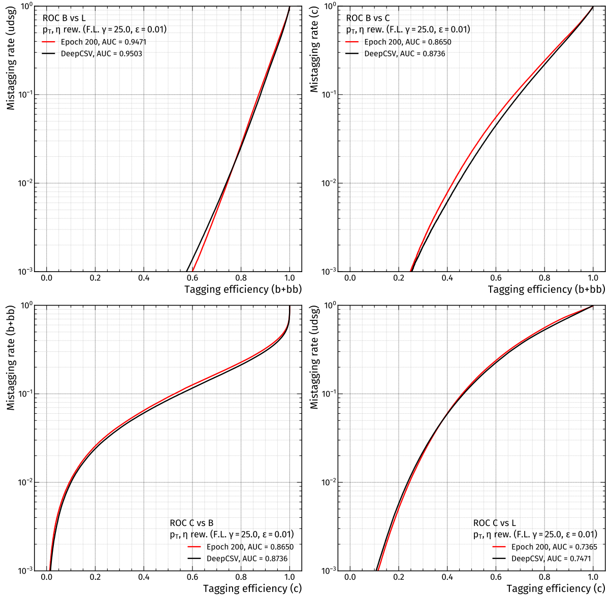
Figure A.15: ROC curves for the adversarial training with \gamma = 25 , for four different discriminators: BvsL, BvsC, CvsB and CvsL. The custom tagger is shown in red, the DeepCSV classifier is visualized with black lines.
