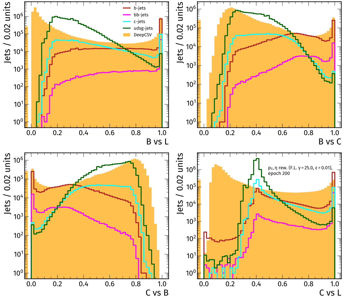
Figure A.13: Discriminators, evaluating the adversarial training with \gamma = 25 (split by flavour) and DeepCSV (stacked) on test inputs. Each subfigure represents one discriminator between two flavours (with category b and bb merged into “B”).
