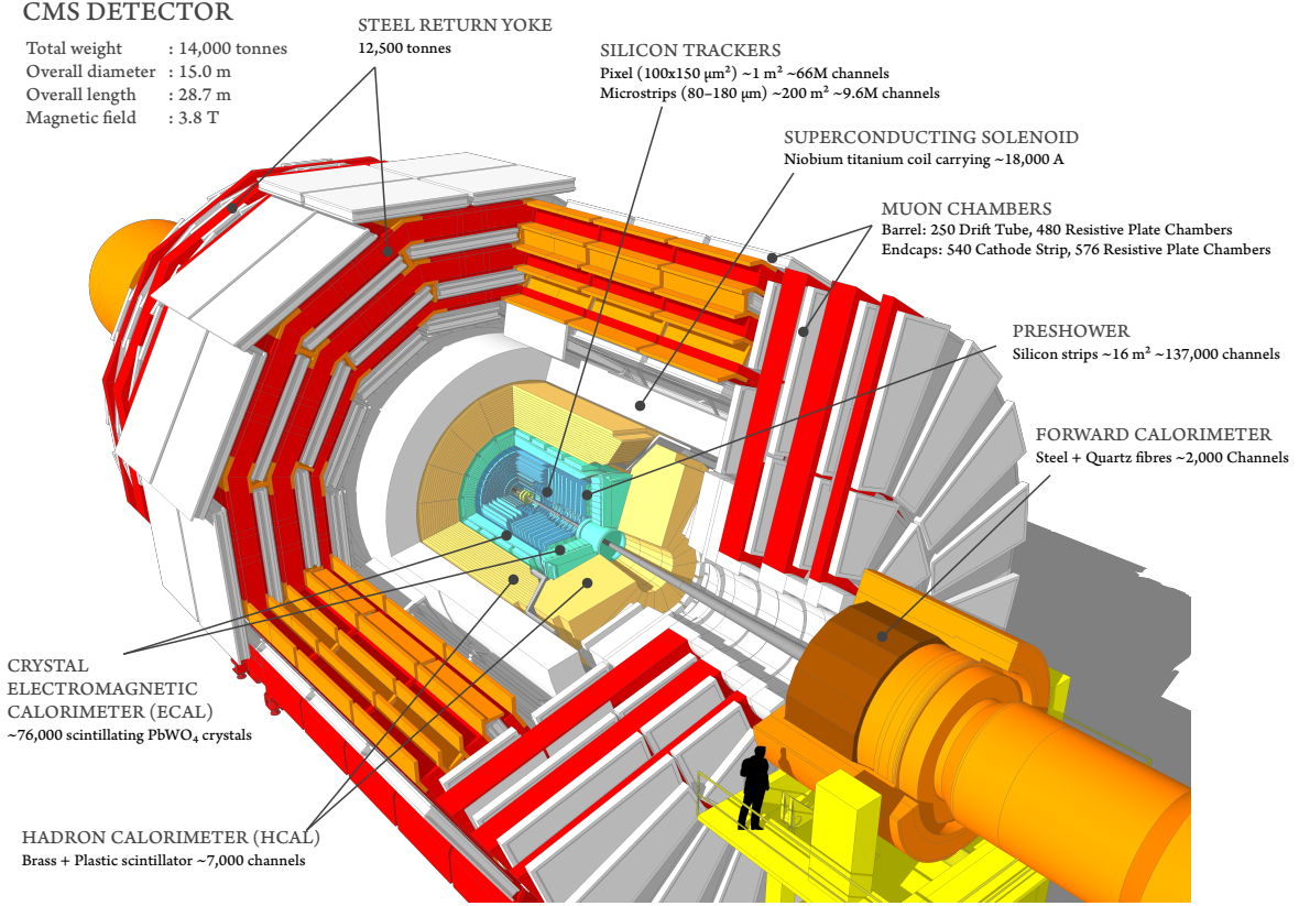
Figure 1.4: The CMS detector with its components, visualized with a 3D model [35]. The denoted dimensions differ slightly from the original configuration [24].
