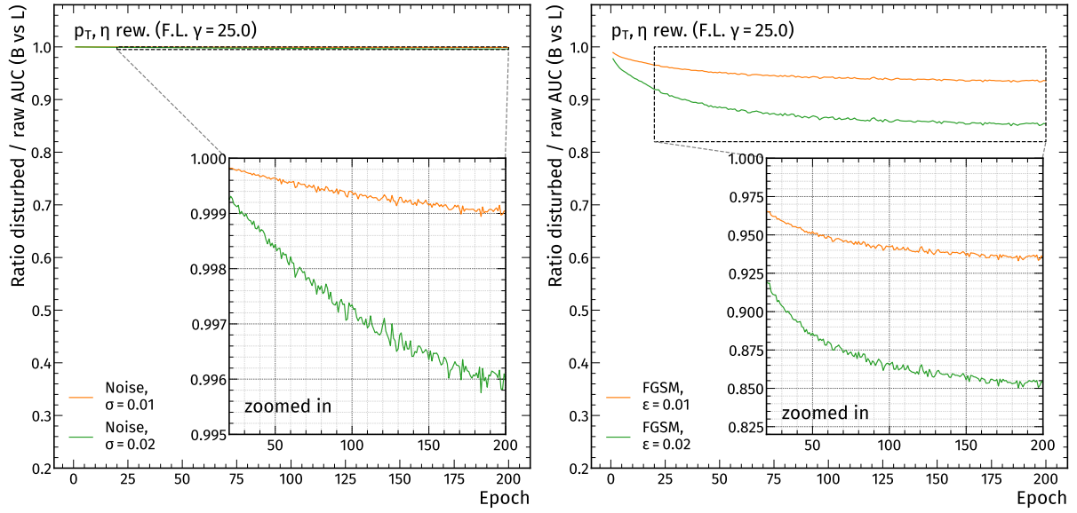
Figure 4.9: Evolution of the ratio between distorted and raw BvsL-AUC with the number of epochs for the basic training, evaluated on raw and distorted inputs (adding noise with \sigma = 0.01 and \sigma = 0.02 (left) or by using the FGSM attack with \epsilon = 0.01 and \epsilon = 0.02 (right)).
