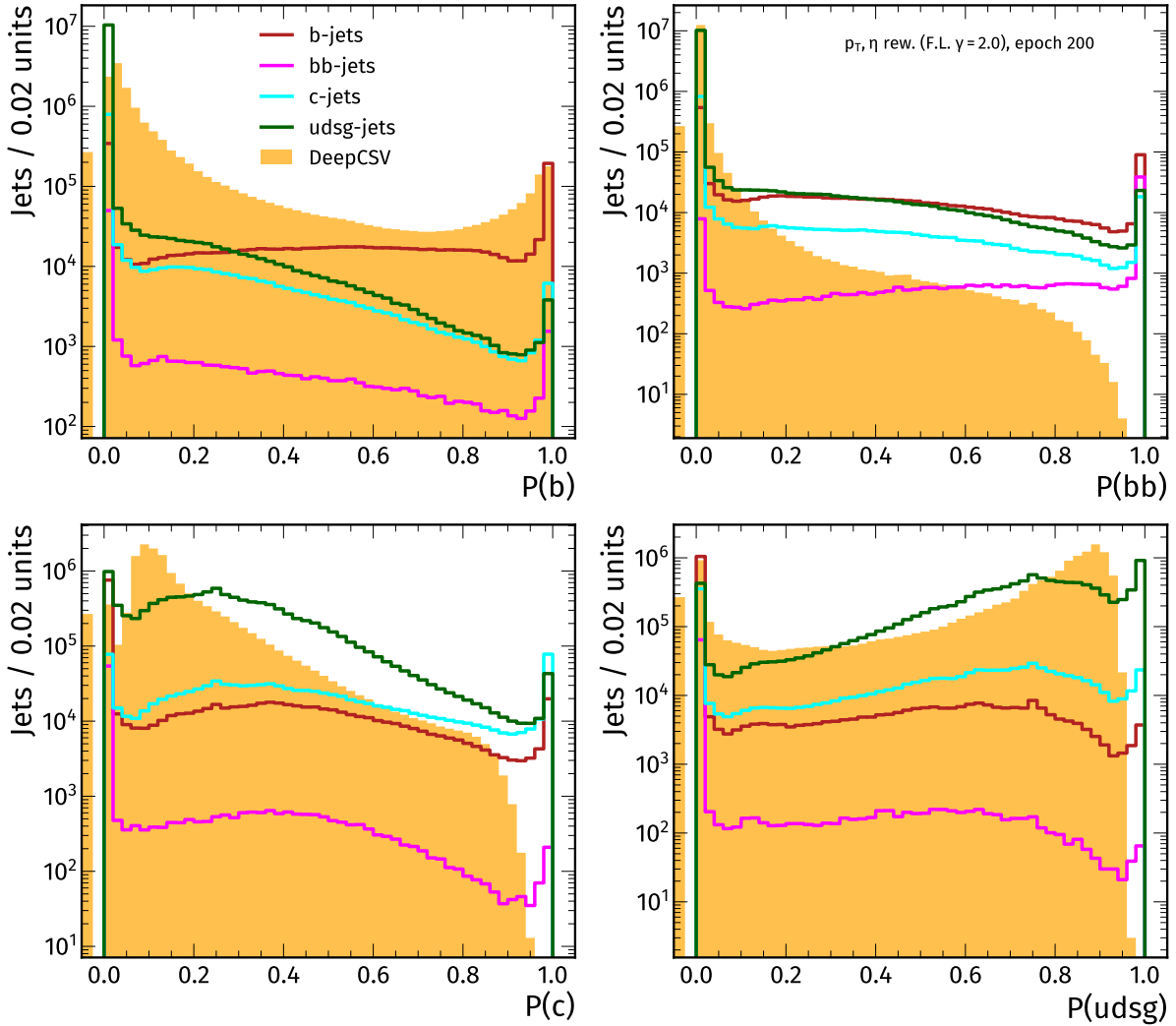
Figure A.3: Tagger outputs, evaluating the basic training with \gamma = 2 (split by flavour) and DeepCSV (stacked) on test inputs. Each subfigure represents one output node of the model.
