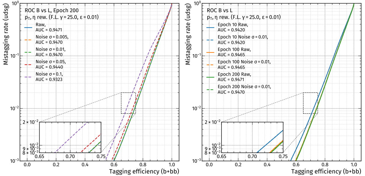
Figure A.16: ROC curves for the BvsL discriminator, evaluating the adversarially trained model with raw and randomly distorted inputs (Gaussian noise), either with a fixed epoch with different parameters \sigma , or with a fixed parameter \sigma , but evaluated at different checkpoints of the training. The left subfigure uses epoch 200, different colours represent different magnitudes of the distortion. On the right, a fixed parameter \sigma = 0.01 (dashed lines) is utilized in comparison with raw inputs (solid lines), for different epochs in different colours.
