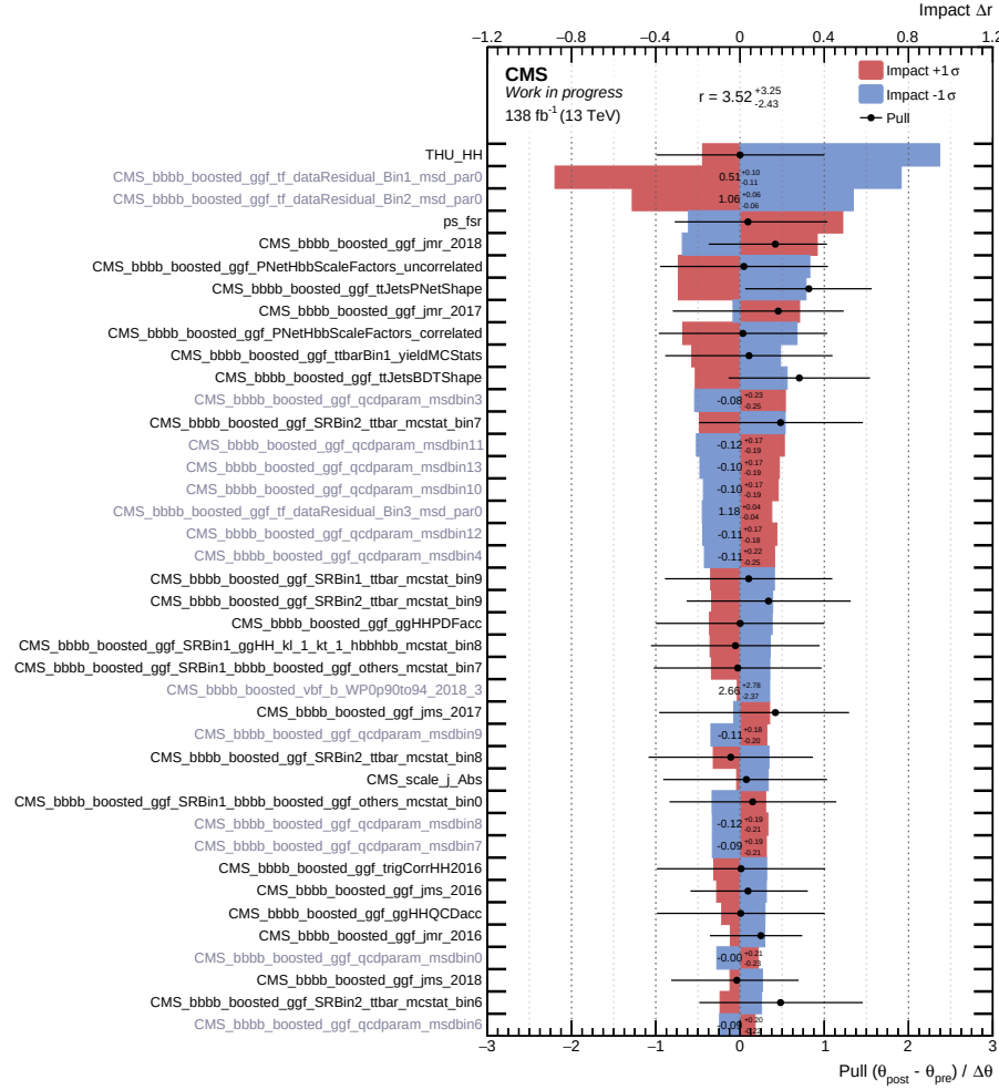
Figure 6.51: Pulls and impacts of the first 40 nuisance parameters ranked by impact.
