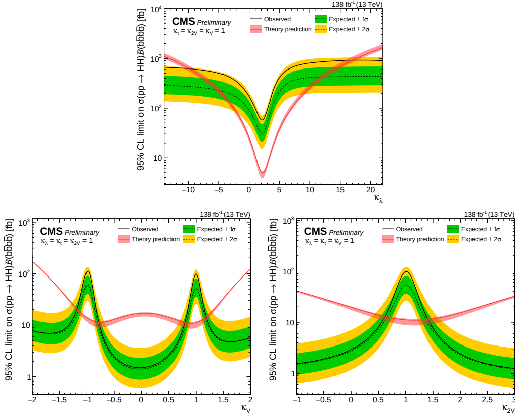
Figure 6.55: 1D upper limits on the inclusive HH cross section as a function of \kappa_\lambda (top), \kappa_V (bottom left), and \kappa_{2V} (bottom right) for the combined ggF and VBF channels.
