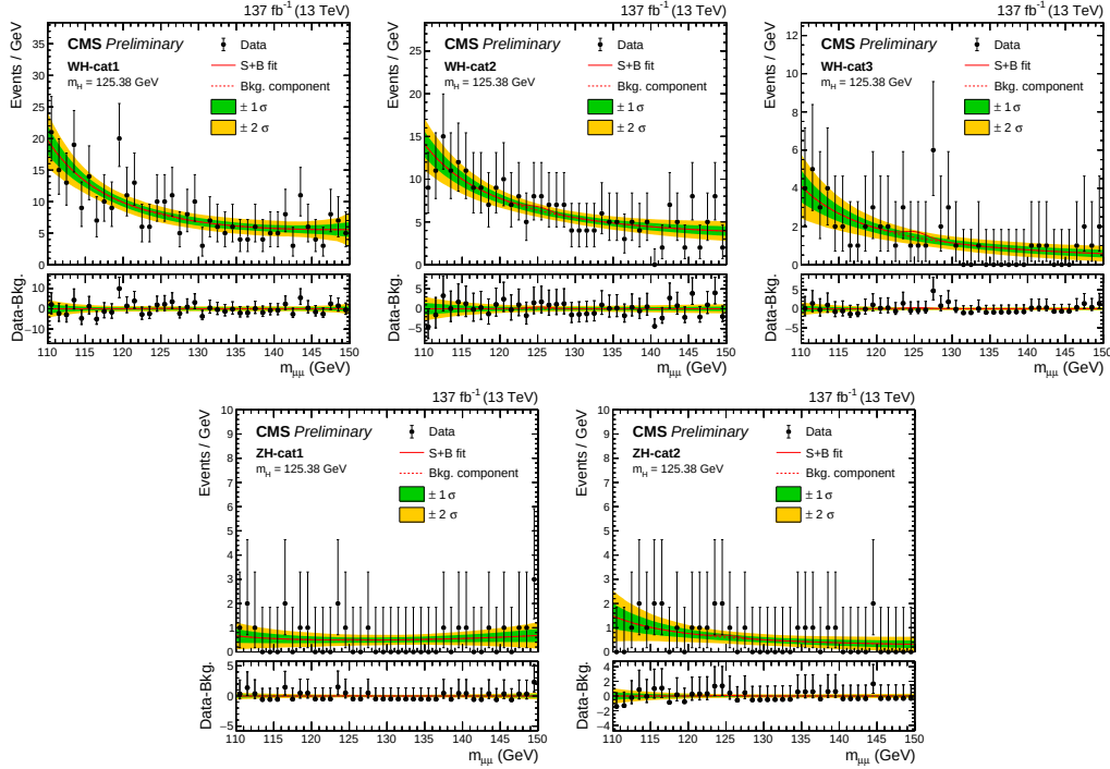
Figure 5.37: Comparison between the observed data and the total background extracted from a signal-plus-background fit performed across WH (first row) and ZH (second row) event categories. First row, from left to right: WH -cat1, WH -cat2, and WH -cat3. Second row, from left to right: ZH -cat1 and ZH -cat2. The one (green) and two (yellow) standard deviation bands include the uncertainties in the background component of the fit. The lower panel shows the residuals after the background subtraction, where the red line indicates the signal with m_H = 125.38 GeV extracted from the fit.
