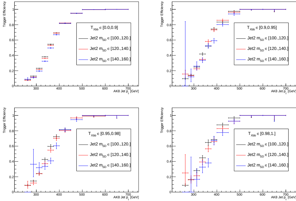
Figure 6.34: The trigger efficiency for the 2016 dataset is measured as a function of the AK8 jet p_T in four bins of the T_{Xbb} score: 0.0–0.90 (top left), 0.90–0.95 (top right), 0.95–0.98 (bottom left), 0.98–1.00 (bottom right). The different colors represent different ranges of jet m_{SD} .
