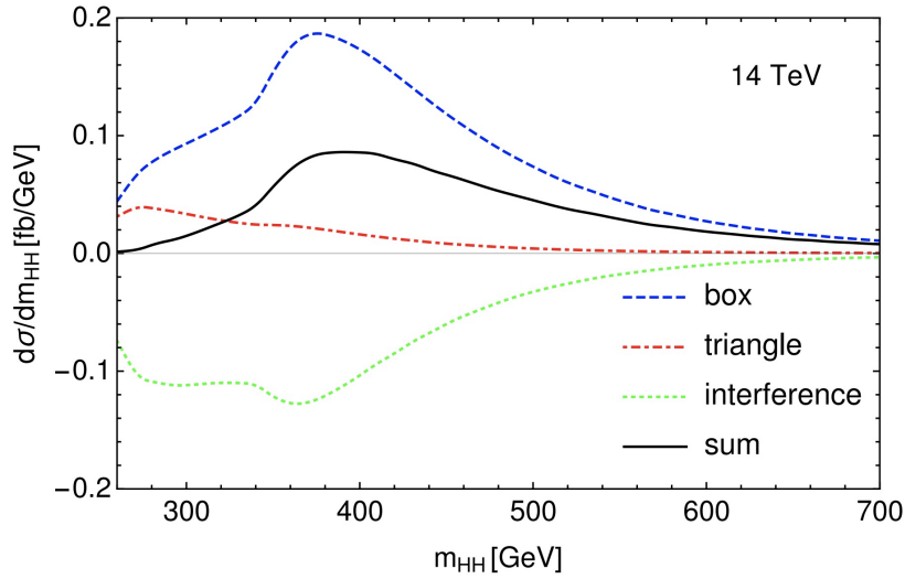
Figure 6.1: In the SM, the box (blue dashed line) and triangle diagram (red dashed line) for the ggHH process interfere destructively. The dependence of the interference term as a function of m_{HH} is shown with the green dashed line. This results in a smaller overall cross-section for the ggHH process, as shown by the black solid line [174].
