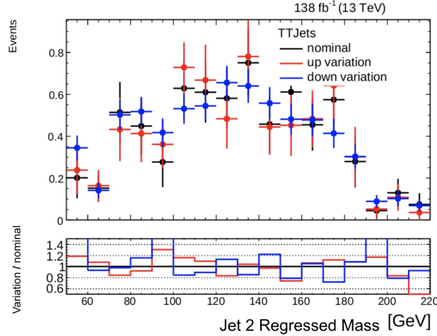
Figure 6.40: Uncertainty on the Jet 2 regressed mass shape in event category 1 for the t\bar{t} process due to different T_{Xbb} score selections. The nominal shape is obtained after imposing a requirement of T_{Xbb} > 0.9 , and the up and down variations are obtained by requiring T_{Xbb} > 0.92 and T_{Xbb} > 0.2 , respectively.
