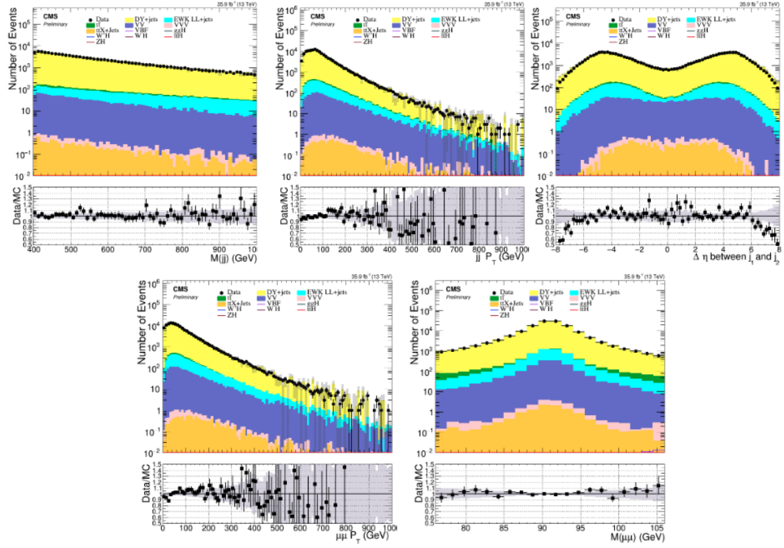
Figure 5.14: Data/MC comparisons for some of the VBF discriminating variables in 2016. (Top) m(jj) (left), p_T(jj) (center) and \eta(jj) (right). (Bottom) p_T(\mu\mu) (left) and M(\mu\mu) (right).
