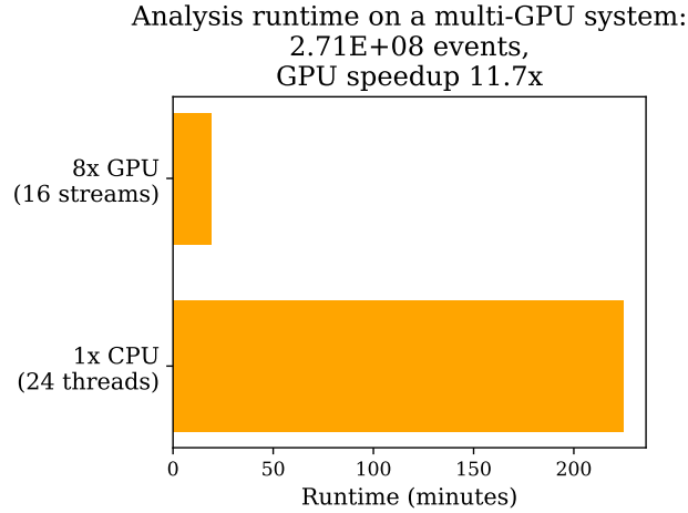
Figure D.2: Benchmarks of the full analysis with 270M events, 100GB of numerical data on a multi-GPU system. We find that by using 8x nVidia GTX 1080 GPUs, 2 compute streams per device, we can reduce the analysis runtime by a factor of 12x, compared to using multiple threads on the CPU alone.
