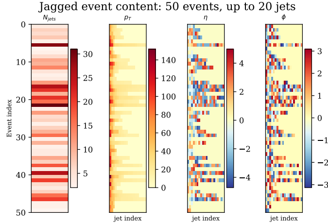
Figure D.1: A visual representation of the jagged data structure of the jet p_T , \eta and \phi content in 50 simulated events. On the leftmost figure, we show the number of jets per event, one event per row, derived from the offset array. In the three rightmost columns, we show the jet content in events, visualizing the p_T , \eta and \phi of the first 20 jets for each event.
