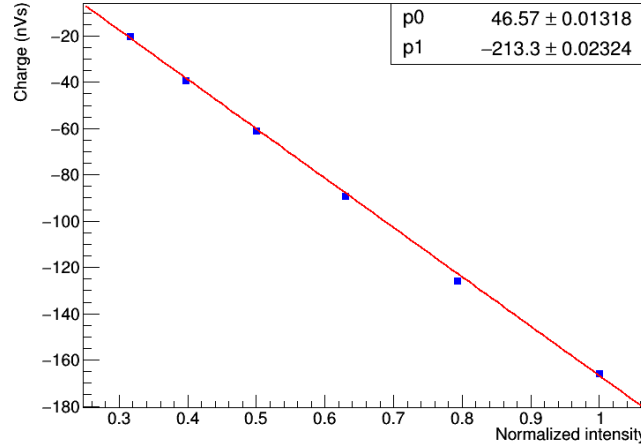
Figure 4.13: The charge deposited in a SiPM scales linearly with the intensity of the laser light.
