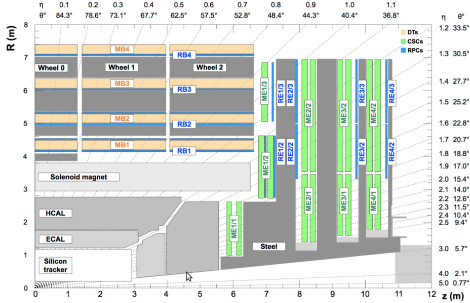
Figure 3.11: A schematic view of one quadrant of the CMS muon chamber. DTs are shown in orange and labeled as MB1/2/3/4; CSCs are shown in green and labeled as ME n /m, where n is the index in the z direction and m is the index in the r direction; RPCs are shown in blue and labeled as RB1/2/3/4 for barrel RPCs and RE n /m for the endcaps. [81].
