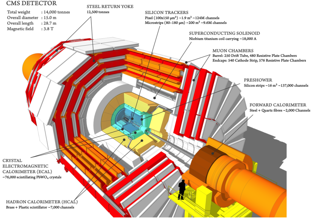
Figure 3.4: A cutaway diagram of the CMS experiment, indicating its various subsystems [67].
