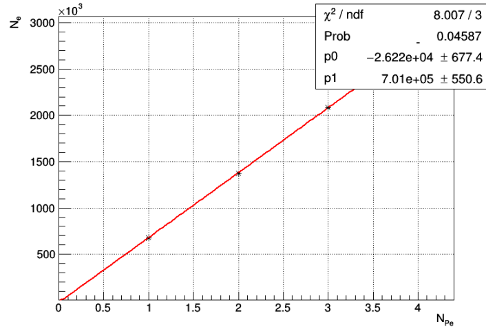
Figure 4.12: The number of electrons plotted against the number of photoelectrons.
