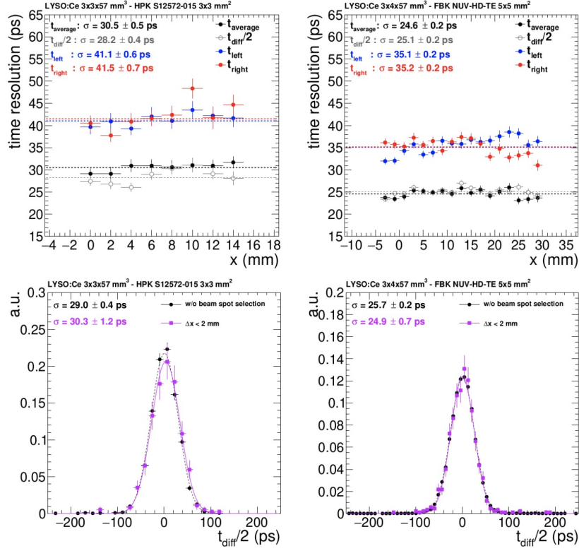
Figure 4.18: Time resolution measurements from the Fermilab April 2019 test beam. (Top) Time resolution of the left and right SiPMs, their average, and half of the time difference as a function of the MIP impact point for a 3 \times 3 \times 57 \text{ mm}^3 LYSO:Ce bar coupled to HPK SiPMs (left) and for a 3 \times 4 \times 57 \text{ mm}^3 LYSO:Ce bar coupled to FBK SiPMs (right). (Bottom) Global and local time resolution for a 3 \times 3 \times 57 \text{ mm}^3 LYSO:Ce bar coupled to HPK SiPMs (left) and for a 3 \times 4 \times 57 \text{ mm}^3 LYSO:Ce bar coupled to FBK SiPMs (right).
