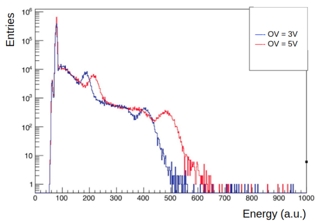
Figure B.10: The energy spectrum recorded in one of the BTL module channels connected to the T2TB tester board. The spectrum shifts to the right when increasing the SiPM over voltage.
