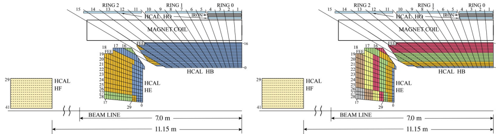
Figure 3.8: The depth segmentation in the previous (left) and upgraded (right) HCAL detector. A depth is a collection of scintillator layers (columns) depicted with the same color, per \Delta\eta division. Light from the different layers in the same depth and \Delta\eta division are optically added together before reaching the photosensors [75].
