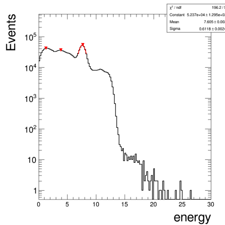
Figure B.3: The energy spectrum of channel 32 and the fit of the 511 keV peak.
