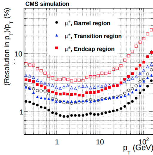
Figure 5.2: Resolution, as a function of p_T , for single, isolated muons in the barrel ( |\eta| < 0.9 ), transition ( 0.9 < |\eta| < 1.4 ), and endcap regions ( 1.4 < |\eta| < 2.5 ). For each bin, the solid (open) symbols correspond to the half-width for 68% (90%) intervals of the residuals distribution [89].
