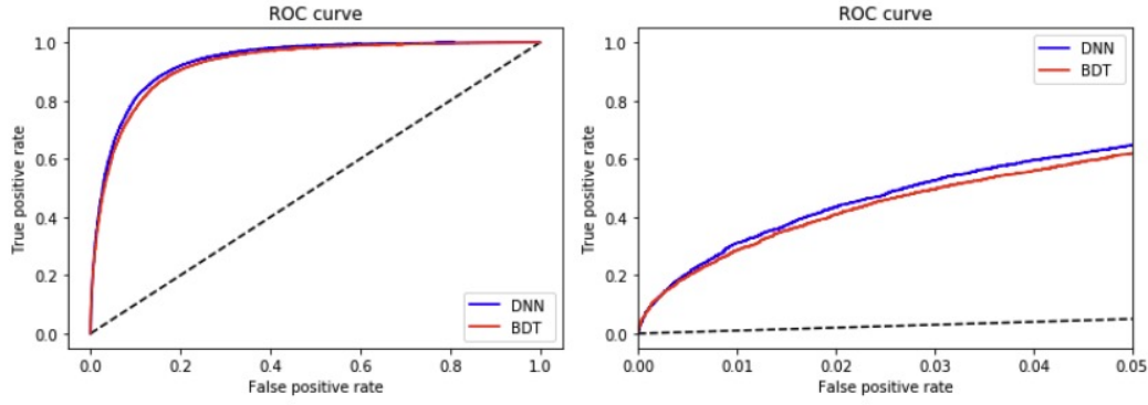
Figure 5.17: BDT vs DNN performance. (Left) A ROC curve comparison of the performances of the preliminary BDT and DNN. (Right) A zoomed in version of the ROC curve. The DNN performs slightly better than the BDT.
