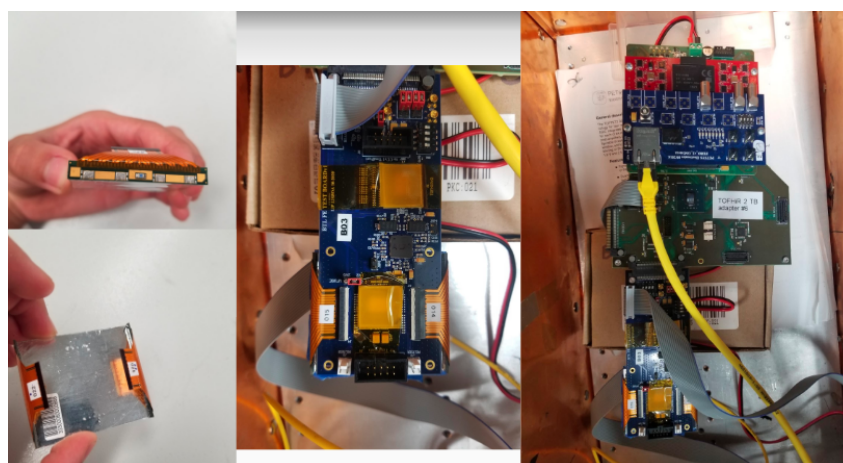
Figure B.9: The experimental setup with the TOFHIR2A.
