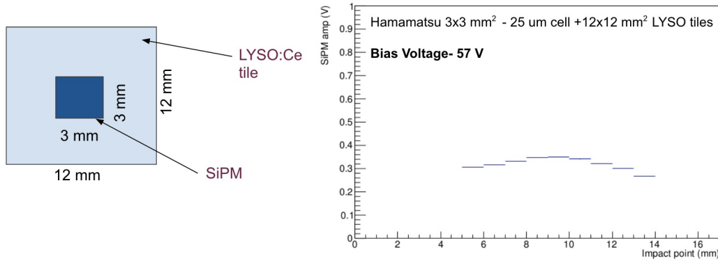
Figure 4.7: Impact point studies with a laser. (Left) A schematic of a 3 \times 3 \text{ mm}^2 SiPM coupled with a 12 \times 12 \times 4 \text{ mm}^3 LYSO tile using optical grease. (Right) Amplitude recorded as a function of the MIP impact position on the SiPM +LYSO tile configuration.
