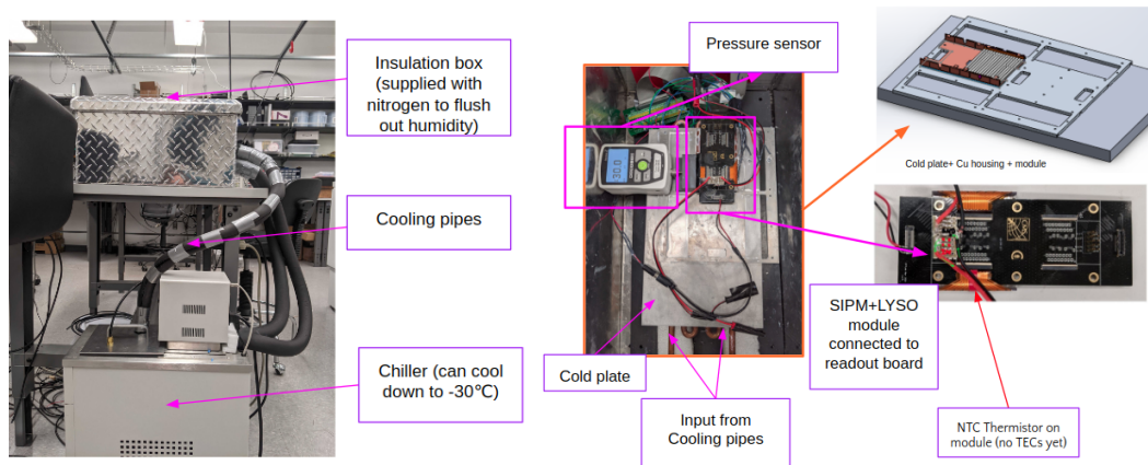
Figure 4.20: Mock cooling setup at the CPT Lab. (Left) The Aluminium box connected to the Isotemp cooler using insulated pipes. (Right) The inside of the Aluminium box consists of a BTL module connected to a tester readout board and placed inside a Copper housing.
