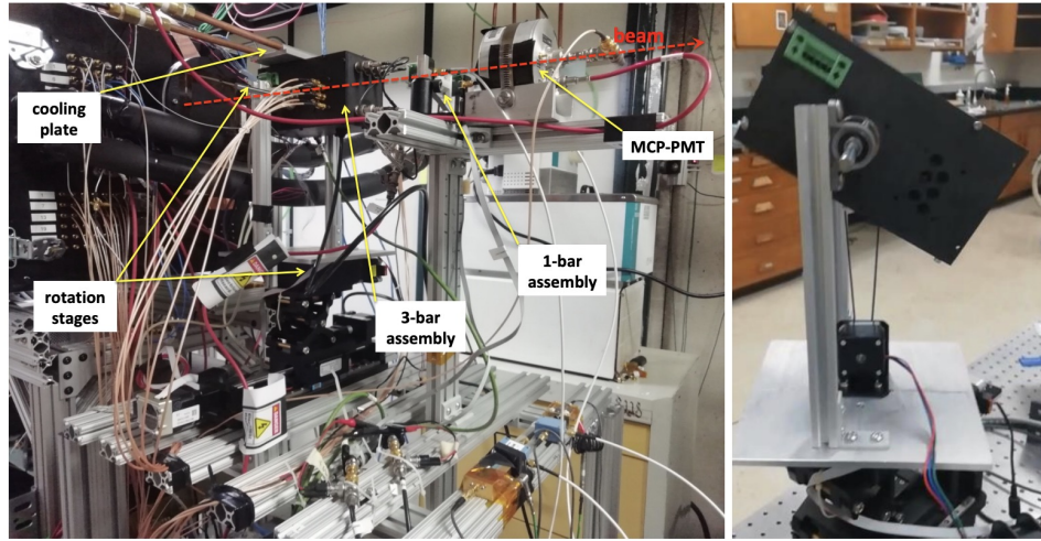
Figure 4.16: Fermilab April 2019 test beam. (Left) The experimental setup at FTBF. (Right) The box and mechanical structure capable of rotating the 3-bar assembly.
