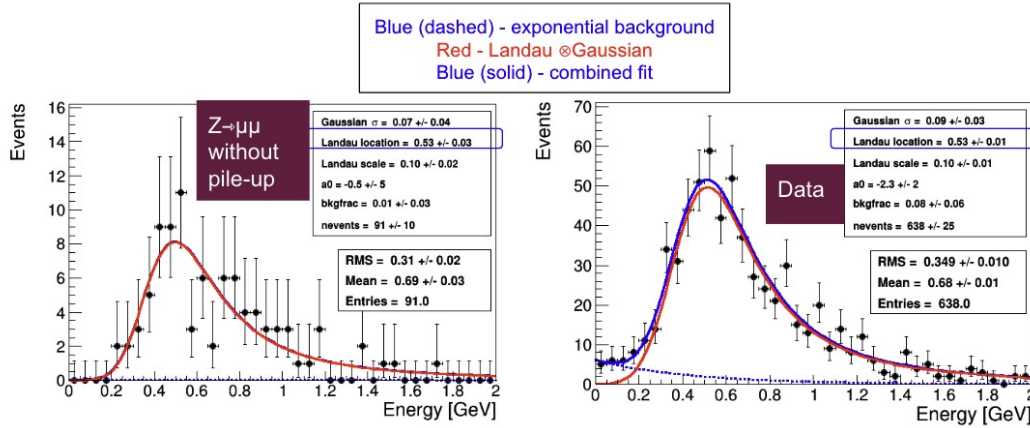
Figure A.4: Comparison of deposited energy profiles in Depth 6 for |i\eta| = 25 (for both HE detectors combined), in events with a real reconstructed second muon in that i\eta tower. The left distribution is for Z \rightarrow \mu\mu MC (no pileup) simulation events and the right distribution is data. The signal is modeled using a convolution of Gaussian and Landau distributions (in red), while the background is modeled by an exponential function (dashed blue). The combined signal + background fit is shown in solid blue. The most probable value of deposited energy is similar in both the simulation and data.
