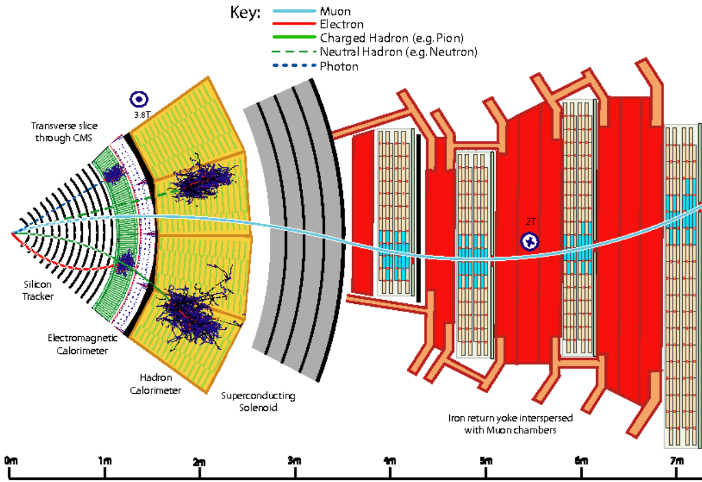
Figure 3.12: A transverse slice of the CMS detector indicating the different signatures left by various particles in the sub-systems [87].
