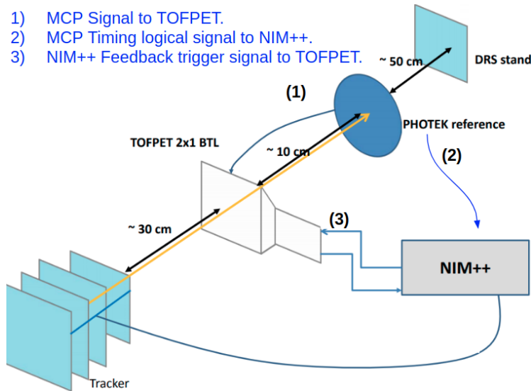
Figure B.6: The DAQ at the Fermilab December 2017 test beam.
