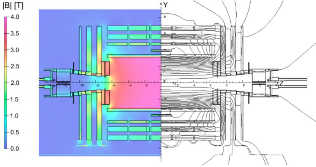
Figure 3.9: The magnetic field and field lines inside the CMS detector volume [78].
