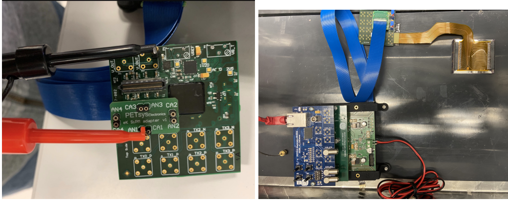
Figure B.2: The readout test setup. (Left) The SiPM adapter board. (Right) The TOFPET FEB/D is connected to the LYSO bar + SiPM array through an adapter board.
