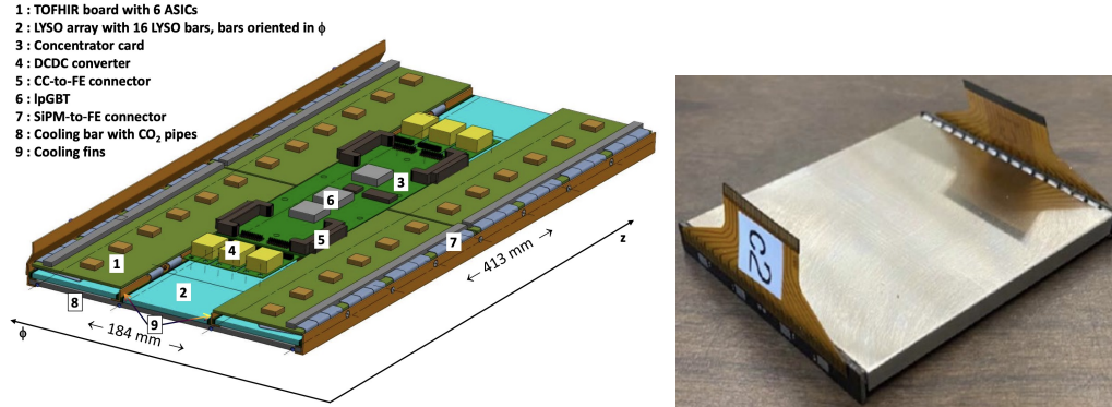
Figure 4.6: Various BTL components. (Left) A BTL Readout unit, consisting of 24 BTL modules of LYSO:Ce bars + SiPMs. Each RU has a total of 768 SiPMs. (Right) A BTL module consisting of 16 LYSO:Ce bars + 32 SiPMs. The module is connected to the FE boards using flex cables, as can be seen in the figure.
