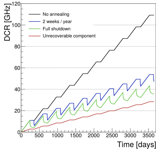
Figure 4.5: Expected growth of DCR for various annealing scenarios at fixed OV of 1.5 V during the detector lifetime [92].
