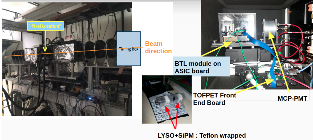
Figure B.5: The experimental setup at the Fermilab December 2017 test beam.
