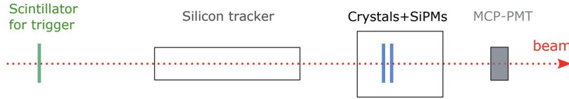
Figure 4.15: The test beam setup at Fermilab. From left to right, the scintillator is used for trigger, the silicon tracker defines the MIP impact position in the x-y plane, and the MCP-PMT is used to provide a reference time. The LYSO+SiPMs test setups, one for the 1-bar and the other for the 3-bar array, are positioned along the beamline. The beam direction is the z-axis.
