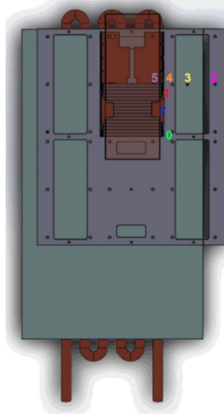
Figure 4.21: A SOLIDWORKS simulation of the cold plate setup. This simulation was performed by Caltech SURF student Esme Knabe in Summer 2021 [108]. Colored numbers indicate the position of the thermistors.
