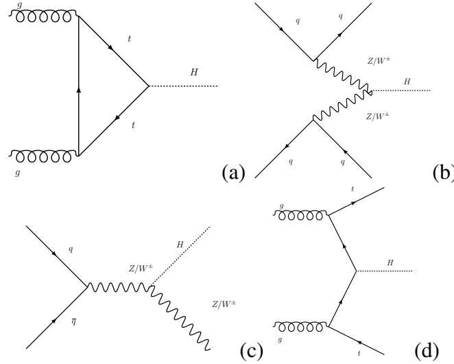
Figure 2.3: Different production modes for the Higgs boson at the LHC : (a) ggH, (b) VBF, (c) VH, and (d) ttH.
