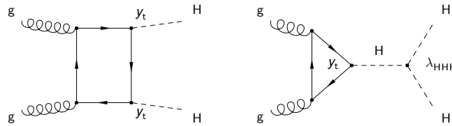
Figure 2.4: Feynman diagrams that contribute to ggHH at leading order. The left and right diagrams correspond to SM processes, referred to as the box and triangle diagrams, respectively.
