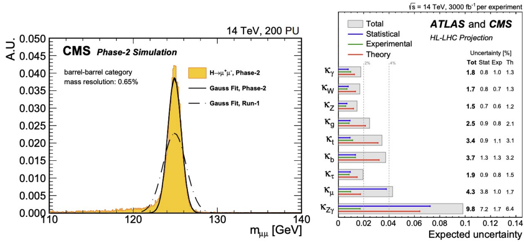
Figure 5.45: HL-LHC projection for H \rightarrow \mu\mu channel. (Left) The di-muon invariant mass distribution for H \rightarrow \mu\mu decays for muons in the central region, simulated with the Phase-2 CMS detector [170]. (Right) Summary plot showing the total expected \pm 1\sigma uncertainties on the coupling modifier parameters from the combination of ATLAS and CMS measurements at the HL-LHC. For each measurement, the total uncertainty is indicated by a grey box while the statistical, experimental and theory uncertainties are indicated by a blue, green and red line, respectively. \kappa_\mu is expected to be measured with a total uncertainty of 4% [173].
