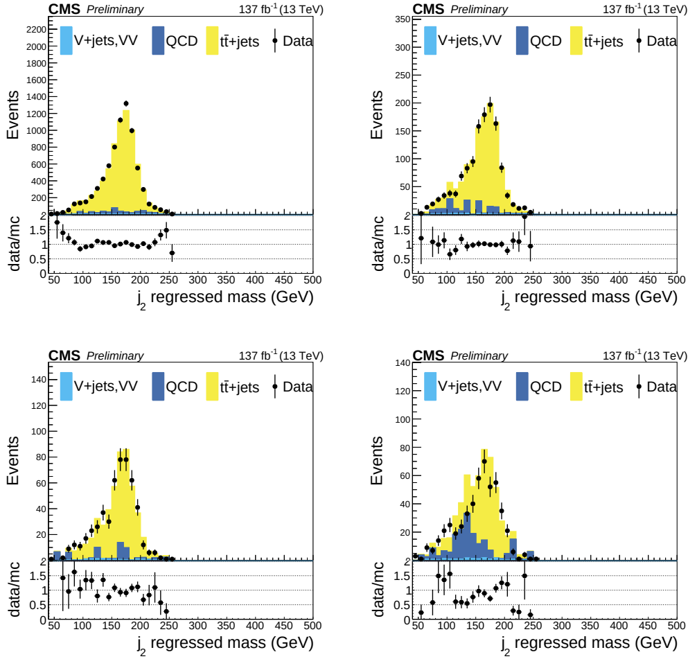
Figure 6.27: The top mass in different BDT bins (BDT range of top left: 0 - 0.00008; top right: 0.00008 - 0.0002; bottom left: 0.0002 - 0.0004; bottom right: 0.0004 - 1.0) for the full Run2 dataset. Here, the top recoil correction and the T_{Xbb} shape correction are already applied.
