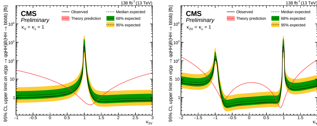
Figure 6.50: (Left): Observed (solid line) and expected (dashed line) 95% CL exclusion limits on \sigma(pp \rightarrow qqHH) \times \mathcal{B}(HH \rightarrow b\bar{b}b\bar{b}) , as a function of the \kappa_{2V} coupling, with other couplings fixed to the SM values. (Right): Observed (solid line) and expected (dashed line) 95% CL exclusion limits on \sigma(pp \rightarrow qqHH) \times \mathcal{B}(HH \rightarrow b\bar{b}b\bar{b}) , as a function of the \kappa_V coupling, with other couplings fixed to the SM values.
