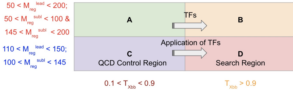
Figure 6.48: The ABCD method used for QCD background estimation in the VBF analysis.
