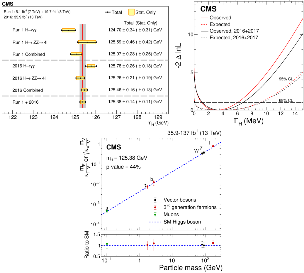
Figure 2.7: Various Higgs measurements from CMS: (Top left) Summary of the measured Higgs boson mass in the H \rightarrow \gamma\gamma and H \rightarrow ZZ^* \rightarrow 4l decay channels, and their combination [39]. (Top right) Likelihood scan of the Higgs decay width [53]. (Bottom) Coupling strengths of various SM particles to the Higgs boson as a function of the particle mass. The bottom panel compares the observed values with the prediction of SM [24].
