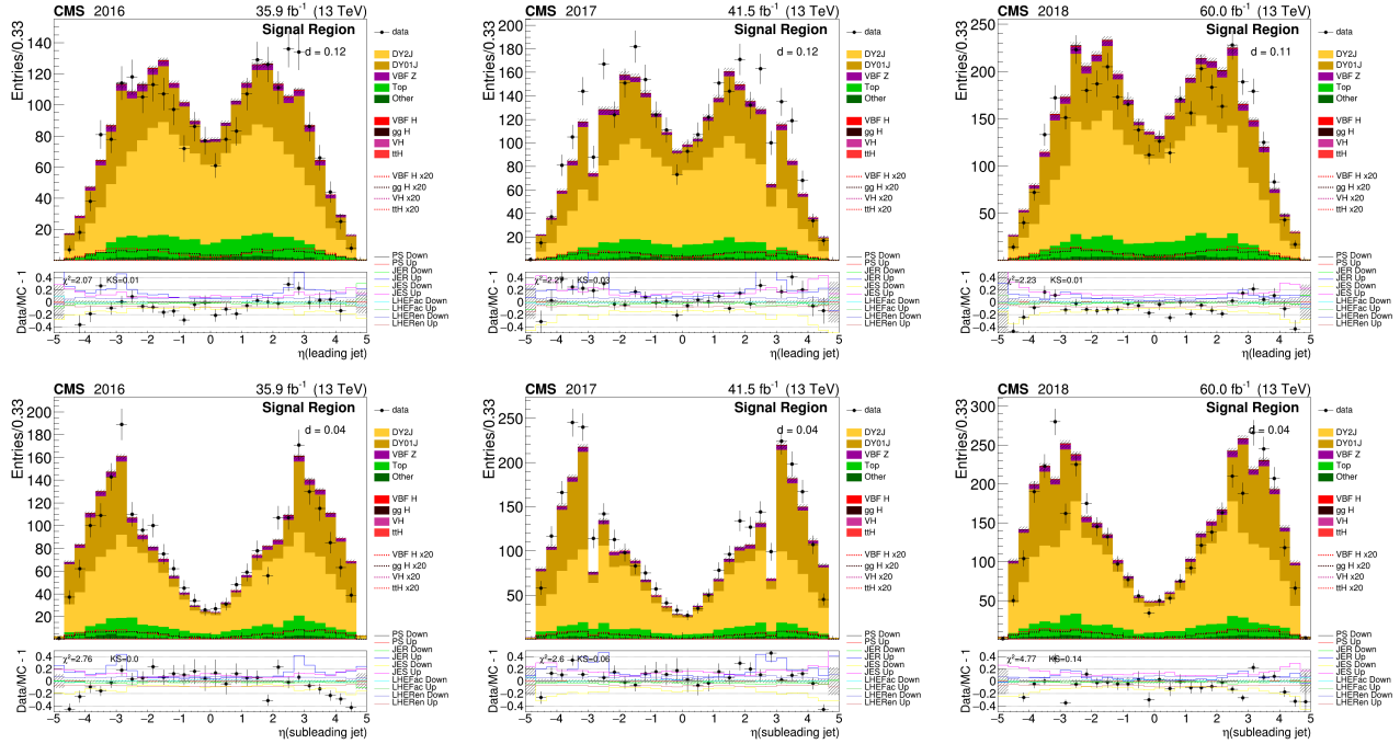
Figure 5.22: Pseudorapidity distributions for leading (top) and subleading (bottom) jets after the event selection in the Signal Region for 2016 (left), 2017 (center), and 2018 (right) [150].
