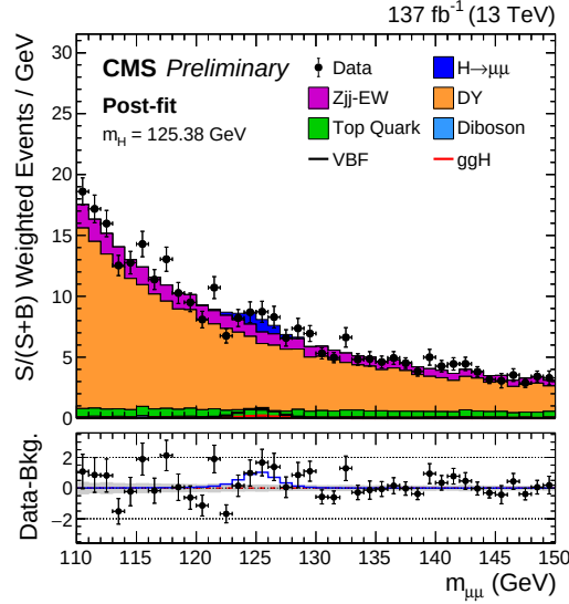
Figure 5.33: The m_{\mu\mu} distribution for the weighted combination of VBF-SB and VBF-SR events. Each event is weighted proportionally to the S/(S+B) ratio, calculated as a function of the mass-decorrelated DNN output. The lower panel shows the residuals after subtracting the background prediction from the signal-plus-background fit. The best-fit H \rightarrow \mu\mu signal contribution is indicated by the blue line, and the grey band indicates the total background uncertainty from the background-only fit.
