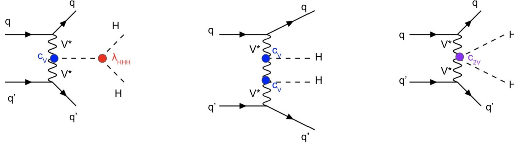
Figure 2.5: Feynman diagrams that contribute to qqHH at leading order. The qqHH process is sensitive to c_V and the c_{2V} couplings.
