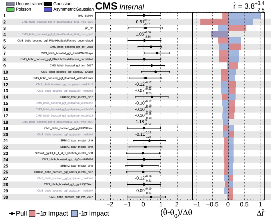
Figure 6.42: The impact pulls of top-ranked systematic uncertainties. The dominant sources of uncertainty are the QCD multi-jet modelling, the t\bar{t} background modelling, the ggHH signal modelling and the jet energy and mass scale and resolution.
