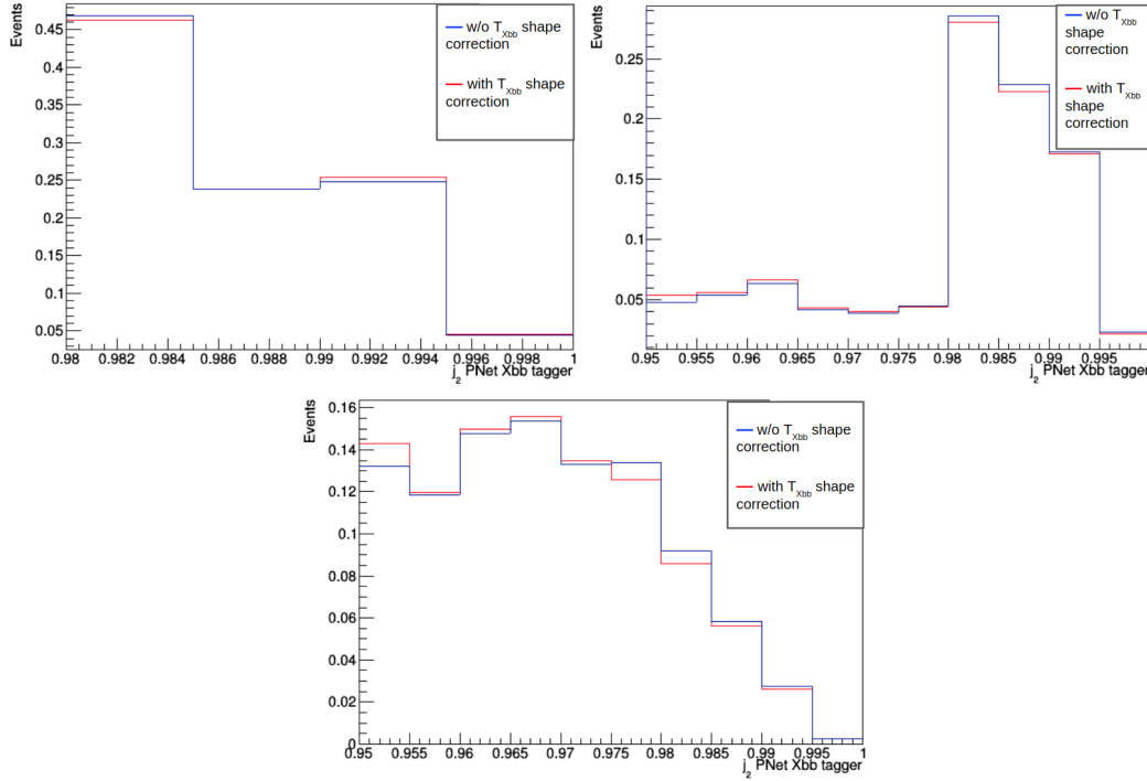
Figure 6.18: The distribution of the second jet T_{Xbb} score in the signal region for the t\bar{t} background, for event category 1 (top left), category 2 (top right), and category 3 (bottom). The histograms are normalized to unit area.
