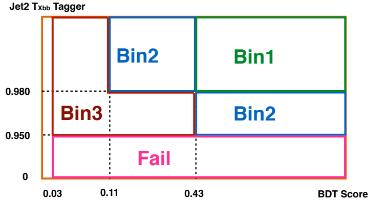
Figure 6.14: The event categories in the ggHH analysis are visually represented in a 2D grid of the BDT score and the jet 2 T_{Xbb} score.
