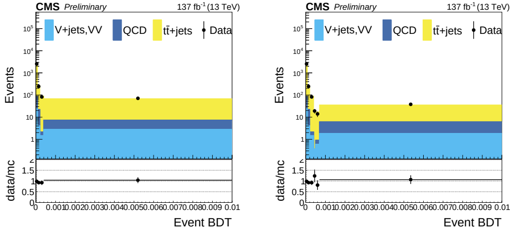
Figure 6.30: The event BDT distribution in the t\bar{t} all-hadronic control region is shown for the data and simulation prediction, for the full Run2 dataset. The binning edges are [0.000-0.00008], [0.00008-0.0002], [0.0002-0.0004], [ >0.0004 ] for the left plot, and [0.000-0.00008], [0.00008-0.0002], [0.0002-0.0004], [0.0004-0.0005], [0.0005-0.0007], [ >0.0007 ] for the right plot. The left plot is used to derive uncertainties for the BDT shape modeling in the t\bar{t} simulation.
