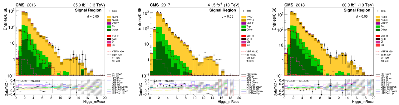
Figure 5.20: Dimuon mass uncertainty \Delta m_{\mu\mu} after the event selection in the Signal Region for 2016 (left), 2017 (center), and 2018 (right) [150].
