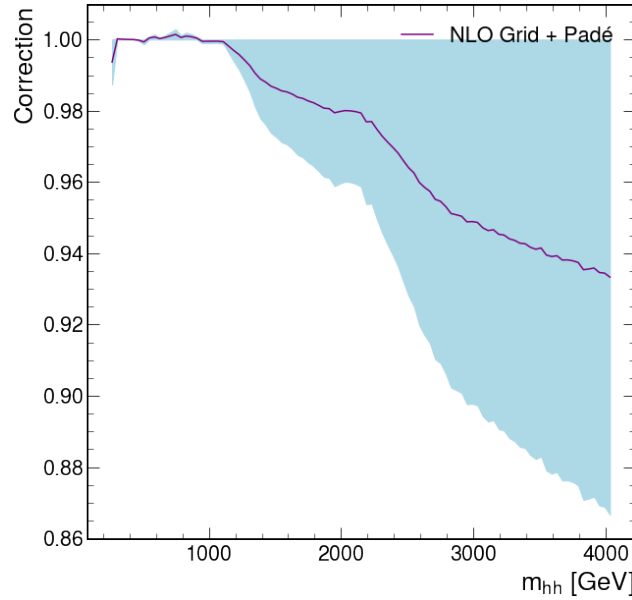
Figure 6.39: Correction factors to re-weight the current NLO calculation of m_{HH} in our signal simulation, to NLO calculations based on Pade approximations for virtual corrections, based on the high-energy expansion of the form factors [226].
