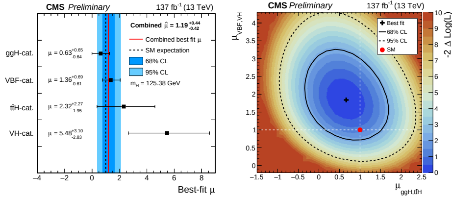
Figure 5.42: Results on the H \rightarrow \mu\mu signal strength. (Left) signal strength modifiers measured for m_H = 125.38 GeV in each production category (black points) are compared to the result of the combined fit (solid red line) and the SM expectation (dashed grey line). (Right) scan of the profiled likelihood ratio as a function of \mu_{ggH,t\bar{t}H} and \mu_{VBF,VH} with the corresponding 1\sigma and 2\sigma uncertainty contours. The black cross indicates the best-fit values (\hat{\mu}_{ggH,t\bar{t}H}, \hat{\mu}_{VBF,VH}) = (0.66, 1.84) , while the red circle represents the SM expectation.
