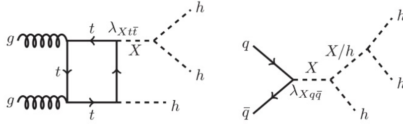
Figure 7.1: Semiresonant (left) and other resonant and nonresonant (right) tri-Higgs production diagrams via heavier scalar particle X [230].
