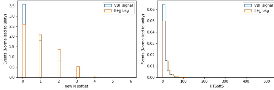
Figure 5.11: Variable comparisons between VBF Higgs signal (blue) and Drell-Yan + Electro-weak Z backgrounds (orange). (Left) N_5^{\text{soft}} and (Right) H_{T5}^{\text{soft}} .
