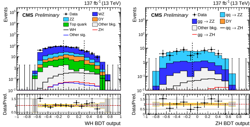
Figure 5.36: The observed BDT output distribution in the WH (left) and ZH (right) categories compared to the prediction from the simulation of various SM background processes. Signal distributions expected from different production modes of the 125 GeV Higgs boson are overlaid. The description of the ratio panel is the same as in Fig. 5.34. The dashed vertical lines indicate the boundaries of the optimized event categories.
