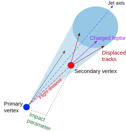
Figure 6.5: The hadronization of a b quark results in a B meson, which travels O(\sim \text{mm}) before decaying, resulting in a displaced secondary vertex (SV) inside the jet. This feature is exploited for b-jet tagging.
