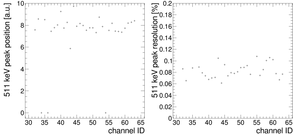
Figure B.4: The fitted position for each channel (Left) and the resolution of each channel (Right).
