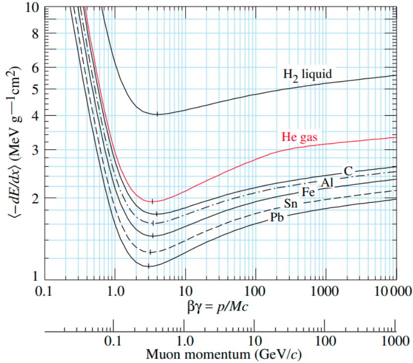
Figure 3.10: Mean energy loss of a muon traversing through different materials as a function of the muon p_T [79].
