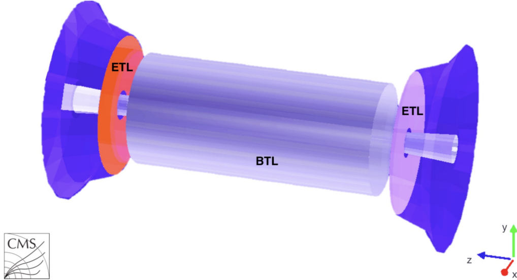
Figure 4.2: A schematic view of the GEANT geometry of the MTD, comprising a barrel layer (grey cylinder), at the interface between the tracker and the ECAL, and two silicon endcap (orange and light violet discs) timing layers in front of the endcap calorimeter [92].
