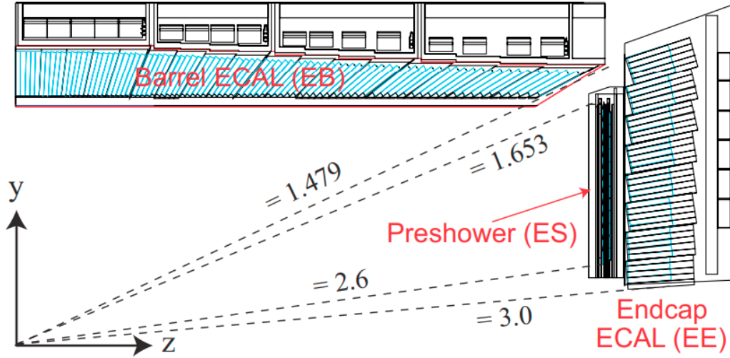
Figure 3.7: A geometric view of one quadrant of the ECAL [73].
