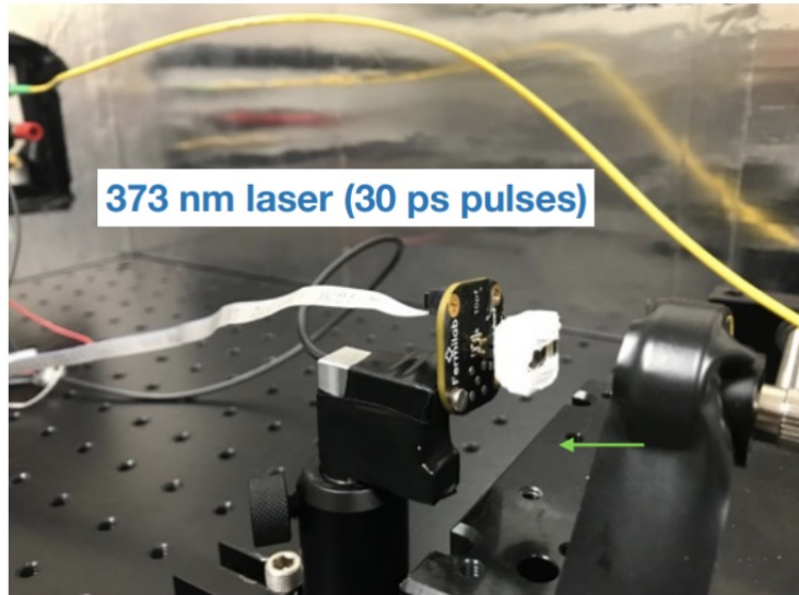
Figure 4.10: The SiPM is wrapped with Teflon and mounted on circuit board. A 373 nm UV laser is directly pointed at the center of the SiPM.
