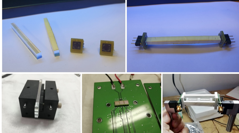
Figure 4.17: Sensors used at the Fermilab April 2019 test beam. (Top) Naked and wrapped individual crystal bars with the two FBK SiPMs (left) and single wrapped bar glued to SiPMs (right). (Bottom) Three-bar assembly in a crystal holder with the screws used to adjust the alignment of the crystals to the SiPMs (left); HPK SiPMs soldered onto a readout board (middle); single bar assembly (right).
