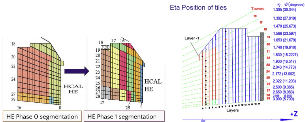
Figure A.2: Longitudinal segmentation of HE before and after the Phase I upgrade and the i\eta and pseudorapidity mapping of HE.
