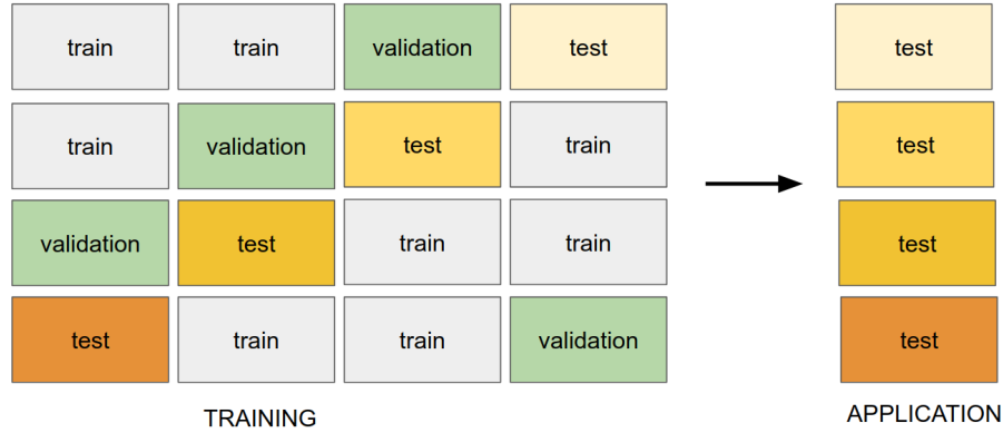
Figure 5.18: Scheme of the 4-fold training, validation and evaluation procedure.
