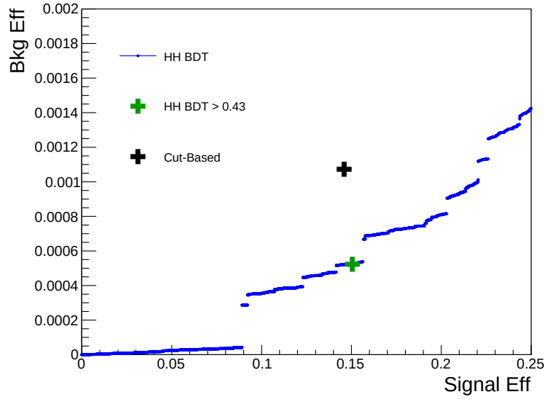
Figure 6.12: The ROC curve for the BDT is shown in this figure. The signal efficiency vs the background efficiency is plotted as one scans the requirement on the BDT output score. The black cross corresponds to the working point for the cut-based analysis selection (defined in text). The green cross corresponds to BDT score > 0.43 , which is the requirement in the most optimized analysis category (defined in Sec. 6.4.1.3). The discontinuities observed here arise due to certain large weight events in the QCD simulation samples.
