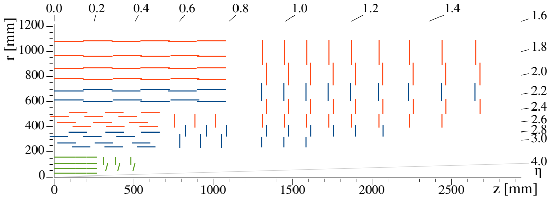
Figure 3.6: A schematic view of one quadrant of the Phase-1 CMS tracking system in the r - z plane. The pixel detector is shown in green, while single-sided and double-sided strip modules are depicted as red and blue segments, respectively [71].
