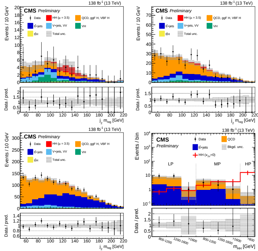
Figure 6.52: This figure shows post-fit distributions for the different event categories in the ggF and VBF analyses, corresponding to the best-fit parameters. (Top left) ggF event category 1, (top right) ggF event category 2, (bottom left) ggF event category 3 and (bottom right) VBF Signal Region.
