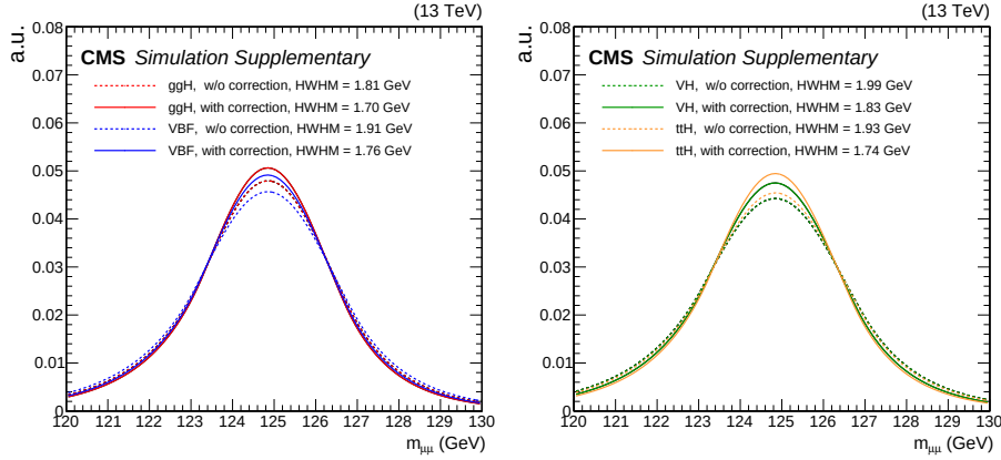
Figure 5.3: The expected m_{\mu\mu} distributions in simulated signal events with m_H = 125 GeV, passing the event selection requirements described in Sec. 5.5, obtained with (solid) and without (dashed) including the interaction point as an additional constraint for the muon track. Left: ggH and VBF processes. Right: VH and ttH. The signal peak is modelled using a double-sided Crystal Ball parametric function. The inclusive improvement in the mass resolution, estimated by comparing the HWHM of the corresponding signal peaks, ranges between 5-10% depending on the production mode.
