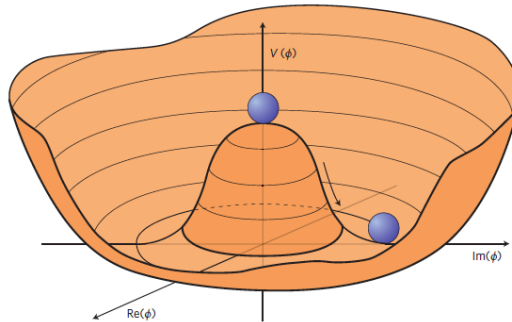
Figure 2.2: The Mexican hat shaped Higgs potential.
