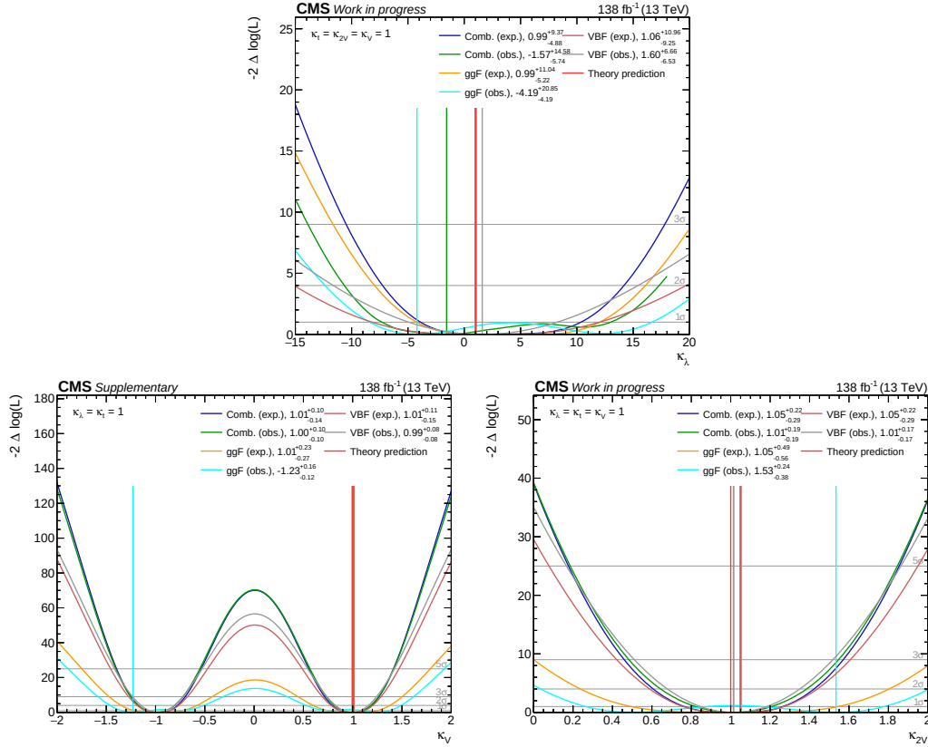
Figure 6.54: Comparison of the 1D expected and observed likelihood scans in \kappa_\lambda (top), \kappa_V (bottom left), and \kappa_{2V} (bottom right) for the ggF channel, VBF channel, and combined ggF and VBF channels.
