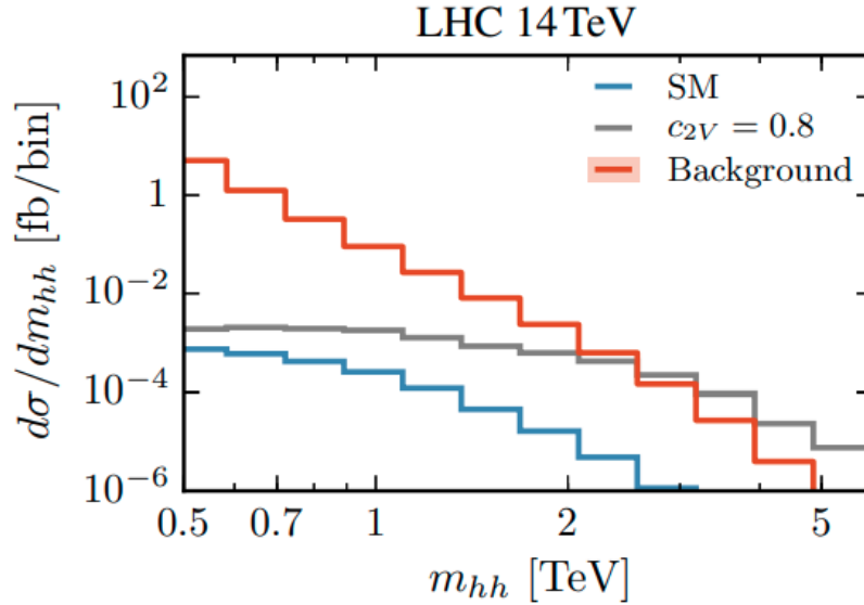
Figure 6.3: The m_{HH} spectra for different values of \kappa_{2V} [177].
