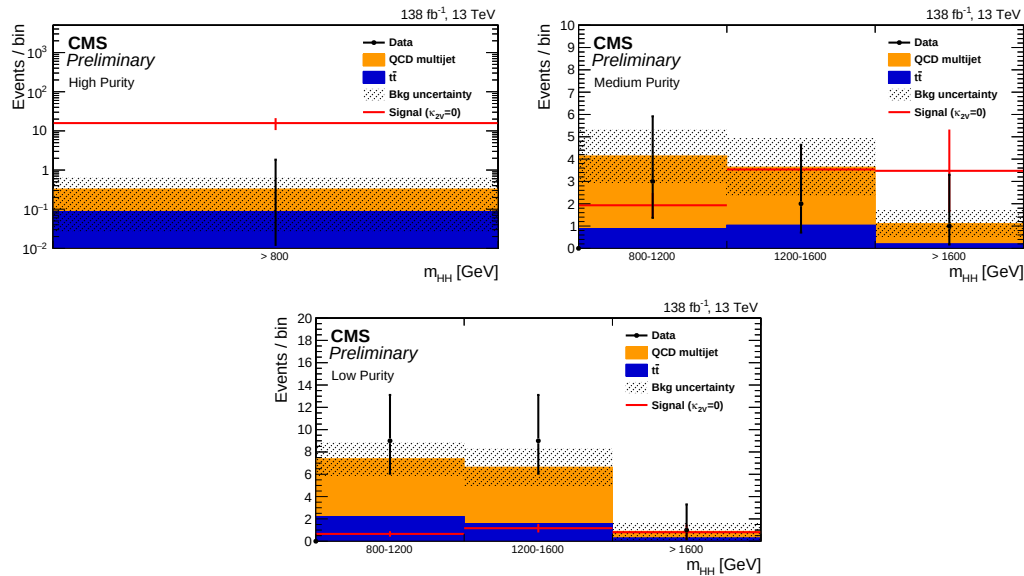
Figure 6.49: The m_{HH} distribution is shown here with a background-only fit to the data, for the HP (upper), MP (middle), and LP (lower) categories.
