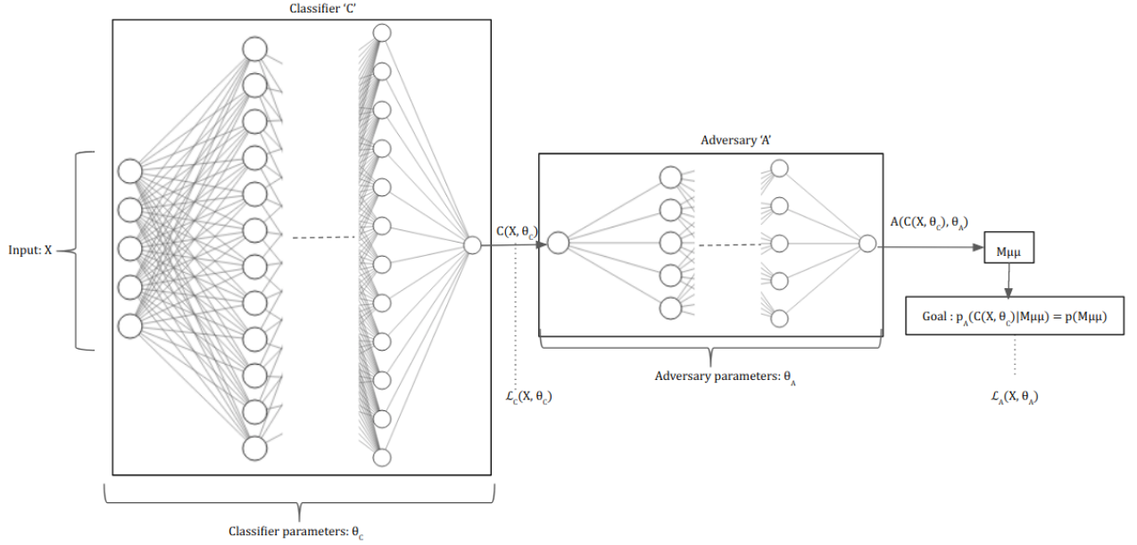
Figure C.1: Adversarial network.
