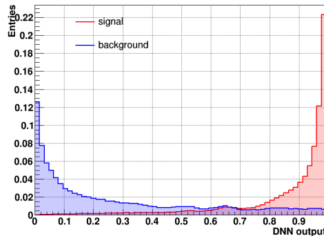
Figure 5.28: Plot of the signal and background normalized distributions for the DNN output score. The simulated samples of 2016, 2017, and 2018 are used all together.
