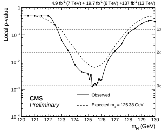
Figure 5.43: Observed (solid black) and expected (dashed black) local p-values as a function of m_H , extracted from the combined fit performed on data recorded at \sqrt{s} = 7, 8 , and 13 TeV, are shown. The expected p-values are calculated using the background expectation obtained from the signal-plus-background fit and injecting a signal with m_H = 125.38 GeV and \mu = 1 .
