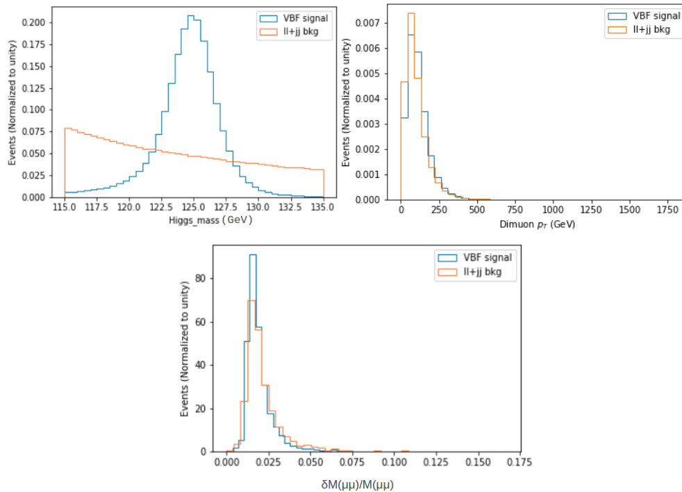
Figure 5.6: Variable comparisons between VBF Higgs signal (blue) and Drell-Yan + Electro-weak Z backgrounds (orange). (Top Left) m(\mu\mu) , (Top Right) p_T(\mu\mu) and (Bottom) \delta M(\mu\mu)/M(\mu\mu) .
