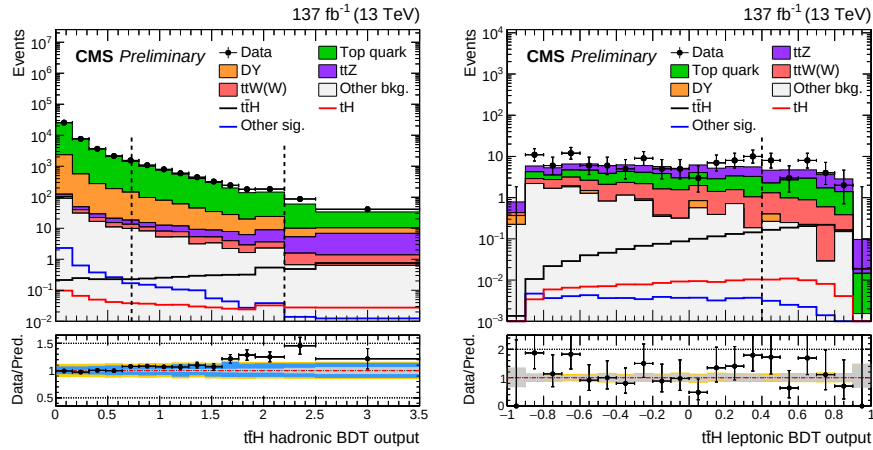
Figure 5.38: The observed BDT output distribution in the t\bar{t}H hadronic (left) and leptonic (right) categories compared to the prediction from the simulation of various SM background processes. The dashed vertical lines indicate the boundaries of the optimized event categories. The description of the ratio panels is the same as in Fig. 5.34.
