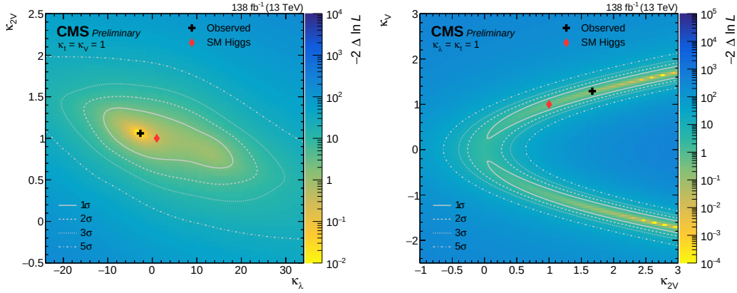
Figure 6.56: 2D profile likelihood scan as a function of \kappa_\lambda and \kappa_{2V} (left) and \kappa_V and \kappa_{2V} (right).
