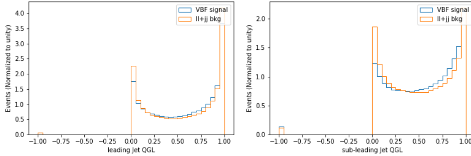
Figure 5.10: Variable comparisons between VBF Higgs signal (blue) and Drell-Yan + Electro-weak Z backgrounds (orange). (Left) QGL(j_1) and (Right) QGL(j_2) . Some jets have spurious QGL values of -1, which indicates the jet had very few constituents for a QGL value to be calculated effectively.
