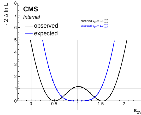
Figure 6.47: The observed and expected 1D likelihood scan of the HHVV coupling factor, \kappa_{2V} , assuming other Higgs boson couplings to be at their SM values.
