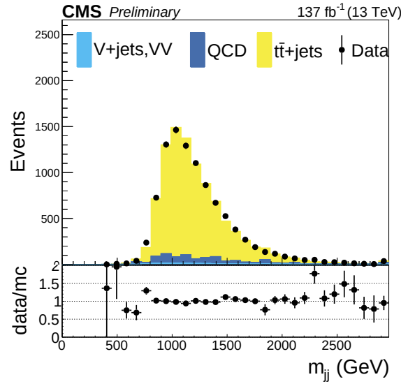
Figure 6.25: The distribution of the dijet mass is shown for events in the top control region using the full Run 2 dataset corresponding to 137 \text{ fb}^{-1} .
