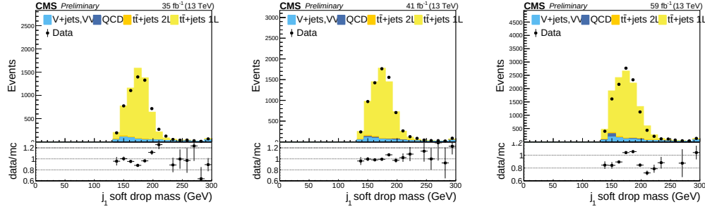
Figure 6.15: The distribution of the AK8 jet SD mass in the semi-leptonic t\bar{t} control region after imposing all requirements. The 2016, 2017, and 2018 datasets are shown in the left, center, and right plots, respectively.
