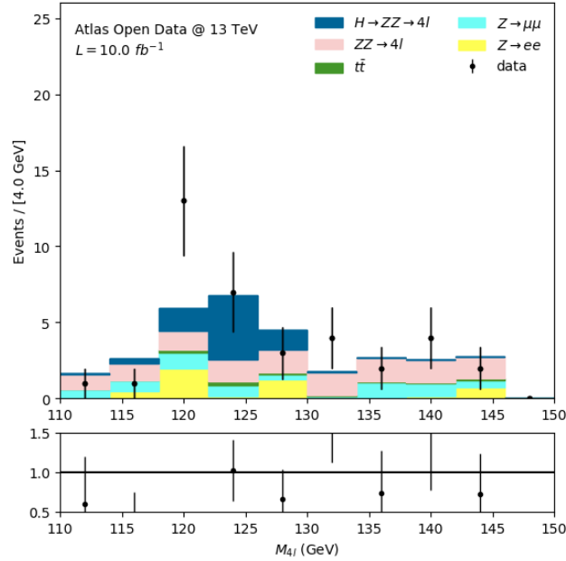
Figure D.3: The 4 lepton invariant mass peaks near 125 GeV.
