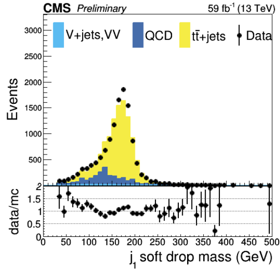
Figure 6.26: The Jet 1 m_{SD} in the t\bar{t} hadronic control region. The 80–120 GeV region shows that a factor of two increase or decrease to the QCD background would be incompatible with the observed data.
