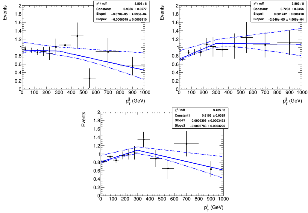
Figure 6.21: This figure shows the results of the “ramp-model” fit (solid blue line) in the hadronic t\bar{t} control region, for 2016 (top left), 2017 (top right), and 2018 (bottom) datasets. The black points here represent the residual data (data subtracted with non-top backgrounds) divided by the t\bar{t} simulation in different bins of p_T^{jj} . The fit uncertainties (shown with the dotted blue line) are propagated as systematic uncertainties for this correction in the final signal extraction fit.
