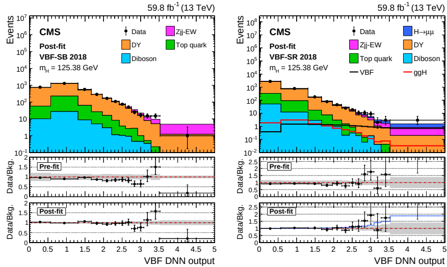
Figure 5.31: The observed DNN output distribution in the VBF-SB (left) and VBF-SR (right) regions compared to the post-fit background estimate for various SM processes. The predicted backgrounds are obtained from a combined signal-plus-background fit performed across analysis regions and eras. Distributions reported are related to the 2018 data-taking period. The description of ratio panels is the same as in Fig. 5.29.
