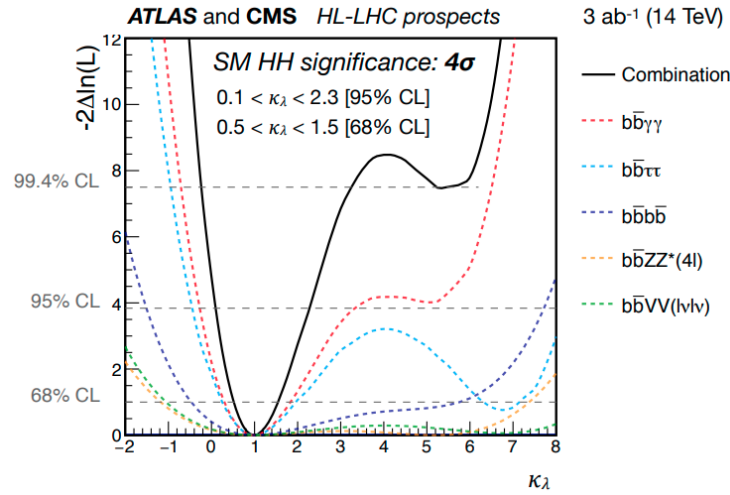
Figure 6.57: A projected likelihood scan of \kappa_\lambda at HL-LHC, calculated by performing a conditional signal+background fit to the background and SM signal. The coloured dashed lines correspond to the combined ATLAS and CMS results by channel, and the black line to their combination. Plot is taken from [173].
