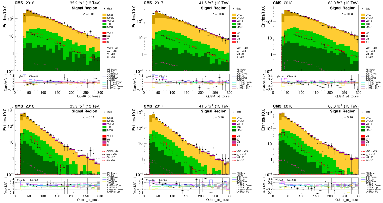
Figure 5.21: Transverse momentum distributions for leading (top) and subleading (bottom) jets after the event selection in the Signal Region for 2016 (left), 2017 (center), and 2018 (right) [150].
