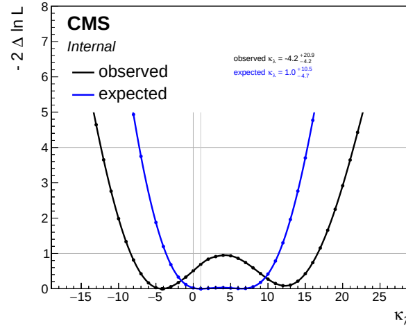
Figure 6.46: The observed and expected 1D likelihood scan of the Higgs boson self-coupling factor, \kappa_\lambda , assuming all other Higgs boson couplings to be at their SM values.
