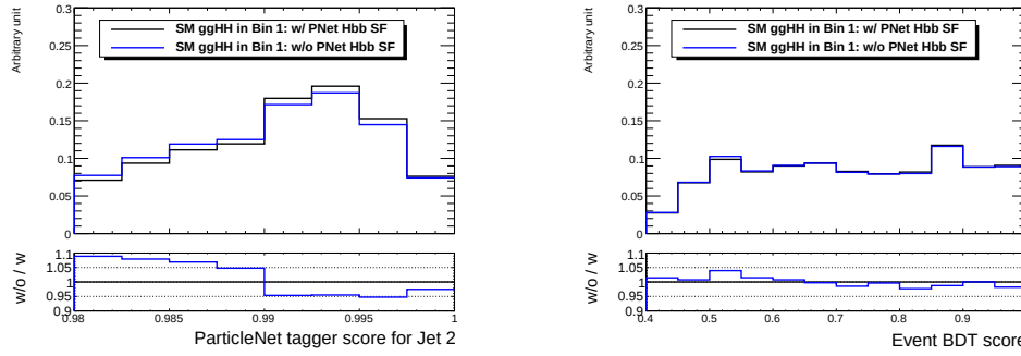
Figure 6.38: The impact of the measured T_{Xbb} correction factors on the ParticleNet tagger score for Jet 2 (left) and BDT discriminant (right) for the SM ggHH signal in event category 1. The histograms are normalized to unit area to show the change in shape.
