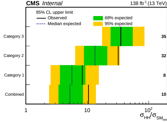
Figure 6.44: Observed (expected) 95% CL upper limits on the \sigma_{HH} \times \mathcal{B}(HH \rightarrow b\bar{b}b\bar{b}) , in different event categories, and by combining all categories are presented by the solid (dashed) black line. The green and yellow bands represent the expected one and two standard deviation uncertainty bands on the expected limit, respectively.
