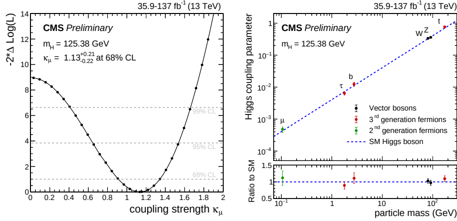
Figure 5.44: Higgs boson coupling modifiers. (Left) observed profile likelihood ratio as a function of \kappa_\mu for m_H = 125.38 \text{ GeV} , obtained from a combined fit with Ref. [167] in the \kappa -framework model. The best-fit value for \kappa_\mu is 1.13 and the corresponding observed 68% CL interval is 0.91 < \kappa_\mu < 1.34 . (Right) the best-fit estimates for the coupling parameters compared to their corresponding prediction from the SM, as function of the particle mass. The error bars represent 68% CL intervals for the measured parameters. The lower panel shows the ratios of the measured coupling modifiers values to their SM predictions.
