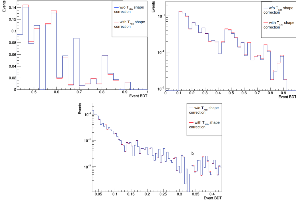
Figure 6.19: The distribution of the event BDT score in the signal region for the t\bar{t} background, for event category 1 (top left), category 2 (top right), and category 3 (bottom). The histograms are normalized to unit area.
