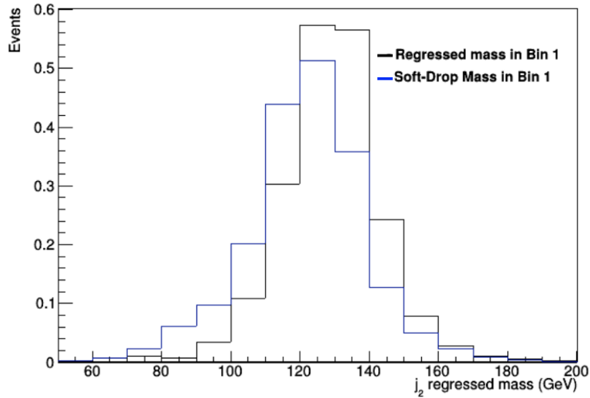
Figure 6.8: Comparison of the mass resolution for one of the H \rightarrow b\bar{b} jets from the SM ggHH signal in the most sensitive category of this analysis (category 1, as explained in Sec. 6.4.1.1). The performance of the soft drop mass algorithm is shown in blue and the regressed mass algorithm is shown in black. The regressed jet mass algorithm improves our overall signal sensitivity by 25%.
