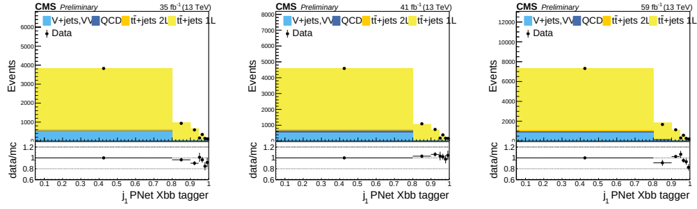
Figure 6.16: The distribution of the jet T_{Xbb} score in the 1\ell+1j t\bar{t} control region for 2016 (left), 2017 (middle), and 2018 (right); the first bin includes underflow events in each plot.
