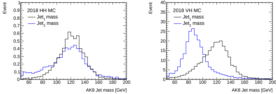
Figure 6.9: After pre-selection requirements, the distributions of the first and second jet mass for HH signal (left) and VH background (right) are shown in this figure. The second jet in VH background events tends to be the W or Z boson instead of the Higgs boson.
