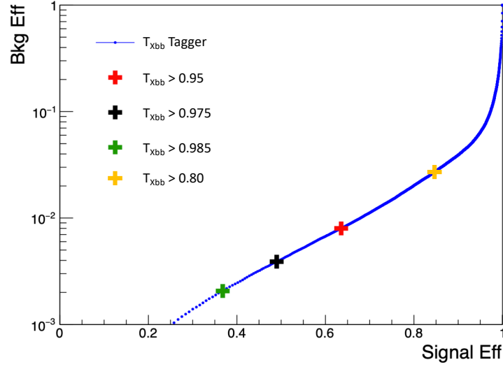
Figure 6.7: The ROC curve for the ParticleNet X \rightarrow b\bar{b} tagger is shown in this figure. The signal here corresponds to reconstructed AK8 jets matched to truth level Higgs bosons from the ggHH simulation samples, and the background corresponds to AK8 jets from the QCD multijet sample. The events selected for this figure contain two AK8 jets with p_T > 300 GeV and a soft drop mass > 40 GeV each. The signal efficiency is plotted against the background efficiency as one scans the tagger score for the jets. The red, black, green, and orange crosses correspond to various working points for the tagger, relevant for this analysis.
