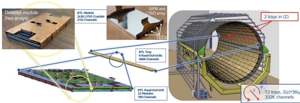
Figure 4.4: A schematic view of the structure and design of BTL [101].
