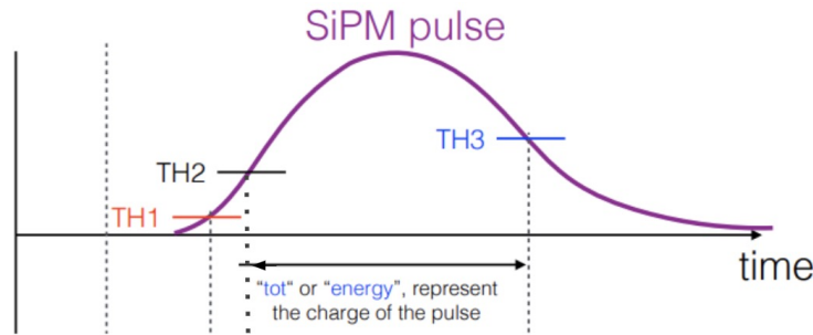
Figure B.1: The discriminator thresholds of the TOFPET 2 ASIC.
