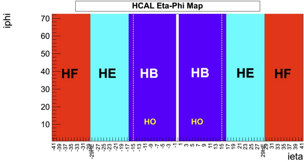
Figure A.1: The HCAL i\eta - i\phi map [231]. HB covers the range |\eta| \leq 16 ; HE covers the range 17 \leq |\eta| \leq 29 ; HF covers the range |\eta| > 29 ; HO covers the range |\eta| \leq 15 (the region within the dashed yellow lines).
