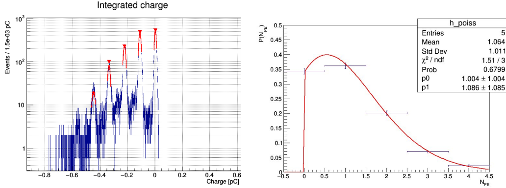
Figure 4.11: Single photoelectron measurements with a UV laser. (Left) The recorded charge spectrum. The different peaks correspond to different values of N_{p.e.} . (Right) Poisson fit to the number of photo-electrons.
