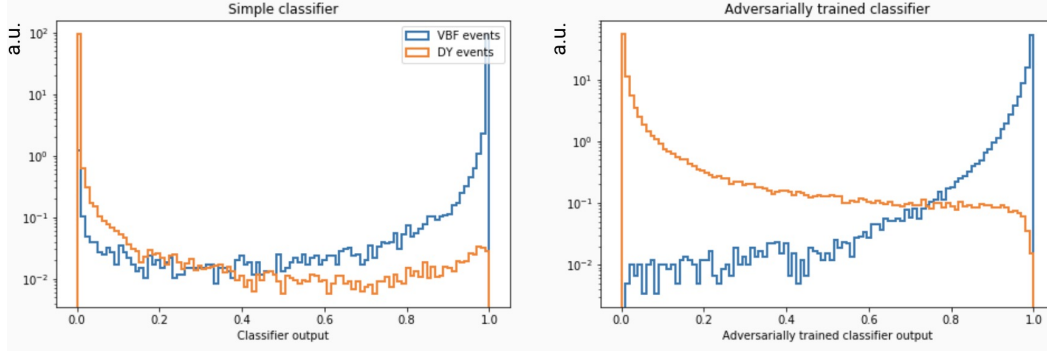
Figure C.2: The output score of the network. (Left) Simple classifier and (Right) Adversarial network. The simple classifier has a better separation power.
