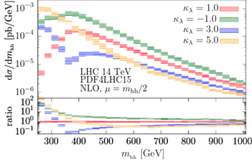
Figure 6.2: The m_{HH} spectra for different values of \kappa_\lambda [176].
