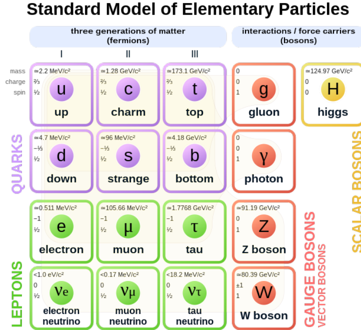
Figure 2.1: The elementary particles in the SM [27].
