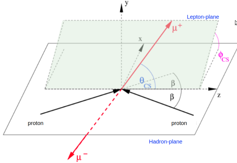
Figure 5.12: An illustration of the Collins-Soper frame.
