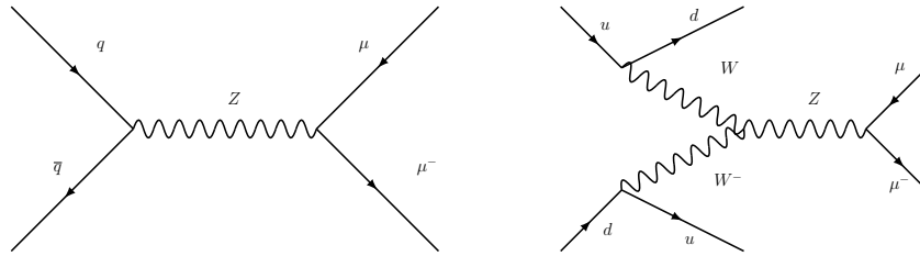
Figure 5.1: The Drell-Yan (left) and electroweak production (right) of a Z boson decaying to a pair of muons.
