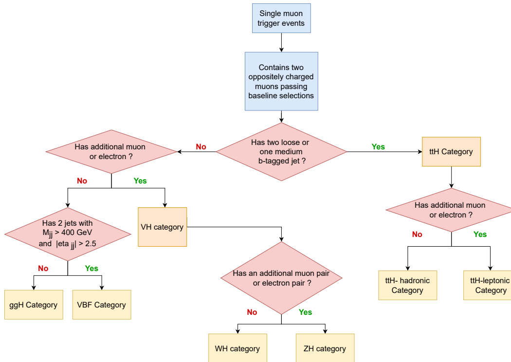
Figure 5.5: Graphical summary of the logical definition of each event category from the baseline dimuon selection. Exclusive channels are defined to target the following production modes: ttH (leptonic or hadronic t\bar{t} final states), leptonic WH and ZH, VBF, and ggH.
