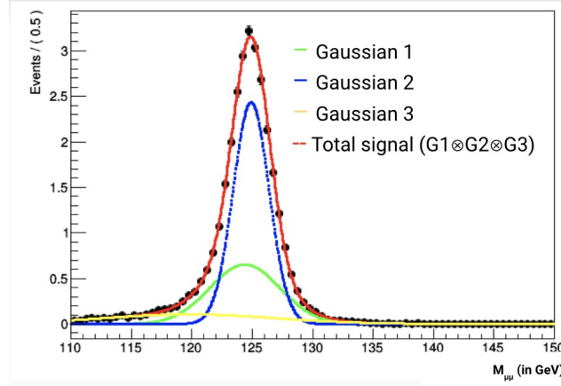
Figure C.4: The ggH + VBF signal is modelled with a sum of 3 Gaussian functions.
