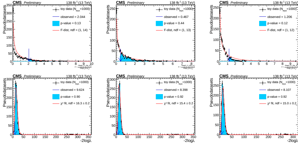
Figure 6.31: Deriving transfer factors for QCD parametric alphabet fit. (Top) F-distribution of poly-0 vs poly-1 (left), poly-1 vs poly-2 (middle), poly-2 vs poly-3 (right); (Bottom) GOF test of poly-0 (left), poly-1 (middle), poly-2 (right). These plots are for event category 1. Poly-0 is the selected model from the F-test and GOF-tests as it passes both tests.
