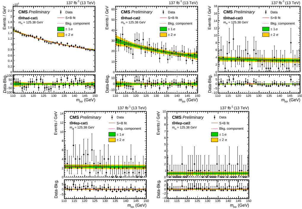
Figure 5.39: Comparison between the observed data and the total background extracted from a signal-plus-background fit performed across t\bar{t}H hadronic (first row) and leptonic (second row) event categories. First row, from left to right: t\bar{t}H had-cat1, t\bar{t}H had-cat2, and t\bar{t}H had-cat3. Second row, from left to right: t\bar{t}H lep-cat1 and t\bar{t}H lep-cat2. The one (green) and two (yellow) standard deviation bands include the uncertainties in the background component of the fit. The lower panel shows the residuals after the background subtraction, where the red line indicates the signal with m_H = 125.38 GeV extracted from the fit.
