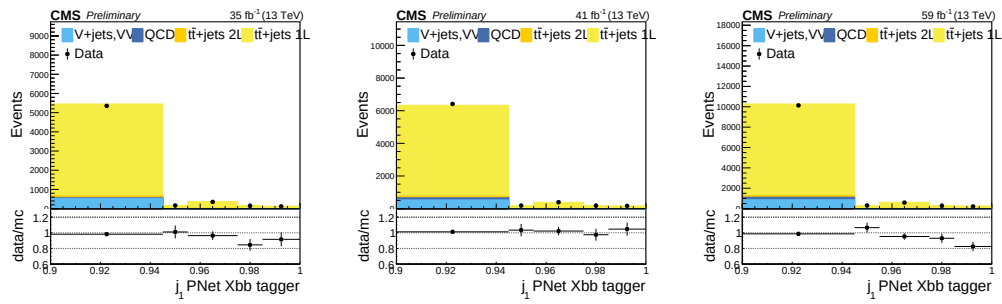
Figure 6.17: The distribution of the jet T_{Xbb} score in the 1\ell+1j t\bar{t} control region for 2016 (left), 2017 (middle), and 2018 (right) showing the most important bins.
