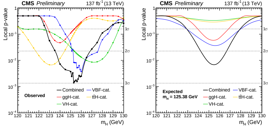
Figure 5.41: p-value vs m_H scan. (Left) observed local p-values as a function of m_H , extracted from the combined fit as well as from each individual production category, are shown. (Right) the expected p-values are calculated using the background expectation obtained from the signal-plus-background fit and injecting a signal with m_H = 125.38 GeV and \mu = 1 .
