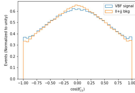
Figure 5.13: Variable comparisons between VBF Higgs signal (blue) and Drell-Yan + Electro-weak Z backgrounds (orange): \cos(\theta_{CS}) .
