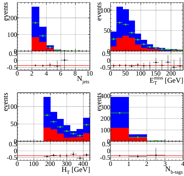
Figure 7-10. Closure test for electrons in W +jets MC with dilepton selection for (A) nonprompt e and (B) H_T > 160 GeV, N_{\text{jets}} \geq 2 . Observed number of events is shown by filled histograms: red shows events where a nonprompt lepton comes from a b-jet, green shows leptons from c-jet, blue shows leptons from light jets. Predicted number of events is shown by points. The red line corresponds to a fit with a constant.
