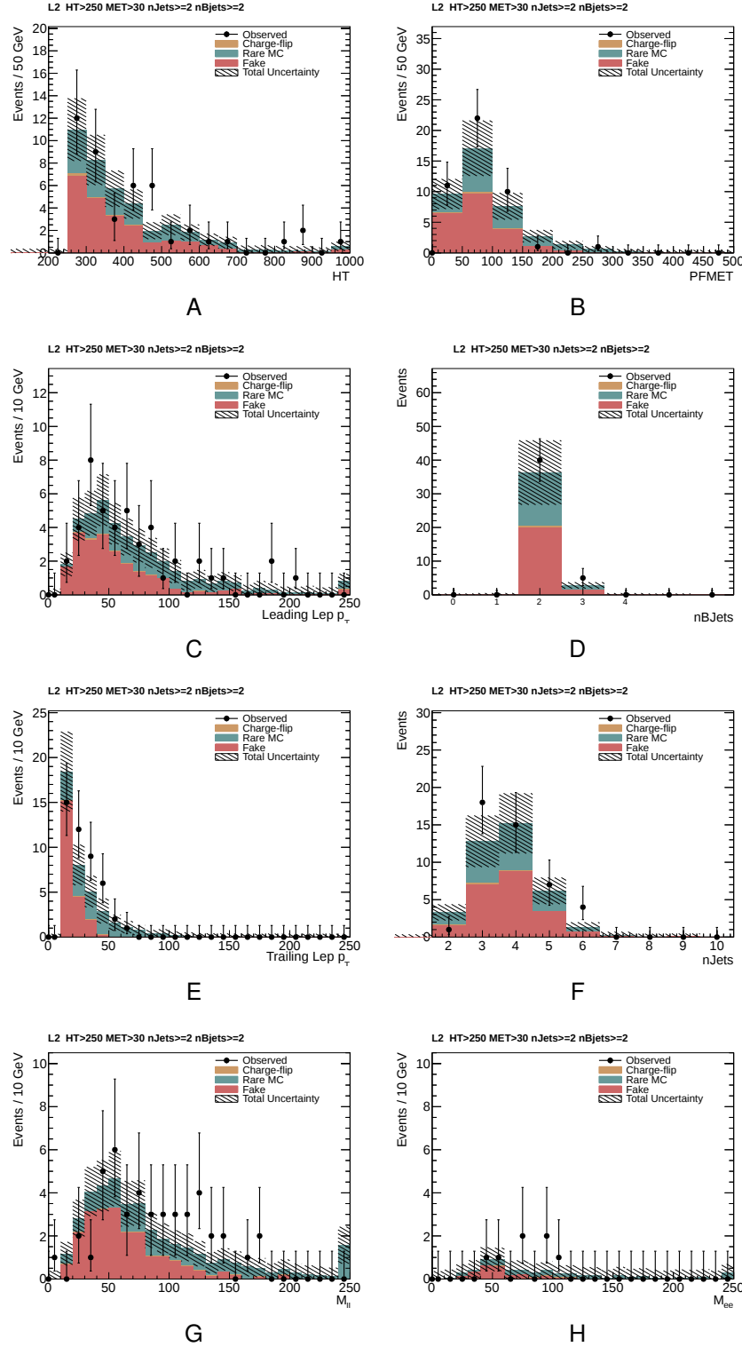
Figure 7-23. L2 kinematic distributions of predicted SM backgrounds and observed number of events are shown for: (A) H_T , (B) E_T , (C) leading lepton p_T , (D) N_{b\text{-jets}} , (E) trailing lepton p_T , (F) N_{\text{jets}} , (G) M_{ll} , and (H) M_{ee} are plotted. The results correspond to the low- p_T baseline selection where H_T > 250 \text{ GeV} , E_T > 30 \text{ GeV} , N_{b\text{-jets}} \geq 2 .
