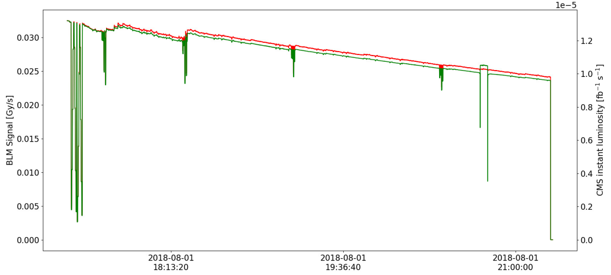
Figure 18: BLM signal of a detector located near IP5 and instant luminosity in CMS during a STABLE beam mode period. The BLM signal is indicated in red and the instant luminosity in green.
