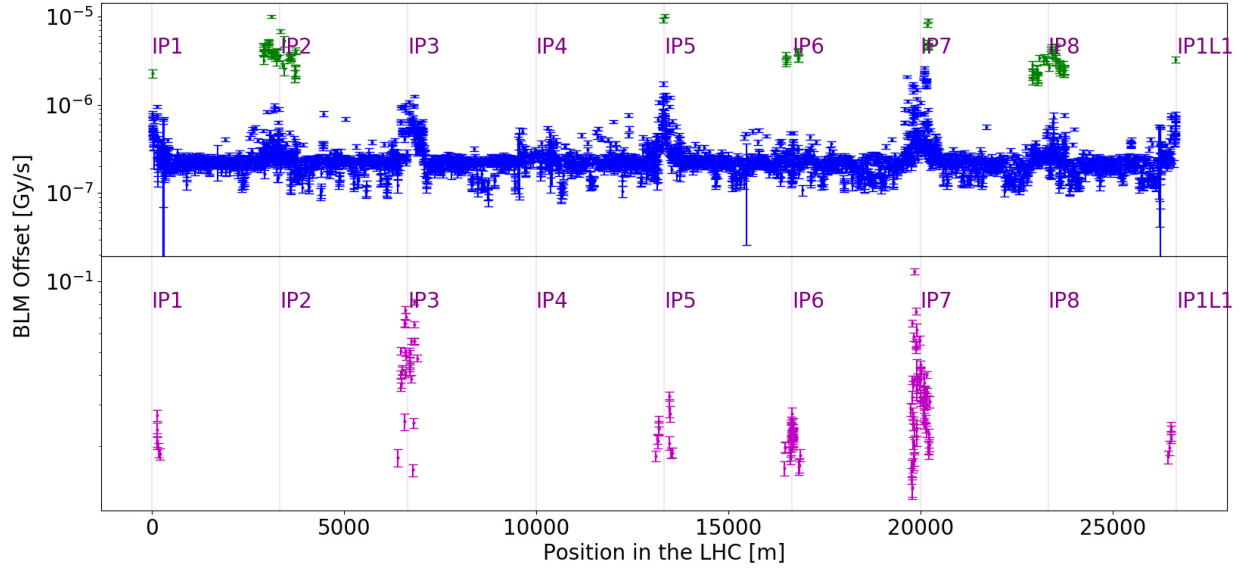
Figure 10: BLM signal offset distribution along the LHC ring for the three types of BLM detectors (ICs in blue, LICs in green and SEMs in magenta). The standard deviations of the calculated offset values are indicated as error bars. The positions of the different IPs are indicated with vertical lines.
