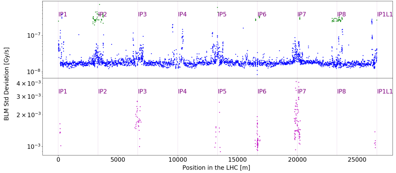
Figure 13: Distribution of the standard deviation of the BLM signal offset in the LHC. Each point corresponds to the standard deviation of a LHC BLM detector. ICs are indicated in blue, LICs in green and SEMs in magenta. The positions of the different IPs are indicated with vertical lines.
