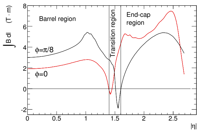
Figure 3.7: Predicted field integral as a function of |\eta| for infinite momentum muons. The integral is calculated for two values of the azimuthal angle \phi .
