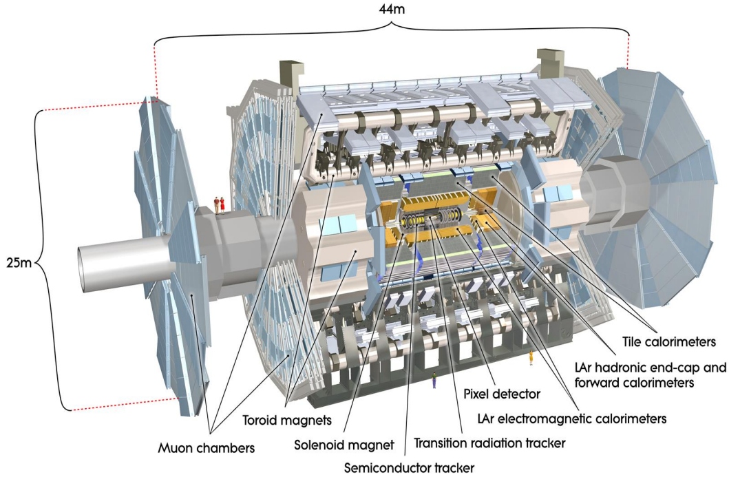
Figure 3.4: Cutaway view of the whole ATLAS detector and its sub-systems [71].
