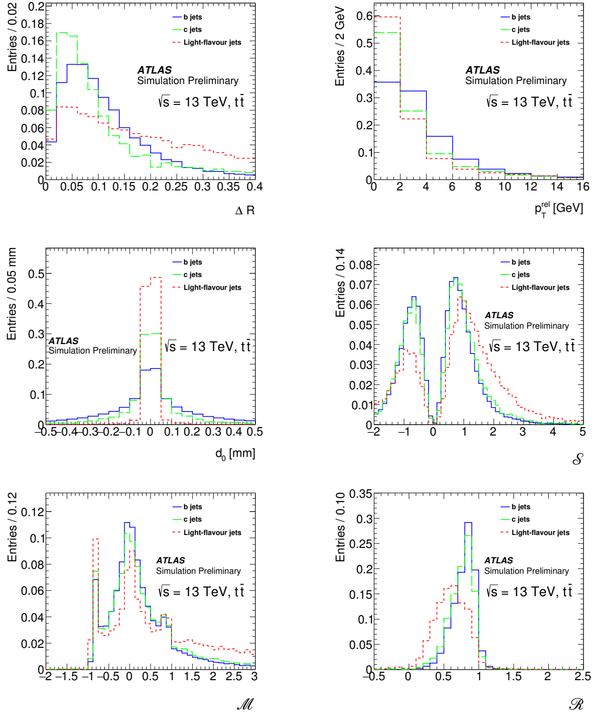
Figure 4.10: Normalised distributions of the six SMT input variables for reconstructed CB muons associated to b -jets (blue), c -jets (green) and light-flavour jets (red) in simulated t\bar{t} events [134].
