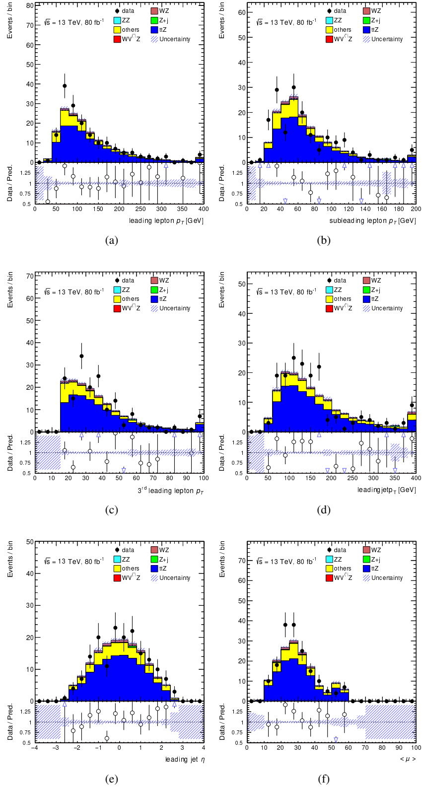
Figure A.3: Data/simulation comparison in the t\bar{t}Z \rightarrow 3\ell control region, comparing the full 80 fb -1 dataset to mc16a and mc16d, for: (a) the leading lepton p_T , (b) the subleading lepton p_T , (c) the 3 rd leading lepton p_T , (d) the leading jet p_T , (e) the leading jet \eta and (f) the \langle \mu \rangle . The lower panel shows the data-to-simulation ratio. Only statistical uncertainties are shown.
