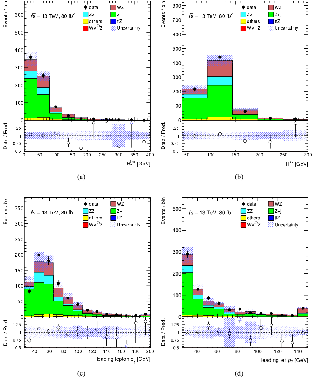
Figure 6.11: Data/simulation comparison in the 3\ell Z + jets validation region for (a) H_T^{\text{had}} , (b) H_T^{\text{lep}} , the leading (c) lepton and (d) jet p_T , comparing the full 80 \text{ fb}^{-1} dataset to mc16a and mc16d. The lower panel shows the data-to-simulation ratio. Only statistical uncertainties are shown.
