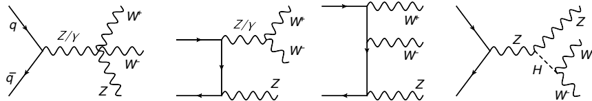
Figure 6.1: Example diagrams for massive triple vector boson production W^\pm W^\mp Z [188].
