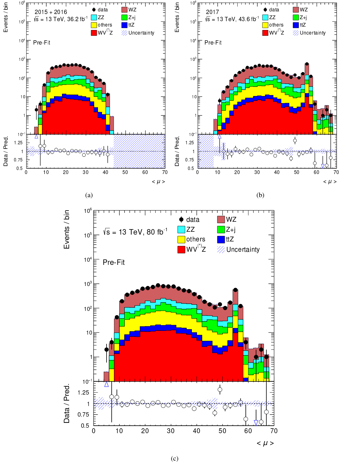
Figure 6.6: Data/simulation comparison in the 3\ell pre-MVA region for the average pile-up profile comparing (a) data collected in 2015 and 2016 ( 36.2 \text{ fb}^{-1} ) to mc16a, (b) data collected in 2017 ( 43.6 \text{ fb}^{-1} ) to mc16d and (c) the full 80 \text{ fb}^{-1} dataset to mc16a and mc16d. The lower panel shows the data-to-simulation ratio. Only statistical uncertainties are shown.
