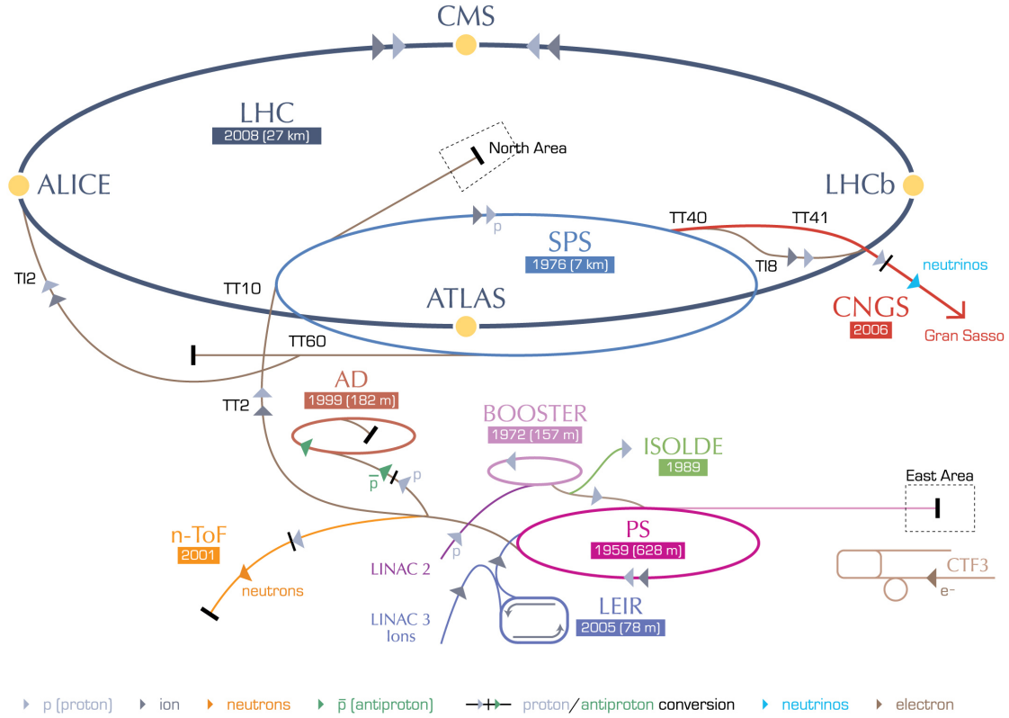
Figure 3.2: Overview of the accelerator complex at CERN [25].
