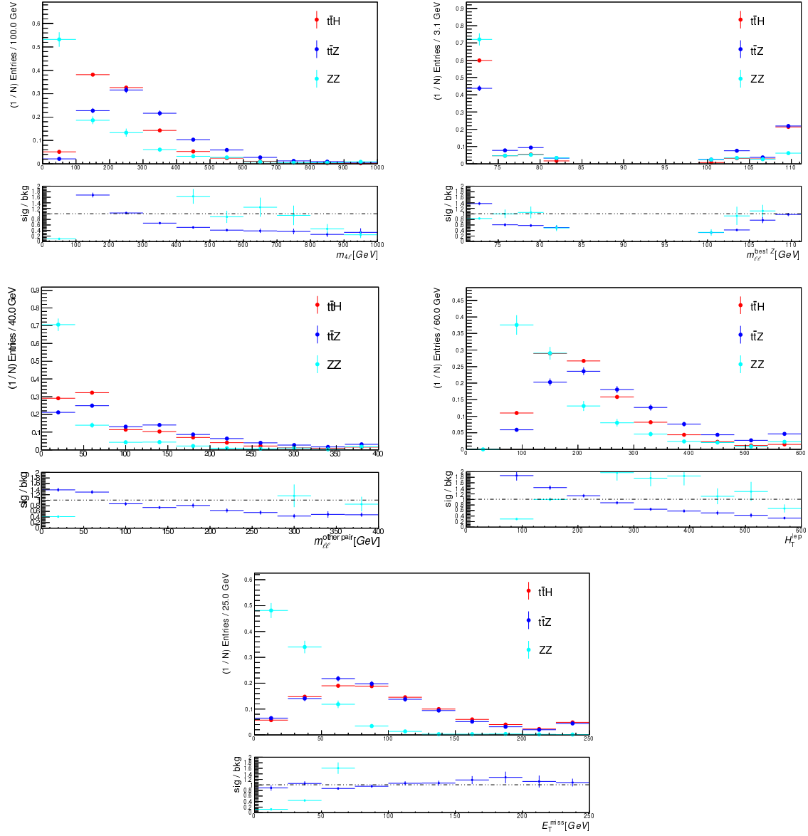
Figure 5.15: Distributions of five BDTG input variables: m_{4\ell} , m_{\ell\ell}^{\text{best } Z} , m_{\ell\ell}^{\text{other pair}} , H_T^{\text{lep}} and E_T^{\text{miss}} ; the t\bar{t}H (red), t\bar{t}Z (blue) and ZZ (light blue) shapes are compared in the Z-enriched signal region.
