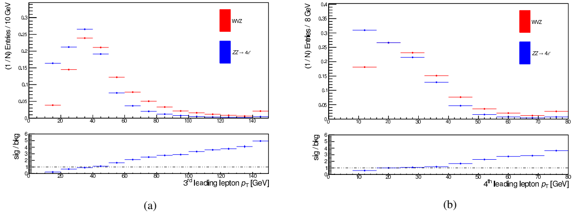
Figure 6.5: Shape comparison for the (a) 3 rd and (b) 4 th leading lepton p_T for the WVZ (red) and ZZ (blue) processes, requiring four loose reconstructed leptons with total charge zero. The lower panels show the ratio between the WVZ and ZZ shapes. Statistical-only uncertainties are shown.
