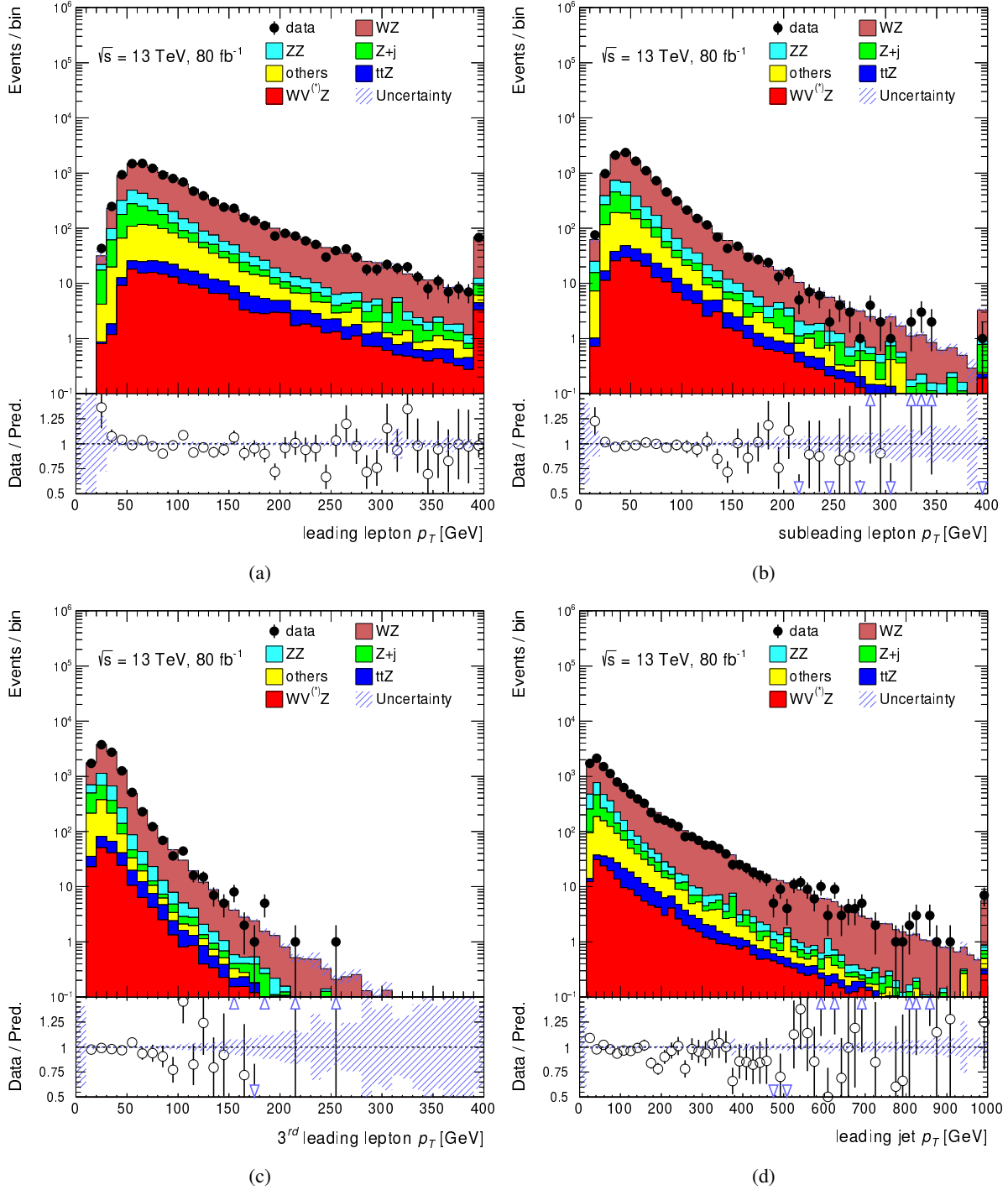
Figure A.2: Data/simulation comparison in the 3\ell pre-MVA region for the (a) leading lepton p_T , (b) sub-leading lepton p_T , (c) third leading lepton p_T and (d) leading jet p_T . The full 80\text{ fb}^{-1} dataset is compared to the complete set of simulation samples. The lower panel shows the data-to-simulation ratio. Only statistical uncertainties are shown.
