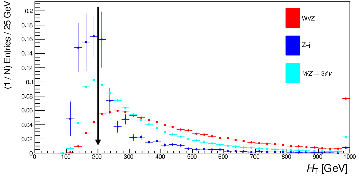
Figure 6.15: Comparison between the expected H_T shapes for WVZ , Z + \text{jets} and WZ in the 3\ell pre-selection region. The black arrow shows the H_T > 200 GeV requirement applied to events entering the 3\ell pre-MVA region. Statistical-only uncertainties are shown.
