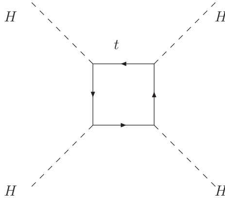
Figure 2.9: Feynman diagram representing the top-quark one-loop contribution, reported in Eq. 2.53, to the Higgs-field effective potential.
