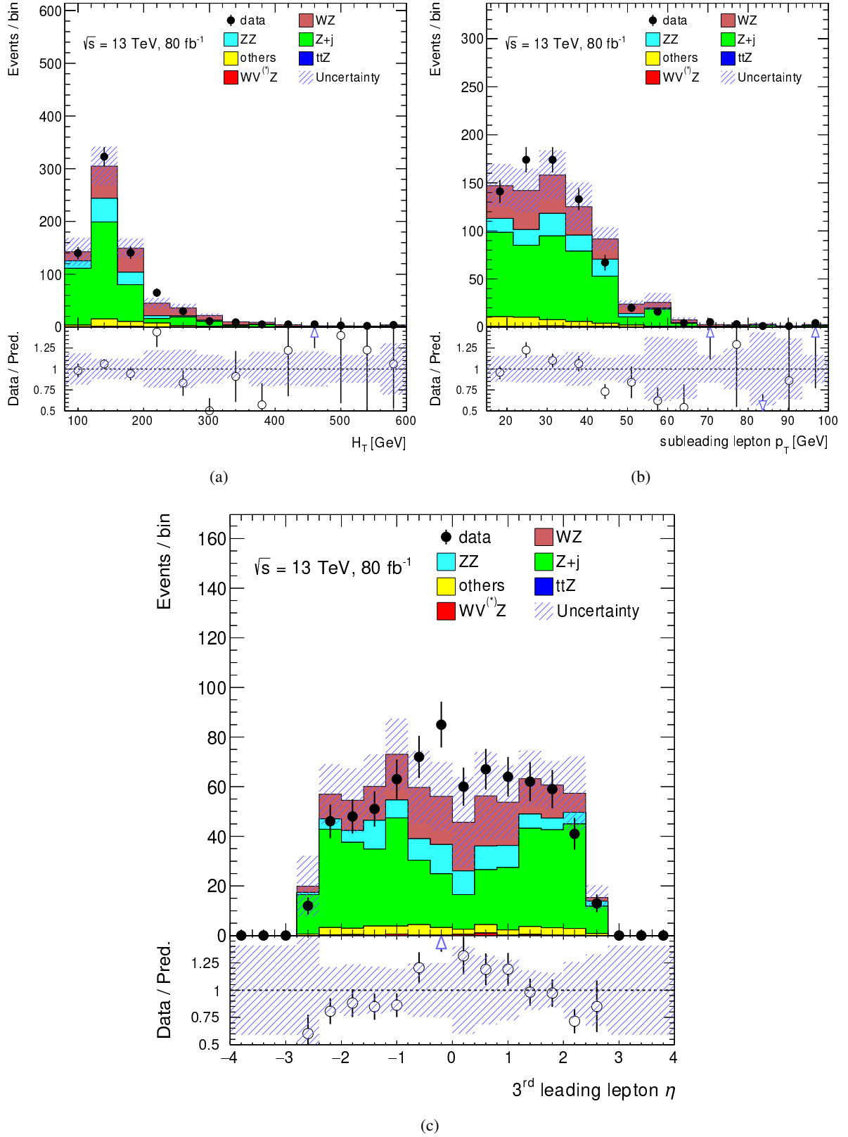
Figure A.5: Data/simulation comparison in the 3\ell Z + \text{jets} validation region for (a) H_T , (b) the subleading lepton p_T and (c) the third leading lepton \eta , comparing the full 80 \text{ fb}^{-1} dataset to mc16a and mc16d. The lower panel shows the data-to-simulation ratio. Only statistical uncertainties are shown.
