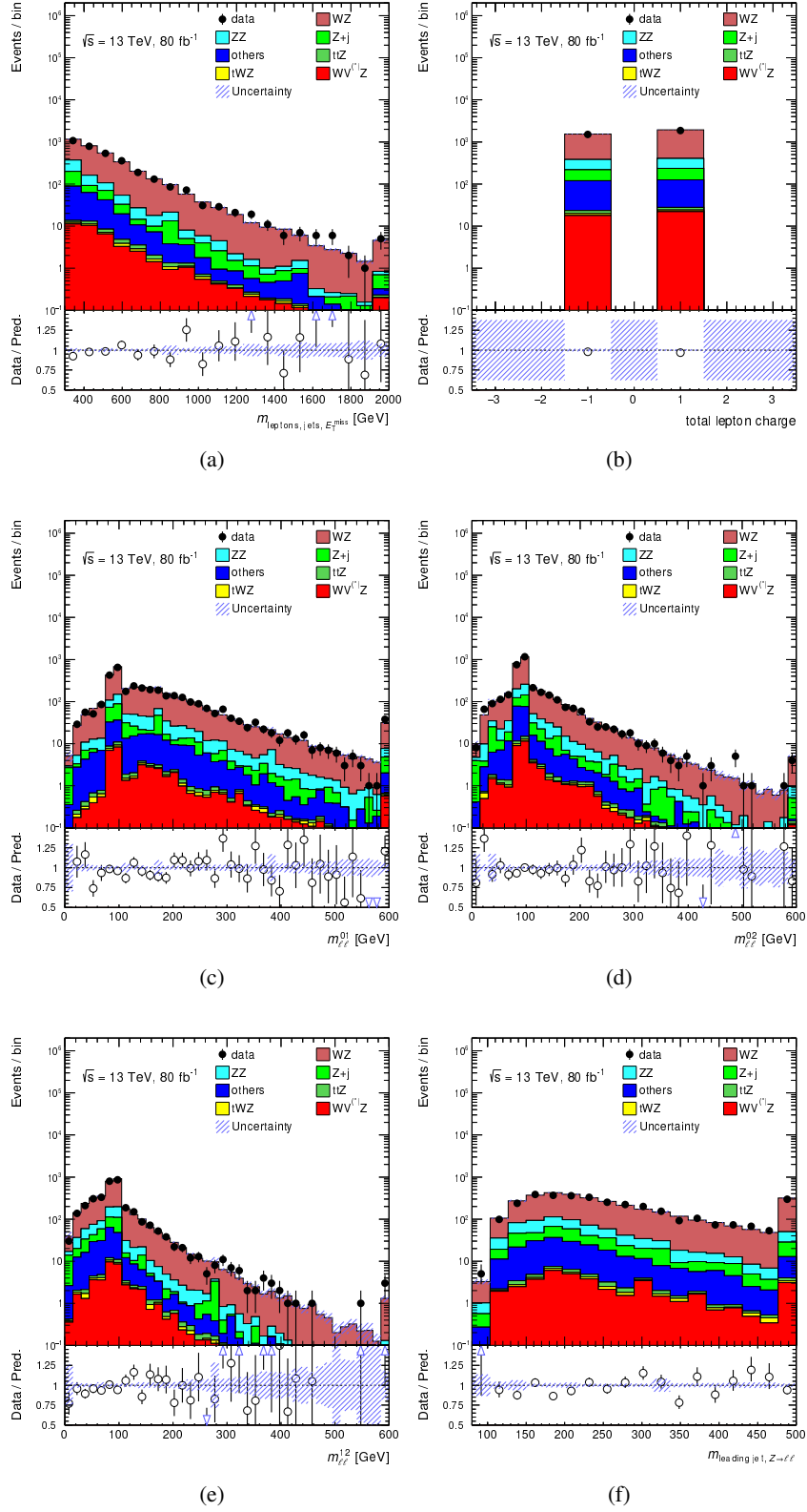
Figure C.2: Data/MC comparison in the 3\ell 1j region for: (a) the invariant mass of leptons, jets and E_T^{\text{miss}} , (b) the total lepton charge, (c) m_{\ell\ell}^{01} , (d) m_{\ell\ell}^{02} , (e) m_{\ell\ell}^{12} and (f) the invariant mass of best Z \rightarrow \ell\ell candidate and the leading jet. Only statistical uncertainties are shown.
