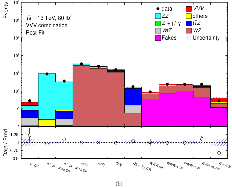
Figure 6.33: Comparison between prediction and observed data, (a) before and (b) after the fit, in the twelve regions entering the combined VVV profile likelihood fit. Contributions due to charge-flip and fake/non-prompt processes entering the WWW channels are labelled as “Fakes”. The lower panel shows the data-to-simulation ratio. The overall uncertainties are indicated by the shaded blue bands.
