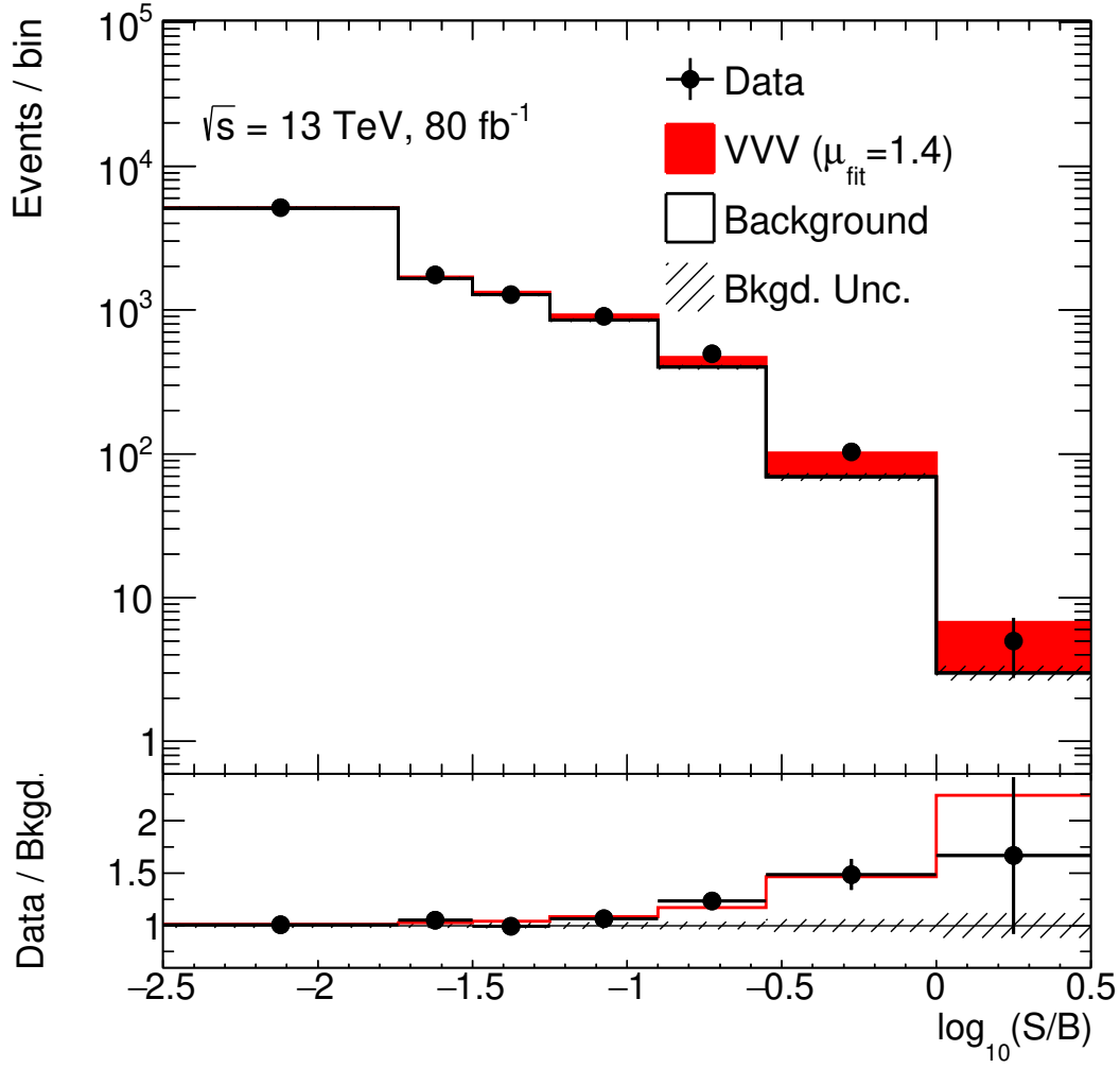
Figure 6.34: Event yields as a function of \log_{10}(S/B) , where S ( B ) indicates the signal (background) expected yield in the corresponding bin. Events in all of the twelve fitted regions are included and the predicted background yield is obtained from the global signal-plus-background fit. The VVV signal is shown for the best-fit ( \mu = 1.4 ) value.
