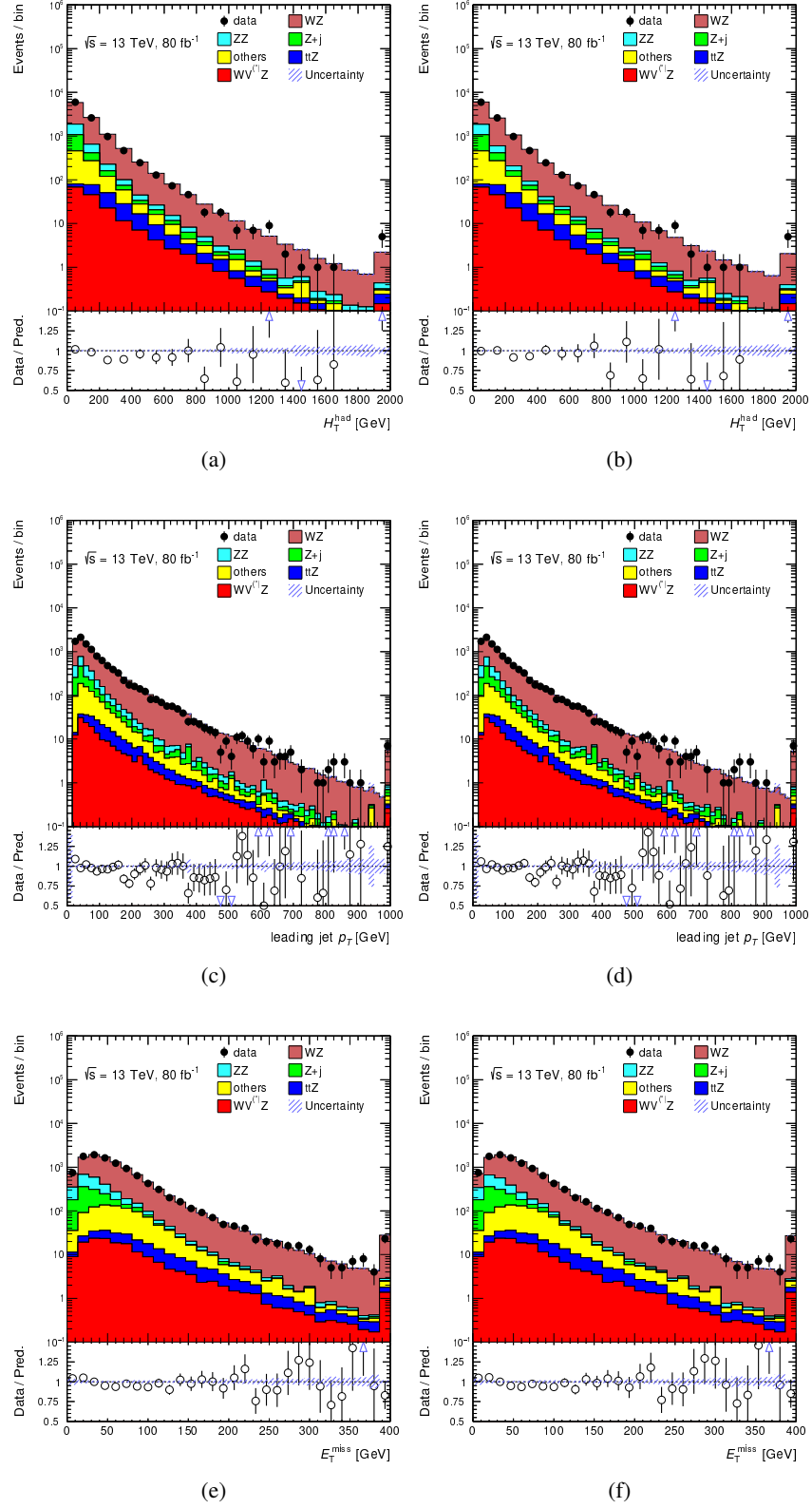
Figure B.1: Data/MC comparison before (left column) and after (right column) reweighting for: (a)(b) H_T^{\text{had}} , (c)(d) the leading jet p_T and (e)(f) E_T^{\text{miss}} . Only statistical uncertainties are shown.
