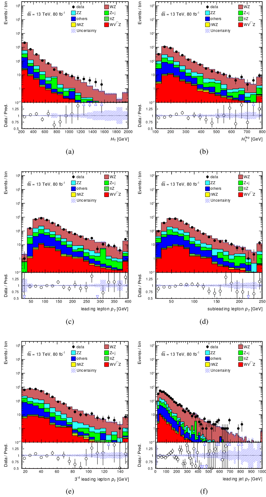
Figure C.1: Data/MC comparison in the 3\ell 1j region for: (a) H_T , (b) H_T^{\text{lep}} , (c) the leading lepton p_T , (d) the subleading lepton p_T , (e) the third leading lepton p_T and (f) the leading jet p_T . Only statistical uncertainties are shown.
