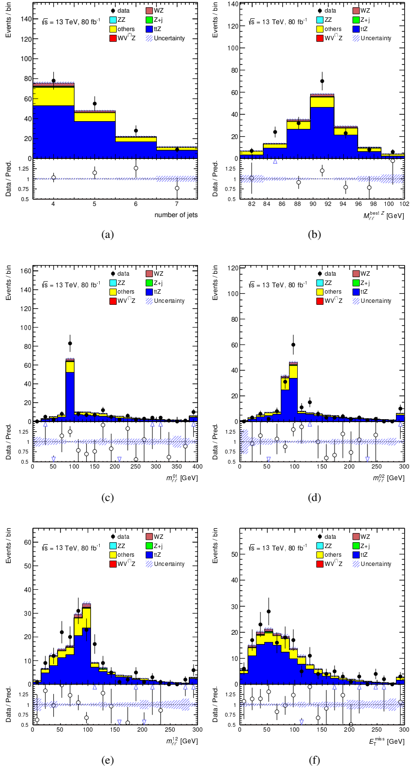
Figure 6.10: Data/simulation comparison in the t\bar{t}Z \rightarrow 3\ell control region, comparing the full 80 fb -1 dataset to mc16a and mc16d, for: (a) the number of jets, (b) the best Z-candidate invariant mass, (c) m_{\ell\ell}^{01} , (d) m_{\ell\ell}^{02} , (e) m_{\ell\ell}^{12} and (f) E_T^{\text{miss}} . The lower panel shows the data-to-simulation ratio. Only statistical uncertainties are shown.
