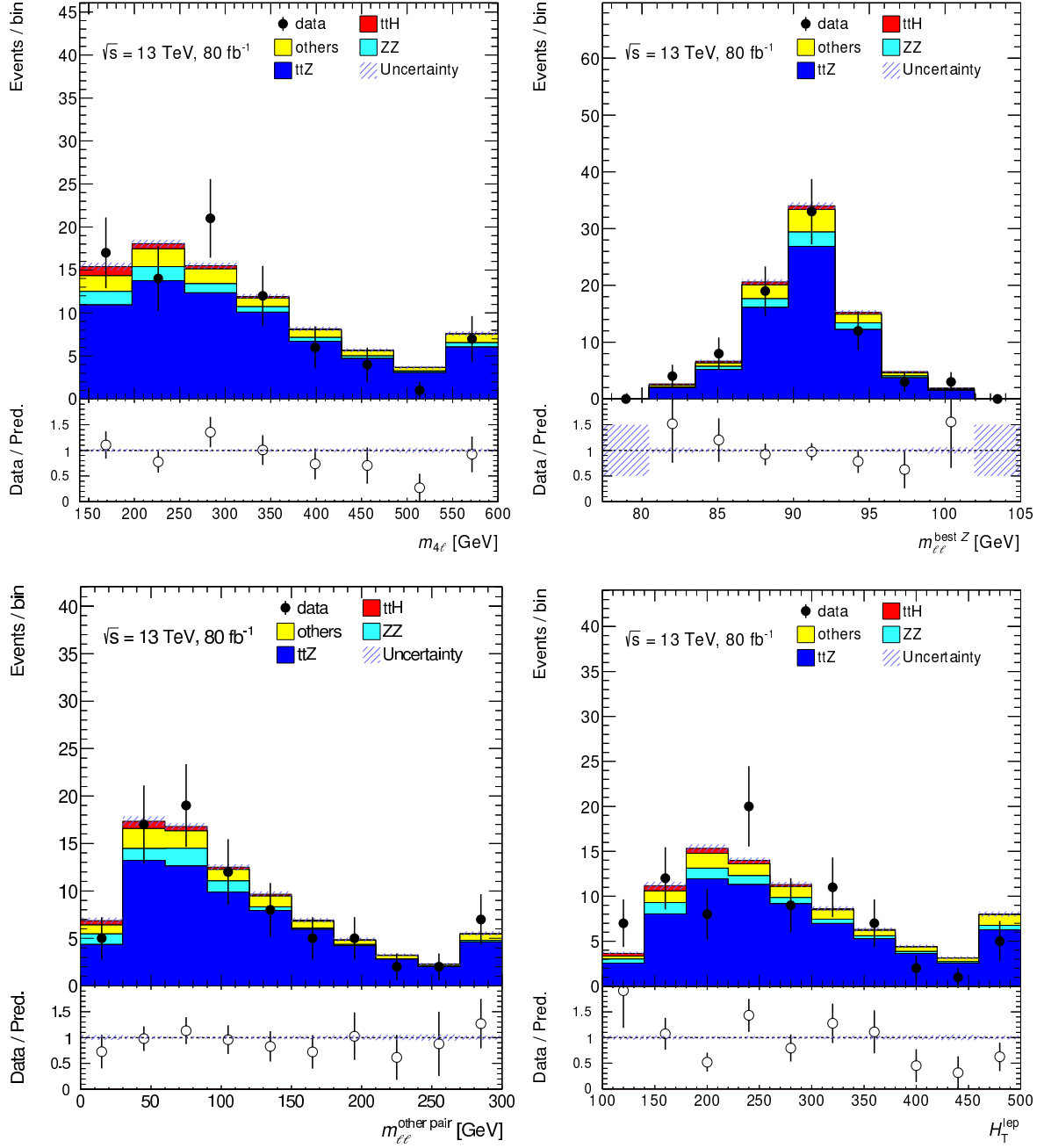
Figure 5.19: Data-to-simulation comparison in the four-lepton t\bar{t}Z control region for four of the input variables to the BDTG training: m_{4\ell} , m_{\ell\ell}^{\text{best } Z} , m_{\ell\ell}^{\text{other pair}} and H_T^{\text{lep}} . The t\bar{t}Z normalisation is scaled by 1.10 to match the number of observed data events. Shown uncertainties are only statistical.
