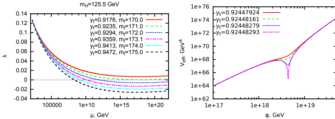
Figure 2.11: Left: RG running of the Higgs-boson self-coupling for several values of the top-quark Yukawa coupling y_t ( \mu = 173.2 GeV) and fixed 125.5 GeV Higgs-boson mass [39]. Right: a very small change in the top-quark Yukawa coupling y_t converts the monotonic behaviour of the effective potential for the Higgs field to that with an extra minimum at large values of the Higgs field [53].
