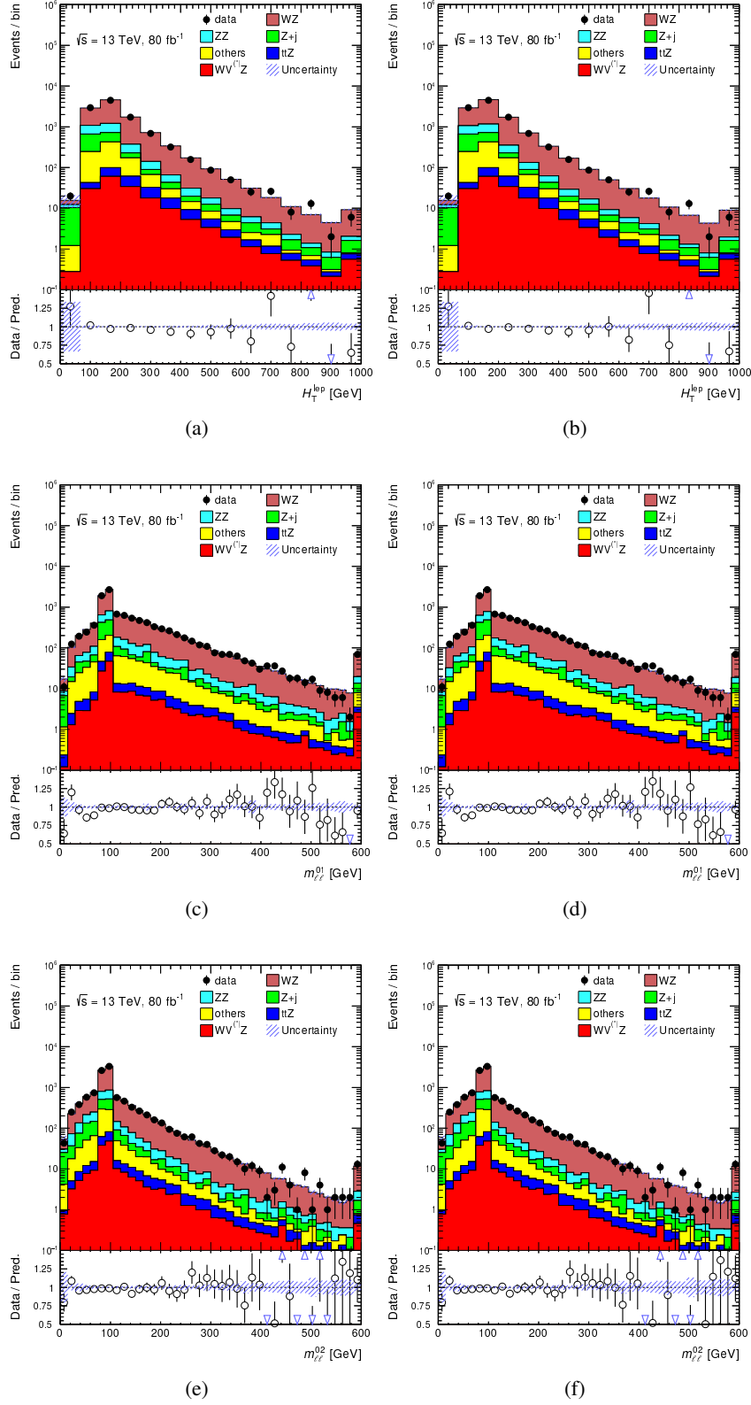
Figure B.2: Data/MC comparison before (left column) and after (right column) reweighting for: (a)(b) H_T^{\text{lep}} , (c)(d) m_{\ell\ell}^{01} and (e)(f) m_{\ell\ell}^{02} . Only statistical uncertainties are shown.
