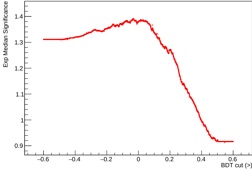
Figure 5.21: Expected median significance for the rejection of the background-only hypothesis as a function of a requirement on the BDTG score in the 4\ell Z-enriched signal region. The significance is compared for 2400 different profile likelihood fits combining both 4\ell signal regions.
