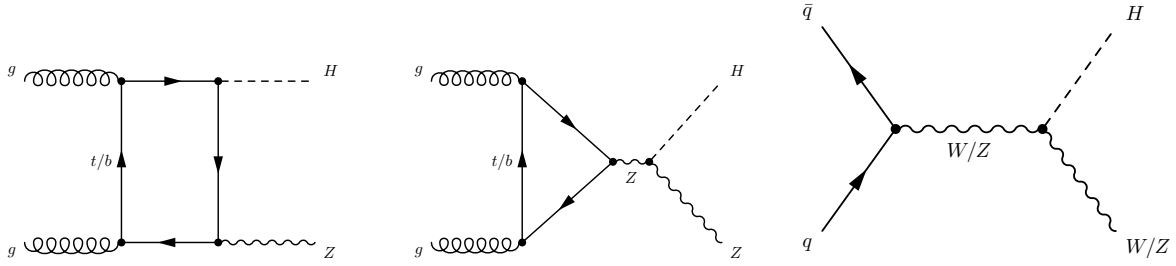
Figure 2.4: Leading order diagrams for the production of a Higgs boson in association with a vector boson.
