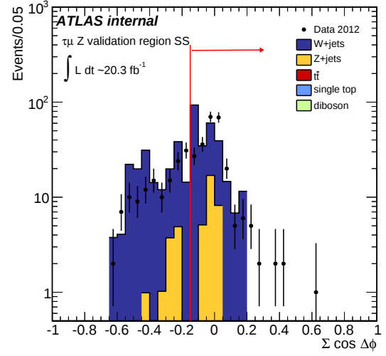
(b) Same Sign
