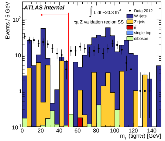
(b) Same Sign
