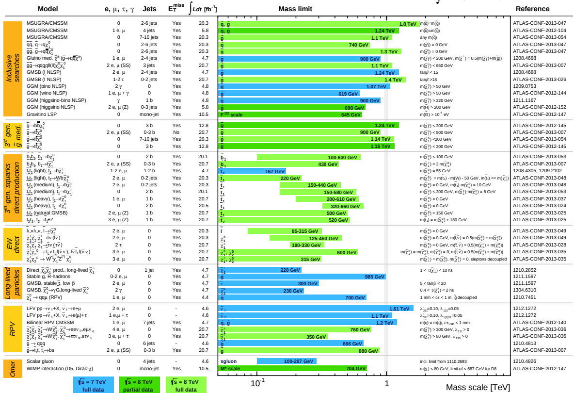
Figure 2.3: Mass reach of ATLAS searches for Supersymmetry [21].
