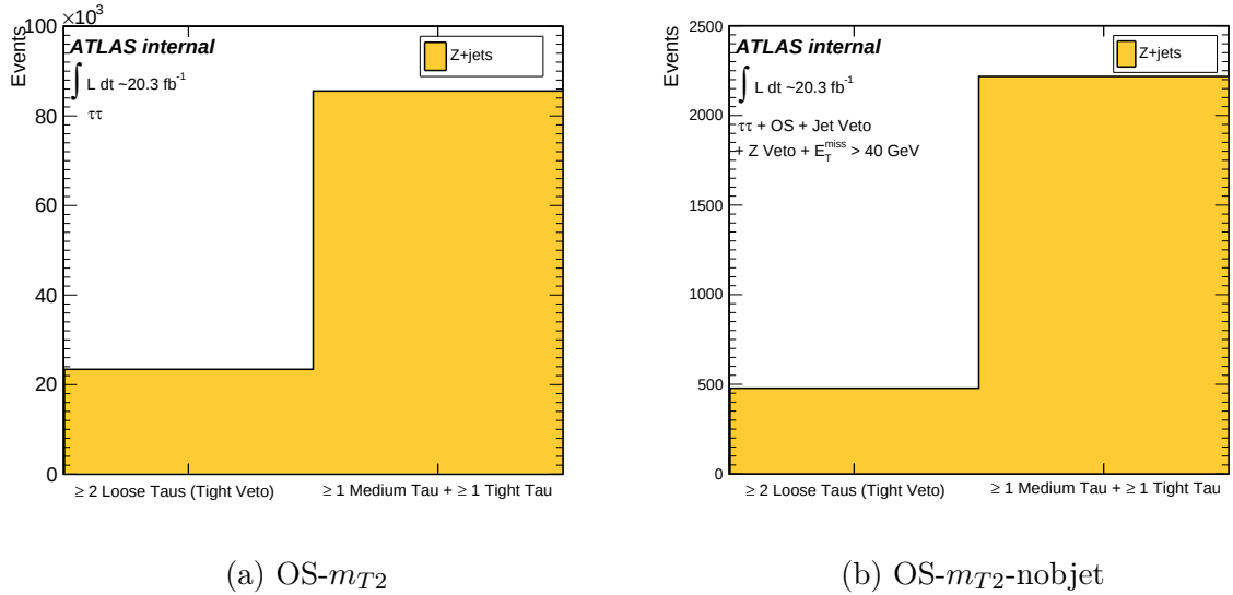
Figure 6.1: Distribution of different tau quality criteria for Monte Carlo generated Z + jets events with the requirement two taus in the event (6.1a) or with the requirements of signal region OS- m_{T2} before the m_{T2} cut (6.1b).
