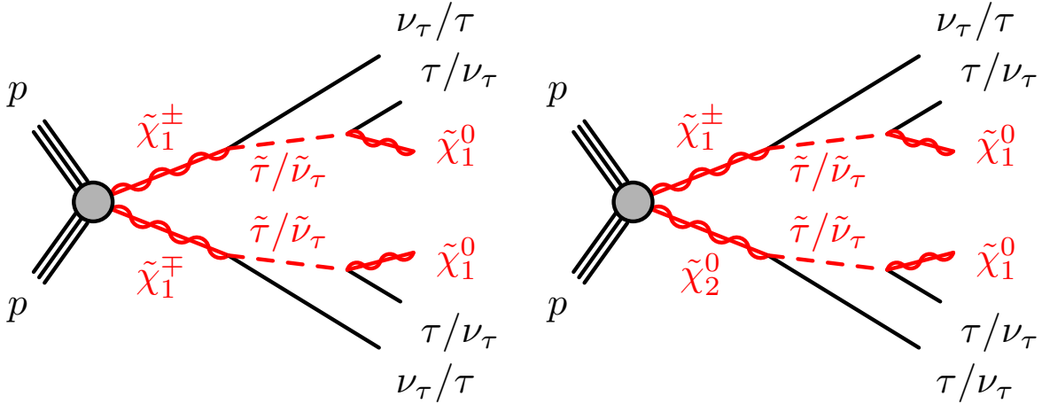
Figure 4.1: Feynman diagram for \tilde{\chi}_1^\pm\tilde{\chi}_1^\mp production (left) and for \tilde{\chi}_2^0\tilde{\chi}_1^\pm production (right), which then decay via an intermediate left-handed stau or stau neutrino.
