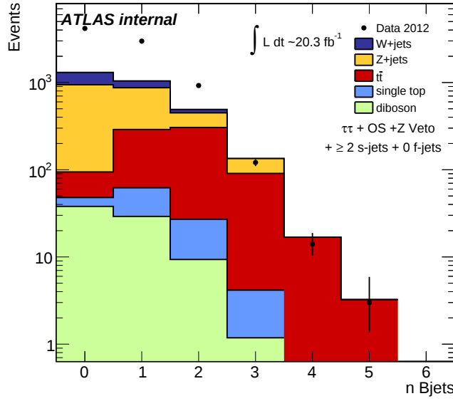
Figure 7.7: Distribution of the number of b-jets. The difference between the data event yield and the stacked simulated background predictions is expected to be from the QCD multi-jet background.
