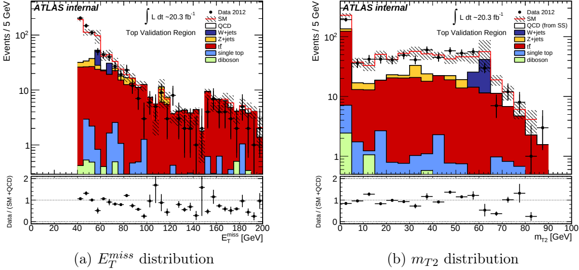
Figure 7.10: Comparison of data and background event yields in the top validation region for the E_T^{miss} distribution (7.10) and the m_{T2} distribution (7.10b). The QCD multi-jet background is estimated from the validation region with same sign requirement.
