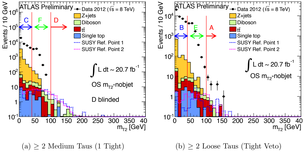
Figure 5.3: m_{T2} distribution for the OS- m_{T2} -nobjjet signal region before applying the m_{T2} cut (5.3a). In (5.3b) the tau identification criteria are changed to \geq 2 loose taus with tight tau veto instead of \geq 1 medium taus and \geq 1 tight taus. The Standard Model backgrounds are stacked. Together the two histograms show the distribution in all regions of the ABCD method for the QCD multi-jet & W + \text{jets} estimation. [38]
