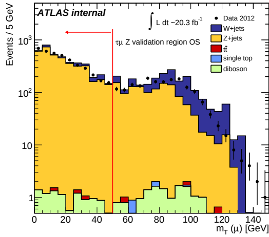
(a) Opposite Sign
