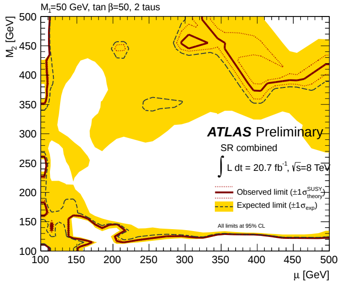
Figure 8.5: 95% CL exclusion limits in the \mu - M_2 mass plane of the pMSSM grid with M_1 = 50 \text{ GeV} , \tan \beta = 50 for the signal region with the best expected limit at each grid point. The black dashed line shows the 95% CLs expected limit. The solid band around the expected limit shows the \pm 1\sigma result where all uncertainties, except those on the signal cross-sections, are considered. The \pm 1\sigma lines around the observed limit represent the results obtained when moving the nominal signal cross section up and down by the \pm 1\sigma theoretical uncertainty. [38]
