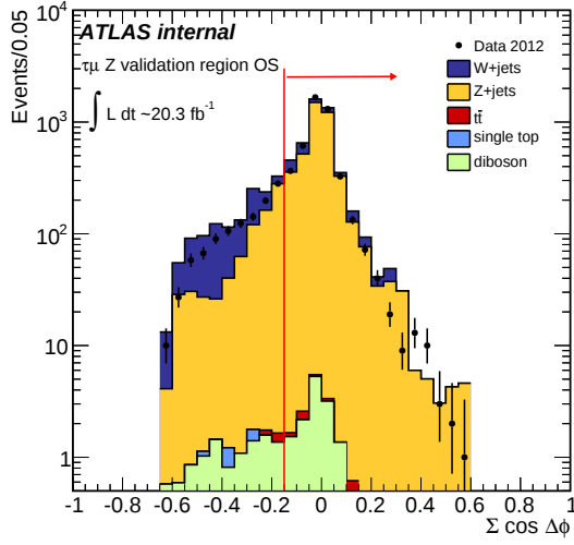
(a) Opposite Sign
