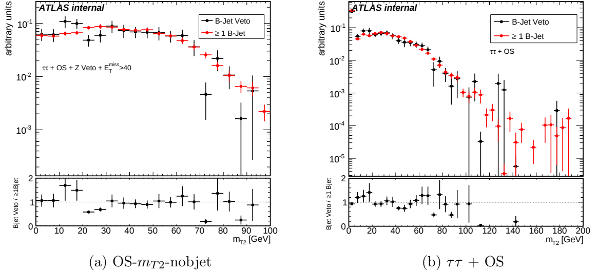
Figure 6.6: m_{T2} distribution for Monte Carlo generated top events with b-jet veto (black) and with \geq 1 b-jet (red) for OS- m_{T2} -nobjjet (6.6a) before the m_{T2} cut and for a looser selection with just a \tau\tau + \text{OS} requirement (6.6b) to compare the shapes with higher statistics. The distributions are scaled to unity to compare the shapes. In the bottom plots the ratio between the distributions is shown.
