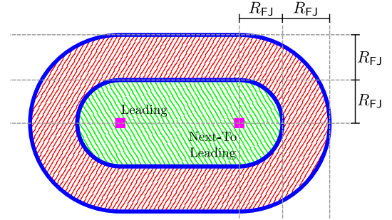
Fig. 7: Schematic drawing of the areas which are used for calculation of E_{IFJ} (hatched green) and E_{CFJ} (hatched red); R_{FJ} is a jet cone parameter (typical R_{FJ} \sim 0.3 ); magenta coloured squares denote position of leading and next-to leading fat-jet subjects.
