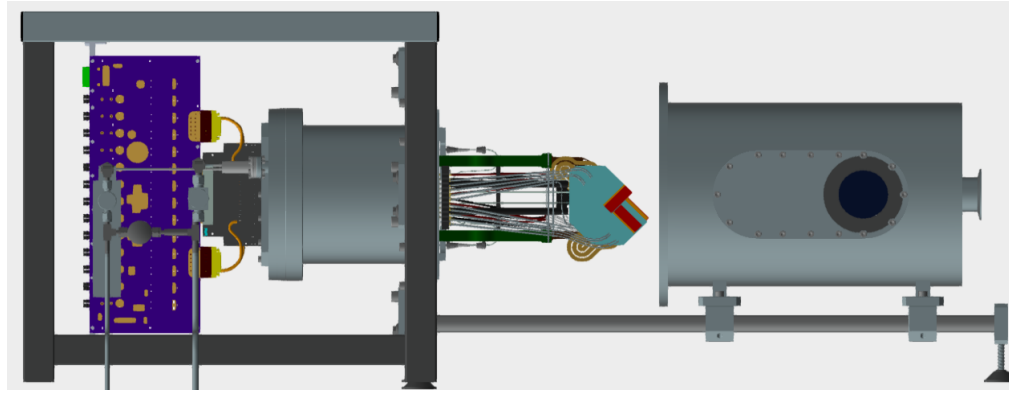
Figure 3.9: CAD model of the module test setup in UoM.
