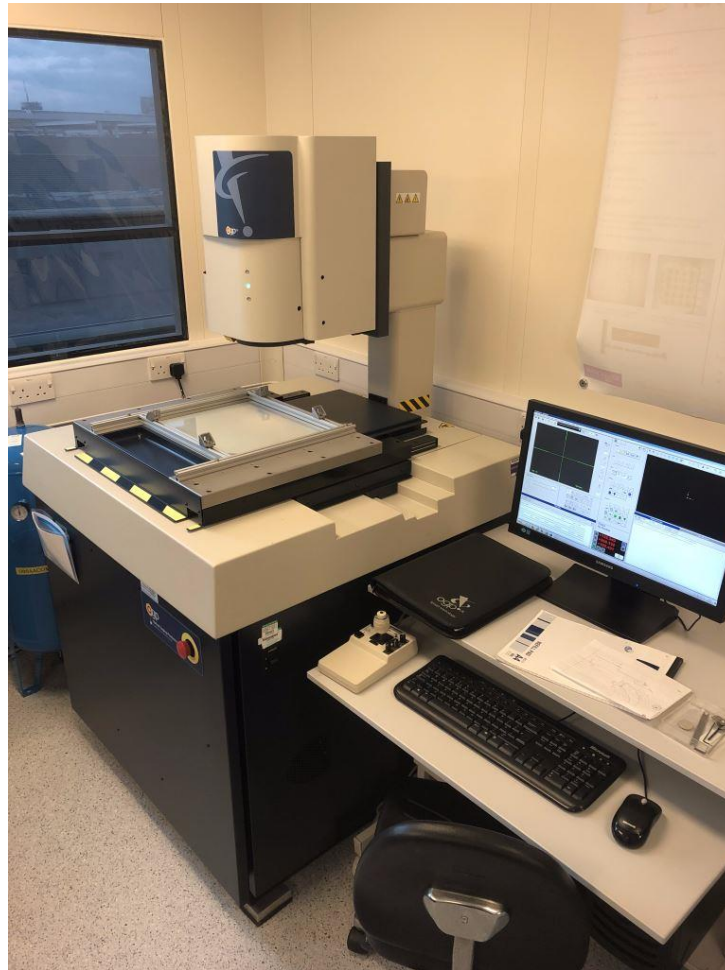
Figure 3.6: SmartScope device with laser and optical sensors used for mechanical measurements.
