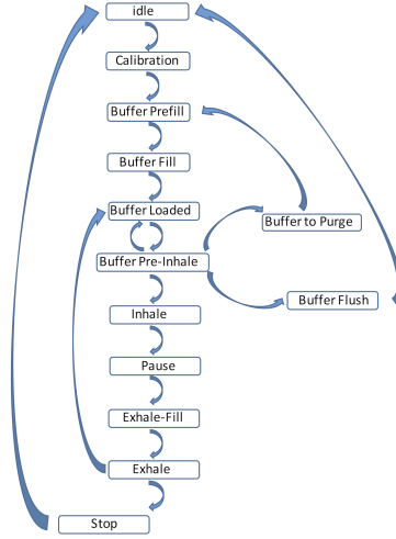
Figure 2: HEV Ventilator State Chart.
