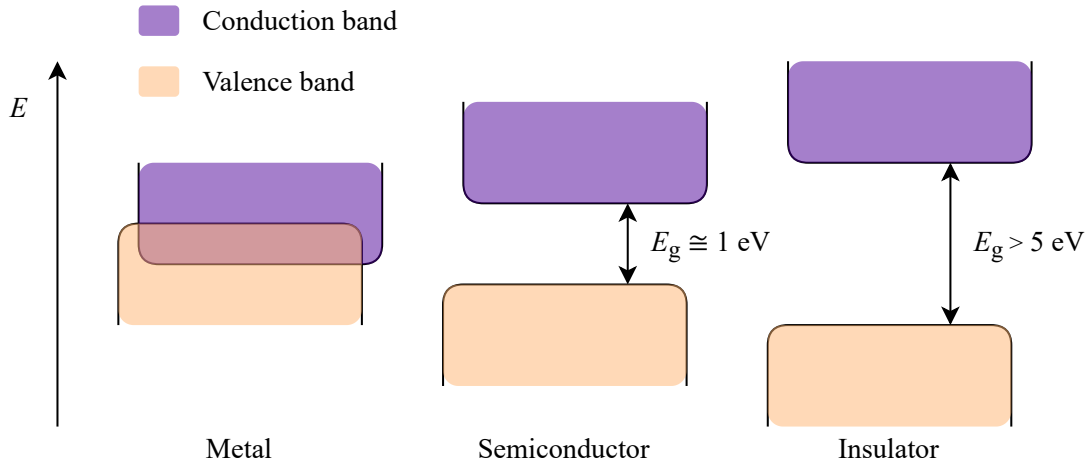
Figure 2.4: Comparison of the band structure for metal, semiconductor and insulator materials.
