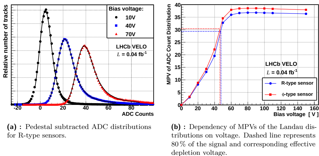
Figure 5.2: Example of the CCE scan for the Run 1 and 2 VELO. [90]
