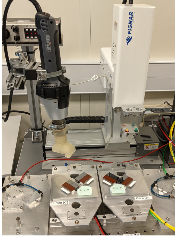
Figure 3.2: Gluing robot Fisnar F5200N with a heat gun.
