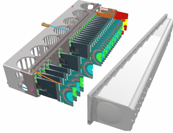
Figure 1.5: Schematic view of VELO modules with the RF box. [15]
