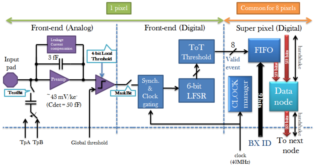
Figure 1.20: Schematic of the pixel architecture. [40]
