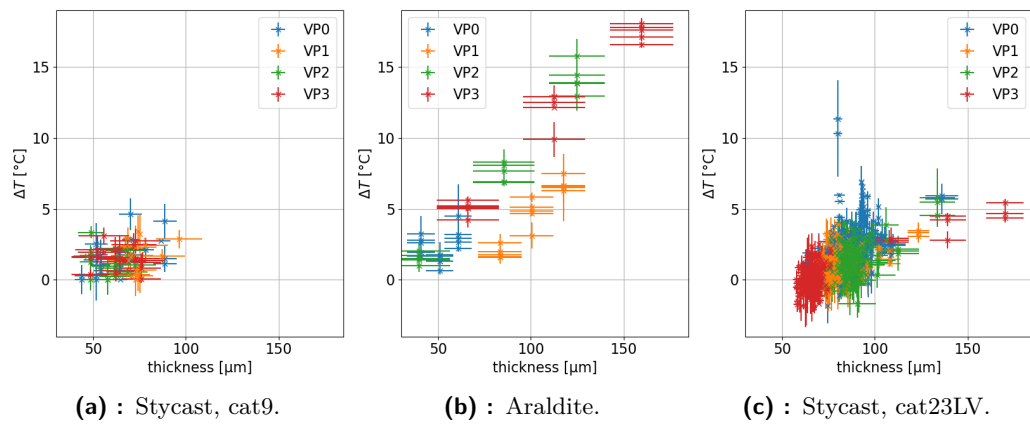
Figure 4.24: Comparison of the cooling performance based on the glue layer thickness.
