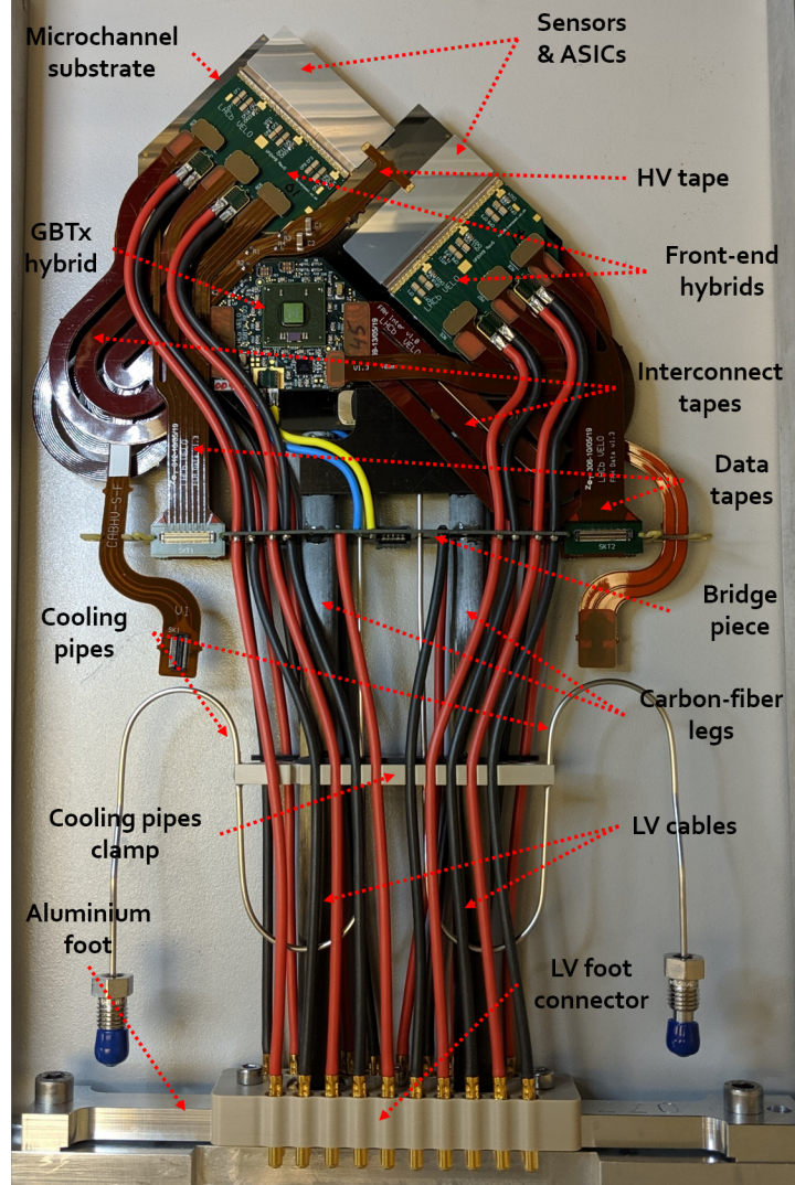
Figure 1.18: Fully assembled VELO module.
