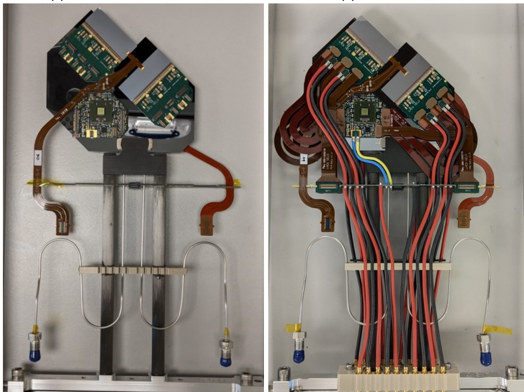
(c) : Hybrid attachment and wire-bonding.
