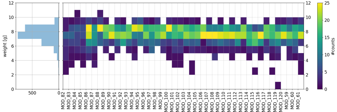
Figure 4.12: Trend of all pull test forces.
