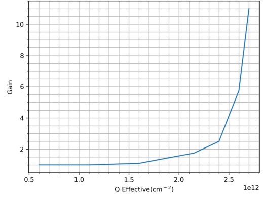
Figure 6.6: Simulation results of dependency of LGAD gain on Q-effective for 400 V reverse bias. [110]
