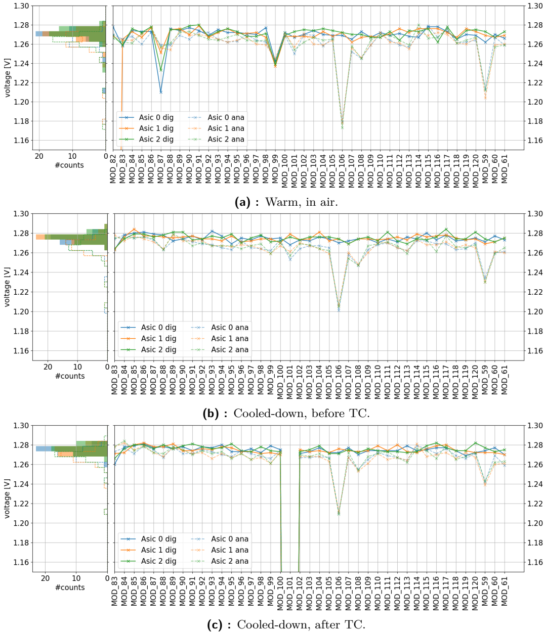
Figure 4.15: Trend of analogue and digital voltage during communication tests of NSI (VP2) tile.
