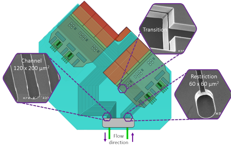
Figure 1.16: Final design of the silicon cooling substrate with visualised position of the channels and front-end readout electronics. [38] The embedded images show detailed photographs of various channel regions provided by ©CEA.
