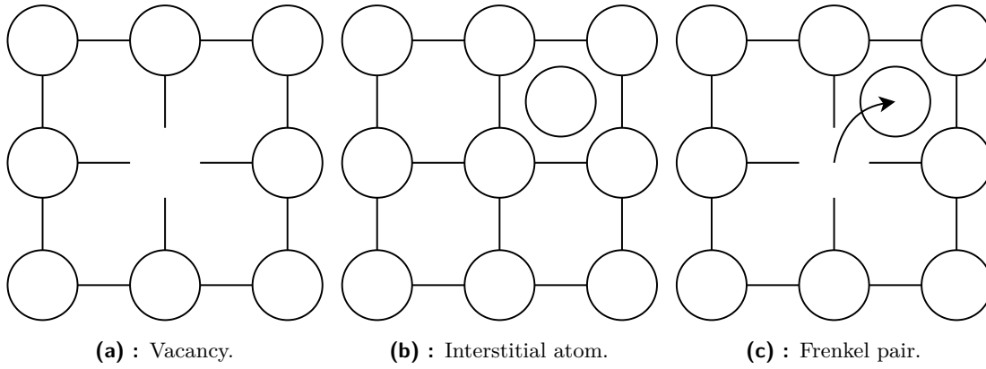
Figure 2.11: Visualisation defects in the crystal lattice.
