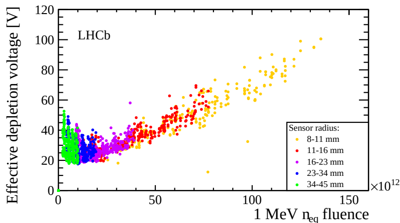
Figure 5.1: Dependency of effective depletion voltage on fluence for the Run 1 and 2 VELO sensors. Results after the end of Run 1 with total integrated luminosity 3.4 \text{ fb}^{-1} . [22]
