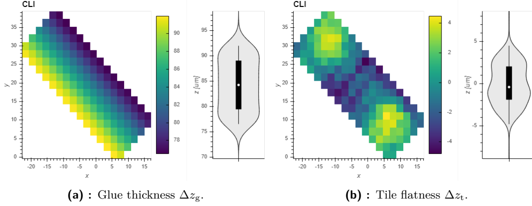
Figure 4.5: Measurement of glue layer thickness and tile flatness of CLI, MOD_120. Heatmaps show the spatial profile of \Delta z_{g(t)} , the violin plots show the distribution, highlighting quartiles. Overhanging regions are plotted in both cases, visually worsening the glue thickness profiles.
