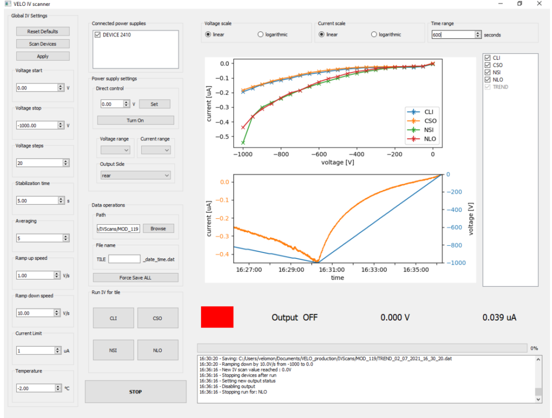
Figure 3.18: Screenshot of the software developed for controlling the PSU.
