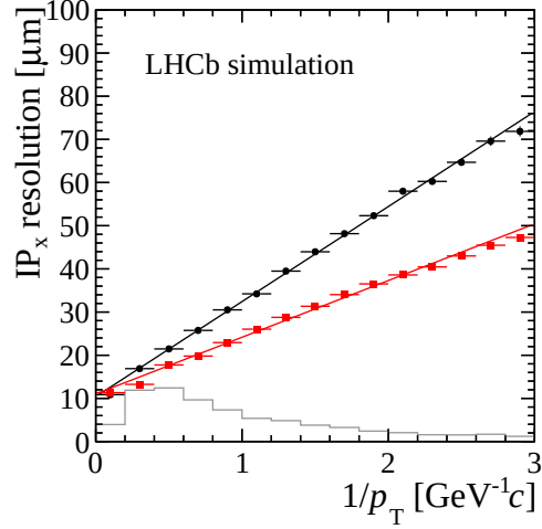
Figure 1.14: Simulated IP_x resolution of VELO and VELO Upgrade as a function of inverse momentum. The black and red points correspond to the old and upgrade detector, respectively. [24]
