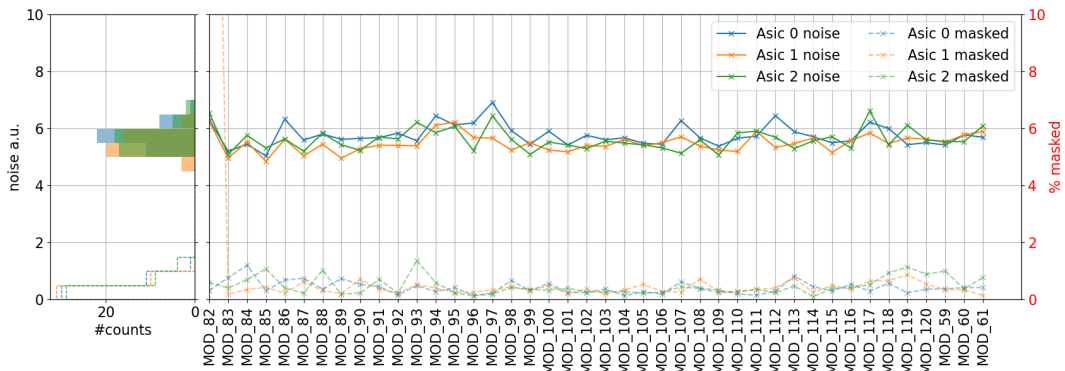
Figure 4.21: Trend of mean noise and percentage of masked pixels in VeloPix ASICs, shown for NSI (VP2) after TC.
