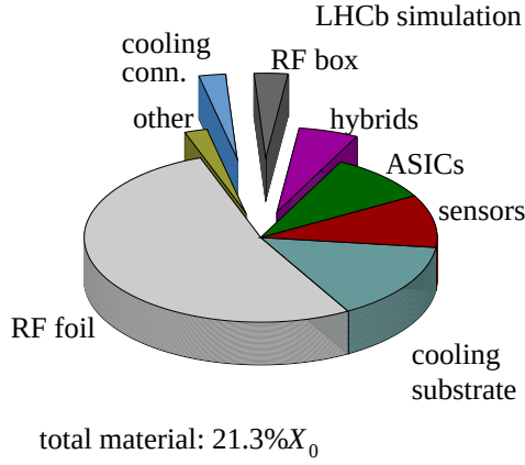
Figure 1.13: Material budget of the VELO Upgrade. [24]
