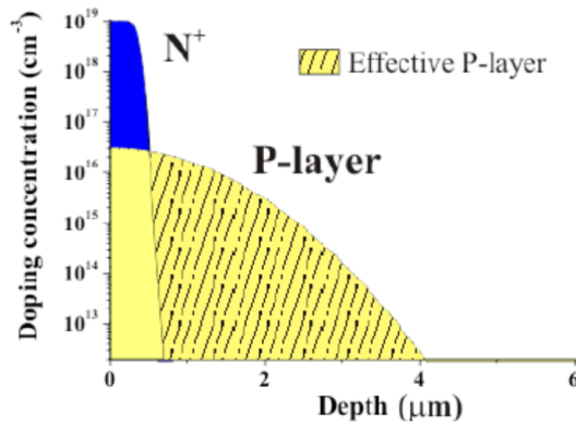
Figure 6.5: Q-effective representation from doping profile of LGAD. [111]
