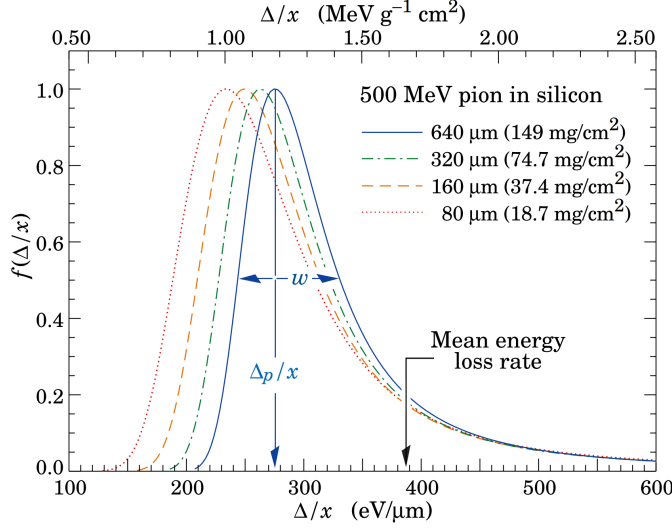
Figure 2.2: Probability of energy loss interactions for 500 MeV pions in silicon, \Delta_p represents the most probable value. A broadening of the distribution following the decrease of the silicon thickness is visible, best described by Straggling functions. [52, 55]
