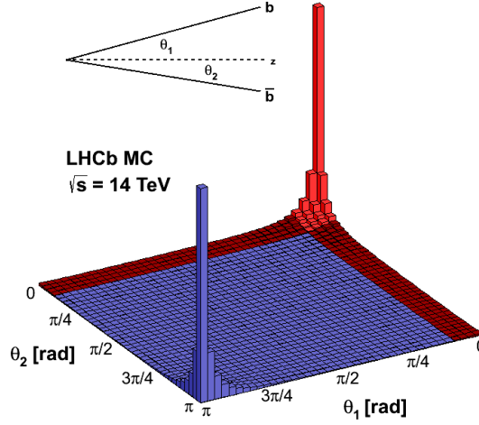
Figure 1.3: The angular distribution of b\bar{b} pair production. The red region represents the LHCb acceptance. [18]
