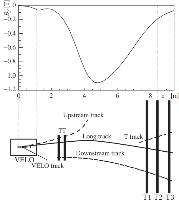
Figure 1.6: Intensity of the magnetic field for trackers. [25]
