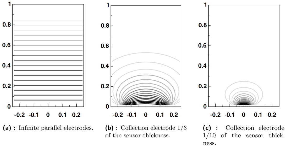
Figure 2.10: Comparison of the weighting field for a planar and segmented device based on the electrode size. [62]
