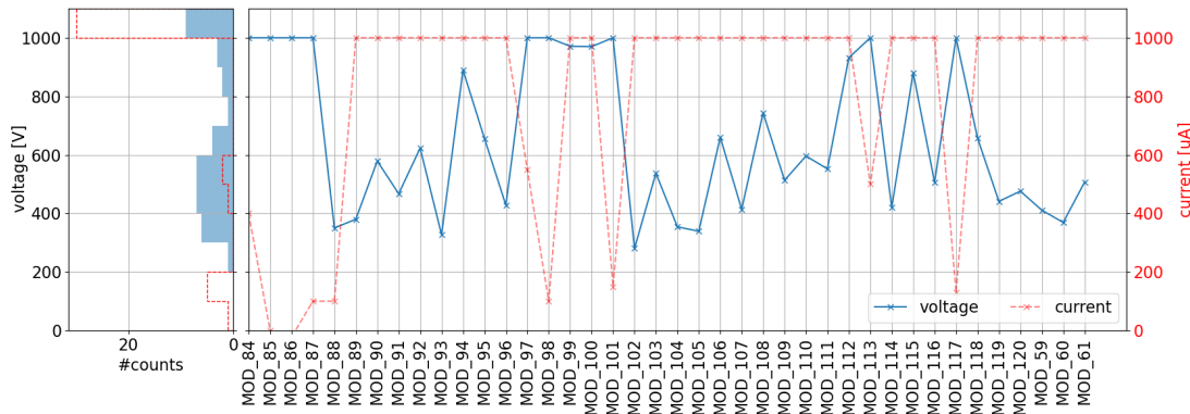
Figure 4.29: Trend of ramp-up results for NLO (VP1) tile.
