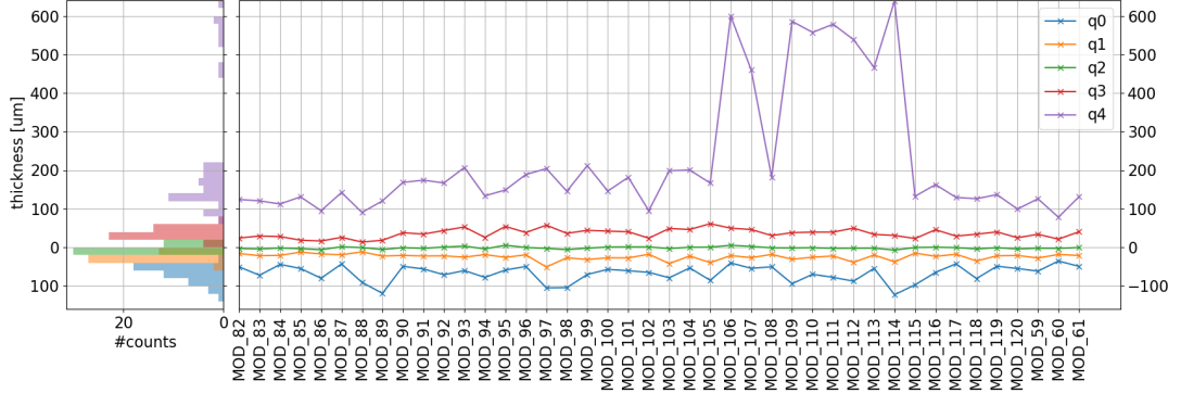
Figure 4.4: Trend of substrate flatness results, showing the quartiles of the \Delta z distribution.
