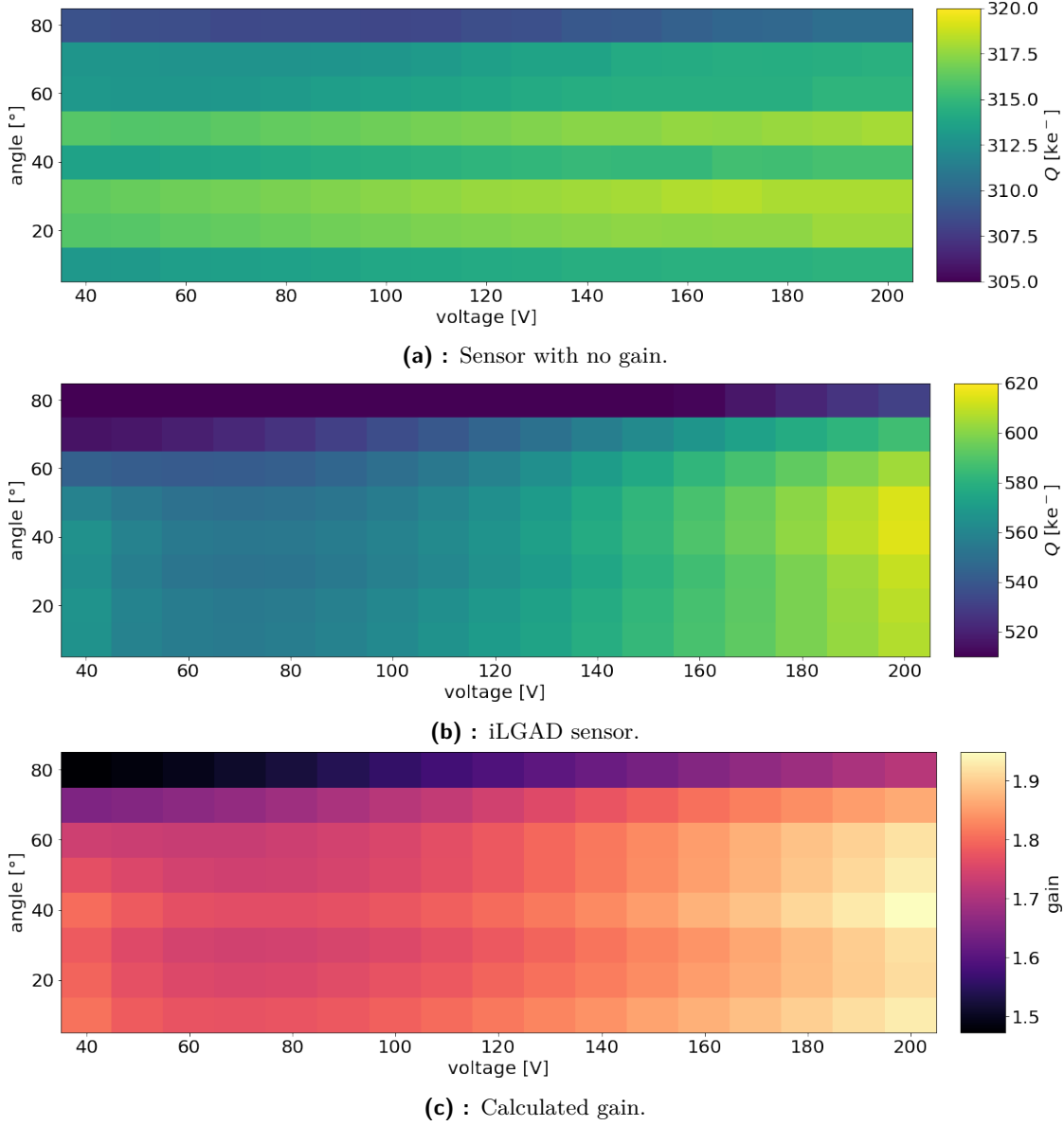
Figure 6.22: Comparison of the collected charge Q for sensors without gain and iLGADs, based on the bias voltage and incidence angle of the proton beam of energy 1.6 MeV.
