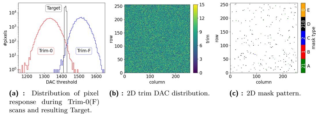
Figure 4.19: Example of equalisation results for NSI (VP2). Scan done after TC in MOD_103.
