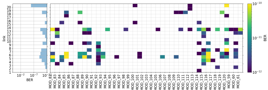
Figure 4.18: Trend of PRBS test BER from before TC. White means no errors detected in the 1 \cdot 10^{12} bits tested.
