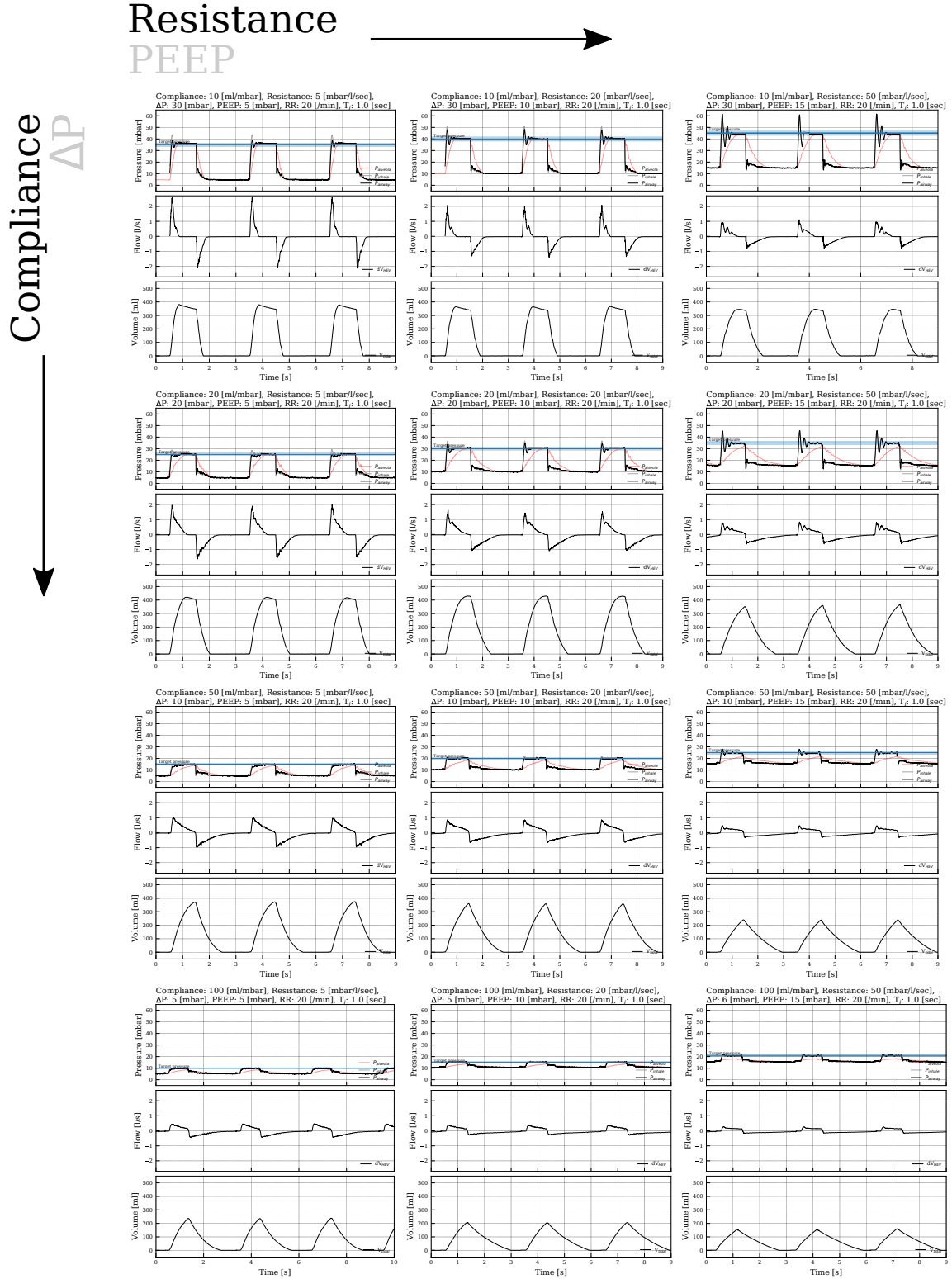
Figure 16: Pressure, flow and volume registered for patient configurations with increasing lung compliance and airway resistance. As expected, the flow is more peaked with reduced resistance and compliance.
