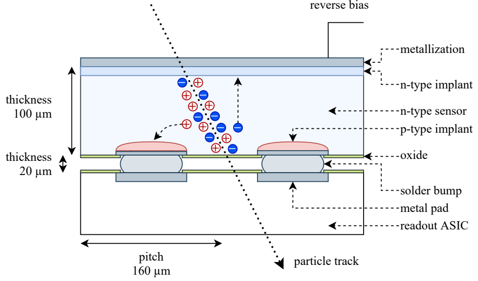
Figure 2.9: Schematic cross-section of a hybrid pixel detector.
