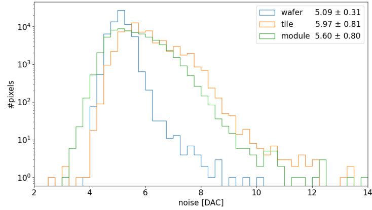
Figure 4.20: Comparison of noise results in NSI (VP2) for different tests. The tile is used in MOD_103.
