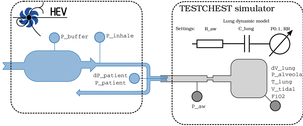
Figure 13: Test setup schematics.
