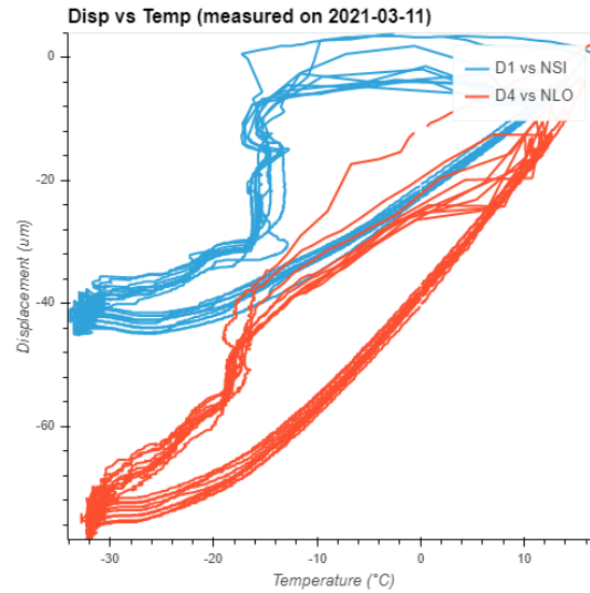
(c) : Correlation of displacement and temperature from 10 cycles.
