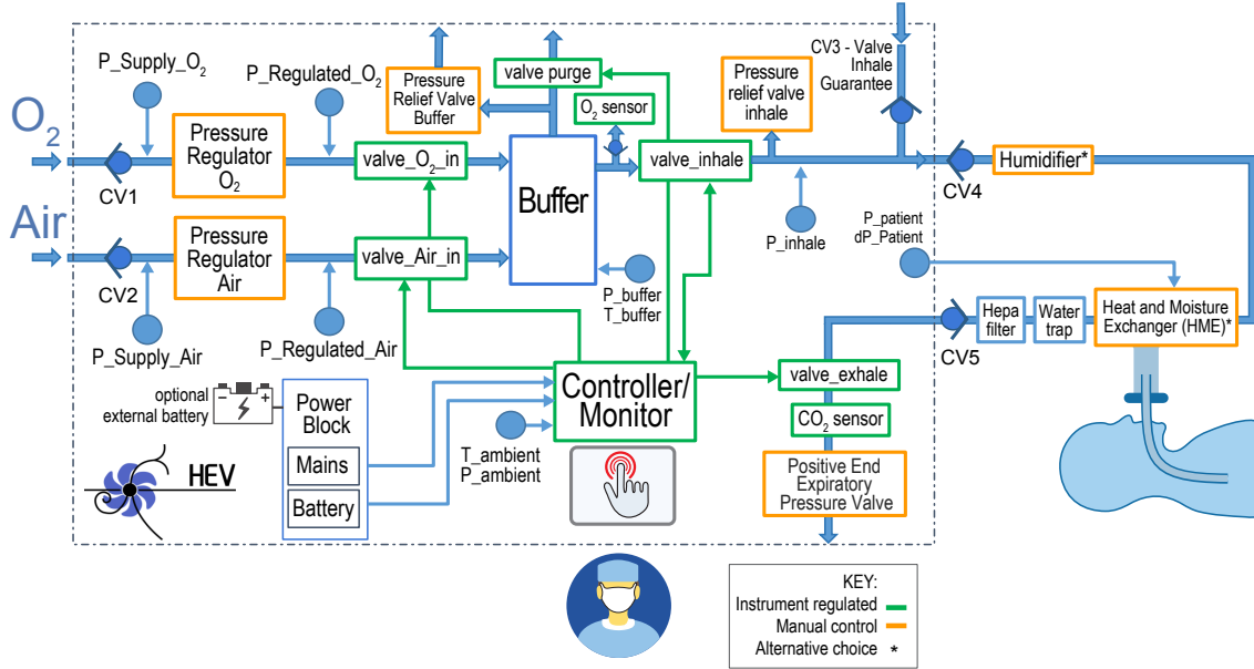
Figure 1: Conceptual design of the HEV ventilator.
