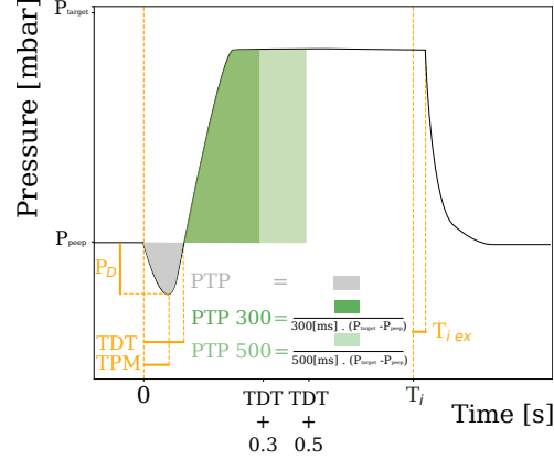
Figure 17: Measured parameters to qualify the inhalation trigger. The variables used in this work are based on the work presented in [34] and [35]
