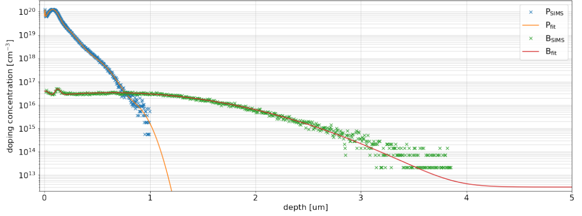
Figure 6.9: Approximation of the process simulation data of n-implant (phosphorus) and p-multiplication (boron). The data points compare the result of the SIMS process of an older sensor production run and the approximated analytical fits.
