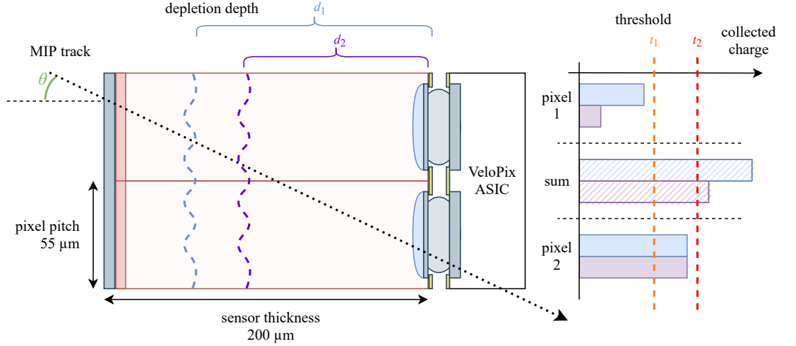
Figure 5.4: Schematic view of a MIP traversing two pixels under an angle \theta . Dependency of the collected charge based on the depletion depth d is visualised on the right side. Since the signal is discriminated on a per-pixel basis, the threshold t affects the amount of reconstructed charge as it does not follow the sum of the two pixels.
