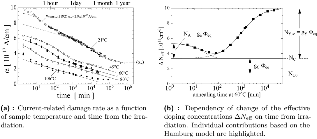
Figure 2.16: Annealing behaviour of selected detector properties [75].
