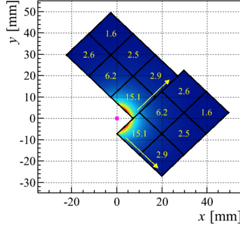
Figure 1.22: Simulation of the expected data rates (Gbit/s) in the VeloPix ASICs. [43]
