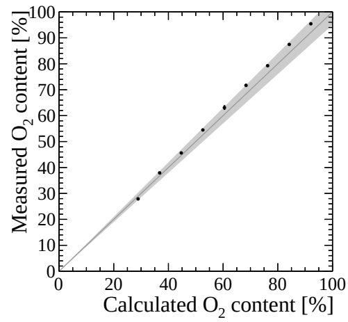
Figure 18: Measured FIO 2 as function of the expected O 2 percentage as calculated from the relative time opening of valve_O 2 _in and valve_Air_in . The grey band represents the region within \pm 5\% of the set value.
