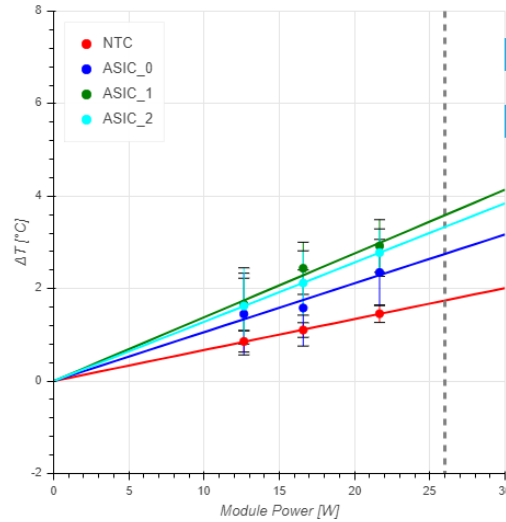
(b) : Fitted cooling performance of the CLI (VP0) tile.
