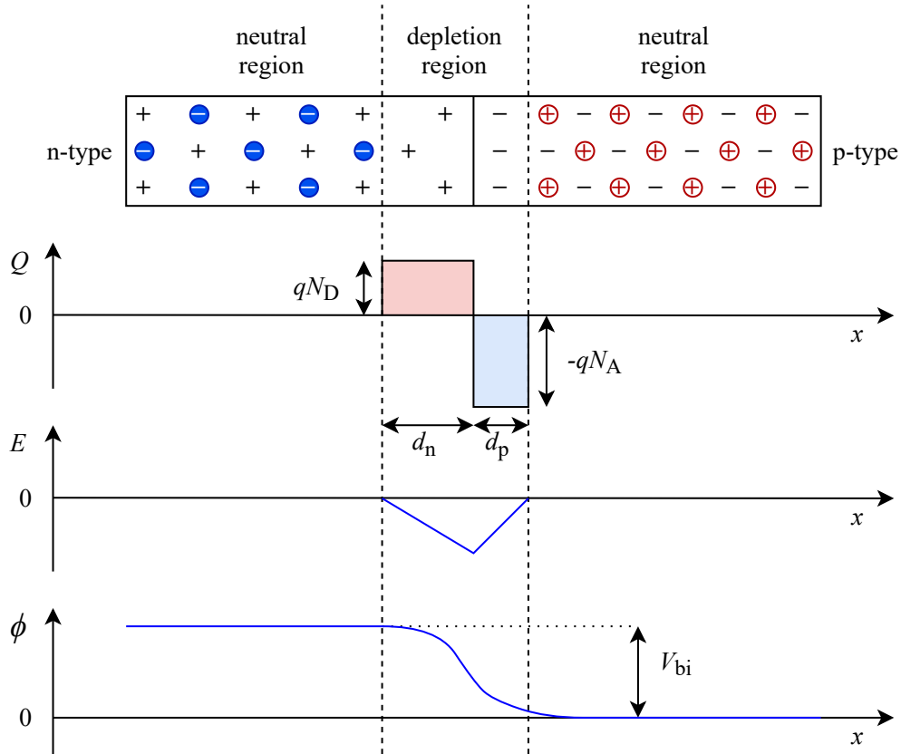
Figure 2.7: Schematic visualisation of the p-n junction.
