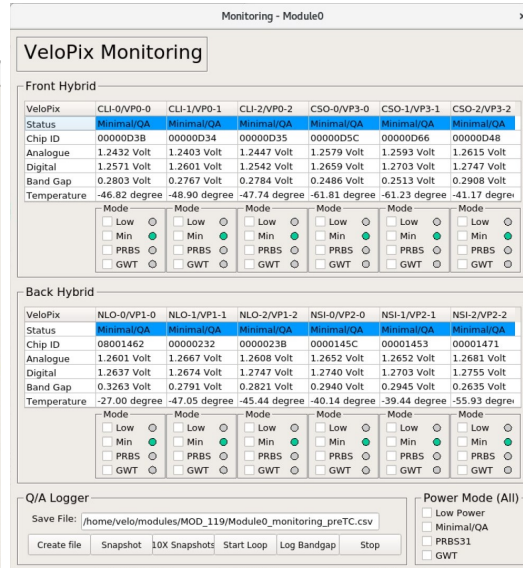
Figure 3.14: Module monitoring panel. Used for communication and cooling performance tests.
