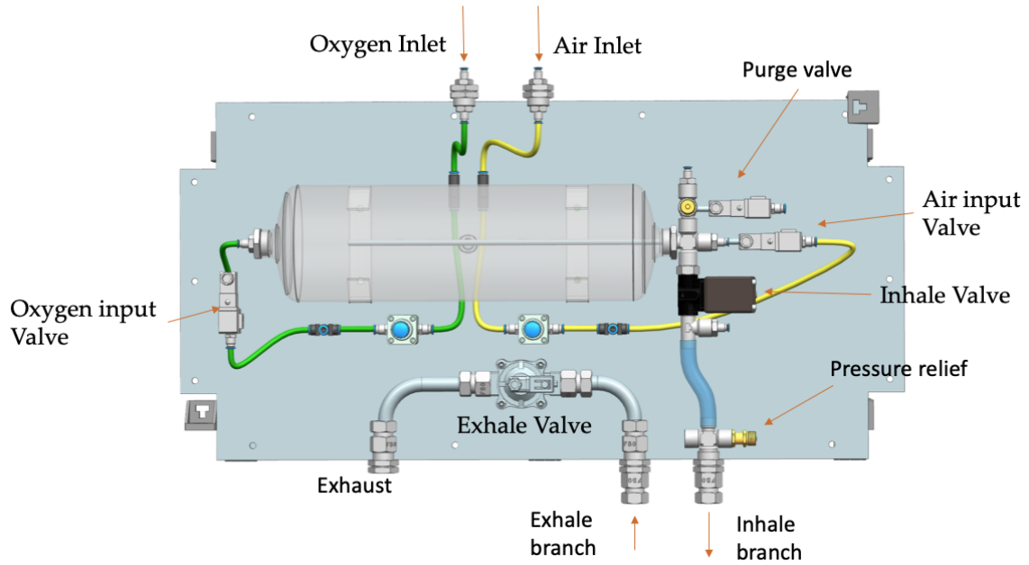
Figure 3: Schematic of the pneumatic part of the HEV system.
