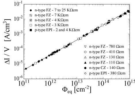
Figure 2.13: Dependency of leakage current on the neutron fluence equivalent for different silicon resistivity and doping. Measured right after the irradiation. [75]
