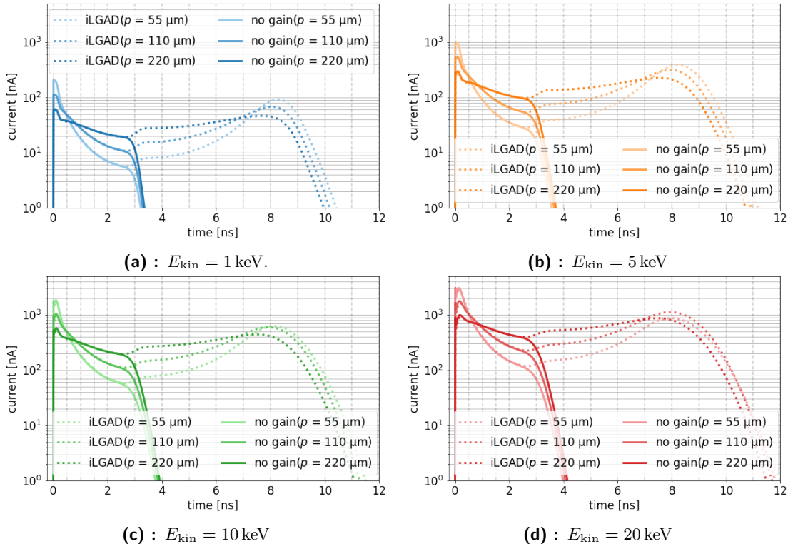
Figure 6.15: Current profiles registered by the central electrode of 250 \mu\text{m} thick sensors. The vertical lines correspond to the 2D profiles shown in the Figs. 6.13 and 6.14.
