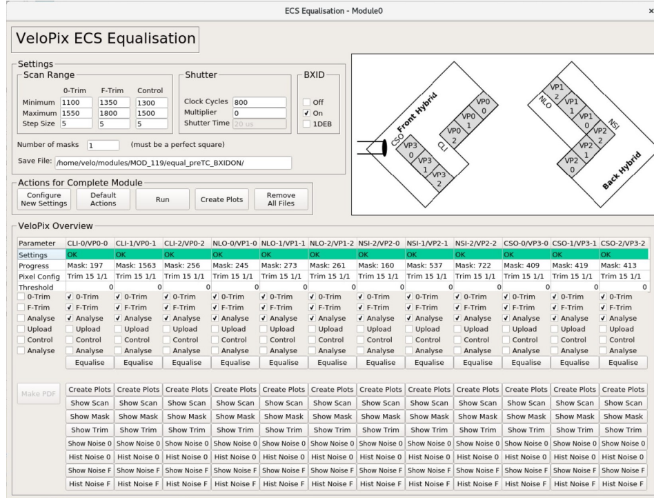
Figure 3.17: Module noise and equalisation panel.
