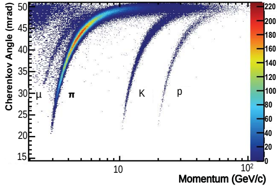
Figure 1.8: Reconstructed Cherenkov angle for isolated tracks based on the particle momentum in the C_4F_{10} radiator. [23]
