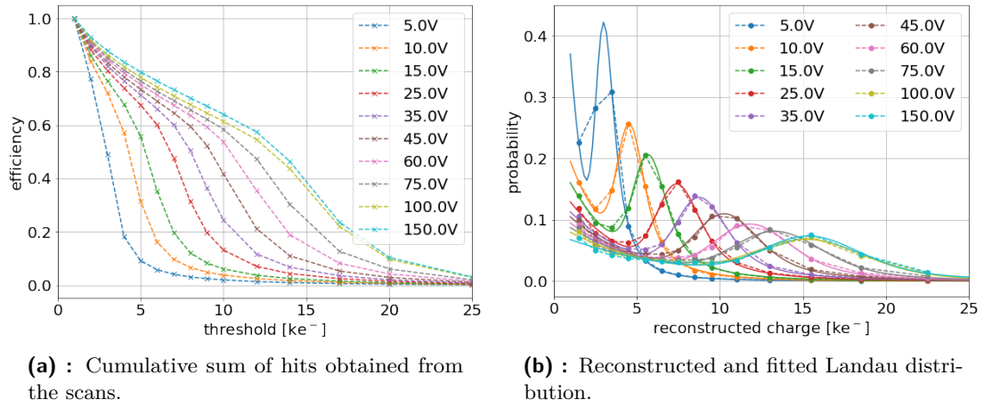
Figure 5.7: Simulation results of a threshold scan for non-irradiated VELO sensors, made for different bias voltages. Data are normalised based on the cumulative sum. The lines for 100 V and 150 V overlap due to reaching maximal depletion.
