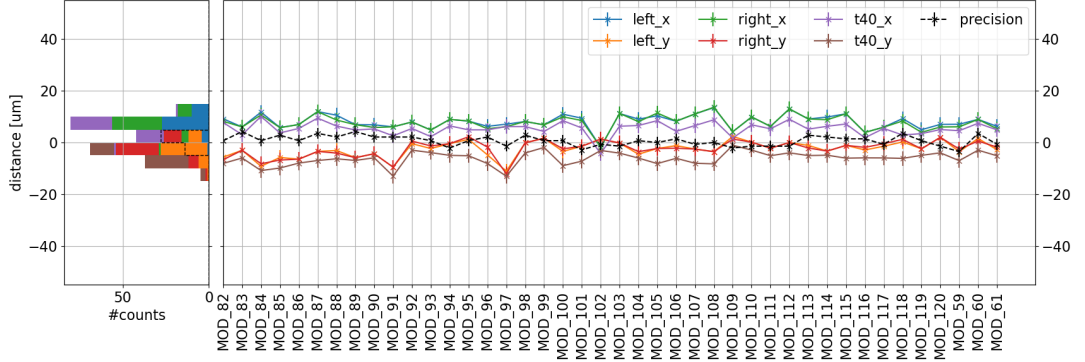
(a) : Difference between the ideal and measured distance of the corner fiducials.
