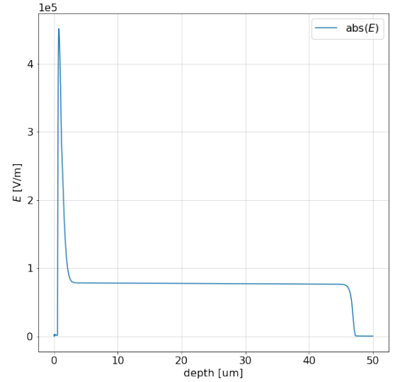
Figure 6.11: Absolute electric field profile of the simulated iLGAD with thickness 50 μm. A high field region is visible in the multiplication layer in the first few μm.
