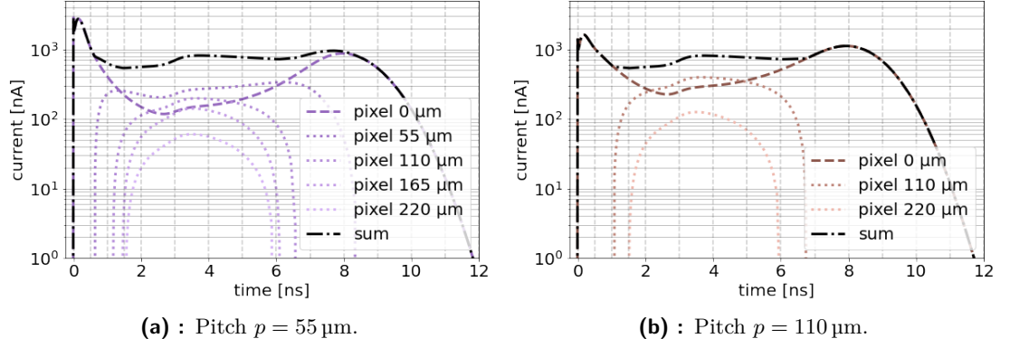
Figure 6.17: Induced current of the neighbouring channels for a different distance from the central point. Because of the symmetry around zero, the channel response is summed.
