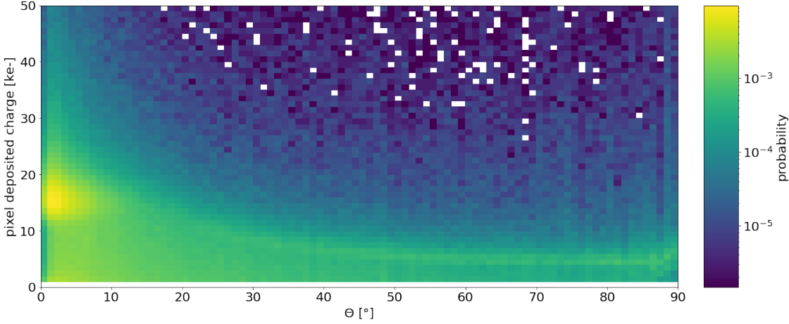
Figure 5.5: Angular dependency of the pixel collected charge, obtained at 100 V, full depletion of the simulated sensors. A visible decrease of the per-pixel deposited charge may be observed with an increasing impact angle.
