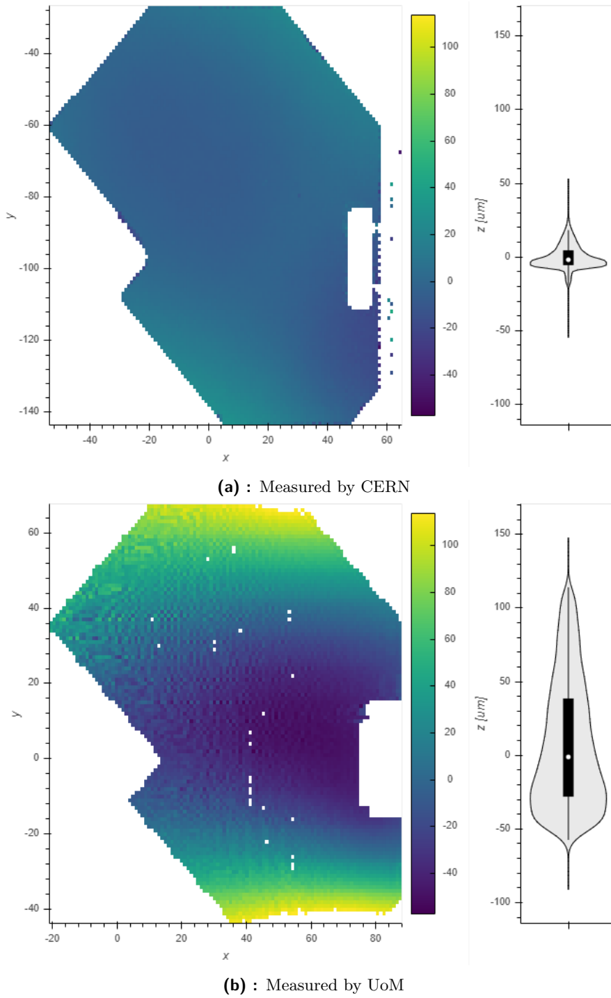
Figure 4.3: Comparison of substrate flatness measurements performed by CERN and UoM on SUB79, used in MOD_100. Left plots are x, y maps of \Delta z and the right violin plots show \Delta z distribution, highlighting median and quantiles.
