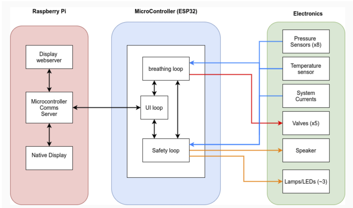
Figure 7: Diagram of the location of the different elements of hardware and software in the two computers (Microcontroller and Raspberry Pi) and the circuit board attached to the Microcontroller.
