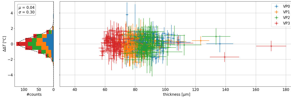
Figure 4.26: Dependency of thermal degradation on glue layer thickness after TC. The glue used was Stycast catalyst 23LV.
