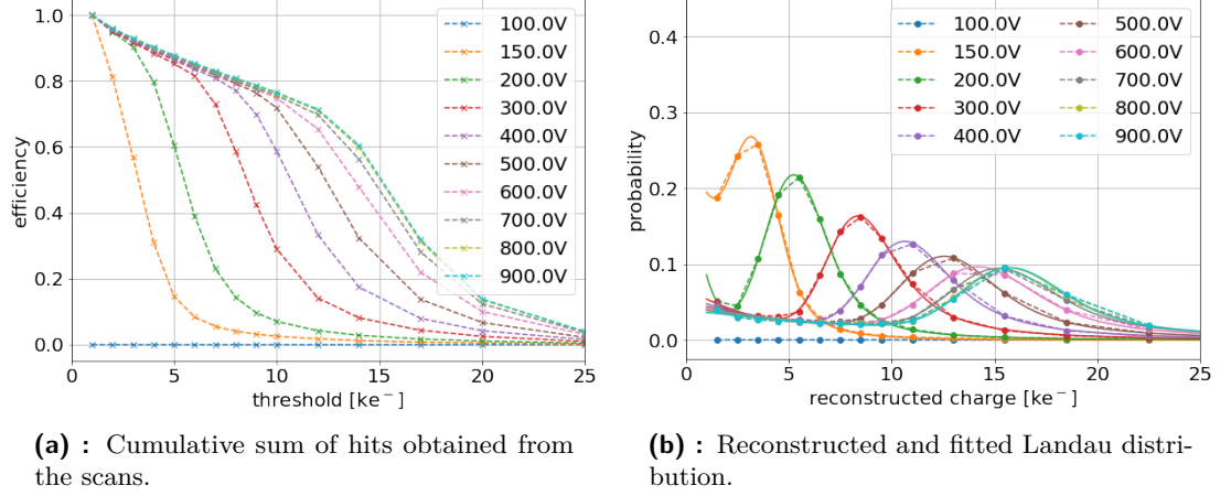
Figure 5.8: Simulation results of a threshold scan for irradiated VELO sensors, made for different bias voltages. Data are normalised based on the cumulative sum, the simulated fluence is in range 0.5 \cdot 10^{15} \text{ 1 MeV n}_{\text{eq}} \text{ cm}^{-2} to 1 \cdot 10^{15} \text{ 1 MeV n}_{\text{eq}} \text{ cm}^{-2} .
