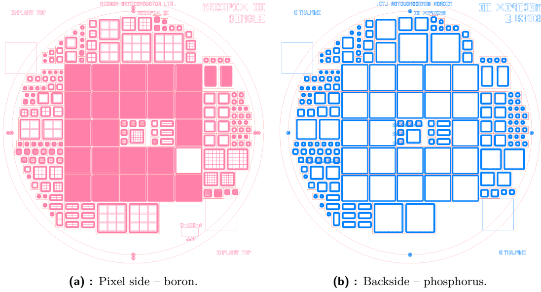
Figure 6.8: Implant masks used for the implantation in the recent iLGAD sensors run, produced by collaboration between the UoG, the UoM and Micron.
