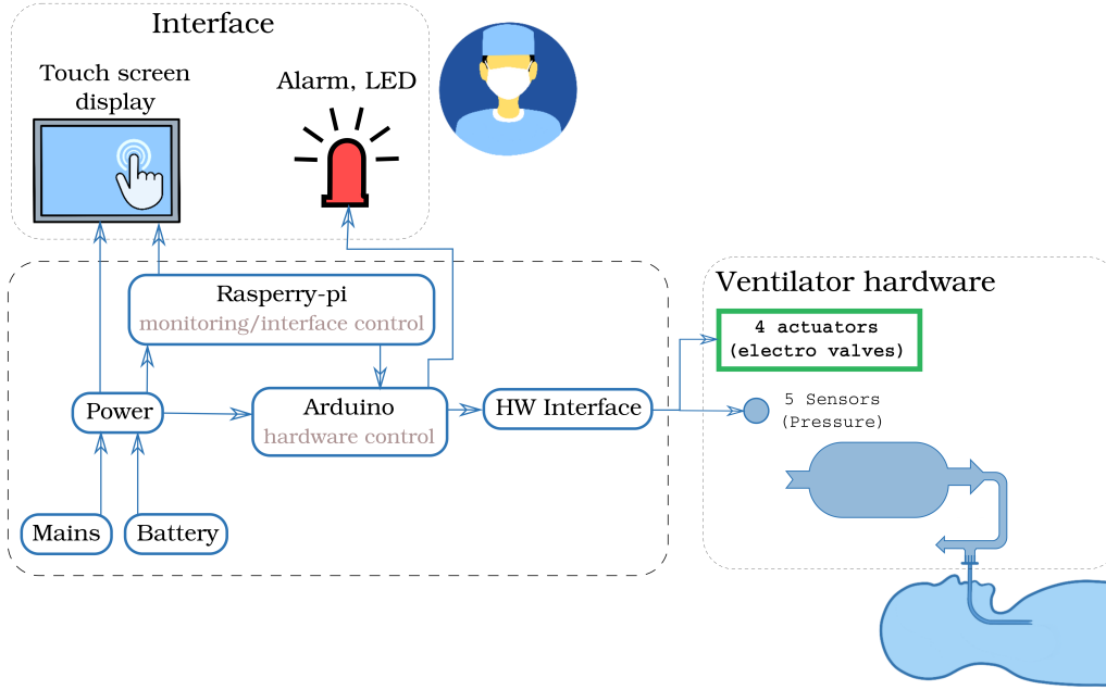
Figure 6: Conceptual layout of the controls and user interface.
