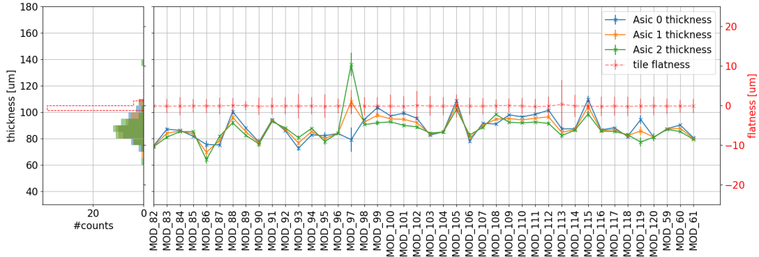
Figure 4.6: Trend of CLI (VP0) tile mean glue thickness and mean tile flatness results.
