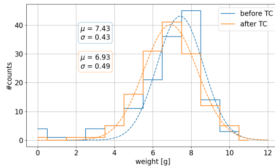
Figure 4.11: Distribution of pull test strengths before and after TC.
