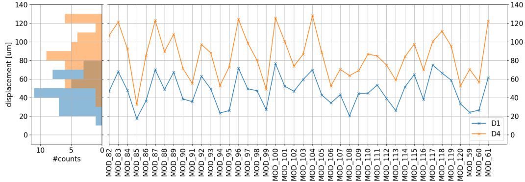
Figure 4.13: Trend of the maximal displacement during the module cool-down.
