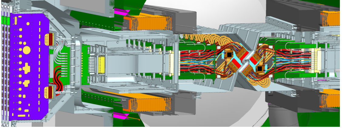
Figure 1.12: VELO Upgrade detector visualisation. The main components being: sensors (red), microchannels (blue), RF foil (grey), OPB (purple). [35]
