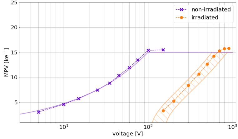
Figure 5.9: Dependency of the MPV from the Landau fit on voltage for normal and irradiated sensors. The solid line and filled region represents the underlying input of the simulation.
