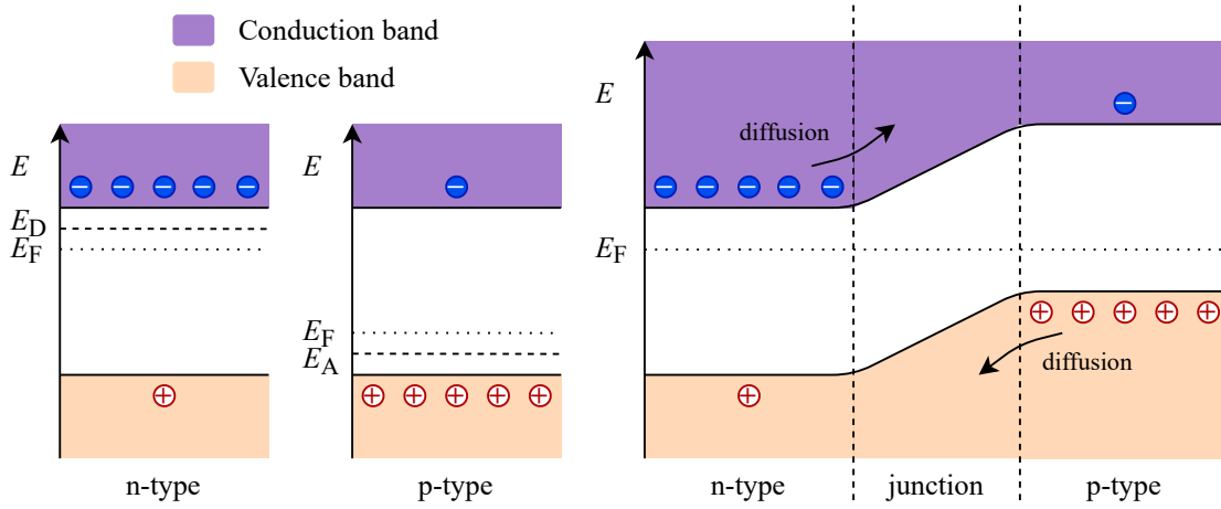
Figure 2.7: Schematic visualisation of the p-n junction.
