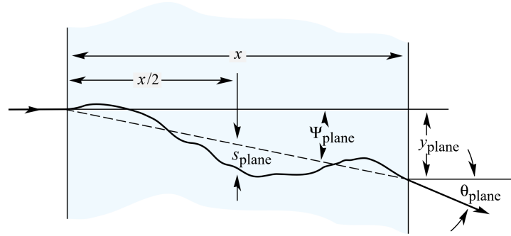
Figure 2.3: Schematic visualisation of the Coulomb scattering. [52]
