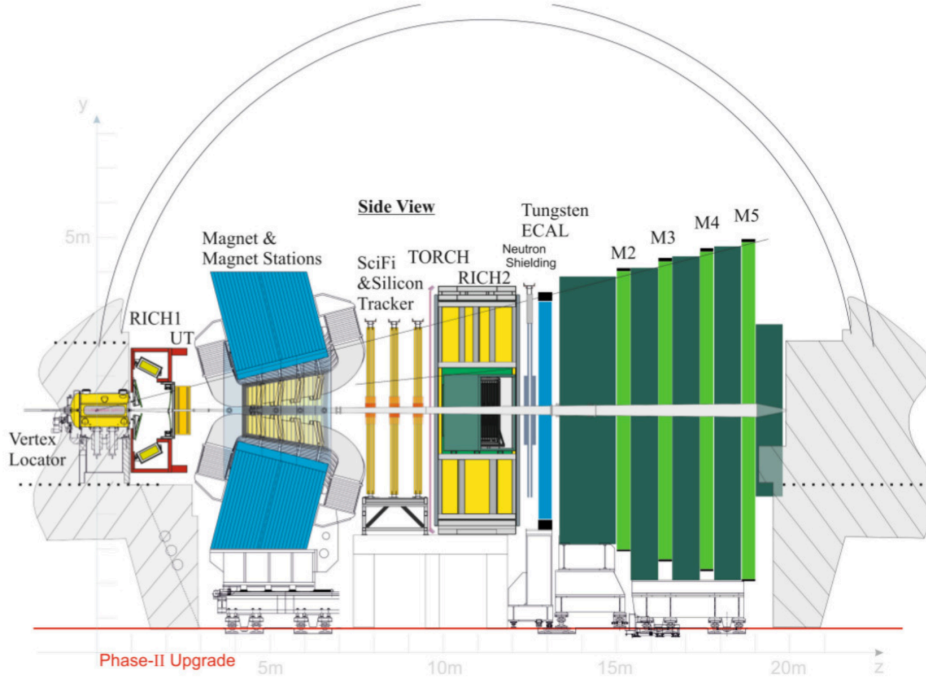
Figure 6.1: Schematic view of the LHCb Upgrade II detector. [95]
