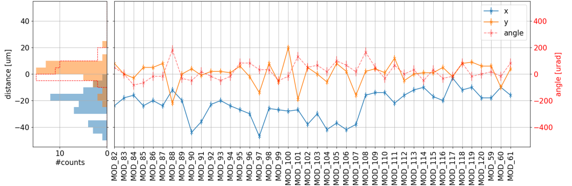
(b) : Offset of the middle point in x and y along with the rotation of the CLI (VP0) tile.
