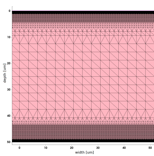
Figure 6.10: Meshing map of the simulated diode with thickness 50 μm. The meshing is more refined in the implant regions in order to better simulate the avalanche process in the multiplication layer.
