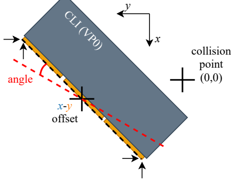
Figure 4.8: Visualised tile position calculated variables x , y and angle.
