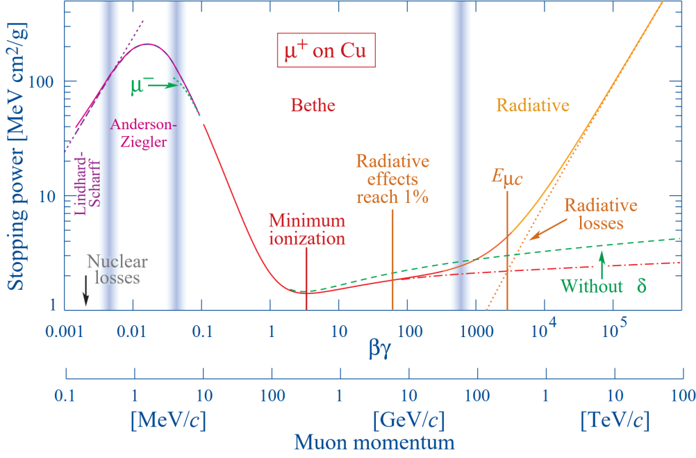
Figure 2.1: Mean energy loss of a positive muon in copper as a function of momentum. The graph is horizontally split to regions based on the approximations of the interactions. [52]
