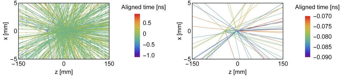
Figure 6.2: Visualisation of the interactions from a single bunch crossing in VELO (left plot). Using a time cut on the tracks of 20 ps (right plot) reduces the complexity of reconstructing the vertices. [95]
