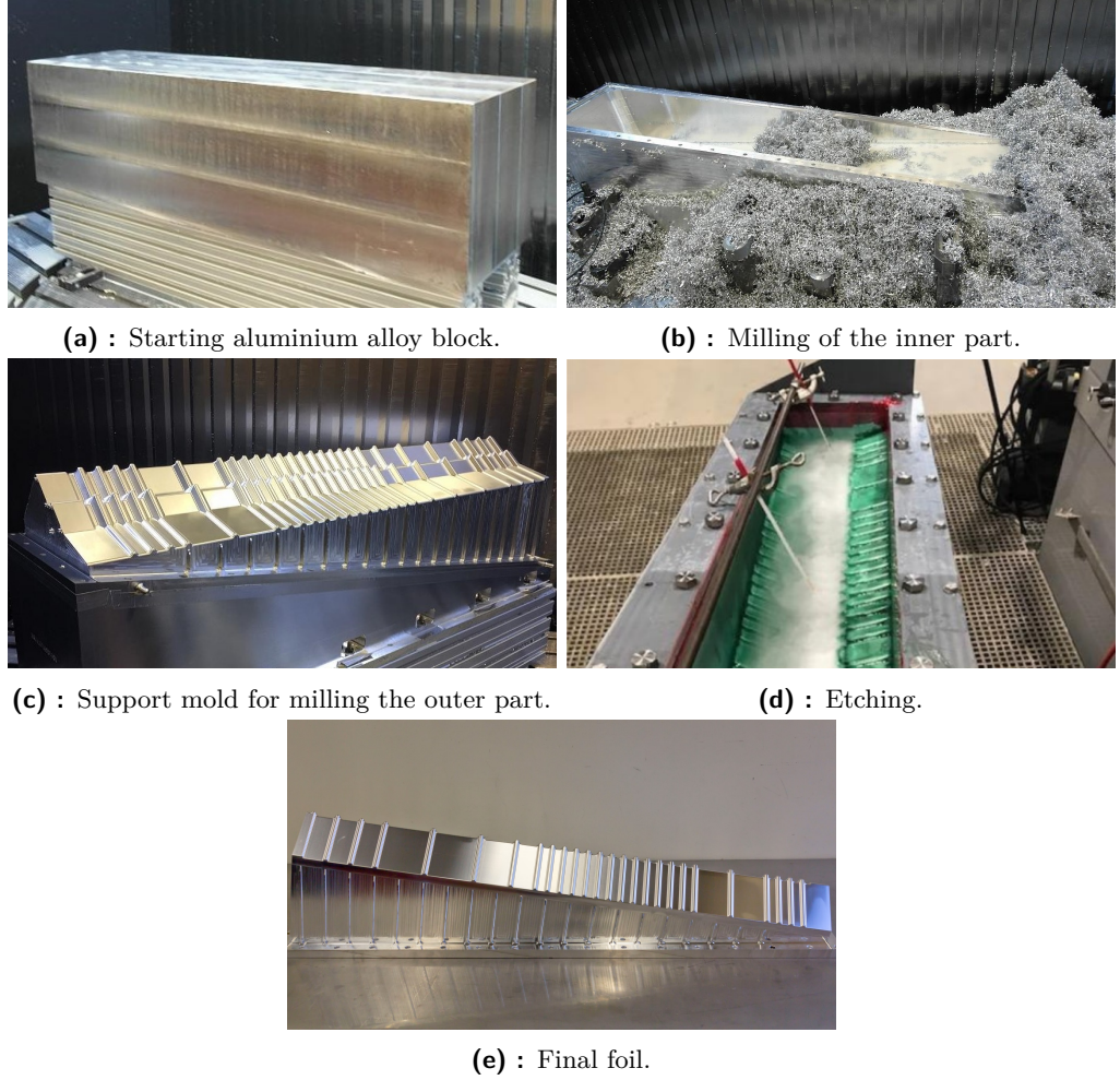
Figure 1.15: Steps of the RF foil production at Nikhef. [35]
