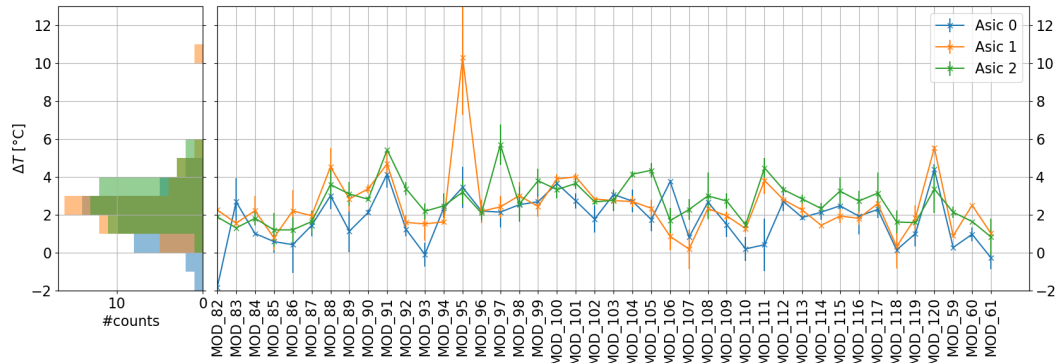
Figure 4.25: Trend of cooling performance for CLI (VP0) before TC.
