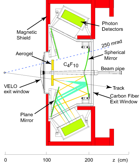
Figure 1.9: Schematic view of RICH1 detector. [15]
