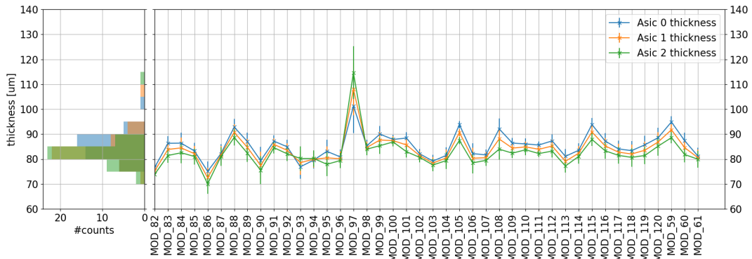
Figure 4.7: Average glue thickness of ASICs under CLI and NLO tiles.
