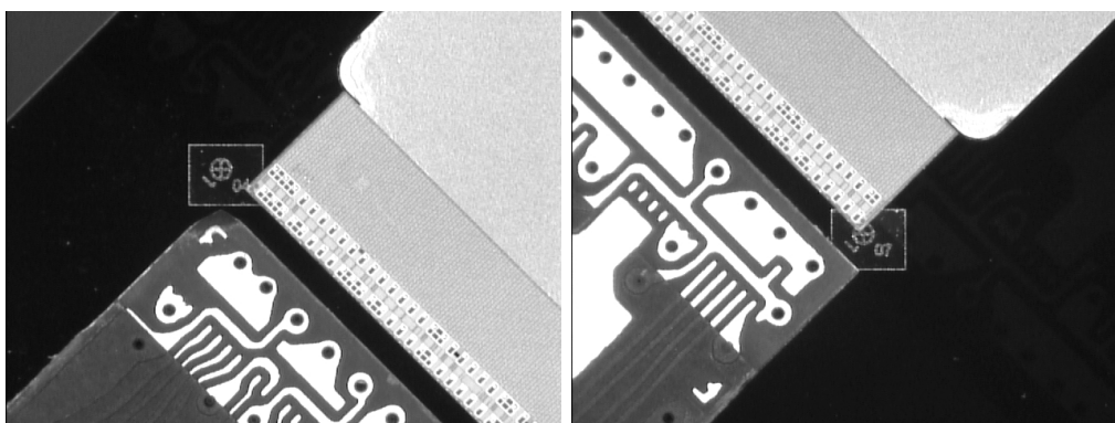
Figure 3.5: Zoomed in image of a glued FE hybrid next to a CLI tile, showing both corners.
