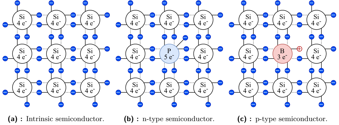
Figure 2.5: visualisation of the silicon valence band with four covalent bonds.
