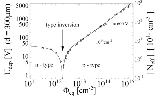
Figure 2.14: Dependency of depletion voltage and effective doping concentration on the neutron fluence equivalent. Measured right after the irradiation. [73]
