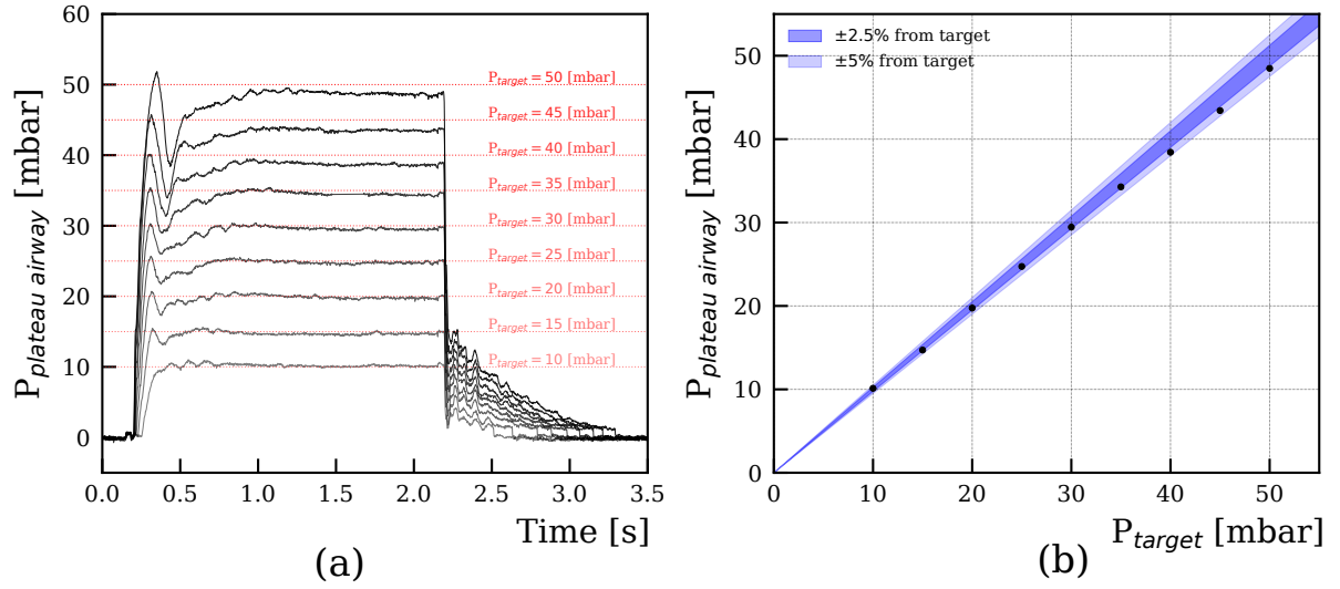
Figure 14: Left: pressurisation of a 50 ml/mbar compliance, 5 mbar/l/sec resistance patient with various target pressures. The inhalation time is set to 1.5 seconds, and is followed by a pause of 0.5 seconds. Right: the deviation of the inhale pressure from the target is computed during the pause.
