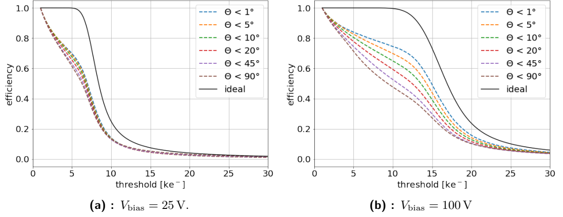
Figure 5.6: Dependency of the hit reconstruction efficiency on the applied threshold for different angular cuts.
