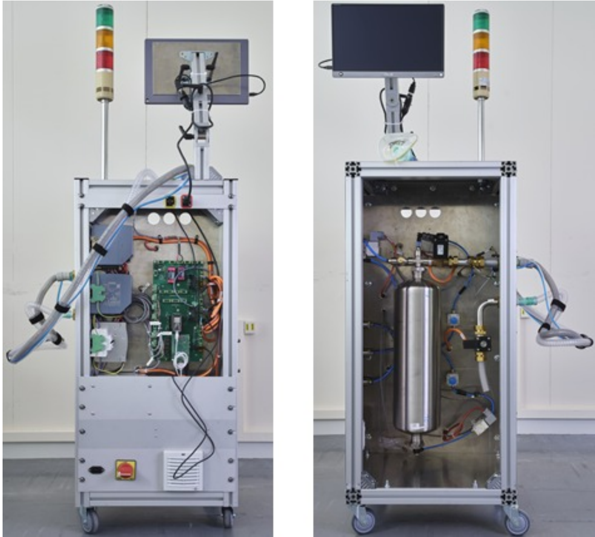
Figure 10: HEV prototypes as tested for full functionality.
