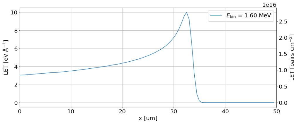
(b) : Dependency of the LET on the distance travelled. Right axis is converted to the format imported into the TCAD.
