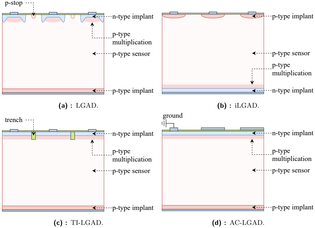
Figure 6.4: Comparison of LGAD types of devices, visualised as 100 \mu\text{m} thick sensor with pixel pitch 50 \mu\text{m} .
