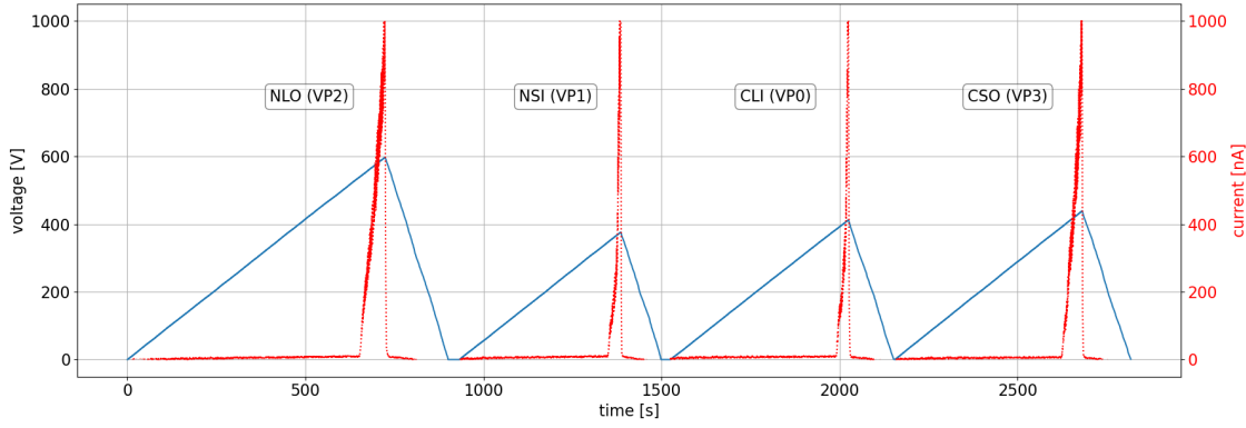
Figure 4.28: Example of voltage ramp with current monitoring for MOD_110.
