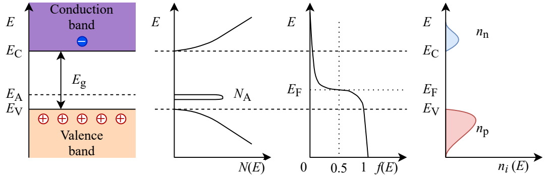
(c) : p-type semiconductor. E_A and N_A represent the acceptor impurity energy level and concentration, respectively.
