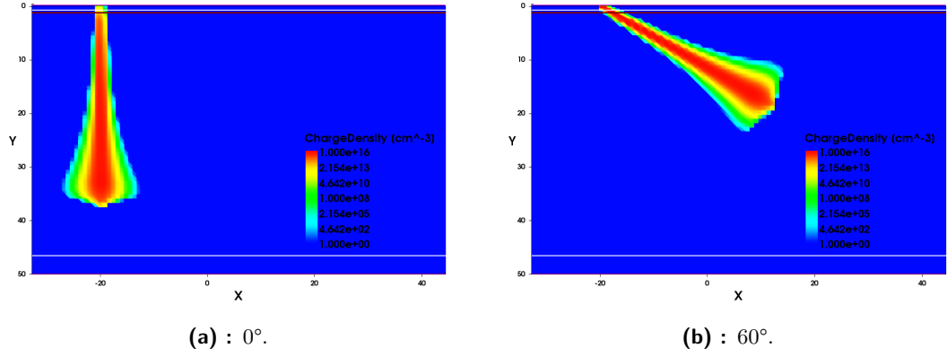
Figure 6.21: Example of the TCAD implemented single proton energy deposition. The kinetic energy of the proton beam is 1.6 MeV.
