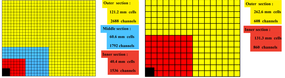
Figure 1.10: Segmentation of the quarter of the Electromagnetic Calorimeter (ECAL) and Hadron Calorimeter (HCAL) to readout channels. The black square represents clearance around the beam-pipe. [15]
