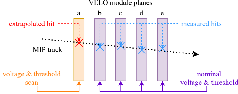
Figure 5.10: Schematic view of the CCE scan where one of the five modules is tested, the remaining four modules are operated in the nominal conditions.
