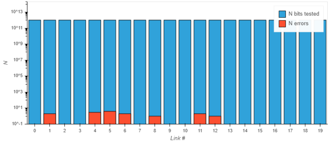
Figure 4.17: Example of PRBS test data showing 1 \cdot 10^{12} bits tested along with the number of errors. Test was done before TC on MOD_60.
