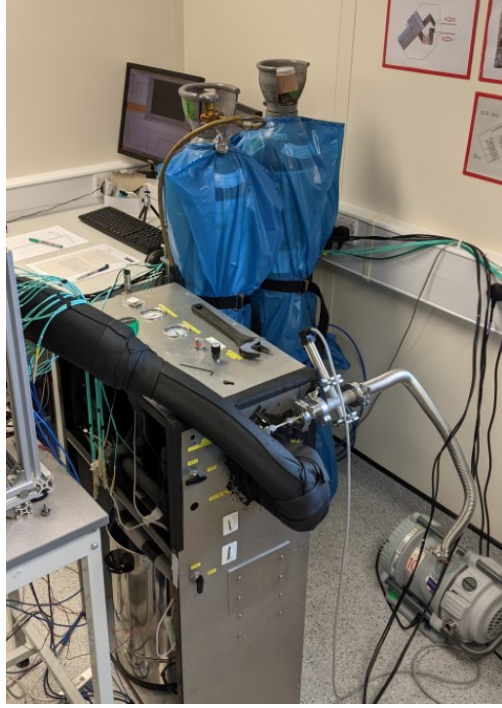
(a) : Picture. The probes and the heat exchanger are inside the large box.
