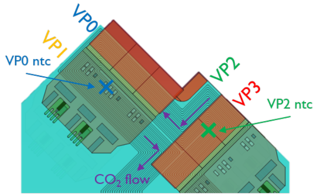
Figure 4.23: Position of tiles and NTC sensors on a module.
