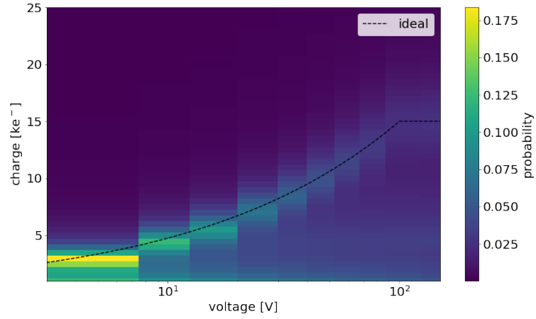
Figure 5.3: Raw data output from simulated dependency of charge on voltage for non-irradiated VELO. The Monte-Carlo results follow the ideal dependency defined by Eq. (5.1).
