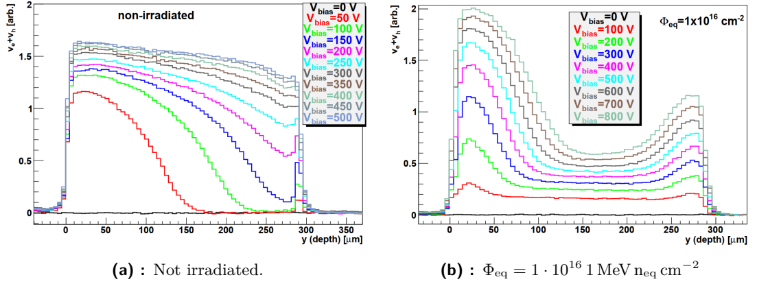
Figure 2.15: Velocity profiles of electron-hole pairs for different bias voltages and irradiation. [78].
