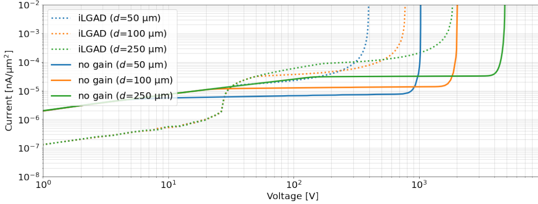
Figure 6.12: IV curve of no gain (solid lines) and iLGAD (dotted lines) devices. The dependency is shown for different thicknesses from 50 \mu\text{m} to 250 \mu\text{m} , thinner diodes have smaller breakdown voltage value.
