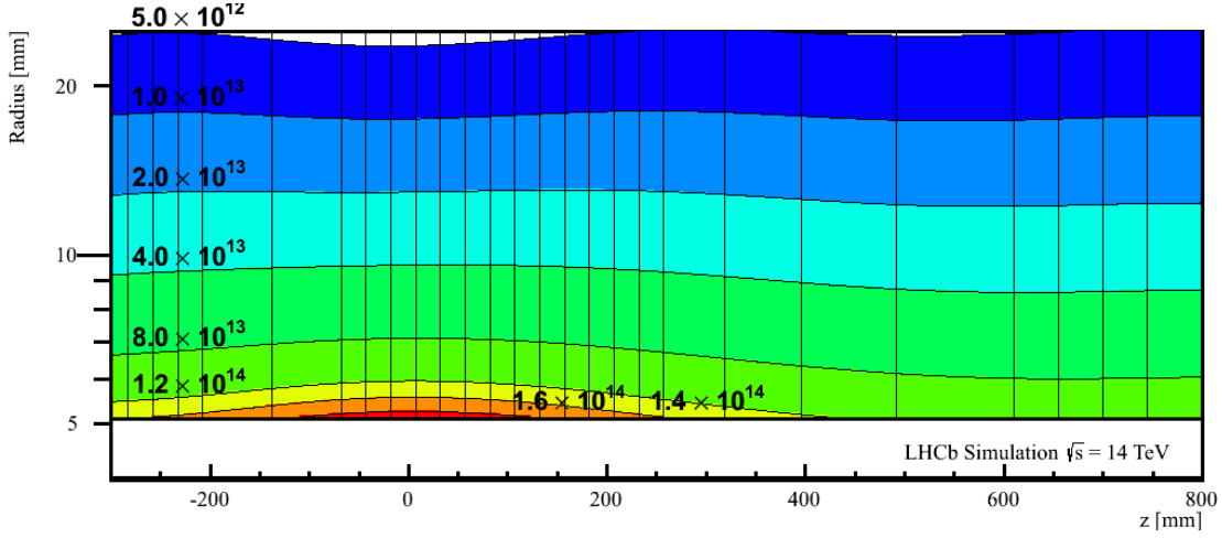
Figure 1.19: Simulated radiation map as a function of position and radial distance from the beam. The colours represent units of n_{\text{eq}}\text{cm}^{-2} for integrated luminosity L = 1\text{ fb}^{-1} [24]. The expected value by the end of Run4 is L = 50\text{ fb}^{-1} .
