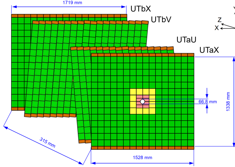
Figure 1.7: Geometry of the Upstream Tracker (UT) detector, showing the x-u-v-x pattern. The colour coding represent modification of the strip pitch and number of channels. [29]
