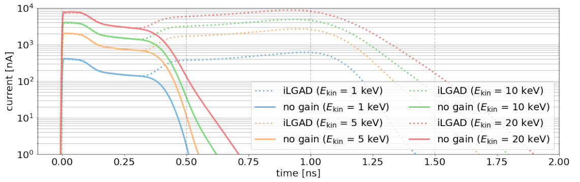
Figure 6.18: Current profiles registered by the central electrode of 50 \mu\text{m} thick sensors.
