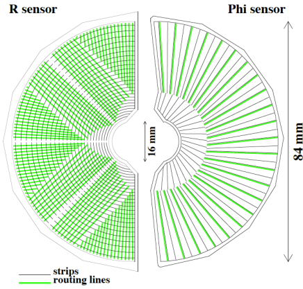
Figure 1.4: Schematic view of VELO R and Phi sensors. [22]
