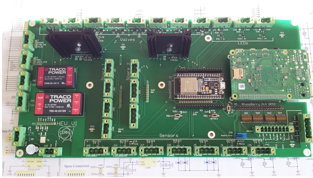
Figure 5: Photograph of the PCB motherboard as implemented for the HEV prototype.
