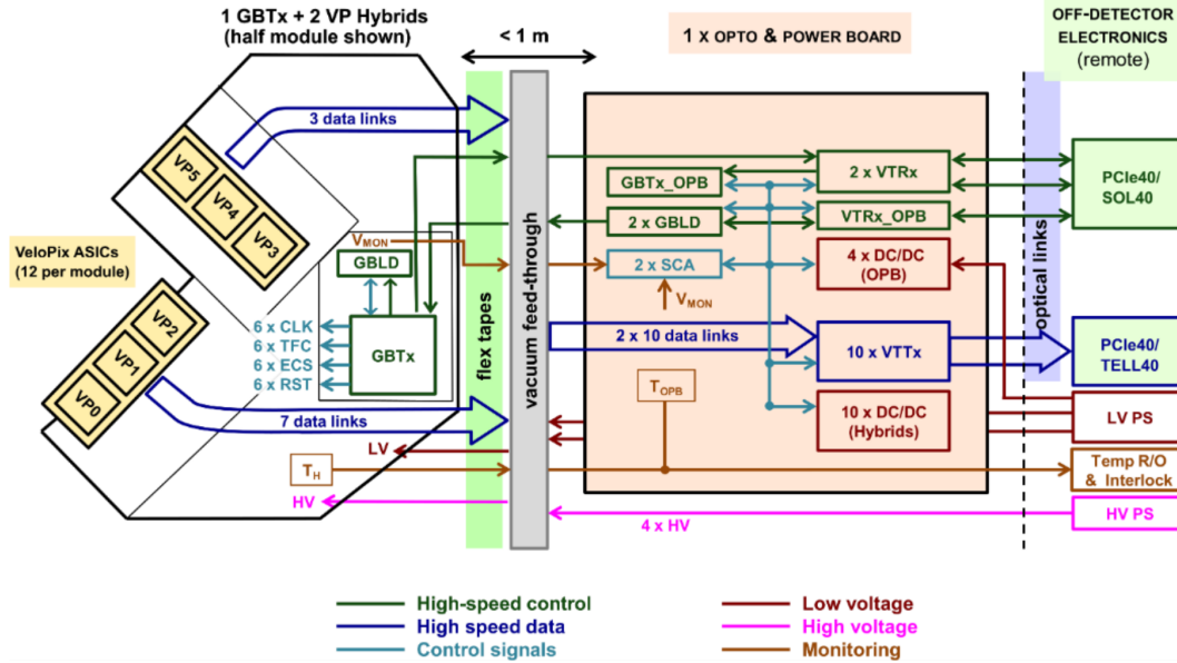
Figure 1.21: Schematic of module readout. The visualisation is made only for one side of the module (effectively halving the number of links and ASICs). [46]
