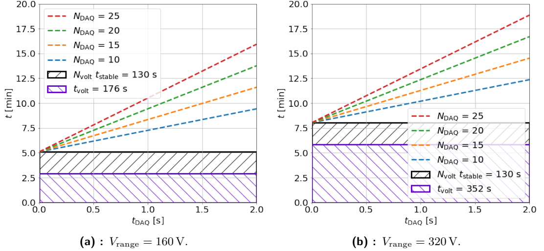
Figure 5.11: The CCE scan duration estimates, applicable to a subset (fifth) of the modules. Plotted for a different number of threshold scan points N_{\text{DAQ}} as a function of DAQ duration.
