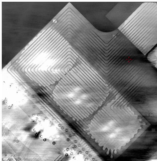
Figure 3.4: CT scan of tiles attached to the cooling substrate using simple star pattern. The small lines are individual channels in the silicon substrate. [35]
