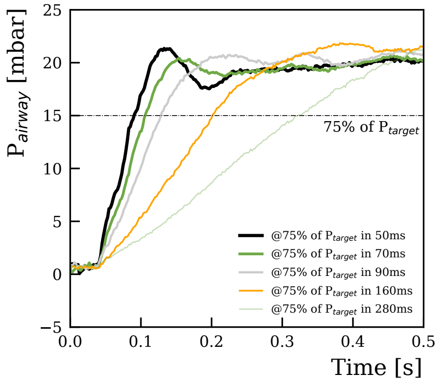
Figure 15: Rising edge of the inhalation for various rise time setting. The lung compliance here is 50 ml/mbar for a resistance of 5 mbar/l/s
