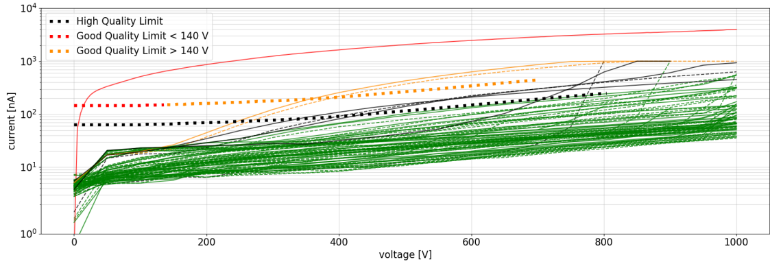
Figure 4.27: All IV curves for the NSI (VP2) tile. Plotted results before and after TC as solid and dashed dotted lines, respectively. The black, orange and red dots represent defined quality limits.
