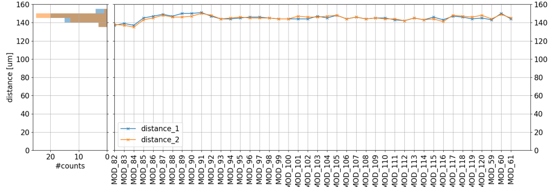
(c) : Distance between corners of NSI and NLO.
