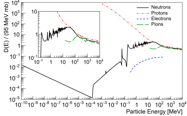
Figure 2.12: Dependency of damage cross-section on particle energy, plotted for different particles. [77]
