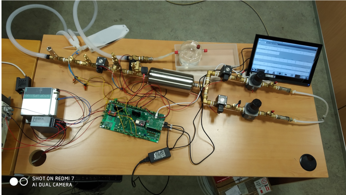
Figure 11: Functional table top prototype produced for collaboration and development purposes.
