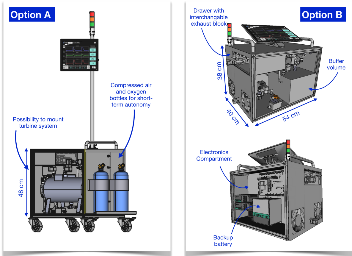
Figure 12: Potential alternative mechanical designs with an identical functionality to the HEV prototypes.
