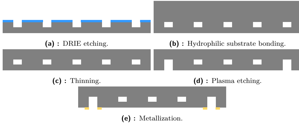
Figure 1.17: Steps of the silicon microchannel substrates production. Silicon (gray), mask (blue), metallisation (gold).
