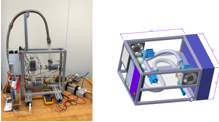
Figure 4: Left: prototype of the turbine system proposed as an alternative to the compressed air supply. Right: drawing of the concept for a complete system which is a box divided in two parts: the top contains the turbines, the bottom contains the corrugated steel pipe, the thermal and pressure sensors and the outlet connector. Mounted on the left side of the box are the air filter, the power supply and the box containing the controller. The blue box on the right provides an enclosure for the optional battery system.
