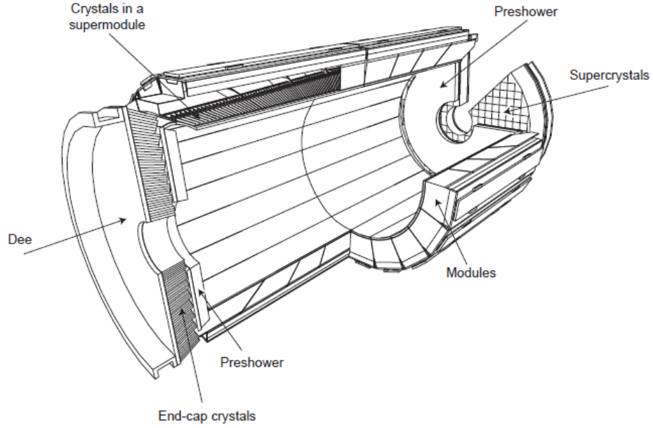
Figure 2.10: Schematics of CMS Electromagnetic Calorimeter (ECAL) [124].
