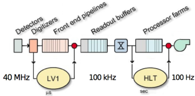
Figure 2.16: Data rates are shown at different stages between detectors and final data storage [127].
