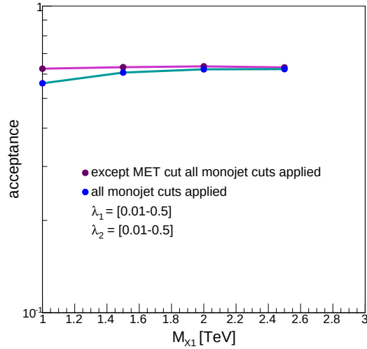
Figure 4.14: Acceptance as a function of resonance mass. The pink plot is after all monojet cuts applied (except \cancel{E}_T cut), whereas blue is for all monojet selections applied including \cancel{E}_T > 250 GeV. The acceptance shows almost constant behavior with increasing resonance mass.
