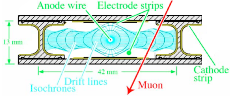
Figure 2.15: Schematics of a DT cell [124].
