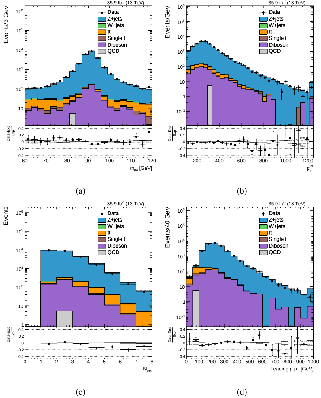
Figure 9.6: Comparison between data and Monte Carlo simulation in the dimuon region for (a) dimuon mass distribution, (b) leading jet p_T , (c) AK4 jet multiplicity and (d) leading muon p_T .
