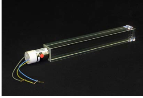
Figure 2.11: Lead Tungstate \text{PbWO}_4 crystal with its avalanche photodiode photodetector used in ECAL barrel region is shown [123].
