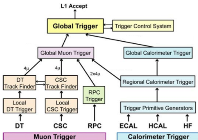
Figure 2.17: CMS triggers use information from sub-detectors. Figure shows L1T decision flow, if the event passes at this stage then data is transferred to DAQ system [124].
