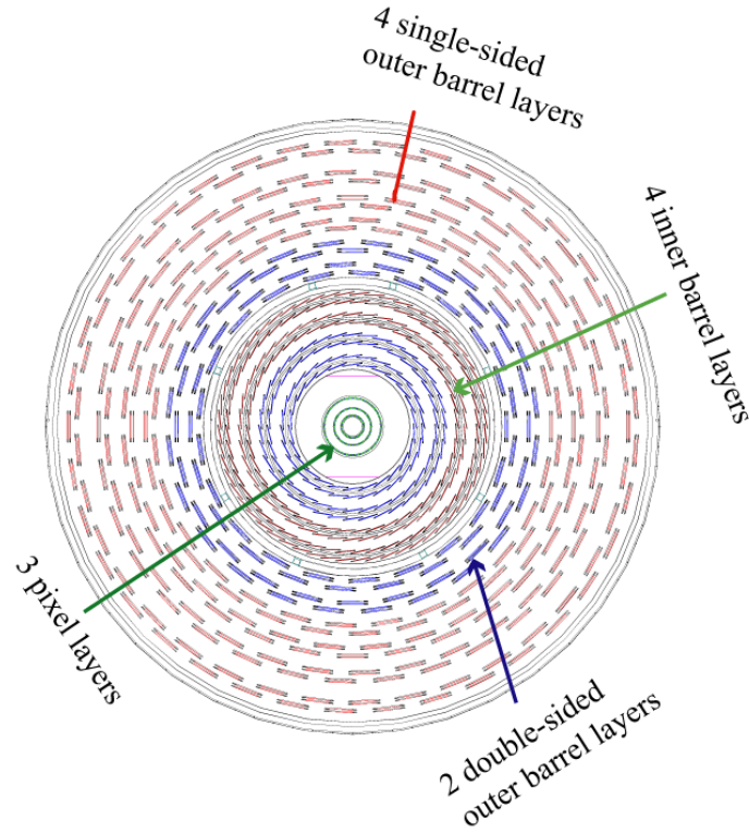
Figure 2.8: Silicon Pixel detector layers are shown in the plane perpendicular to the beam direction [122].
