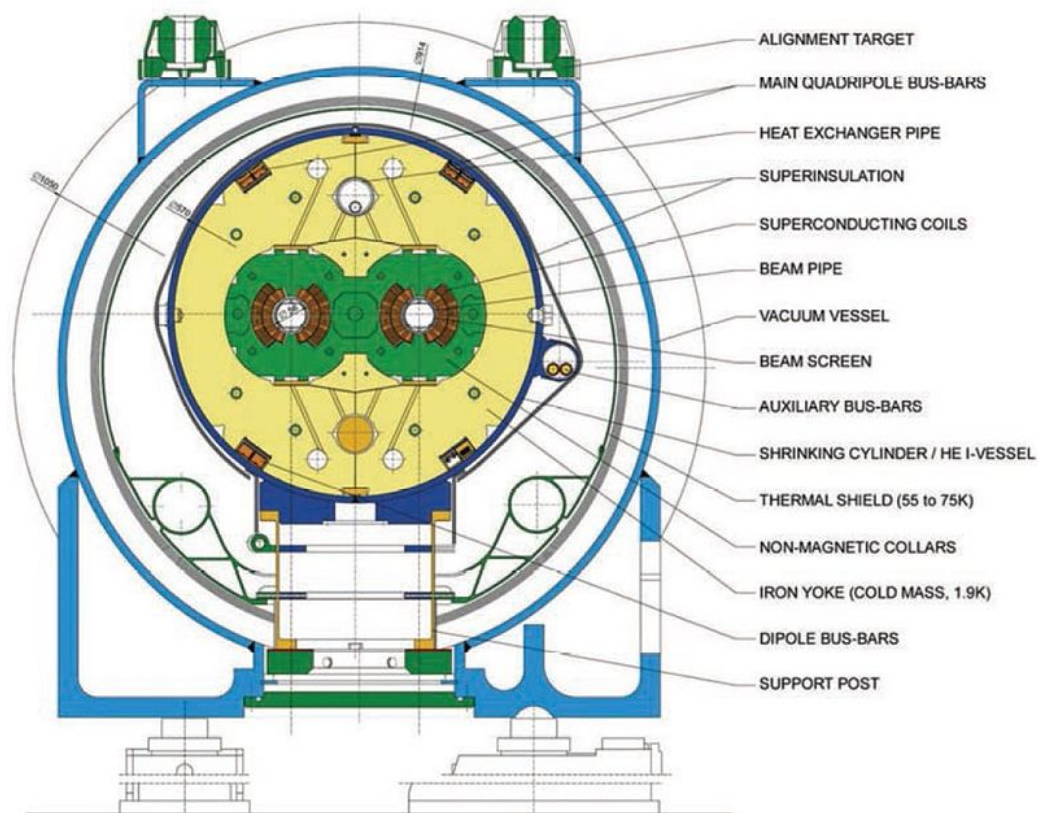
Figure 2.2: Cross section of the two-in-one magnetic design for main LHC dipole magnets [108].
