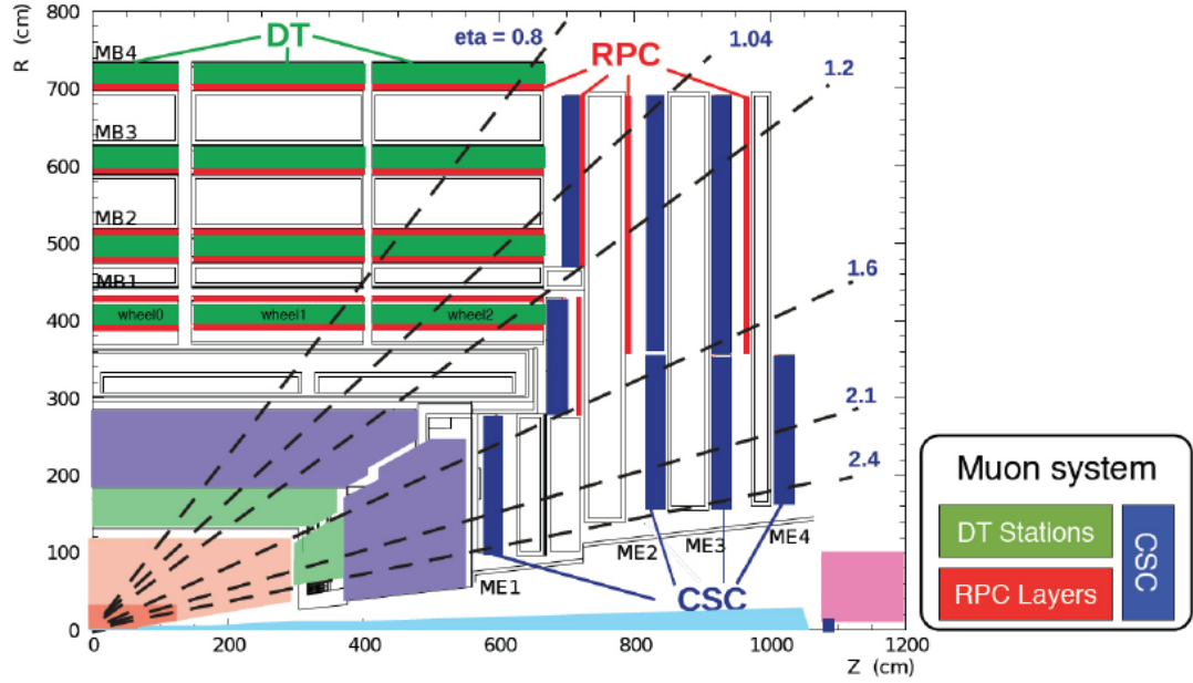
Figure 2.14: Schematic layout of one CMS quadrant. Green parts represent four DT stations in the barrel (MB1-MB4), the four CSC stations in the endcap (ME1-ME4) are shown in blue and the RPC stations are in red [126].
