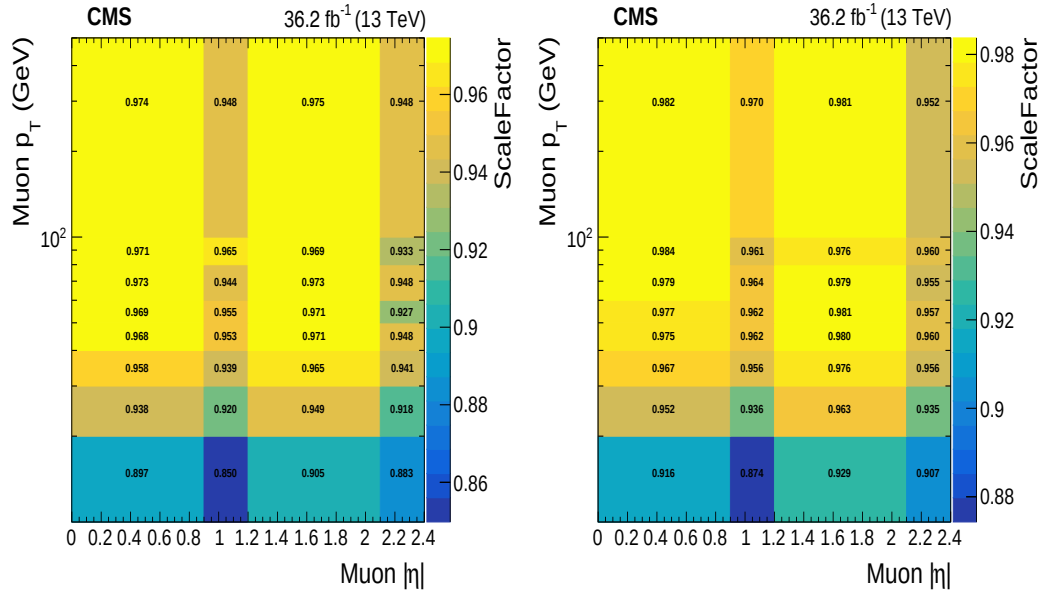
Figure 6.2: Data-MC scale factors for tight muon selection as a function of muon p_T and \eta with number of vertices N_{PV} > 17 (left) and N_{PV} \leq 17 (right) [138].
