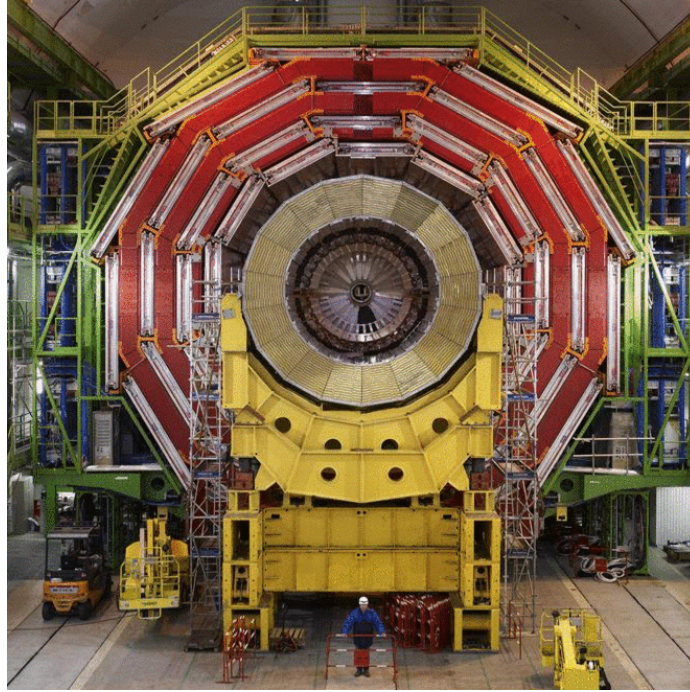
Figure 2.5: The Compact Muon Solenoid (CMS) detector at the Large Hadron Collider, with human figure for scale [119].
