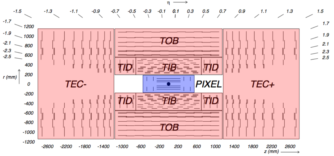
Figure 2.9: Several detectors in the silicon tracker. Silicon pixel detector is shown in blue whereas silicon strip detectors i.e. TIB, TID, TOB and TEC, are shown in red [123].
