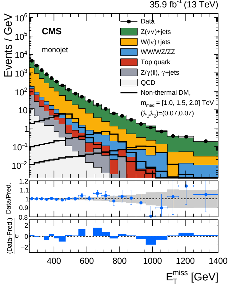
Figure 8.2: \cancel{E}_T distributions for data and various SM backgrounds in signal region. No excess of data over the SM expectation is observed. The background processes are estimated by performing maximum likelihood fit to the data in all the control regions as well as in the signal region. Black curves represent \cancel{E}_T distributions from Non-thermal DM model with M_{X_1} = 1.0, 1.5 and 2.0 TeV, peaking at 500, 750 and 1000 GeV respectively. Signal curves are plotted for couplings (\lambda_1, \lambda_2) = (0.07, 0.07) . Data to predicted MC ratio is shown in the middle panel where gray bands indicate the post-fit uncertainty in the background prediction. Bottom panel shows the distributions of the pulls, defined as the difference between data and the post-fit background prediction relative to sum in quadrature of the post-fit uncertainty in the prediction and the statistical uncertainty on data.
