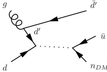
Figure 4.3: Initial state gluon splitting process (2 jets + \cancel{E}_T ) .
