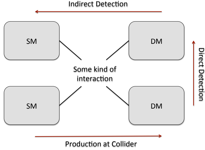
Figure 1.5: Different dark matter detection strategies are explained in a toy Feynman diagram.
