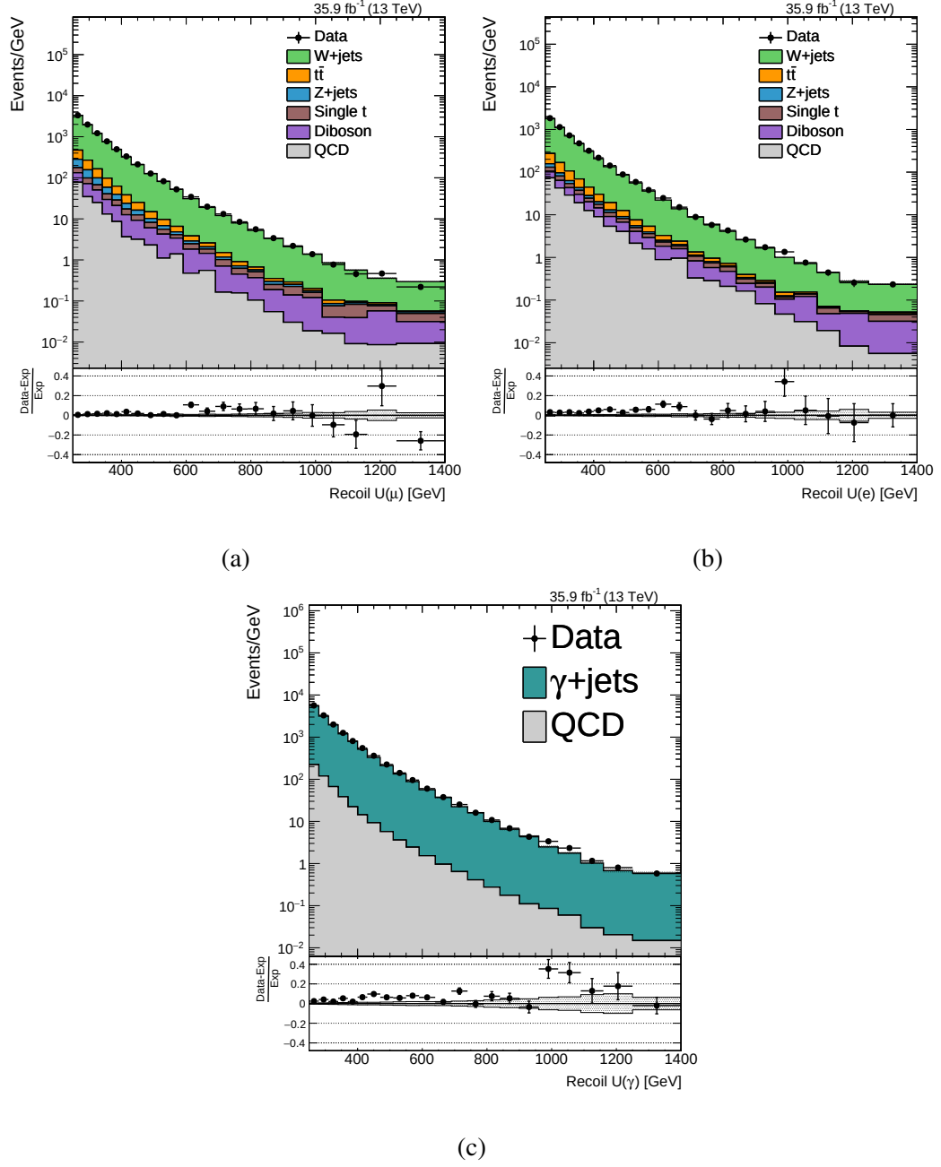
Figure 7.3: Comparison between data and Monte Carlo simulation for recoil distribution in the (a) single muon CR, (b) single electron CR and (c) single photon CR. Overall good agreement is observed.
