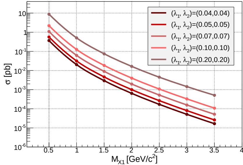
Figure 4.11: Cross-section \sigma as a function of mediator mass M_{X_1} . Each curve is for a fixed (\lambda_1, \lambda_2)
