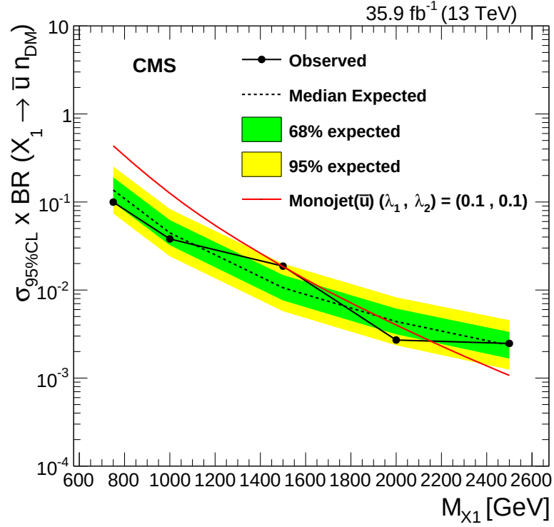
Figure 8.6: 95% C.L. observed and expected upper limits on production cross-section for resonance process are shown where the mediator decays to a light quark jet and a light weakly interacting particle. The expected limit is model independent and holds for the range of 0.01 to 0.5 for each of \lambda_1 and \lambda_2 . Red curve is for nonthermal DM cross-section for (\lambda_1, \lambda_2) = (0.1, 0.1) .
