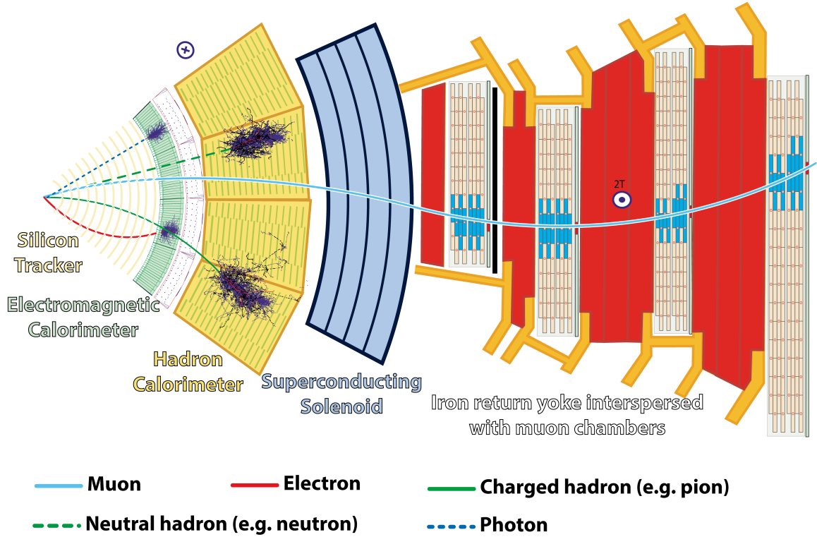
Figure 2.6: Schematic cross section of CMS detector [120].
