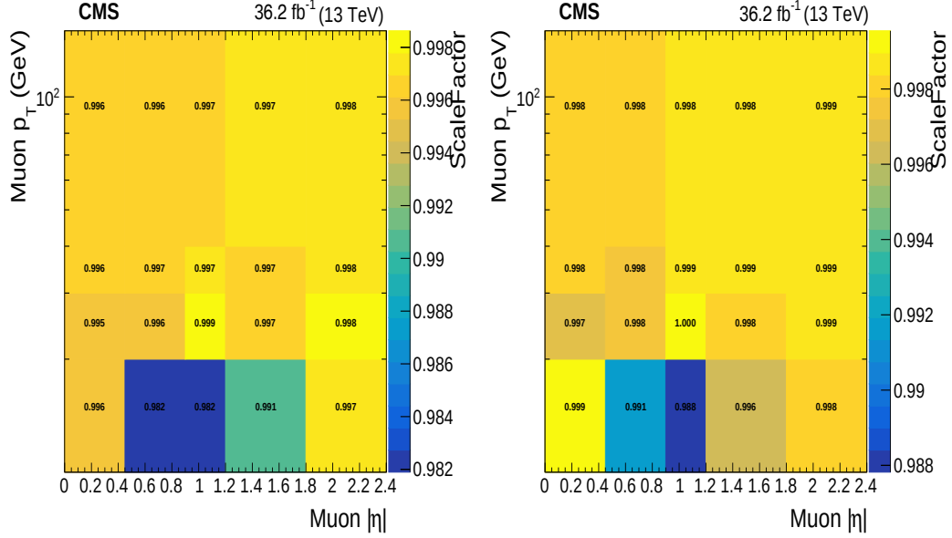
Figure 6.3: Data-MC scale factors for muon tracking efficiency as a function of muon p_T and \eta with number of vertices N_{PV} > 17 (left) and N_{PV} \leq 17 (right) [138].
