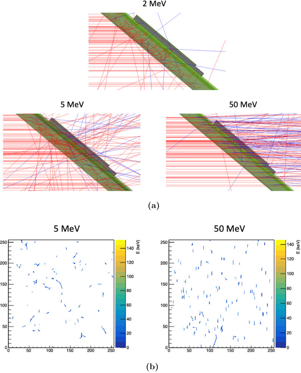
Fig. 2.3.3. (a) Simulations of a 2, 5 and 50 MeV electron beam directed at a TPX detector, equipped with a similar casing than ATLAS-TPX detectors. The detector is irradiated from the back (left side on the pictures), to show the effect of the casing on electron trajectories (red lines). The silicon sensor is the last gray layer on the right, and blue lines represent photons emitted by Bremsstrahlung. (b) Example frames of the 5 MeV and 50 MeV beams, showing the 2D projection of electron trajectories in the sensor. Simulations were performed using the Allpix2 framework [4].
