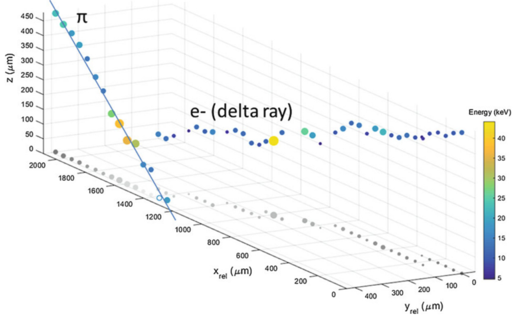
Fig. 2.2.5. 120 GeV/c pion track with ejected delta ray recorded by a TPX3 detector [69]. In contrast to figure 2.2.4, the cluster can be represented with a fourth dimension (z-coordinate of the particle trajectory) due to the simultaneous TOT and TOA operation of the TPX3 chip.
