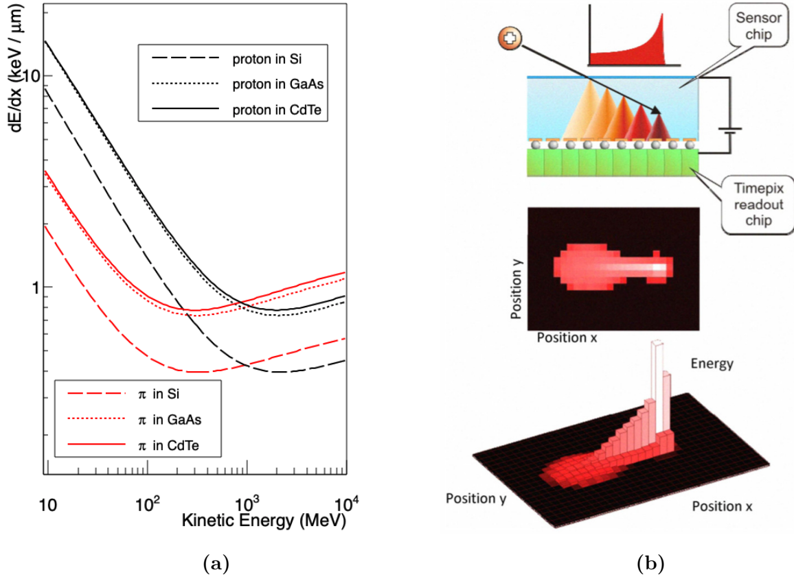
Fig. 2.3.1. (a) Energy loss of heavy charged particles in different sensor materials. The stopping power ( dE/dx ) is calculated using the Bethe-Bloch formula [18]. Multiplying the y-axis by 55 \mu\text{m} , one gets an idea of the deposited energy per pixel if the particle is parallel to the sensor surface. b) Illustration of energy loss measurement by a TPX detector [72]. Here, a heavy charged particle is stopped in the sensor. The measured track reproduce the Bragg curve (shown on the very top).
