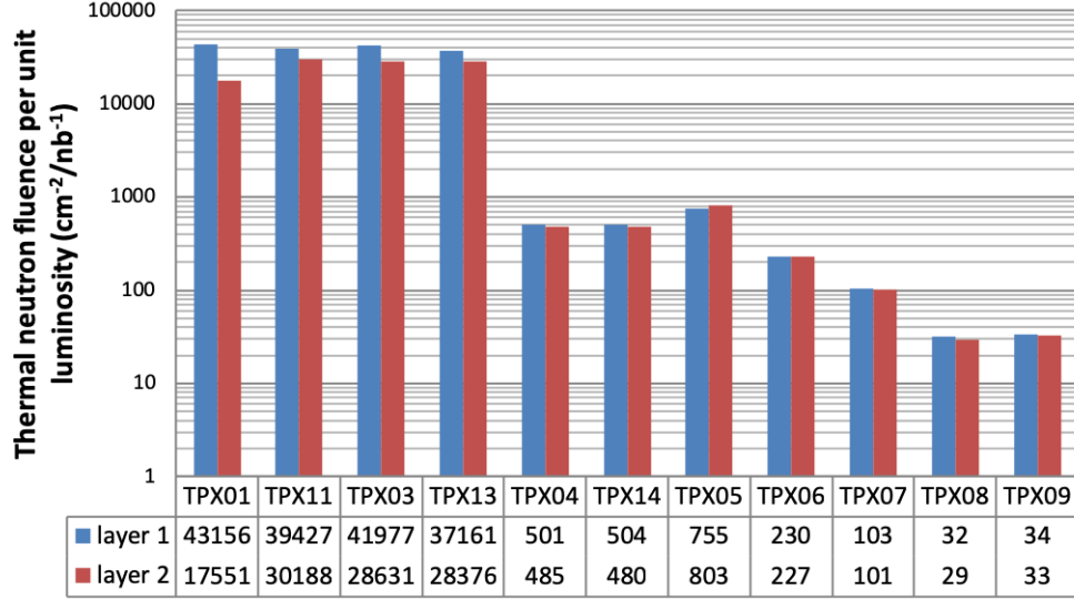
Fig. 3.3.10. Thermal neutron fluences per unit luminosity for the different ATLAS-TPX devices as measured during LHC Fill 4965 on May 31, 2016 (accumulated luminosity: 160 \text{ pb}^{-1} ) [117].
