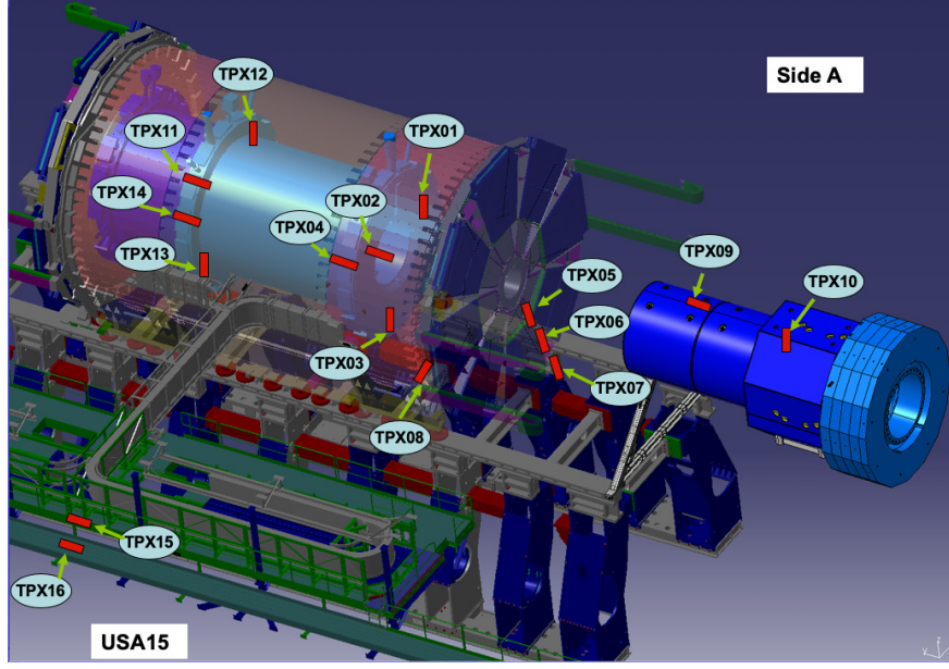
Fig. 3.3.2. Position of ATLAS-TPX detectors in ATLAS.
