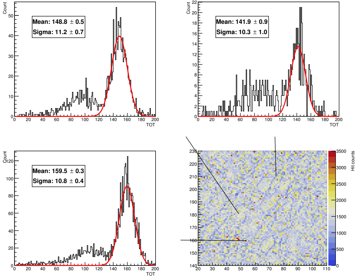
Fig. 4.4.5. Zoom on the dashed area of figure 4.4.4 a) with pixel spectra from different regions. Gaussian fits are displayed in red, along with the fit parameters. The detector is operated in TOT mode, which allows the measurement of deposited energy and photon counting at the same time.
