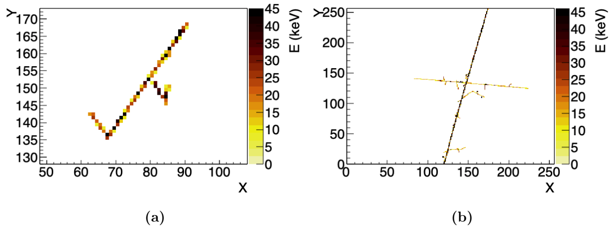
Fig. 3.3.8. Examples of overlapping clusters. a) One MIP emitting \delta -rays and b) two MIPs crossing each other (also with \delta -rays).
