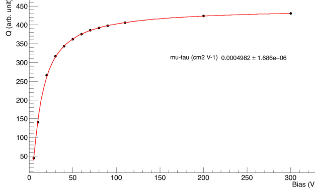
Fig. 4.3.4. Collected charge (arbitrary units) as a function of bias for TPX-CdTe irradiated with 800 keV protons. The collected charge is assumed to be proportional to cluster volumes obtained with the per pixel calibration. Error bars (errors on the means as calculated by Minuit-Migrad) are not visible.
