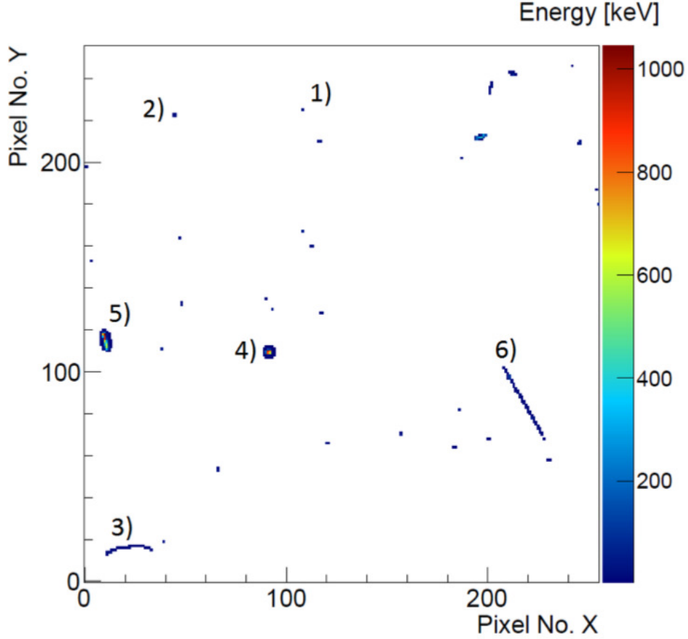
Fig. 3.2.4. Example of a frame recorded by ATLAS-TPX, showing the different categories of clusters (see section 2.4): dots (1, 2) and curly tracks (3) originate either from X/ \gamma rays or electrons below their MIP regime, straight tracks (6) come from MIPs and HETEs (4,5) are typical neutron-induced events.
