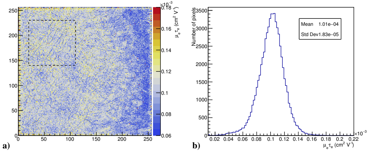
Fig. 4.4.8. \mu_e \tau_e map (a) and distribution (b) obtained from the 23 keV source. The dashed area on a) is enlarged in figure 4.4.9 a).
