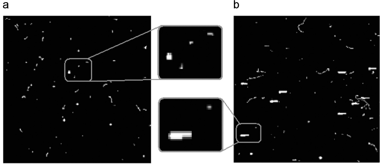
Fig. 2.2.2. Example of frames recorded by a MPX2 detector exposed to ^{241}\text{Am} , ^{106}\text{Ru} , ^{137}\text{Cs} and 10 MeV protons at 0^\circ (left) and 85^\circ (right) [60]. Large tracks are due to protons or to 5.48 MeV \alpha -particles from ^{241}\text{Am} , while thin tracks come from electrons (up to 39 keV from ^{106}\text{Ru} ) and photons (662 keV from ^{137}\text{Cs} ).
