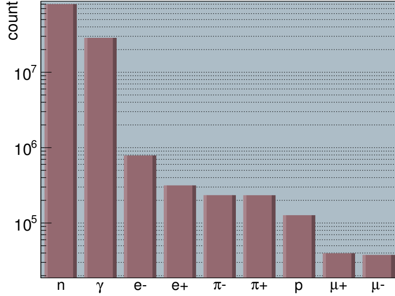
Fig. 3.2.1. Proportion of radiation field components in the region of the TPX01 detector (see table 3.3.1 for detector position in ATLAS), as obtained from simulations [97]. The y-axis is the number of particles hitting the TPX01 region for 10^5 proton-proton collisions. To increase statistics, the detector region is taken to be a cut-away ring of the ATLAS cylinder where TPX01 is placed, assuming that radiation fluences are symmetrical around the longitudinal axis. Hence, the particle count is higher than the one actually measured by TPX01 for the same number of proton-proton collisions.
