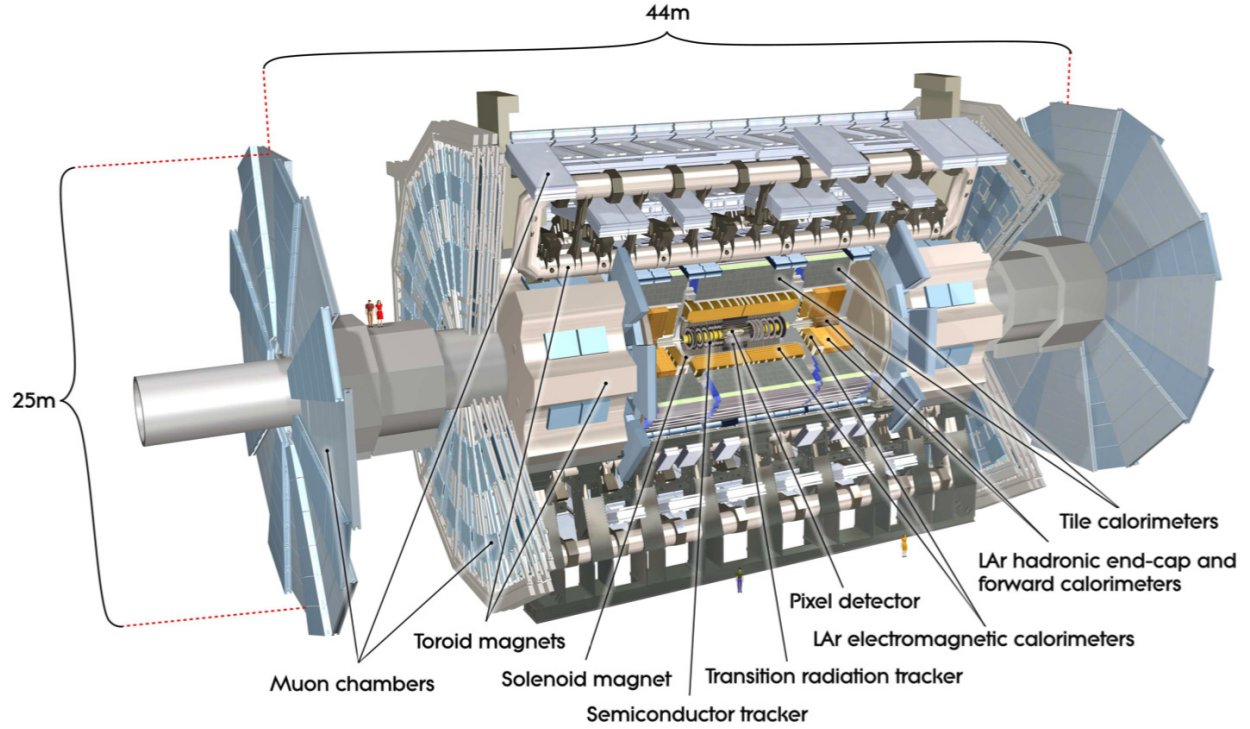
Fig. 1.3.1. Overview of the ATLAS detector [11].
