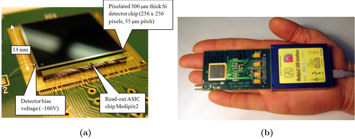
Fig. 2.2.1. Illustration of a MPX2 detector [59]. a) Description of the Medipix2 chip and its sensor. b) Photo of the whole detector with its USB interface (blue box) for connection to a computer.
