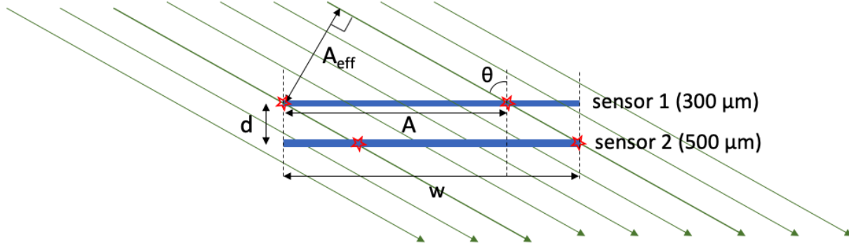
Fig. 3.2.3. Side view illustration of the ATLAS-TPX effective area used for the measurement of MIP fluences. \phi cannot be indicated on side view, see figure 2.4.2.
