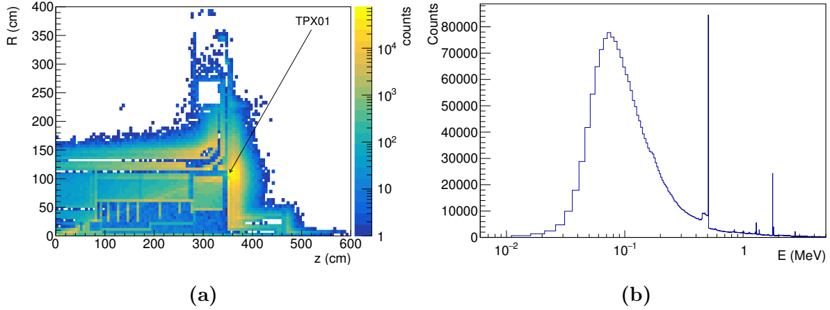
Fig. 4.5.1. Birth position of photons hitting the location of TPX01 in ATLAS (a) and their spectra (b), as obtained from simulations [97]. See table 3.3.1 for the detector location in ATLAS. See figure 3.4.1 and 3.2.2 for comparisons with charged particles and neutrons.
