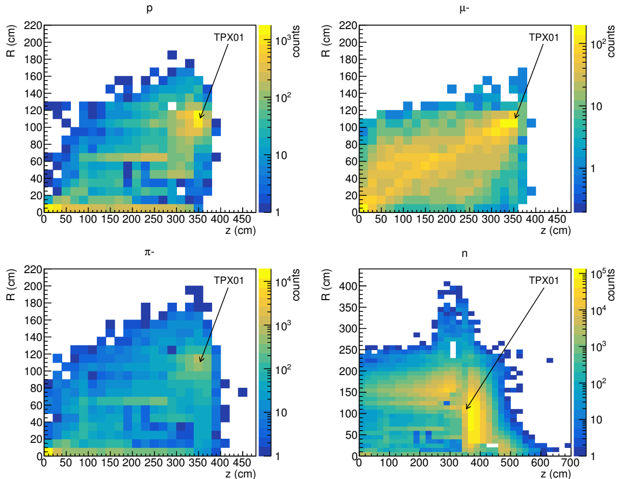
Fig. 3.4.1. Birth position of protons (p), muons ( \mu^- ), pions ( \pi^- ) and neutrons (n) hitting the location of TPX01 in ATLAS (see table 3.3.1 for the detector location in ATLAS), as obtained from simulations [97]. The coordinate system origin is the interaction point, on the bottom left corner. The Z-axis is the distance along the beam pipe, and the R coordinate is the cylindrical radial distance. The ATLAS geometry, and consequently, the radiation field, are considered symmetrical around the Z-axis. Note the different scale and binning between charged particles and neutrons.
