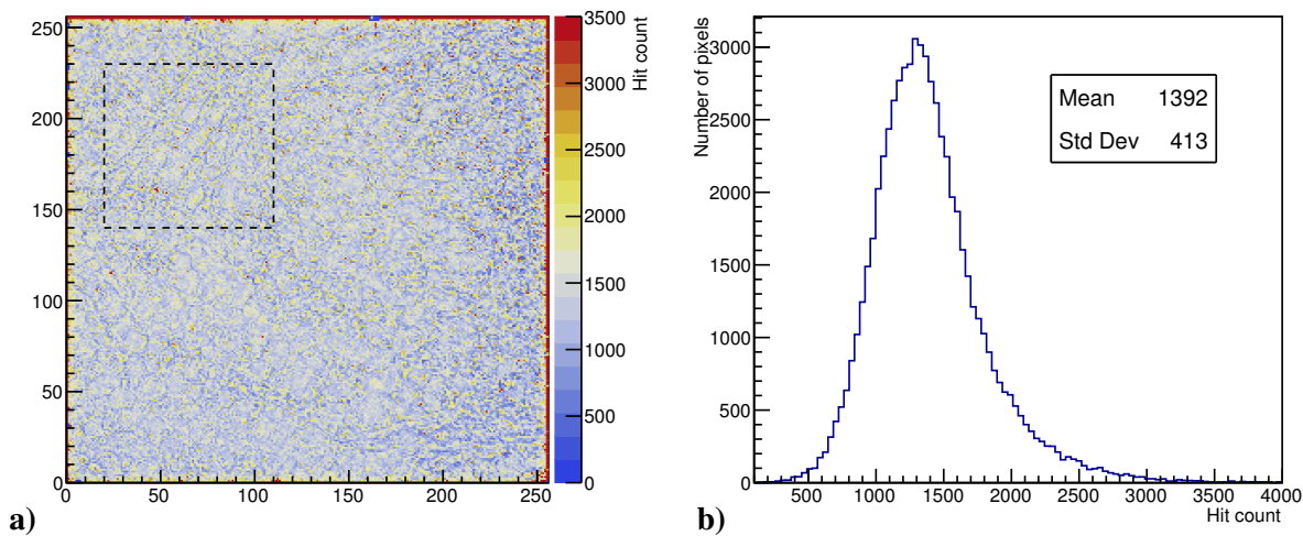
Fig. 4.4.4. Map (a) and distribution (b) of hit counts per-pixel for the 23 keV X-ray irradiation at -300 V. The dashed area on the map is enlarged in figure 4.4.5.
