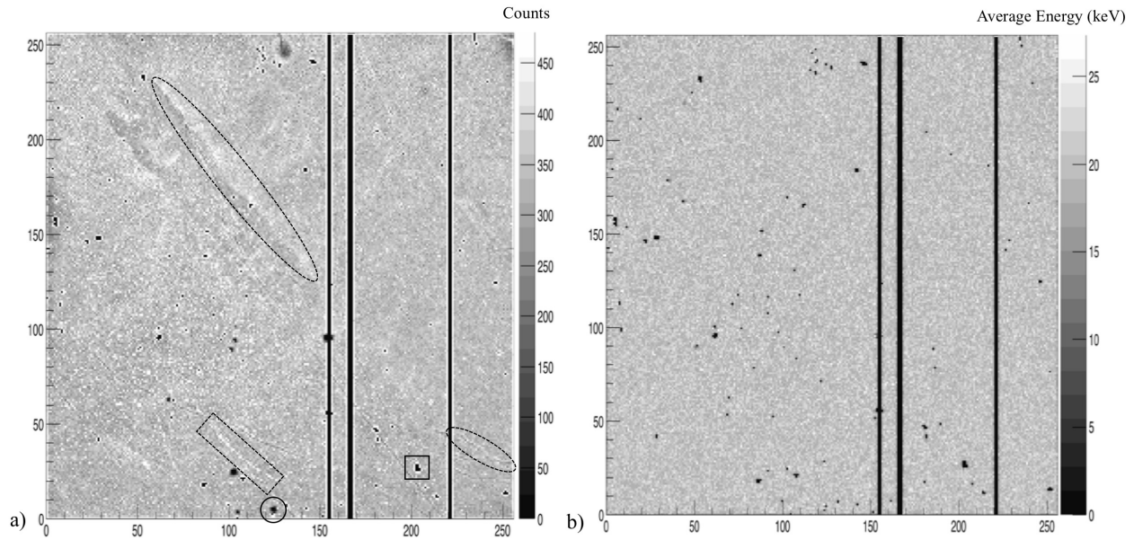
Fig. 4.3.7. Response of TPX-CdTe to X-rays from Cd fluorescence. a) Total number of single pixel clusters. b) Average energy of single pixel clusters. The detector was operated at -300\text{V} during \sim 45\text{ mn} with an acquisition time of 1\text{ ms} .
