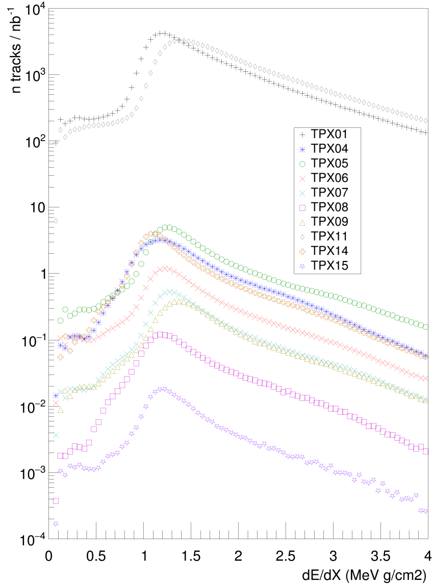
Fig. 3.3.11. Stopping power ( dE/dX ) of tracks measured by the ATLAS-TPX detectors with logarithmic scale (see detector positions in Table 3.3.1). The number of tracks per dE/dX bin is scaled per integrated luminosity. Data were measured during LHC Fill 4965 on May 31, 2016 (accumulated luminosity: 160 \text{ pb}^{-1} ).
