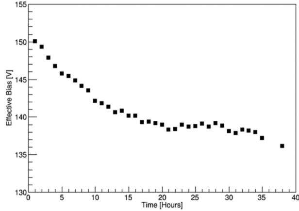
Fig. 4.3.6. The behaviour of the effective bias with time, calculated from the dependence of the cluster size on time and bias.
