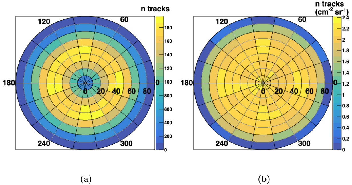
Fig. 3.3.7. Reconstructed MIP directions from the simulation described in Fig. 3.3.6. a) Raw track count and b) track count corrected for effective area and solid angle. The radial axis ( \theta ) represents the incident angle with respect to the sensor surface, as illustrated in Fig. 3.3.4 ( \theta = 0^\circ means the particle is perpendicular to the surface).
