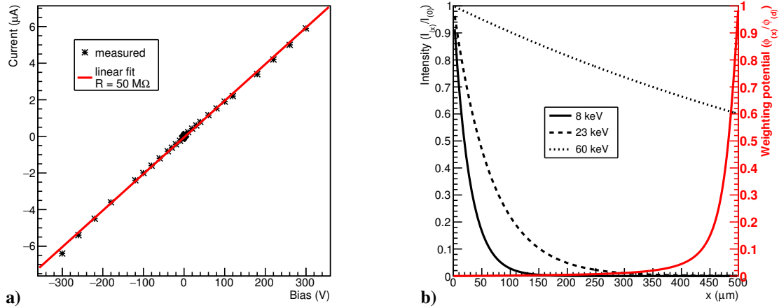
Fig. 4.4.1. a) IV curve of the GaAs:Cr sensor obtained with a Keithley source meter at room temperature, with a linear fit and the resulting resistance. b) Penetration curves (black) of 8 keV, 23 keV and 60 keV X-rays in a 500 \mu\text{m} thick GaAs layer and weighting potential [56] (red) for a charge carrier traveling along the center of a pixel. I(x)/I(0) is the fraction of photons left at a depth x in the sensor from an incoming intensity I(0) .
