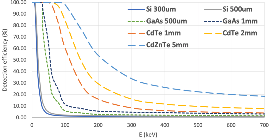
Fig. 4.1.1. Photon detection efficiency as a function of energy for different sensors currently available. The calculation is done for a photon arriving perpendicularly to the sensor surface, with data from Ref. [128]. Displayed sensors can be bump-bonded to either TPX or TPX3.
