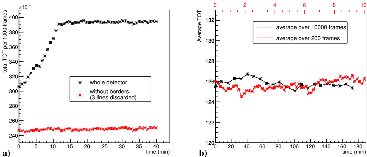
Fig. 4.4.3. a) Total TOT (summed over 1000 frames) as a function of time for the 23 keV source with a -300 V bias. The black graph includes all pixels whereas the red graph excludes 3 lines of pixels on each border of the detector. b) Average TOT of single pixel hits as a function of time for the same measurement, illustrated with two different time scales.
