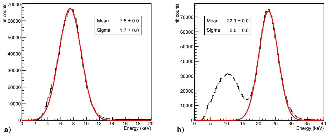
Fig. 4.4.2. X-ray spectrum of the 8 keV (a) and 23 keV (b) source obtained from Cu and Cd fluorescence emission, respectively, using the per-pixel calibration. Only single pixel hits are taken into account. Gaussian fits are displayed in red, along with the fit parameters.
