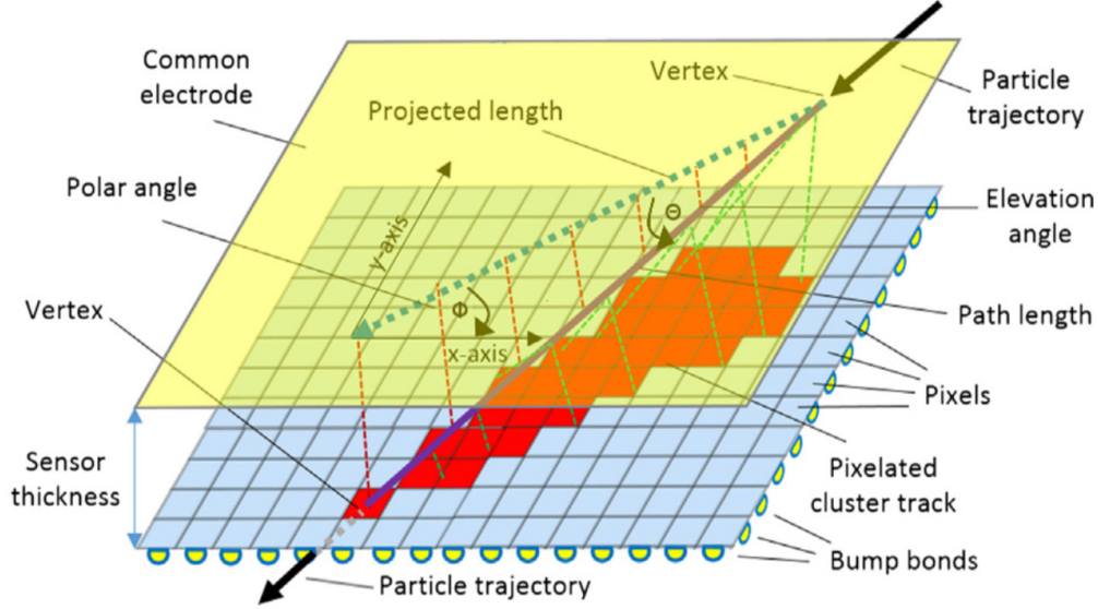
Fig. 2.4.2. Reconstruction of incident angles using the track shape [79].
