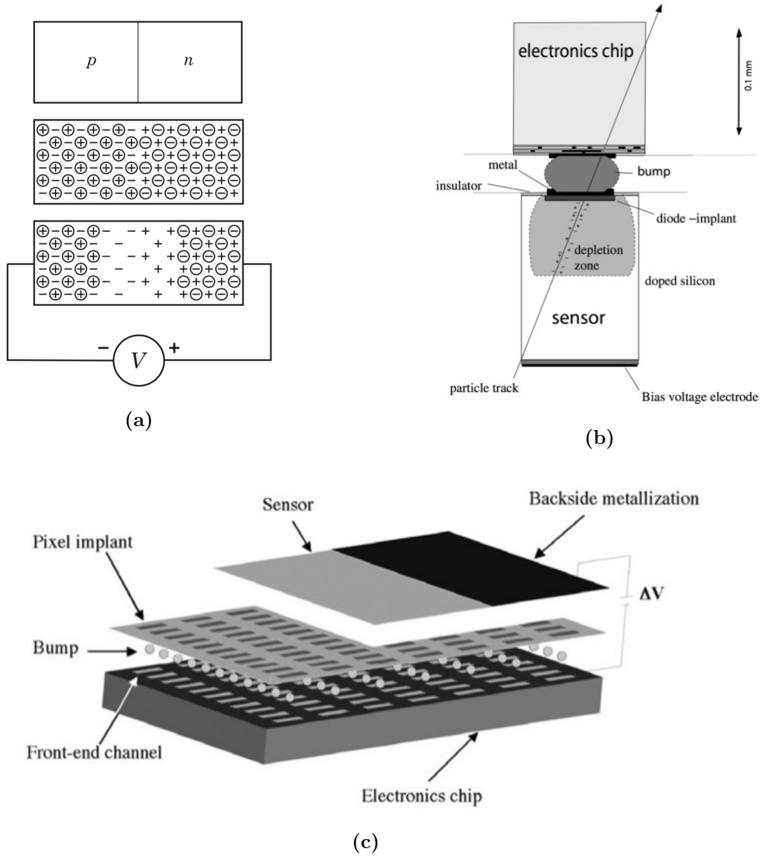
Fig. 2.1.1. Working principle of a hybrid pixel detector. (a) Standard silicon sensors are doped (p-type on one side, n-type on the other), creating a depletion region at the p-n junction, which must be extended by applying a bias voltage [48]. Sensors are then bump-bonded to a pixelated electronics chip. (b) When a particle interacts in the depletion zone of a sensor, electron-hole pairs are created, and charge carriers move toward the pixel electrodes ( e^- towards anode, holes towards cathode) under influence of the electric field [46]. (c) 3D schematics of the pixel detector [46].
