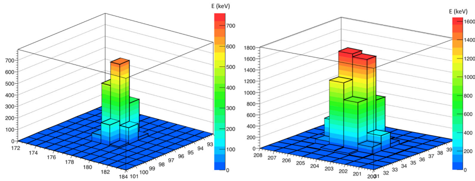
Fig. 4.3.1. Tracks left by a 2 MeV (left) and a 10 MeV (right) proton on TPX-CdTe. The applied bias is -300 V and protons hit the sensor's surface perpendicularly. X and Y axes are pixel coordinates. E is the deposited energy per pixel.
