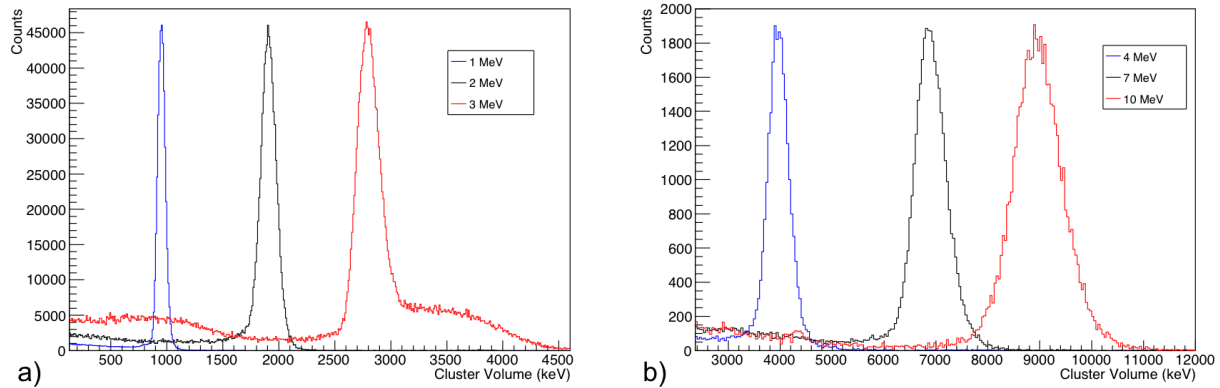
Fig. 4.3.3. Proton spectra for different energies with a) TPX-Si operated at 100V and b) TPX-CdTe operated at -300 V. For each figure, the spectra y-axis are scaled according to the lowest energy proton peak. Cluster volumes are computed using each detector’s specific per-pixel calibration, as described in the text.
