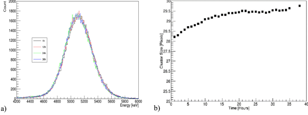
Fig. 4.3.5. Energy spectra of 5.5 MeV alpha particles as a function of time for TPX-CdTe exposed to ^{241}\text{Am} . The spectra were measured over 36 hours under continuous bias application. b) Cluster size of 5.5 MeV alpha particles as a function of time for TPX-CdTe exposed to ^{241}\text{Am} alpha-particles.
