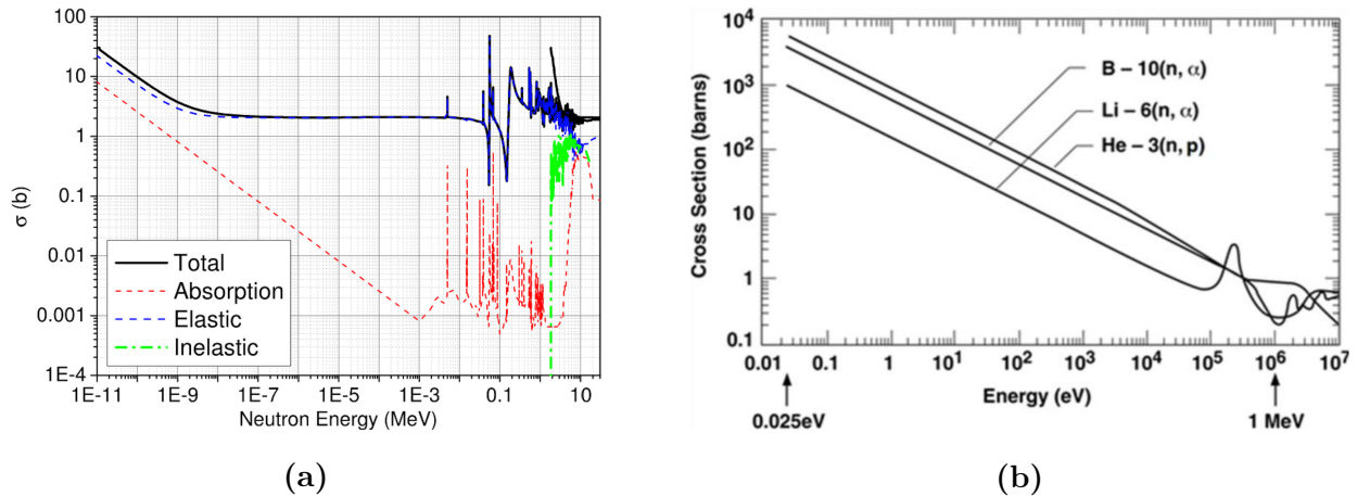
Fig. 2.3.5. (a) Cross section of neutron interactions in silicon [75]. For comparison with photon cross sections in Si given in figure 2.3.4, the y-axis here must be divided by 50 to obtain \sigma in \text{cm}^2/\text{g} . (b) Cross section of neutron absorption in different materials [76].
