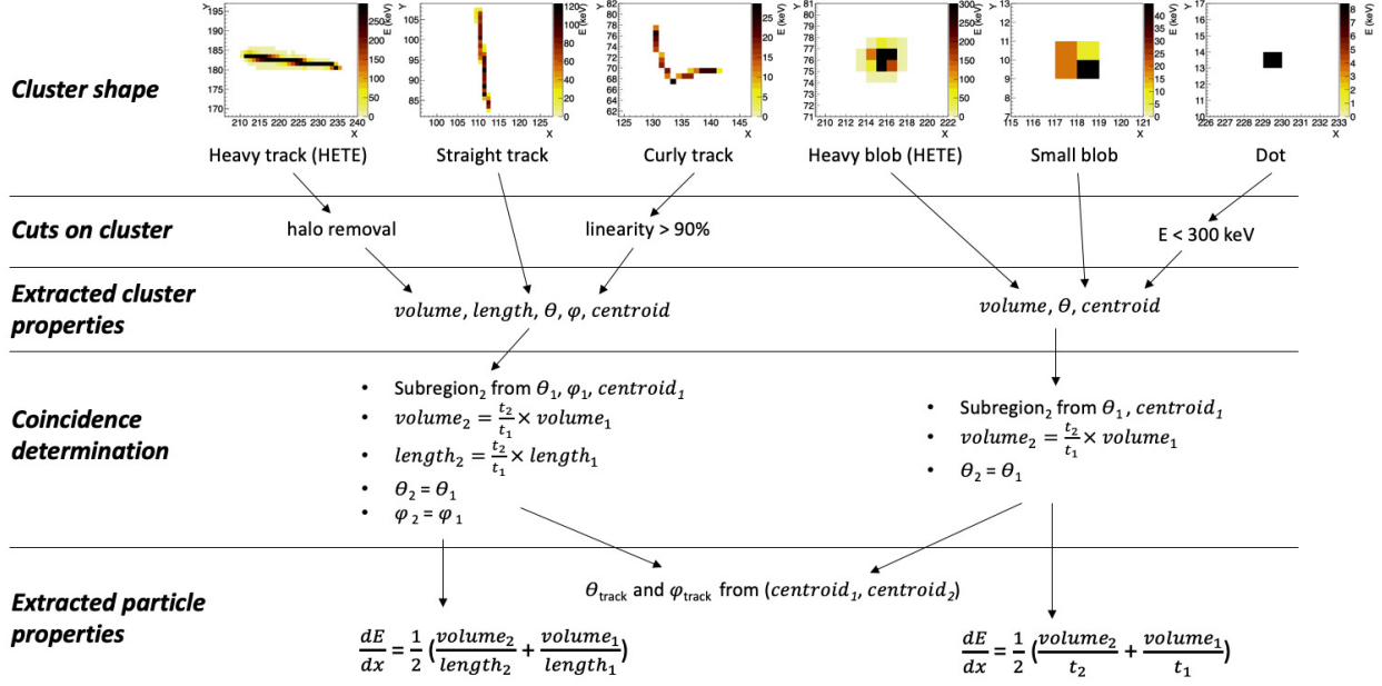
Fig. 3.3.3. Description of cluster processing in order to reconstruct charged particles incident angle and stopping power. t_1 and t_2 are the thickness of the two Si sensor layers, 300 \mu\text{m} and 500 \mu\text{m} respectively (the subscripts of other cluster properties refer to the corresponding layer). See text for more details.
