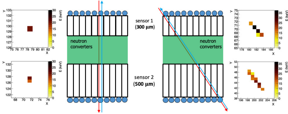
Fig. 3.3.5. Illustration of detected coincident events for MIPs crossing the hodoscope at different angles.
