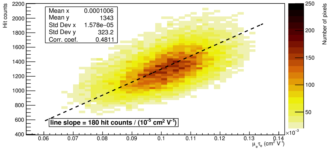
Fig. 4.4.10. Correlation between the photon count map at -300 V and the \mu_e \tau_e map for the 23 keV irradiation. Each bin corresponds to the number of pixels with a specific \mu_e \tau_e and photon count.
