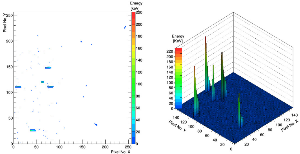
Fig. 2.2.4. Example of frame recorded with a TPX detector exposed to ^{241}\text{Am} , ^{106}\text{Ru} , ^{137}\text{Cs} and 10 MeV protons at 75^\circ [65, 66]. The frame is not full of clusters due to the positioning of the detector compared to the beam and sources. In contrast to figure 2.2.2, the frame has a third dimension (represented in color on the left, and with 3D view on the right), thanks to the TOT mode of the TPX chip.
