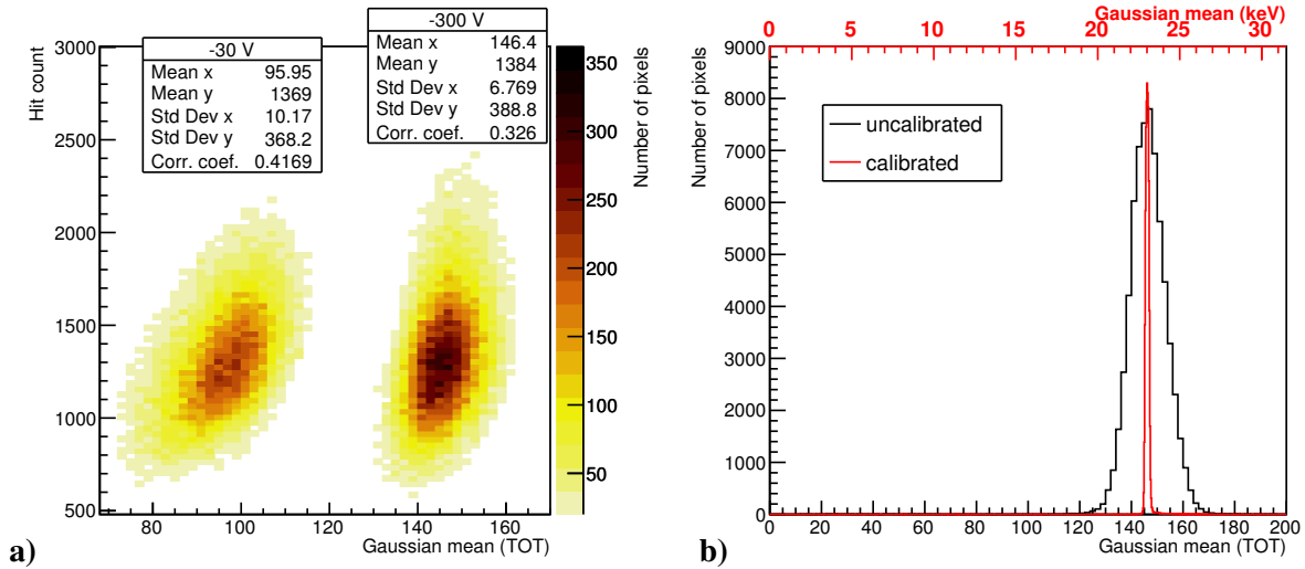
Fig. 4.4.7. a) Correlation between the photon count map and the Gaussian mean map for the 23 keV irradiation at -30 V (left) and -300 V (right). Each bin corresponds to the number of pixels with a specific Gaussian mean and photon count. b) Comparison of Gaussian mean distributions with calibrated and uncalibrated data for the 23 keV irradiation at -300 V.
