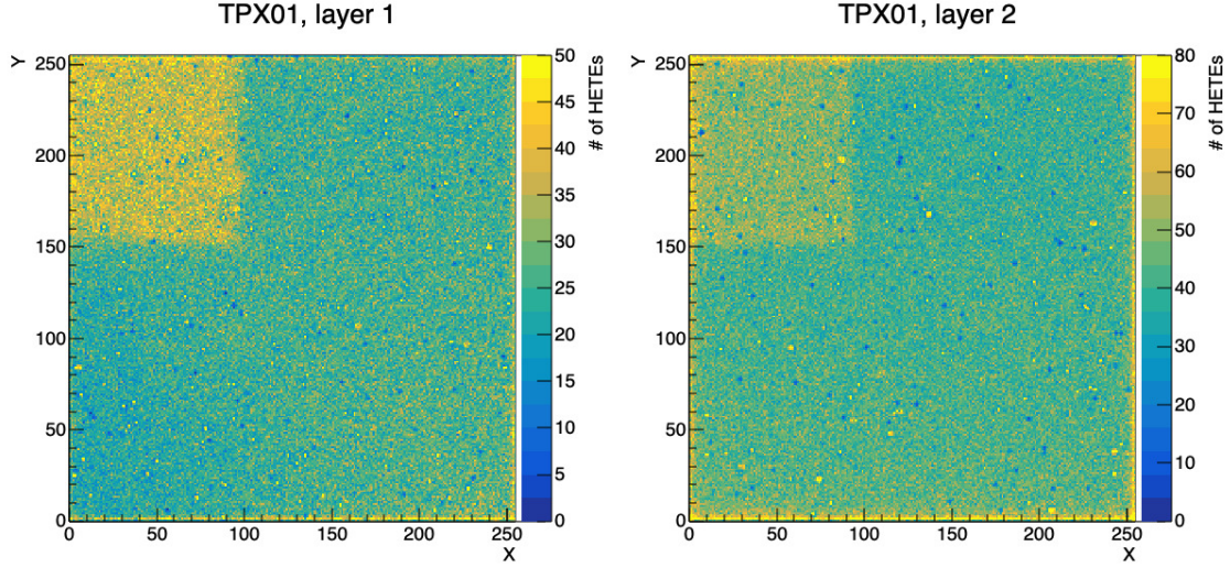
Fig. 3.3.9. Number of HETEs registered per pixel with TPX01 during several LHC runs in May 2016 (accumulated luminosity: 530 \text{ pb}^{-1} ). HETE locations are determined from the cluster centroid. The neutron converters placed in-between the two sensor layers are indicated, correspondingly to Fig. 3.3.1. The thermal neutron signal below the LiF+Al converter does not fully cover the delimited area due to the gaps between the different converters. For each pixel, the number of recorded events is incremented when the centroid of a HETE cluster is detected.
