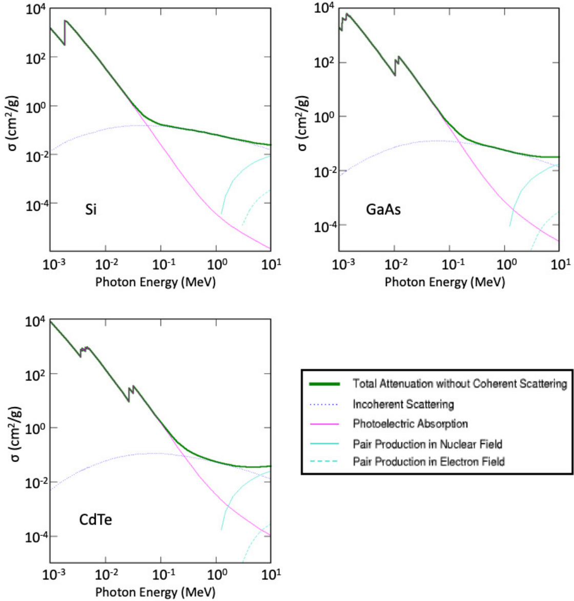
Fig. 2.3.4. Cross section of photon interactions in TPX sensor materials as a function of energy [74].
