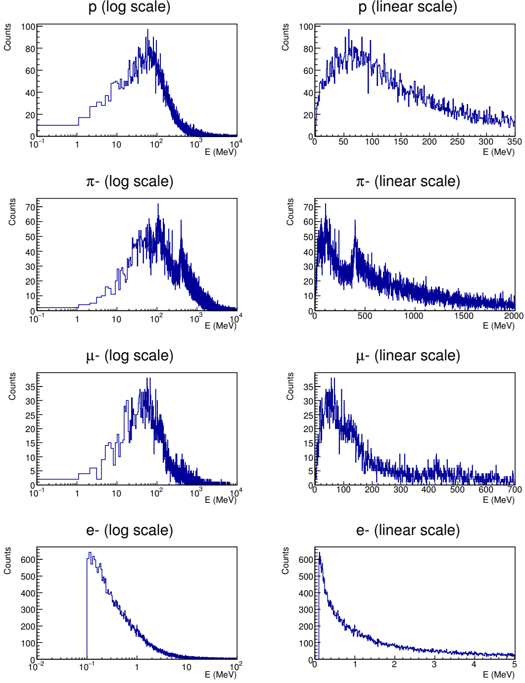
Fig. 3.2.2. Spectra of charged particles hitting the location of TPX01 in ATLAS (see table 3.3.1), as obtained from simulations [97]. On the left spectra, the x-axis is in logarithmic scale. Note the different x-axis range between heavy charged particles (protons, muons, pions), where 1 bin = 1 MeV, and electrons, where 1 bin = 10 keV.
