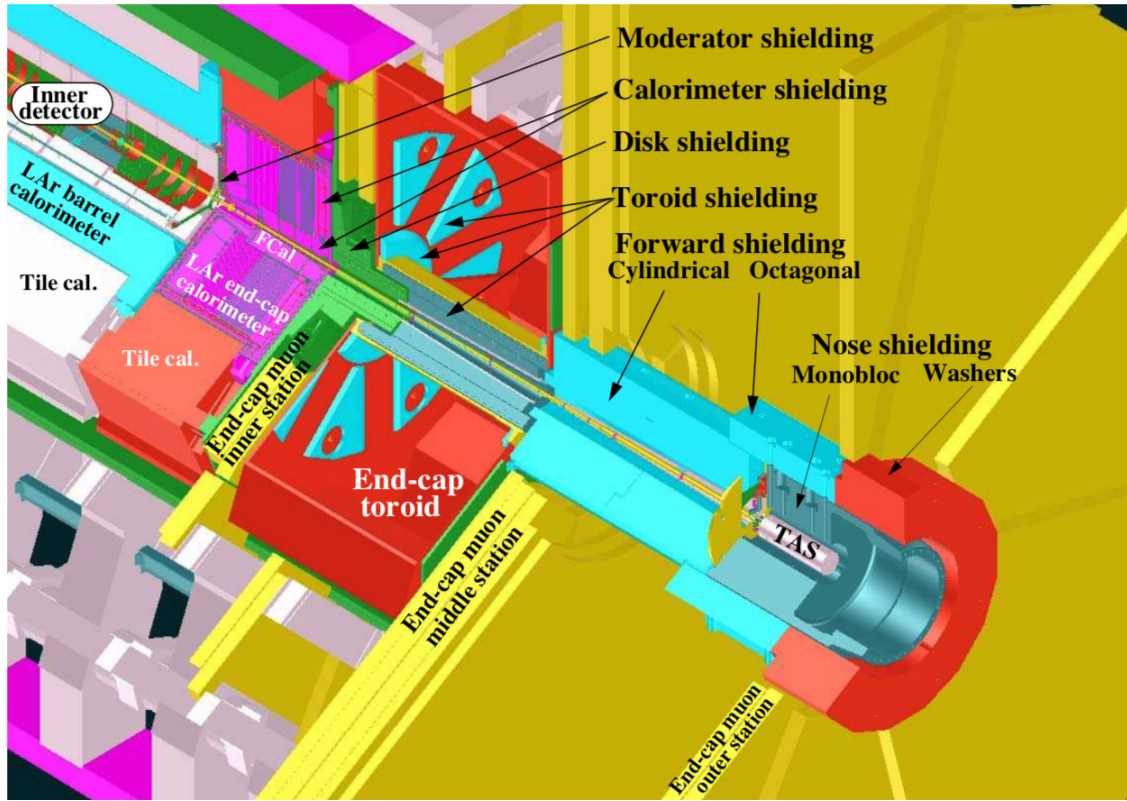
Fig. 1.3.3. The radiation shielding in ATLAS [11]. Shielding components are indicated with arrows. See text for more details.
