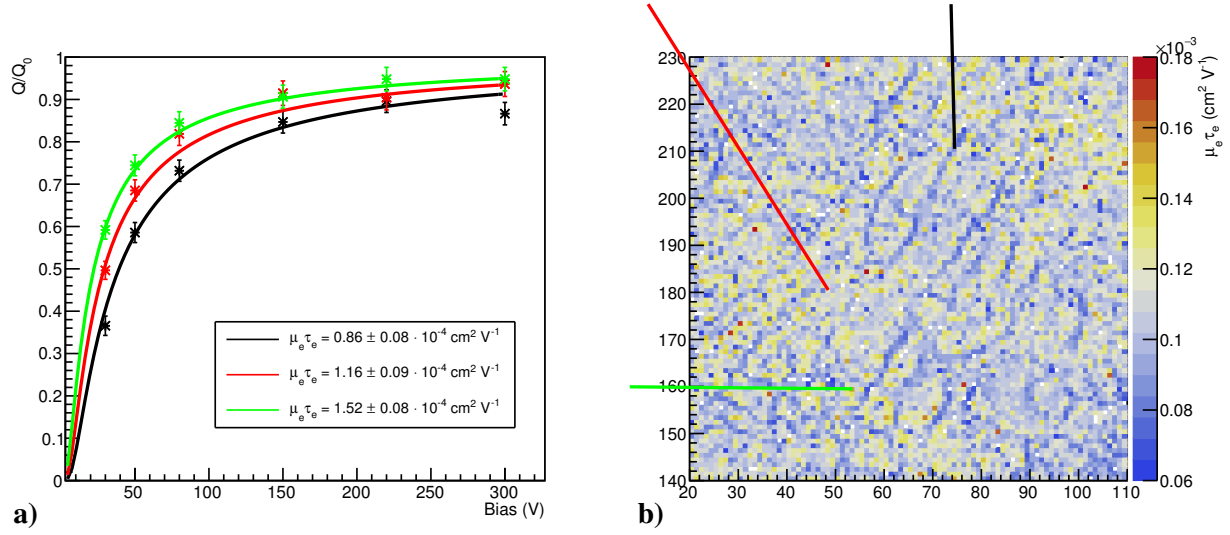
Fig. 4.4.9. a) Hecht graphs and fit functions for the same pixels as figure 4.4.5. For each point, the error bar was calculated from the statistical errors on the TOT Gaussian mean and calibration coefficients. b) Zoom on the dashed area of figure 4.4.8 (same area as figure 4.4.5). The arrow colors refer to the graphs on the left.
