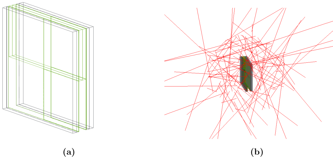
Fig. 3.3.6. Simulation of an ATLAS-TPX detector irradiated with an isotropic source of 500 MeV pions. (a) The geometry includes the two Timepix chips with their sensors and the neutron converters. (b) The particles are shot with random directions, from a sphere surrounding the detector.
