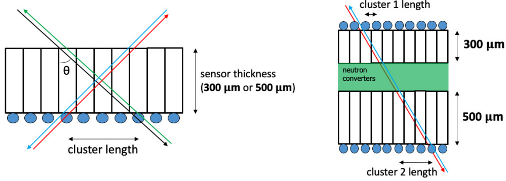
Fig. 3.3.4. Possibilities for wrong direction identification of incident angle according to the number of sensor layers (diagrams not in scale). With one layer (left), the same cluster can represent 4 particle directions. With two layers (right), the same combination of 2 clusters can represent 2 particle directions only.
