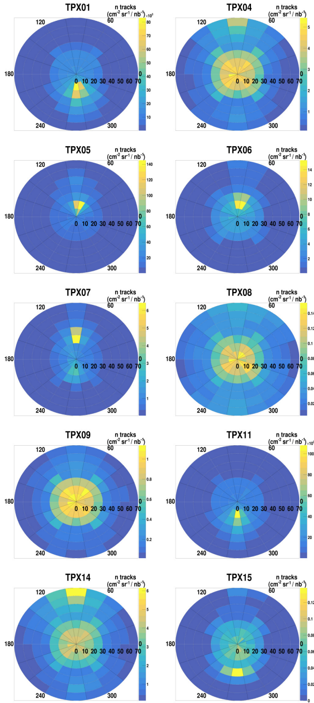
Fig. 3.3.13. MIP directions measured by the ATLAS-TPX detectors (see detector positions in Table 3.3.1). The radial axis ( \theta ) represents the incident angle with respect to the sensor surface ( \theta = 0^\circ means the particle is perpendicular to the surface). Data were measured during LHC Fill 4965 on May 31, 2016 (accumulated luminosity: 160 \text{ pb}^{-1} ).
