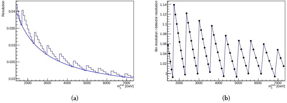
Figure 8.20: The bin resolution (black) is approximately larger than or equal to the fit representing the detector resolution (blue). Here (a) shows a comparison as a function of the m_{jj}^{\text{truth}} and (b) shows the ratio.
