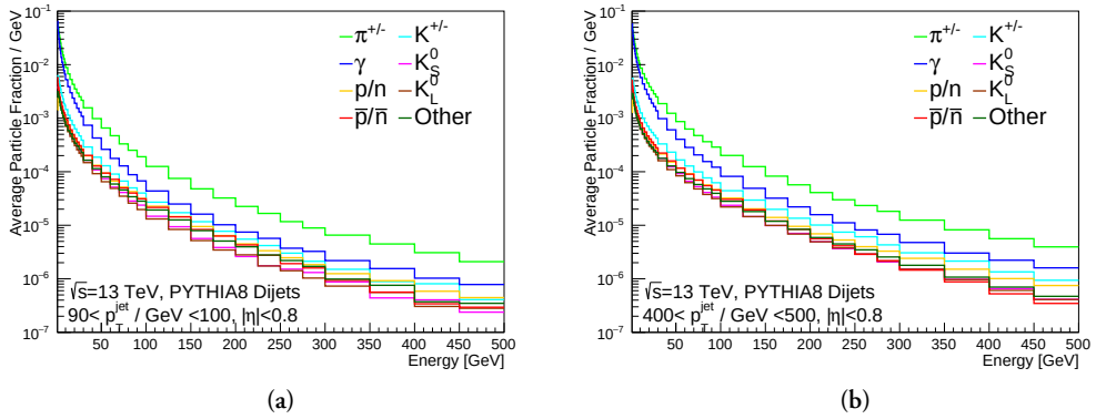
Figure 7.1: Average particle fraction as a function of the particle energy for different types of particles for jets with (a) 90 < p_T^{\text{jet}} / \text{GeV} < 100 and (b) 400 < p_T^{\text{jet}} / \text{GeV} < 500 .
