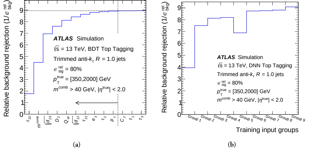
Figure 5.17: Background rejection of (a) the BDT and (b) the DNN as a function of the included variables [91].
