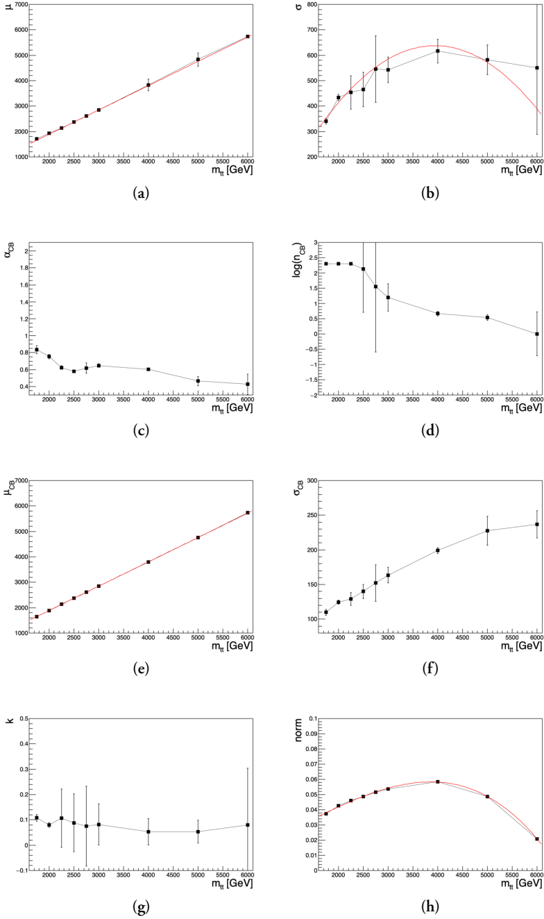
Figure 8.25: Linear interpolation and polynomial fits to the parameters of the Crystal Ball plus Gaussian function for the 1b signal region.
