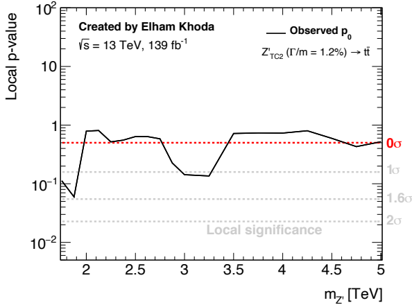
Figure 8.39: The observed p_0 -value as a function of the Z'_{\text{TC2}} mass (created by Elham Khoda).
