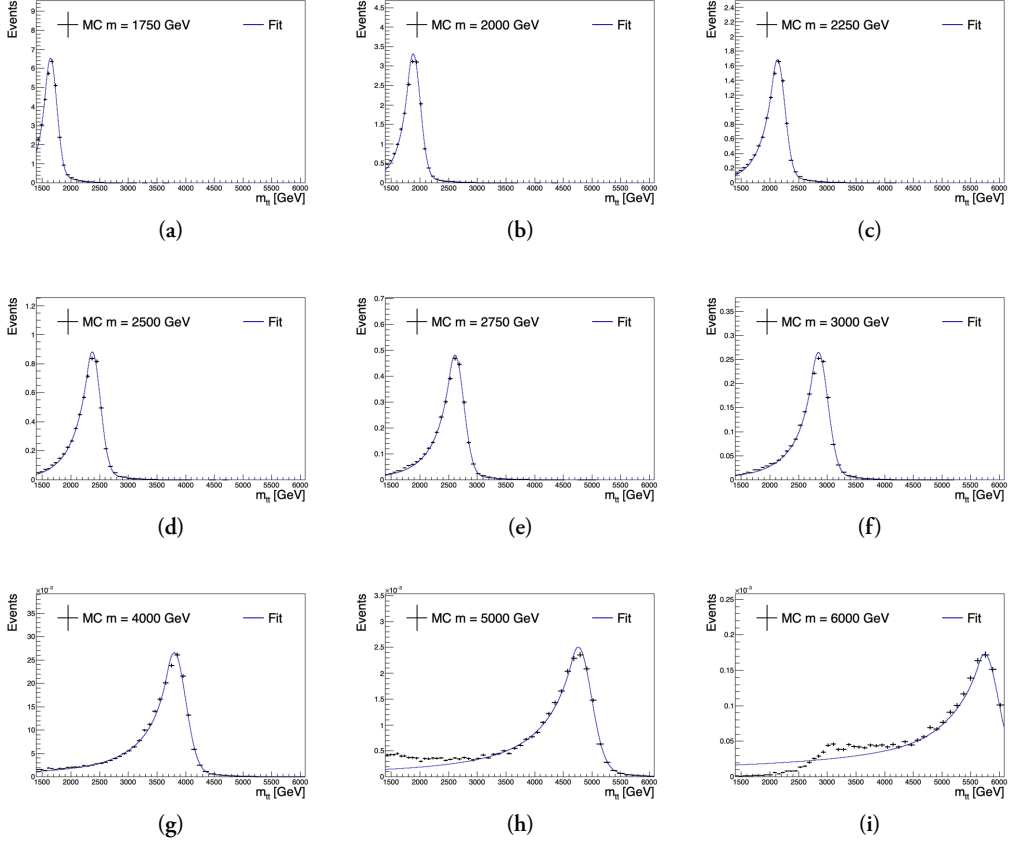
Figure 8.23: Crystal Ball plus Gaussian function fit to the mass distribution of Z'_{C2} samples in the 1b signal region. The low mass tail is not well described for the 5 and 6 TeV signal, but this does not have a large effect on the limit due to the steeply falling background (see discussion in text).
