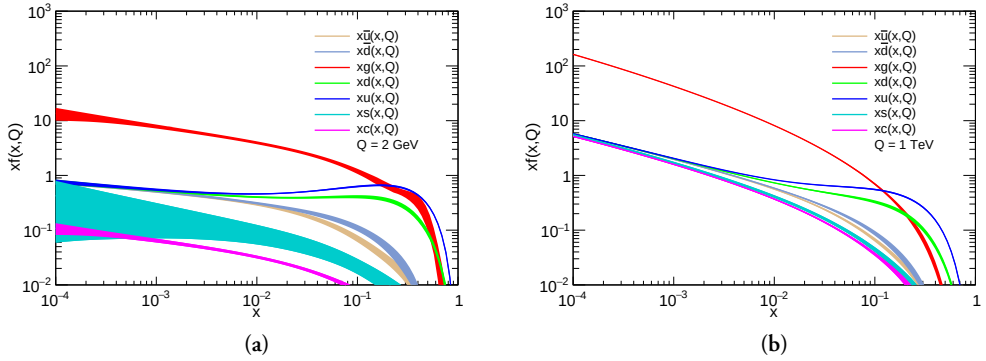
Figure 2.6: Parton distribution function for the proton with (a) Q = 2 GeV and (b) Q = 1 TeV. The width of the functions shows the 1\sigma band. The figures are generated with APFEL 2.7.1 Web [21, 22] using the NNPDF2.3 LO PDF set [23].
