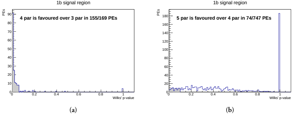
Figure 8.21: Wilks' p-value for the pseudo-experiments comparing good fits with (a) 3 and 4 parameters and (b) 4 and 5 parameters in the 1b signal region. The gray histogram indicates the pseudo-experiments, where the higher number of parameters are favored.
