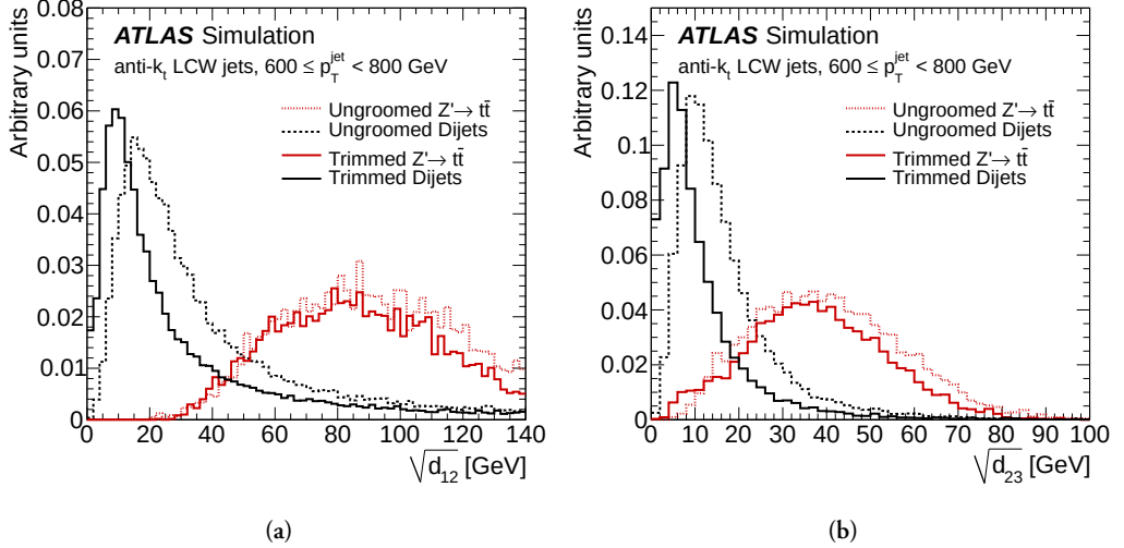
Figure 5.16: Discriminating power of (a) \sqrt{d_{12}} and (b) \sqrt{d_{23}} for Z' \rightarrow t\bar{t} versus dijet events measured at \sqrt{s} = 7 \text{ TeV} [100].
