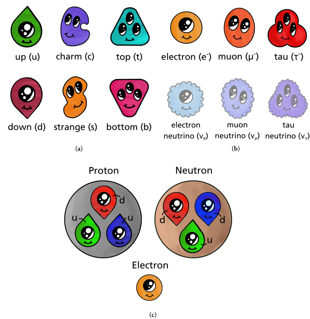
Figure A.1: The fundamental fermions are (a) quarks and (b) leptons and (c) a few of them (up quark, down quark and electron) make up all the ordinary matter around us.
