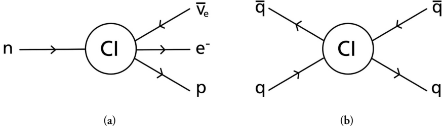
Figure 2.11: Feynman diagrams illustrating (a) the beta decay and (b) an unresolved interaction leading to q\bar{q} production.
