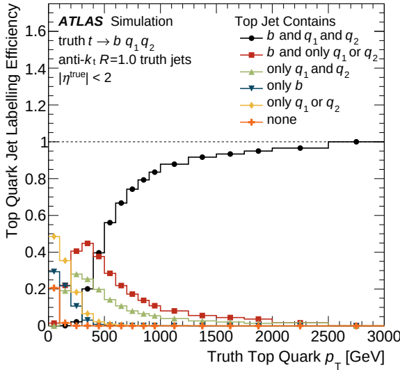
Figure 5.11: Top quark jet labeling efficiency as a function of the truth top quark p_T [91].
