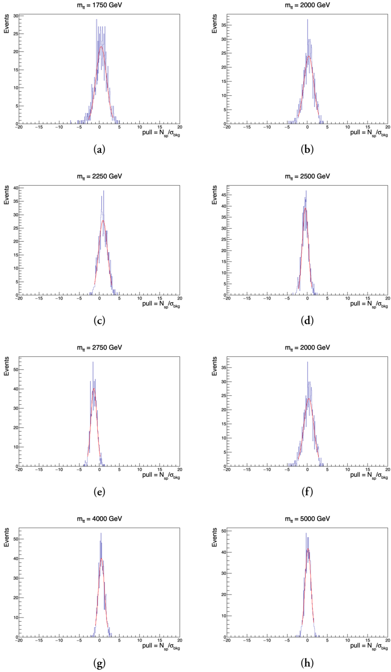
Figure 8.35: Gaussian fits to spurious signal pull in 1\sigma signal region for 4-parameter fit for the different signal masses.
