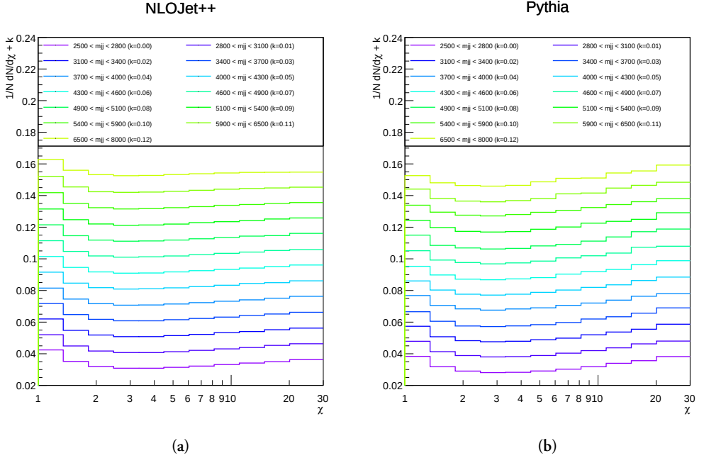
Figure 9.12: The inputs for NLO k -factor calculations are (a) NLO calculations from NLOJet++ with "error function" bins and (b) LO calculations including parton showering from Pythia. A constant k is added to the distributions in the figure in order to better see the features.
