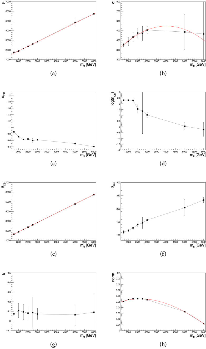
Figure 8.27: Linear interpolation and polynomial fits to the parameters of the Crystal Ball plus Gaussian function for the 2b signal region with the 4 TeV sample removed for the closure test.
