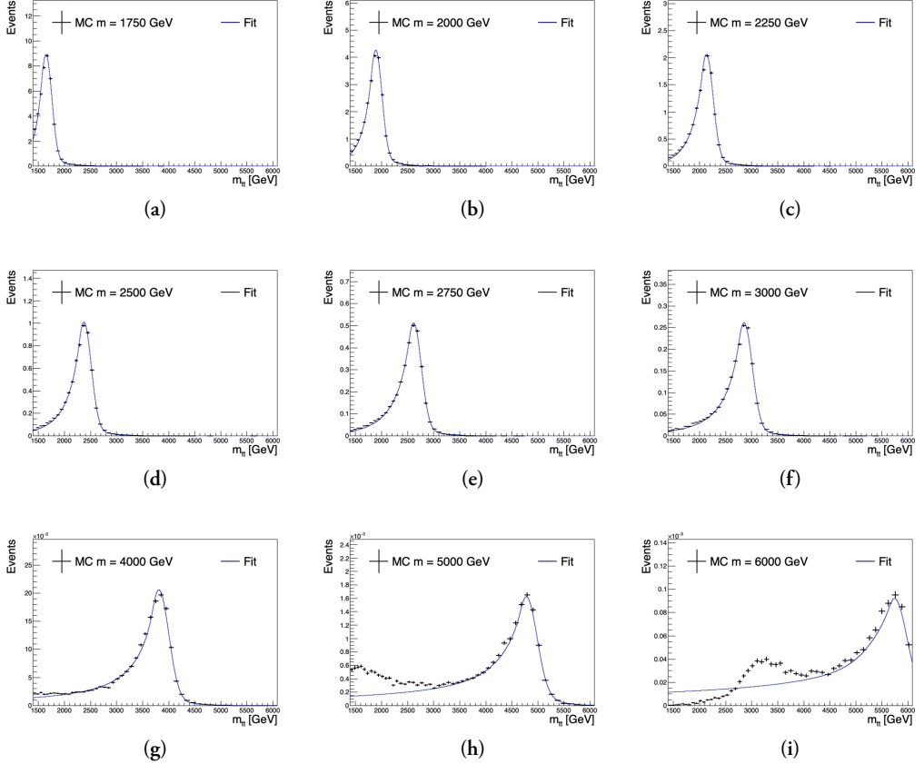
Figure 8.24: Crystal Ball plus Gaussian function fit to the mass distribution of Z'_{TC2} samples in the 2b signal region. The low mass tail is not well described for the 5 and 6 TeV signal, but this does not have a large effect on the limit due to the steeply falling background (see discussion in text).
