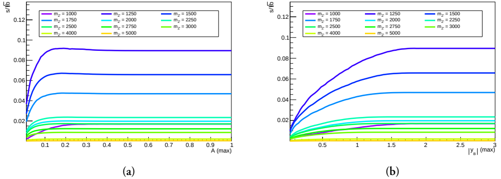
Figure 8.8: Significance as a function of the maximum cut value of (a) the p_T balance, A , and (b) the rapidity boost, y_B .
