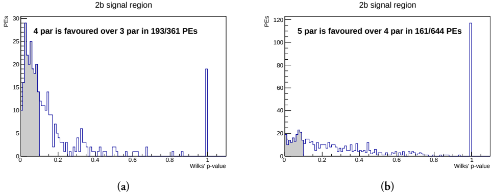
Figure 8.22: Wilks' p-value for the pseudo-experiments comparing good fits with (a) 3 and 4 parameters and (b) 4 and 5 parameters in the 2b signal region. The gray histogram indicates the pseudo-experiments, where the higher number of parameters are favored.
