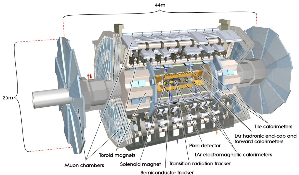
Figure 4.1: Sketch of the ATLAS detector [54].
