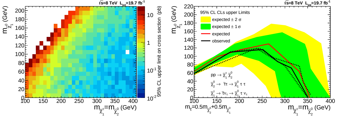
Figure 9.4.: 95% CL exclusion limits in the m_{\tilde{\chi}_1^\pm}(=m_{\tilde{\chi}_2^0}) m_{\tilde{\chi}_1^0} plane for the tau dominated scenario. This plot corresponds to the moderate stau mass scenario. On the left-hand side, the observed 95% CL exclusion limit on the cross section is shown. The right-hand side shows the 95% CL excluded phase space by assuming wino-like \tilde{\chi}_1^\pm \tilde{\chi}_2^0 production and a branching ratio of 1.
