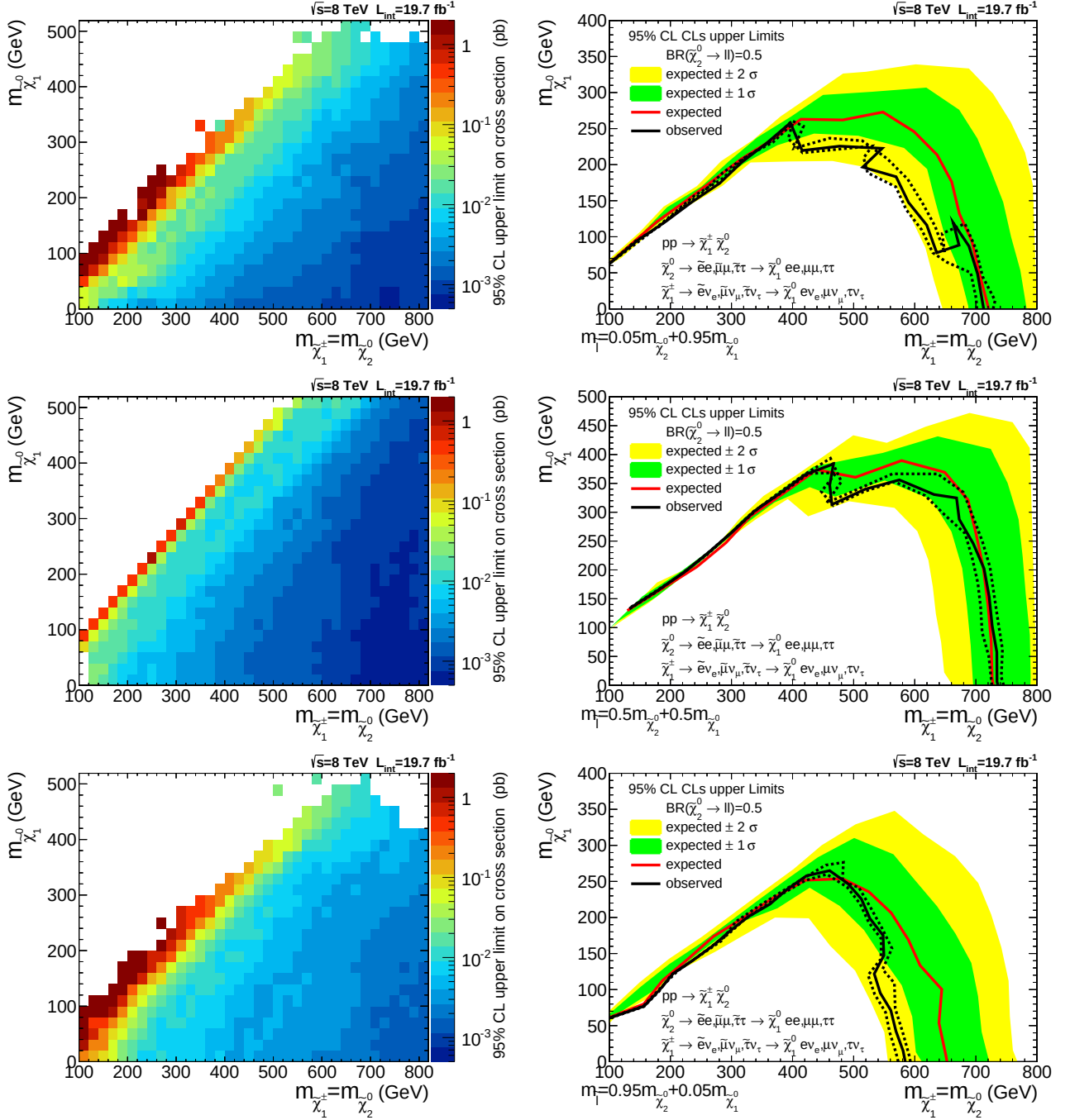
Figure 9.2.: 95% CL exclusion limits in the m_{\tilde{\chi}_1^\pm}(=m_{\tilde{\chi}_2^0}) - m_{\tilde{\chi}_1^0} plane for three different flavor democratic scenarios are presented. The light/moderate/heavy slepton scenario is shown in the top/middle/bottom. On the left-hand side the observed 95% CL exclusion limit on cross section is shown. The right-hand side shows the 95% CL excluded parameter space by assuming wino like \tilde{\chi}_1^\pm \tilde{\chi}_2^0 production and a branching ratio of 0.5.
