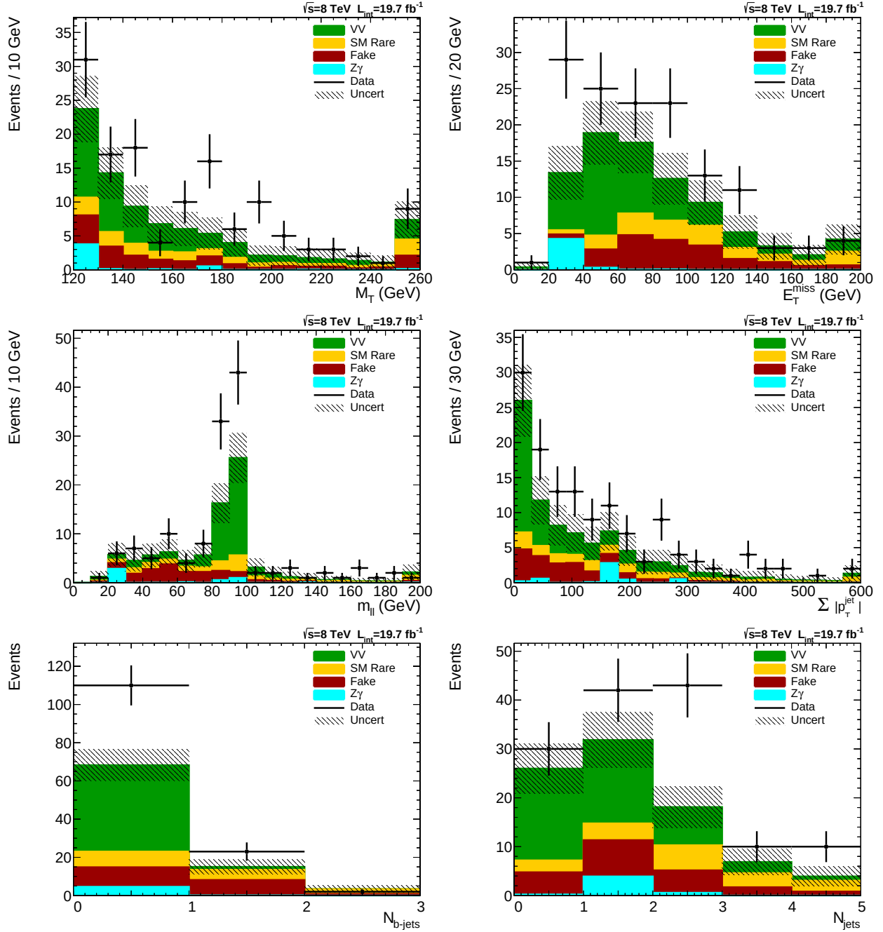
Figure 8.8.: 3ℓ events with M_T > 120 GeV are for data and background prediction are plotted. On the top left the M_T distribution and on the top right the E_T^{miss} distribution are shown. The middle row presents the m_{\ell+\ell-} for the lepton pairs best matching a Z boson on the left and the right the scalar sum of all jets. On the bottom left (right) the number b-jets (jets) are shown.
