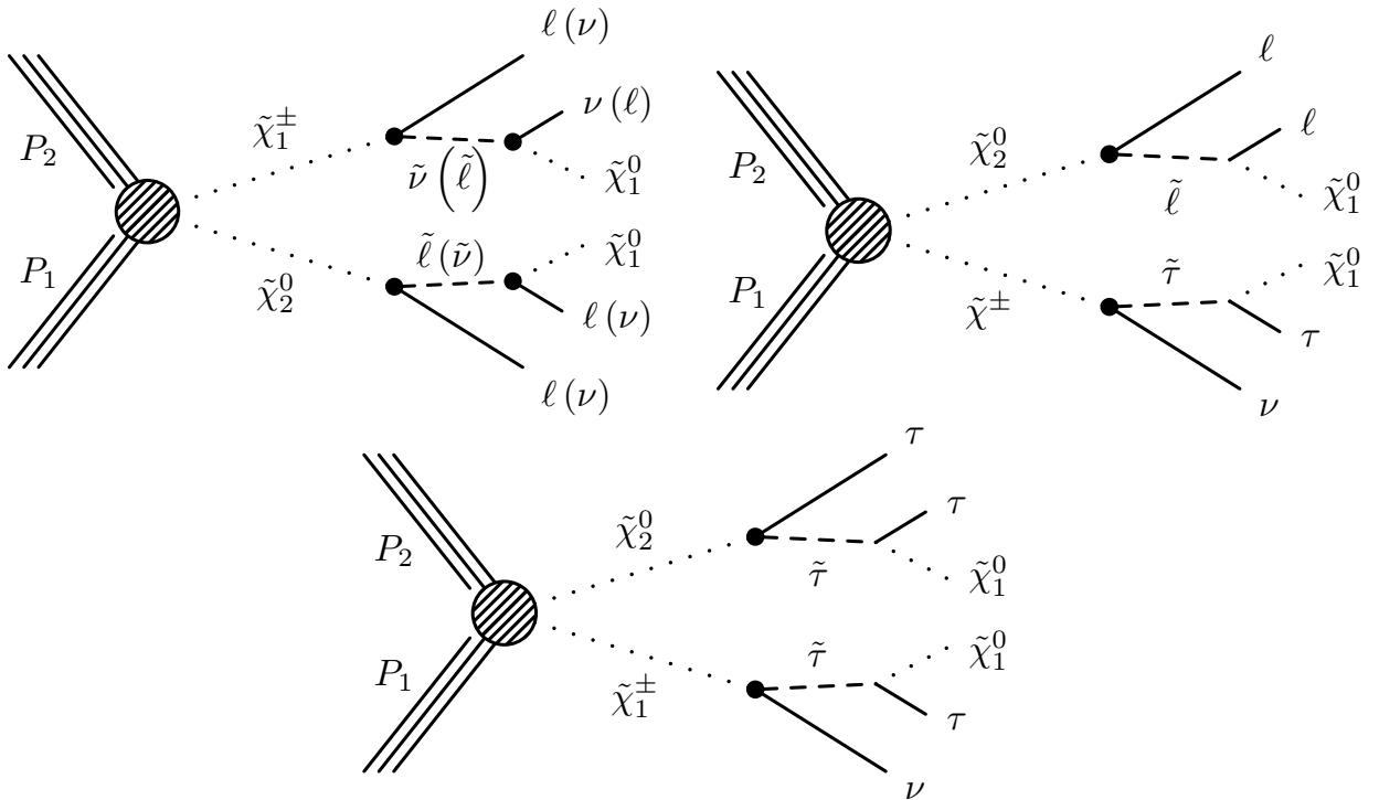
Figure 6.1.: Feynman diagrams for Chargino Neutralino production with slepton mediated decays. On the top left, the flavor democratic scenario is illustrated. On the top right the tau enriched and on the bottom the tau dominated scenario. Explanations can be found in the text.
