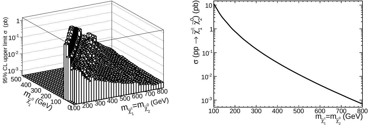
Figure 9.1.: The 95% CL upper limit on the cross section for a simplified model is shown on the left. The cross section for the process pp \rightarrow \tilde{\chi}_1^\pm \tilde{\chi}_2^0 at a center of mass energy of \sqrt{s}=8 TeV is presented on the right.
