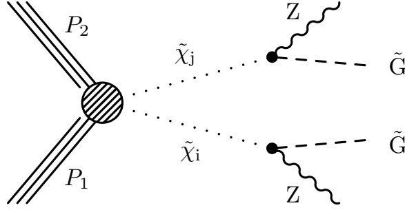
Figure 6.3.: Feynman diagrams for the GMSB model. Details can be found in the text.
