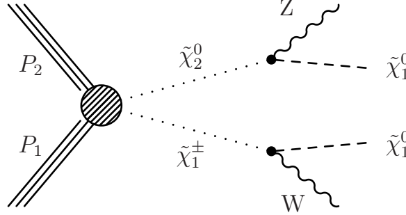
Figure 6.2.: Feynman diagrams for Chargino Neutralino production with decay into a W boson and a Z boson.
