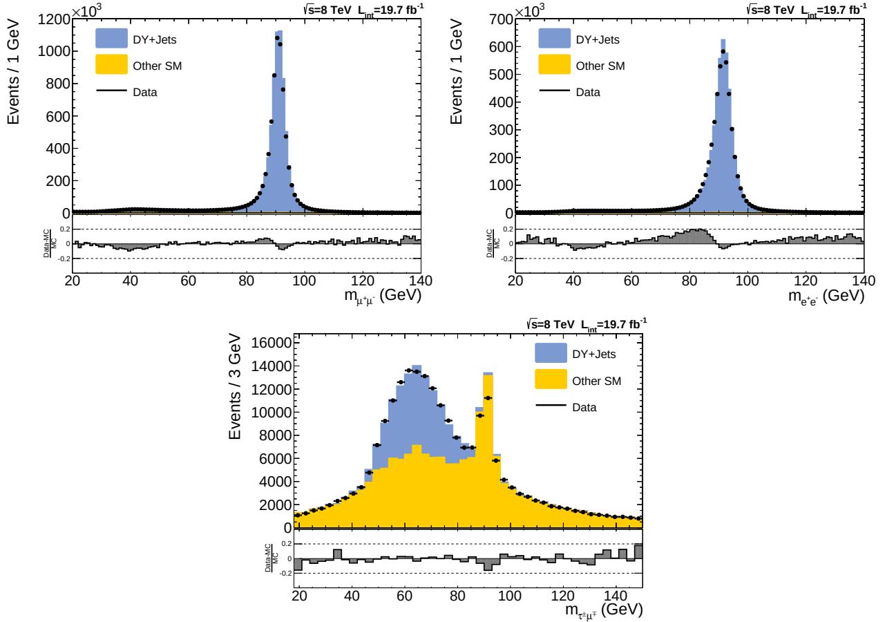
Figure 7.1.: Invariant mass distribution for events with two opposite sign leptons. On the top left (right) the invariant mass distribution for tow opposite sign muons (electrons) are shown. On the bottom, the invariant mass distribution of a tau and a muon is shown.
