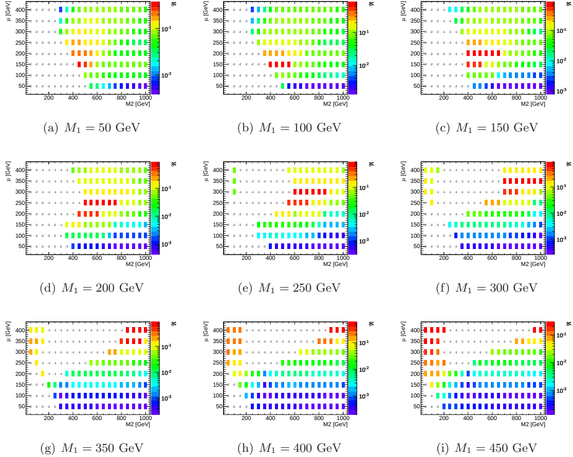
Figure 6.5: The ratio \mathcal{R} as a function of M_2 and \mu for different values of M_1 . Small parts of the parameter space of the pMSSM show values of \mathcal{R} \gtrsim 0.5 , such that a search with four leptons in the final state might be more sensitive to new physics than a search with three leptons in the final states in these regions.
