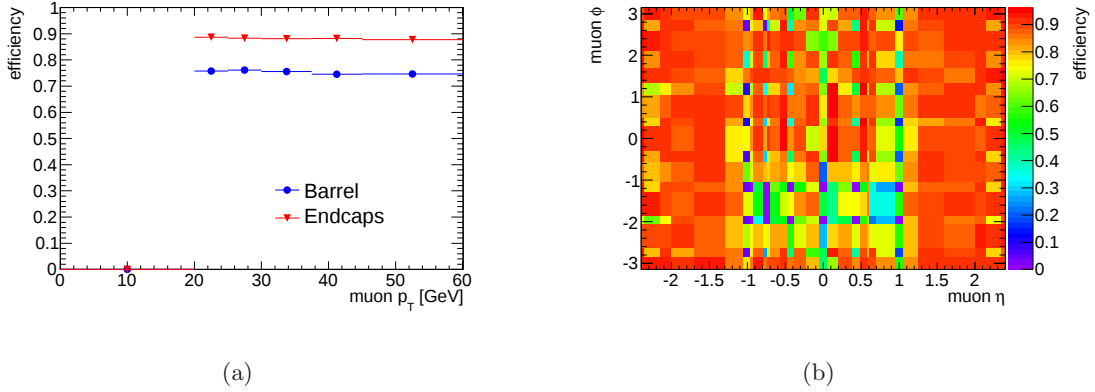
Figure 5.13: The absolute efficiency with respect to reconstruction of the trigger item EF_mu18. The efficiency is shown as a function of the muon transverse momentum for all muons passing the offline selection cuts in (a), where the barrel region is defined by |\eta| < 1.05 and the endcap regions are defined by 1.05 < |\eta| < 2.4 . In (b) the efficiency is shown as a function of the muon \eta and \phi for all muons passing the offline selection cuts and p_T > 20 GeV. The efficiency has been measured using data taken in 2011 from data taking periods A to I. In the barrel region, for \phi \sim -1 and \phi \sim -2 the efficiency drops to very low values, which is mainly due to a lack in coverage due to the support structure for the detector that is located in that region. Overall, the efficiency is a highly inhomogeneous function in the barrel region.
