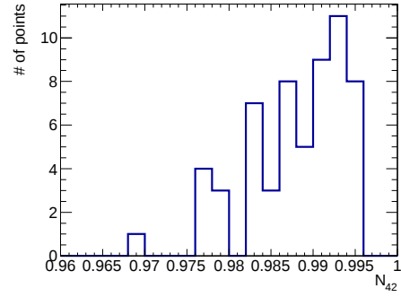
(b) Wino component of \tilde{\chi}_4^0
