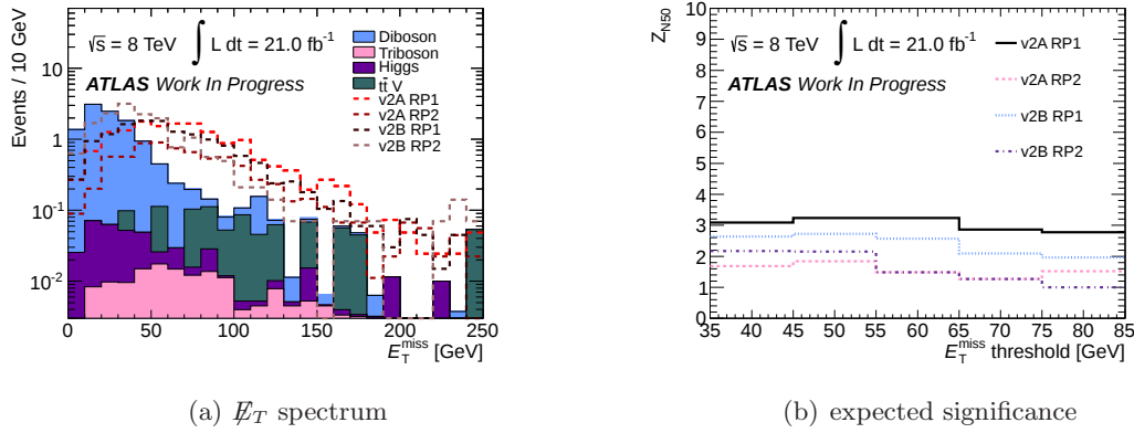
Figure 6.12: Distribution of a variable with a possible relevance to the expected significance. Figure (a) shows the distribution of the missing transverse energy after requiring at least four reconstructed signal leptons and no reconstructed Z candidate in the event. Figure (b) shows the expected significance as a function of E_T threshold, where an uncertainty of 50% on the background expectation is taken into account.
