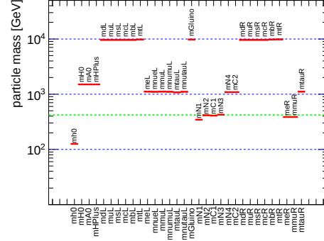
(b) M_1 = 350 GeV, M_2 = 1000 GeV, \mu = 400 GeV
