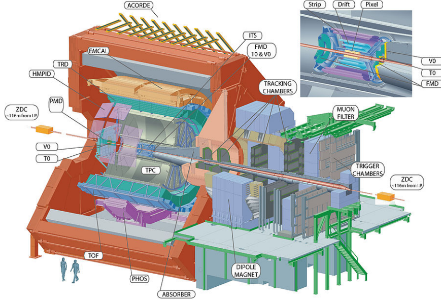
Figure 4.2: ALICE detector layout.
