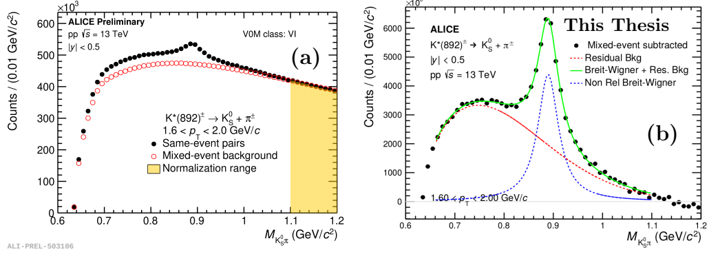
Figure 7.1: The K_S^0 \pi^\pm invariant mass distribution for the 1.6 < p_T < 2.0 GeV/c bin in the VI V0M class (black full circles), before (a) and after (b) the uncorrelated background subtraction. Left panel: the red open circles describe the background shape evaluated via the event-mixing technique, while the yellow-filled area is the normalization region. Right panel: the solid green curve is the result of the final fit, the dashed red line represents the residual background, while the dashed blue line is the non-relativistic Breit-Wigner function.
