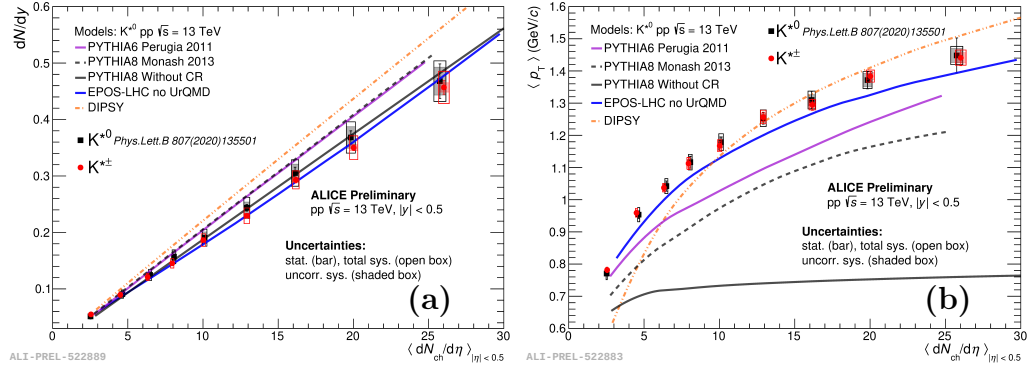
Figure 10.7: Integrated yields dN/dy (a) and mean transverse momenta \langle p_T \rangle (b) for K^{*\pm} and K^{*0} as a function of \langle dN_{ch}/d\eta \rangle_{|\eta| < 0.5} . The \langle dN_{ch}/d\eta \rangle_{|\eta| < 0.5} values used for the K^{*0} analysis are referred to the LHC15 period [38]. Bars represent statistical uncertainties, open boxes represent total systematic uncertainties, and shaded boxes are the systematic uncertainties uncorrelated with multiplicity. The measurements are also compared to several model predictions [26–28, 32, 80].
