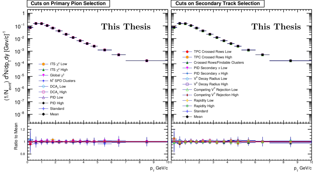
Figure 9.3: The V_{mean,j} p_T spectra of the cuts used for systematic uncertainty estimation in the primary pion identification ( left panel ) and in the secondary tracks and K^0_S selection ( right panel ) in the III VOM class. The V_{MEAN} p_T distribution is also reported. Lower panels: V_{mean,j}/V_{MEAN} ratios as a function of p_T bins.
