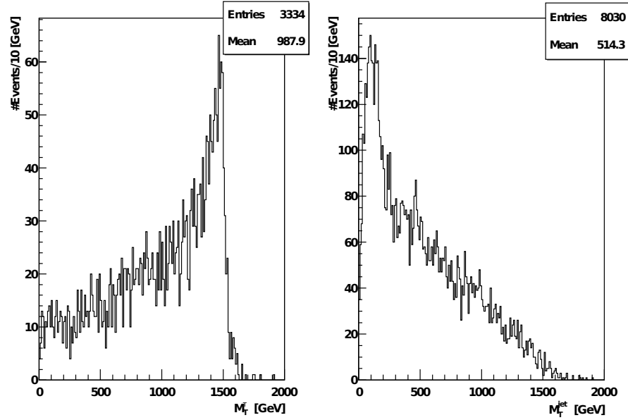
Figure A.3: M_T^\tau vs. M_T^{jets} : Transverse mass of the tau and neutrino from the W' decay and transverse mass calculated out of the hadronic jet coming from the tau decay and the two neutrinos in the event as missing transverse energy.
