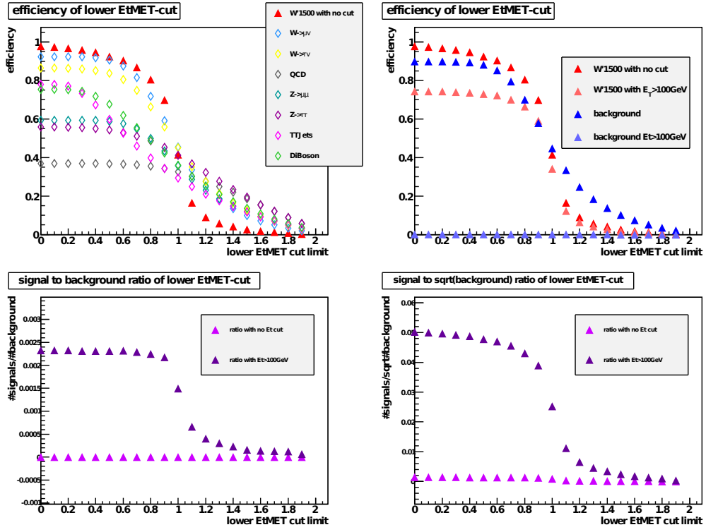
Figure A.7: Muon lower E_T/\ell_T cut
