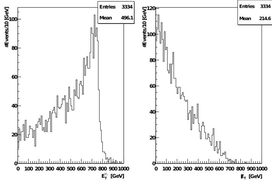
Figure A.2: E_T^{\nu\tau} vs. E_T : Transverse energy of the neutrino coming from the W' decay and the missing transverse energy calculated out of the three neutrinos in a leptonic decaying tau.
