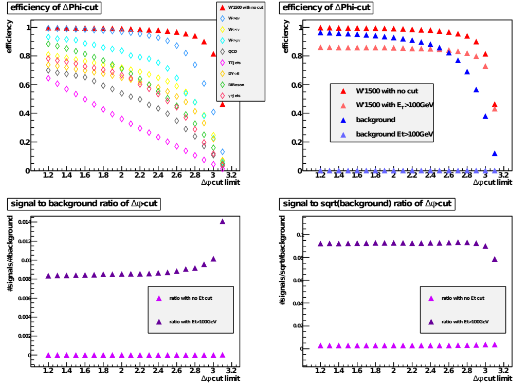
Figure A.5: Electron \Delta\phi cut
