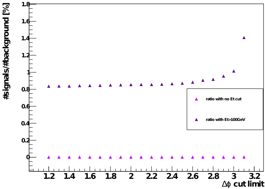
Figure 7.5: Electron \Delta\phi cut
