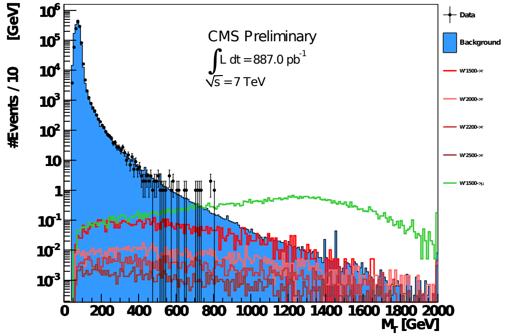
Figure 7.7: Resulting data muons: As in the electron distribution we can see the Standard Model W peak in the low M_T region and signal is evenly distributed with no characteristic peak an event display of the highest M_T event can be seen in the appendix (see section A.5). As a comparison the final M_T -distribution of a W' \rightarrow \mu\nu sample with a mass of 1500 GeV is shown, like for the electrons we see the jacobean peak and the over all bigger signal, because of the higher branching ratio, the difference to the electron channel can be explained by the lower p_T resolution for high p_T -muons.
