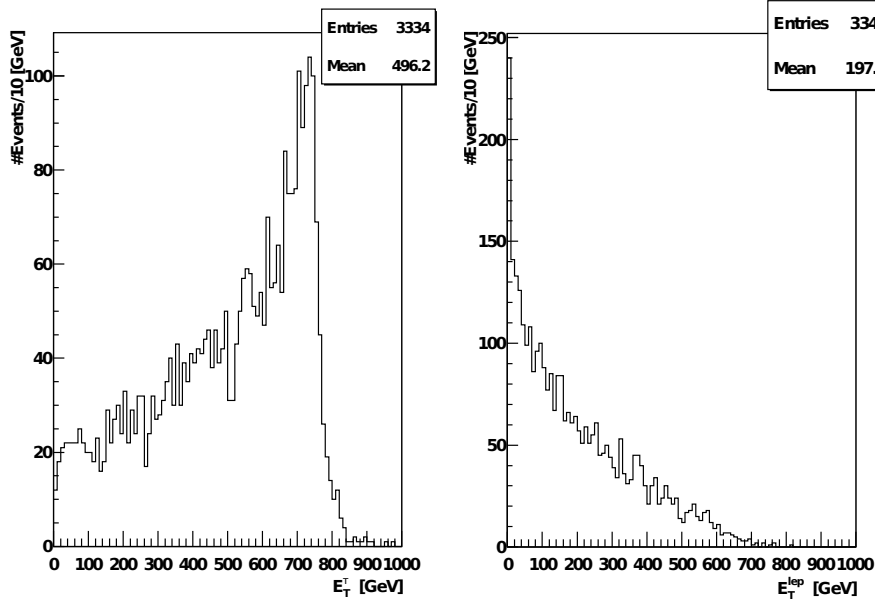
Figure 6.5: E_T^{\tau} vs. E_T^{\text{lep}} : As we can see that the energy of the tau is clearly defined, with a peak at 750 GeV, but the charged leptons that come from the decay of the tau do not have this clear shape anymore, this can be explained by the subsequent decay of the tau which results in a smearing of E_T due to more decay products.
