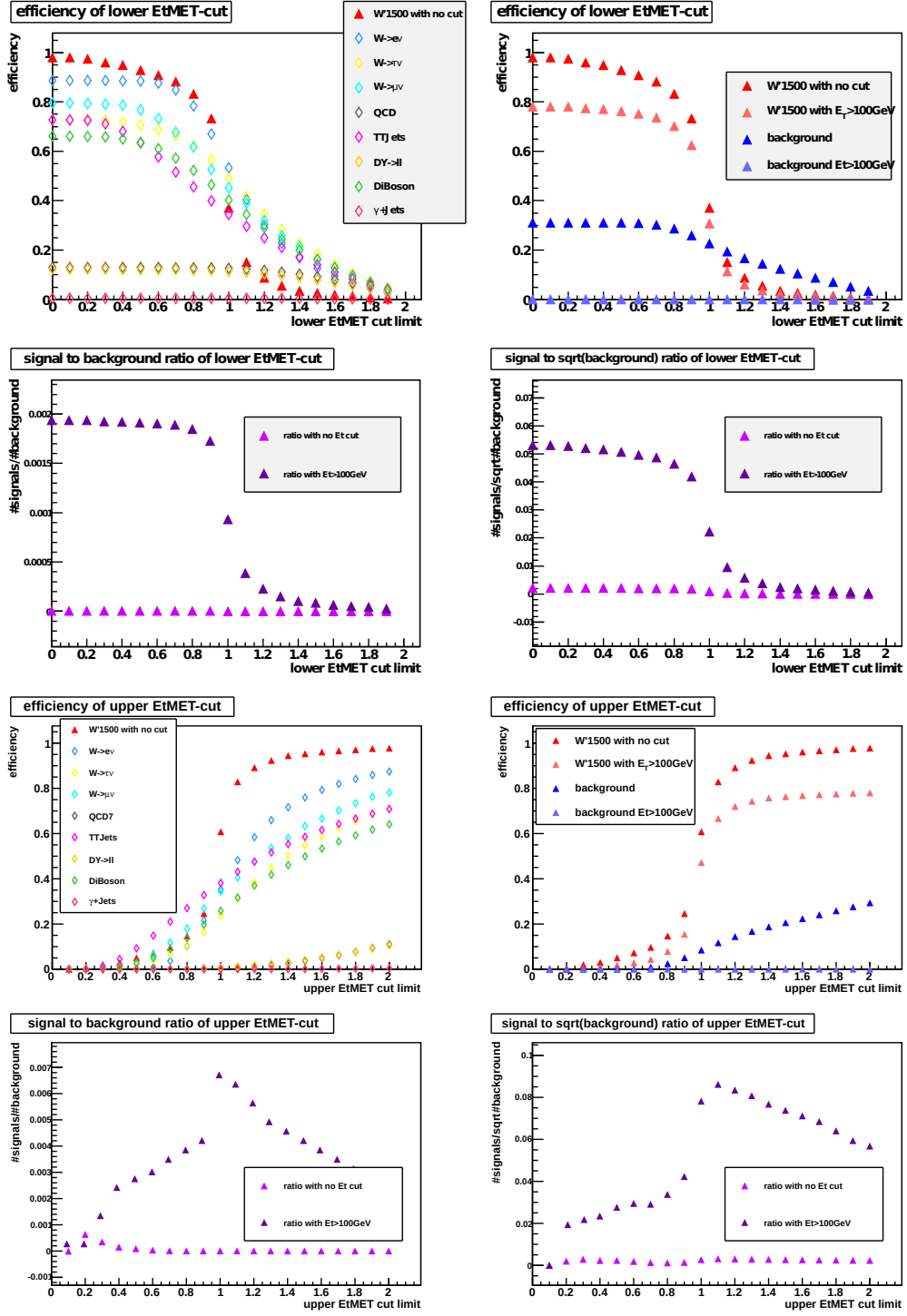
Figure A.4: Electron E_T/\cancel{E}_T cut
