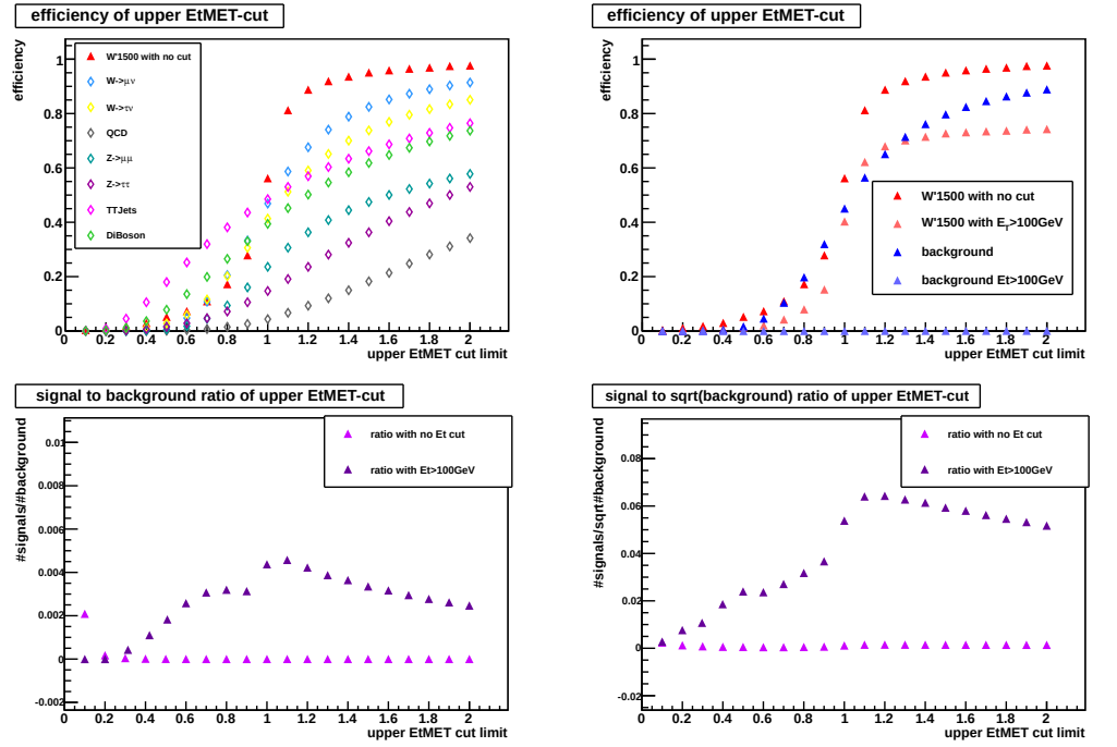
Figure A.6: Muon upper E_T/|E_T| cut
