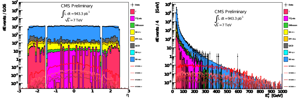
Figure A.13: Electrons: \eta and E_T distributions
