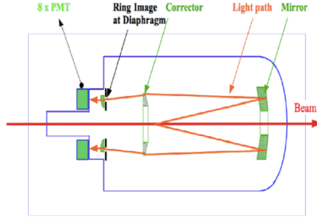
Figure 2.3: Schematic layout of a standard CERN SPS CEDAR.
