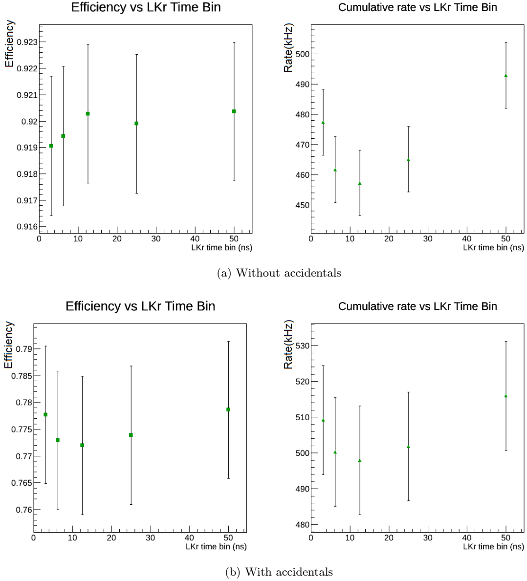
Figure 4.18: Efficiency and rate dependence on LKr cell hit separation time parameter.
