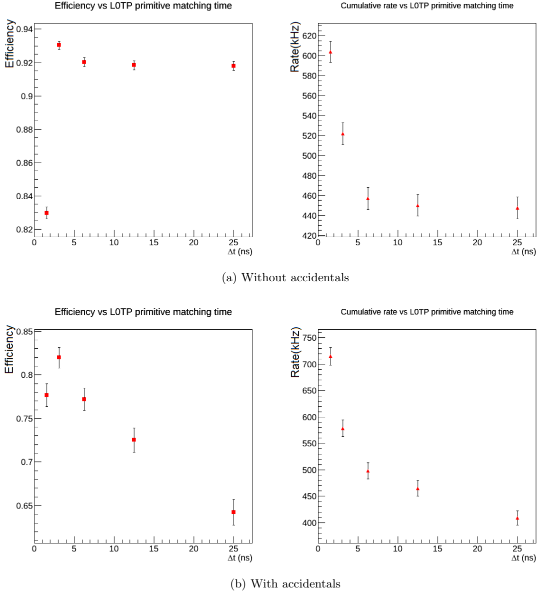
Figure 4.22: Efficiency and rate dependence on L0TP matching time parameter.
