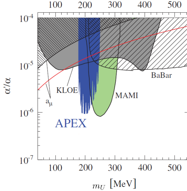
Figure 5.9: The 90% confidence upper limit on \alpha'/\alpha = \epsilon^2 versus the vector boson mass for the APEX experiment [111], compared with other 90% confidence level limits from the muon anomalous magnetic moment, KLOE, A1 at MAMI and BABAR.
