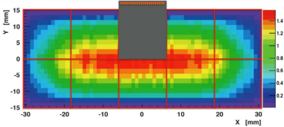
Figure 2.5: Beam intensity distribution over GTK3 (MHz/mm 2 ). In grey one of the 2 \times 5 readout chips.
