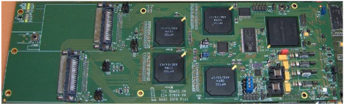
Figure 3.4: The TDCB daughter-board.
