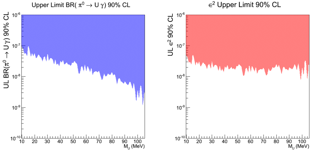
Figure 5.27: Expected NA62 upper limits at 90% confidence level for the Branching Ratio of \pi^0 \rightarrow \gamma U (left) and for \epsilon^2 as a function of the U boson mass, assuming no trigger downscaling.
