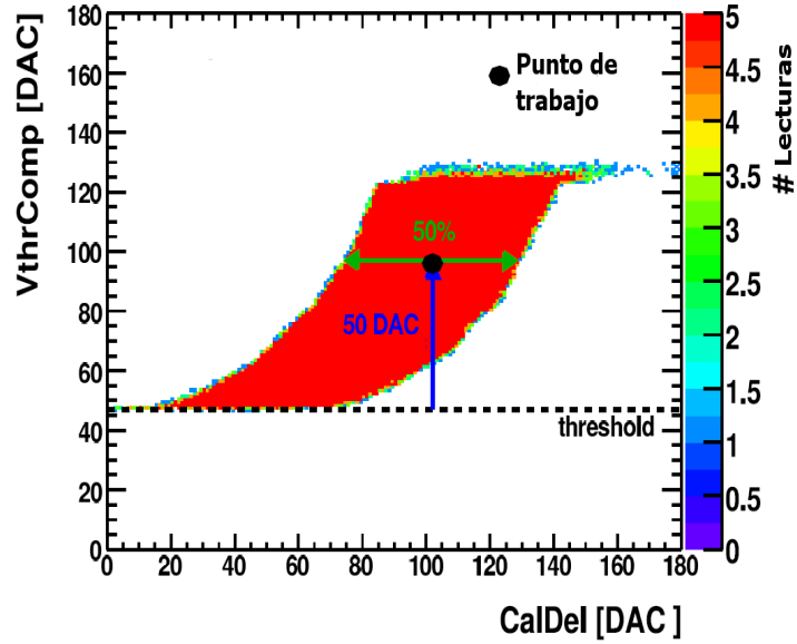
Figura 6-1: VThreshold (voltaje umbral) Vs CalDel.
